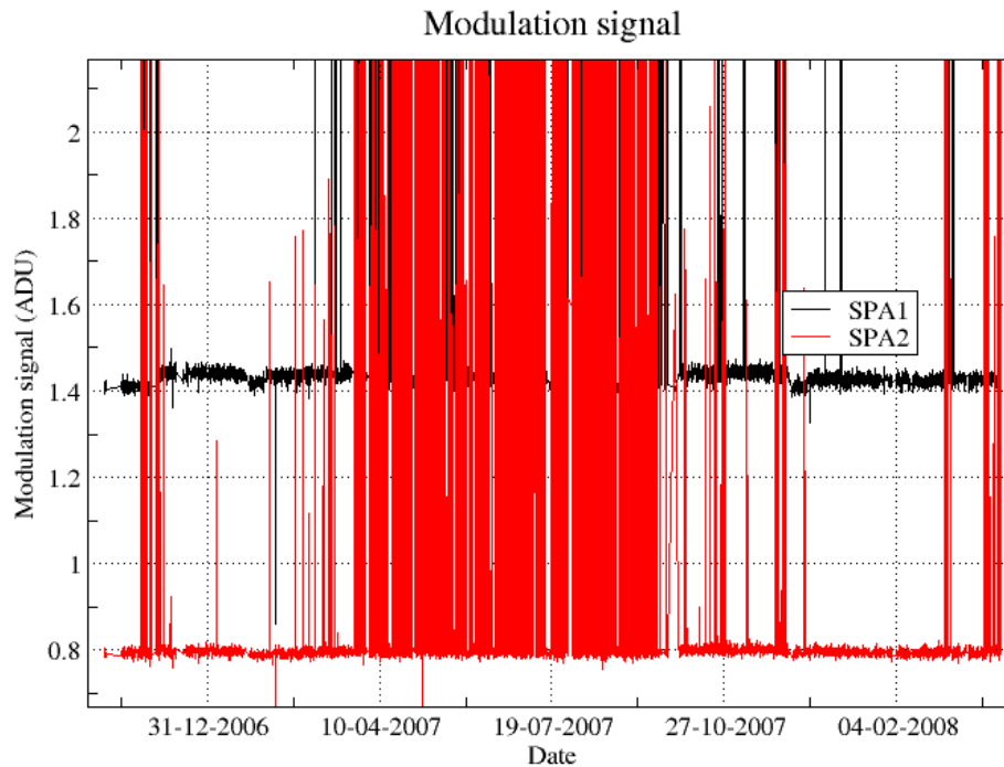
Figure 4.5-4: Modulation signal
