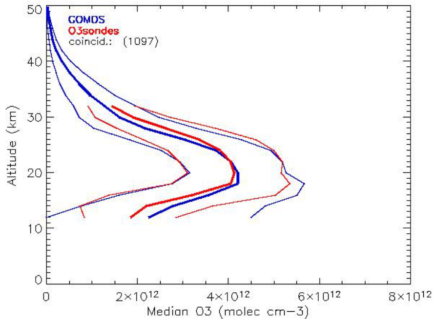
Figure 7.2-5: Same as Figure 7.2-1 for GOMOS (blue thick line) and for ozonesonde (red thick line) measurements in close coincidence (1097 profiles)
