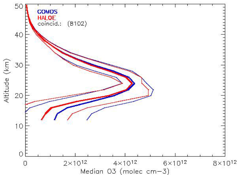
Figure 7.2-1: Vertical profiles of the median of O 3 local density from GOMOS (blue thick line) and from HALOE (red thick line) measurements in close coincidence (8102 profiles). The envelop of each median profile is computed as the half difference between 84 th percentile limit and 16 th percentile limit (thin lines)
