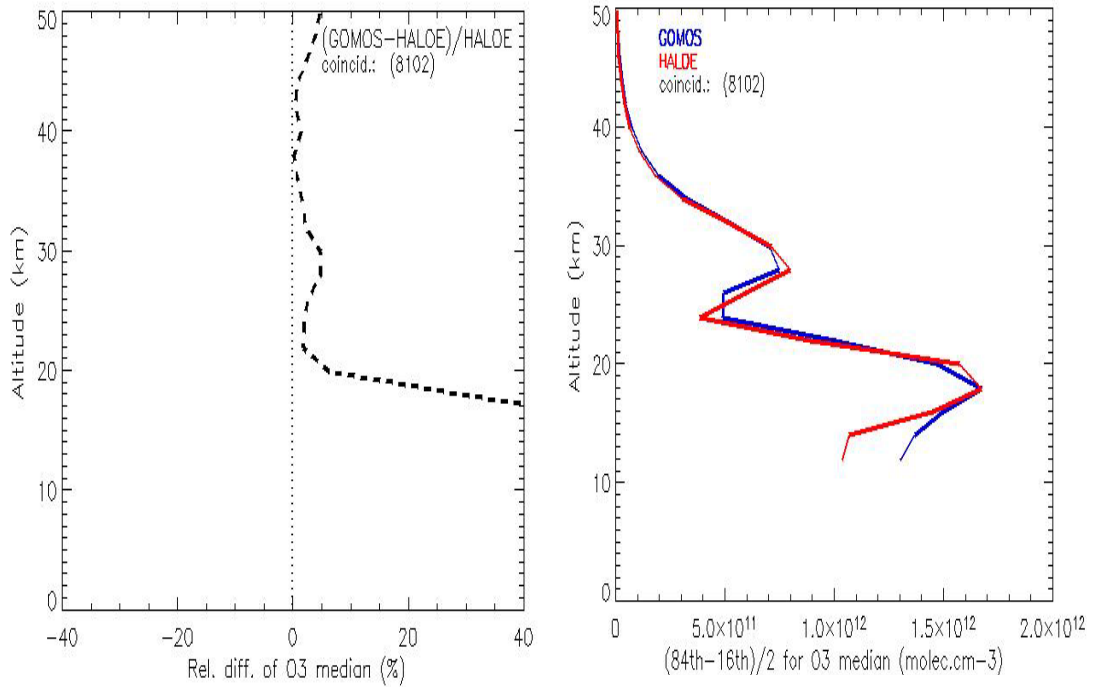
Figure 7.2-2: Relative difference in % of the median profiles plotted in Figure 7.2-1 (left figure). Half difference between 84 th percentile limit and 16 th percentile limit (right figure)
