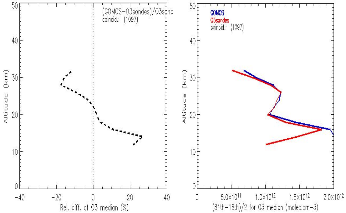
Figure 7.2-6: Relative difference in % of the median profiles plotted in Figure 7.2-5 (left figure). Half difference between 84 th percentile limit and 16 th percentile limit (right figure)
