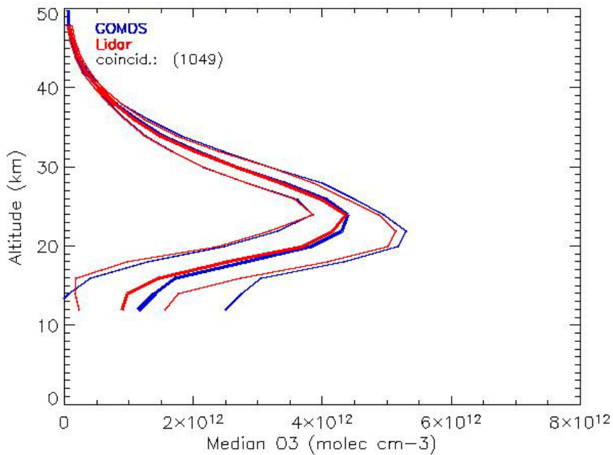
Figure 7.2-3: Same as Figure 7.2-1 for GOMOS (blue thick line) and for lidar (red thick line) measurements in close coincidence (1049 profiles)
