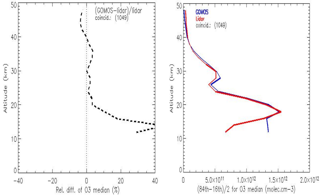
Figure 7.2-4: Relative difference in % of the median profiles plotted in Figure 7.2-3 (left figure). Half difference between 84 th percentile limit and 16 th percentile limit (right figure)
