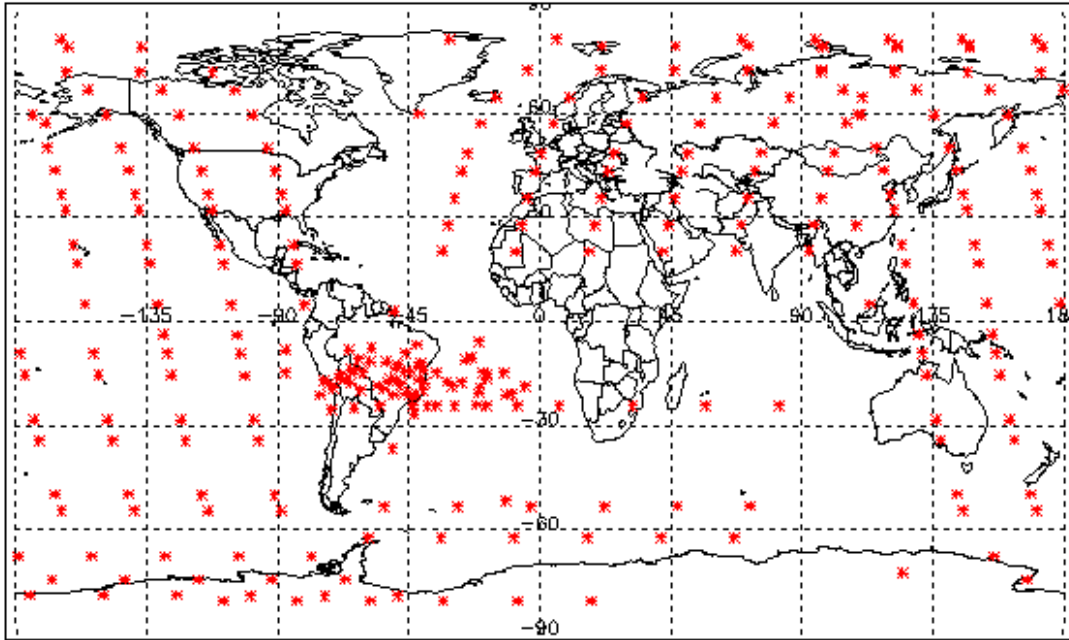
Figure 3.4-2: The red points are the occultation geolocation (starting) corresponding to planned data acquisitions for which no GOMOS level 0 product has become available
