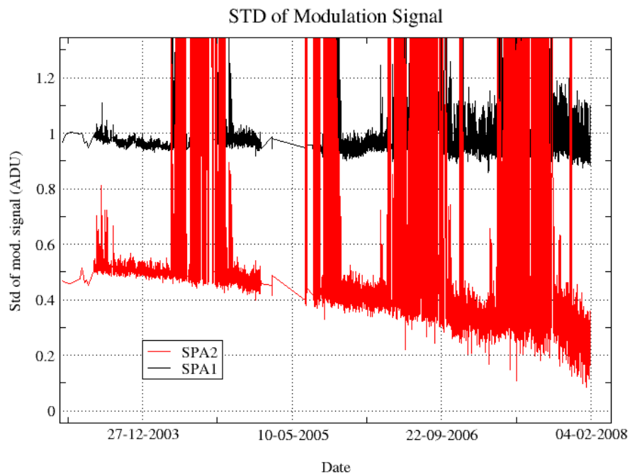
Figure 4.5-4b: Standard deviation of the modulation signal
