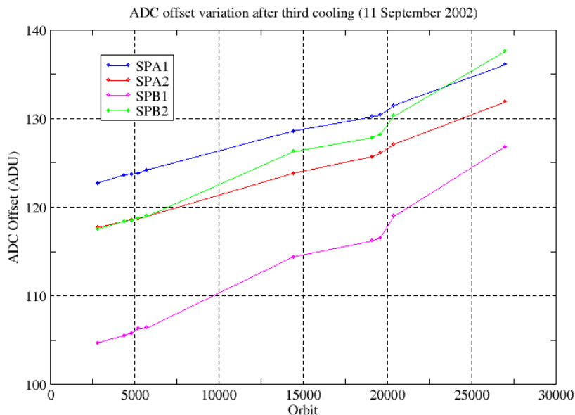
Figure 4.5-5: ADC offset evolution for each spectrometer electronic chain
