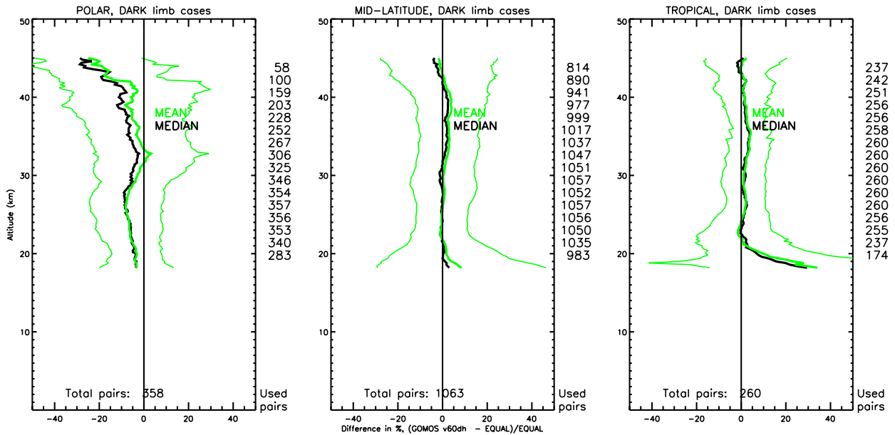
Figure 7.2-1: Mean and median of ozone differences between GOMOS and lidar
