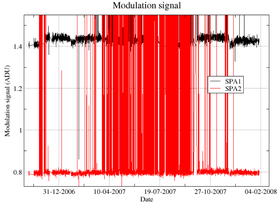
Figure 4.5-4a: Modulation signal
