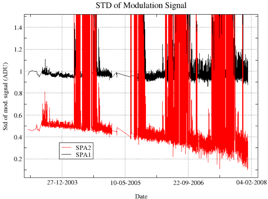
Figure 4.5-4: Standard deviation of the modulation signal
