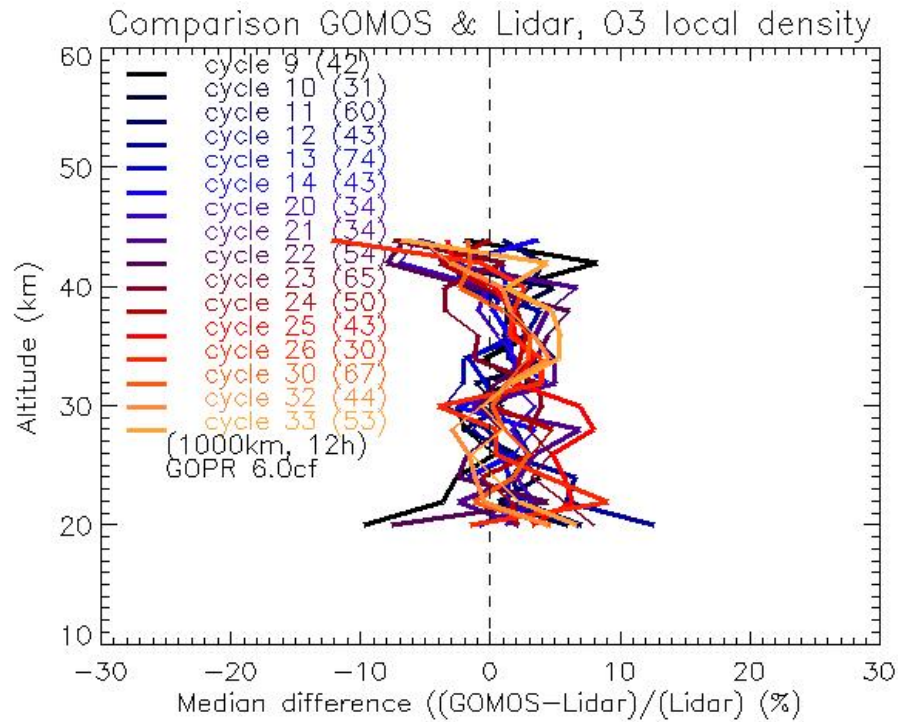
Figure 7.2-1: Vertical profiles of the median of the relative difference between O 3 local density retrieved from GOMOS measurements and O 3 local density provided by ground-based lidar instruments for profiles in close coincidence (distance lower than 1000km; time difference lower than 12h). The median value is calculated for all coincidences by ENVISAT cycle, for some specific cycles with a significant number of coincidences (given in brackets for each cycle)
