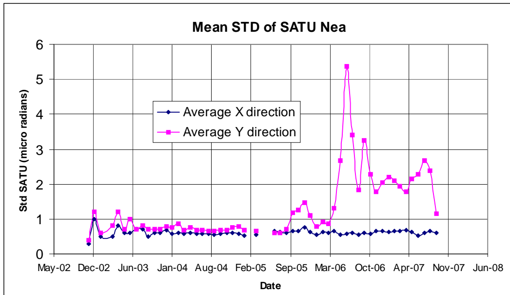
Figure 4.6-1: Average value per day of SATU NEA STD above 105 km
