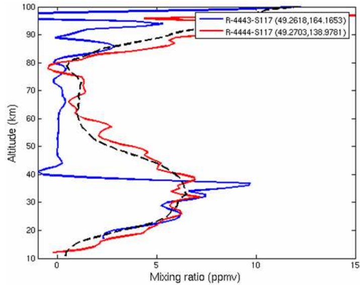
Figure 7.2-5: Vertical profiles of O 3 mixing ratio for two successive occultations of S117 (T = 3800K).
