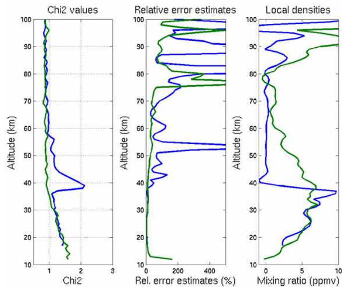
Figure 7.2-6: Vertical profiles of \chi^2 , relative O 3 error estimates (%), and O 3 mixing ratio (ppmv) for the same two occultations as in Figure 7.2- (blue line:R4443/S117; green line: R4444/S117)
