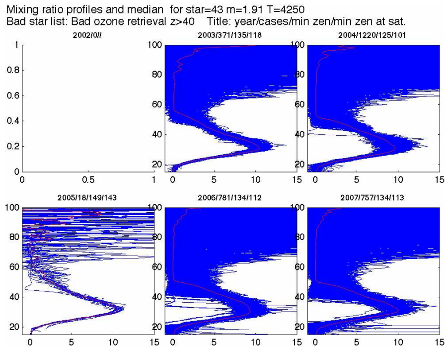
Figure 7.2-1: Vertical profiles of O3 mixing ratio per year between 2002 and 2007 for star 43 (T = 4250K). The red line is the yearly median profile.
