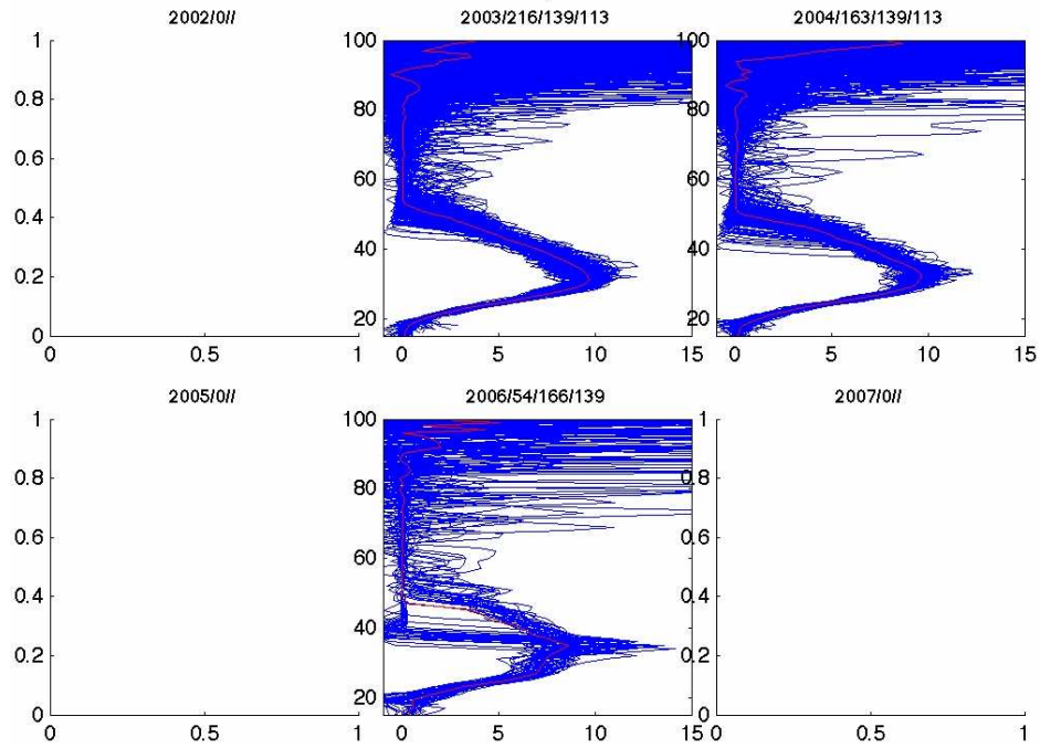
Figure 7.2-4: Vertical profiles of O3 mixing ratio per year between 2002 and 2007 for star 84 (T = 4500K). The red line is the yearly median profile.
