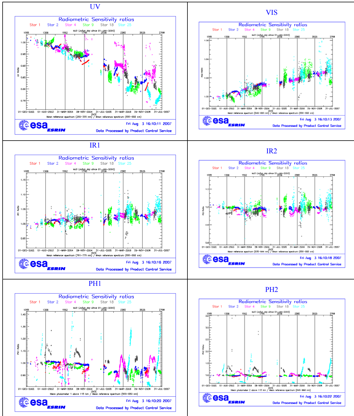
Figure 5.4-1: Radiometric sensitivity ratios since December 2002
