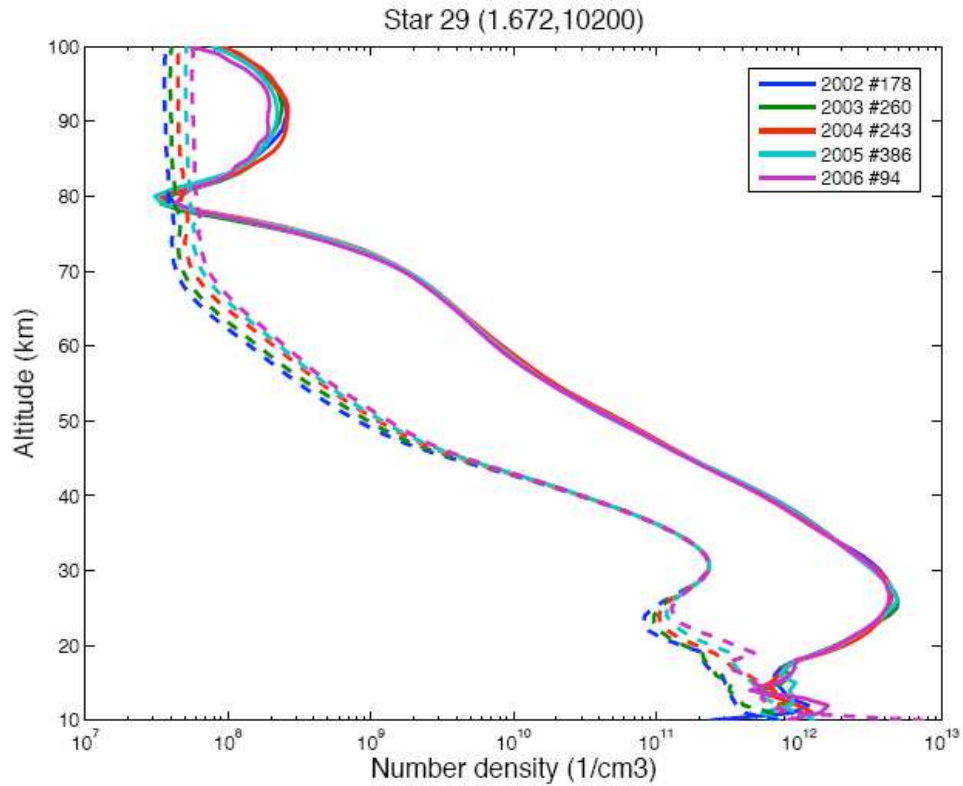
Figure 8.1-3: Median of the local ozone densities (solid line) and their error estimates (dashed line) during each year using star number 29 at latitude band [0°, 10°].
