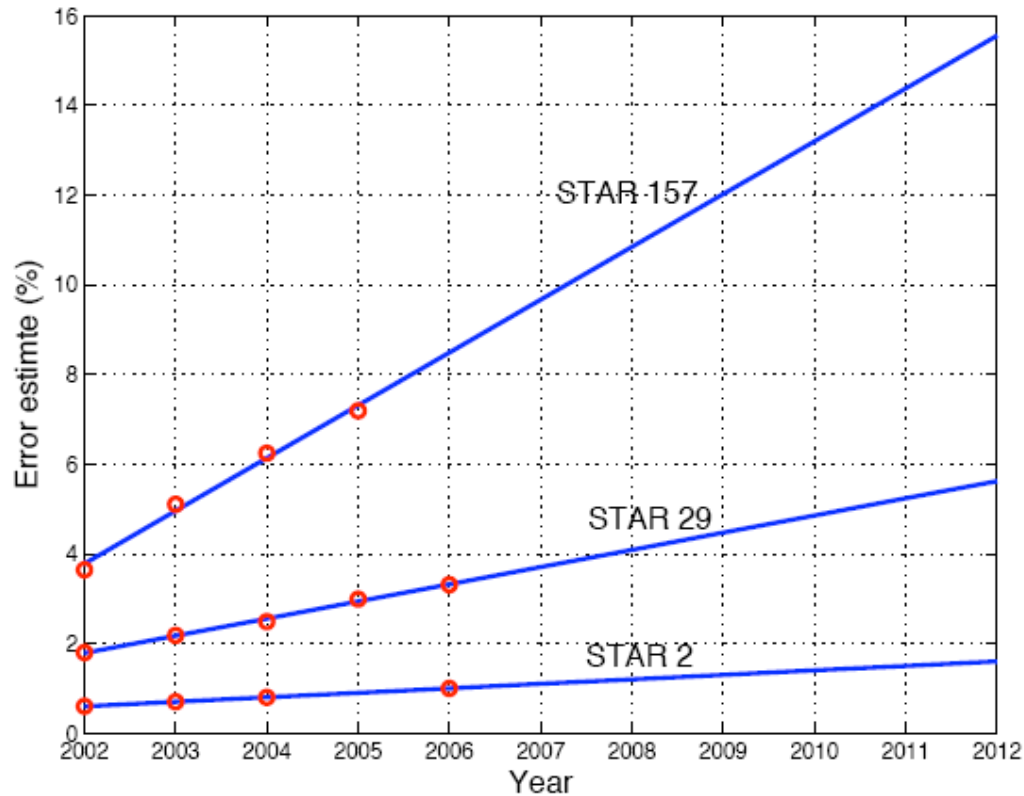
Figure 8.1.4: Linearly approximated evolution of the error estimates of stars 2, 29 and 157 at 60 km altitude. The measured values are denoted with red circles.
