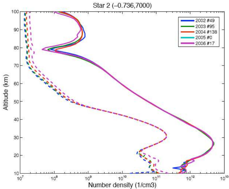
Figure 8.1-2: Median of the local ozone densities (solid line) and their error estimates (dashed line) during each year using star number 2 at latitude band [0^\circ, 10^\circ] .
