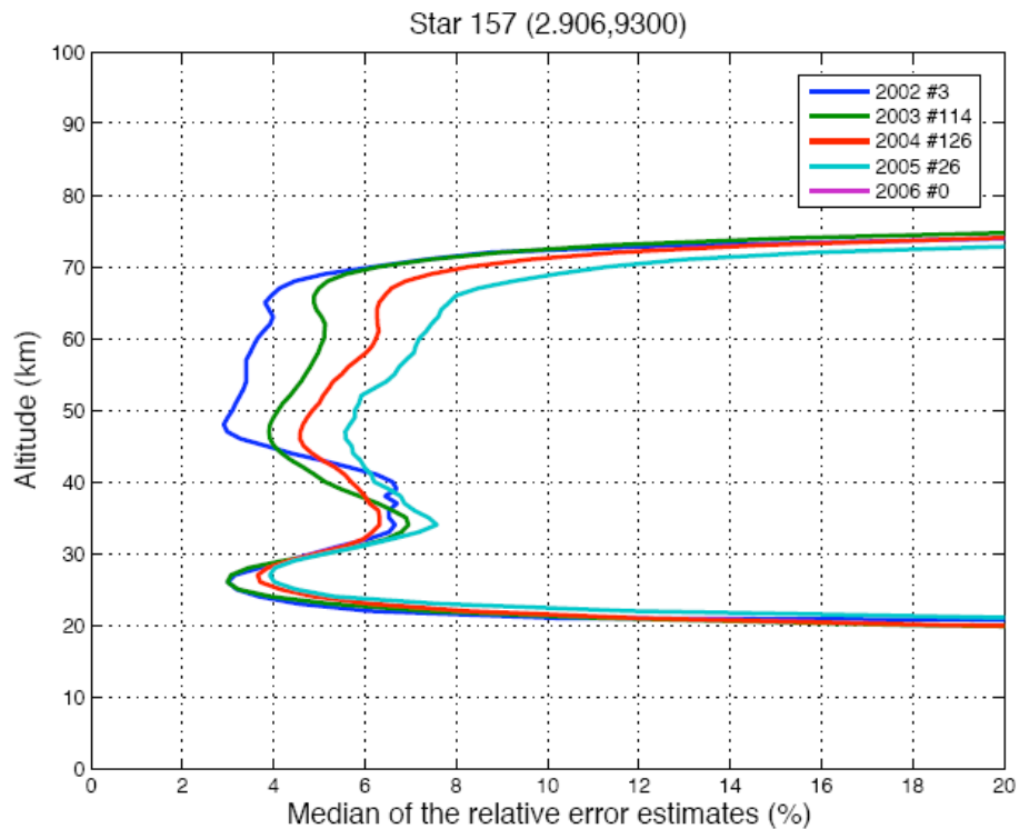
Figure 8.1-3: Yearly median of the relative error estimates of ozone using star number 157 ( M_v = 2.9, T = 9300K ) at latitude band [0^\circ, 10^\circ] . Years 2002–2005 are shown. The number of occultations in each year is indicated in the figure.
