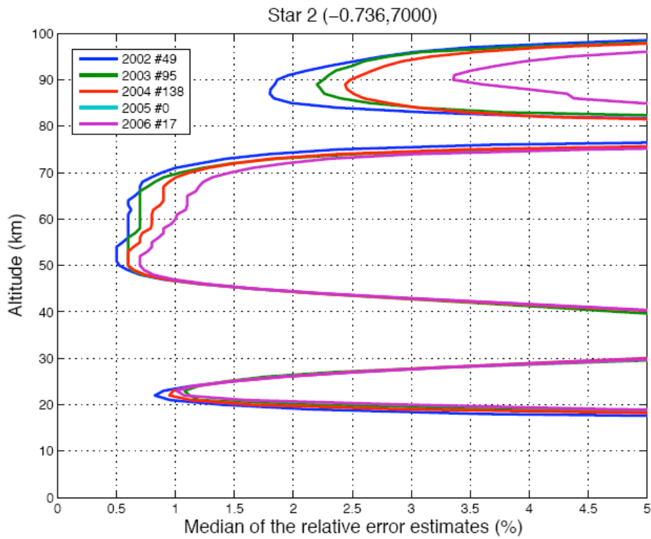
Figure 8.1-1: Yearly median of the relative error estimates of ozone using star number 2 ( M_v = -0.74 , T = 7000\text{K} ) at latitude band [0^\circ, 10^\circ] . Years 2002–2006 except 2005 are shown. The number of occultations in each year is indicated in the figure.
