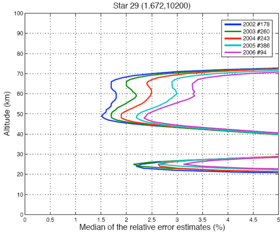
Figure 8.1-2: Yearly median of the relative error estimates of ozone using star number 29 ( M_v = 1.67, T = 10200K ) at latitude band [0^\circ, 10^\circ] . Years 2002–2006 are shown. The number of occultations in each year is indicated in the figure.
