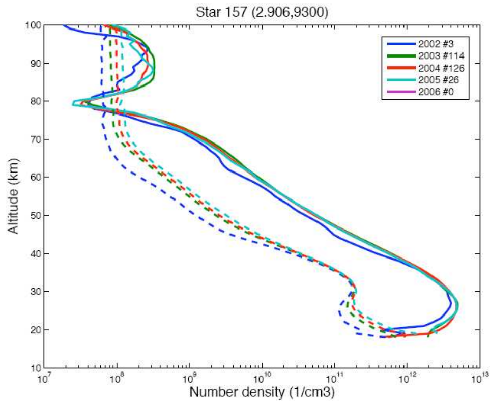
Figure 8.1-6: Median of the local ozone densities (solid line) and their error estimates (dashed line) during each year using star number 157 at latitude band [0°, 10°].
