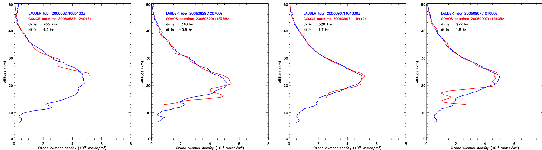
Figure 5: Comparison of GOMOS vertical profile (red line) of O 3 local density ( 10^{18} molec m -3 ) and coincident profile measured by LIDAR (blue line) at Lauder (45.04°S, 169.68°E) on 27/08/2006, 29/08/2006 and 07/09/2006 (two figures).
