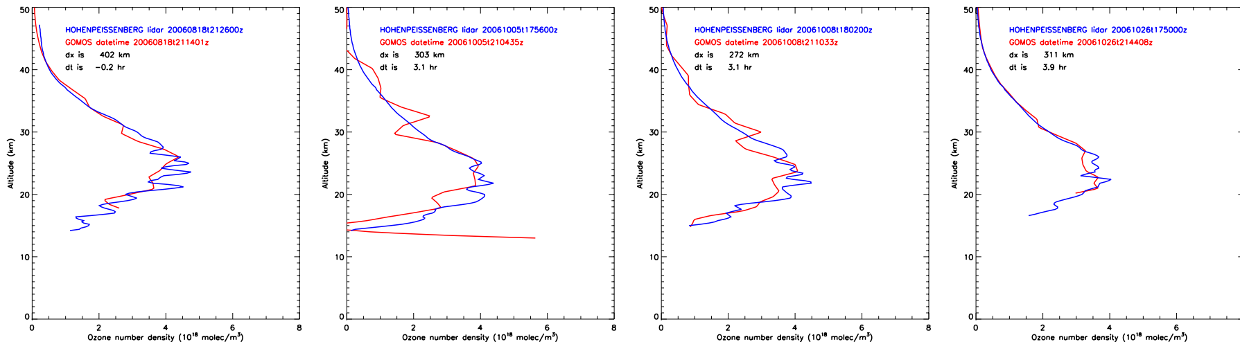
Figure 3: Comparison of GOMOS vertical profile (red line) of O_3 local density ( 10^{18} \text{ molec m}^{-3} ) and coincident profile measured by LIDAR (blue line) at Hohenpeissenberg ( 47.80^\circ\text{N} , 11.02^\circ\text{E} ) on 18/08/2006, 05/10/2006, 08/10/2006, and 26/10/2006.
