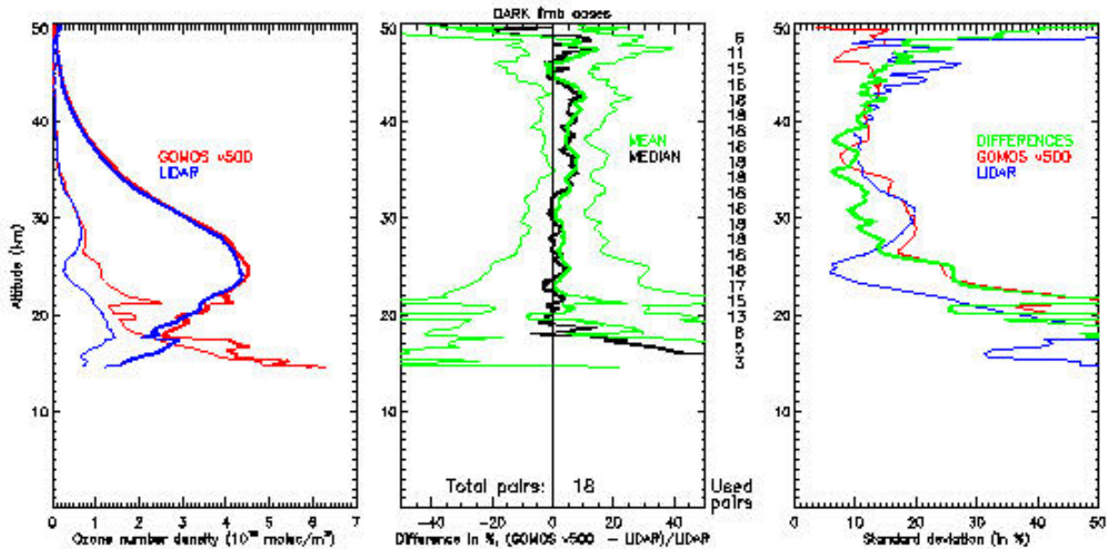
Figure 6: Averaged analysis results of GOMOS ozone profiles compared to LIDAR, for measurements made during the second half of 2006; (left) Mean GOMOS (bold red line) and LIDAR (bold blue line) ozone profiles and their standard deviations (thin lines in corresponding colours). (middle) Mean (bold green line) and median (black line) differences between all the paired GOMOS and LIDAR data as a percentage of the latter. For the mean profile, we also plotted the ( 1\sigma ) standard deviation of the differences (thin green line). Numbers at the right of the middle panel indicate, for some altitude levels, the number of pairs used at that level. (right) A comparison between the standard deviation of the differences (green line) and the standard deviation of all GOMOS (red line) and LIDAR (blue line) ozone profiles.
