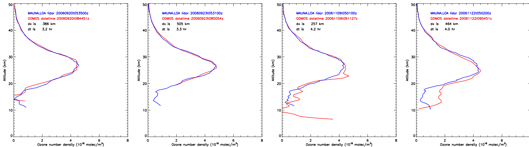
Figure 4: Comparison of GOMOS vertical profile (red line) of O 3 local density ( 10^{18} molec m -3 ) and coincident profile measured by LIDAR (blue line) at Mauna Loa (19.54°N, 155.58°W) on 20/09/2006, 23/09/2006, 09/11/2006 and 22/11/2006.
