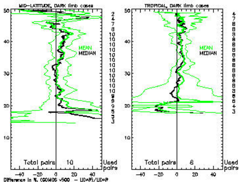
Figure 7: Same as middle figure of Figure 36 for mid-latitude (left figure) and tropical cases (right figure).
