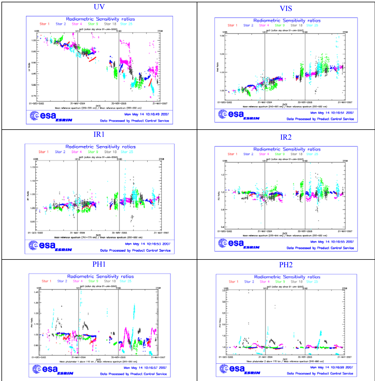
Figure 5.4-1: Radiometric sensitivity ratios since December 2002
