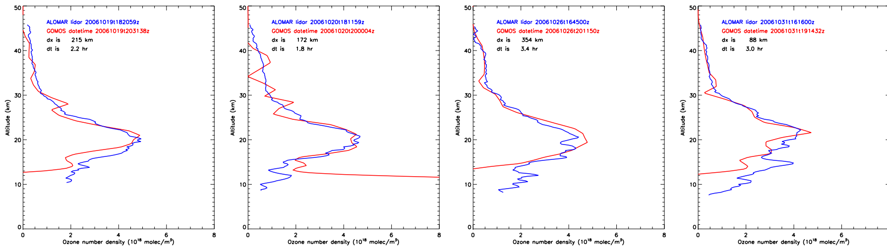
Figure 2: Comparison of GOMOS vertical profile (red line) of O_3 local density ( 10^{18} \text{ molec m}^{-3} ) and coincident profile measured by LIDAR (blue line) at Alomar ( 69.30^\circ\text{N} , 16.00^\circ\text{E} ) on 19/10/2006, 20/10/2006, 26/10/2006, and 31/10/2006.
