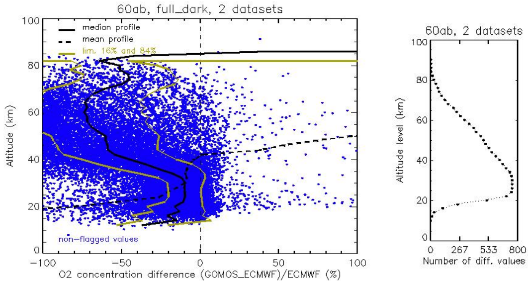
Figure 7.1-1: Left figure: Relative difference of O 2 concentration from GOMOS measurements and from ECMWF data (O_{2,GOMOS} - O_{2,ECMWF}) / O_{2,ECMWF} in % as a function of vertical altitude (blue dots); vertical profile of the median of the difference (black solid line); vertical profile of the mean of the difference (black dashed line); 84 and 16 percentile limits (yellow solid lines). Only non-flagged values are used. Results are based on a dataset of about 800 dark limb occultations at various latitudes processed with GOPR version 6.0ab. Right figure: number of difference values used at each altitude level to calculate the statistical quantities
