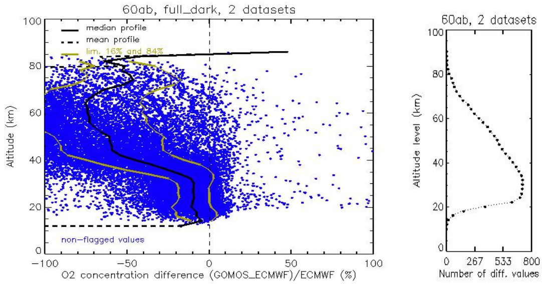
Figure 7.1-3: Same as fig. 7.1-1 for common non-flagged values between 6.0ab and 6.0cf
