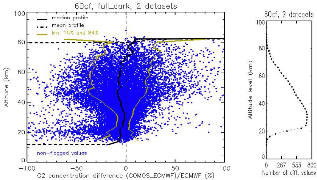
Figure 7.1-4: Same as fig. 7.1-2 for common non-flagged values between 6.0ab and 6.0cf
