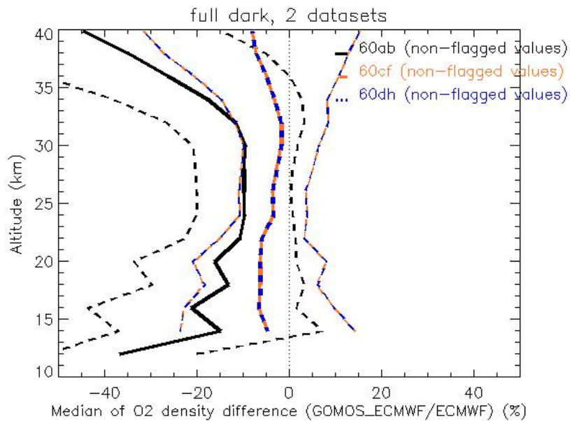
Figure 7.1-5: vertical profiles of the median of the difference (thick solid line); vertical profiles of 84 and 16 percentile limits (thin dashed lines) of results shown in fig. 7.1-1 and fig. 7.1-2 (all non-flagged values) between 10km and 40km. Also plotted are results for GPR 6.0dh (blue lines)
