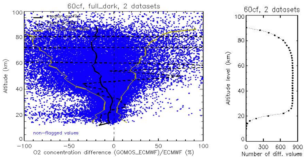
Figure 7.1-2: Same as fig. 7.1-1 for the dataset processed with GOPR version 6.0cf
