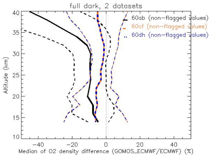
Figure 7.1-6: vertical profiles of the median of the difference (thick solid line); vertical profiles of 84 and 16 percentile limits (thin dashed lines) of results shown in fig. 7.1-3 and fig. 7.1-4 (only common non-flagged values) between 10km and 40km. Also plotted are results for GPR 6.0dh (blue lines)
