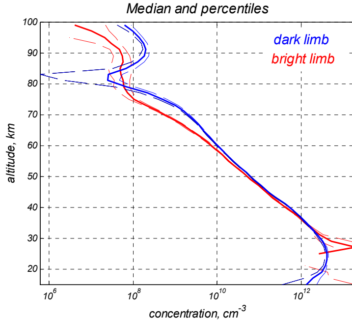
Figure 7.4-3: Comparison of collocated GOMOS dark and bright limb occultations: median profiles and percentiles (16th and 84th)
