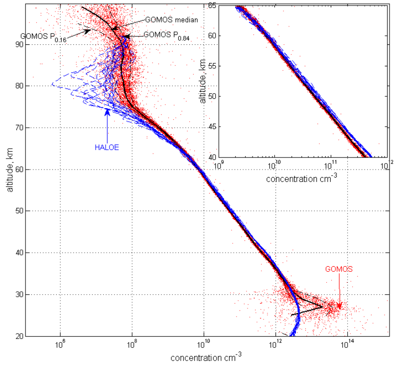
Figure 7.5-1: Comparison of GOMOS and HALOE data
