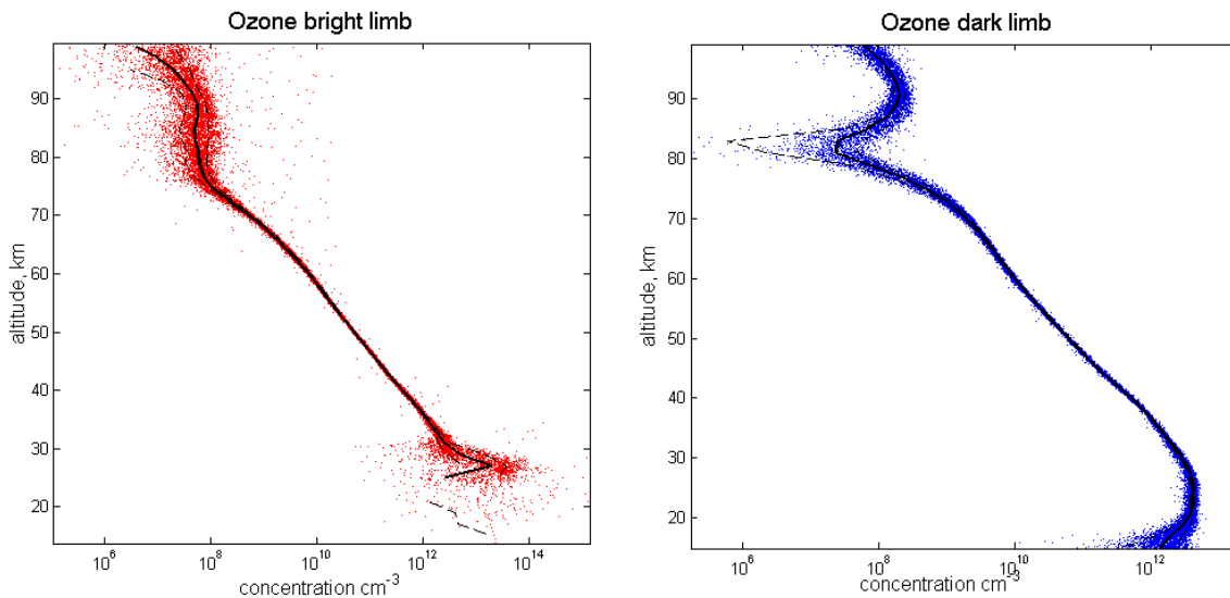
Figure 7.4-2: Comparison of collocated GOMOS dark and bright limb occultations: all profiles
