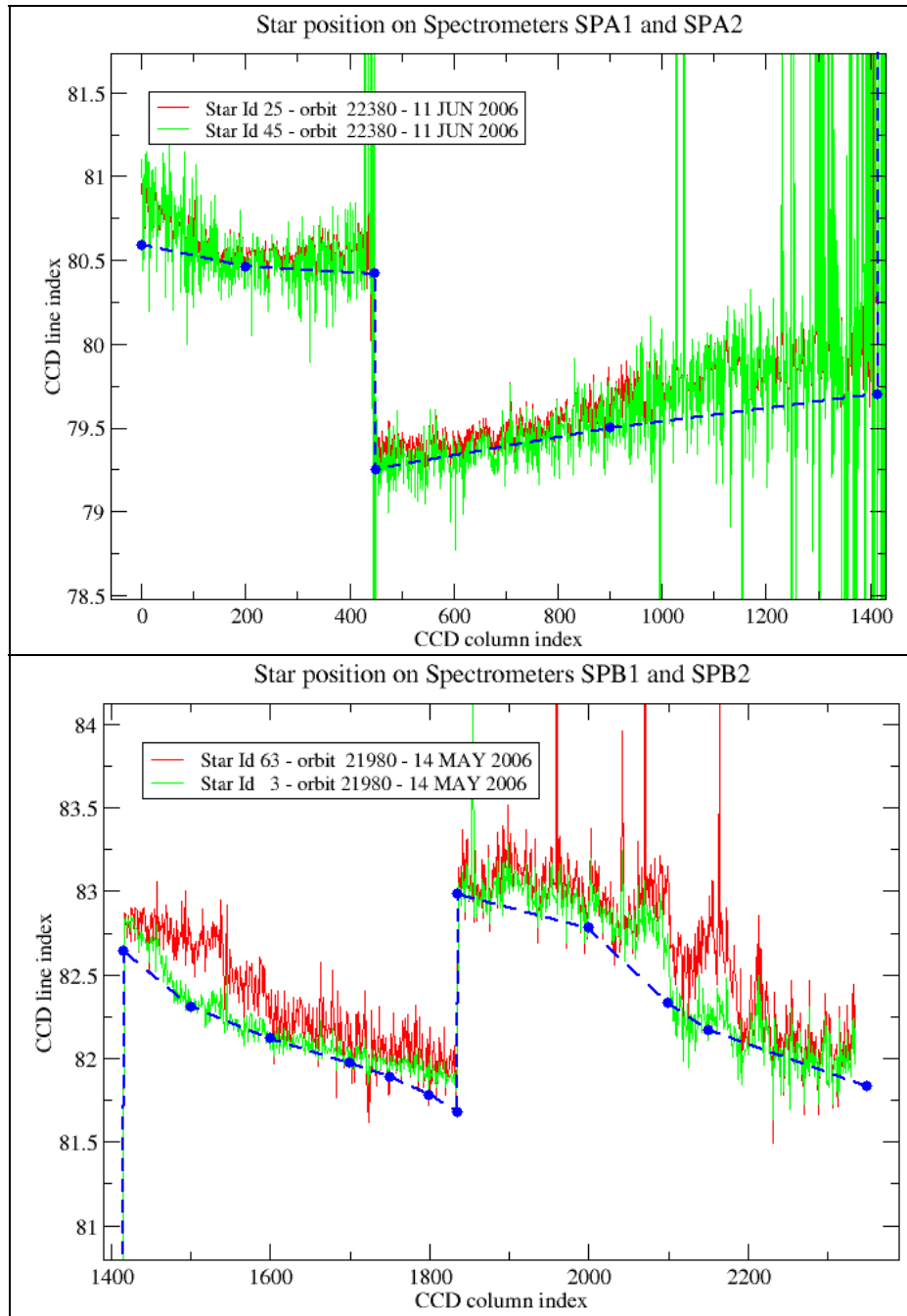
Figure 4.4-1: Average position of star spectra on the CCD for SPA (upper) and SPB (lower)
