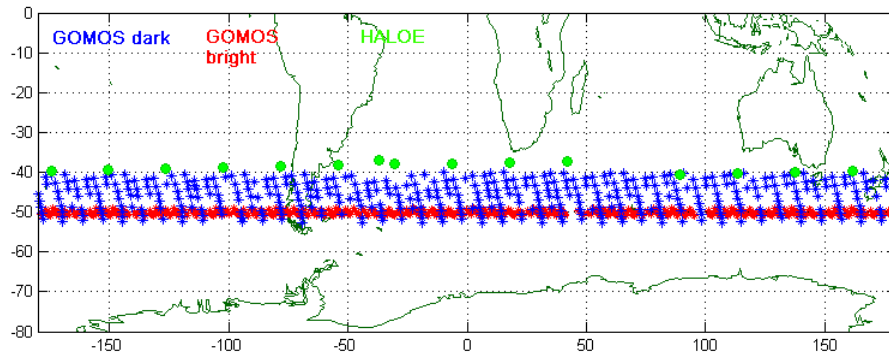
Figure 7.4-1: Location of occultations (Jan-Feb 2004) selected for the comparison
