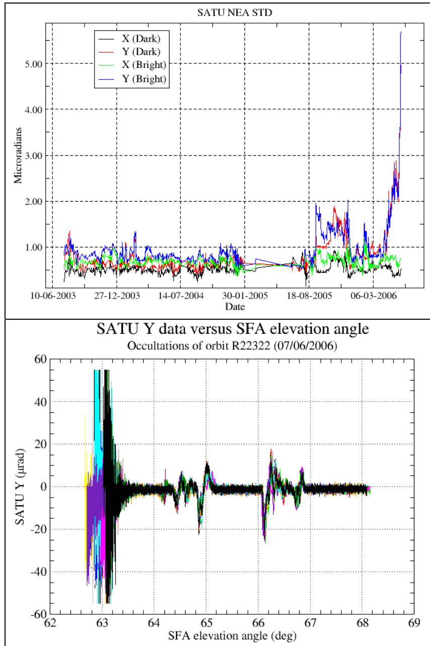
Figure 4.6-1: (Upper plot) Average value per day of SATU NEA STD above 105 km. (Lower plot) SATU 'Y' data as a function of elevation angle
