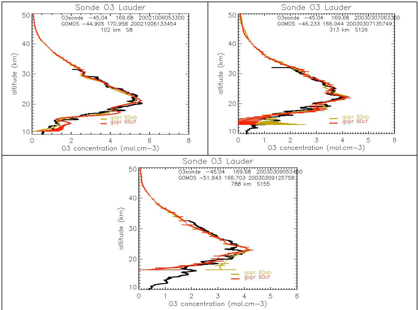
Figure 7.5-4: Comparison between GOMOS vertical profile of O3 local density for different occultations and coincident profile measured by ozonesonde at Lauder and Legionowo stations. Yellow line: GOMOS profile retrieved with GPR 6.0ab; red line: GOMOS profile retrieved with GPR 6.0cf; black line: profile measured by ozonesonde. Date and location of the measurements are given in the figures, as well as the distance between the GOMOS and the sonde profiles
