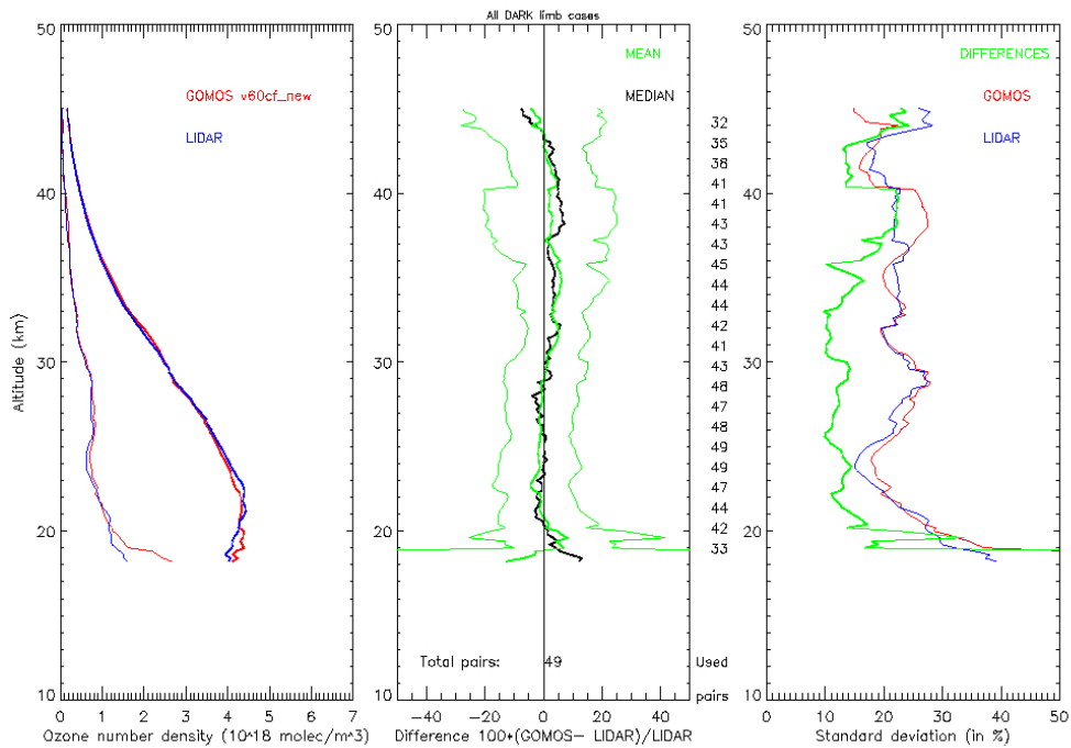
Figure 7.5-2: Results of the comparison between GOMOS O 3 vertical profiles from occultations measured in full dark limb between August 2005 and March 2006 and ground-based measurements. Left figure: Vertical profiles of the average and of the dispersion of O 3 local density retrieved with GPR 6.0cf (red line), and measured by ground-based lidar instruments (blue line), between 0 and 50km. Middle figure: Vertical profiles of the average relative difference between O 3 local density retrieved with GPR 6.0cf and measured by ground-based lidar instruments (in %); vertical profile of the mean relative difference and of its dispersion (green line); vertical profile of the median
