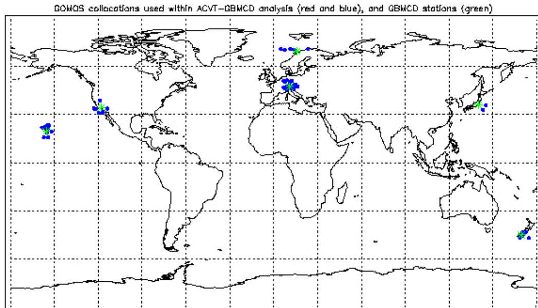
Figure 7.5-1: Map of the co-locations between GOMOS measurements and ground-based lidar stations used for the analysis
