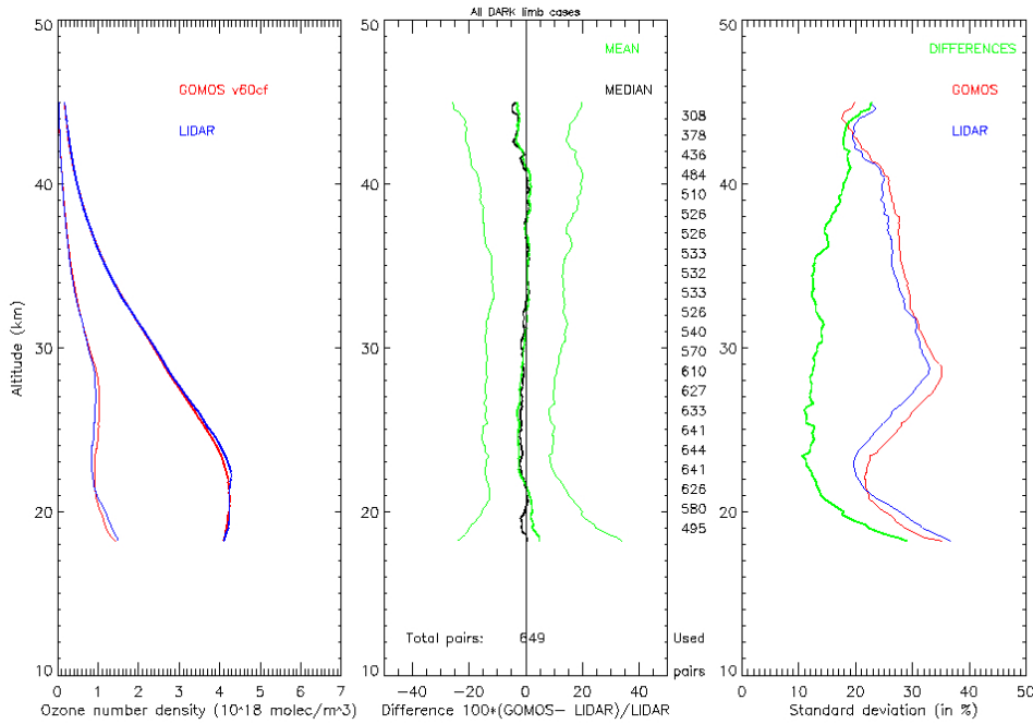
Figure 7.5-3: Same as fig. 7-5.2 for GOMOS measurements between July 2002 and March 2005
