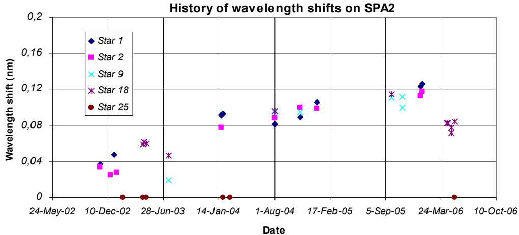
Figure 5.3-1: Wavelength shifts on SPA2 since 12 th November 2002 calculated using different stars
