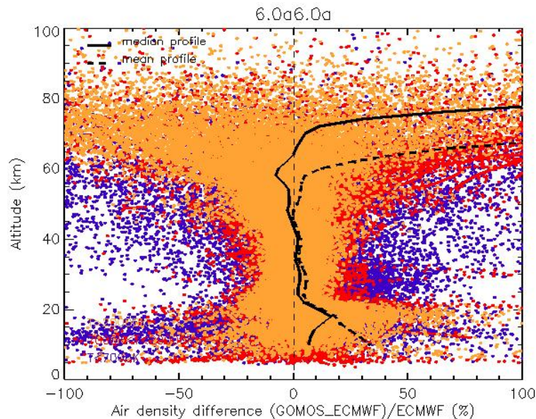
Figure 7.1-3: Values of the difference between GOMOS air density and ECMWF air density for 2000 full dark measurements of cycle 22 (v6.0a6.0a); vertical profiles of the median difference (solid line) and of the mean difference (dashed line). The colour code is as follows: T < 7000K ; 7000K < T < 20000K ; T > 20000K
