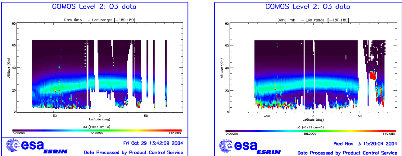
Figure 6.3-1: Average GOMOS O 3 profile during September (left) and October (right): average in a grid of 0.5° latitude x 1 km altitude
