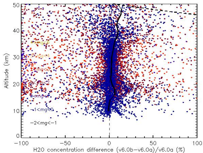
Figure 7.4-1: Values of the difference between H 2 O concentration values processed from GOPR v6.0b6.0a and GOPR v6.0a6.0a for 1000 full dark occultations of cycle 22; vertical profile of the median of the difference (solid line); vertical profile of the mean of the difference (dashed line).
