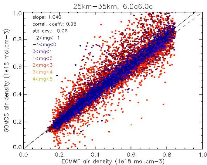
Figure 7.1-1: Air density values inferred from GOMOS measurements versus air density values by ECMWF, for 2000 full dark measurements of cycle 22 (v6.0a6.0a) and at altitudes between 25km and 35 km.
