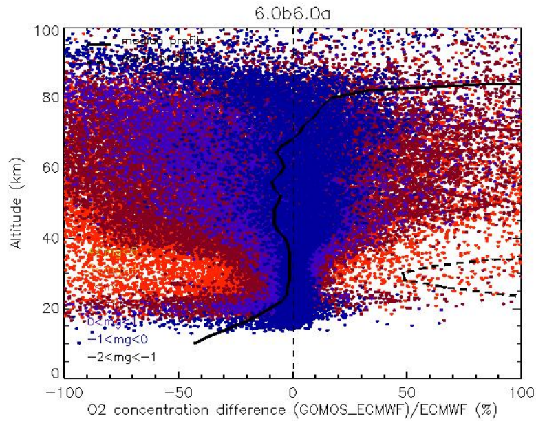
Figure 7.1-5: Same as fig. 7.1-4 for GOMOS profiles processed with GOPR version 6.0b6.0a. The colour code according to the star magnitude is as follows: -2 < mg < -1; -1 < mg < 0; 0 < mg < 1; 1 < mg < 2; 2 < mg < 3; 3 < mg < 4 4 < mg < 5
