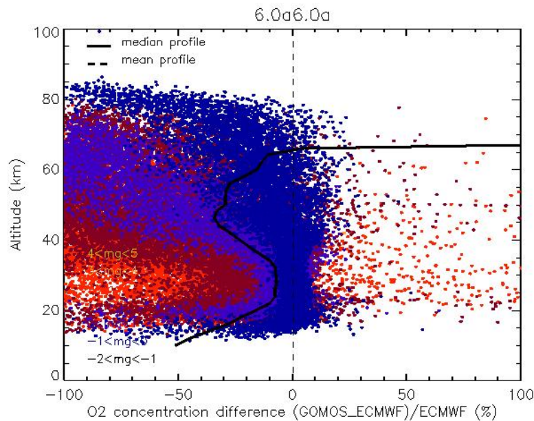
Figure 7.1-4: Values of the difference between GOMOS O 2 concentration and ECMWF O 2 concentration for 2000 full dark measurements of cycle 22 (GOPR version 6.0a6.0a); vertical profiles of the median difference (solid line). The colour code according to the star magnitude is as follows: -2 < mg < -1; -1 < mg < 0; 0 < mg < 1; 1 < mg < 2; 2 < mg < 3; 3 < mg < 4; 4 < mg < 5
