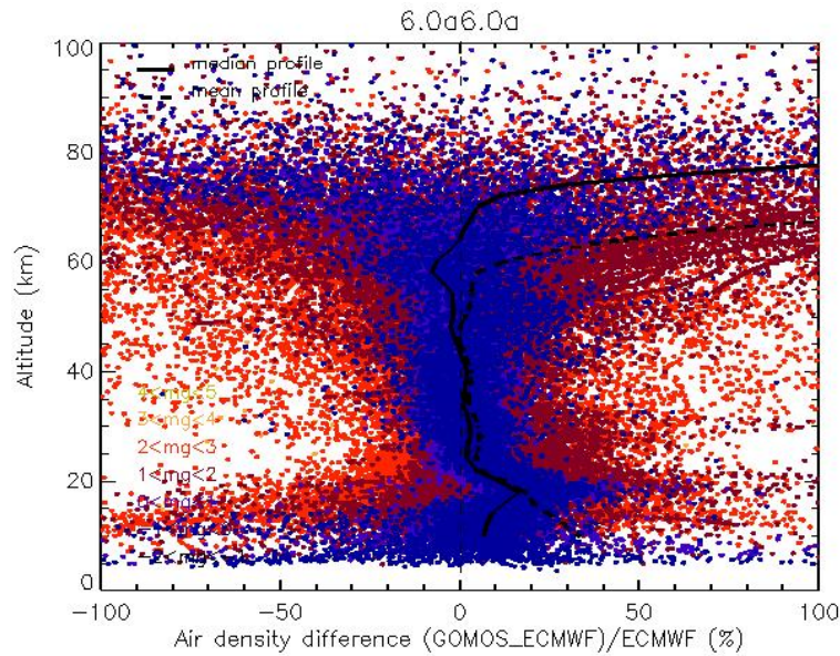
Figure 7.1-2: Values of the difference between GOMOS air density and ECMWF air density for 2000 full dark measurements of cycle 22 (v6.0a6.0a); vertical profiles of the median difference (solid line) and of the mean difference (dashed line). The colour code according to the star magnitude is as follows: -2 < mg < -1 ; -1 < mg < 0 ; 0 < mg < 1 ; 1 < mg < 2 ; 2 < mg < 3 ; 3 < mg < 4 ; 4 < mg < 5
