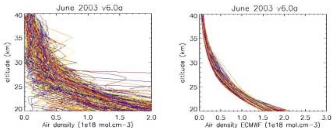
Figure 7.1-2: Vertical profiles of air density values inferred from GOMOS measurements (left figure), and air density values given by ECMWF (right figure), for altitudes between 20km and 40km, for full dark occultations
