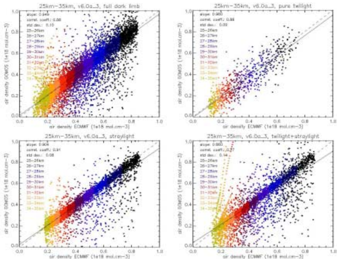
Figure 7.1-1: Correlation between air density values inferred from GOMOS measurements, and air density values given by ECMWF, for altitudes between 25km and 35km, for the four illumination condition types. Values of the correlation coefficient are given on the figures
