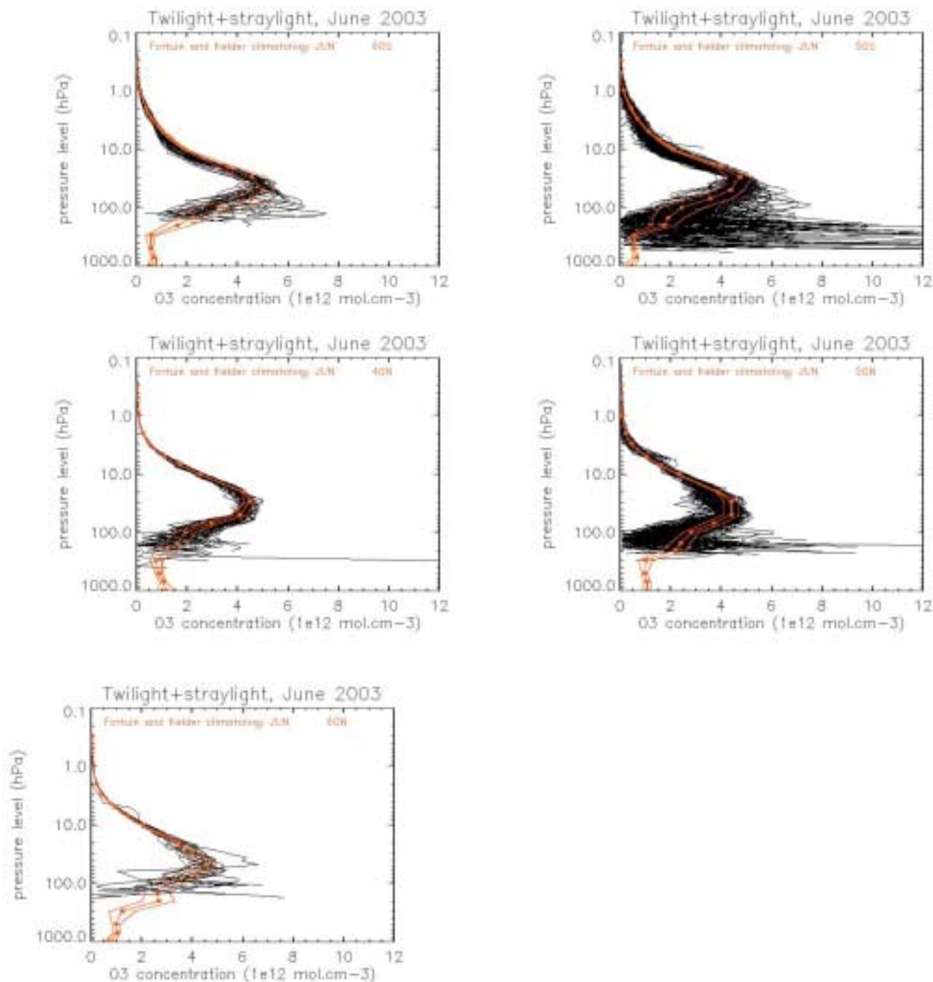
Figure 7.2-1: Vertical profiles of O 3 concentration from GOMOS (black solid lines), for the four illumination condition types, within different latitude bands; vertical profile of O 3 concentration and its variability from Fortuin-Kelder climatology for the corresponding latitude band (orange solid lines)
