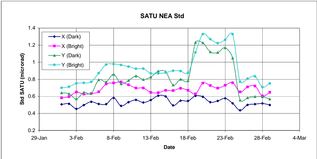
Figure 4.5-1: Average value per day of SATU NEA std above 105 km
