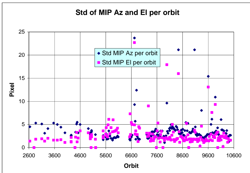
Figure 4.5-7: Standard deviation of MIP Azimuth and Elevation for some orbits since 1 st September 2002 (see table 4.5-1)
