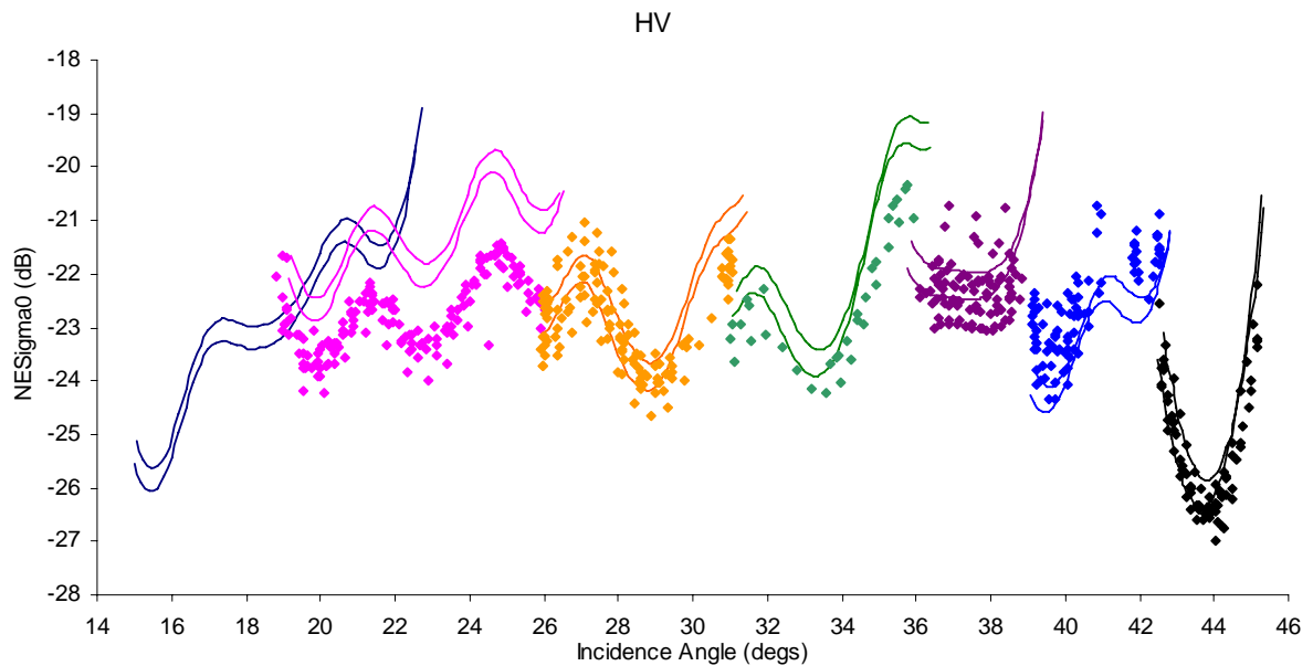
Figure 6.3(a). NESigma0 measurements from AP products and HV polarisation.
