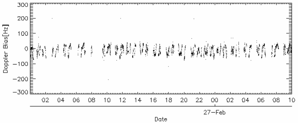
(b) residual Doppler evolution versus time of day
