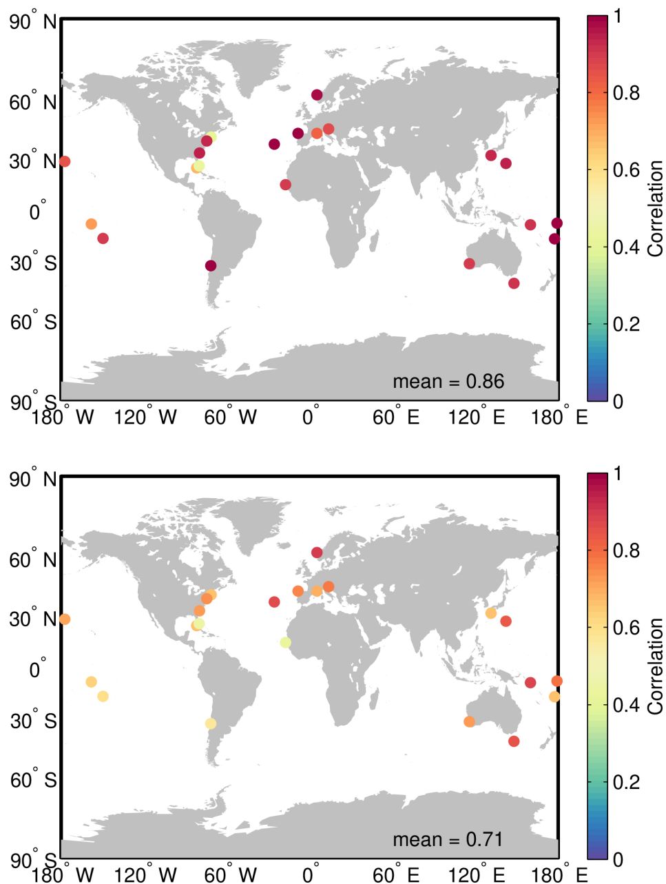
Figure 106. Map showing the correlation between the GOP SSH anomaly and the sea level from tide gauge records over the period January 2022 to December 2023 for the cases with (top) and without (bottom) the tidal component. For this comparison the atmospheric component has not been subtracted. Empty dots denote statistically non-significant correlation.
