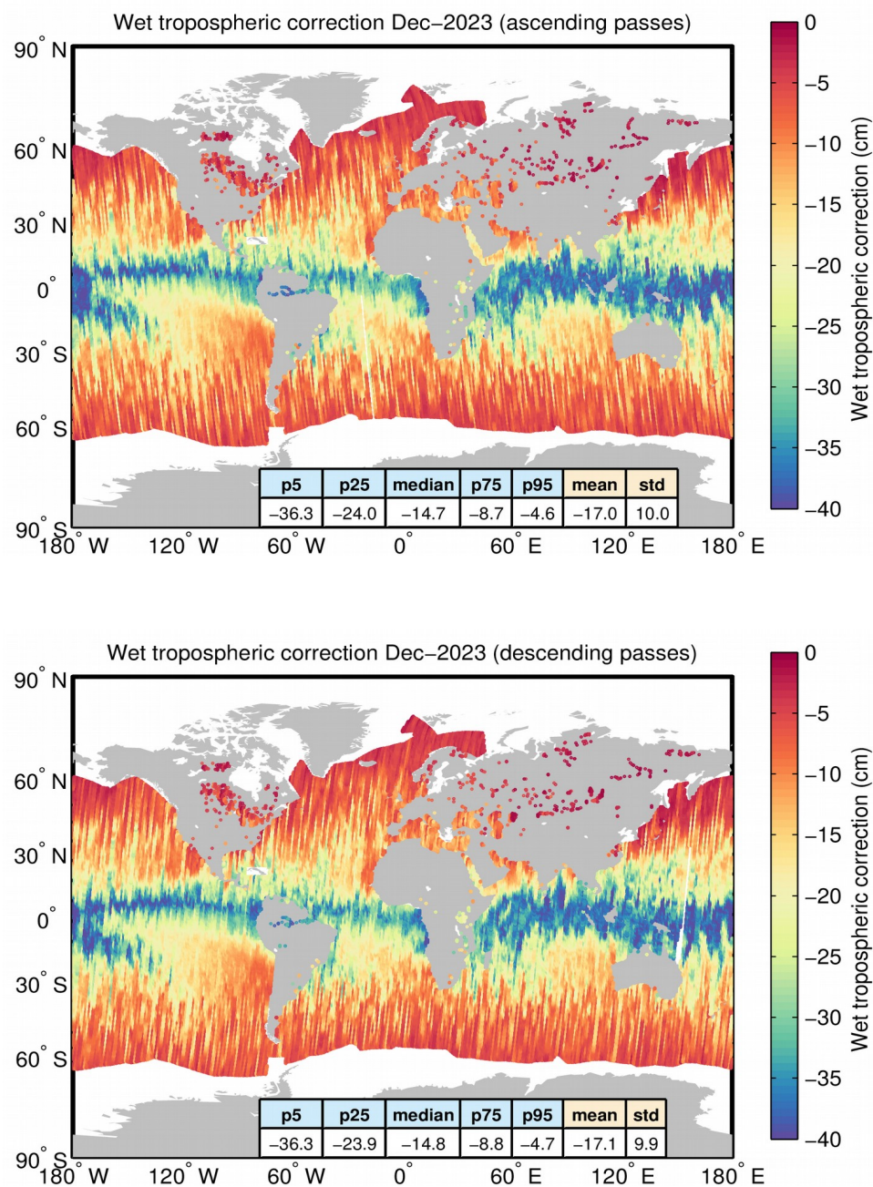
Figure A1. Geographical distribution of the wet tropospheric correction over oceans and lakes for ascending (top) and descending (bottom) passes for December 2023. The statistical values shown in the table refer to the wet tropospheric correction in cm. Measurements taken over polar polygons have been excluded from the computation of the statistical values. The black lines mark the outer limit of the Arctic and Antarctic polar polygons.
