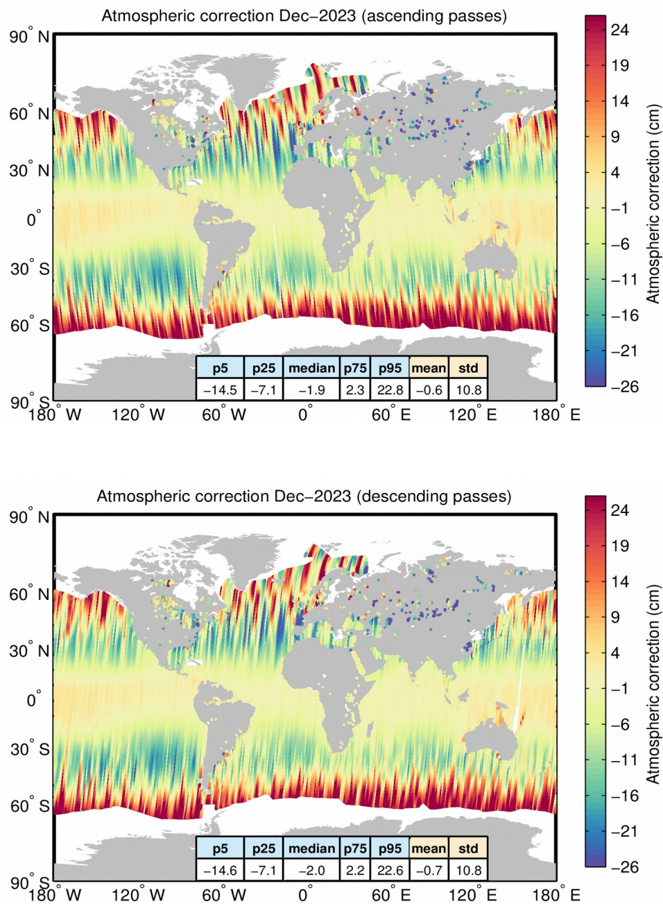
Figure A5. Geographical distribution of the atmospheric correction over oceans and lakes for ascending (top) and descending (bottom) passes for December 2023. The statistical values shown in the table refer to the atmospheric correction in cm. Measurements taken over polar polygons have been excluded from the computation of the statistical values. The black lines mark the outer limit of the Arctic and Antarctic polar polygons.
