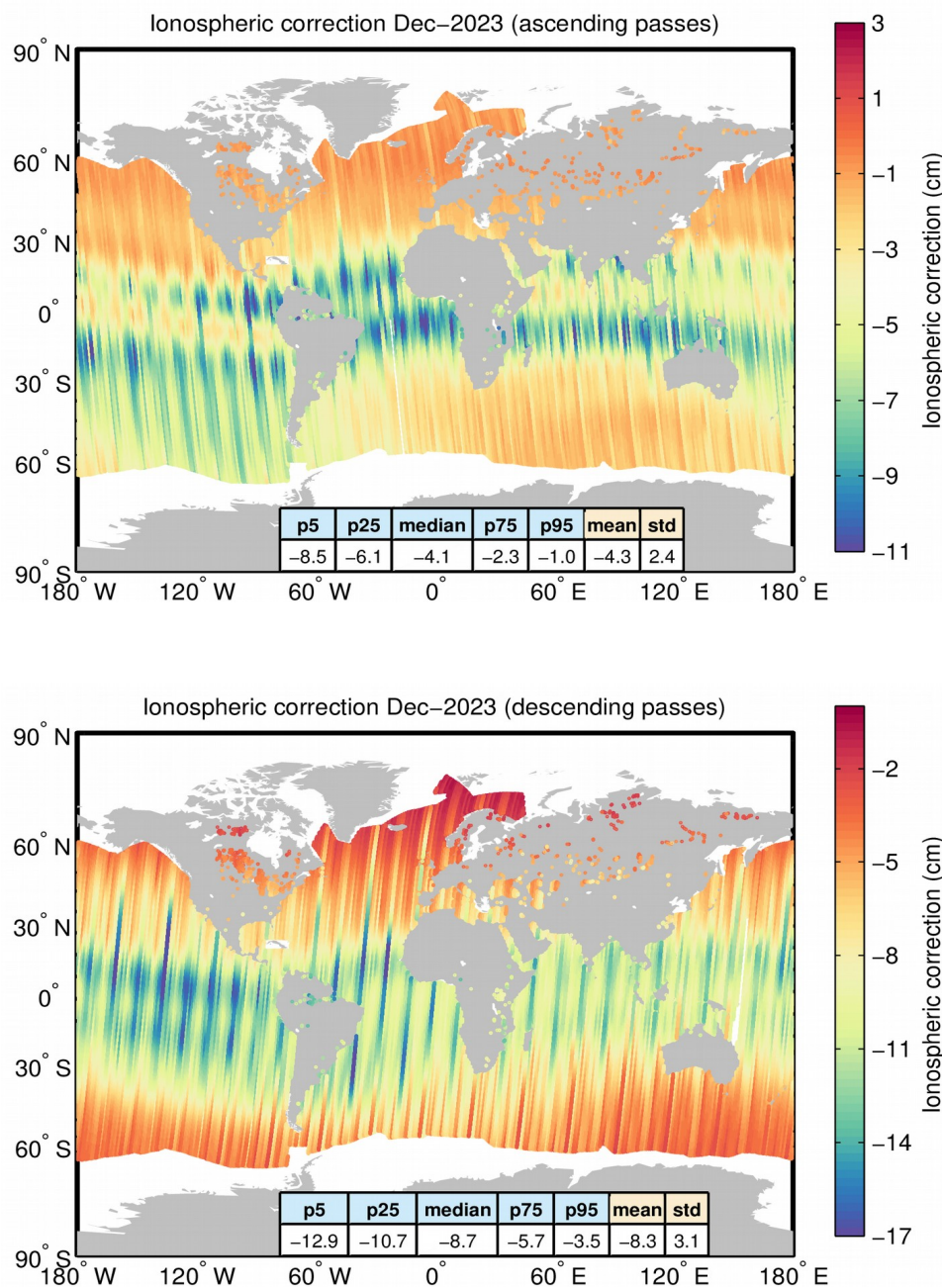
Figure A3. Geographical distribution of the Ionospheric correction over oceans and lakes for ascending (top) and descending (bottom) passes for December 2023. The statistical values shown in the table refer to the Ionospheric correction in cm. Measurements taken over polar polygons have been excluded from the computation of the statistical values. The black lines mark the outer limit of the Arctic and Antarctic polar polygons.
