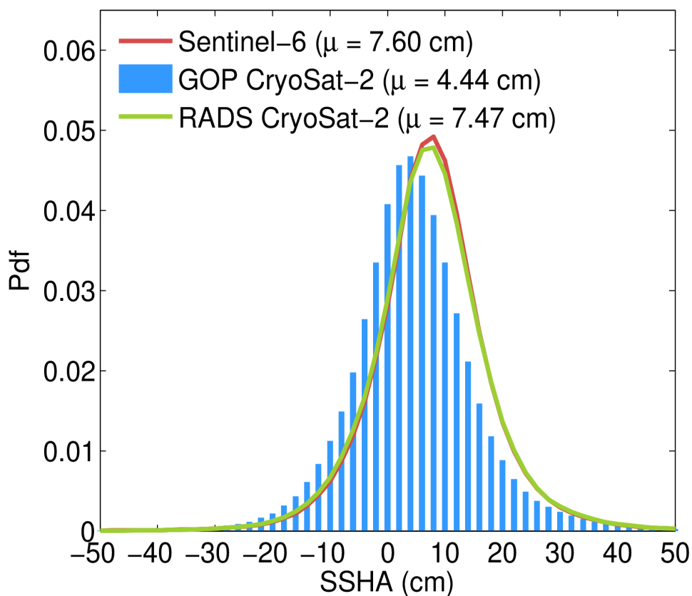
Figure 127. Histograms (normalized to have a total area of 1) of the SSH anomaly from GOP (blue bars), reference mission (red line) and RADS CryoSat-2 (green) for December 2023.
