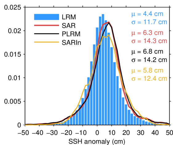
Figure 75. Histogram of science-valid GOP SSH anomaly over oceans and lakes for LRM (blue), SAR (red), PLRM (black) and SARIn (orange) for December 2023. The mean ( \mu )
