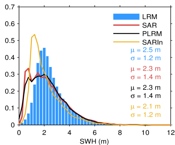
Figure 17. Histogram of science-valid NOP SWH over oceans and lakes for LRM (blue), SAR (red), PLRM (black) and SARIn (orange) for December 2023. The mean ( \mu ) and standard deviation ( \sigma ) are also shown. Values larger than 12 m are excluded from the histogram for the sake of readability but not from the computation of \mu and \sigma .
