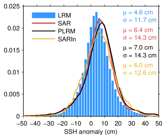
Figure 41. Histogram of science-valid IOP SSH anomaly over oceans and lakes for LRM (blue), SAR (red), PLRM (black) and SARIn (orange) for December 2023. The mean ( \mu ) and standard deviation ( \sigma ) are also shown. Values outside [-50, 50] cm are excluded from the histogram for the sake of readability but not from the computation of \mu and \sigma .
