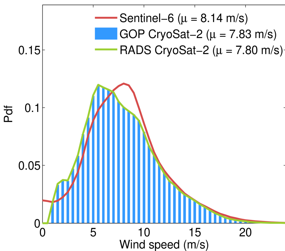
Figure 129. Histograms (normalized to have a total area of 1) of the wind speed from GOP (blue bars), reference mission (red line) and RADS CryoSat-2 (green) for December 2023.
