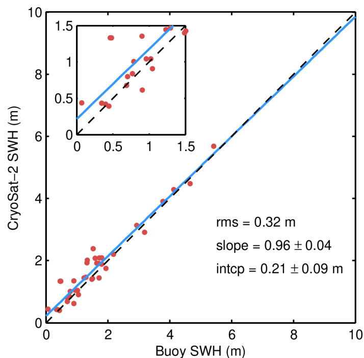
Figure 112. Scatter plot showing a comparison of GOP SWH with SWH from NDBC buoy data for December 2023. The inset plot shows a zoomed-in for SWH < 1.5 m.
