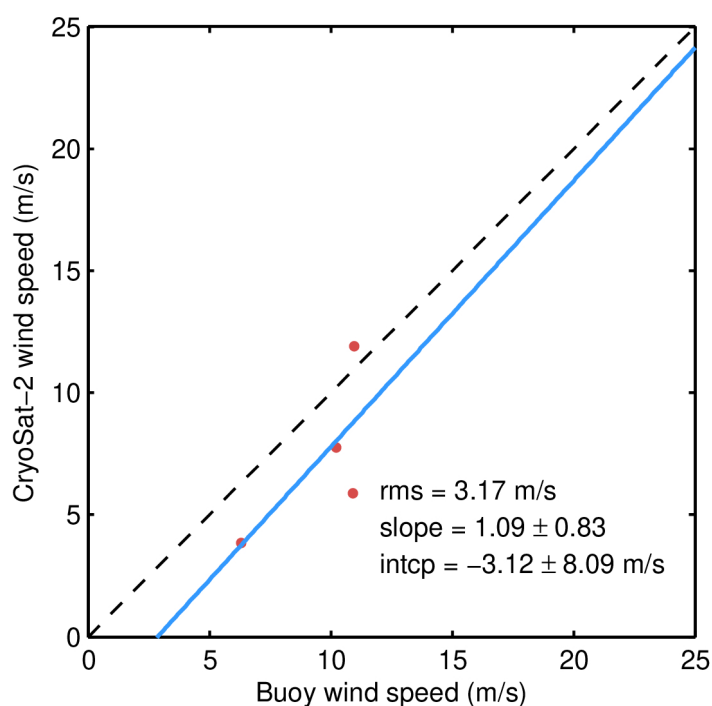
Figure 115. Scatter plot showing a comparison of GOP wind speed with wind speed from NDBC buoy data for December 2023.
