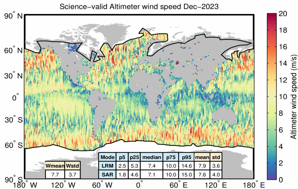
Figure 98. Geographical distribution of science-valid GOP wind data over oceans and lakes for December 2023. The statistical values shown in the table refer to the wind in m and are calculated separately for LRM and SAR regions. Wmean and Wstd denote the spatial area-weighted average and its standard deviation. Measurements taken over polar polygons have been excluded from the computation of the statistical values. The black lines mark the outer limit of the Arctic and Antarctic polar polygons.
