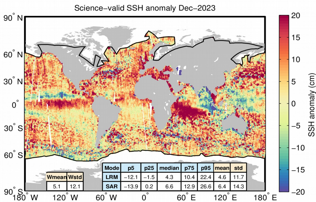
Figure 40. Geographical distribution of science-valid IOP 1-Hz SSH anomaly data over oceans and lakes for December 2023. The statistical values shown in the table refer to the SSH anomaly in cm and are calculated separately for LRM and SAR regions. Wmean and Wstd denote the spatial area-weighted average and its standard deviation. Measurements taken over polar polygons have been excluded from the computation of the statistical values. The black lines mark the outer limit of the Arctic and Antarctic polar polygons.
