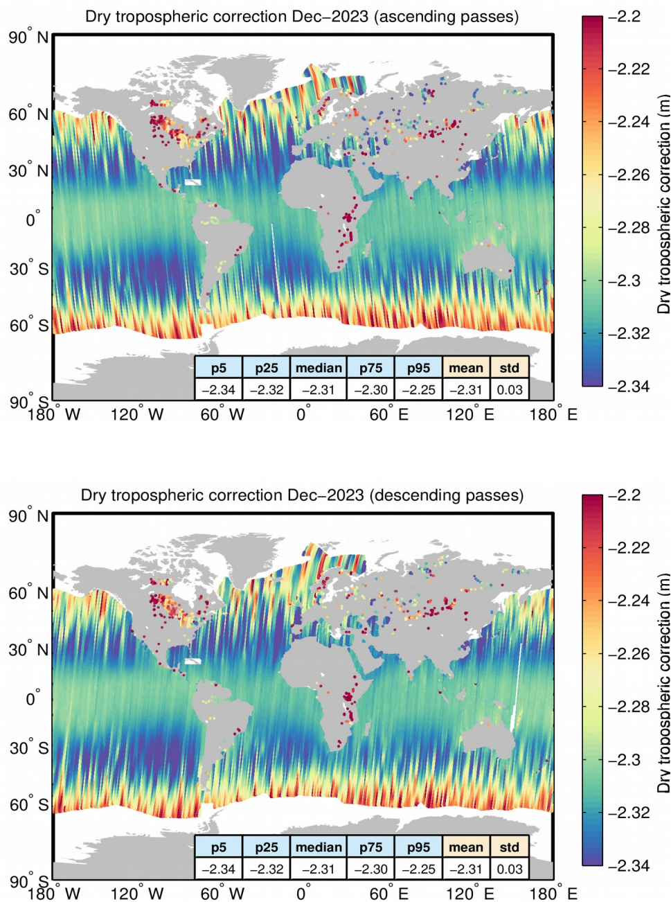
Figure A2. Geographical distribution of the dry tropospheric correction over oceans and lakes for ascending (top) and descending (bottom) passes for December 2023. The statistical values shown in the table refer to the dry tropospheric correction in m. Measurements taken over polar polygons have been excluded from the computation of the statistical values. The black lines mark the outer limit of the Arctic and Antarctic polar polygons.
