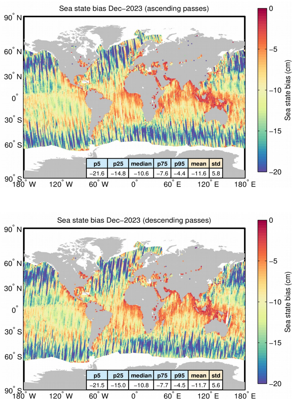
Figure A4. Geographical distribution of the sea state bias over oceans and lakes for ascending (top) and descending (bottom) passes for December 2023. The statistical values shown in the table refer to the sea state bias in cm. Measurements taken over polar polygons have been excluded from the computation of the statistical values. The black lines mark the outer limit of the Arctic and Antarctic polar polygons.
