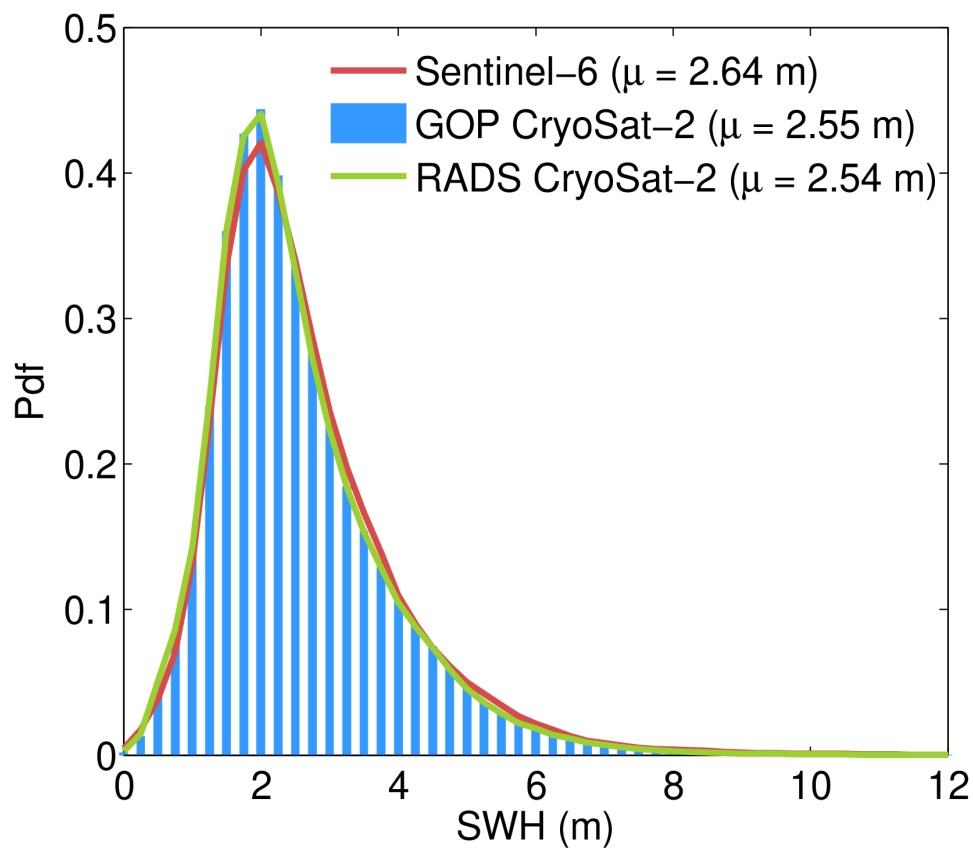
Figure 128. Histograms (normalized to have a total area of 1) of the SWH from GOP (blue bars), reference mission (red line) and RADS CryoSat-2 (green) for December 2023.
