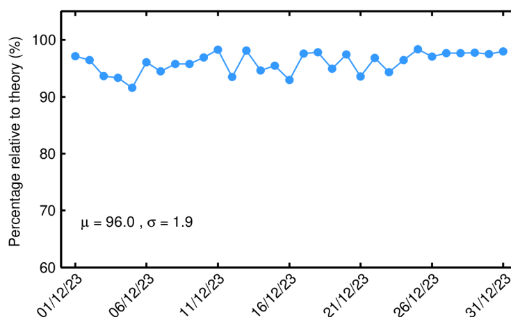
Figure 84. Percentage of science-valid GOP 1-Hz SWH records over ocean and lakes relative to theory for each day in December 2023. The mean ( \mu ) and standard deviation ( \sigma ) are also shown.
