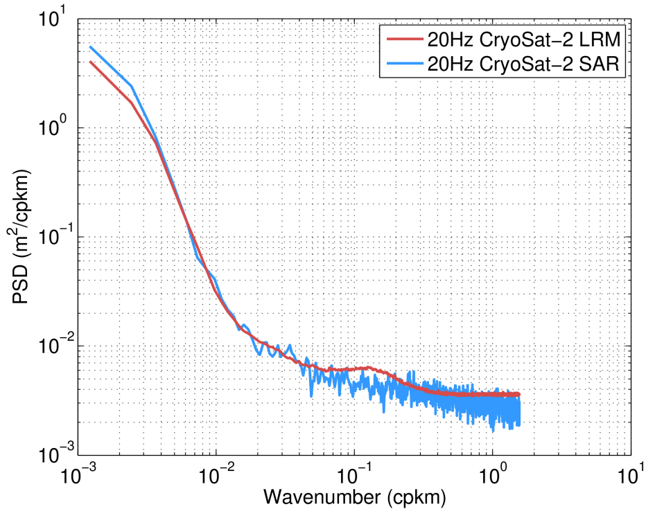
Figure 76. Along-track power spectrum density of the science-valid 20 Hz GOP SSH anomaly over oceans and lakes for LRM (red) and SAR (blue) for December 2023.
