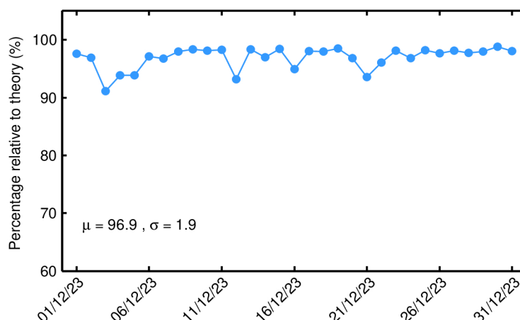
Figure 28. Percentage of science-valid NOP 1-Hz wind records over ocean and lakes relative to theory for each day in December 2023. The mean ( \mu ) and standard deviation ( \sigma ) are also shown.
