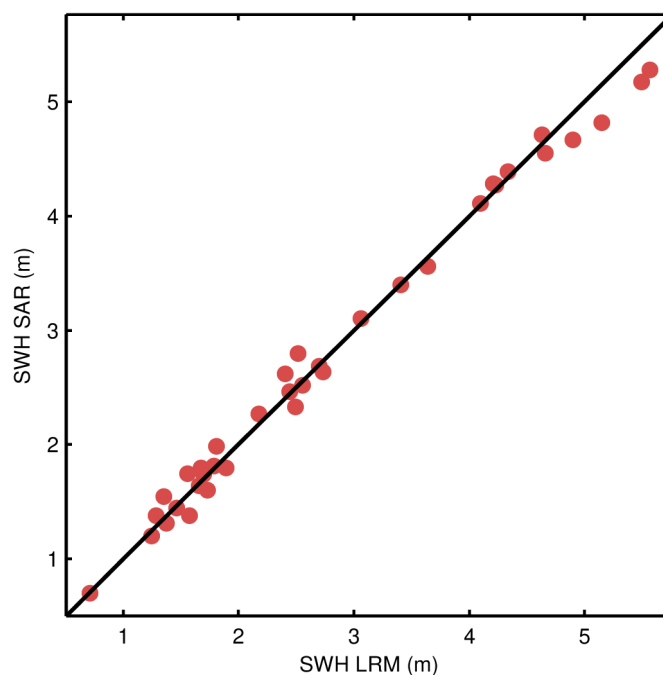
Figure 90. Scatter plot of the science-valid GOP SWH at the two nearest points outside (LRM, x-axis) and inside (SAR, y-axis) the Pacific SAR mode box for each pass. The RMS of the differences is 14.5 cm for the pairs shown in the figure as compared to a RMS of 18.2 cm for the differences between such outside points and their respective nearest neighbour also outside the box in the LRM region.
