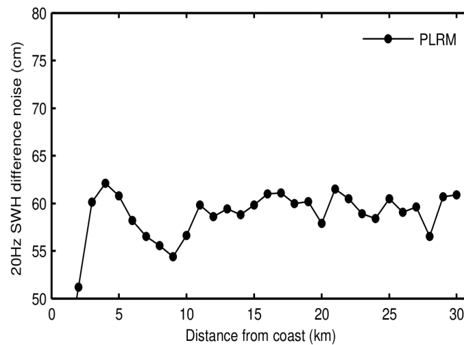
Figure 20. Science-valid NOP 20-Hz SWH noise as a function of distance from the coast for SAR (top panel), LRM (middle panel), and PLRM (bottom panel) for December 2023. Noise values have been calculated as the median of the absolute value of the difference between consecutive 20-Hz records.
