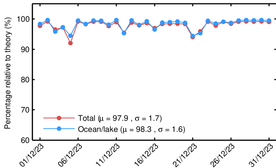
Figure 37. Percentage of IOP 1-Hz records over land and ocean/lake (red) and only over ocean/lake (blue) relative to the theoretically expected number from the orbits ground tracks for each day in December 2023.
