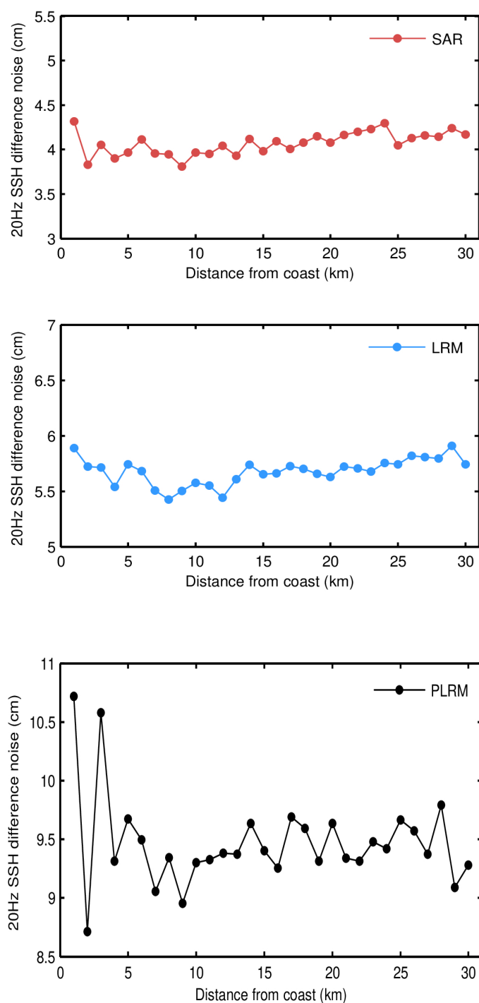
Figure 44. Science-valid IOP 20-Hz SSH anomaly noise as a function of distance from the coast for SAR (top panel), LRM (middle panel), and PLRM (bottom panel) for December 2023. Noise values have been calculated as the median of the absolute value of the difference between consecutive 20-Hz records.
