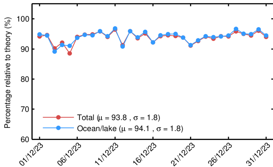
Figure 3. Percentage of NOP 1-Hz records over land and ocean/lake (red) and only over ocean/lake (blue) relative to the theoretically expected number from the orbits ground tracks for each day in December 2023.
