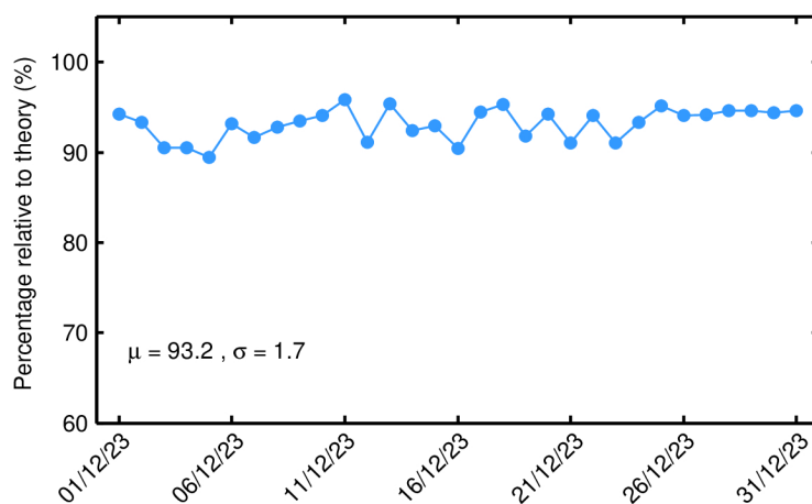
Figure 91. Percentage of science-valid GOP 1-Hz sigma0 records over ocean and lakes relative to theory for each day in December 2023. The mean ( \mu ) and standard deviation ( \sigma ) are also shown.
