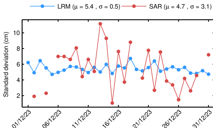
Figure 83. Standard deviation of differences at crossovers for GOP SSH anomaly for each day in December 2023. The values shown in this figure have been computed for the science-valid data further edited according to the following two additional criteria: 1) rejecting crossover differences larger than 20 cm; and 2) rejecting shallow waters (1000 m). The mean ( \mu ) and standard deviation ( \sigma ) are also shown.
