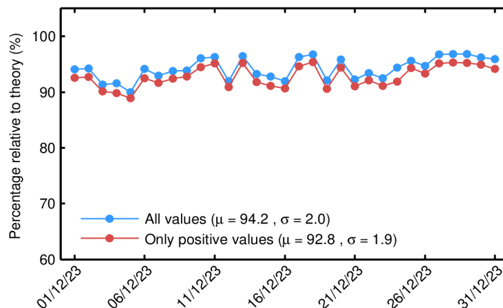
Figure 101. Percentage of science-valid GOP 1-Hz mispointing records over ocean and lakes relative to theory for each day in December 2023. The mean ( \mu ) and standard deviation ( \sigma ) are also shown.
