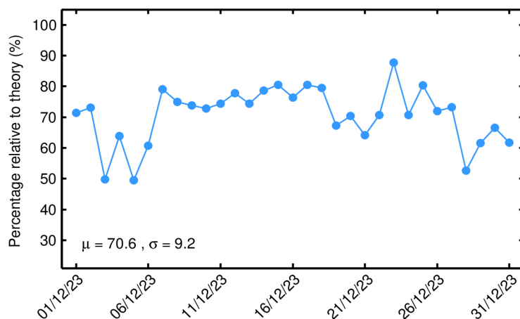
Figure 5. Percentage of science-valid NOP 1-Hz SSH records over ocean and lakes relative to theory for each day in December 2023. The mean ( \mu ) and standard deviation ( \sigma ) are also shown.
