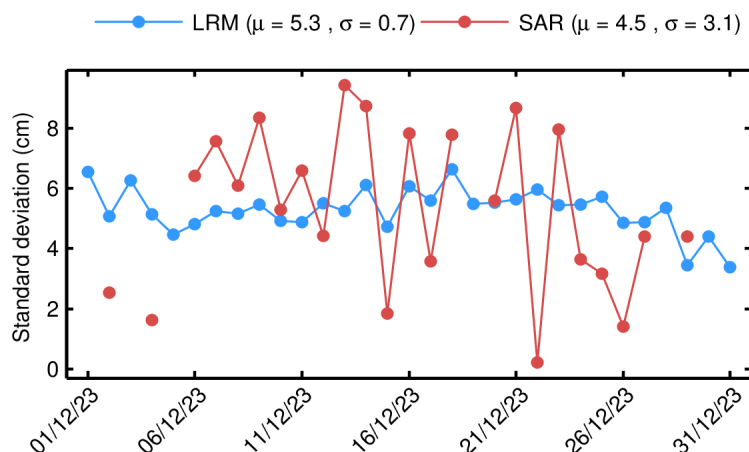
Figure 48. Standard deviation of differences at crossovers for IOP SSH anomaly for each day in December 2023. The values shown in this figure have been computed for the science-valid data further edited according to the following two additional criteria: 1) rejecting crossover differences larger than 20 cm; and 2) rejecting shallow waters (1000 m). The mean ( \mu ) and standard deviation ( \sigma ) are also shown.
