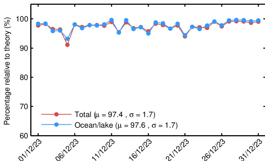
Figure 71. Percentage of GOP 1-Hz records over land and ocean/lake (red) and only over ocean/lake (blue) relative to the theoretically expected number from the orbits ground tracks for each day in December 2023.
