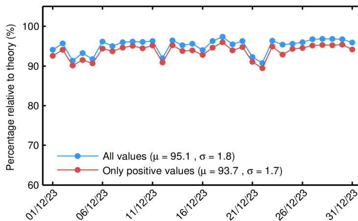
Figure 66. Percentage of science-valid IOP 1-Hz mispointing records over ocean and lakes relative to theory for each day in December 2023. The mean ( \mu ) and standard deviation ( \sigma ) are also shown.
