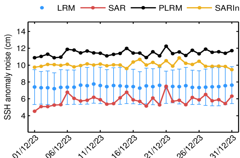
Figure 43. Mean science-valid IOP SSH anomaly noise for LRM (blue dot), SAR (red dot), PLRM (black dot) and SARIn (orange dot) for each day in December 2023. The corresponding standard deviation for LRM (blue error bar) is also shown.
