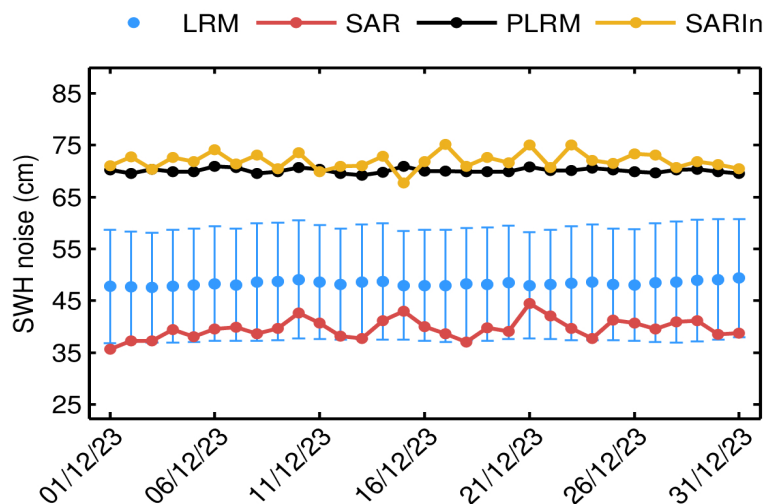
Figure 19. Mean science-valid NOP SWH noise for LRM (blue dot), SAR (red dot), PLRM (black dot) and SARIn (orange dot) for each day in December 2023. The corresponding standard deviation for LRM (blue error bar) is also shown.
