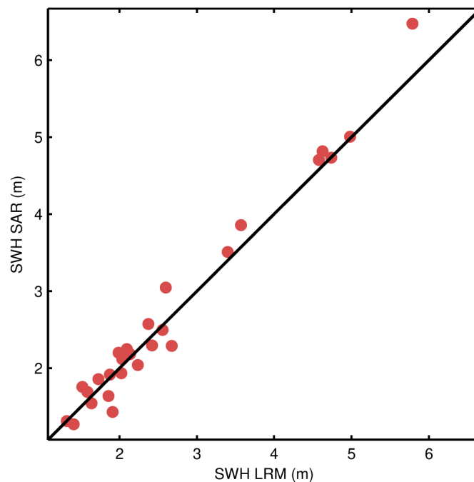
Figure 21. Scatter plot of the science-valid NOP SWH at the two nearest points outside (LRM, x-axis) and inside (SAR, y-axis) the Pacific SAR mode box for each pass. The RMS of the differences is 23.9 cm for the pairs shown in the figure as compared to a RMS of 14.1 cm for the differences between such outside points and their respective nearest neighbour also outside the box in the LRM region.
