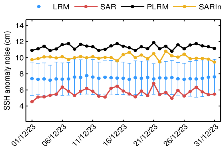
Figure 9. Mean science-valid NOP SSH anomaly noise for LRM (blue dot), SAR (red dot), PLRM (black dot) and SARIn (orange dot) for each day in December 2023. The corresponding standard deviation for LRM (blue error bar) is also shown.
