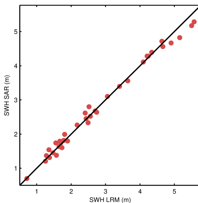
Figure 55. Scatter plot of the science-valid IOP SWH at the two nearest points outside (LRM, x-axis) and inside (SAR, y-axis) the Pacific SAR mode box for each pass. The RMS of the differences is 14.5 cm for the pairs shown in the figure as compared to a RMS of 18.2 cm for the differences between such outside points and their respective nearest neighbour also outside the box in the LRM region.
