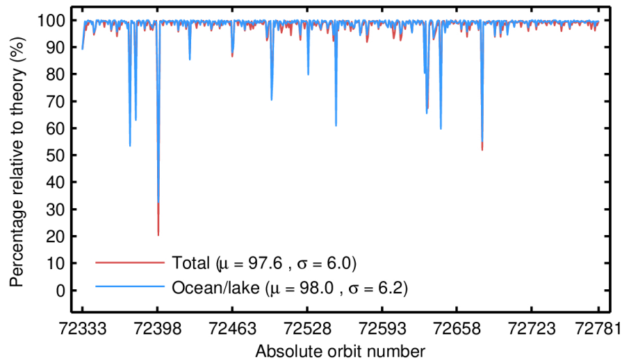
Figure 38. Percentage of IOP 1-Hz records over land and ocean/lake (red) and only over ocean/lake (blue) relative to the theoretically expected number from the orbits ground tracks for each orbit in December 2023. The mean ( \mu ) and standard deviation ( \sigma ) are also shown.
