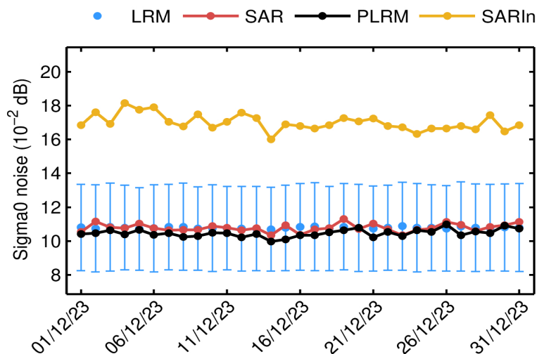
Figure 95. Mean science-valid GOP sigma0 noise for LRM (blue dot), SAR (red dot), PLRM (black dot) and SARIn (orange dot) for each day in December 2023. The corresponding standard deviation for LRM (blue error bar) is also shown.
