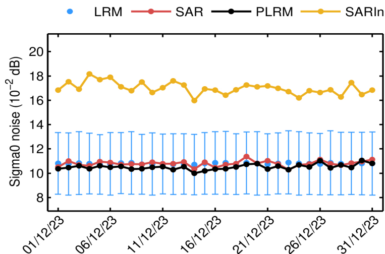
Figure 26. Mean science-valid NOP sigma0 noise for LRM (blue dot), SAR (red dot), PLRM (black dot) and SARIn (orange dot) for each day in December 2023. The corresponding standard deviation for LRM (blue error bar) is also shown.
