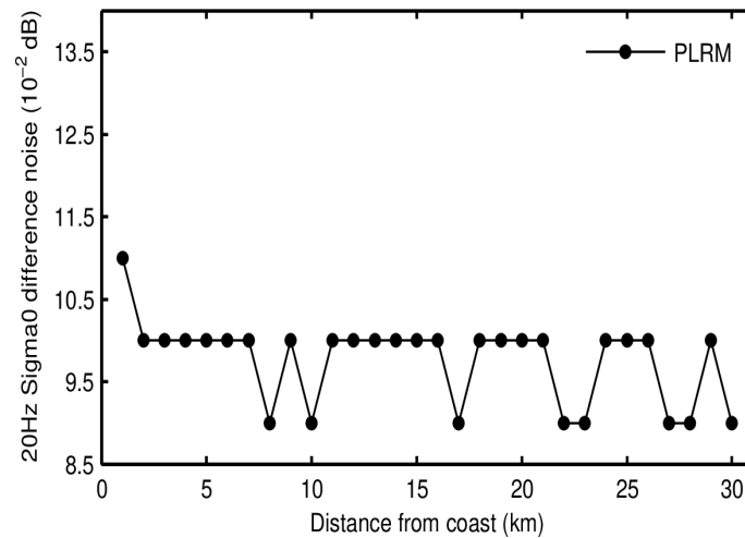
Figure 27. Science-valid NOP 20-Hz sigma0 noise as a function of distance from the coast for SAR (top panel), LRM (middle panel), and PLRM (bottom panel) for December 2023. Noise values have been calculated as the median of the absolute value of the difference between consecutive 20-Hz records.
