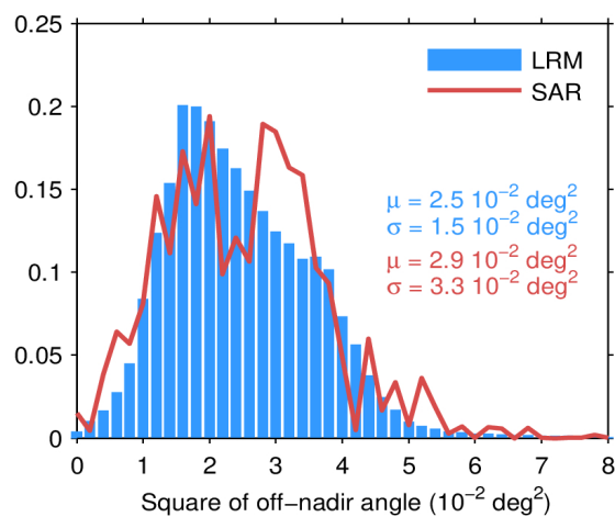
Figure 103. Histogram of science-valid GOP mispointing over oceans and lakes for LRM (blue) and SAR (red) for December 2023. The mean ( \mu ) and standard deviation ( \sigma ) are also shown. Note that values larger than 12 m are excluded from the histogram for the sake of readability but not from the computation of \mu and \sigma .
