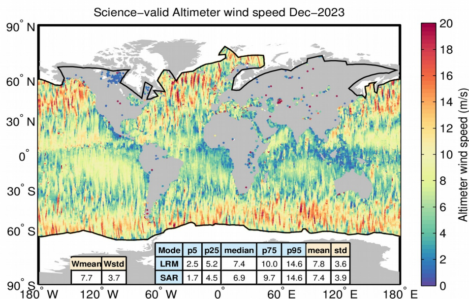
Figure 29. Geographical distribution of science-valid NOP wind data over oceans and lakes for December 2023. The statistical values shown in the table refer to the wind in m and are calculated separately for LRM and SAR regions. Wmean and Wstd denote the spatial area-weighted average and its standard deviation. Measurements taken over polar polygons have been excluded from the computation of the statistical values. The black lines mark the outer limit of the Arctic and Antarctic polar polygons.
