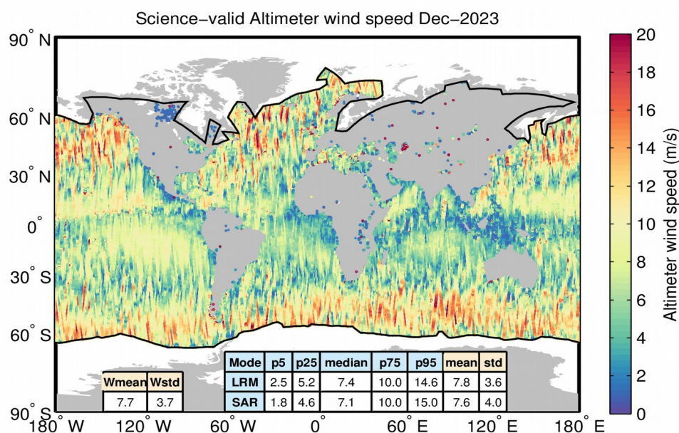
Figure 63. Geographical distribution of science-valid IOP wind data over oceans and lakes for December 2023. The statistical values shown in the table refer to the wind in m and are calculated separately for LRM and SAR regions. Wmean and Wstd denote the spatial area-weighted average and its standard deviation. Measurements taken over polar polygons have been excluded from the computation of the statistical values. The black lines mark the outer limit of the Arctic and Antarctic polar polygons.
