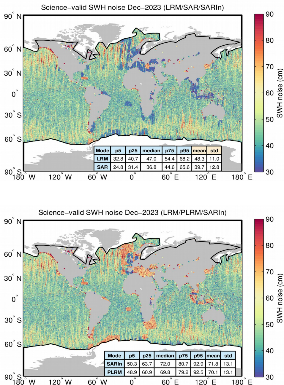
Figure 18. Geographical distribution of flag-valid 20-Hz SWH measurement noise over oceans and lakes for LRM/SAR/SARIn (top) and LRM/PLRM/SARIn (bottom) and for December 2023. The statistical values shown in the table refer to the SWH noise and are calculated separately for LRM, SAR/PLRM and SARIn regions. Measurements taken over polar polygons have been excluded from the computation of the statistical values. The black lines mark the outer limit of the Arctic and Antarctic polar polygons.
