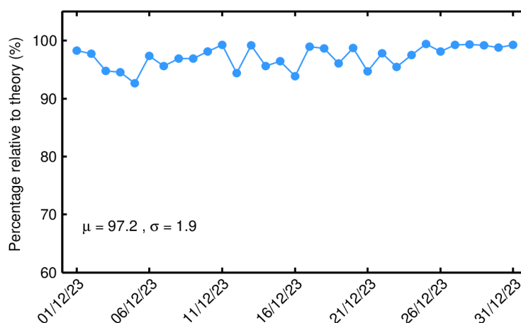
Figure 97. Percentage of science-valid GOP 1-Hz wind records over ocean and lakes relative to theory for each day in December 2023. The mean ( \mu ) and standard deviation ( \sigma ) are also shown.
