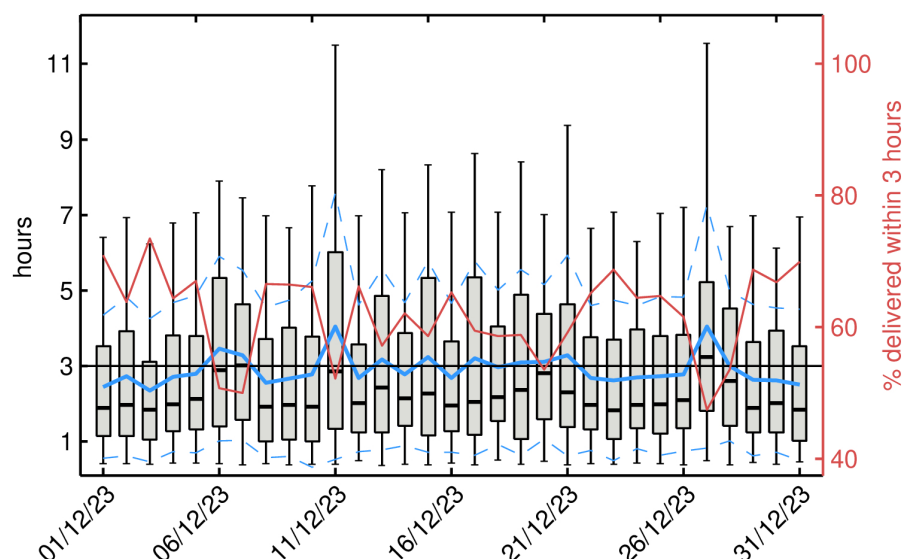
Figure 1. Box-and-whiskers plot for the NOP latency showing for each day in December 2023 the first and third quartiles (bottom and top of the box), the median (thick black), the
