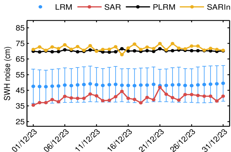
Figure 88. Mean science-valid GOP SWH noise for LRM (blue dot), SAR (red dot), PLRM (black dot) and SARIn (orange dot) for each day in December 2023. The corresponding standard deviation for LRM (blue error bar) is also shown.
