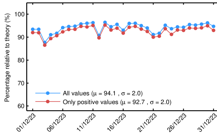
Figure 32. Percentage of science-valid NOP 1-Hz mispointing records over ocean and lakes relative to theory for each day in December 2023. The mean ( \mu ) and standard deviation ( \sigma ) are also shown.
