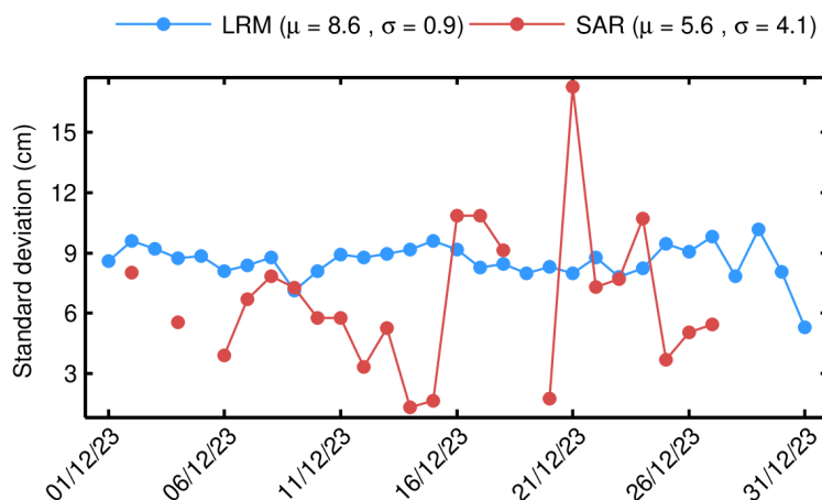
Figure 14. Standard deviation of differences at crossovers for NOP SSH anomaly for each day in December 2023. The values shown in this figure have been computed for the science-valid data further edited according to the following two additional criteria: 1) rejecting crossover differences larger than 20 cm; and 2) rejecting shallow waters (1000 m). The mean ( \mu ) and standard deviation ( \sigma ) are also shown.
