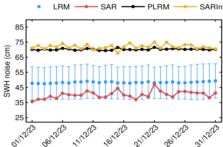
Figure 53. Mean science-valid IOP SWH noise for LRM (blue dot), SAR (red dot), PLRM (black dot) and SARIn (orange dot) for each day in December 2023. The corresponding standard deviation for LRM (blue error bar) is also shown.
