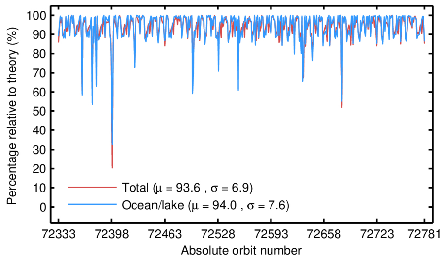
Figure 4. Percentage of NOP 1-Hz records over land and ocean/lake (red) and only over ocean/lake (blue) relative to the theoretically expected number from the orbits ground tracks for each orbit in December 2023. The mean ( \mu ) and standard deviation ( \sigma ) are also shown.
