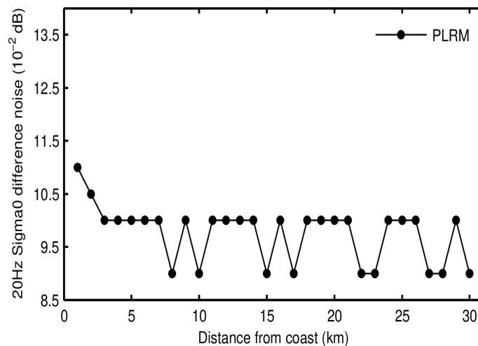
Figure 61. Science-valid IOP 20-Hz sigma0 noise as a function of distance from the coast for SAR (top panel), LRM (middle panel), and PLRM (bottom panel) for December 2023. Noise values have been calculated as the median of the absolute value of the difference between consecutive 20-Hz records.
