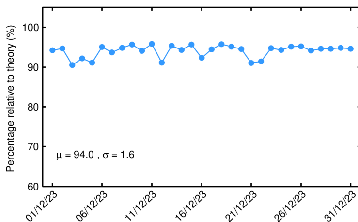
Figure 56. Percentage of science-valid IOP 1-Hz sigma0 records over ocean and lakes relative to theory for each day in December 2023. The mean ( \mu ) and standard deviation ( \sigma ) are also shown.
