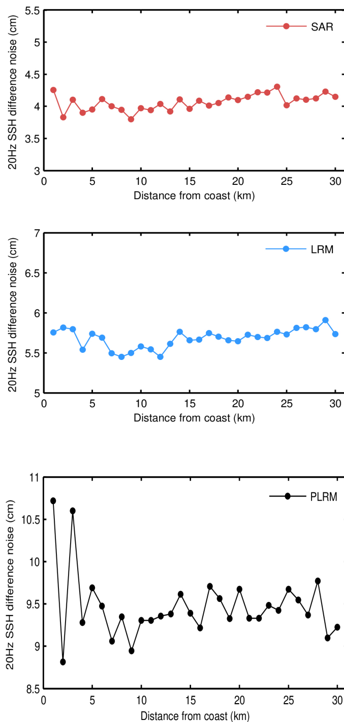
Figure 79. Science-valid GOP 20-Hz SSH anomaly noise as a function of distance from the coast for SAR (top panel), LRM (middle panel), and PLRM (bottom panel) for December 2023. Noise values have been calculated as the median of the absolute value of the difference between consecutive 20-Hz records.
