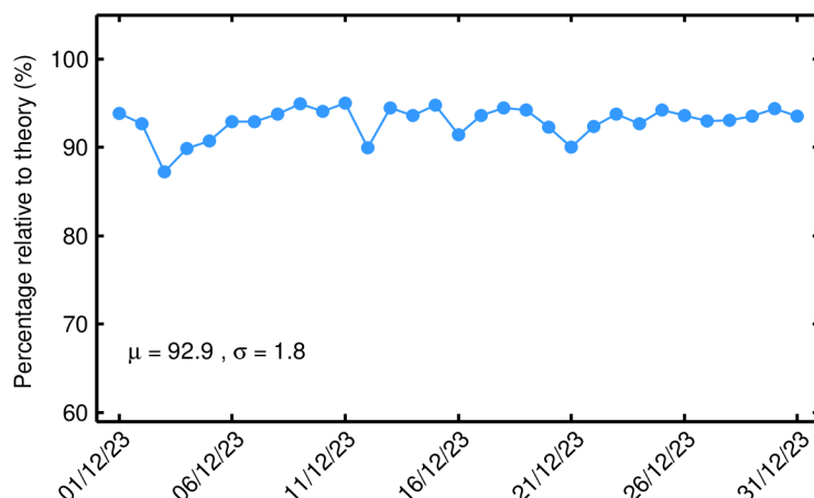
Figure 22. Percentage of science-valid NOP 1-Hz sigma0 records over ocean and lakes relative to theory for each day in December 2023. The mean ( \mu ) and standard deviation ( \sigma ) are also shown.
