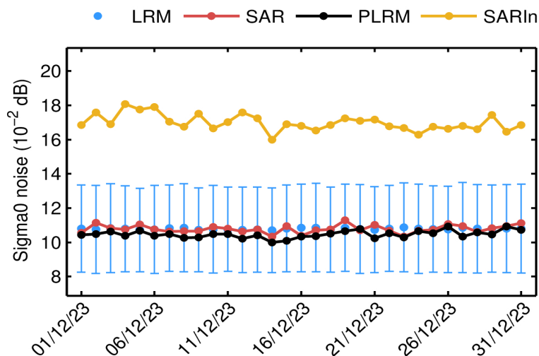
Figure 60. Mean science-valid IOP sigma0 noise for LRM (blue dot), SAR (red dot), PLRM (black dot) and SARIn (orange dot) for each day in December 2023. The corresponding standard deviation for LRM (blue error bar) is also shown.
