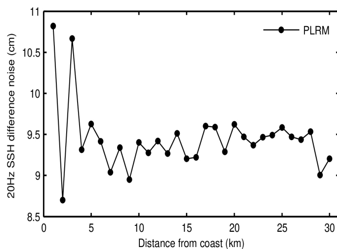
Figure 10. Science-valid NOP 20-Hz SSH anomaly noise as a function of distance from the coast for SAR (top panel), LRM (middle panel), and PLRM (bottom panel) for December 2023. Noise values have been calculated as the median of the absolute value of the difference between consecutive 20-Hz records.
