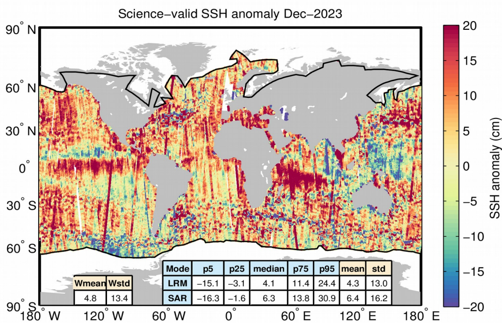
Figure 6. Geographical distribution of science-valid NOP 1-Hz SSH anomaly data over oceans and lakes for December 2023. The statistical values shown in the table refer to the SSH anomaly in cm and are calculated separately for LRM and SAR regions. Wmean and Wstd denote the spatial area-weighted average and its standard deviation. Measurements taken over polar polygons have been excluded from the computation of the statistical values. The black lines mark the outer limit of the Arctic and Antarctic polar polygons.
