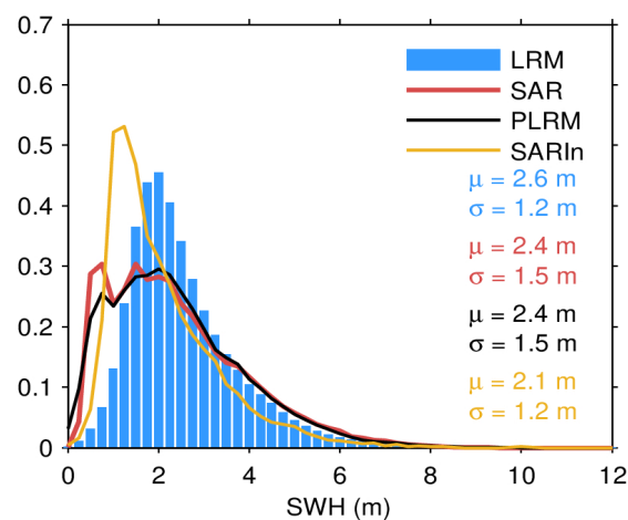
Figure 51. Histogram of science-valid IOP SWH over oceans and lakes for LRM (blue), SAR (red), PLRM (black) and SARIn (orange) for December 2023. The mean ( \mu ) and standard deviation ( \sigma ) are also shown. Values larger than 12 m are excluded from the histogram for the sake of readability but not from the computation of \mu and \sigma .
