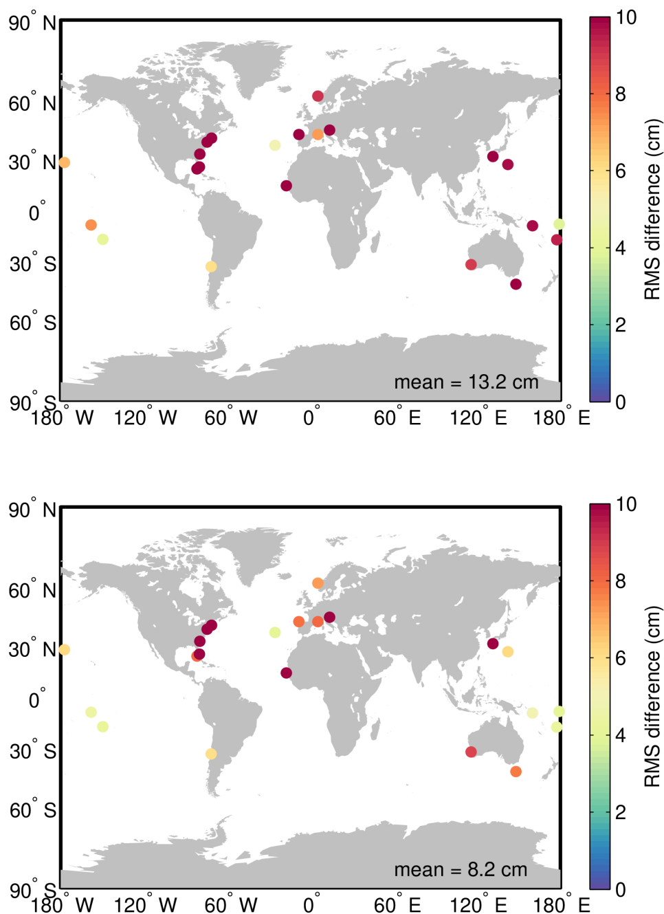
Figure 107. Map showing the RMS difference between the GOP SSH anomaly and the sea level from tide gauge records over the period January 2022 to December 2023 for the cases with (top) and without (bottom) the tidal component. For this comparison the atmospheric component has not been subtracted.
