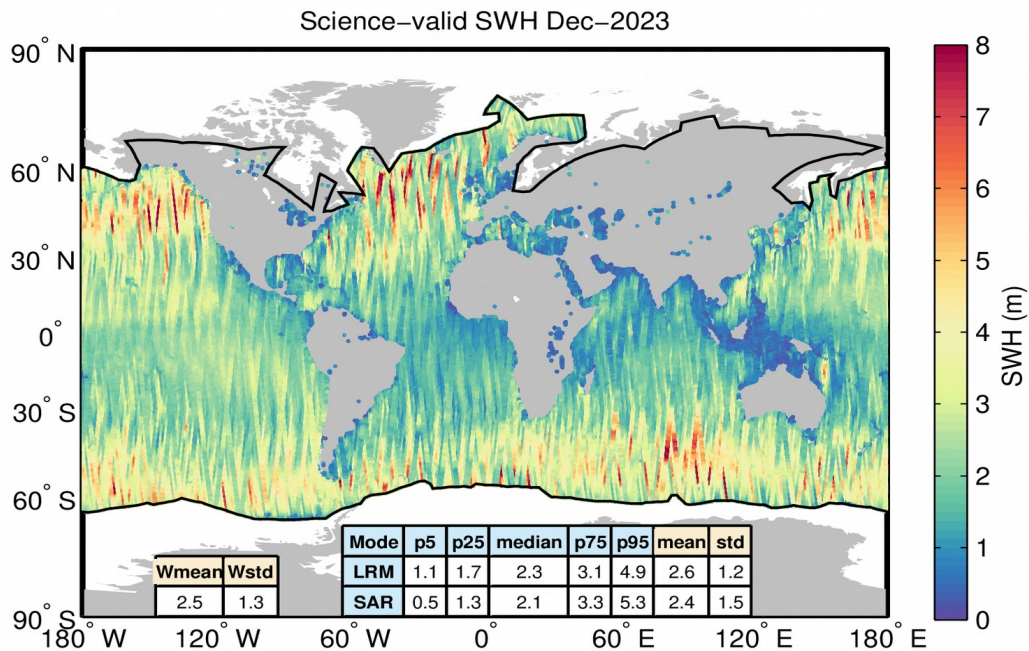
Figure 50. Geographical distribution of science-valid IOP SWH data over oceans and lakes for December 2023. The statistical values shown in the table refer to the SWH in m and are calculated separately for LRM and SAR regions. Wmean and Wstd denote the spatial area-weighted average and its standard deviation. Measurements taken over polar polygons have been excluded from the computation of the statistical values. The black lines mark the outer limit of the Arctic and Antarctic polar polygons.
