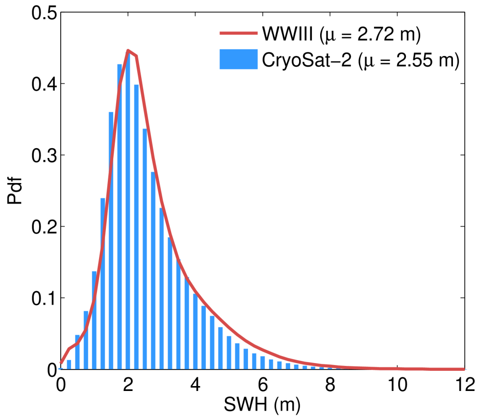
Figure 118. Histograms (normalized to have a total area of 1) of the GOP SWH (blue bars) and the SWH from the Wavewatch III model (red line) for December 2023.
