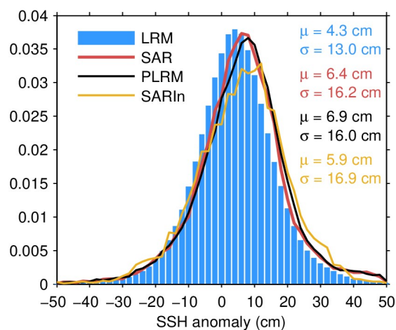
Figure 7. Histogram of science-valid NOP SSH anomaly over oceans and lakes for LRM (blue), SAR (red), PLRM (black) and SARIn (orange) for December 2023. The mean ( \mu ) and standard deviation ( \sigma ) are also shown. Values outside [-50 \ 50] cm are excluded from the histogram for the sake of readability but not from the computation of \mu and \sigma .
