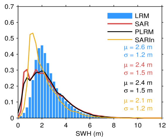
Figure 86. Histogram of science-valid GOP SWH over oceans and lakes for LRM (blue), SAR (red), PLRM (black) and SARIn (orange) and for December 2023. The mean ( \mu ) and standard deviation ( \sigma ) are also shown. Values larger than 12 m are excluded from the histogram for the sake of readability but not from the computation of \mu and \sigma .
