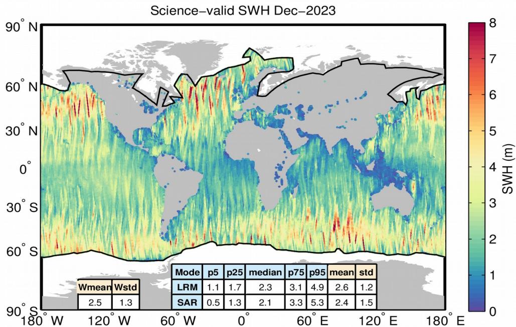
Figure 85. Geographical distribution of science-valid GOP SWH data over oceans and lakes for December 2023. The statistical values shown in the table refer to the SWH in m and are calculated separately for LRM and SAR regions. Wmean and Wstd denote the spatial area-weighted average and its standard deviation. Measurements taken over polar polygons have been excluded from the computation of the statistical values. The black lines mark the outer limit of the Arctic and Antarctic polar polygons.
