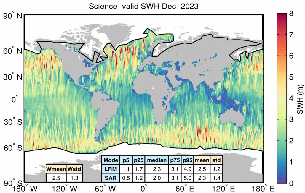
Figure 16. Geographical distribution of science-valid NOP SWH data over oceans and lakes for December 2023. The statistical values shown in the table refer to the SWH in m and are calculated separately for LRM and SAR regions. Wmean and Wstd denote the spatial area-weighted average and its standard deviation. Measurements taken over polar polygons have been excluded from the computation of the statistical values. The black lines mark the outer limit of the Arctic and Antarctic polar polygons.
