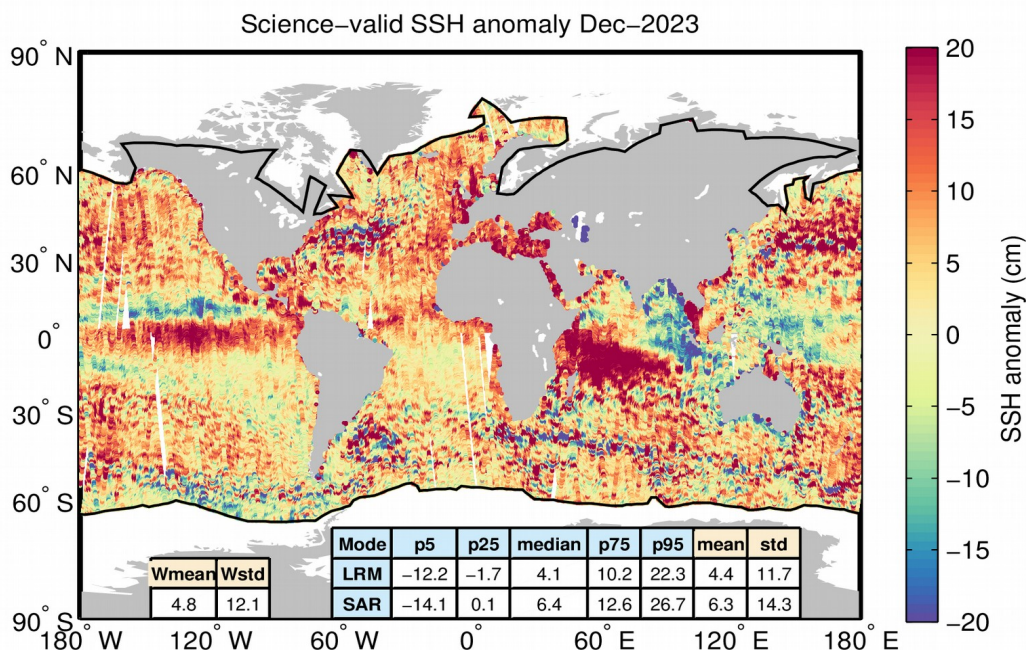
Figure 74. Geographical distribution of science-valid GOP 1-Hz SSH anomaly data over oceans and lakes for December 2023. The statistical values shown in the table refer to the SSH anomaly in cm and are calculated separately for LRM and SAR regions. Wmean and Wstd denote the spatial area-weighted average and its standard deviation. Measurements taken over polar polygons have been excluded from the computation of the statistical values. The black lines mark the outer limit of the Arctic and Antarctic polar polygons.
