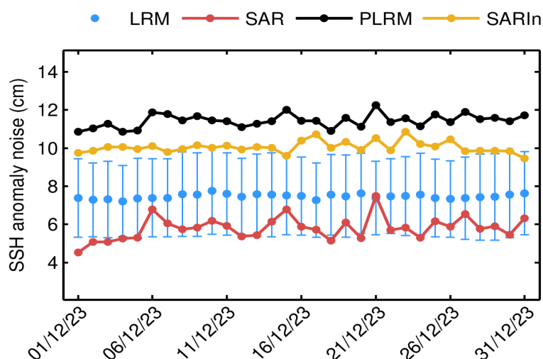
Figure 78. Mean science-valid GOP SSH anomaly noise for LRM (blue dot), SAR (red dot), PLRM (black dot) and SARIn (orange dot) for each day in December 2023. The corresponding standard deviation for LRM (blue error bar) is also shown.
