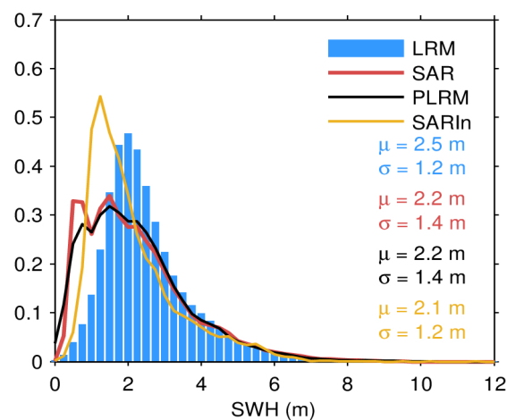
Figure 86. Histogram of science-valid GOP SWH over oceans and lakes for LRM (blue), SAR (red), PLRM (black) and SARIn (orange) and for November 2023. The mean ( \mu ) and standard deviation ( \sigma ) are also shown. Values larger than 12 m are excluded from the histogram for the sake of readability but not from the computation of \mu and \sigma .
