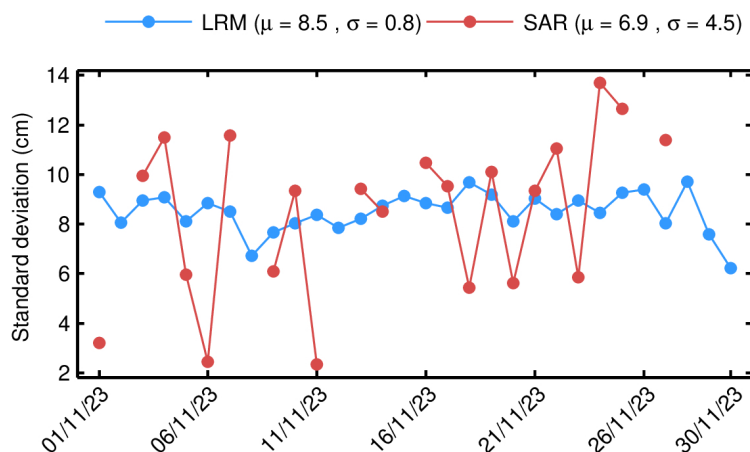
Figure 14. Standard deviation of differences at crossovers for NOP SSH anomaly for each day in November 2023. The values shown in this figure have been computed for the science-valid data further edited according to the following two additional criteria: 1) rejecting crossover differences larger than 20 cm; and 2) rejecting shallow waters (1000 m). The mean ( \mu ) and standard deviation ( \sigma ) are also shown.
