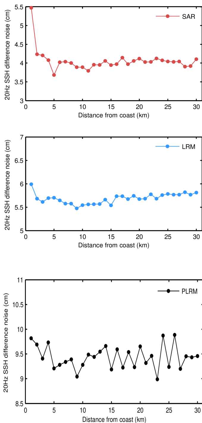
Figure 44. Science-valid IOP 20-Hz SSH anomaly noise as a function of distance from the coast for SAR (top panel), LRM (middle panel), and PLRM (bottom panel) for November 2023. Noise values have been calculated as the median of the absolute value of the difference between consecutive 20-Hz records.
