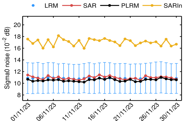
Figure 60. Mean science-valid IOP sigma0 noise for LRM (blue dot), SAR (red dot), PLRM (black dot) and SARIn (orange dot) for each day in November 2023. The corresponding standard deviation for LRM (blue error bar) is also shown.
