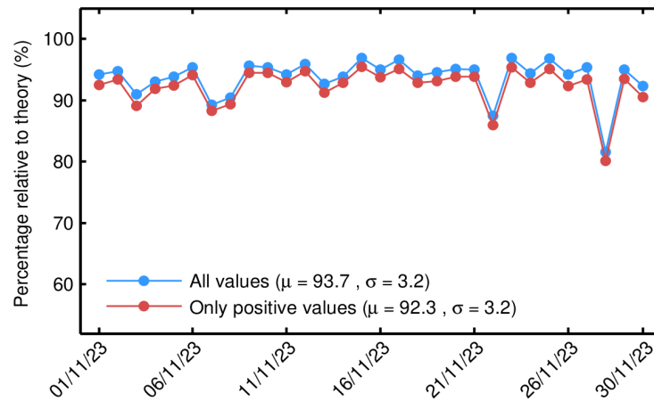
Figure 32. Percentage of science-valid NOP 1-Hz mispointing records over ocean and lakes relative to theory for each day in November 2023. The mean ( \mu ) and standard deviation ( \sigma ) are also shown.
