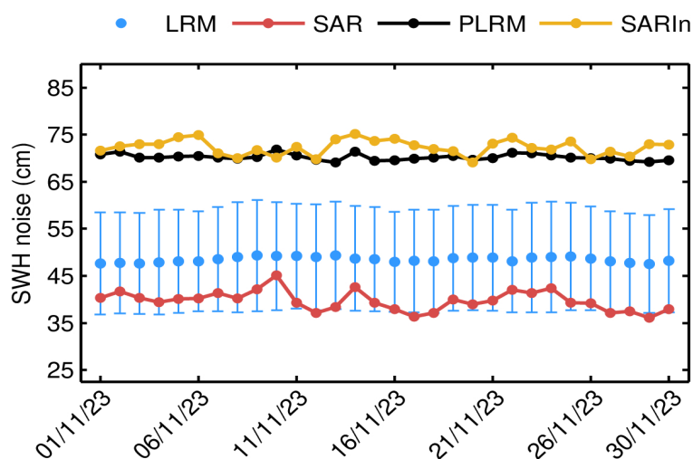
Figure 88. Mean science-valid GOP SWH noise for LRM (blue dot), SAR (red dot), PLRM (black dot) and SARIn (orange dot) for each day in November 2023. The corresponding standard deviation for LRM (blue error bar) is also shown.
