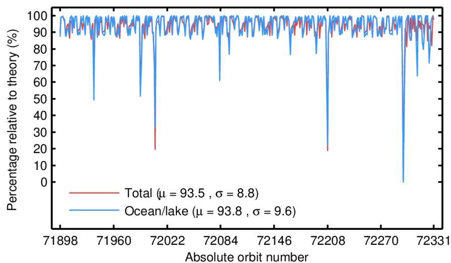
Figure 4. Percentage of NOP 1-Hz records over land and ocean/lake (red) and only over ocean/lake (blue) relative to the theoretically expected number from the orbits ground tracks for each orbit in November 2023. The mean ( \mu ) and standard deviation ( \sigma ) are also shown.
