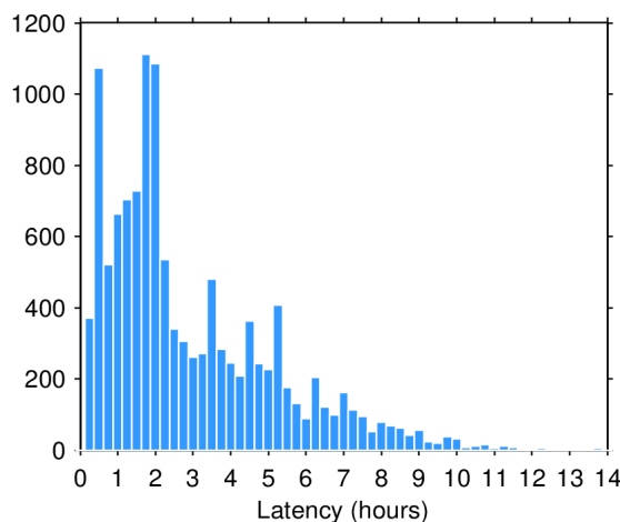
Figure 2. Histogram of the NOP data latency for November 2023. The y-axis denotes the number of files that are made available with a delay of x-hours with respect to the mean time of the records stored in the file.
