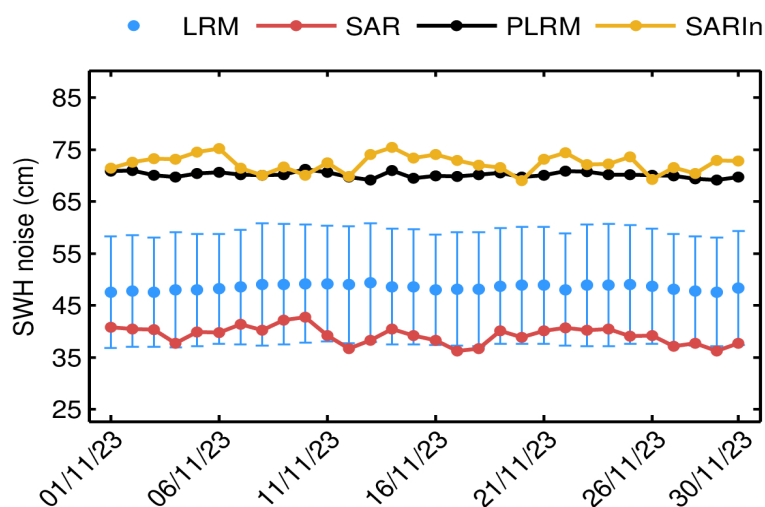
Figure 19. Mean science-valid NOP SWH noise for LRM (blue dot), SAR (red dot), PLRM (black dot) and SARIn (orange dot) for each day in November 2023. The corresponding standard deviation for LRM (blue error bar) is also shown.
