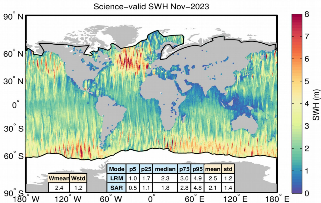
Figure 16. Geographical distribution of science-valid NOP SWH data over oceans and lakes for November 2023. The statistical values shown in the table refer to the SWH in m and are calculated separately for LRM and SAR regions. Wmean and Wstd denote the spatial area-weighted average and its standard deviation. Measurements taken over polar polygons have been excluded from the computation of the statistical values. The black lines mark the outer limit of the Arctic and Antarctic polar polygons.
