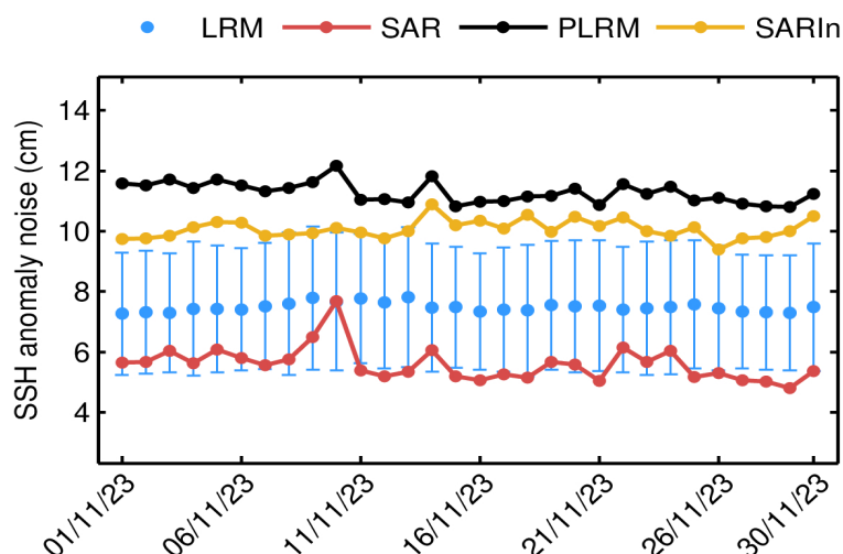
Figure 43. Mean science-valid IOP SSH anomaly noise for LRM (blue dot), SAR (red dot), PLRM (black dot) and SARIn (orange dot) for each day in November 2023. The corresponding standard deviation for LRM (blue error bar) is also shown.
