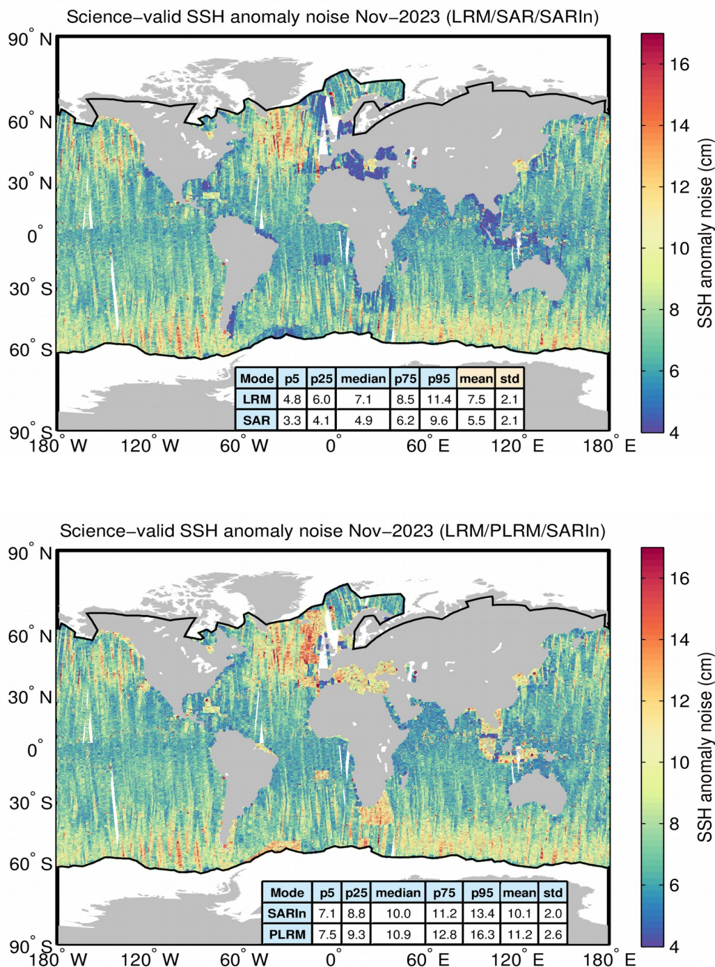
Figure 8. Geographical distribution of flag-valid 20-Hz SSH anomaly measurement noise over oceans and lakes for LRM/SAR/SARIn (top) and LRM/PLRM/SARIn (bottom) and for November 2023. The statistical values shown in the tables refer to the SSH anomaly noise and are calculated separately for LRM, SAR/PLRM, and SARIn regions. Measurements
