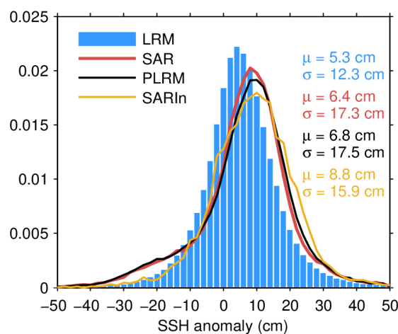
Figure 75. Histogram of science-valid GOP SSH anomaly over oceans and lakes for LRM (blue), SAR (red), PLRM (black) and SARIn (orange) for November 2023. The mean ( \mu )
