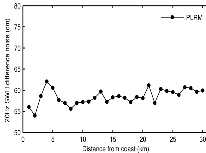
Figure 20. Science-valid NOP 20-Hz SWH noise as a function of distance from the coast for SAR (top panel), LRM (middle panel), and PLRM (bottom panel) for November 2023. Noise values have been calculated as the median of the absolute value of the difference between consecutive 20-Hz records.
