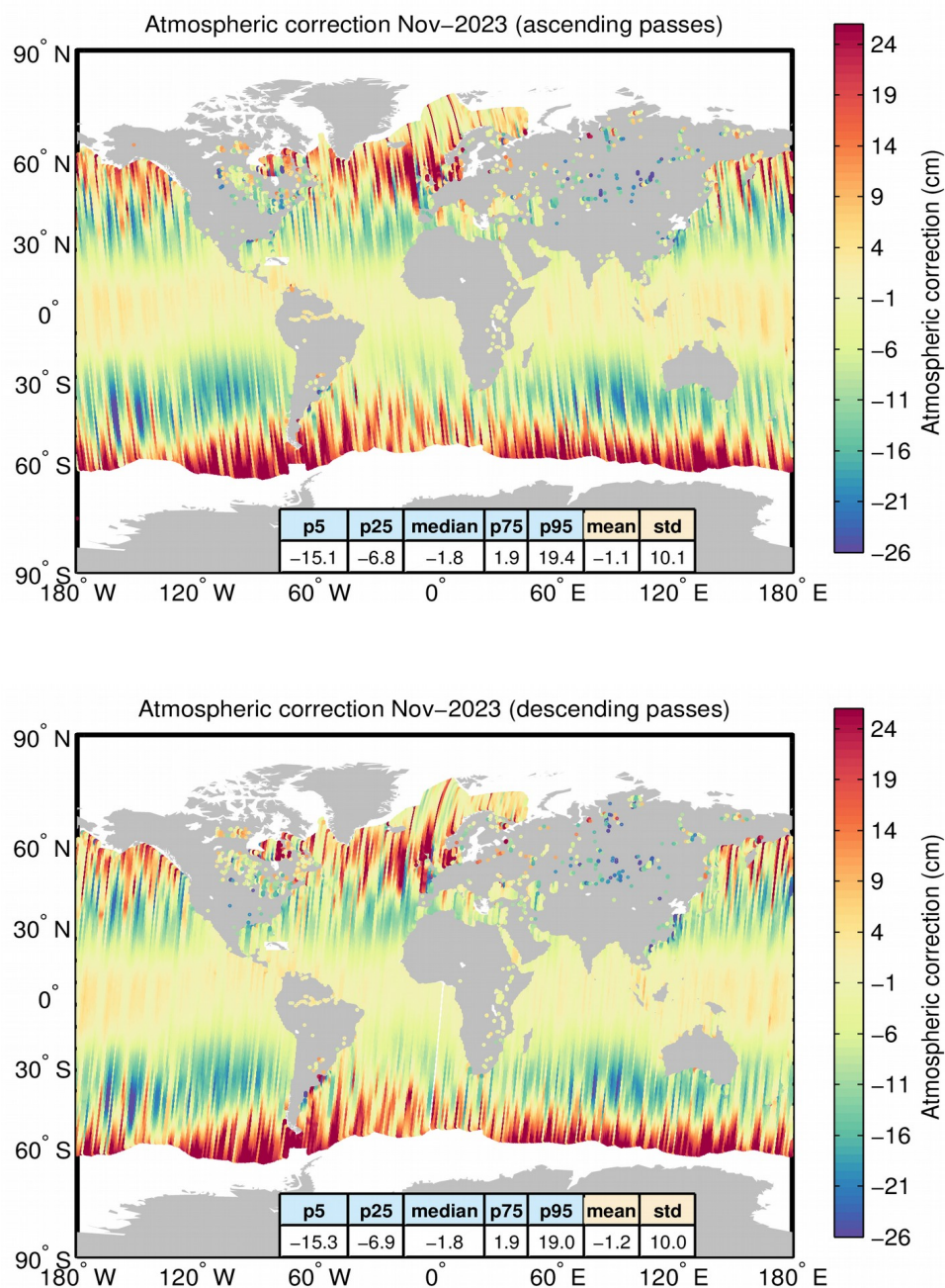
Figure A5. Geographical distribution of the atmospheric correction over oceans and lakes for ascending (top) and descending (bottom) passes for November 2023. The statistical values shown in the table refer to the atmospheric correction in cm. Measurements taken over polar polygons have been excluded from the computation of the statistical values. The black lines mark the outer limit of the Arctic and Antarctic polar polygons.
