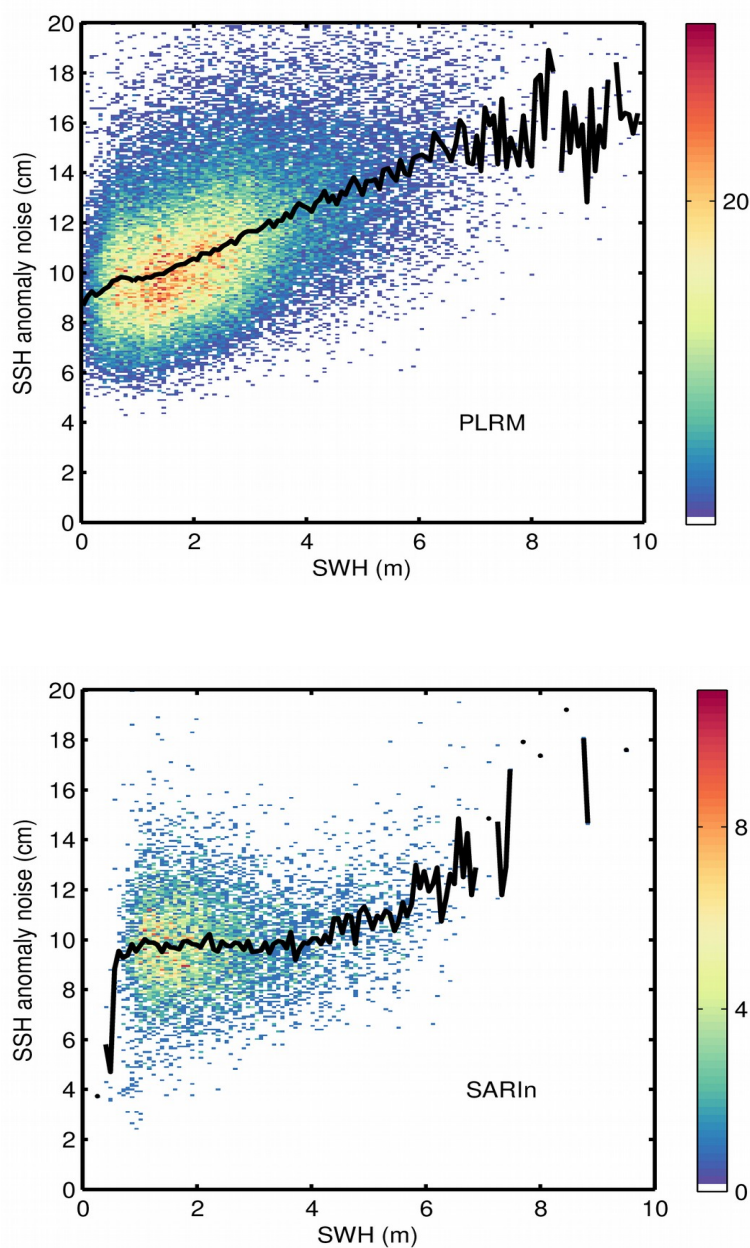
Figure 45. 2D histogram showing science-valid IOP SSH anomaly noise as a function of SWH for SAR, LRM, PLRM, and SARIn (from top to bottom) for November 2023. The black line denotes the median SSH anomaly noise as a function of SWH.
