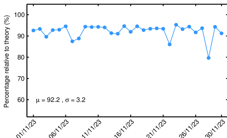
Figure 22. Percentage of science-valid NOP 1-Hz sigma0 records over ocean and lakes relative to theory for each day in November 2023. The mean ( \mu ) and standard deviation ( \sigma ) are also shown.
