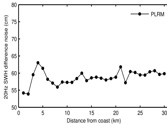
Figure 54. Science-valid IOP 20-Hz SWH noise as a function of distance from the coast for SAR (top panel), LRM (middle panel), and PLRM (bottom panel) for November 2023. Noise values have been calculated as the median of the absolute value of the difference between consecutive 20-Hz records.
