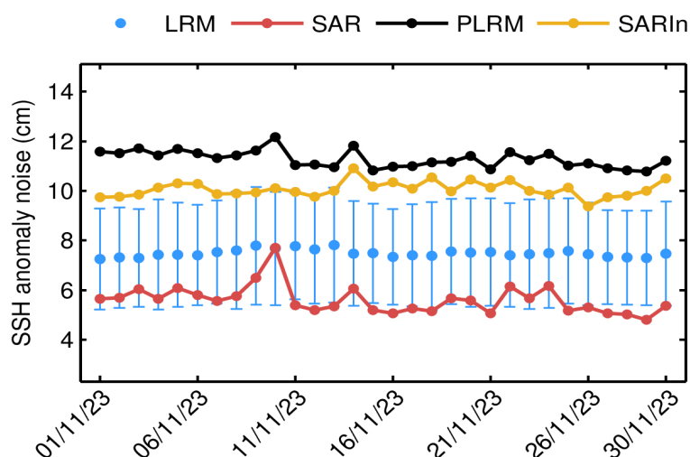
Figure 78. Mean science-valid GOP SSH anomaly noise for LRM (blue dot), SAR (red dot), PLRM (black dot) and SARIn (orange dot) for each day in November 2023. The corresponding standard deviation for LRM (blue error bar) is also shown.
