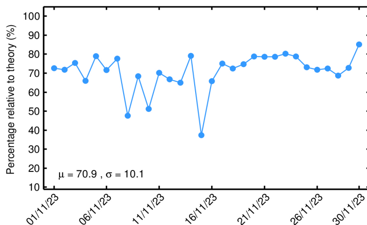
Figure 5. Percentage of science-valid NOP 1-Hz SSH records over ocean and lakes relative to theory for each day in November 2023. The mean ( \mu ) and standard deviation ( \sigma ) are also shown.
