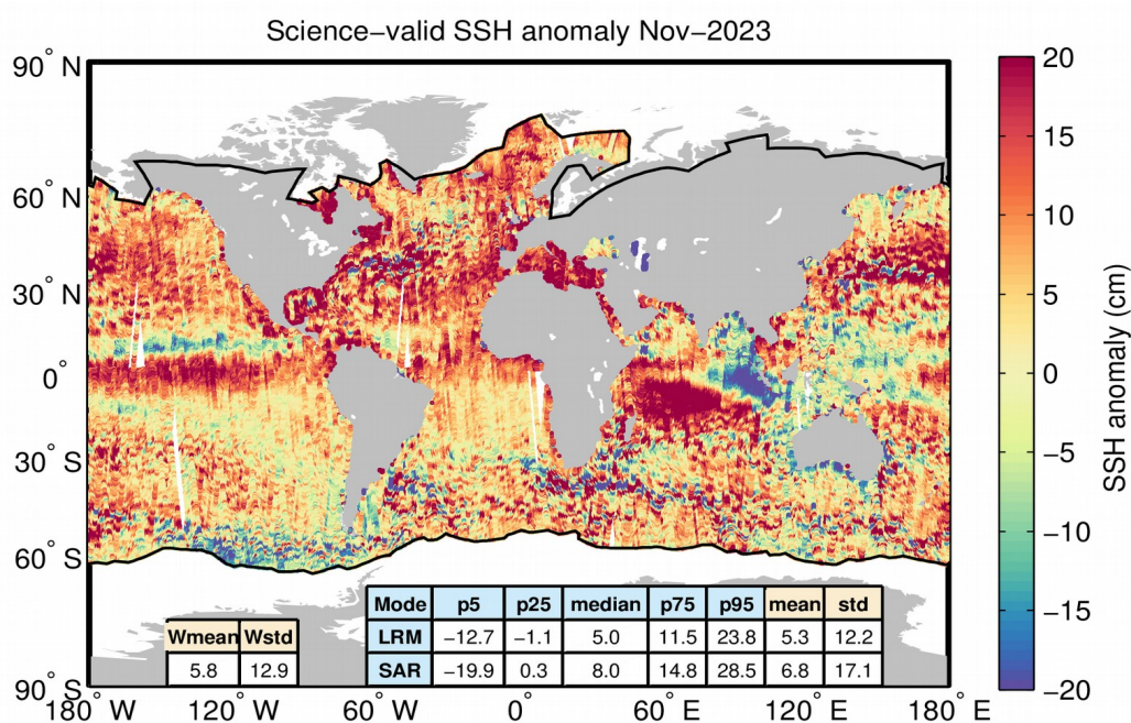
Figure 40. Geographical distribution of science-valid IOP 1-Hz SSH anomaly data over oceans and lakes for November 2023. The statistical values shown in the table refer to the SSH anomaly in cm and are calculated separately for LRM and SAR regions. Wmean and Wstd denote the spatial area-weighted average and its standard deviation. Measurements taken over polar polygons have been excluded from the computation of the statistical values. The black lines mark the outer limit of the Arctic and Antarctic polar polygons.
