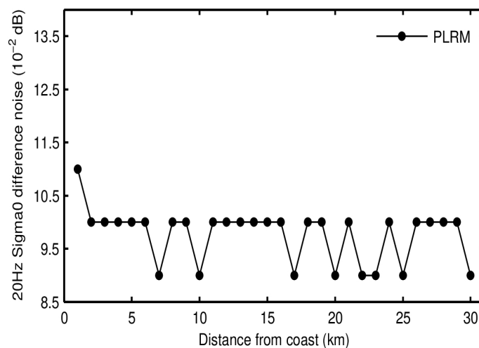
Figure 61. Science-valid IOP 20-Hz sigma0 noise as a function of distance from the coast for SAR (top panel), LRM (middle panel), and PLRM (bottom panel) for November 2023. Noise values have been calculated as the median of the absolute value of the difference between consecutive 20-Hz records.
