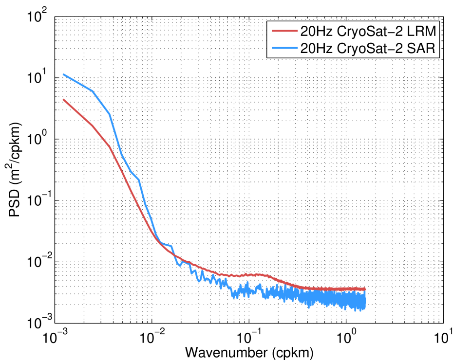
Figure 76. Along-track power spectrum density of the science-valid 20 Hz GOP SSH anomaly over oceans and lakes for LRM (red) and SAR (blue) for November 2023.
