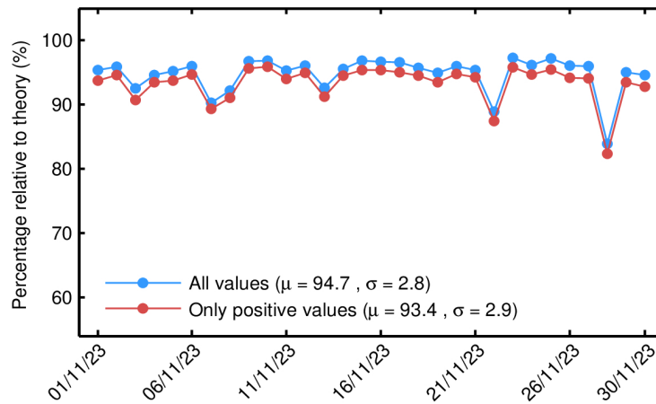
Figure 66. Percentage of science-valid IOP 1-Hz mispointing records over ocean and lakes relative to theory for each day in November 2023. The mean ( \mu ) and standard deviation ( \sigma ) are also shown.
