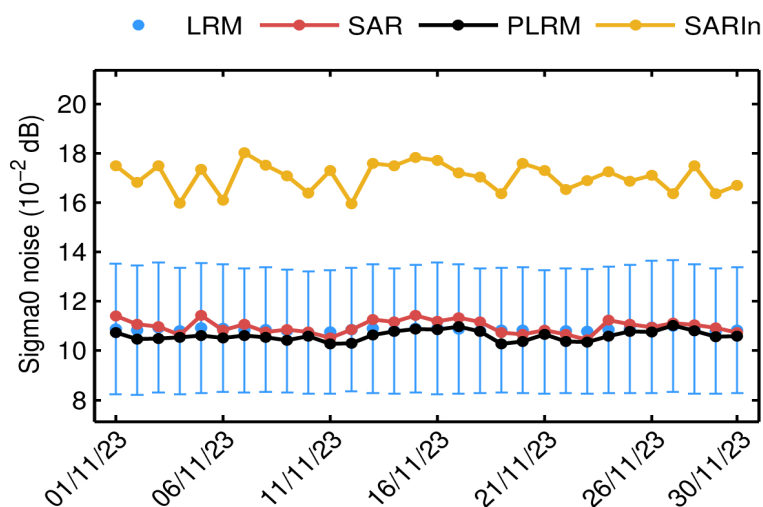
Figure 26. Mean science-valid NOP sigma0 noise for LRM (blue dot), SAR (red dot), PLRM (black dot) and SARIn (orange dot) for each day in November 2023. The corresponding standard deviation for LRM (blue error bar) is also shown.
