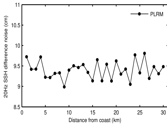
Figure 10. Science-valid NOP 20-Hz SSH anomaly noise as a function of distance from the coast for SAR (top panel), LRM (middle panel), and PLRM (bottom panel) for November 2023. Noise values have been calculated as the median of the absolute value of the difference between consecutive 20-Hz records.
