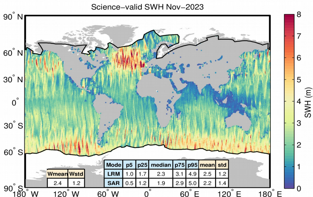
Figure 50. Geographical distribution of science-valid IOP SWH data over oceans and lakes for November 2023. The statistical values shown in the table refer to the SWH in m and are calculated separately for LRM and SAR regions. Wmean and Wstd denote the spatial area-weighted average and its standard deviation. Measurements taken over polar polygons have been excluded from the computation of the statistical values. The black lines mark the outer limit of the Arctic and Antarctic polar polygons.
