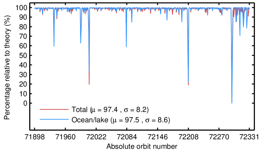
Figure 38. Percentage of IOP 1-Hz records over land and ocean/lake (red) and only over ocean/lake (blue) relative to the theoretically expected number from the orbits ground tracks for each orbit in November 2023. The mean ( \mu ) and standard deviation ( \sigma ) are also shown.
