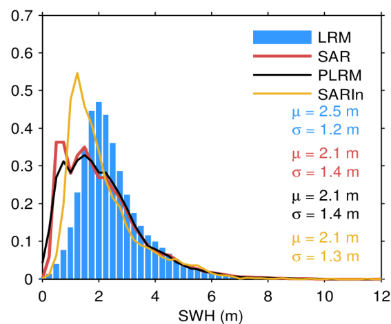
Figure 17. Histogram of science-valid NOP SWH over oceans and lakes for LRM (blue), SAR (red), PLRM (black) and SARIn (orange) for November 2023. The mean ( \mu ) and standard deviation ( \sigma ) are also shown. Values larger than 12 m are excluded from the histogram for the sake of readability but not from the computation of \mu and \sigma .
