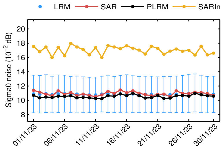
Figure 95. Mean science-valid GOP sigma0 noise for LRM (blue dot), SAR (red dot), PLRM (black dot) and SARIn (orange dot) for each day in November 2023. The corresponding standard deviation for LRM (blue error bar) is also shown.
