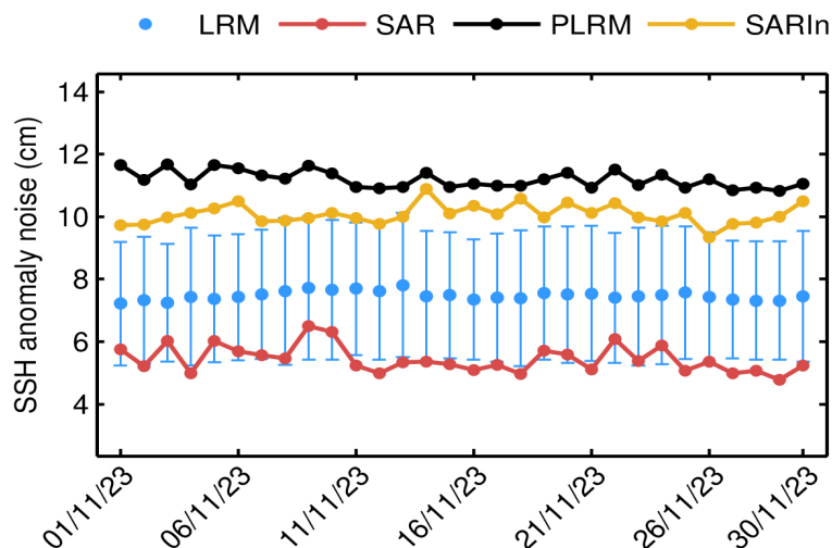
Figure 9. Mean science-valid NOP SSH anomaly noise for LRM (blue dot), SAR (red dot), PLRM (black dot) and SARIn (orange dot) for each day in November 2023. The corresponding standard deviation for LRM (blue error bar) is also shown.
