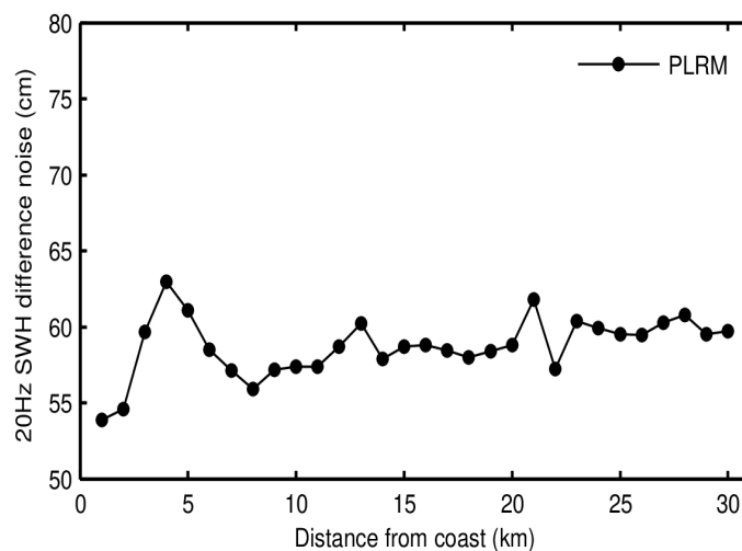
Figure 89. Science-valid GOP 20-Hz SWH noise as a function of distance from the coast for SAR (top panel), LRM (middle panel), and PLRM (bottom panel) for November 2023. Noise values have been calculated as the median of the absolute value of the difference between consecutive 20-Hz records.
