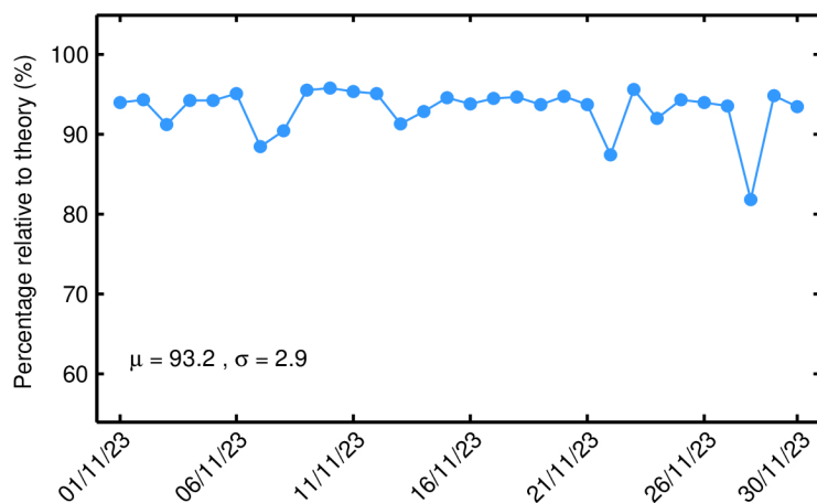
Figure 91. Percentage of science-valid GOP 1-Hz sigma0 records over ocean and lakes relative to theory for each day in November 2023. The mean ( \mu ) and standard deviation ( \sigma ) are also shown.
