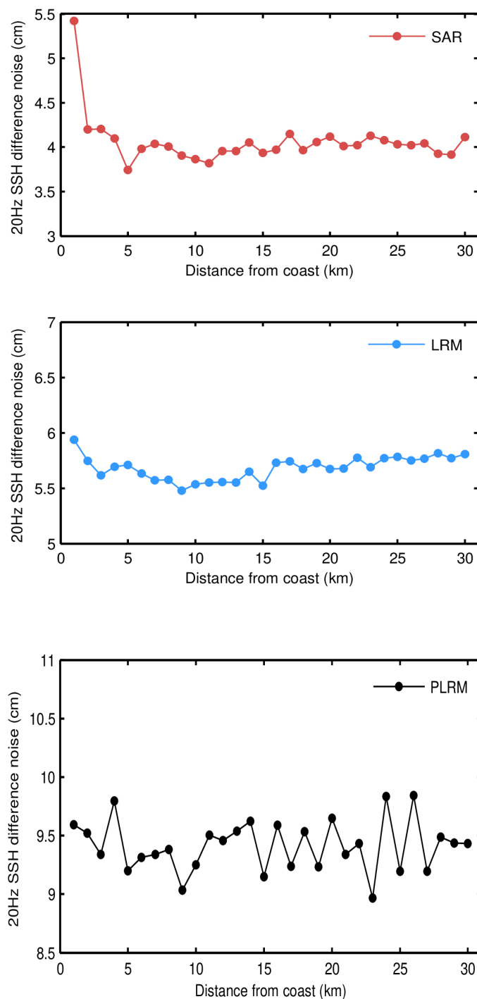
Figure 79. Science-valid GOP 20-Hz SSH anomaly noise as a function of distance from the coast for SAR (top panel), LRM (middle panel), and PLRM (bottom panel) for November 2023. Noise values have been calculated as the median of the absolute value of the difference between consecutive 20-Hz records.
