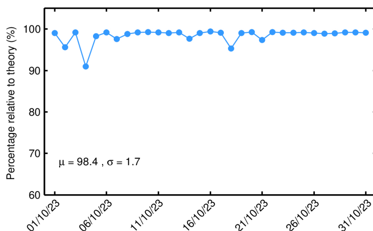
Figure 97. Percentage of science-valid GOP 1-Hz wind records over ocean and lakes relative to theory for each day in October 2023. The mean ( \mu ) and standard deviation ( \sigma ) are also shown.
