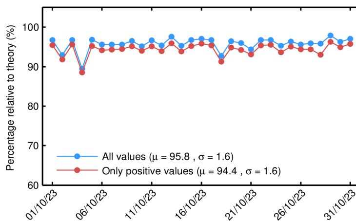
Figure 66. Percentage of science-valid IOP 1-Hz mispointing records over ocean and lakes relative to theory for each day in October 2023. The mean ( \mu ) and standard deviation ( \sigma ) are also shown.
