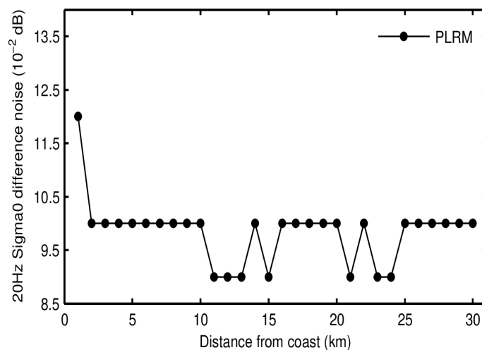
Figure 27. Science-valid NOP 20-Hz sigma0 noise as a function of distance from the coast for SAR (top panel), LRM (middle panel), and PLRM (bottom panel) for October 2023. Noise values have been calculated as the median of the absolute value of the difference between consecutive 20-Hz records.
