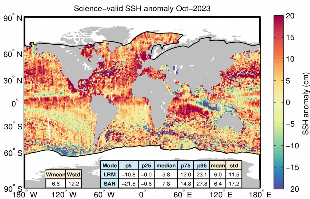
Figure 40. Geographical distribution of science-valid IOP 1-Hz SSH anomaly data over oceans and lakes for October 2023. The statistical values shown in the table refer to the SSH anomaly in cm and are calculated separately for LRM and SAR regions. Wmean and Wstd denote the spatial area-weighted average and its standard deviation. Measurements taken over polar polygons have been excluded from the computation of the statistical values. The black lines mark the outer limit of the Arctic and Antarctic polar polygons.
