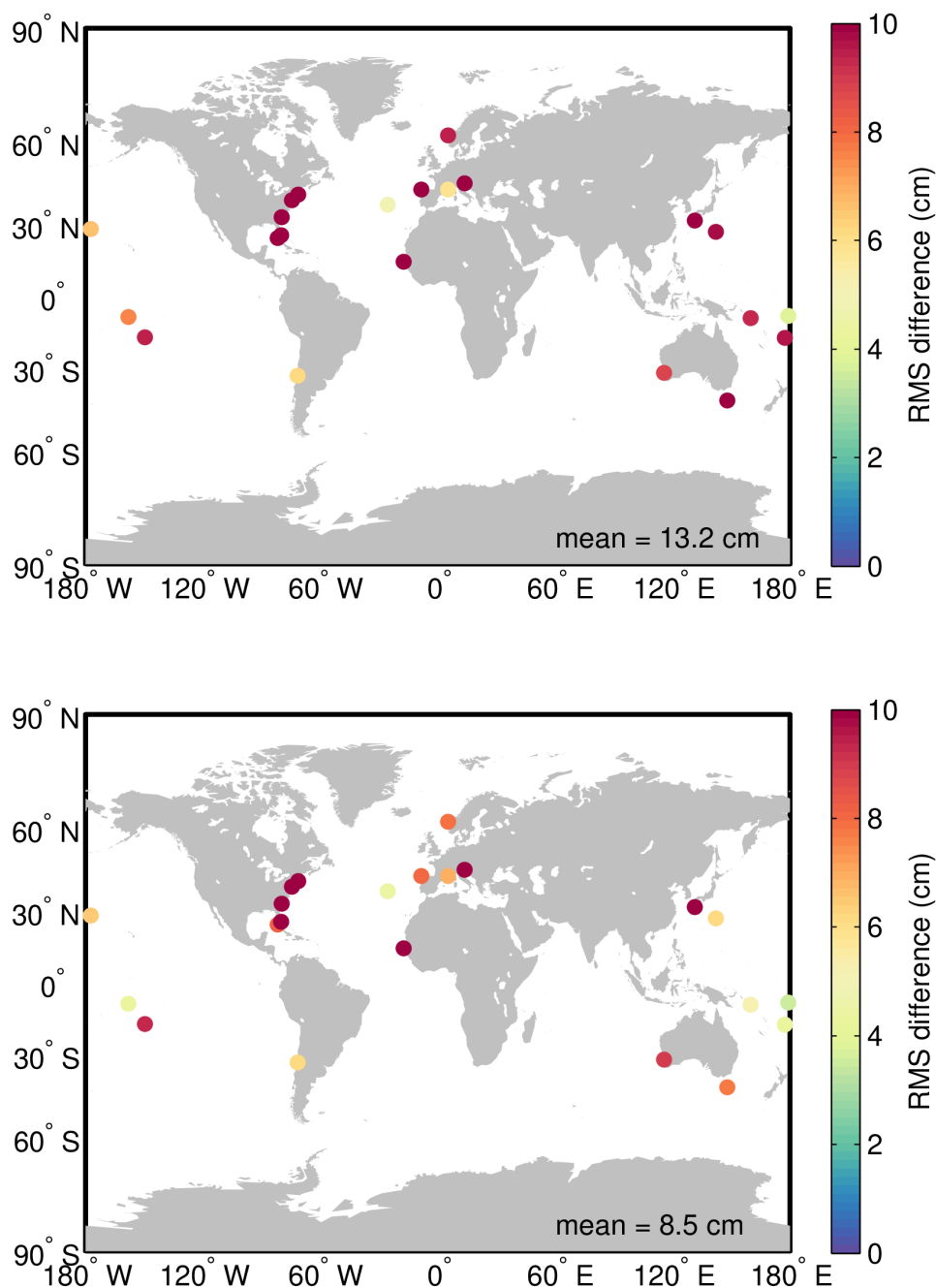
Figure 107. Map showing the RMS difference between the GOP SSH anomaly and the sea level from tide gauge records over the period November 2021 to October 2023 for the cases with (top) and without (bottom) the tidal component. For this comparison the atmospheric component has not been subtracted.
