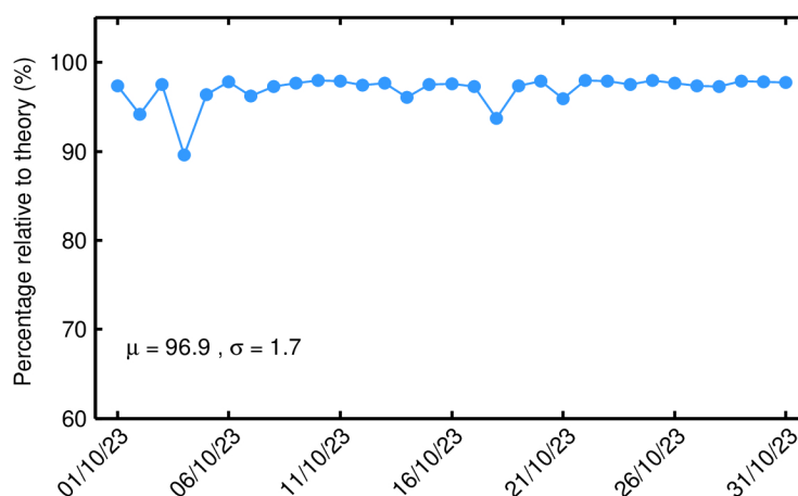
Figure 49. Percentage of science-valid IOP 1-Hz SWH records over ocean and lakes relative to theory for each day in October 2023. The mean ( \mu ) and standard deviation ( \sigma ) are also shown.
