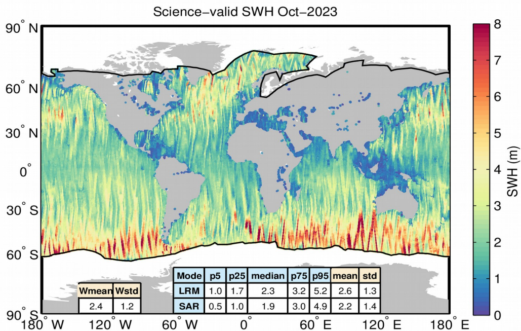
Figure 85. Geographical distribution of science-valid GOP SWH data over oceans and lakes for October 2023. The statistical values shown in the table refer to the SWH in m and are calculated separately for LRM and SAR regions. Wmean and Wstd denote the spatial area-weighted average and its standard deviation. Measurements taken over polar polygons have been excluded from the computation of the statistical values. The black lines mark the outer limit of the Arctic and Antarctic polar polygons.
