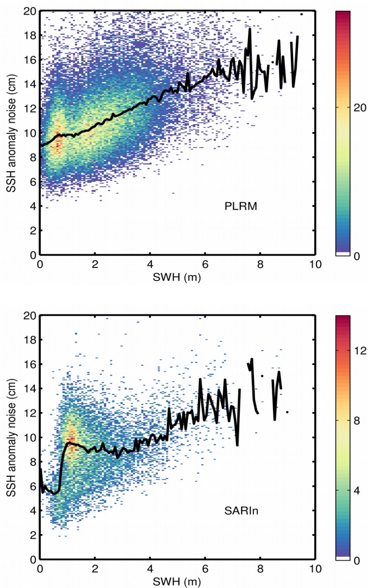
Figure 11. 2D histogram showing science-valid NOP SSH anomaly noise as a function of SWH for SAR, LRM, PLRM, and SARIn (from top to bottom) for October 2023. The black line denotes the median SSH anomaly noise as a function of SWH.
