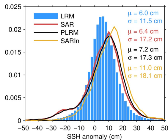
Figure 41. Histogram of science-valid IOP SSH anomaly over oceans and lakes for LRM (blue), SAR (red), PLRM (black) and SARIn (orange) for October 2023. The mean ( \mu ) and standard deviation ( \sigma ) are also shown. Values outside [-50, 50] cm are excluded from the histogram for the sake of readability but not from the computation of \mu and \sigma .
