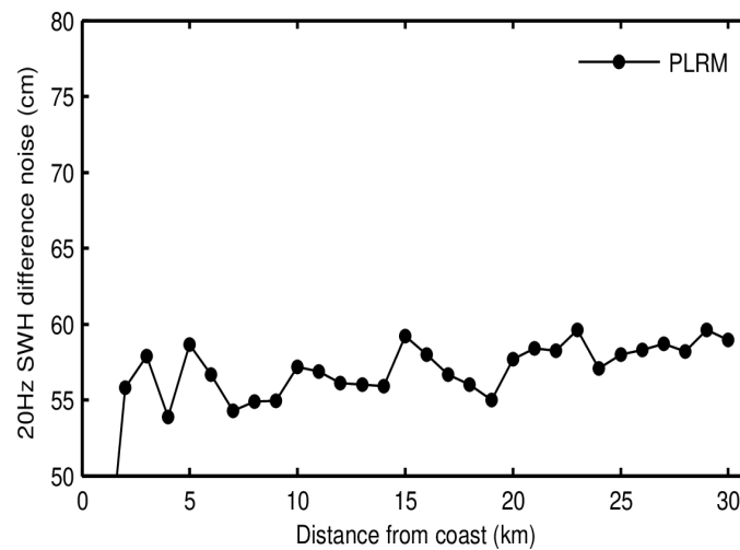
Figure 54. Science-valid IOP 20-Hz SWH noise as a function of distance from the coast for SAR (top panel), LRM (middle panel), and PLRM (bottom panel) for October 2023. Noise values have been calculated as the median of the absolute value of the difference between consecutive 20-Hz records.
