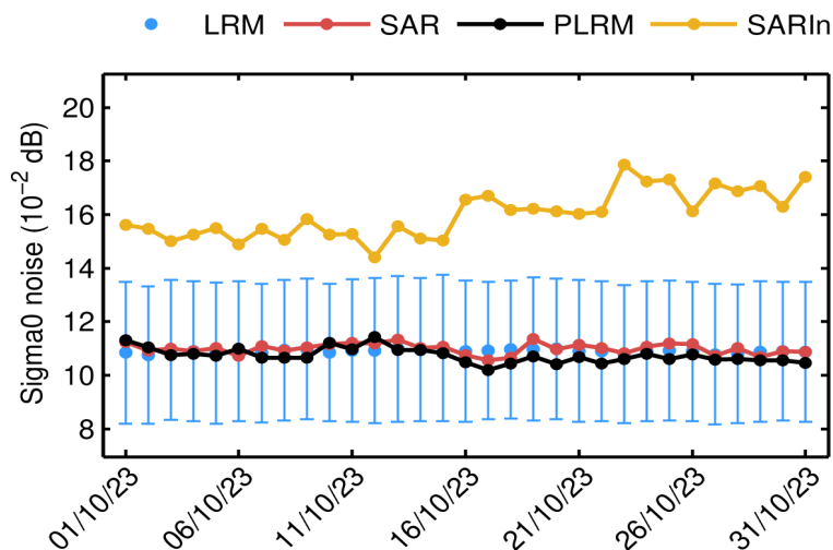
Figure 95. Mean science-valid GOP sigma0 noise for LRM (blue dot), SAR (red dot), PLRM (black dot) and SARIn (orange dot) for each day in October 2023. The corresponding standard deviation for LRM (blue error bar) is also shown.
