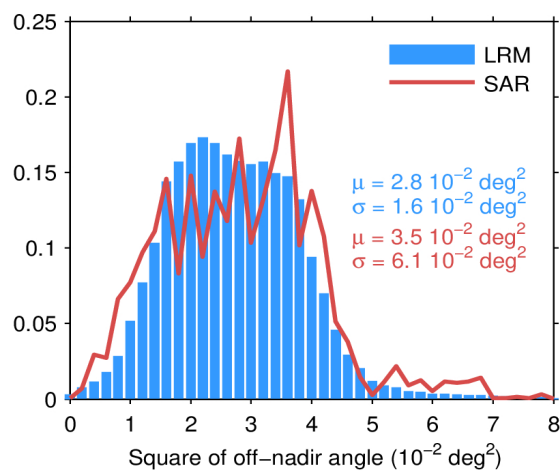
Figure 103. Histogram of science-valid GOP mispointing over oceans and lakes for LRM (blue) and SAR (red) for October 2023. The mean ( \mu ) and standard deviation ( \sigma ) are also shown. Note that values larger than 12 m are excluded from the histogram for the sake of readability but not from the computation of \mu and \sigma .
