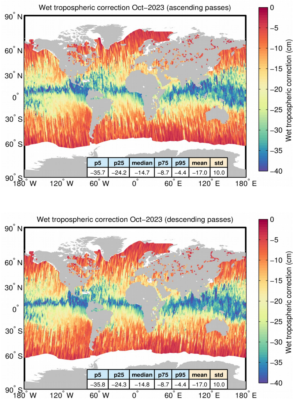
Figure A1. Geographical distribution of the wet tropospheric correction over oceans and lakes for ascending (top) and descending (bottom) passes for October 2023. The statistical values shown in the table refer refer to the wet tropospheric correction in cm. Measurements taken over polar polygons have been excluded from the computation of the statistical values. The black lines mark the outer limit of the Arctic and Antarctic polar polygons.
