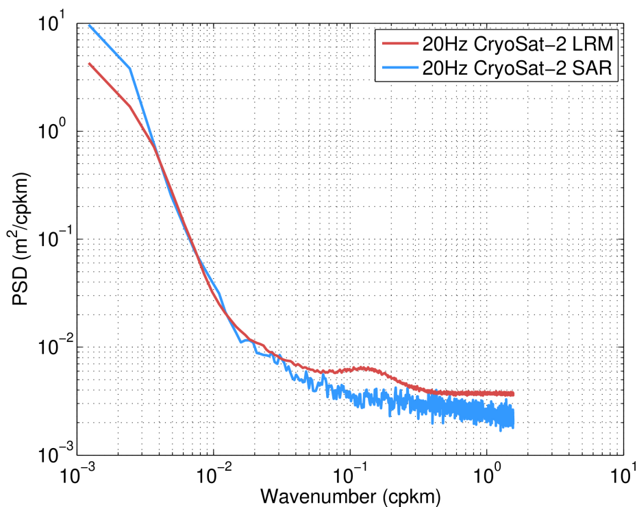
Figure 76. Along-track power spectrum density of the science-valid 20 Hz GOP SSH anomaly over oceans and lakes for LRM (red) and SAR (blue) for October 2023.
