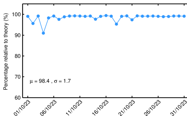
Figure 62. Percentage of science-valid IOP 1-Hz wind records over ocean and lakes relative to theory for each day in October 2023. The mean ( \mu ) and standard deviation ( \sigma ) are also shown.
