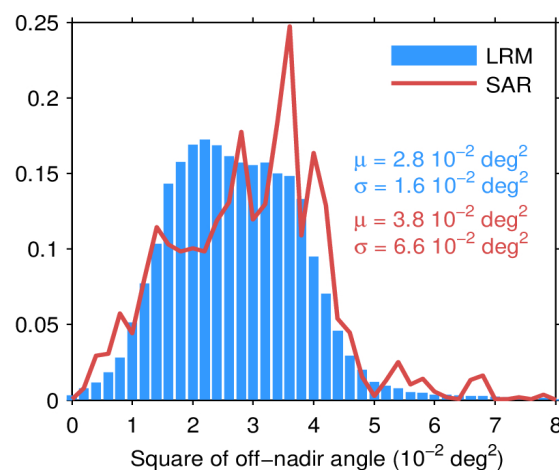
Figure 34. Histogram of science-valid NOP mispointing over oceans and lakes for LRM (blue) and SAR (red) for October 2023. The mean ( \mu ) and standard deviation ( \sigma ) are also shown. Note that values larger than 12 m are excluded from the histogram for the sake of readability but not from the computation of \mu and \sigma .
