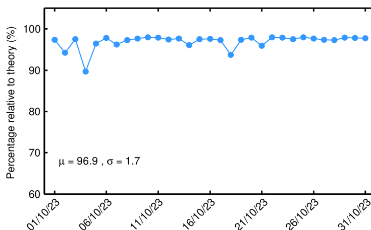
Figure 84. Percentage of science-valid GOP 1-Hz SWH records over ocean and lakes relative to theory for each day in October 2023. The mean ( \mu ) and standard deviation ( \sigma ) are also shown.
