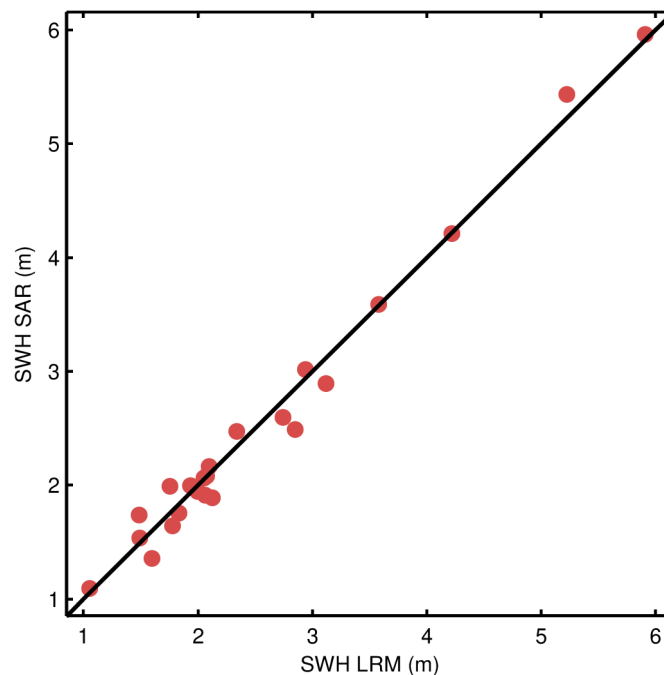
Figure 21. Scatter plot of the science-valid NOP SWH at the two nearest points outside (LRM, x-axis) and inside (SAR, y-axis) the Pacific SAR mode box for each pass. The RMS of the differences is 15.7 cm for the pairs shown in the figure as compared to a RMS of 16.9 cm for the differences between such outside points and their respective nearest neighbour also outside the box in the LRM region.
