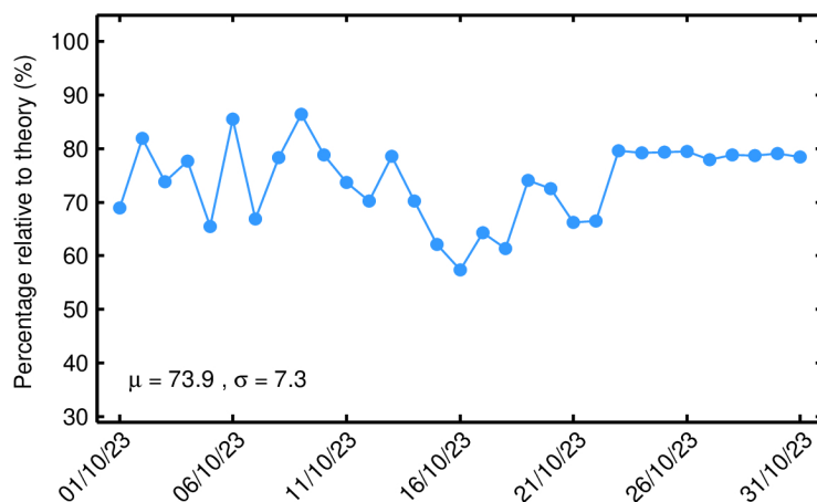
Figure 5. Percentage of science-valid NOP 1-Hz SSH records over ocean and lakes relative to theory for each day in October 2023. The mean ( \mu ) and standard deviation ( \sigma ) are also shown.
