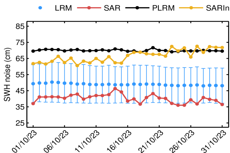
Figure 53. Mean science-valid IOP SWH noise for LRM (blue dot), SAR (red dot), PLRM (black dot) and SARIn (orange dot) for each day in October 2023. The corresponding standard deviation for LRM (blue error bar) is also shown.
