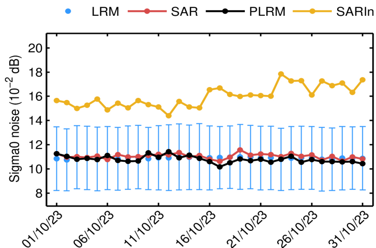
Figure 26. Mean science-valid NOP sigma0 noise for LRM (blue dot), SAR (red dot), PLRM (black dot) and SARIn (orange dot) for each day in October 2023. The corresponding standard deviation for LRM (blue error bar) is also shown.
