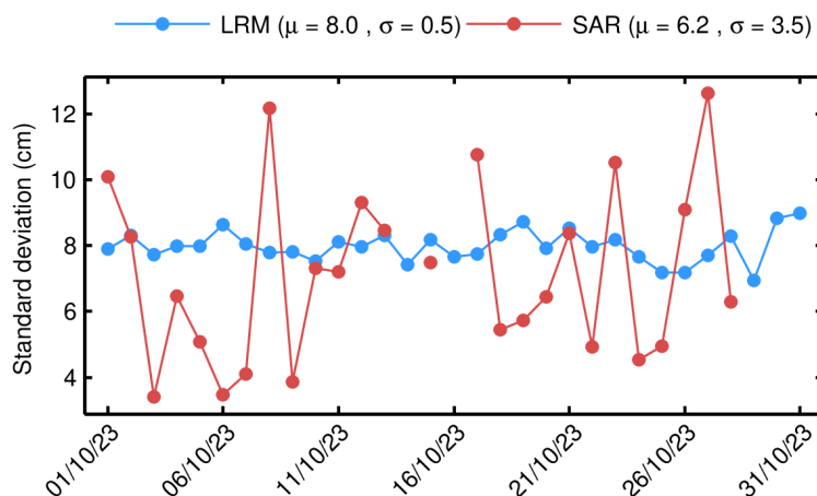
Figure 14. Standard deviation of differences at crossovers for NOP SSH anomaly for each day in October 2023. The values shown in this figure have been computed for the science-valid data further edited according to the following two additional criteria: 1) rejecting crossover differences larger than 20 cm; and 2) rejecting shallow waters (1000 m). The mean ( \mu ) and standard deviation ( \sigma ) are also shown.
