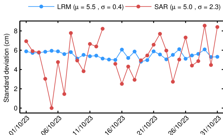
Figure 48. Standard deviation of differences at crossovers for IOP SSH anomaly for each day in October 2023. The values shown in this figure have been computed for the science-valid data further edited according to the following two additional criteria: 1) rejecting crossover differences larger than 20 cm; and 2) rejecting shallow waters (1000 m). The mean ( \mu ) and standard deviation ( \sigma ) are also shown.
