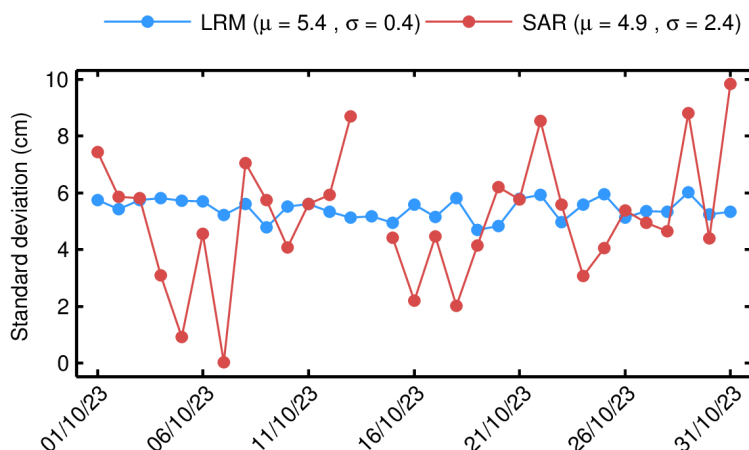
Figure 83. Standard deviation of differences at crossovers for GOP SSH anomaly for each day in October 2023. The values shown in this figure have been computed for the science-valid data further edited according to the following two additional criteria: 1) rejecting crossover differences larger than 20 cm; and 2) rejecting shallow waters (1000 m). The mean ( \mu ) and standard deviation ( \sigma ) are also shown.
