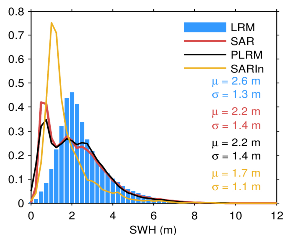
Figure 51. Histogram of science-valid IOP SWH over oceans and lakes for LRM (blue), SAR (red), PLRM (black) and SARIn (orange) for October 2023. The mean ( \mu ) and standard deviation ( \sigma ) are also shown. Values larger than 12 m are excluded from the histogram for the sake of readability but not from the computation of \mu and \sigma .
