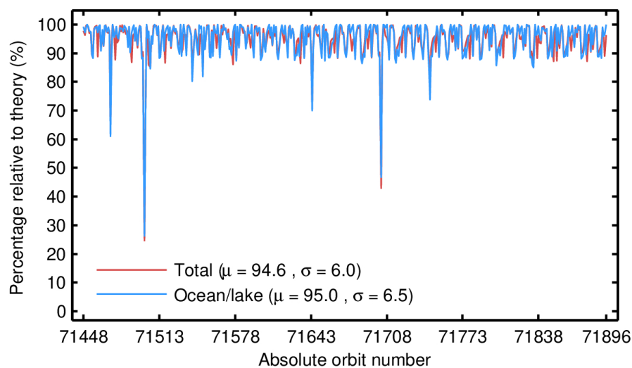
Figure 4. Percentage of NOP 1-Hz records over land and ocean/lake (red) and only over ocean/lake (blue) relative to the theoretically expected number from the orbits ground tracks for each orbit in October 2023. The mean ( \mu ) and standard deviation ( \sigma ) are also shown.
