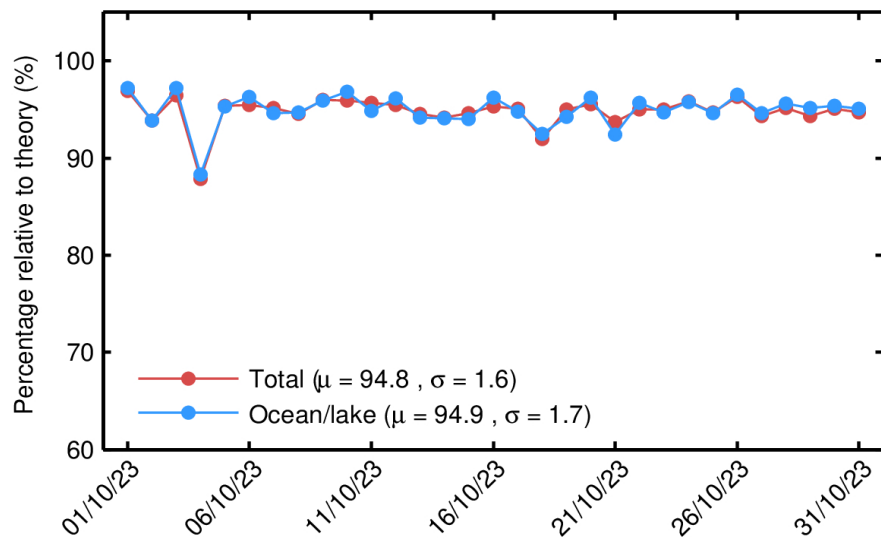
Figure 3. Percentage of NOP 1-Hz records over land and ocean/lake (red) and only over ocean/lake (blue) relative to the theoretically expected number from the orbits ground tracks for each day in October 2023.
