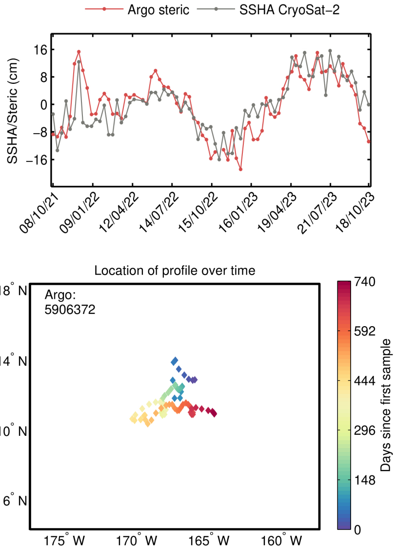
Figure 125. Comparison of the GOP SSH anomaly and the steric height anomaly (referred to 1000 m) for one particular Argo float (top). The location of the Argo float over time is also shown (bottom).
