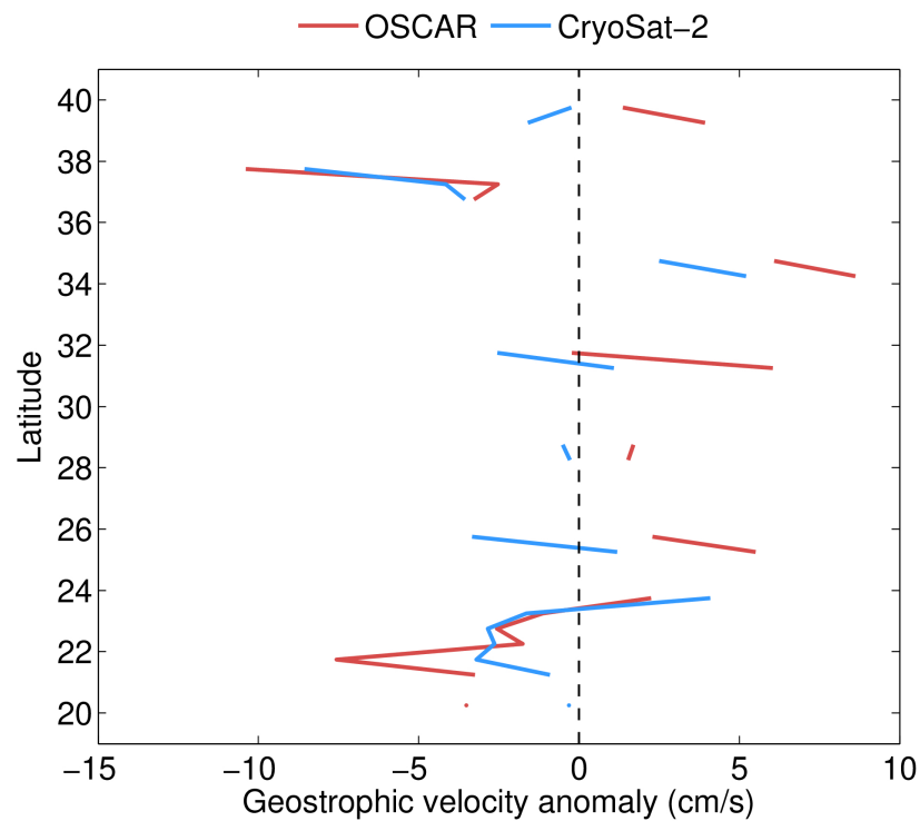
Figure 121. Comparison of the GOP geostrophic velocity anomalies with geostrophic velocities anomalies from the Ocean Surface Current Analyses – Real time (OSCAR) for October 2023 in the Atlantic (top, 20°N – 40°N, 315°E – 325°E) and Pacific (bottom, 20°N – 40°N, 220°E – 230°E) boxes as a function of latitude (i.e., for each latitude the geostrophic velocities have been averaged over the longitudes within the box). GOP geostrophic velocities have been computed using the optimal difference operator by Powell and Leben (2004).
