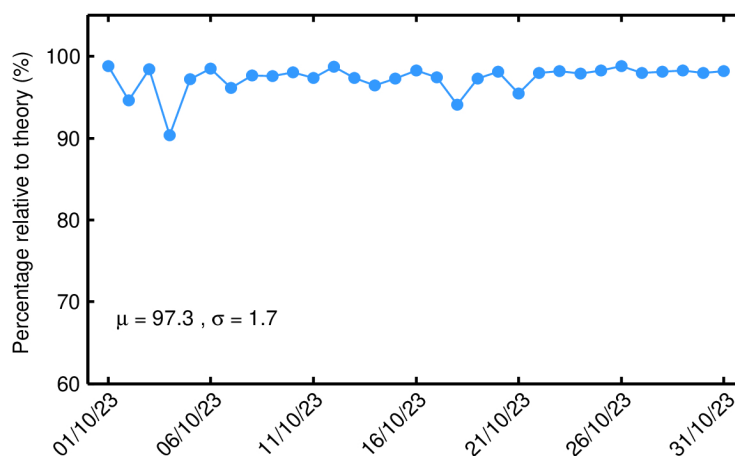
Figure 28. Percentage of science-valid NOP 1-Hz wind records over ocean and lakes relative to theory for each day in October 2023. The mean ( \mu ) and standard deviation ( \sigma ) are also shown.
