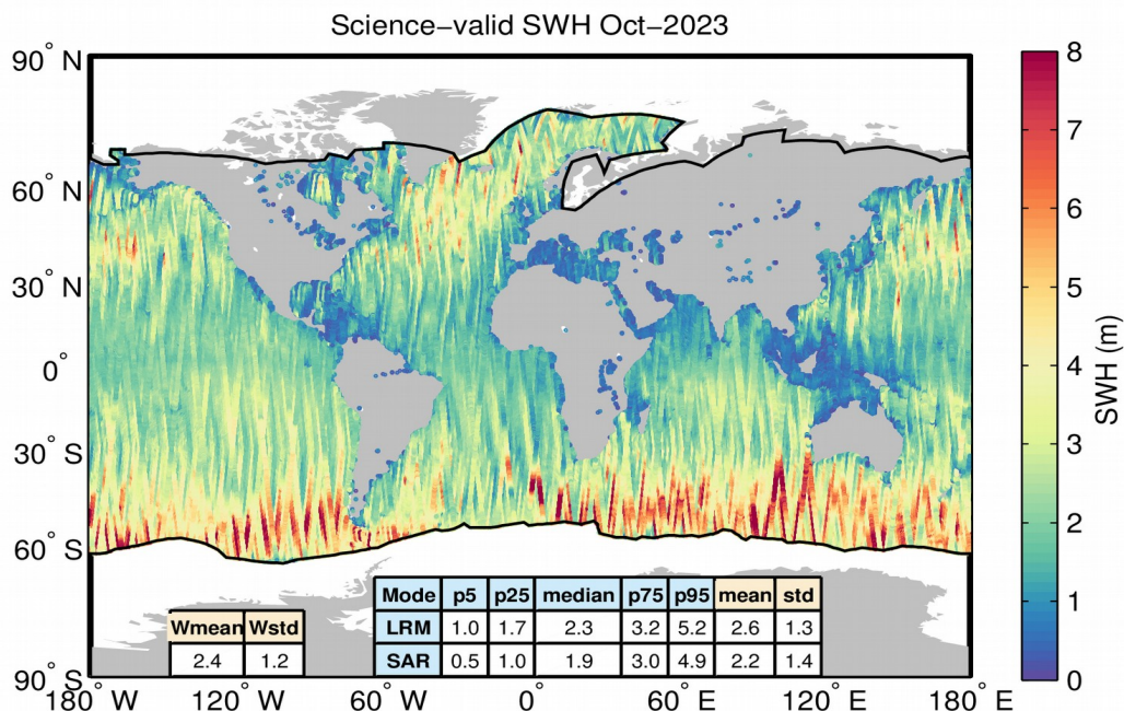
Figure 50. Geographical distribution of science-valid IOP SWH data over oceans and lakes for October 2023. The statistical values shown in the table refer to the SWH in m and are calculated separately for LRM and SAR regions. Wmean and Wstd denote the spatial area-weighted average and its standard deviation. Measurements taken over polar polygons have been excluded from the computation of the statistical values. The black lines mark the outer limit of the Arctic and Antarctic polar polygons.
