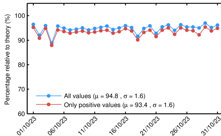
Figure 32. Percentage of science-valid NOP 1-Hz mispointing records over ocean and lakes relative to theory for each day in October 2023. The mean ( \mu ) and standard deviation ( \sigma ) are also shown.
