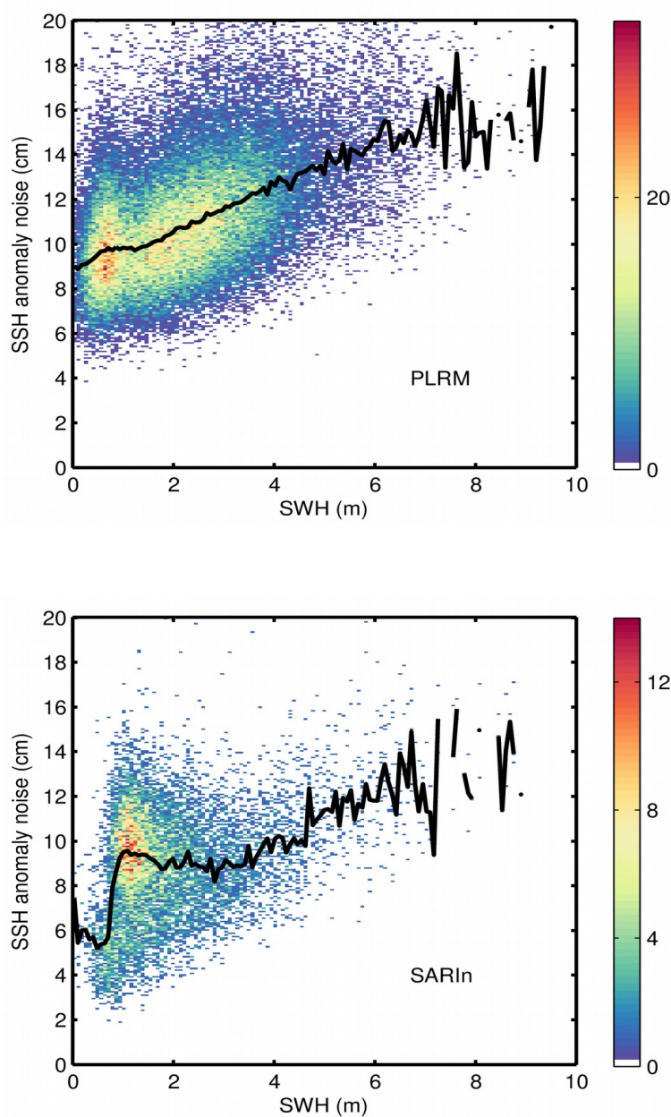
Figure 80. 2D histogram showing science-valid GOP SSH anomaly noise as a function of SWH for SAR, LRM, PLRM, and SARIn (from top to bottom) for October 2023. The black line denotes the median SSH anomaly noise as a function of SWH.
