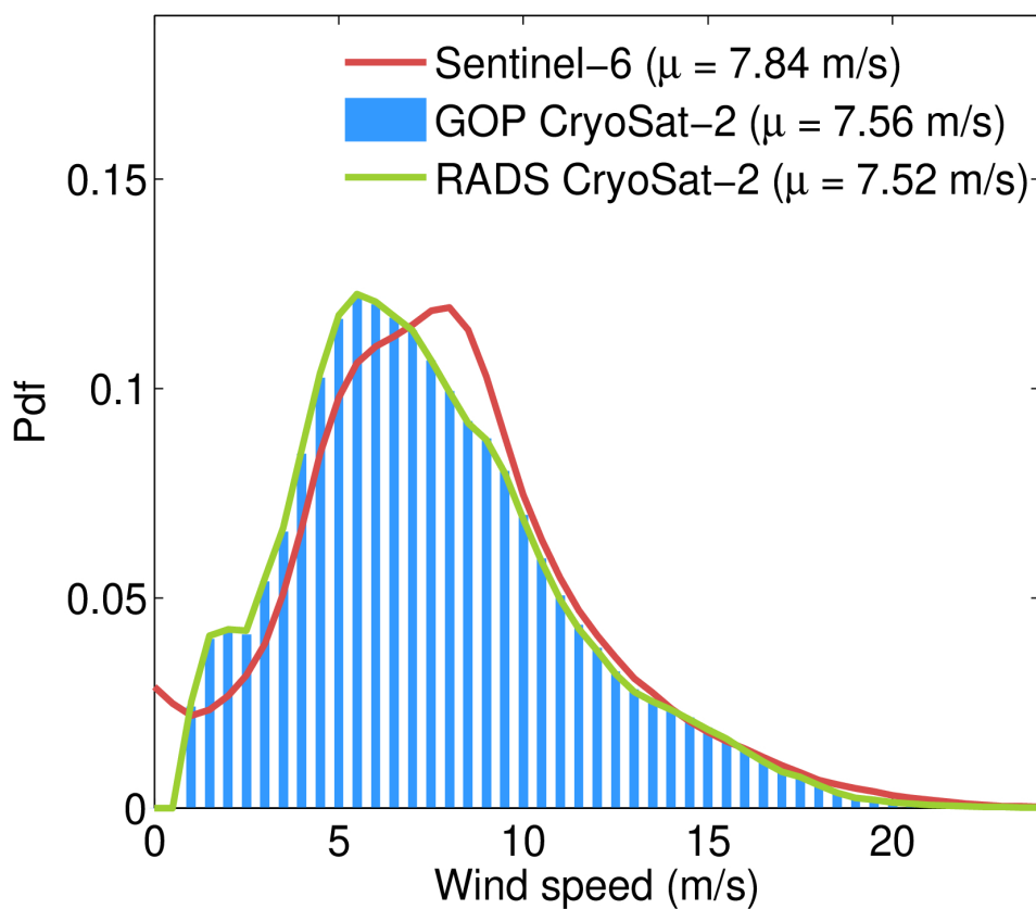
Figure 129. Histograms (normalized to have a total area of 1) of the wind speed from GOP (blue bars), reference mission (red line) and RADS CryoSat-2 (green) for October 2023.
