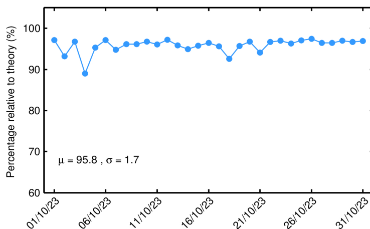
Figure 15. Percentage of science-valid NOP 1-Hz SWH records over ocean and lakes relative to theory for each day in October 2023. The mean ( \mu ) and standard deviation ( \sigma ) are also shown.
