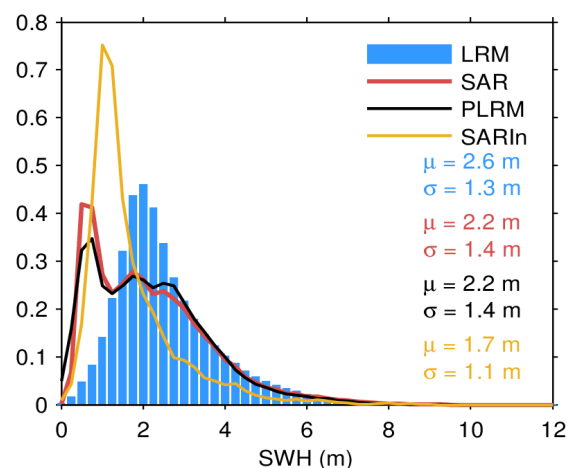
Figure 86. Histogram of science-valid GOP SWH over oceans and lakes for LRM (blue), SAR (red), PLRM (black) and SARIn (orange) and for October 2023. The mean ( \mu ) and standard deviation ( \sigma ) are also shown. Values larger than 12 m are excluded from the histogram for the sake of readability but not from the computation of \mu and \sigma .
