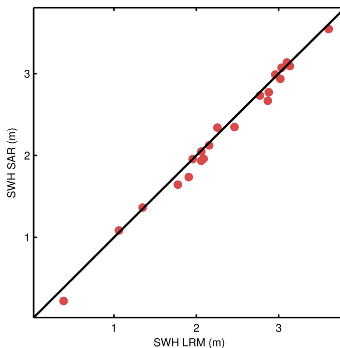
Figure 90. Scatter plot of the science-valid GOP SWH at the two nearest points outside (LRM, x-axis) and inside (SAR, y-axis) the Pacific SAR mode box for each pass. The RMS of the differences is 9.6 cm for the pairs shown in the figure as compared to a RMS of 17.9 cm for the differences between such outside points and their respective nearest neighbour also outside the box in the LRM region.
