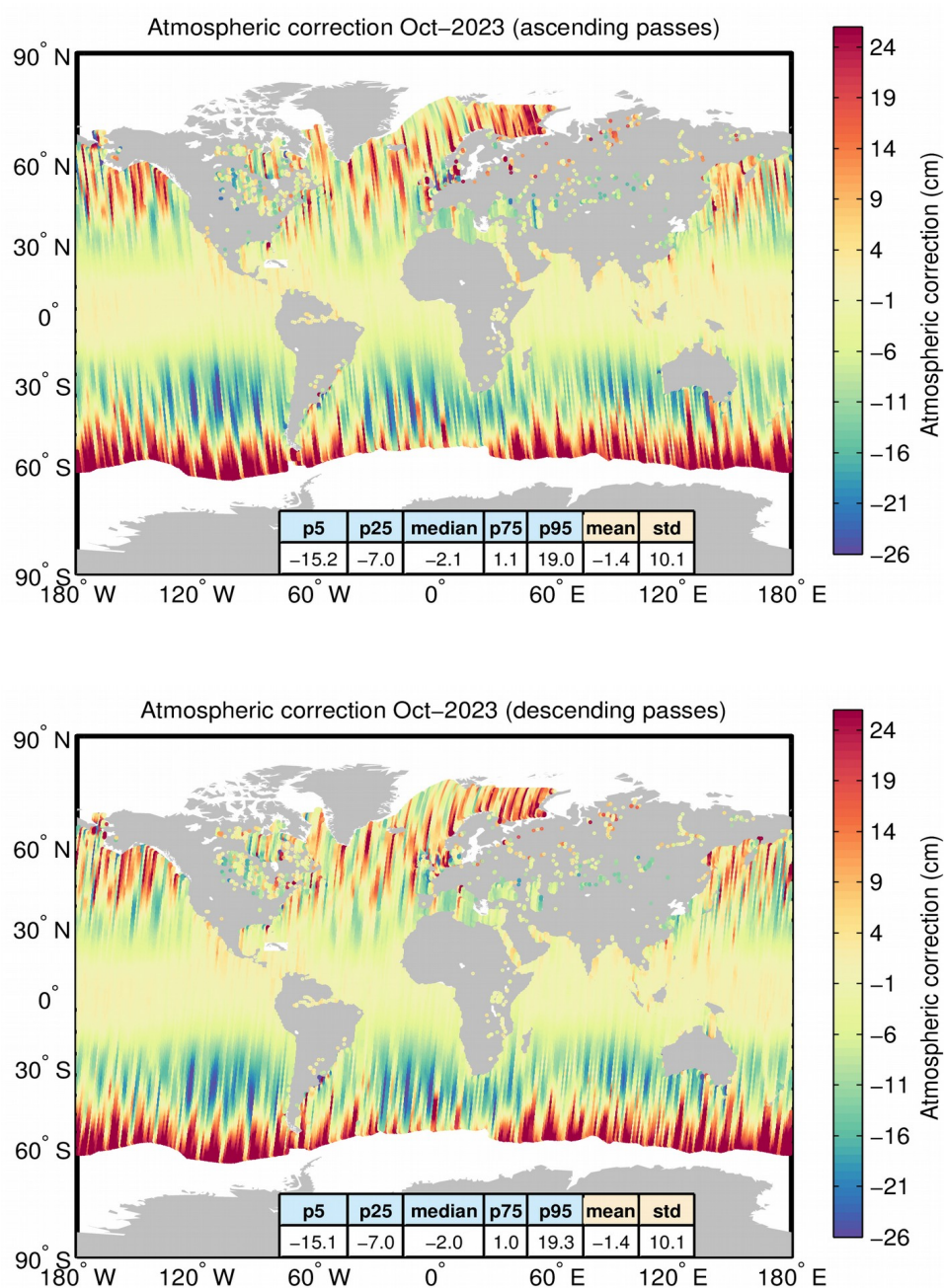
Figure A5. Geographical distribution of the atmospheric correction over oceans and lakes for ascending (top) and descending (bottom) passes for October 2023. The statistical values shown in the table refer to the atmospheric correction in cm. Measurements taken over polar polygons have been excluded from the computation of the statistical values. The black lines mark the outer limit of the Arctic and Antarctic polar polygons.
