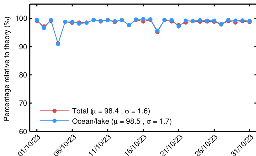
Figure 71. Percentage of GOP 1-Hz records over land and ocean/lake (red) and only over ocean/lake (blue) relative to the theoretically expected number from the orbits ground tracks for each day in October 2023.
