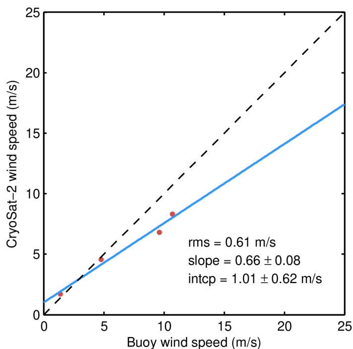
Figure 115. Scatter plot showing a comparison of GOP wind speed with wind speed from NDBC buoy data for October 2023.
