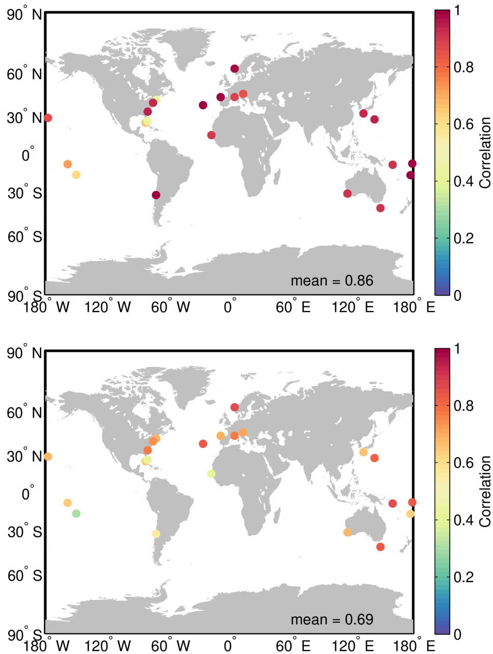
Figure 106. Map showing the correlation between the GOP SSH anomaly and the sea level from tide gauge records over the period November 2021 to October 2023 for the cases with (top) and without (bottom) the tidal component. For this comparison the atmospheric component has not been subtracted. Empty dots denote statistically non-significant correlation.
