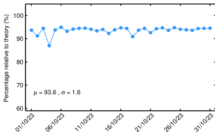
Figure 91. Percentage of science-valid GOP 1-Hz sigma0 records over ocean and lakes relative to theory for each day in October 2023. The mean ( \mu ) and standard deviation ( \sigma ) are also shown.
