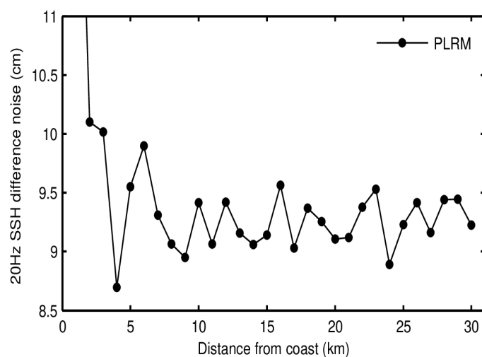
Figure 10. Science-valid NOP 20-Hz SSH anomaly noise as a function of distance from the coast for SAR (top panel), LRM (middle panel), and PLRM (bottom panel) for October 2023. Noise values have been calculated as the median of the absolute value of the difference between consecutive 20-Hz records.
