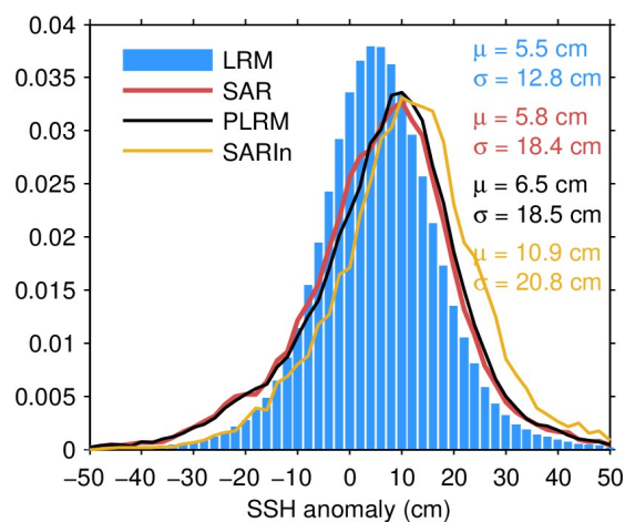
Figure 7. Histogram of science-valid NOP SSH anomaly over oceans and lakes for LRM (blue), SAR (red), PLRM (black) and SARIn (orange) for October 2023. The mean ( \mu ) and standard deviation ( \sigma ) are also shown. Values outside [-50 \ 50] cm are excluded from the histogram for the sake of readability but not from the computation of \mu and \sigma .
