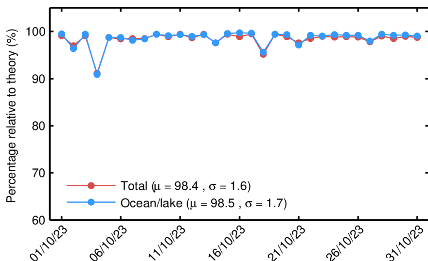
Figure 37. Percentage of IOP 1-Hz records over land and ocean/lake (red) and only over ocean/lake (blue) relative to the theoretically expected number from the orbits ground tracks for each day in October 2023.
