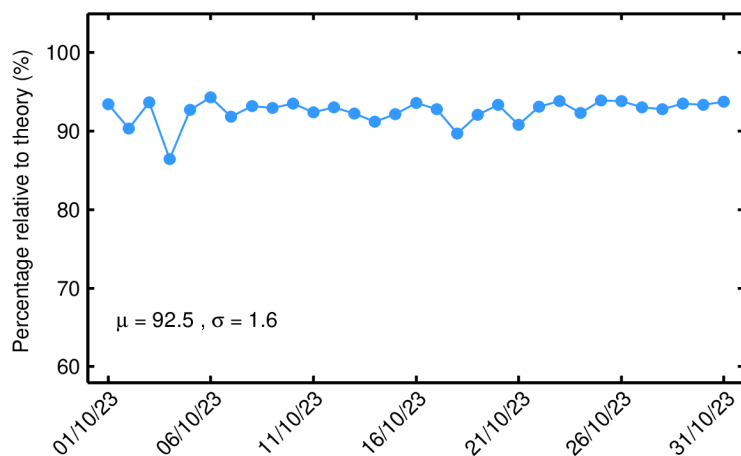
Figure 22. Percentage of science-valid NOP 1-Hz sigma0 records over ocean and lakes relative to theory for each day in October 2023. The mean ( \mu ) and standard deviation ( \sigma ) are also shown.
