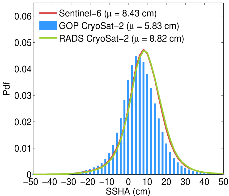
Figure 127. Histograms (normalized to have a total area of 1) of the SSH anomaly from GOP (blue bars), reference mission (red line) and RADS CryoSat-2 (green) for October 2023.
