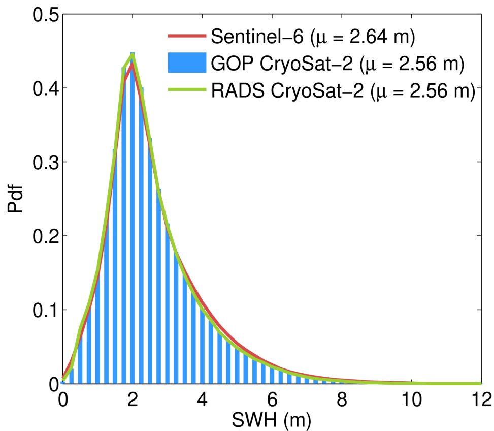
Figure 128. Histograms (normalized to have a total area of 1) of the SWH from GOP (blue bars), reference mission (red line) and RADS CryoSat-2 (green) for October 2023.
