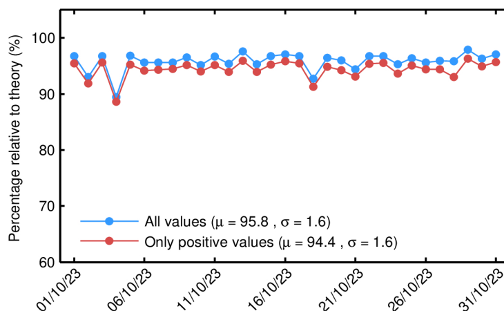
Figure 101. Percentage of science-valid GOP 1-Hz mispointing records over ocean and lakes relative to theory for each day in October 2023. The mean ( \mu ) and standard deviation ( \sigma ) are also shown.
