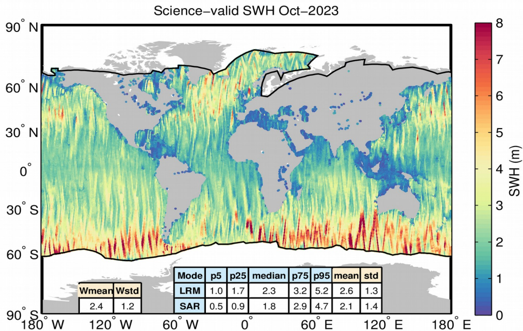
Figure 16. Geographical distribution of science-valid NOP SWH data over oceans and lakes for October 2023. The statistical values shown in the table refer to the SWH in m and are calculated separately for LRM and SAR regions. Wmean and Wstd denote the spatial area-weighted average and its standard deviation. Measurements taken over polar polygons have been excluded from the computation of the statistical values. The black lines mark the outer limit of the Arctic and Antarctic polar polygons.
