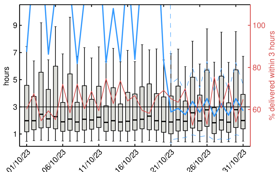
Figure 1. Box-and-whiskers plot for the NOP latency showing for each day in October 2023 the first and third quartiles (bottom and top of the box), the median (thick black), the
