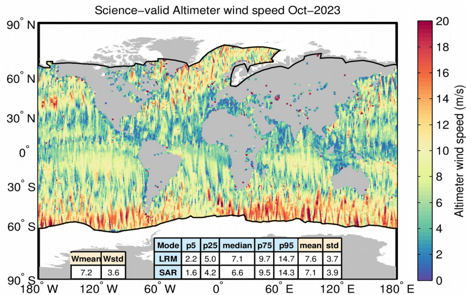
Figure 98. Geographical distribution of science-valid GOP wind data over oceans and lakes for October 2023. The statistical values shown in the table refer to the wind in m and are calculated separately for LRM and SAR regions. Wmean and Wstd denote the spatial area-weighted average and its standard deviation. Measurements taken over polar polygons have been excluded from the computation of the statistical values. The black lines mark the outer limit of the Arctic and Antarctic polar polygons.
