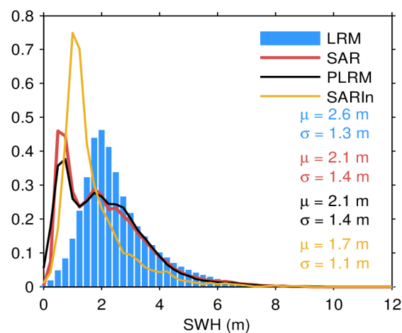
Figure 17. Histogram of science-valid NOP SWH over oceans and lakes for LRM (blue), SAR (red), PLRM (black) and SARIn (orange) for October 2023. The mean ( \mu ) and standard deviation ( \sigma ) are also shown. Values larger than 12 m are excluded from the histogram for the sake of readability but not from the computation of \mu and \sigma .
