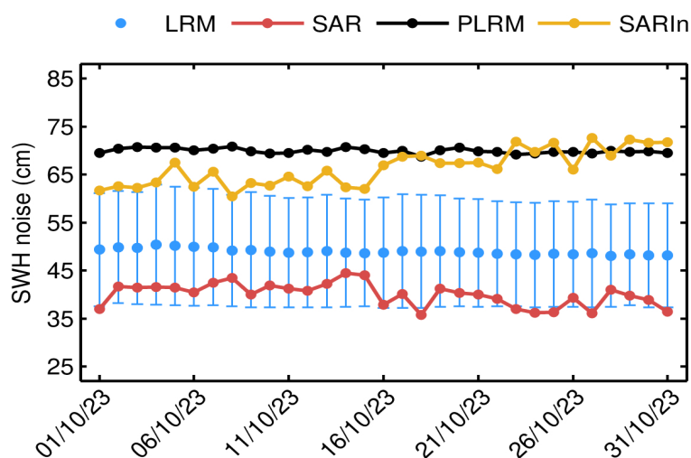
Figure 19. Mean science-valid NOP SWH noise for LRM (blue dot), SAR (red dot), PLRM (black dot) and SARIn (orange dot) for each day in October 2023. The corresponding standard deviation for LRM (blue error bar) is also shown.
