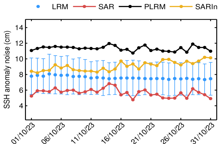
Figure 9. Mean science-valid NOP SSH anomaly noise for LRM (blue dot), SAR (red dot), PLRM (black dot) and SARIn (orange dot) for each day in October 2023. The corresponding standard deviation for LRM (blue error bar) is also shown.
