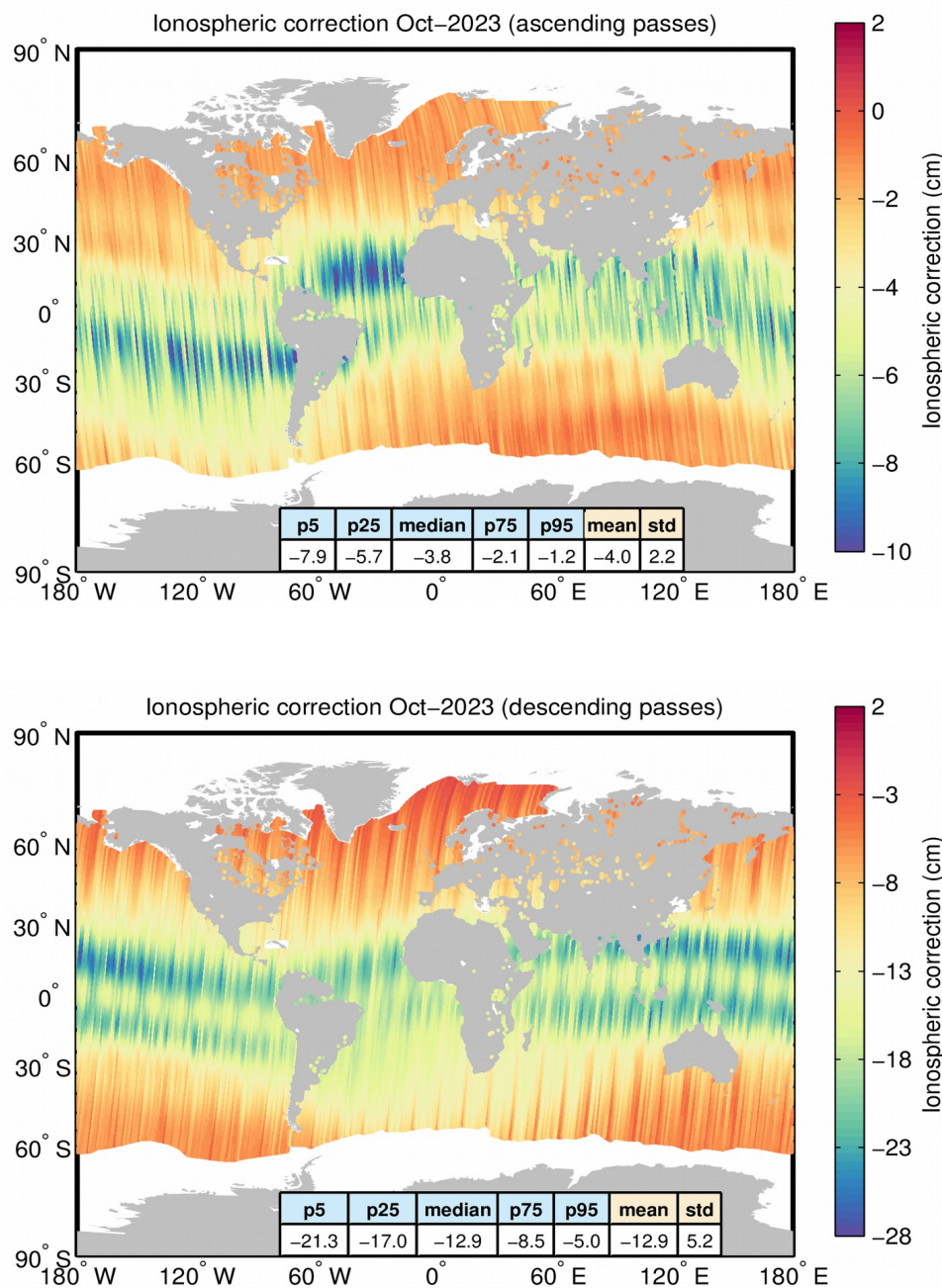
Figure A3. Geographical distribution of the Ionospheric correction over oceans and lakes for ascending (top) and descending (bottom) passes for October 2023. The statistical values shown in the table refer to the Ionospheric correction in cm. Measurements taken over polar polygons have been excluded from the computation of the statistical values. The black lines mark the outer limit of the Arctic and Antarctic polar polygons.
