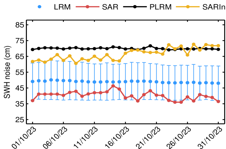
Figure 88. Mean science-valid GOP SWH noise for LRM (blue dot), SAR (red dot), PLRM (black dot) and SARIn (orange dot) for each day in October 2023. The corresponding standard deviation for LRM (blue error bar) is also shown.
