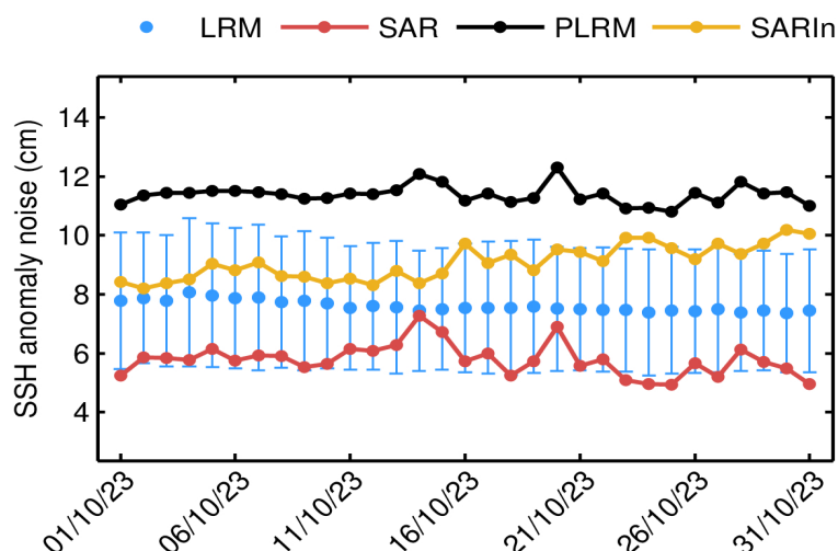
Figure 43. Mean science-valid IOP SSH anomaly noise for LRM (blue dot), SAR (red dot), PLRM (black dot) and SARIn (orange dot) for each day in October 2023. The corresponding standard deviation for LRM (blue error bar) is also shown.
