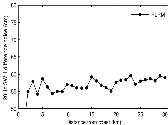
Figure 89. Science-valid GOP 20-Hz SWH noise as a function of distance from the coast for SAR (top panel), LRM (middle panel), and PLRM (bottom panel) for October 2023. Noise values have been calculated as the median of the absolute value of the difference between consecutive 20-Hz records.
