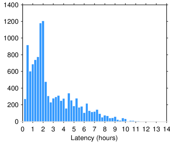
Figure 2. Histogram of the NOP data latency for October 2023. The y-axis denotes the number of files that are made available with a delay of x-hours with respect to the mean time of the records stored in the file.
