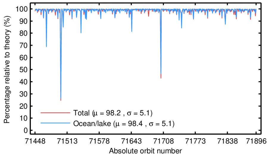
Figure 38. Percentage of IOP 1-Hz records over land and ocean/lake (red) and only over ocean/lake (blue) relative to the theoretically expected number from the orbits ground tracks for each orbit in October 2023. The mean ( \mu ) and standard deviation ( \sigma ) are also shown.
