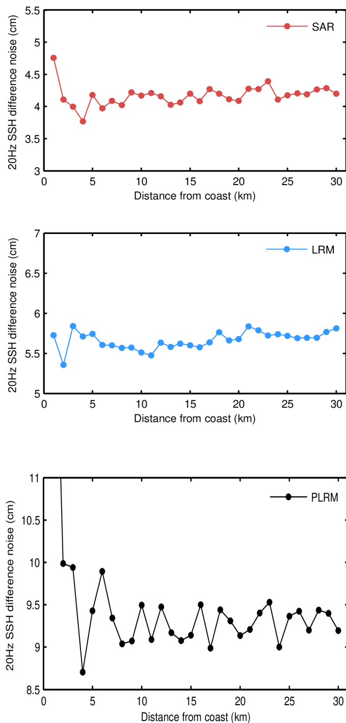
Figure 79. Science-valid GOP 20-Hz SSH anomaly noise as a function of distance from the coast for SAR (top panel), LRM (middle panel), and PLRM (bottom panel) for October 2023. Noise values have been calculated as the median of the absolute value of the difference between consecutive 20-Hz records.
