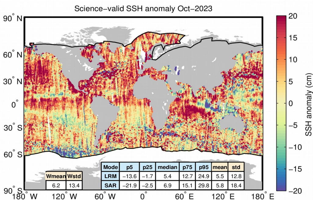
Figure 6. Geographical distribution of science-valid NOP 1-Hz SSH anomaly data over oceans and lakes for October 2023. The statistical values shown in the table refer to the SSH anomaly in cm and are calculated separately for LRM and SAR regions. Wmean and Wstd denote the spatial area-weighted average and its standard deviation. Measurements taken over polar polygons have been excluded from the computation of the statistical values. The black lines mark the outer limit of the Arctic and Antarctic polar polygons.
