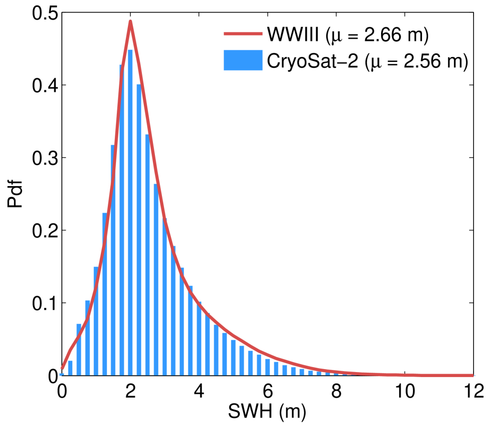
Figure 118. Histograms (normalized to have a total area of 1) of the GOP SWH (blue bars) and the SWH from the Wavewatch III model (red line) for October 2023.
