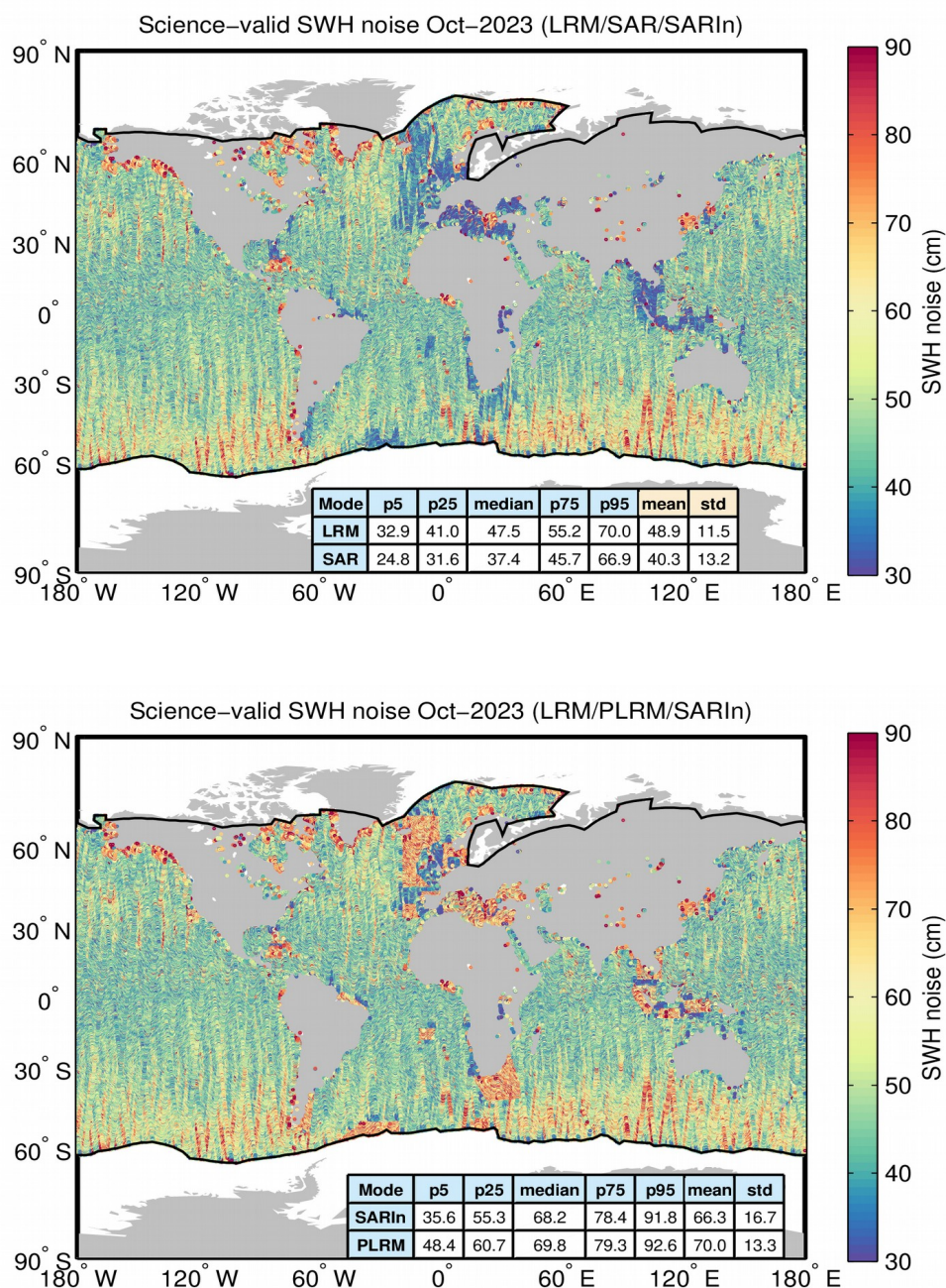
Figure 52. Geographical distribution of flag-valid 20-Hz SWH measurement noise over oceans and lakes for LRM/SAR/SARIn (top) and LRM/PLRM/SARIn (bottom) and for October 2023. The statistical values shown in the table refer to the SWH noise and are calculated separately for LRM, SAR/PLRM and SARIn regions. Measurements taken over polar polygons have been excluded from the computation of the statistical values. The black lines mark the outer limit of the Arctic and Antarctic polar polygons.
