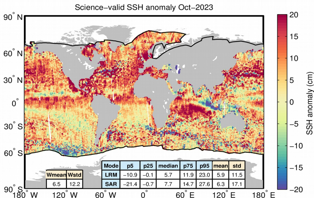
Figure 74. Geographical distribution of science-valid GOP 1-Hz SSH anomaly data over oceans and lakes for October 2023. The statistical values shown in the table refer to the SSH anomaly in cm and are calculated separately for LRM and SAR regions. Wmean and Wstd denote the spatial area-weighted average and its standard deviation. Measurements taken over polar polygons have been excluded from the computation of the statistical values. The black lines mark the outer limit of the Arctic and Antarctic polar polygons.
