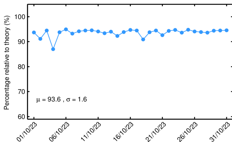
Figure 56. Percentage of science-valid IOP 1-Hz sigma0 records over ocean and lakes relative to theory for each day in October 2023. The mean ( \mu ) and standard deviation ( \sigma ) are also shown.
