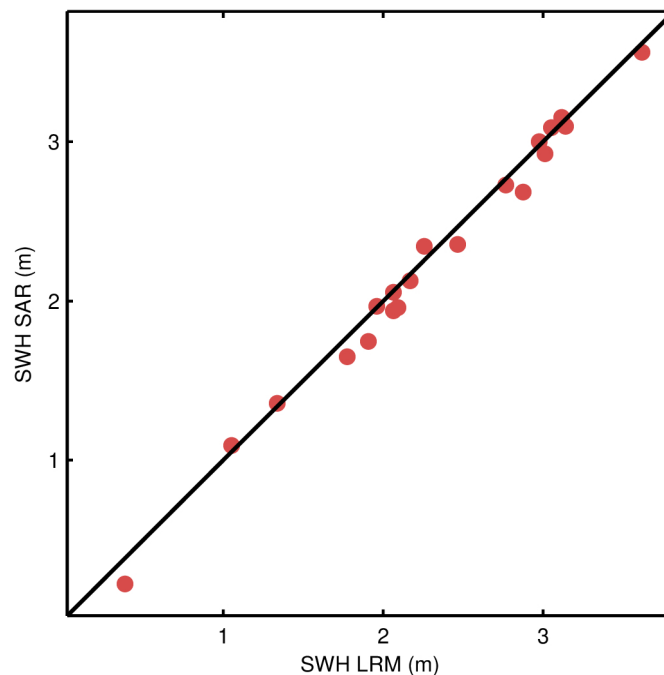
Figure 55. Scatter plot of the science-valid IOP SWH at the two nearest points outside (LRM, x-axis) and inside (SAR, y-axis) the Pacific SAR mode box for each pass. The RMS of the differences is 9.4 cm for the pairs shown in the figure as compared to a RMS of 18.2 cm for the differences between such outside points and their respective nearest neighbour also outside the box in the LRM region.
