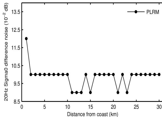
Figure 61. Science-valid IOP 20-Hz sigma0 noise as a function of distance from the coast for SAR (top panel), LRM (middle panel), and PLRM (bottom panel) for October 2023. Noise values have been calculated as the median of the absolute value of the difference between consecutive 20-Hz records.
