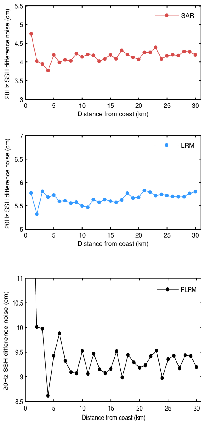
Figure 44. Science-valid IOP 20-Hz SSH anomaly noise as a function of distance from the coast for SAR (top panel), LRM (middle panel), and PLRM (bottom panel) for October 2023. Noise values have been calculated as the median of the absolute value of the difference between consecutive 20-Hz records.
