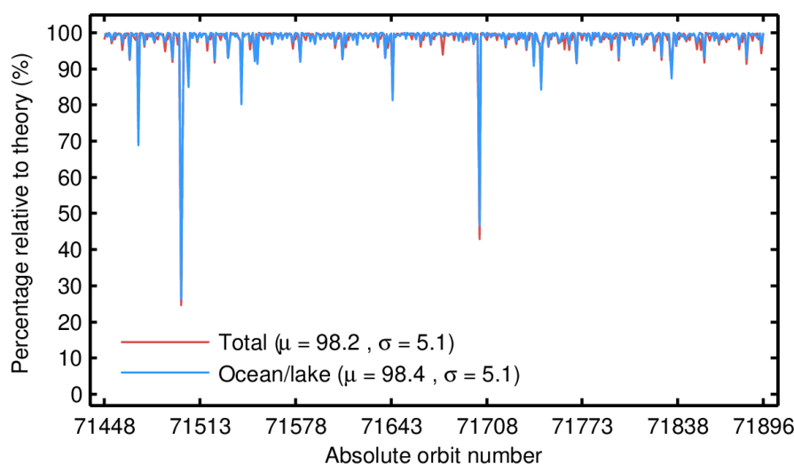
Figure 72. Percentage of GOP 1-Hz records over land and ocean/lake (red) and only over ocean/lake (blue) relative to the theoretically expected number from the orbits ground tracks for each orbit in October 2023. The mean ( \mu ) and standard deviation ( \sigma ) are also shown.
