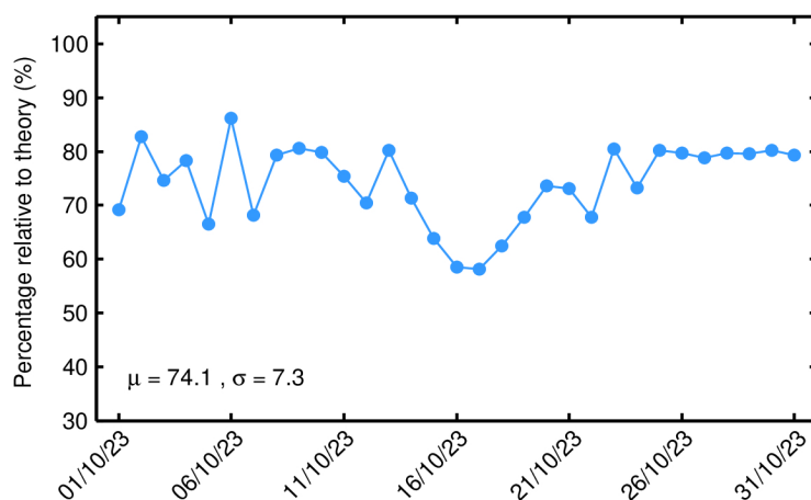
Figure 39. Percentage of science-valid IOP 1-Hz SSH records over ocean and lakes relative to theory for each day in October 2023. The mean ( \mu ) and standard deviation ( \sigma ) are also shown.
