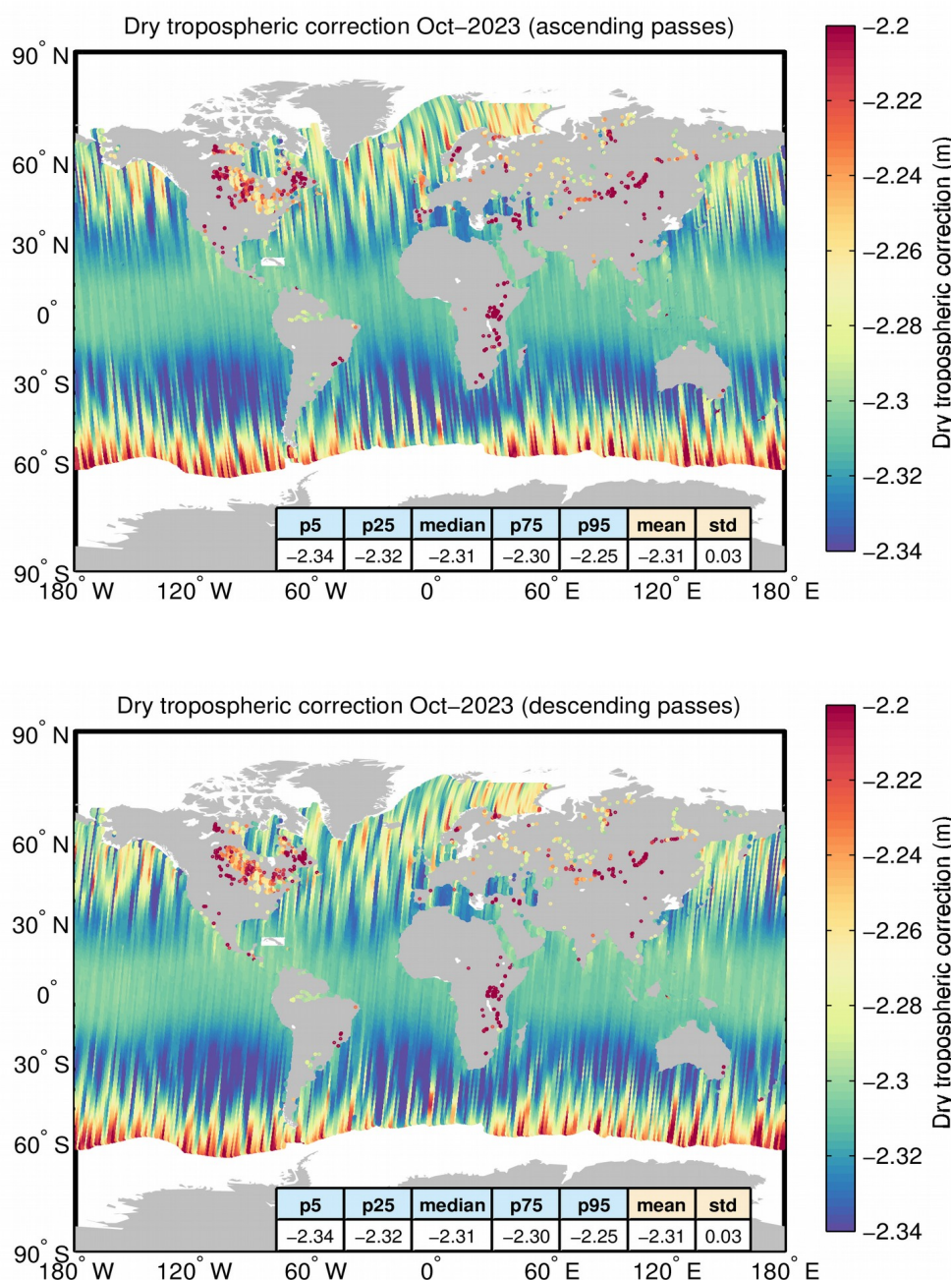
Figure A2. Geographical distribution of the dry tropospheric correction over oceans and lakes for ascending (top) and descending (bottom) passes for October 2023. The statistical values shown in the table refer to the dry tropospheric correction in m. Measurements taken over polar polygons have been excluded from the computation of the statistical values. The black lines mark the outer limit of the Arctic and Antarctic polar polygons.
