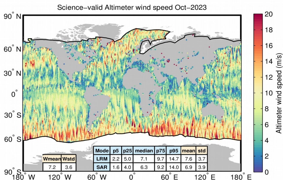
Figure 29. Geographical distribution of science-valid NOP wind data over oceans and lakes for October 2023. The statistical values shown in the table refer to the wind in m and are calculated separately for LRM and SAR regions. Wmean and Wstd denote the spatial area-weighted average and its standard deviation. Measurements taken over polar polygons have been excluded from the computation of the statistical values. The black lines mark the outer limit of the Arctic and Antarctic polar polygons.
