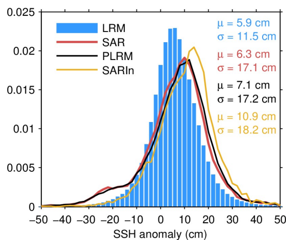
Figure 75. Histogram of science-valid GOP SSH anomaly over oceans and lakes for LRM (blue), SAR (red), PLRM (black) and SARIn (orange) for October 2023. The mean ( \mu ) and
