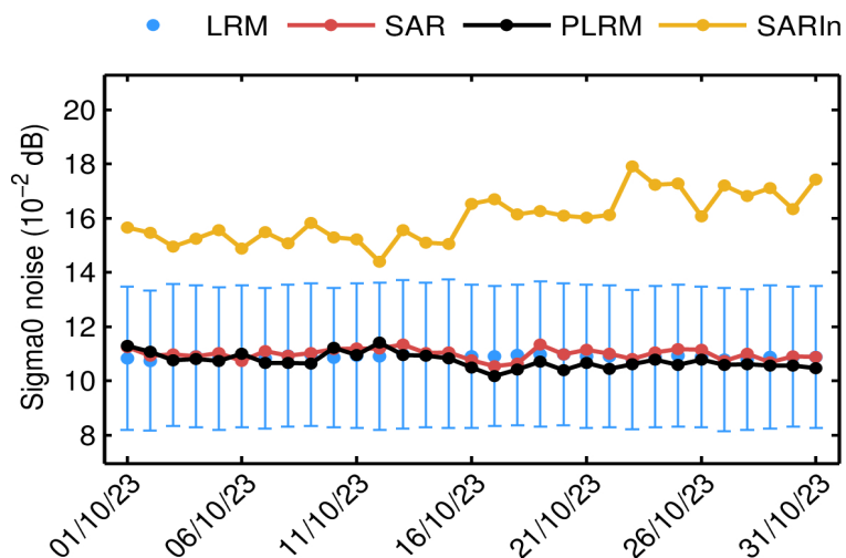
Figure 60. Mean science-valid IOP sigma0 noise for LRM (blue dot), SAR (red dot), PLRM (black dot) and SARIn (orange dot) for each day in October 2023. The corresponding standard deviation for LRM (blue error bar) is also shown.
