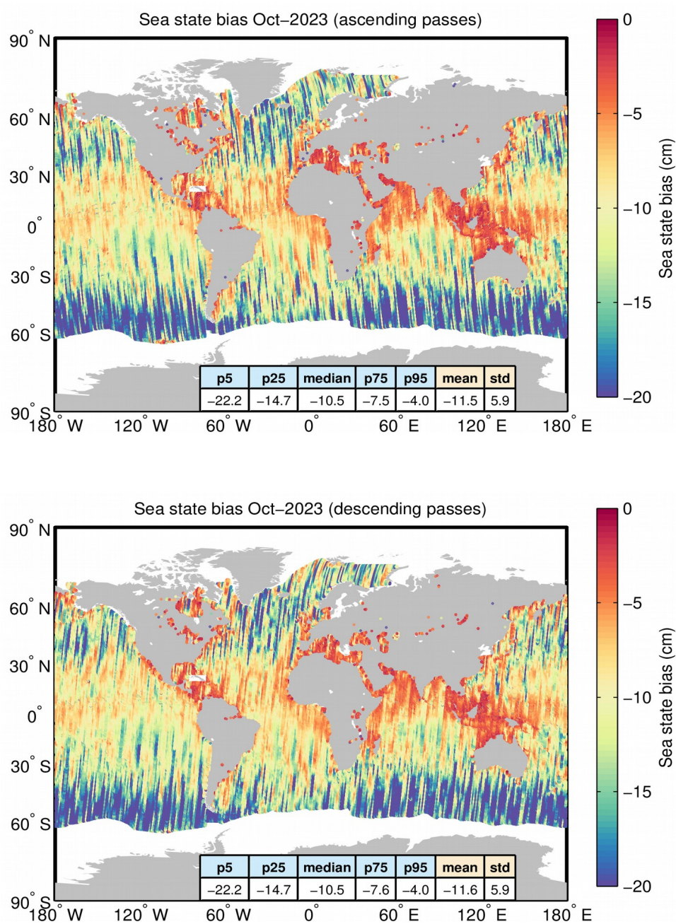
Figure A4. Geographical distribution of the sea state bias over oceans and lakes for ascending (top) and descending (bottom) passes for October 2023. The statistical values shown in the table refer to the sea state bias in cm. Measurements taken over polar polygons have been excluded from the computation of the statistical values. The black lines mark the outer limit of the Arctic and Antarctic polar polygons.
