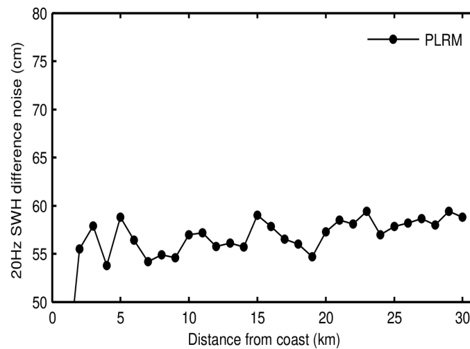
Figure 20. Science-valid NOP 20-Hz SWH noise as a function of distance from the coast for SAR (top panel), LRM (middle panel), and PLRM (bottom panel) for October 2023. Noise values have been calculated as the median of the absolute value of the difference between consecutive 20-Hz records.
