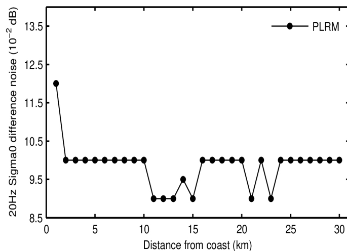
Figure 96. Science-valid GOP 20-Hz sigma0 noise as a function of distance from the coast for SAR (top panel), LRM (middle panel), and PLRM (bottom panel) for October 2023. Noise values have been calculated as the median of the absolute value of the difference between consecutive 20-Hz records.
