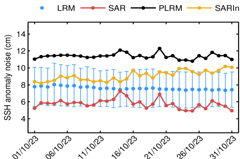
Figure 78. Mean science-valid GOP SSH anomaly noise for LRM (blue dot), SAR (red dot), PLRM (black dot) and SARIn (orange dot) for each day in October 2023. The corresponding standard deviation for LRM (blue error bar) is also shown.
