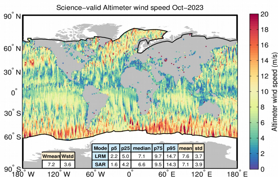
Figure 63. Geographical distribution of science-valid IOP wind data over oceans and lakes for October 2023. The statistical values shown in the table refer to the wind in m and are calculated separately for LRM and SAR regions. Wmean and Wstd denote the spatial area-weighted average and its standard deviation. Measurements taken over polar polygons have been excluded from the computation of the statistical values. The black lines mark the outer limit of the Arctic and Antarctic polar polygons.
