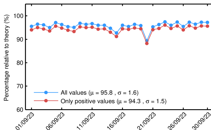
Figure 101. Percentage of science-valid GOP 1-Hz mispointing records over ocean and lakes relative to theory for each day in September 2023. The mean ( \mu ) and standard deviation ( \sigma ) are also shown.
