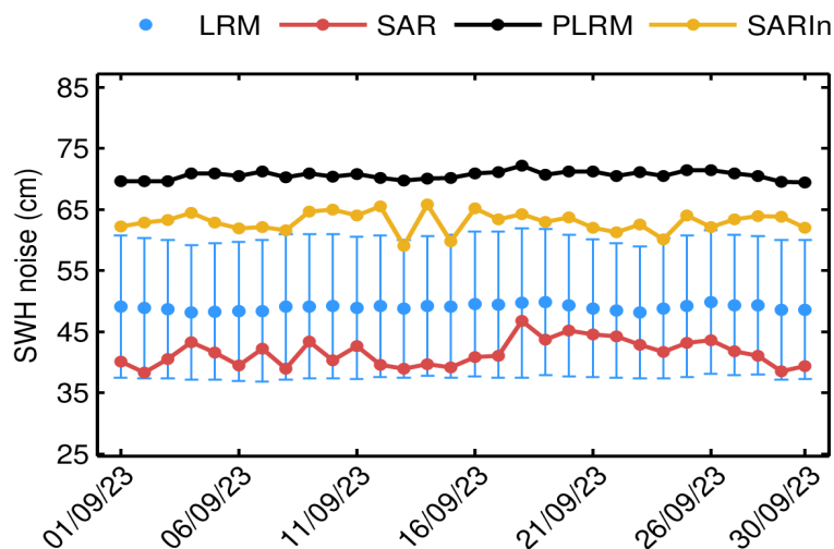
Figure 88. Mean science-valid GOP SWH noise for LRM (blue dot), SAR (red dot), PLRM (black dot) and SARIn (orange dot) for each day in September 2023. The corresponding standard deviation for LRM (blue error bar) is also shown.
