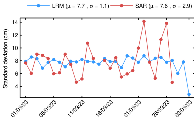
Figure 14. Standard deviation of differences at crossovers for NOP SSH anomaly for each day in September 2023. The values shown in this figure have been computed for the science-valid data further edited according to the following two additional criteria: 1) rejecting crossover differences larger than 20 cm; and 2) rejecting shallow waters (1000 m). The mean ( \mu ) and standard deviation ( \sigma ) are also shown.
