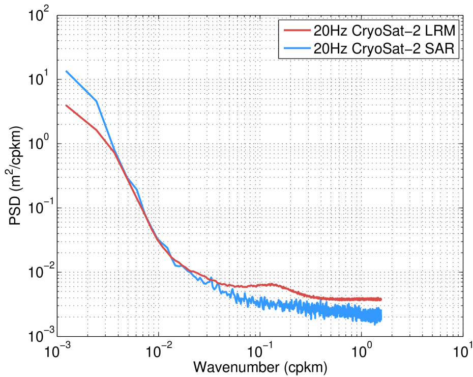
Figure 76. Along-track power spectrum density of the science-valid 20 Hz GOP SSH anomaly over oceans and lakes for LRM (red) and SAR (blue) for September 2023.
