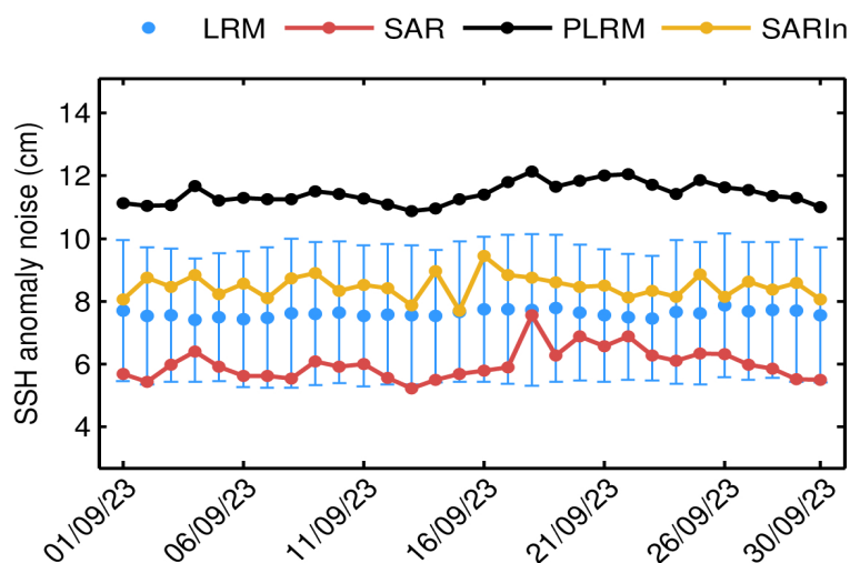
Figure 78. Mean science-valid GOP SSH anomaly noise for LRM (blue dot), SAR (red dot), PLRM (black dot) and SARIn (orange dot) for each day in September 2023. The corresponding standard deviation for LRM (blue error bar) is also shown.
