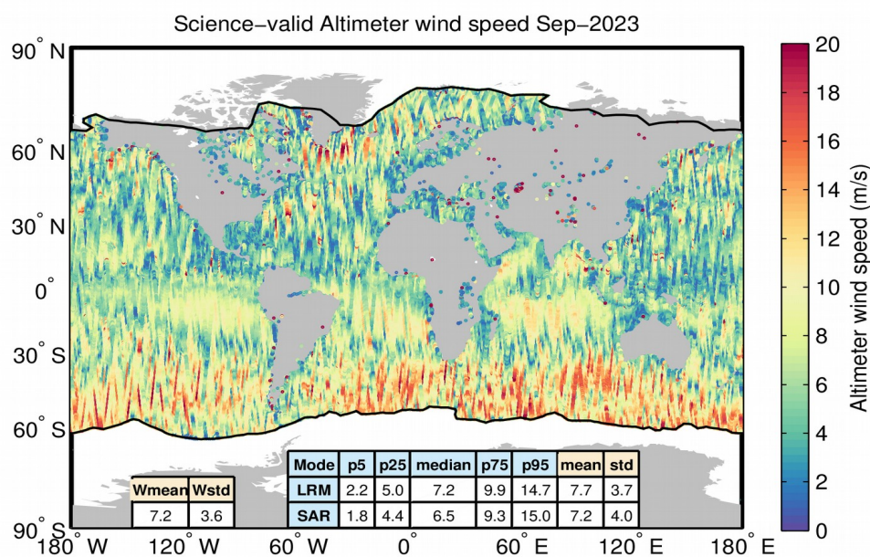
Figure 63. Geographical distribution of science-valid IOP wind data over oceans and lakes for September 2023. The statistical values shown in the table refer to the wind in m and are calculated separately for LRM and SAR regions. Wmean and Wstd denote the spatial area-weighted average and its standard deviation. Measurements taken over polar polygons have been excluded from the computation of the statistical values. The black lines mark the outer limit of the Arctic and Antarctic polar polygons.
