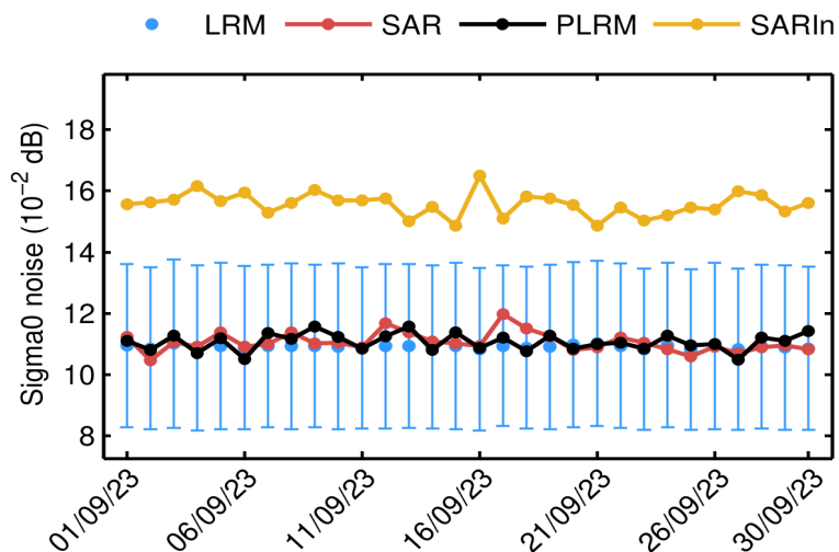
Figure 26. Mean science-valid NOP sigma0 noise for LRM (blue dot), SAR (red dot), PLRM (black dot) and SARIn (orange dot) for each day in September 2023. The corresponding standard deviation for LRM (blue error bar) is also shown.
