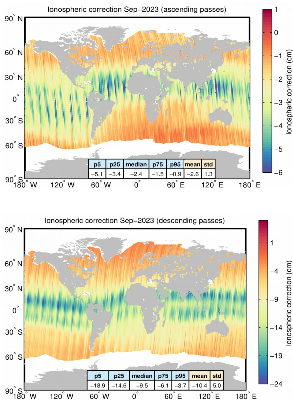
Figure A3. Geographical distribution of the Ionospheric correction over oceans and lakes for ascending (top) and descending (bottom) passes for September 2023. The statistical values shown in the table refer to the Ionospheric correction in cm. Measurements taken over polar polygons have been excluded from the computation of the statistical values. The black lines mark the outer limit of the Arctic and Antarctic polar polygons.
