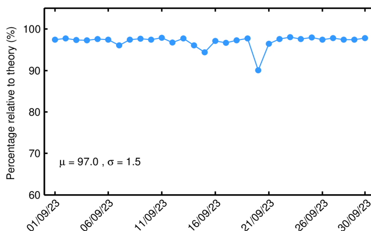
Figure 84. Percentage of science-valid GOP 1-Hz SWH records over ocean and lakes relative to theory for each day in September 2023. The mean ( \mu ) and standard deviation ( \sigma ) are also shown.
