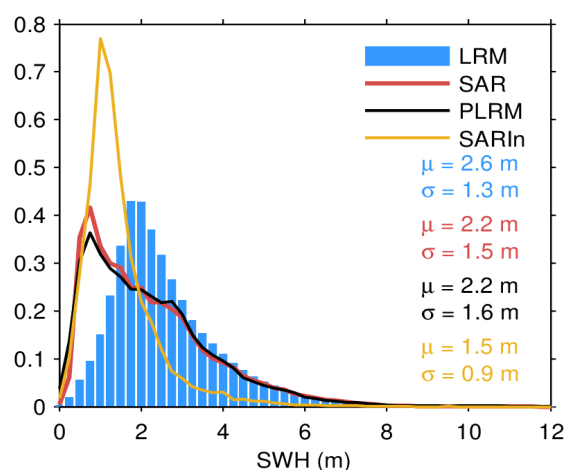
Figure 86. Histogram of science-valid GOP SWH over oceans and lakes for LRM (blue), SAR (red), PLRM (black) and SARIn (orange) and for September 2023. The mean ( \mu ) and standard deviation ( \sigma ) are also shown. Values larger than 12 m are excluded from the histogram for the sake of readability but not from the computation of \mu and \sigma .
