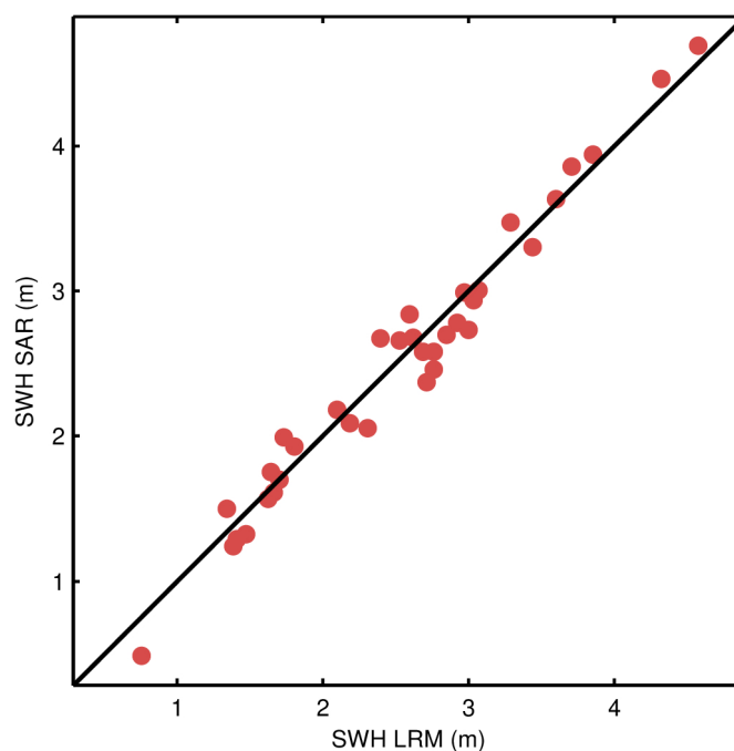
Figure 21. Scatter plot of the science-valid NOP SWH at the two nearest points outside (LRM, x-axis) and inside (SAR, y-axis) the Pacific SAR mode box for each pass. The RMS of the differences is 16.8 cm for the pairs shown in the figure as compared to a RMS of 14.7 cm for the differences between such outside points and their respective nearest neighbour also outside the box in the LRM region.
