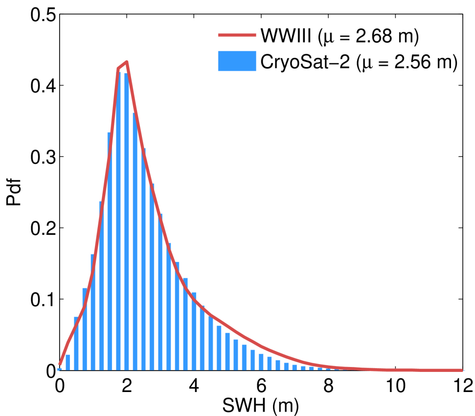
Figure 118. Histograms (normalized to have a total area of 1) of the GOP SWH (blue bars) and the SWH from the Wavewatch III model (red line) for September 2023.
