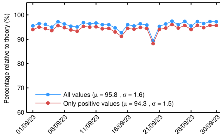
Figure 66. Percentage of science-valid IOP 1-Hz mispointing records over ocean and lakes relative to theory for each day in September 2023. The mean ( \mu ) and standard deviation ( \sigma ) are also shown.
