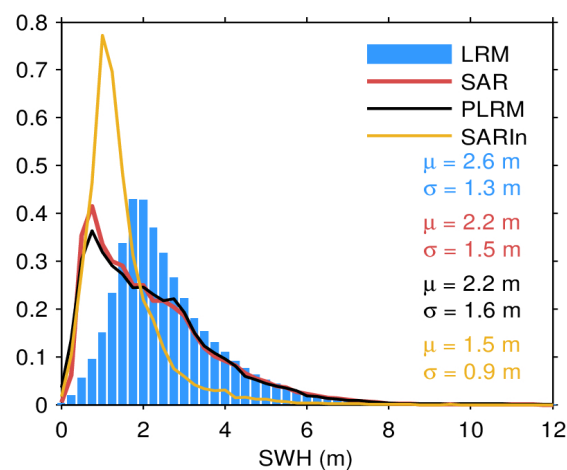
Figure 51. Histogram of science-valid IOP SWH over oceans and lakes for LRM (blue), SAR (red), PLRM (black) and SARIn (orange) for September 2023. The mean ( \mu ) and standard deviation ( \sigma ) are also shown. Values larger than 12 m are excluded from the histogram for the sake of readability but not from the computation of \mu and \sigma .
