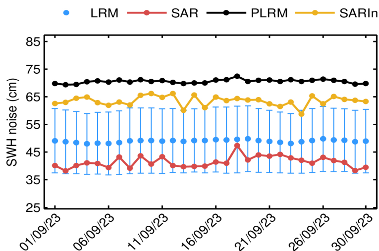
Figure 19. Mean science-valid NOP SWH noise for LRM (blue dot), SAR (red dot), PLRM (black dot) and SARIn (orange dot) for each day in September 2023. The corresponding standard deviation for LRM (blue error bar) is also shown.
