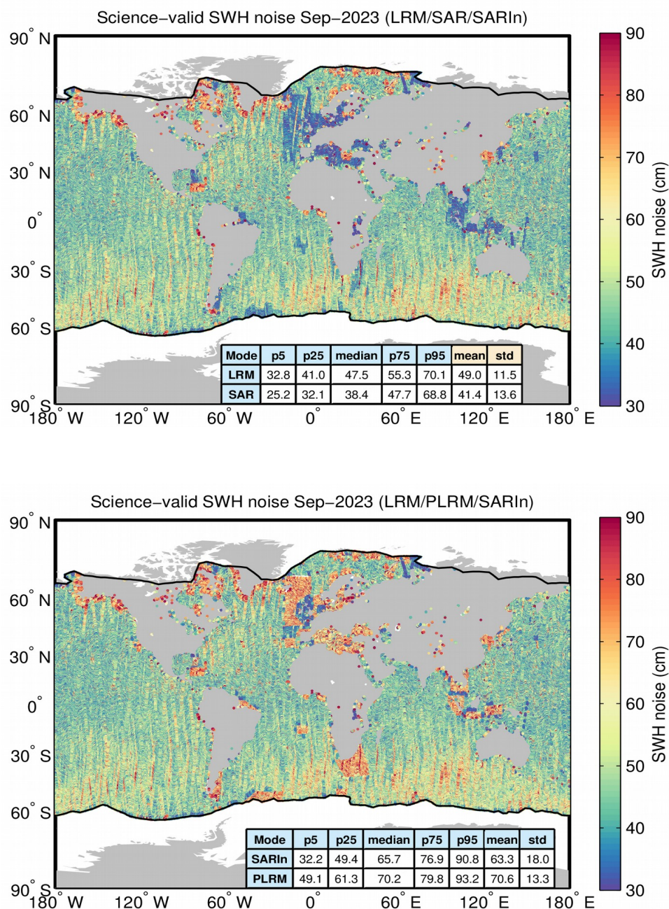
Figure 18. Geographical distribution of flag-valid 20-Hz SWH measurement noise over oceans and lakes for LRM/SAR/SARIn (top) and LRM/PLRM/SARIn (bottom) and for September 2023. The statistical values shown in the table refer to the SWH noise and are calculated separately for LRM, SAR/PLRM and SARIn regions. Measurements taken over polar polygons have been excluded from the computation of the statistical values. The black lines mark the outer limit of the Arctic and Antarctic polar polygons.
