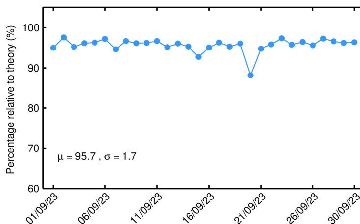
Figure 15. Percentage of science-valid NOP 1-Hz SWH records over ocean and lakes relative to theory for each day in September 2023. The mean ( \mu ) and standard deviation ( \sigma ) are also shown.
