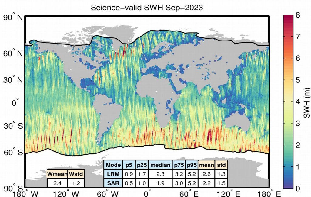
Figure 85. Geographical distribution of science-valid GOP SWH data over oceans and lakes for September 2023. The statistical values shown in the table refer to the SWH in m and are calculated separately for LRM and SAR regions. Wmean and Wstd denote the spatial area-weighted average and its standard deviation. Measurements taken over polar polygons have been excluded from the computation of the statistical values. The black lines mark the outer limit of the Arctic and Antarctic polar polygons.
