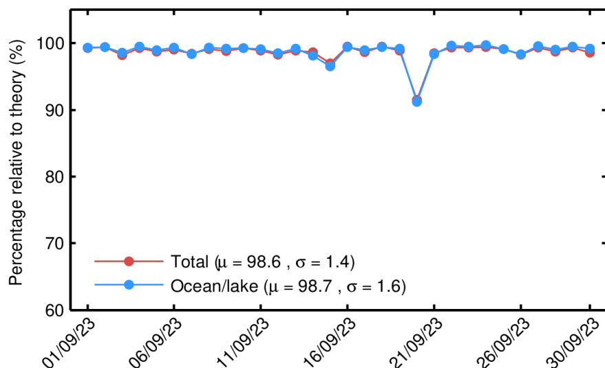
Figure 71. Percentage of GOP 1-Hz records over land and ocean/lake (red) and only over ocean/lake (blue) relative to the theoretically expected number from the orbits ground tracks for each day in September 2023.
