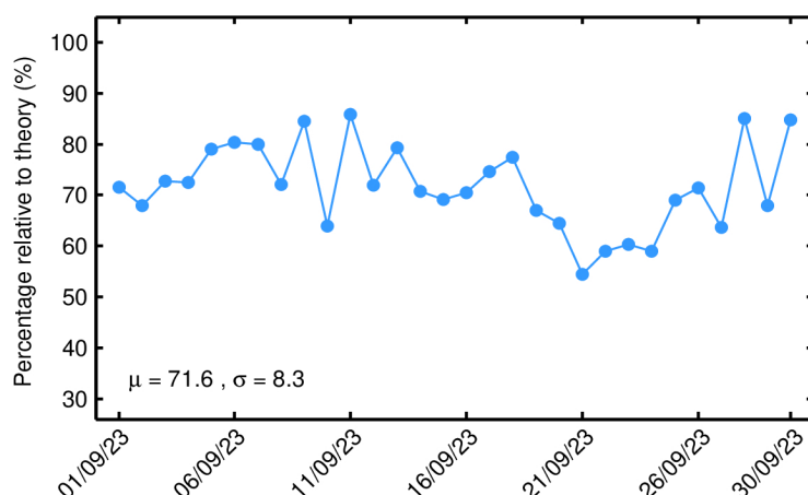
Figure 5. Percentage of science-valid NOP 1-Hz SSH records over ocean and lakes relative to theory for each day in September 2023. The mean ( \mu ) and standard deviation ( \sigma ) are also shown.
