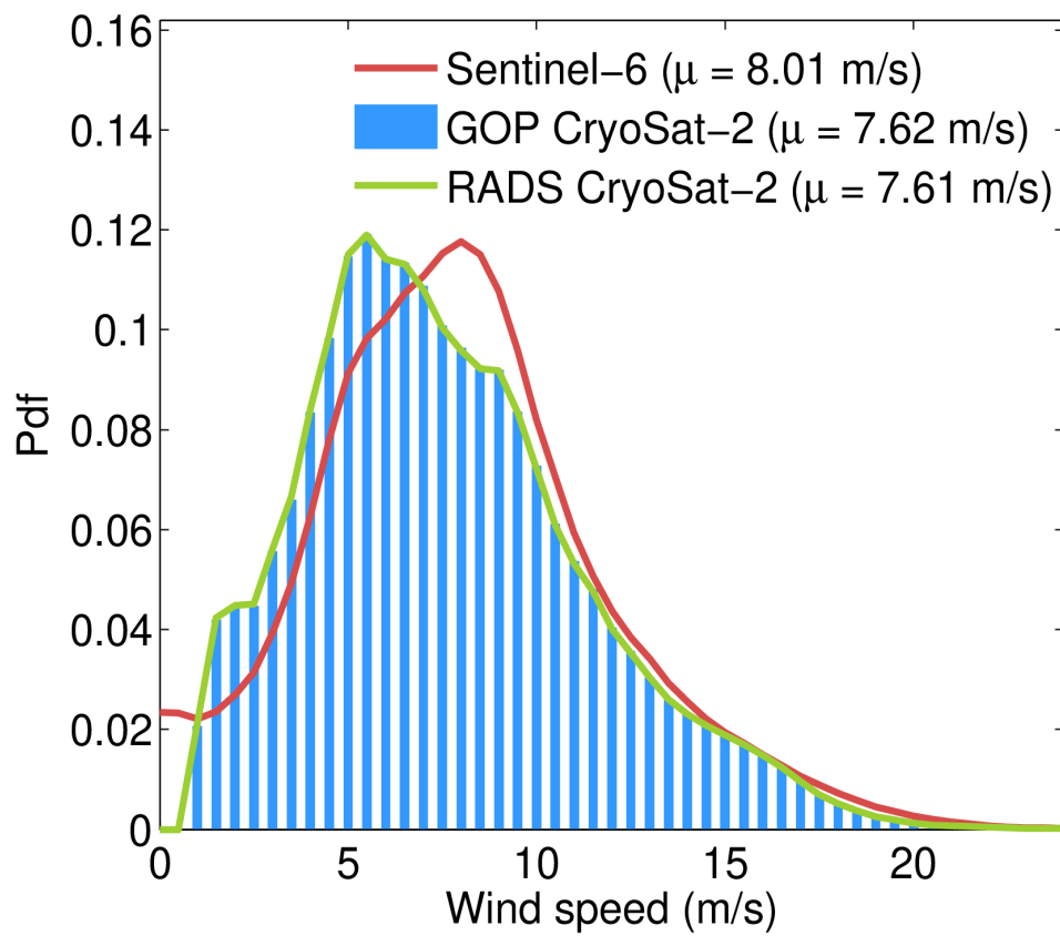
Figure 129. Histograms (normalized to have a total area of 1) of the wind speed from GOP (blue bars), reference mission (red line) and RADS CryoSat-2 (green) for September 2023.
