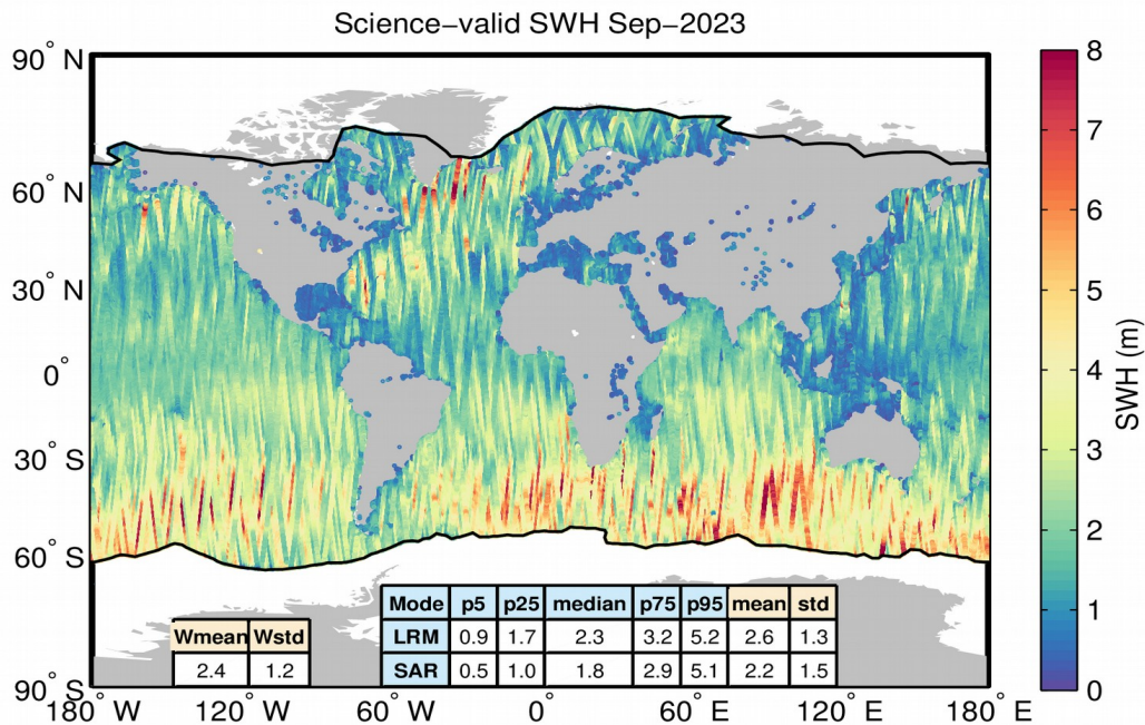
Figure 16. Geographical distribution of science-valid NOP SWH data over oceans and lakes for September 2023. The statistical values shown in the table refer to the SWH in m and are calculated separately for LRM and SAR regions. Wmean and Wstd denote the spatial area-weighted average and its standard deviation. Measurements taken over polar polygons have been excluded from the computation of the statistical values. The black lines mark the outer limit of the Arctic and Antarctic polar polygons.
