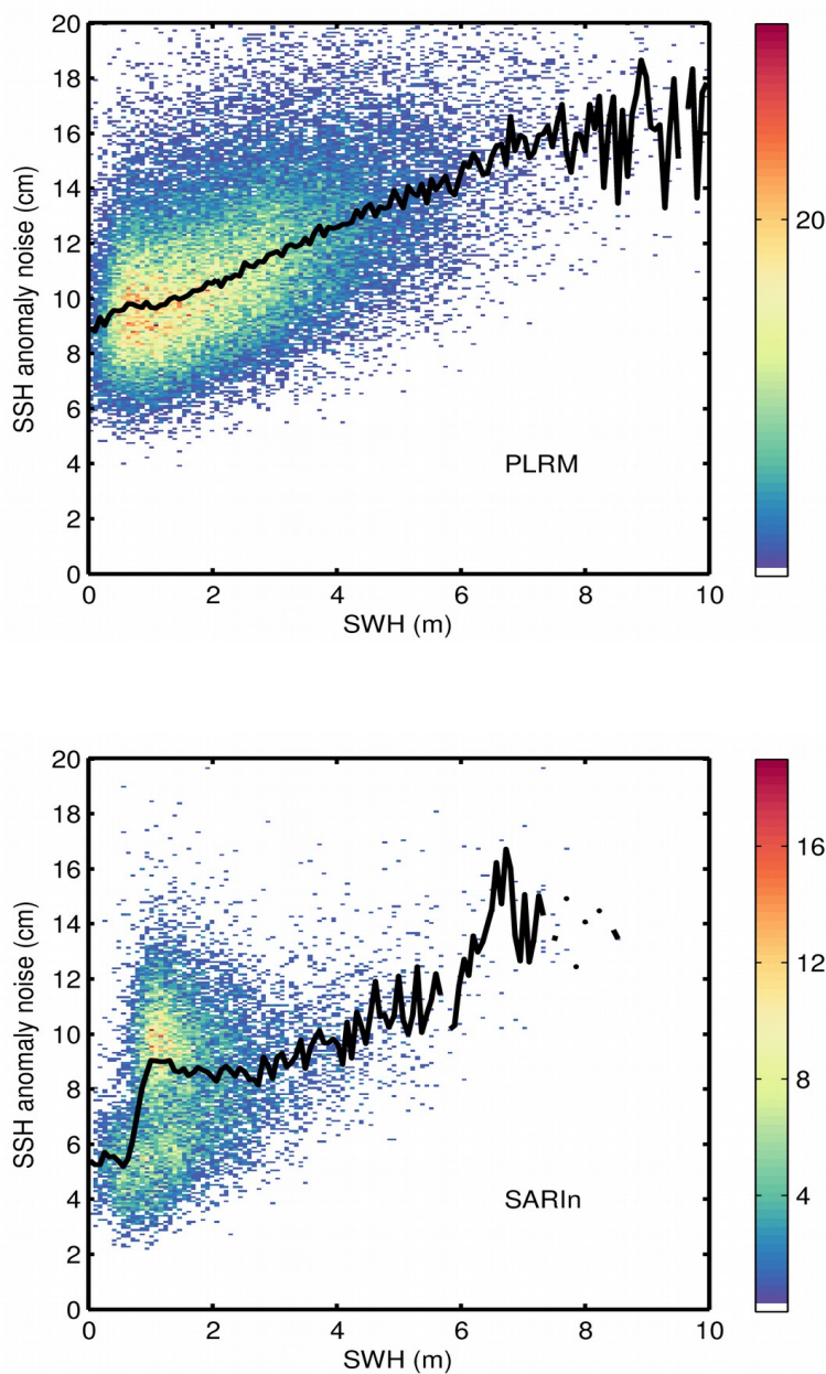
Figure 45. 2D histogram showing science-valid IOP SSH anomaly noise as a function of SWH for SAR, LRM, PLRM, and SARIn (from top to bottom) for September 2023. The black line denotes the median SSH anomaly noise as a function of SWH.
