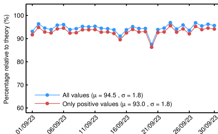
Figure 32. Percentage of science-valid NOP 1-Hz mispointing records over ocean and lakes relative to theory for each day in September 2023. The mean ( \mu ) and standard deviation ( \sigma ) are also shown.
