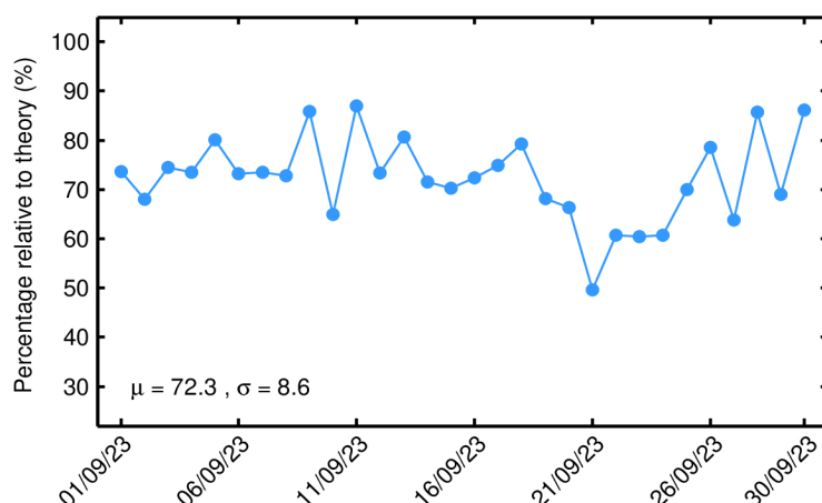
Figure 39. Percentage of science-valid IOP 1-Hz SSH records over ocean and lakes relative to theory for each day in September 2023. The mean ( \mu ) and standard deviation ( \sigma ) are also shown.
