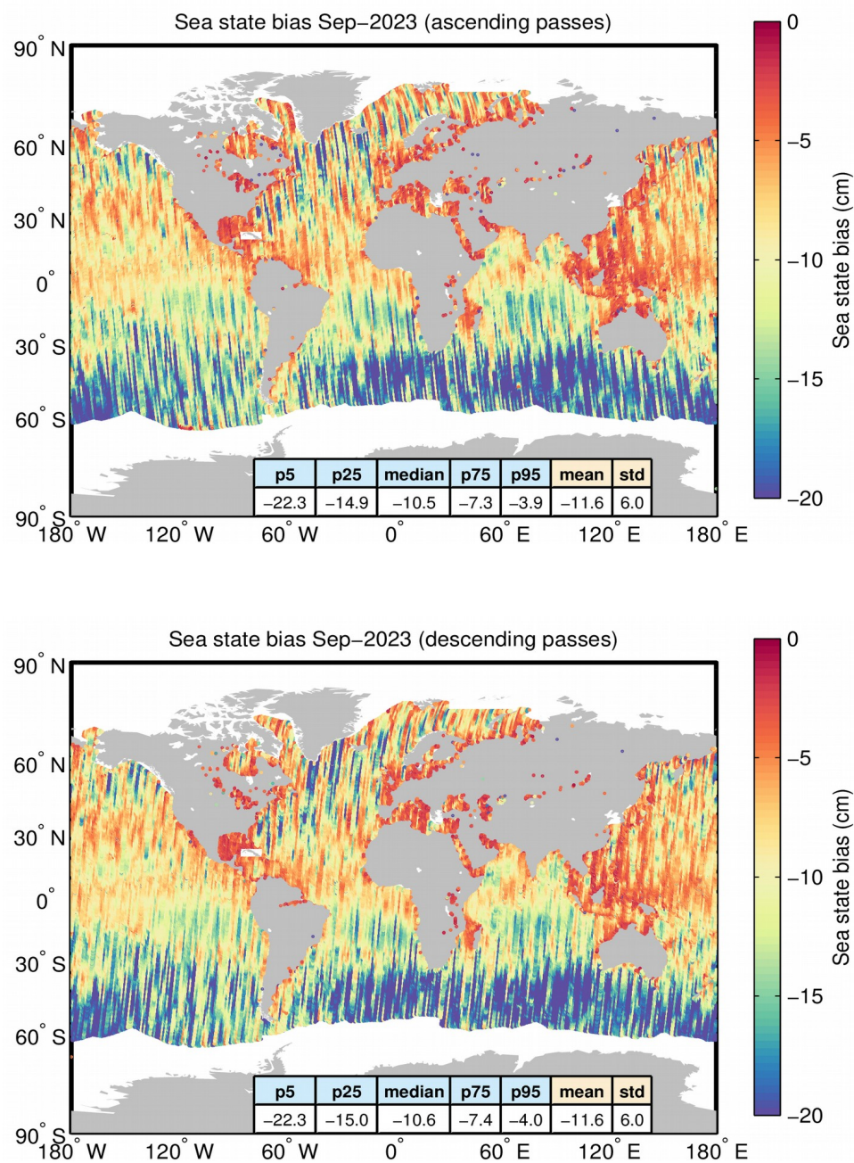
Figure A4. Geographical distribution of the sea state bias over oceans and lakes for ascending (top) and descending (bottom) passes for September 2023. The statistical values shown in the table refer to the sea state bias in cm. Measurements taken over polar polygons have been excluded from the computation of the statistical values. The black lines mark the outer limit of the Arctic and Antarctic polar polygons.
