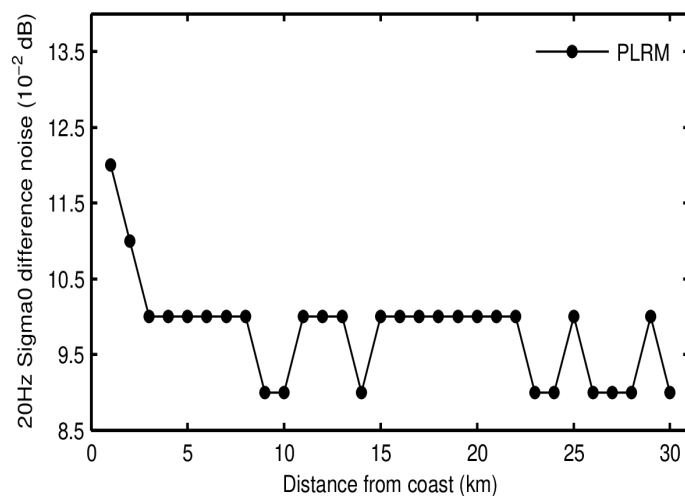
Figure 96. Science-valid GOP 20-Hz sigma0 noise as a function of distance from the coast for SAR (top panel), LRM (middle panel), and PLRM (bottom panel) for September 2023. Noise values have been calculated as the median of the absolute value of the difference between consecutive 20-Hz records.
