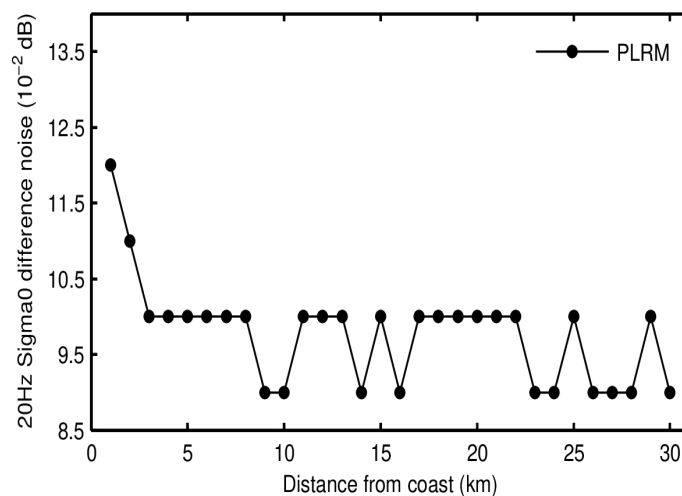
Figure 61. Science-valid IOP 20-Hz sigma0 noise as a function of distance from the coast for SAR (top panel), LRM (middle panel), and PLRM (bottom panel) for September 2023. Noise values have been calculated as the median of the absolute value of the difference between consecutive 20-Hz records.
