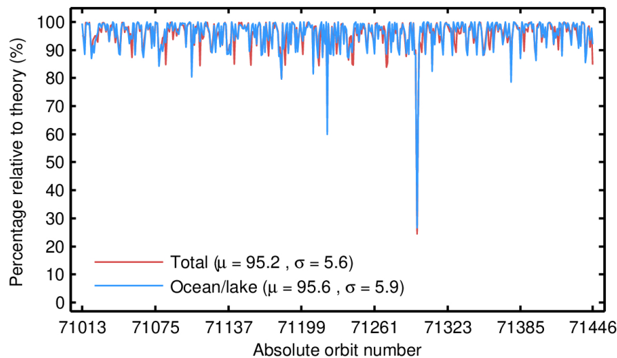
Figure 4. Percentage of NOP 1-Hz records over land and ocean/lake (red) and only over ocean/lake (blue) relative to the theoretically expected number from the orbits ground tracks for each orbit in September 2023. The mean ( \mu ) and standard deviation ( \sigma ) are also shown.
