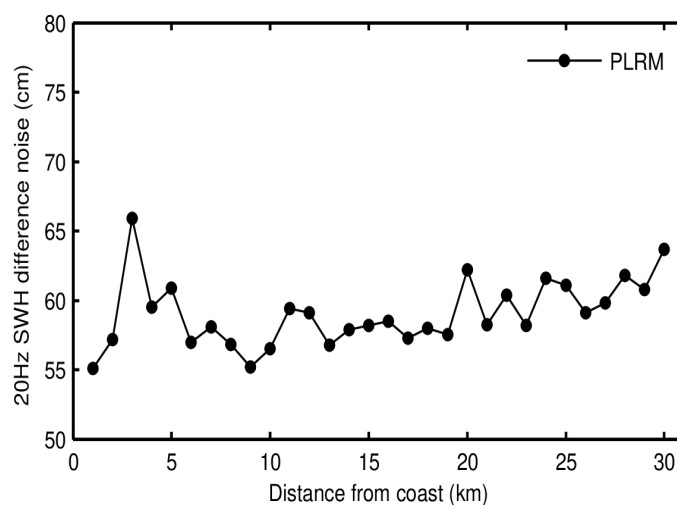
Figure 89. Science-valid GOP 20-Hz SWH noise as a function of distance from the coast for SAR (top panel), LRM (middle panel), and PLRM (bottom panel) for September 2023. Noise values have been calculated as the median of the absolute value of the difference between consecutive 20-Hz records.
