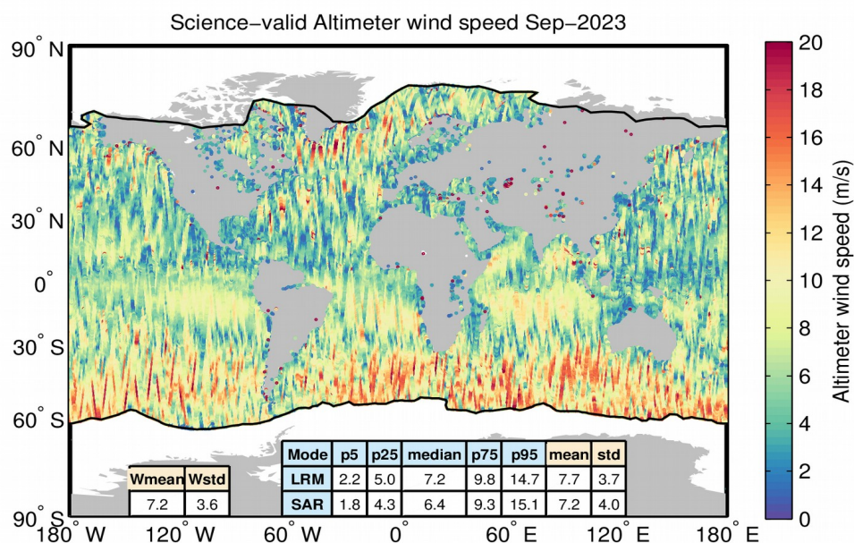
Figure 29. Geographical distribution of science-valid NOP wind data over oceans and lakes for September 2023. The statistical values shown in the table refer to the wind in m and are calculated separately for LRM and SAR regions. Wmean and Wstd denote the spatial area-weighted average and its standard deviation. Measurements taken over polar polygons have been excluded from the computation of the statistical values. The black lines mark the outer limit of the Arctic and Antarctic polar polygons.
