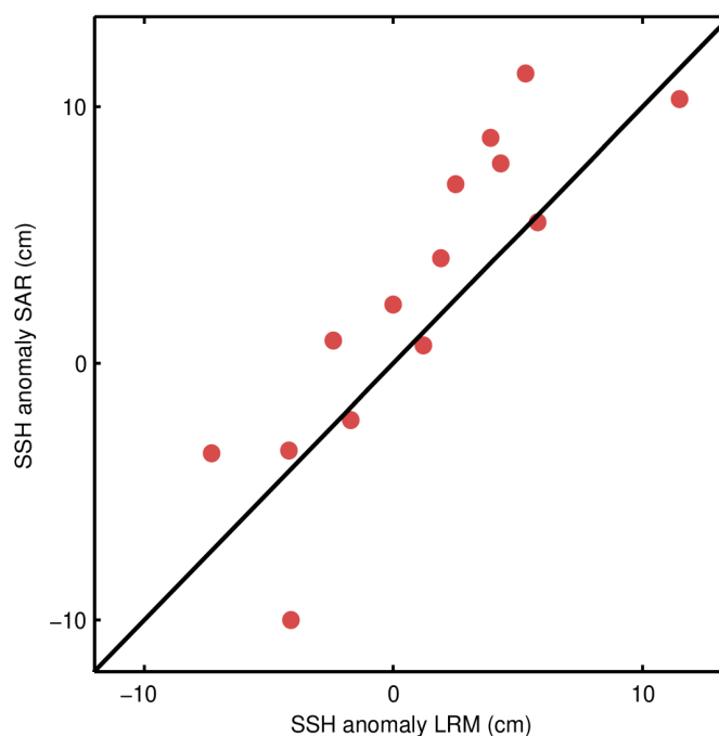
Figure 81. Scatter plot of the science-valid GOP SSH anomaly at the two nearest points outside (LRM, x-axis) and inside (SAR, y-axis) the Pacific SAR mode box for each pass.
