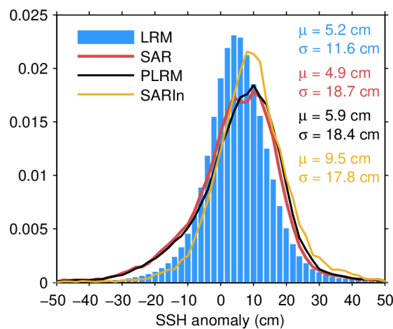
Figure 41. Histogram of science-valid IOP SSH anomaly over oceans and lakes for LRM (blue), SAR (red), PLRM (black) and SARIn (orange) for September 2023. The mean ( \mu ) and standard deviation ( \sigma ) are also shown. Values outside [-50, 50] cm are excluded from the histogram for the sake of readability but not from the computation of \mu and \sigma .
