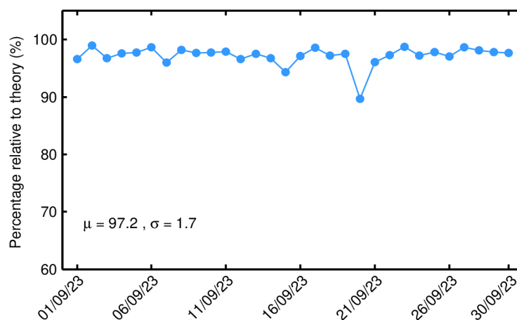
Figure 28. Percentage of science-valid NOP 1-Hz wind records over ocean and lakes relative to theory for each day in September 2023. The mean ( \mu ) and standard deviation ( \sigma ) are also shown.
