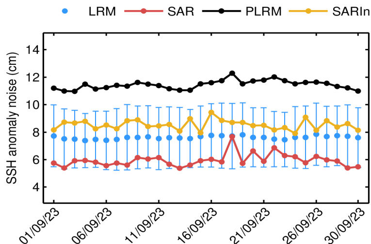
Figure 9. Mean science-valid NOP SSH anomaly noise for LRM (blue dot), SAR (red dot), PLRM (black dot) and SARIn (orange dot) for each day in September 2023. The corresponding standard deviation for LRM (blue error bar) is also shown.
