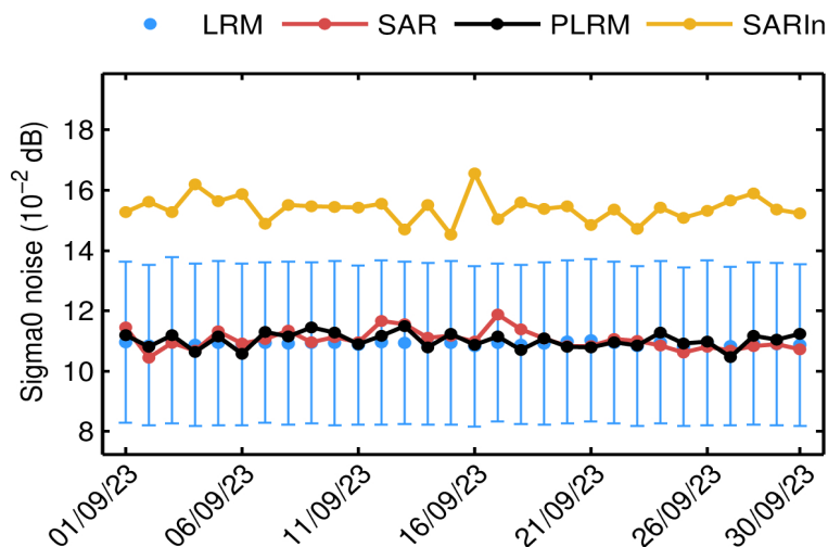
Figure 60. Mean science-valid IOP sigma0 noise for LRM (blue dot), SAR (red dot), PLRM (black dot) and SARIn (orange dot) for each day in September 2023. The corresponding standard deviation for LRM (blue error bar) is also shown.
