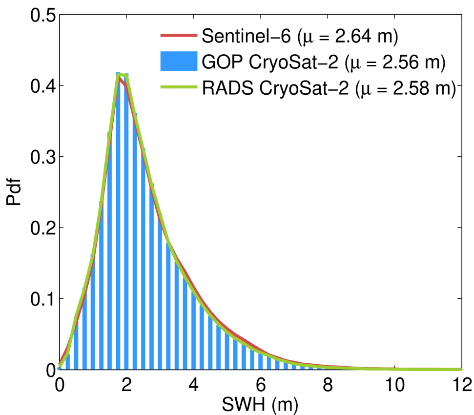
Figure 128. Histograms (normalized to have a total area of 1) of the SWH from GOP (blue bars), reference mission (red line) and RADS CryoSat-2 (green) for September 2023.
