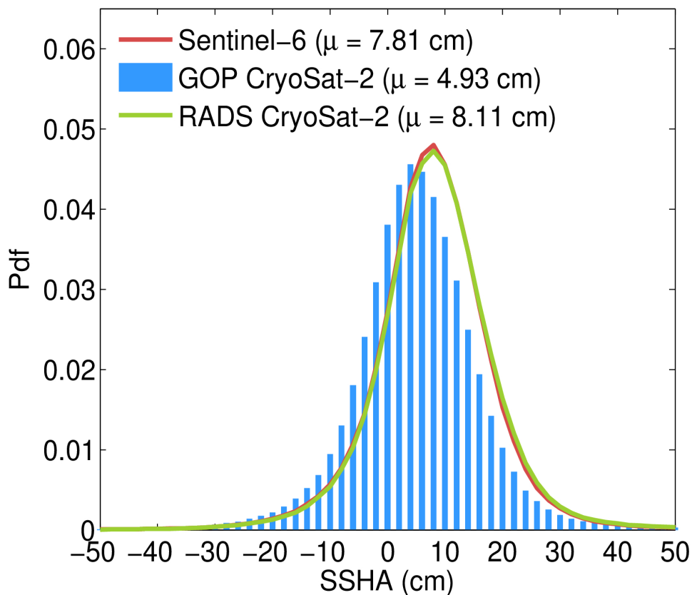
Figure 127. Histograms (normalized to have a total area of 1) of the SSH anomaly from GOP (blue bars), reference mission (red line) and RADS CryoSat-2 (green) for September 2023.
