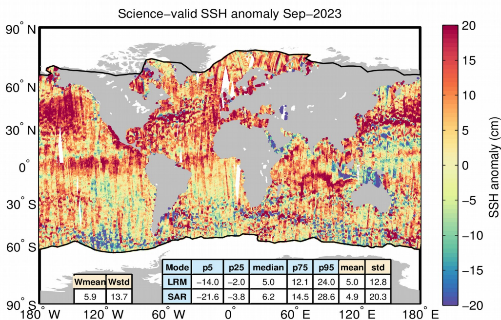
Figure 6. Geographical distribution of science-valid NOP 1-Hz SSH anomaly data over oceans and lakes for September 2023. The statistical values shown in the table refer to the SSH anomaly in cm and are calculated separately for LRM and SAR regions. Wmean and Wstd denote the spatial area-weighted average and its standard deviation. Measurements taken over polar polygons have been excluded from the computation of the statistical values. The black lines mark the outer limit of the Arctic and Antarctic polar polygons.
