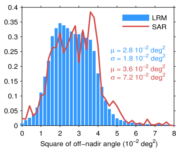
Figure 103. Histogram of science-valid GOP mispointing over oceans and lakes for LRM (blue) and SAR (red) for September 2023. The mean ( \mu ) and standard deviation ( \sigma ) are also shown. Note that values larger than 12 m are excluded from the histogram for the sake of readability but not from the computation of \mu and \sigma .
