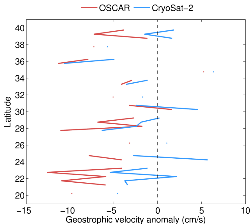
Figure 121. Comparison of the GOP geostrophic velocity anomalies with geostrophic velocities anomalies from the Ocean Surface Current Analyses – Real time (OSCAR) for September 2023 in the Atlantic (top, 20°N – 40°N, 315°E – 325°E) and Pacific (bottom, 20°N – 40°N, 220°E – 230°E) boxes as a function of latitude (i.e., for each latitude the geostrophic velocities have been averaged over the longitudes within the box). GOP geostrophic velocities have been computed using the optimal difference operator by Powell and Leben (2004).
