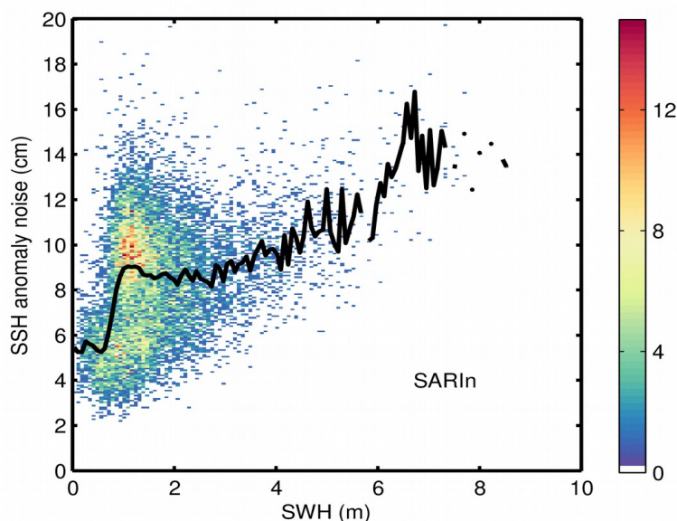
Figure 80. 2D histogram showing science-valid GOP SSH anomaly noise as a function of SWH for SAR, LRM, PLRM, and SARIn (from top to bottom) for September 2023. The black line denotes the median SSH anomaly noise as a function of SWH.
