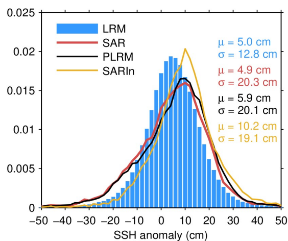
Figure 7. Histogram of science-valid NOP SSH anomaly over oceans and lakes for LRM (blue), SAR (red), PLRM (black) and SARIn (orange) for September 2023. The mean ( \mu ) and standard deviation ( \sigma ) are also shown. Values outside [-50\ 50] cm are excluded from the histogram for the sake of readability but not from the computation of \mu and \sigma .
