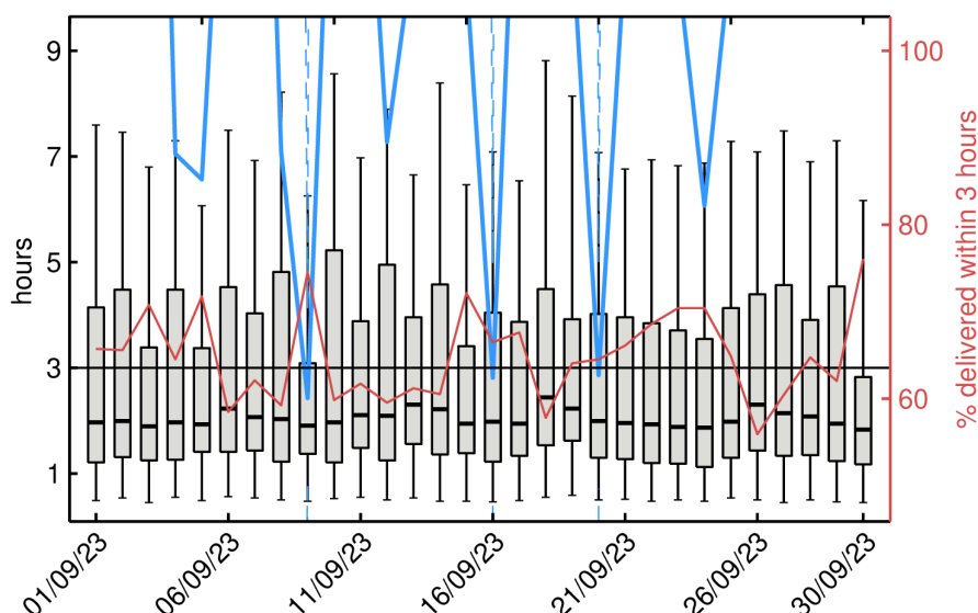
Figure 1. Box-and-whiskers plot for the NOP latency showing for each day in September 2023 the first and third quartiles (bottom and top of the box), the median (thick black), the
