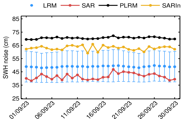
Figure 53. Mean science-valid IOP SWH noise for LRM (blue dot), SAR (red dot), PLRM (black dot) and SARIn (orange dot) for each day in September 2023. The corresponding standard deviation for LRM (blue error bar) is also shown.
