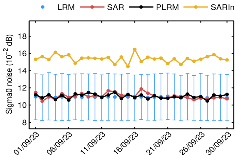
Figure 95. Mean science-valid GOP sigma0 noise for LRM (blue dot), SAR (red dot), PLRM (black dot) and SARIn (orange dot) for each day in September 2023. The corresponding standard deviation for LRM (blue error bar) is also shown.
