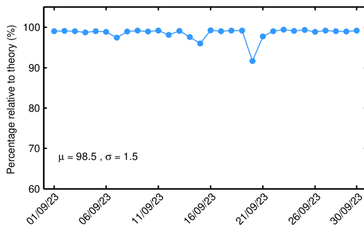
Figure 97. Percentage of science-valid GOP 1-Hz wind records over ocean and lakes relative to theory for each day in September 2023. The mean ( \mu ) and standard deviation ( \sigma ) are also shown.
