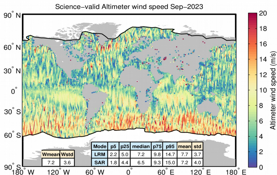
Figure 98. Geographical distribution of science-valid GOP wind data over oceans and lakes for September 2023. The statistical values shown in the table refer to the wind in m and are calculated separately for LRM and SAR regions. Wmean and Wstd denote the spatial area-weighted average and its standard deviation. Measurements taken over polar polygons have been excluded from the computation of the statistical values. The black lines mark the outer limit of the Arctic and Antarctic polar polygons.
