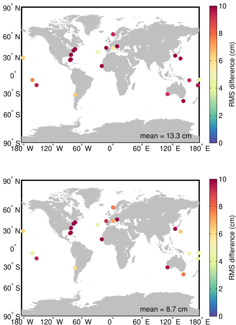
Figure 107. Map showing the RMS difference between the GOP SSH anomaly and the sea level from tide gauge records over the period October 2021 to September 2023 for the cases with (top) and without (bottom) the tidal component. For this comparison the atmospheric component has not been subtracted.
