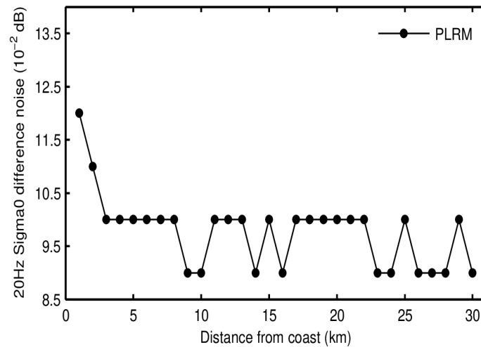
Figure 27. Science-valid NOP 20-Hz sigma0 noise as a function of distance from the coast for SAR (top panel), LRM (middle panel), and PLRM (bottom panel) for September 2023. Noise values have been calculated as the median of the absolute value of the difference between consecutive 20-Hz records.
