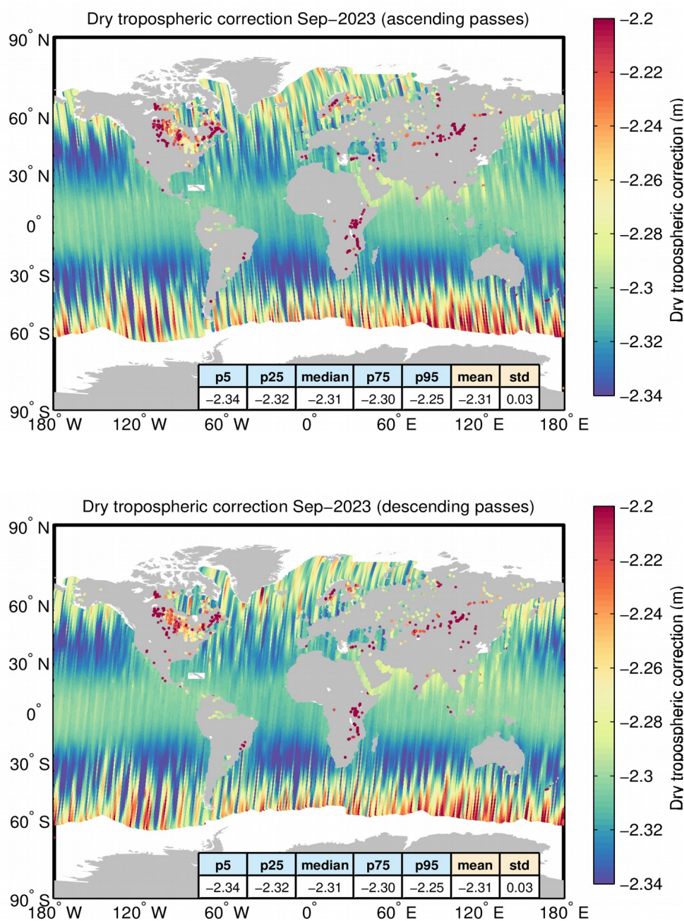
Figure A2. Geographical distribution of the dry tropospheric correction over oceans and lakes for ascending (top) and descending (bottom) passes for September 2023. The statistical values shown in the table refer to the dry tropospheric correction in m. Measurements taken over polar polygons have been excluded from the computation of the statistical values. The black lines mark the outer limit of the Arctic and Antarctic polar polygons.
