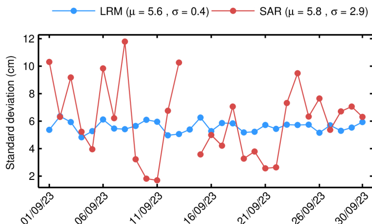
Figure 48. Standard deviation of differences at crossovers for IOP SSH anomaly for each day in September 2023. The values shown in this figure have been computed for the science-valid data further edited according to the following two additional criteria: 1) rejecting crossover differences larger than 20 cm; and 2) rejecting shallow waters (1000 m). The mean ( \mu ) and standard deviation ( \sigma ) are also shown.
