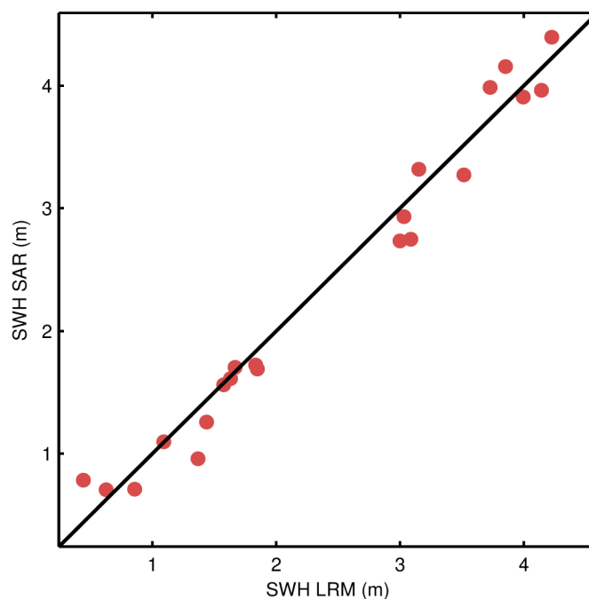
Figure 55. Scatter plot of the science-valid IOP SWH at the two nearest points outside (LRM, x-axis) and inside (SAR, y-axis) the Pacific SAR mode box for each pass. The RMS of the differences is 20.6 cm for the pairs shown in the figure as compared to a RMS of 16.4 cm for the differences between such outside points and their respective nearest neighbour also outside the box in the LRM region.
