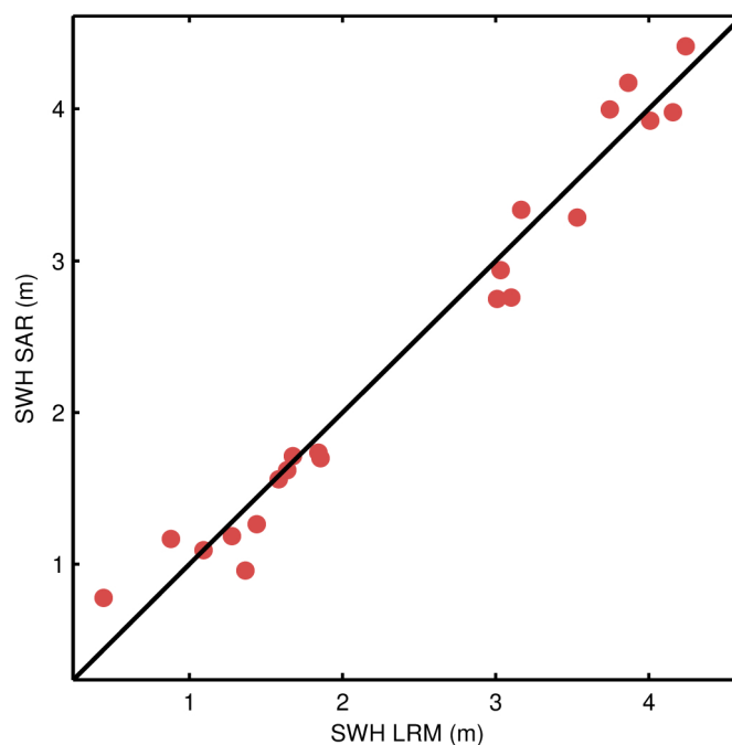
Figure 90. Scatter plot of the science-valid GOP SWH at the two nearest points outside (LRM, x-axis) and inside (SAR, y-axis) the Pacific SAR mode box for each pass. The RMS of the differences is 21.4 cm for the pairs shown in the figure as compared to a RMS of 16.1 cm for the differences between such outside points and their respective nearest neighbour also outside the box in the LRM region.
