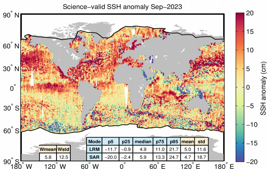
Figure 74. Geographical distribution of science-valid GOP 1-Hz SSH anomaly data over oceans and lakes for September 2023. The statistical values shown in the table refer to the SSH anomaly in cm and are calculated separately for LRM and SAR regions. Wmean and Wstd denote the spatial area-weighted average and its standard deviation. Measurements taken over polar polygons have been excluded from the computation of the statistical values. The black lines mark the outer limit of the Arctic and Antarctic polar polygons.
