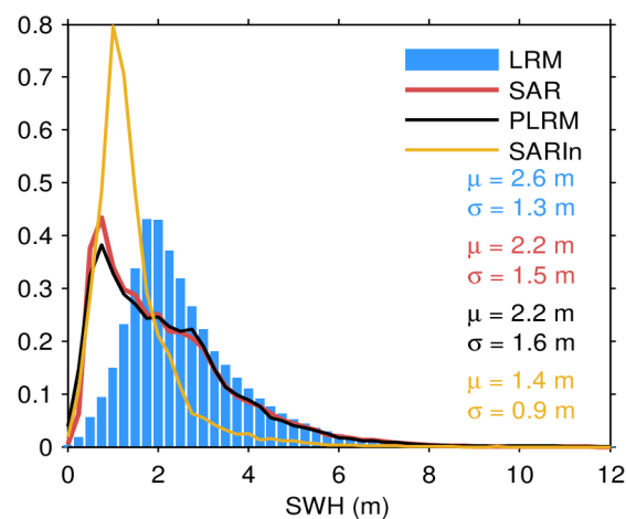
Figure 17. Histogram of science-valid NOP SWH over oceans and lakes for LRM (blue), SAR (red), PLRM (black) and SARIn (orange) for September 2023. The mean ( \mu ) and standard deviation ( \sigma ) are also shown. Values larger than 12 m are excluded from the histogram for the sake of readability but not from the computation of \mu and \sigma .
