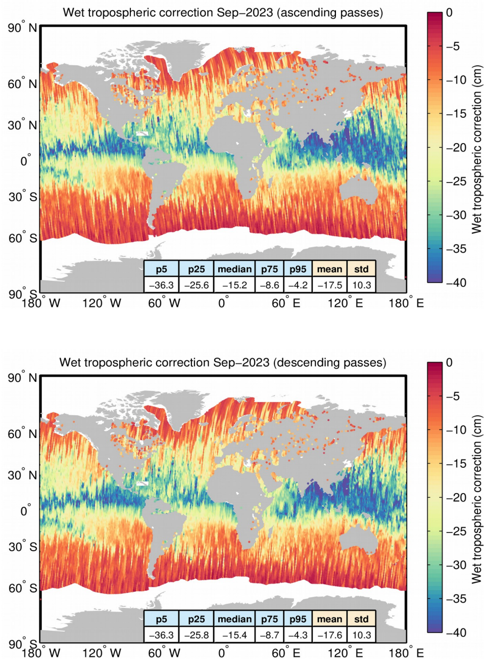
Figure A1. Geographical distribution of the wet tropospheric correction over oceans and lakes for ascending (top) and descending (bottom) passes for September 2023. The statistical values shown in the table refer to the wet tropospheric correction in cm. Measurements taken over polar polygons have been excluded from the computation of the statistical values. The black lines mark the outer limit of the Arctic and Antarctic polar polygons.
