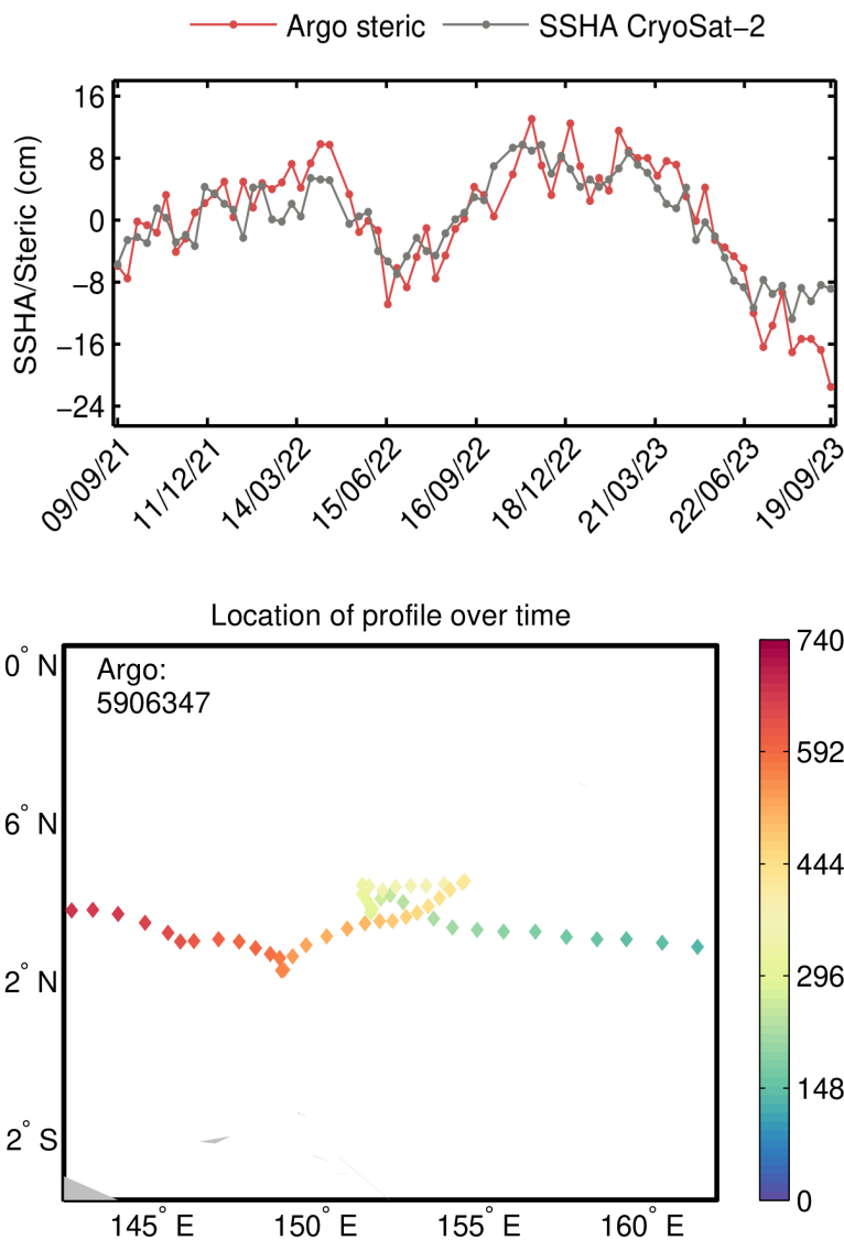
Figure 125. Comparison of the GOP SSH anomaly and the steric height anomaly (referred to 1000 m) for one particular Argo float (top). The location of the Argo float over time is also shown (bottom).
