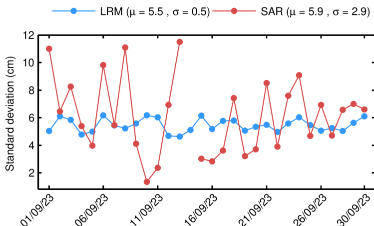
Figure 83. Standard deviation of differences at crossovers for GOP SSH anomaly for each day in September 2023. The values shown in this figure have been computed for the science-valid data further edited according to the following two additional criteria: 1) rejecting crossover differences larger than 20 cm; and 2) rejecting shallow waters (1000 m). The mean ( \mu ) and standard deviation ( \sigma ) are also shown.
