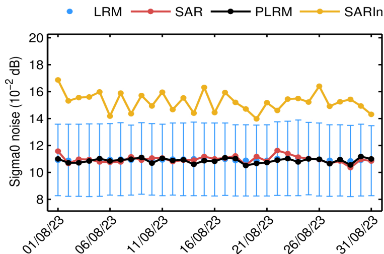
Figure 95. Mean science-valid GOP sigma0 noise for LRM (blue dot), SAR (red dot), PLRM (black dot) and SARIn (orange dot) for each day in August 2023. The corresponding standard deviation for LRM (blue error bar) is also shown.
