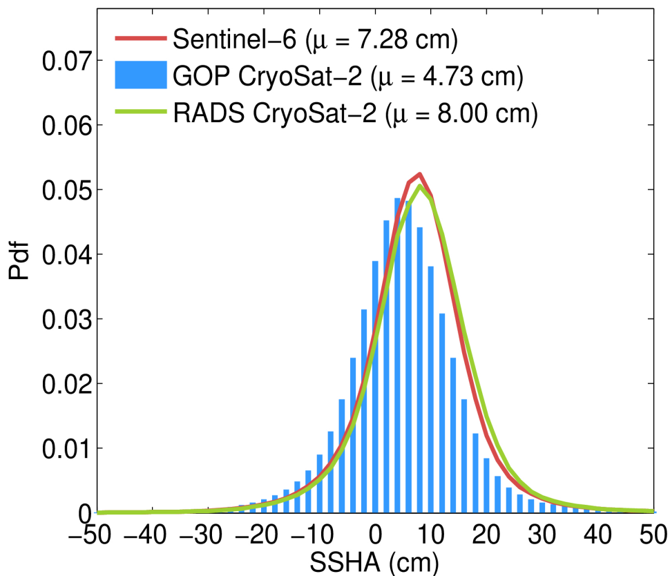
Figure 127. Histograms (normalized to have a total area of 1) of the SSH anomaly from GOP (blue bars), reference mission (red line) and RADS CryoSat-2 (green) for August 2023.
