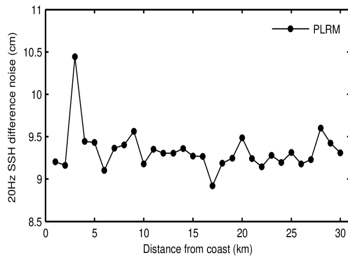
Figure 10. Science-valid NOP 20-Hz SSH anomaly noise as a function of distance from the coast for SAR (top panel), LRM (middle panel), and PLRM (bottom panel) for August 2023. Noise values have been calculated as the median of the absolute value of the difference between consecutive 20-Hz records.
