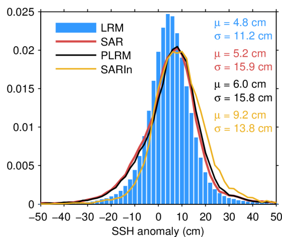
Figure 75. Histogram of science-valid GOP SSH anomaly over oceans and lakes for LRM (blue), SAR (red), PLRM (black) and SARIn (orange) for August 2023. The mean ( \mu ) and
