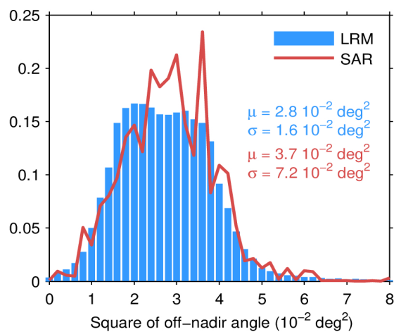
Figure 103. Histogram of science-valid GOP mispointing over oceans and lakes for LRM (blue) and SAR (red) for August 2023. The mean ( \mu ) and standard deviation ( \sigma ) are also shown. Note that values larger than 12 m are excluded from the histogram for the sake of readability but not from the computation of \mu and \sigma .
