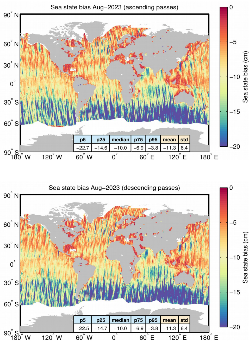
Figure A4. Geographical distribution of the sea state bias over oceans and lakes for ascending (top) and descending (bottom) passes for August 2023. The statistical values shown in the table refer to the sea state bias in cm. Measurements taken over polar polygons have been excluded from the computation of the statistical values. The black lines mark the outer limit of the Arctic and Antarctic polar polygons.
