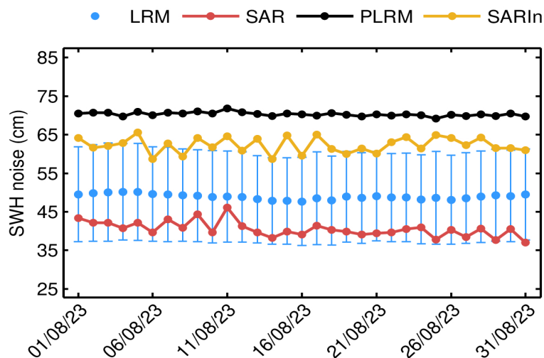
Figure 53. Mean science-valid IOP SWH noise for LRM (blue dot), SAR (red dot), PLRM (black dot) and SARIn (orange dot) for each day in August 2023. The corresponding standard deviation for LRM (blue error bar) is also shown.
