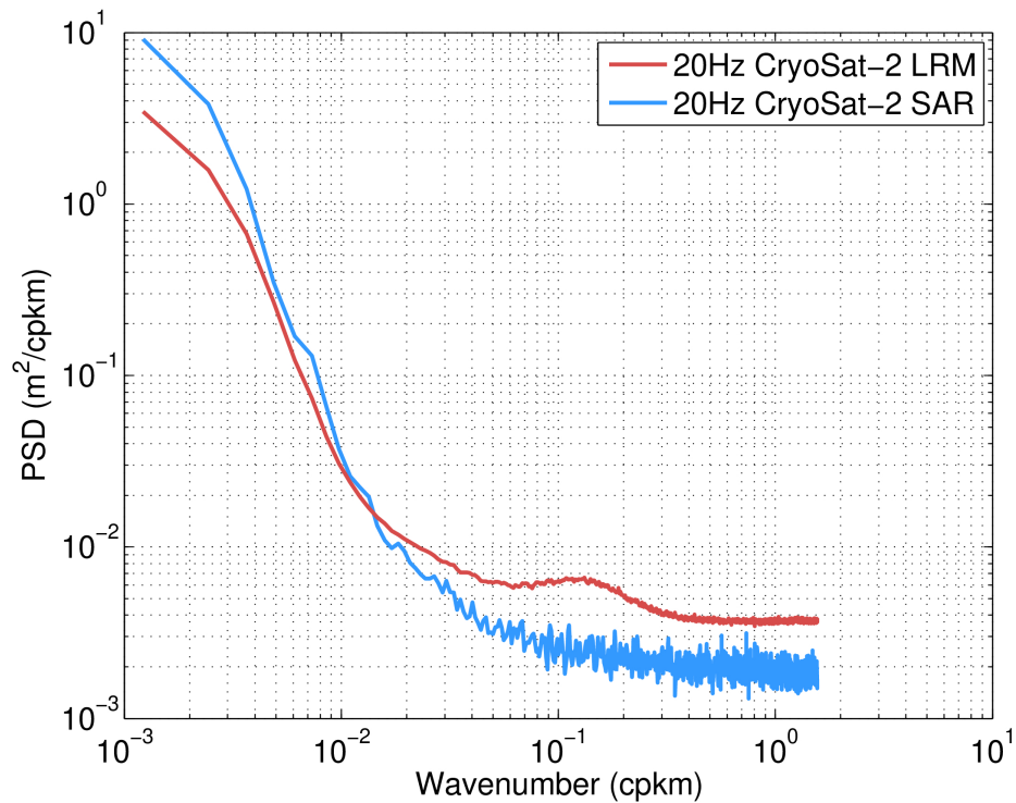
Figure 76. Along-track power spectrum density of the science-valid 20 Hz GOP SSH anomaly over oceans and lakes for LRM (red) and SAR (blue) for August 2023.
