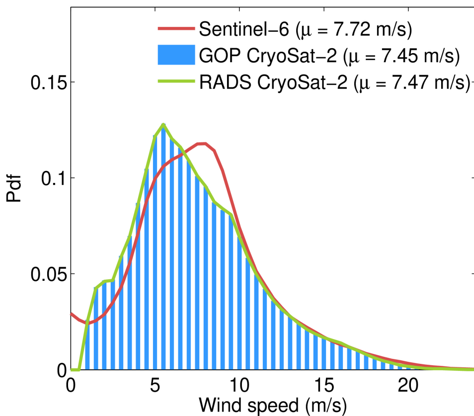
Figure 129. Histograms (normalized to have a total area of 1) of the wind speed from GOP (blue bars), reference mission (red line) and RADS CryoSat-2 (green) for August 2023.
