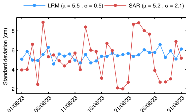
Figure 48. Standard deviation of differences at crossovers for IOP SSH anomaly for each day in August 2023. The values shown in this figure have been computed for the science-valid data further edited according to the following two additional criteria: 1) rejecting crossover differences larger than 20 cm; and 2) rejecting shallow waters (1000 m). The mean ( \mu ) and standard deviation ( \sigma ) are also shown.
