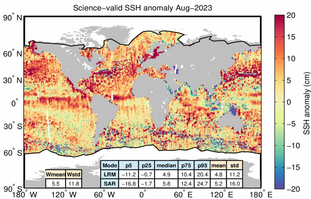
Figure 40. Geographical distribution of science-valid IOP 1-Hz SSH anomaly data over oceans and lakes for August 2023. The statistical values shown in the table refer to the SSH anomaly in cm and are calculated separately for LRM and SAR regions. Wmean and Wstd denote the spatial area-weighted average and its standard deviation. Measurements taken over polar polygons have been excluded from the computation of the statistical values. The black lines mark the outer limit of the Arctic and Antarctic polar polygons.
