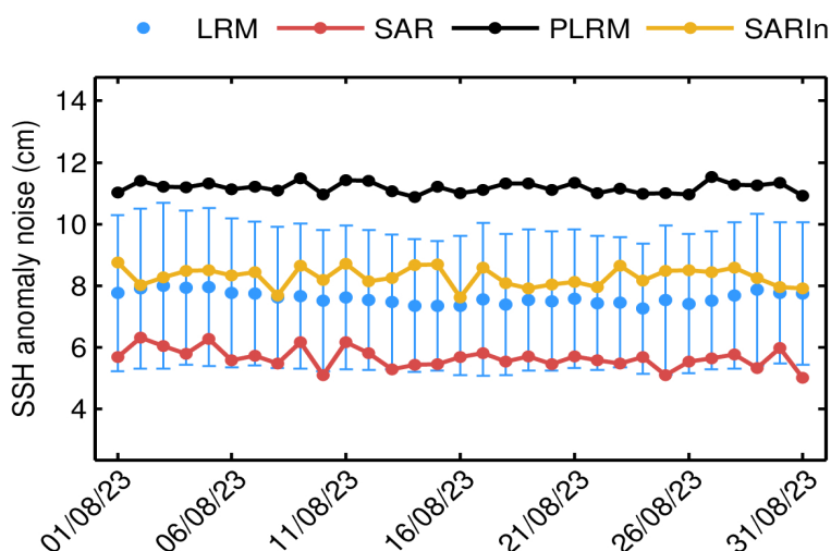
Figure 78. Mean science-valid GOP SSH anomaly noise for LRM (blue dot), SAR (red dot), PLRM (black dot) and SARIn (orange dot) for each day in August 2023. The corresponding standard deviation for LRM (blue error bar) is also shown.
