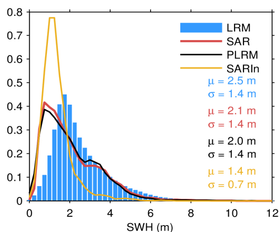
Figure 86. Histogram of science-valid GOP SWH over oceans and lakes for LRM (blue), SAR (red), PLRM (black) and SARIn (orange) and for August 2023. The mean ( \mu ) and standard deviation ( \sigma ) are also shown. Values larger than 12 m are excluded from the histogram for the sake of readability but not from the computation of \mu and \sigma .
