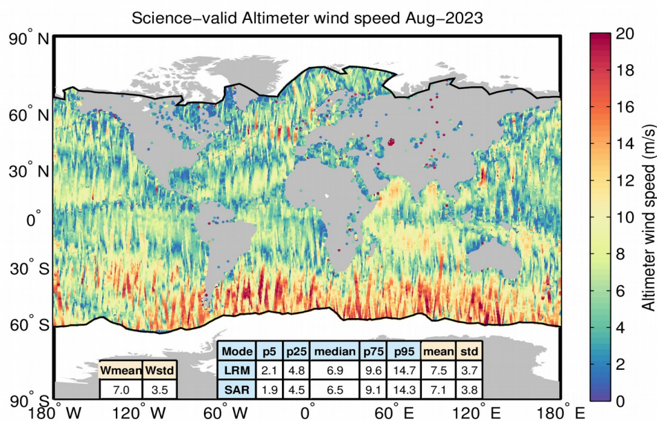
Figure 63. Geographical distribution of science-valid IOP wind data over oceans and lakes for August 2023. The statistical values shown in the table refer to the wind in m and are calculated separately for LRM and SAR regions. Wmean and Wstd denote the spatial area-weighted average and its standard deviation. Measurements taken over polar polygons have been excluded from the computation of the statistical values. The black lines mark the outer limit of the Arctic and Antarctic polar polygons.
