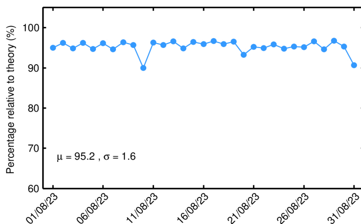
Figure 15. Percentage of science-valid NOP 1-Hz SWH records over ocean and lakes relative to theory for each day in August 2023. The mean ( \mu ) and standard deviation ( \sigma ) are also shown.
