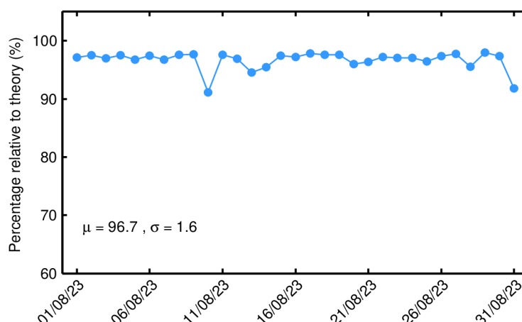
Figure 49. Percentage of science-valid IOP 1-Hz SWH records over ocean and lakes relative to theory for each day in August 2023. The mean ( \mu ) and standard deviation ( \sigma ) are also shown.
