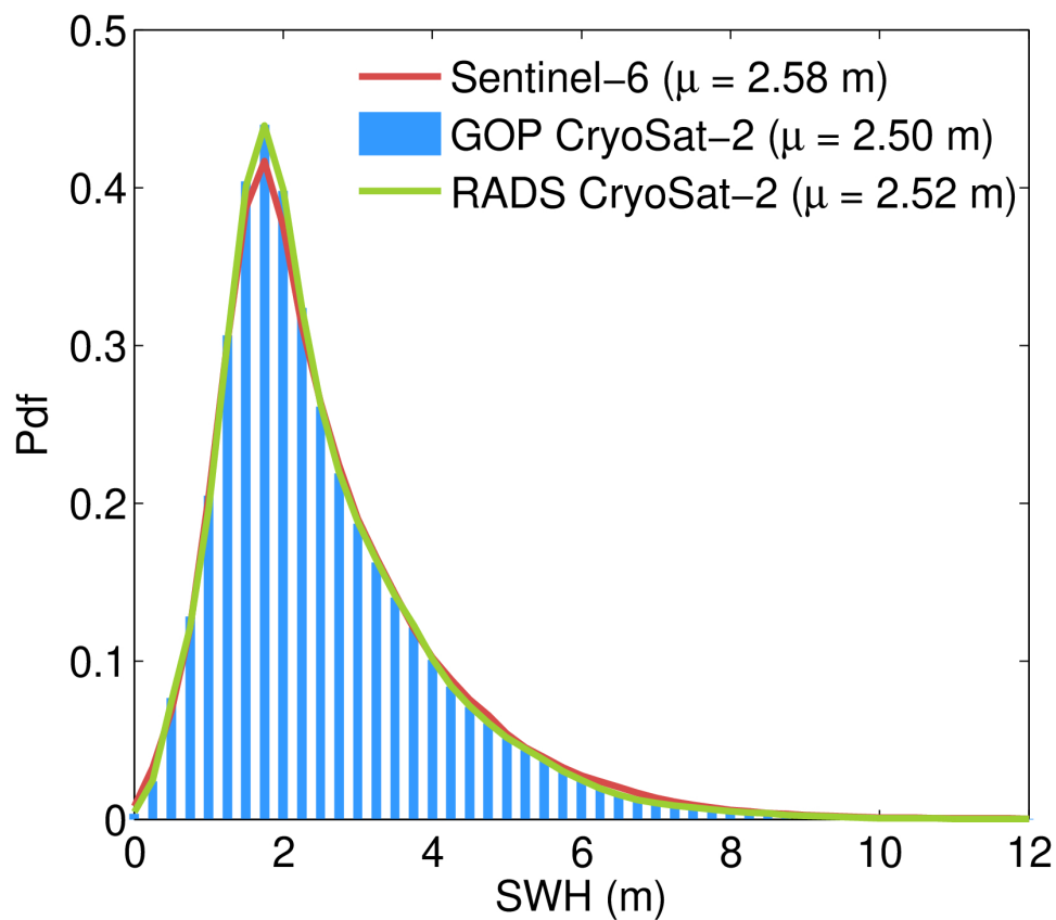
Figure 128. Histograms (normalized to have a total area of 1) of the SWH from GOP (blue bars), reference mission (red line) and RADS CryoSat-2 (green) for August 2023.
