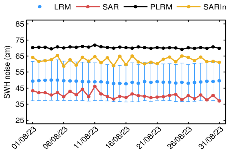
Figure 88. Mean science-valid GOP SWH noise for LRM (blue dot), SAR (red dot), PLRM (black dot) and SARIn (orange dot) for each day in August 2023. The corresponding standard deviation for LRM (blue error bar) is also shown.
