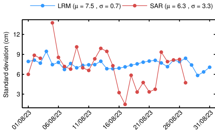
Figure 14. Standard deviation of differences at crossovers for NOP SSH anomaly for each day in August 2023. The values shown in this figure have been computed for the science-valid data further edited according to the following two additional criteria: 1) rejecting crossover differences larger than 20 cm; and 2) rejecting shallow waters (1000 m). The mean ( \mu ) and standard deviation ( \sigma ) are also shown.
