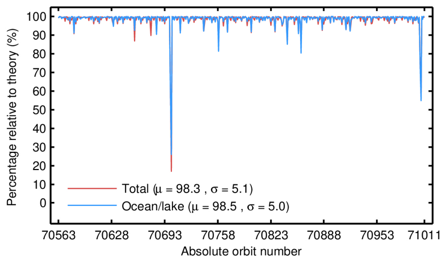
Figure 72. Percentage of GOP 1-Hz records over land and ocean/lake (red) and only over ocean/lake (blue) relative to the theoretically expected number from the orbits ground tracks for each orbit in August 2023. The mean ( \mu ) and standard deviation ( \sigma ) are also shown.
