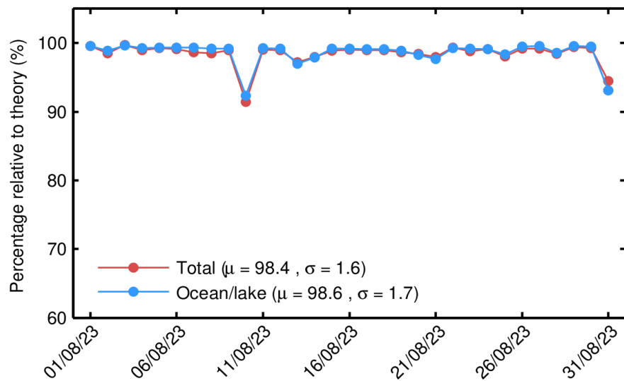
Figure 37. Percentage of IOP 1-Hz records over land and ocean/lake (red) and only over ocean/lake (blue) relative to the theoretically expected number from the orbits ground tracks for each day in August 2023.
