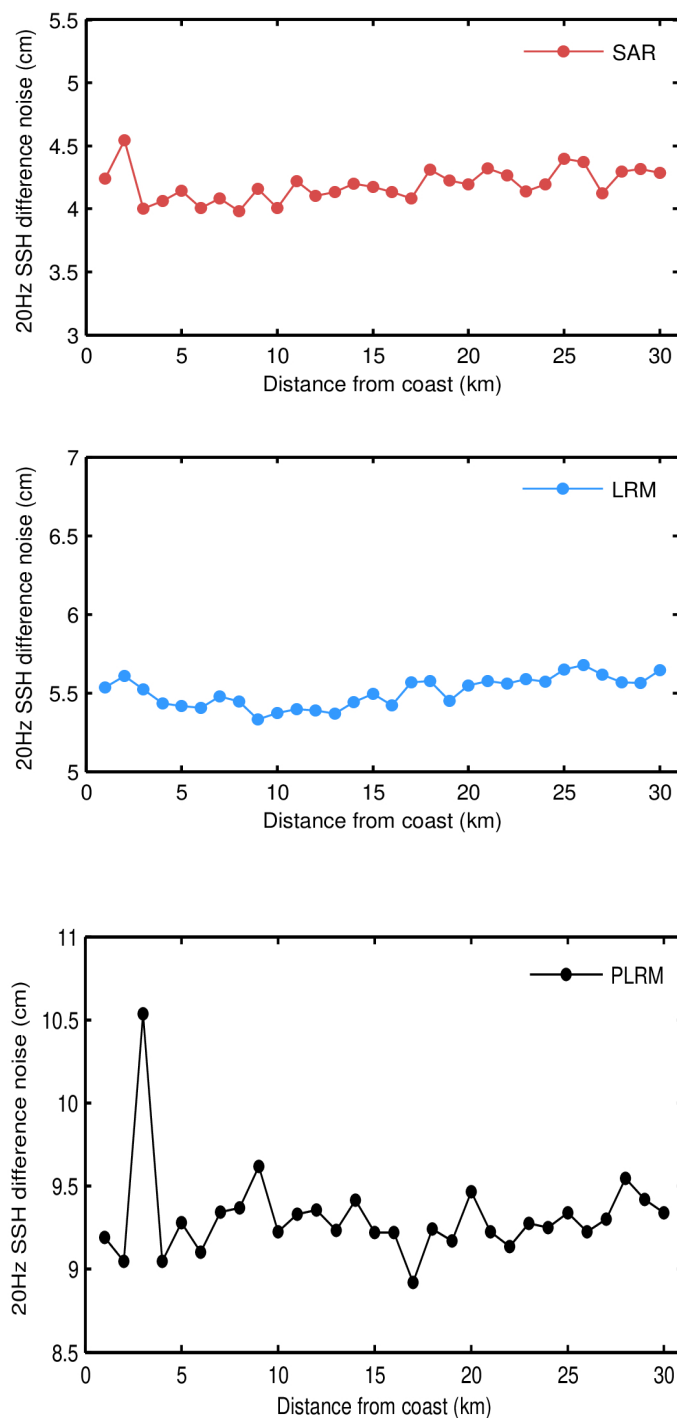
Figure 79. Science-valid GOP 20-Hz SSH anomaly noise as a function of distance from the coast for SAR (top panel), LRM (middle panel), and PLRM (bottom panel) for August 2023. Noise values have been calculated as the median of the absolute value of the difference between consecutive 20-Hz records.
