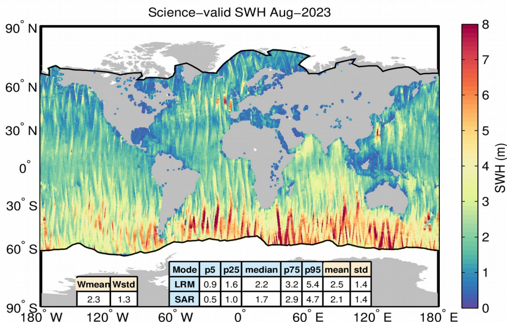
Figure 85. Geographical distribution of science-valid GOP SWH data over oceans and lakes for August 2023. The statistical values shown in the table refer to the SWH in m and are calculated separately for LRM and SAR regions. Wmean and Wstd denote the spatial area-weighted average and its standard deviation. Measurements taken over polar polygons have been excluded from the computation of the statistical values. The black lines mark the outer limit of the Arctic and Antarctic polar polygons.
