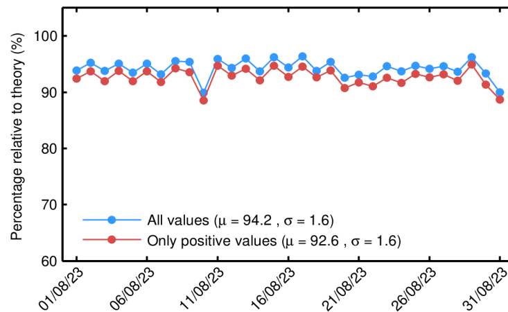
Figure 32. Percentage of science-valid NOP 1-Hz mispointing records over ocean and lakes relative to theory for each day in August 2023. The mean ( \mu ) and standard deviation ( \sigma ) are also shown.
