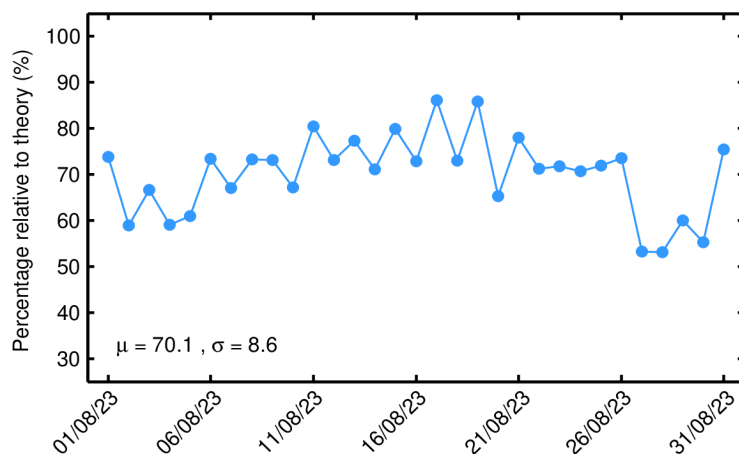
Figure 39. Percentage of science-valid IOP 1-Hz SSH records over ocean and lakes relative to theory for each day in August 2023. The mean ( \mu ) and standard deviation ( \sigma ) are also shown.
