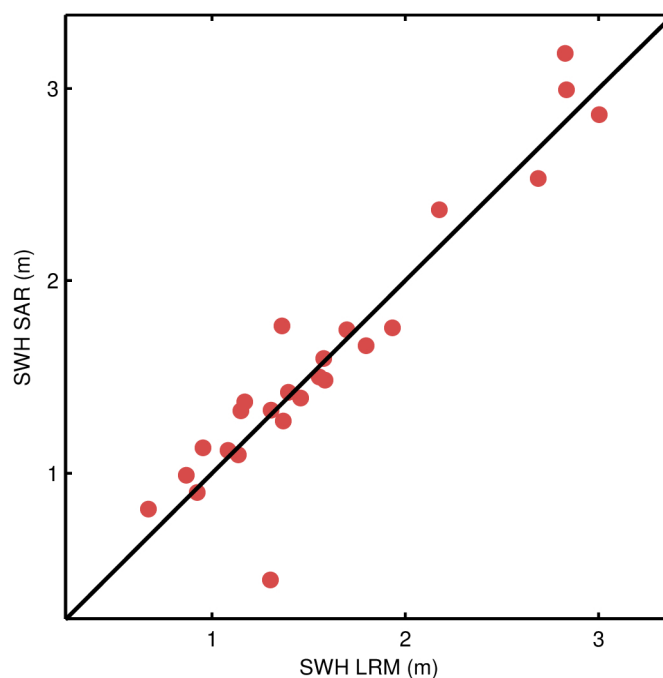
Figure 55. Scatter plot of the science-valid IOP SWH at the two nearest points outside (LRM, x-axis) and inside (SAR, y-axis) the Pacific SAR mode box for each pass. The RMS of the differences is 16.0 cm for the pairs shown in the figure as compared to a RMS of 13.7 cm for the differences between such outside points and their respective nearest neighbour also outside the box in the LRM region.
