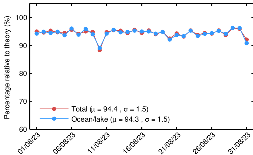
Figure 3. Percentage of NOP 1-Hz records over land and ocean/lake (red) and only over ocean/lake (blue) relative to the theoretically expected number from the orbits ground tracks for each day in August 2023.
