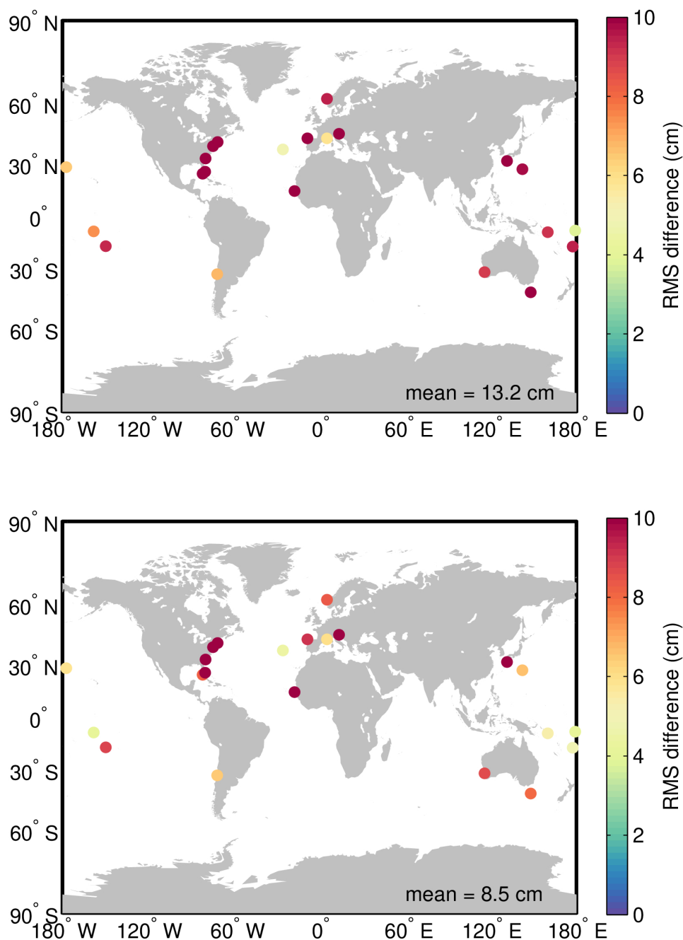
Figure 107. Map showing the RMS difference between the GOP SSH anomaly and the sea level from tide gauge records over the period September 2021 to August 2023 for the cases with (top) and without (bottom) the tidal component. For this comparison the atmospheric component has not been subtracted.
