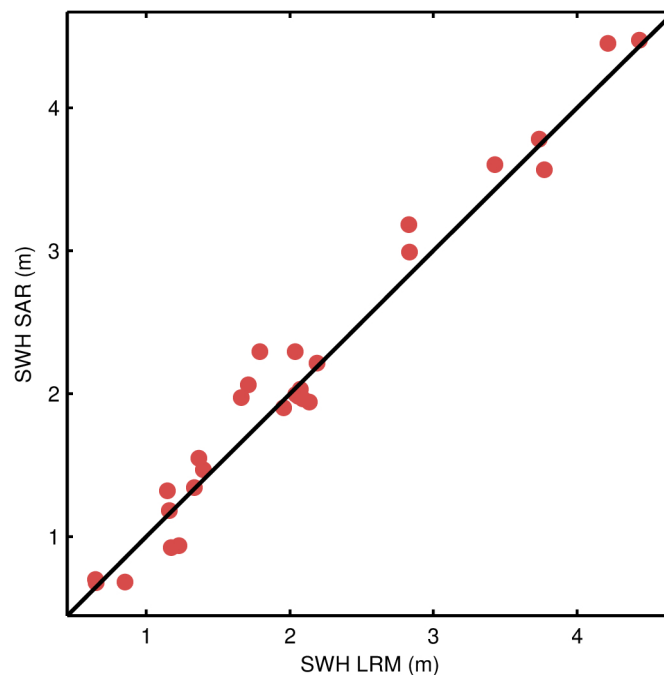
Figure 21. Scatter plot of the science-valid NOP SWH at the two nearest points outside (LRM, x-axis) and inside (SAR, y-axis) the Pacific SAR mode box for each pass. The RMS of the differences is 20.1 cm for the pairs shown in the figure as compared to a RMS of 15.6 cm for the differences between such outside points and their respective nearest neighbour also outside the box in the LRM region.
