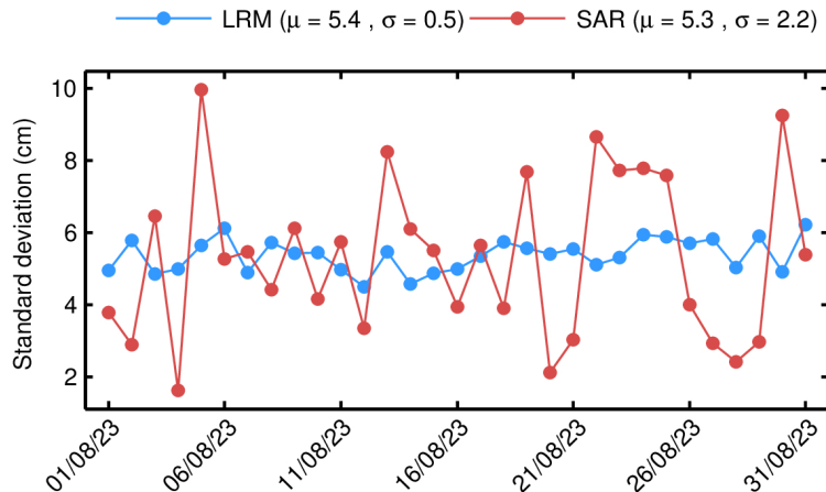
Figure 83. Standard deviation of differences at crossovers for GOP SSH anomaly for each day in August 2023. The values shown in this figure have been computed for the science-valid data further edited according to the following two additional criteria: 1) rejecting crossover differences larger than 20 cm; and 2) rejecting shallow waters (1000 m). The mean ( \mu ) and standard deviation ( \sigma ) are also shown.
