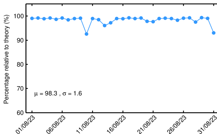
Figure 62. Percentage of science-valid IOP 1-Hz wind records over ocean and lakes relative to theory for each day in August 2023. The mean ( \mu ) and standard deviation ( \sigma ) are also shown.
