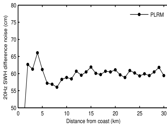
Figure 89. Science-valid GOP 20-Hz SWH noise as a function of distance from the coast for SAR (top panel), LRM (middle panel), and PLRM (bottom panel) for August 2023. Noise values have been calculated as the median of the absolute value of the difference between consecutive 20-Hz records.
