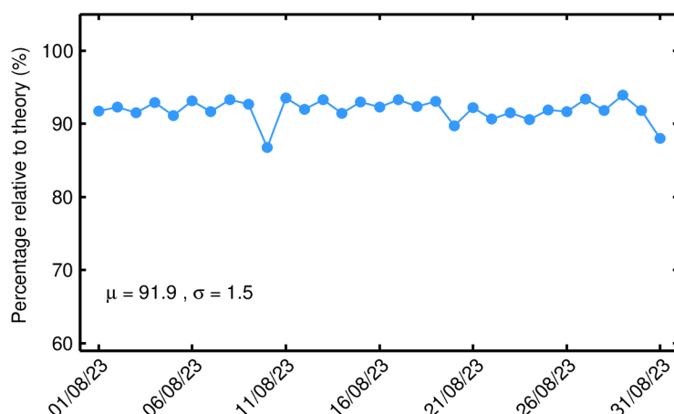
Figure 22. Percentage of science-valid NOP 1-Hz sigma0 records over ocean and lakes relative to theory for each day in August 2023. The mean ( \mu ) and standard deviation ( \sigma ) are also shown.
