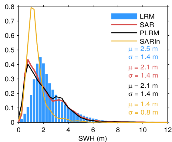
Figure 17. Histogram of science-valid NOP SWH over oceans and lakes for LRM (blue), SAR (red), PLRM (black) and SARIn (orange) for August 2023. The mean ( \mu ) and standard deviation ( \sigma ) are also shown. Values larger than 12 m are excluded from the histogram for the sake of readability but not from the computation of \mu and \sigma .
