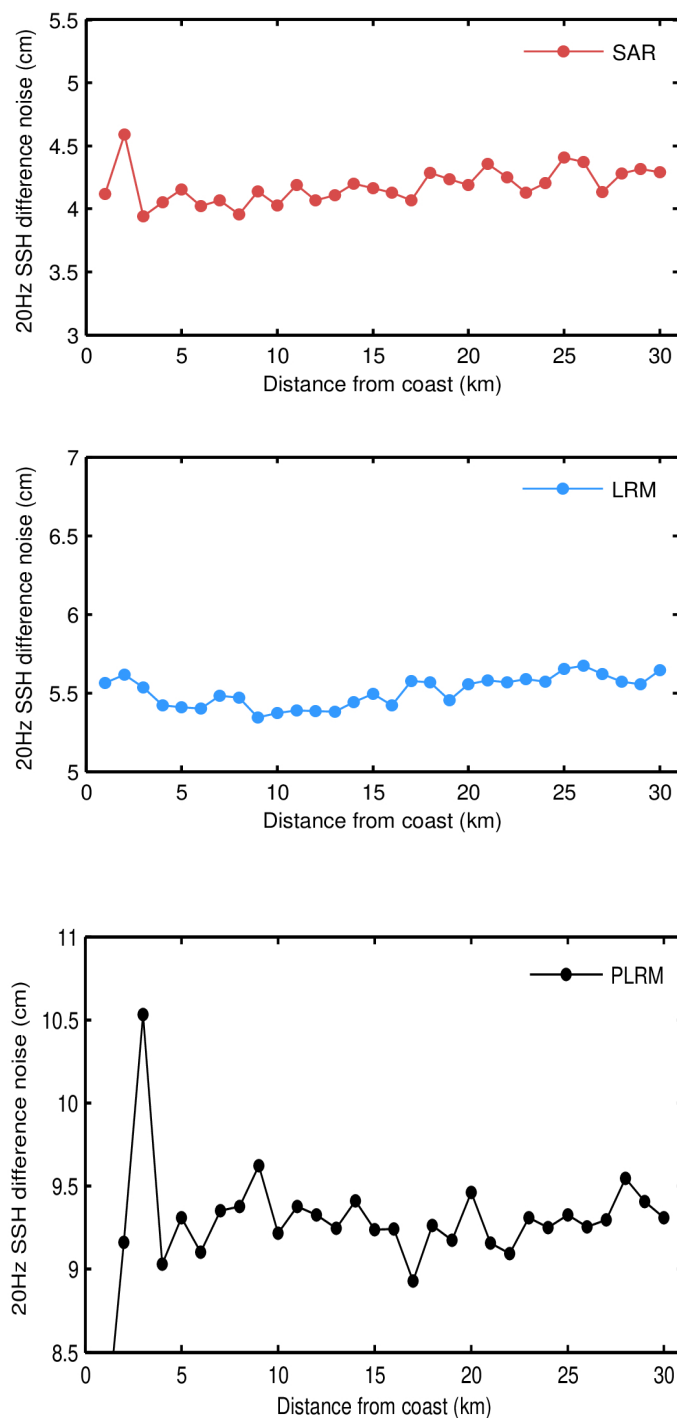
Figure 44. Science-valid IOP 20-Hz SSH anomaly noise as a function of distance from the coast for SAR (top panel), LRM (middle panel), and PLRM (bottom panel) for August 2023. Noise values have been calculated as the median of the absolute value of the difference between consecutive 20-Hz records.
