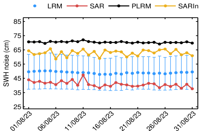
Figure 19. Mean science-valid NOP SWH noise for LRM (blue dot), SAR (red dot), PLRM (black dot) and SARIn (orange dot) for each day in August 2023. The corresponding standard deviation for LRM (blue error bar) is also shown.
