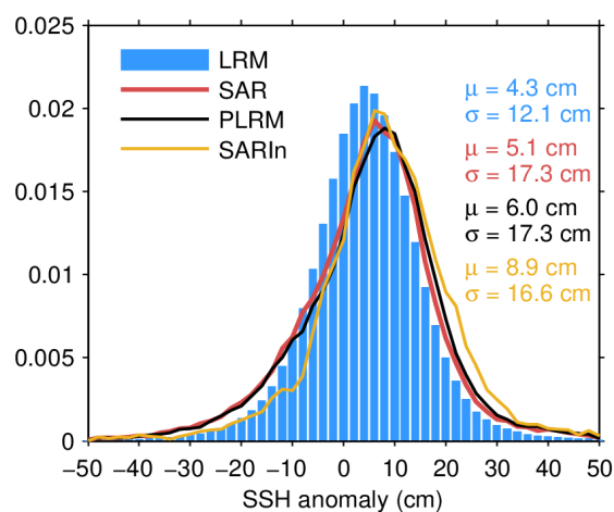
Figure 7. Histogram of science-valid NOP SSH anomaly over oceans and lakes for LRM (blue), SAR (red), PLRM (black) and SARIn (orange) for August 2023. The mean ( \mu ) and standard deviation ( \sigma ) are also shown. Values outside [-50 \ 50] cm are excluded from the histogram for the sake of readability but not from the computation of \mu and \sigma .
