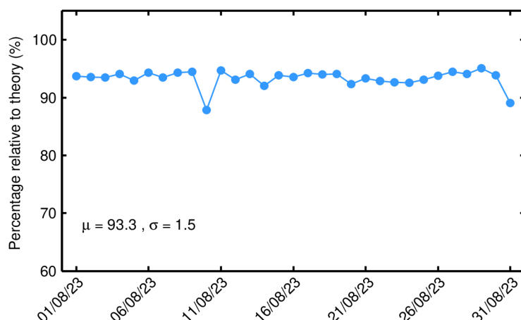
Figure 91. Percentage of science-valid GOP 1-Hz sigma0 records over ocean and lakes relative to theory for each day in August 2023. The mean ( \mu ) and standard deviation ( \sigma ) are also shown.
