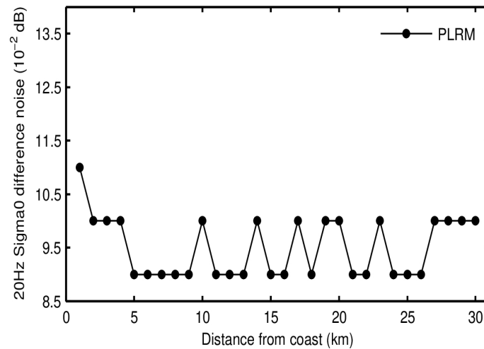
Figure 27. Science-valid NOP 20-Hz sigma0 noise as a function of distance from the coast for SAR (top panel), LRM (middle panel), and PLRM (bottom panel) for August 2023. Noise values have been calculated as the median of the absolute value of the difference between consecutive 20-Hz records.
