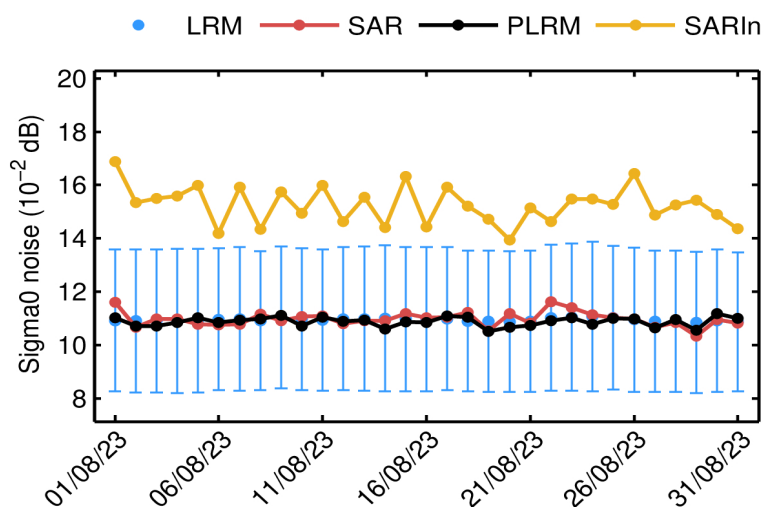
Figure 60. Mean science-valid IOP sigma0 noise for LRM (blue dot), SAR (red dot), PLRM (black dot) and SARIn (orange dot) for each day in August 2023. The corresponding standard deviation for LRM (blue error bar) is also shown.
