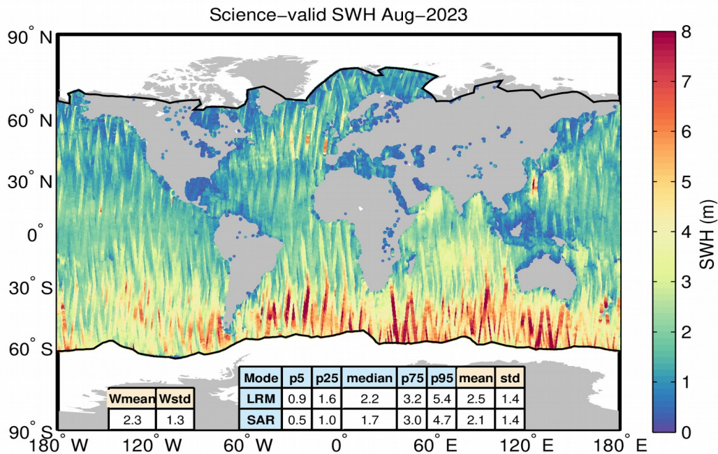
Figure 16. Geographical distribution of science-valid NOP SWH data over oceans and lakes for August 2023. The statistical values shown in the table refer to the SWH in m and are calculated separately for LRM and SAR regions. Wmean and Wstd denote the spatial area-weighted average and its standard deviation. Measurements taken over polar polygons have been excluded from the computation of the statistical values. The black lines mark the outer limit of the Arctic and Antarctic polar polygons.
