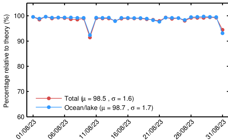
Figure 71. Percentage of GOP 1-Hz records over land and ocean/lake (red) and only over ocean/lake (blue) relative to the theoretically expected number from the orbits ground tracks for each day in August 2023.
