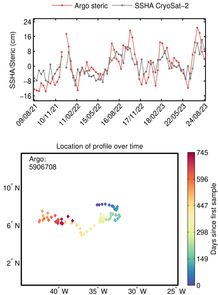
Figure 126. Comparison of the GOP SSH anomaly and the steric height anomaly (referred to 1000 m) for one particular Argo float (top). The location of the Argo float over time is also shown (bottom).
