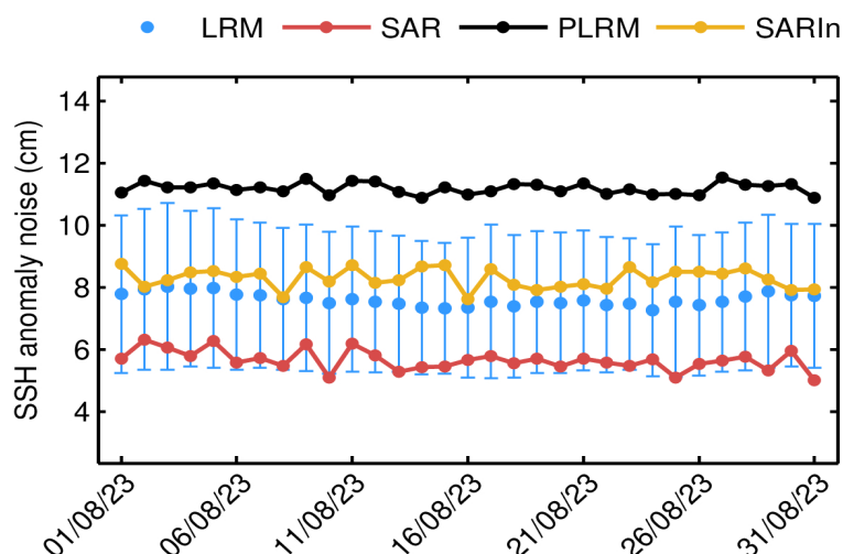
Figure 43. Mean science-valid IOP SSH anomaly noise for LRM (blue dot), SAR (red dot), PLRM (black dot) and SARIn (orange dot) for each day in August 2023. The corresponding standard deviation for LRM (blue error bar) is also shown.
