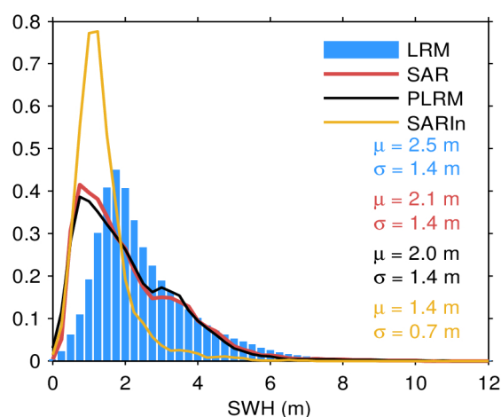
Figure 51. Histogram of science-valid IOP SWH over oceans and lakes for LRM (blue), SAR (red), PLRM (black) and SARIn (orange) for August 2023. The mean ( \mu ) and standard deviation ( \sigma ) are also shown. Values larger than 12 m are excluded from the histogram for the sake of readability but not from the computation of \mu and \sigma .
