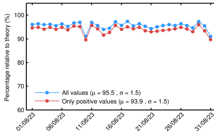
Figure 66. Percentage of science-valid IOP 1-Hz mispointing records over ocean and lakes relative to theory for each day in August 2023. The mean ( \mu ) and standard deviation ( \sigma ) are also shown.
