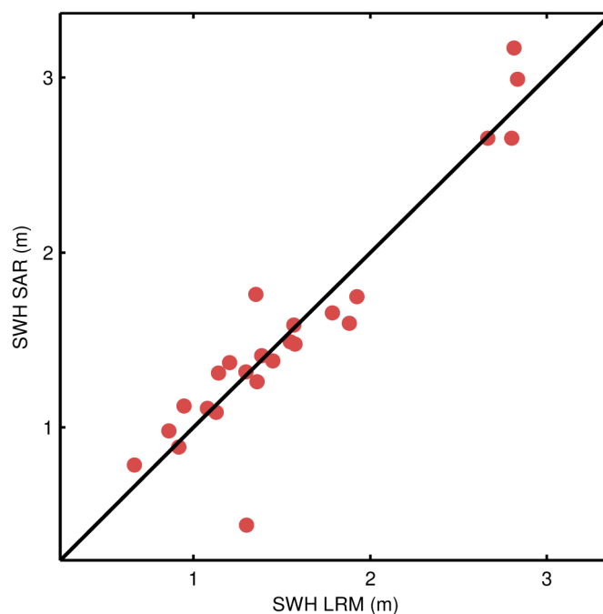
Figure 90. Scatter plot of the science-valid GOP SWH at the two nearest points outside (LRM, x-axis) and inside (SAR, y-axis) the Pacific SAR mode box for each pass. The RMS of the differences is 16.4 cm for the pairs shown in the figure as compared to a RMS of 14.3 cm for the differences between such outside points and their respective nearest neighbour also outside the box in the LRM region.
