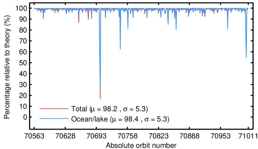
Figure 38. Percentage of IOP 1-Hz records over land and ocean/lake (red) and only over ocean/lake (blue) relative to the theoretically expected number from the orbits ground tracks for each orbit in August 2023. The mean ( \mu ) and standard deviation ( \sigma ) are also shown.
