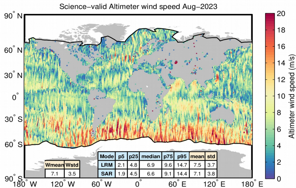
Figure 98. Geographical distribution of science-valid GOP wind data over oceans and lakes for August 2023. The statistical values shown in the table refer to the wind in m and are calculated separately for LRM and SAR regions. Wmean and Wstd denote the spatial area-weighted average and its standard deviation. Measurements taken over polar polygons have been excluded from the computation of the statistical values. The black lines mark the outer limit of the Arctic and Antarctic polar polygons.
