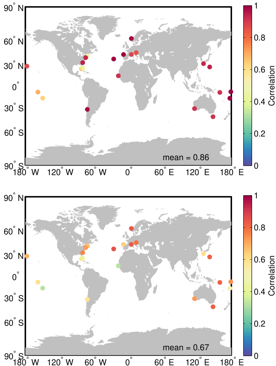
Figure 106. Map showing the correlation between the GOP SSH anomaly and the sea level from tide gauge records over the period September 2021 to August 2023 for the cases with (top) and without (bottom) the tidal component. For this comparison the atmospheric component has not been subtracted. Empty dots denote statistically non-significant correlation.
