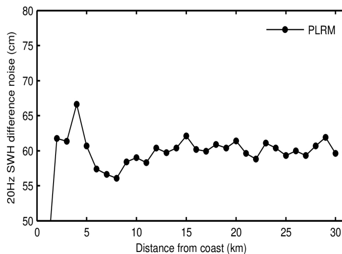
Figure 54. Science-valid IOP 20-Hz SWH noise as a function of distance from the coast for SAR (top panel), LRM (middle panel), and PLRM (bottom panel) for August 2023. Noise values have been calculated as the median of the absolute value of the difference between consecutive 20-Hz records.
