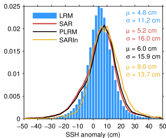
Figure 41. Histogram of science-valid IOP SSH anomaly over oceans and lakes for LRM (blue), SAR (red), PLRM (black) and SARIn (orange) for August 2023. The mean ( \mu ) and standard deviation ( \sigma ) are also shown. Values outside [-50\ 50] cm are excluded from the histogram for the sake of readability but not from the computation of \mu and \sigma .
