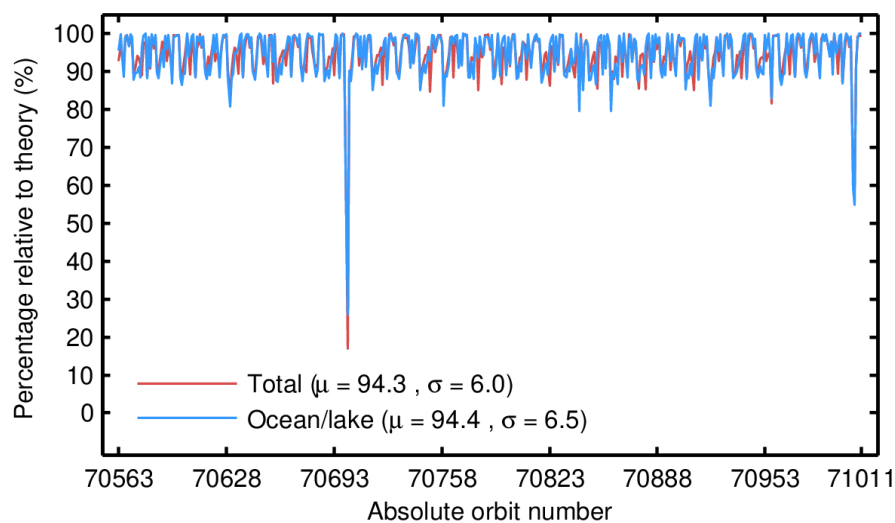
Figure 4. Percentage of NOP 1-Hz records over land and ocean/lake (red) and only over ocean/lake (blue) relative to the theoretically expected number from the orbits ground tracks for each orbit in August 2023. The mean ( \mu ) and standard deviation ( \sigma ) are also shown.
