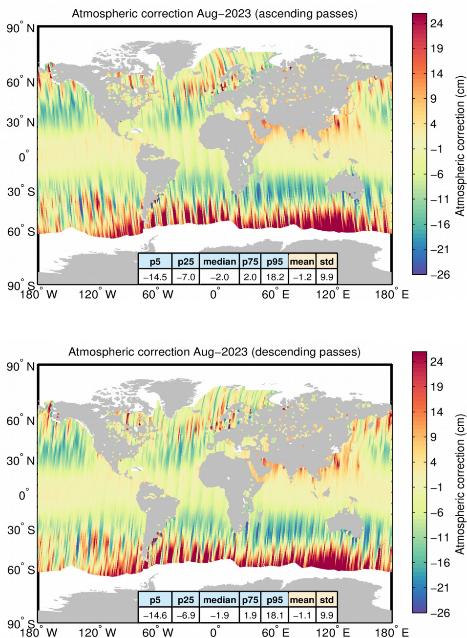
Figure A5. Geographical distribution of the atmospheric correction over oceans and lakes for ascending (top) and descending (bottom) passes for August 2023. The statistical values shown in the table refer to the atmospheric correction in cm. Measurements taken over polar polygons have been excluded from the computation of the statistical values. The black lines mark the outer limit of the Arctic and Antarctic polar polygons.
