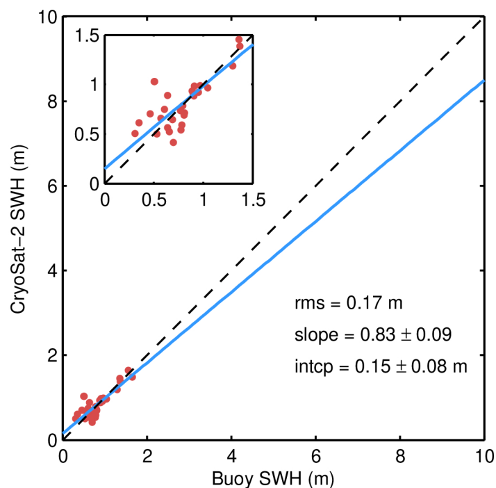
Figure 112. Scatter plot showing a comparison of GOP SWH with SWH from NDBC buoy data for August 2023. The inset plot shows a zoomed-in for SWH < 1.5 m.
