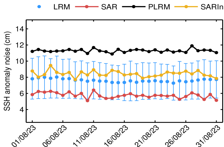
Figure 9. Mean science-valid NOP SSH anomaly noise for LRM (blue dot), SAR (red dot), PLRM (black dot) and SARIn (orange dot) for each day in August 2023. The corresponding standard deviation for LRM (blue error bar) is also shown.
