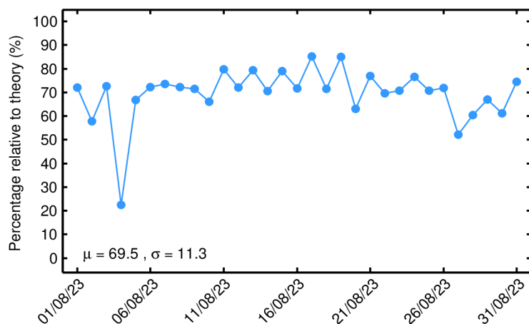
Figure 5. Percentage of science-valid NOP 1-Hz SSH records over ocean and lakes relative to theory for each day in August 2023. The mean ( \mu ) and standard deviation ( \sigma ) are also shown.
