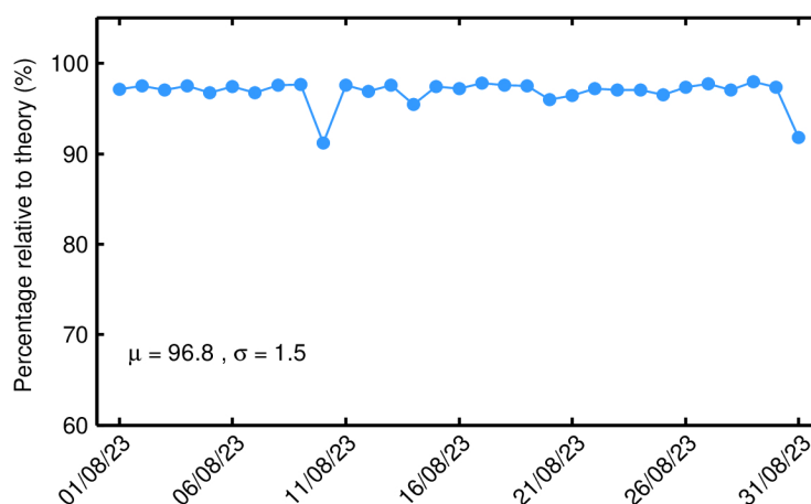
Figure 84. Percentage of science-valid GOP 1-Hz SWH records over ocean and lakes relative to theory for each day in August 2023. The mean ( \mu ) and standard deviation ( \sigma ) are also shown.
