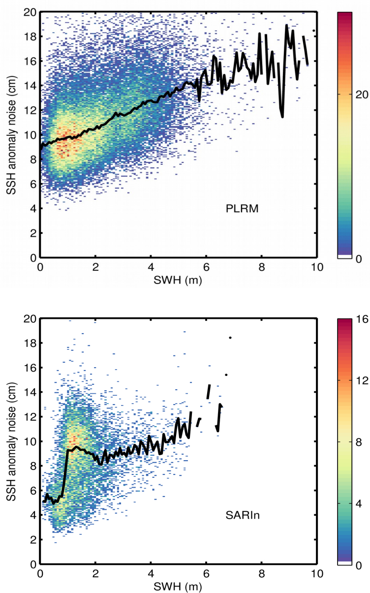
Figure 11. 2D histogram showing science-valid NOP SSH anomaly noise as a function of SWH for SAR, LRM, PLRM, and SARIn (from top to bottom) for August 2023. The black line denotes the median SSH anomaly noise as a function of SWH.
