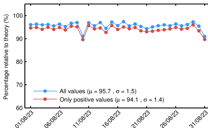
Figure 101. Percentage of science-valid GOP 1-Hz mispointing records over ocean and lakes relative to theory for each day in August 2023. The mean ( \mu ) and standard deviation ( \sigma ) are also shown.
