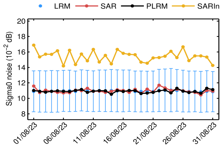
Figure 26. Mean science-valid NOP sigma0 noise for LRM (blue dot), SAR (red dot), PLRM (black dot) and SARIn (orange dot) for each day in August 2023. The corresponding standard deviation for LRM (blue error bar) is also shown.
