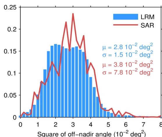
Figure 34. Histogram of science-valid NOP mispointing over oceans and lakes for LRM (blue) and SAR (red) for August 2023. The mean ( \mu ) and standard deviation ( \sigma ) are also shown. Note that values larger than 12 m are excluded from the histogram for the sake of readability but not from the computation of \mu and \sigma .
