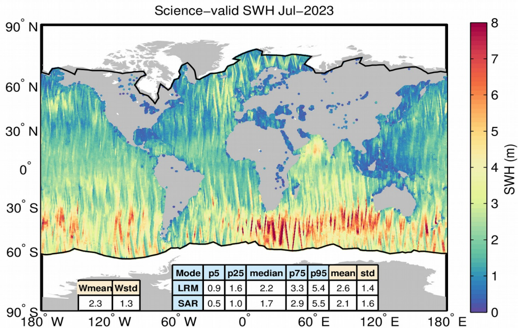
Figure 50. Geographical distribution of science-valid IOP SWH data over oceans and lakes for July 2023. The statistical values shown in the table refer to the SWH in m and are calculated separately for LRM and SAR regions. Wmean and Wstd denote the spatial area-weighted average and its standard deviation. Measurements taken over polar polygons have been excluded from the computation of the statistical values. The black lines mark the outer limit of the Arctic and Antarctic polar polygons.
