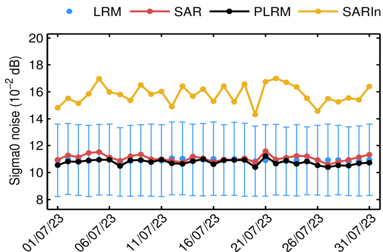
Figure 95. Mean science-valid GOP sigma0 noise for LRM (blue dot), SAR (red dot), PLRM (black dot) and SARIn (orange dot) for each day in July 2023. The corresponding standard deviation for LRM (blue error bar) is also shown.
