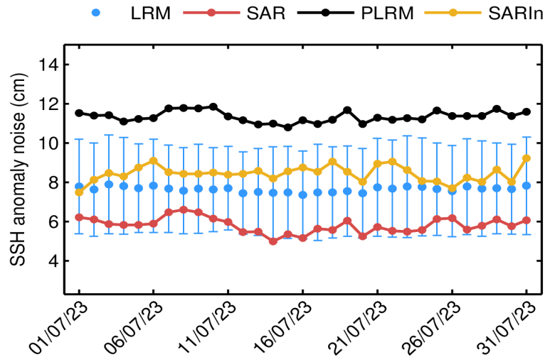
Figure 9. Mean science-valid NOP SSH anomaly noise for LRM (blue dot), SAR (red dot), PLRM (black dot) and SARIn (orange dot) for each day in July 2023. The corresponding standard deviation for LRM (blue error bar) is also shown.
