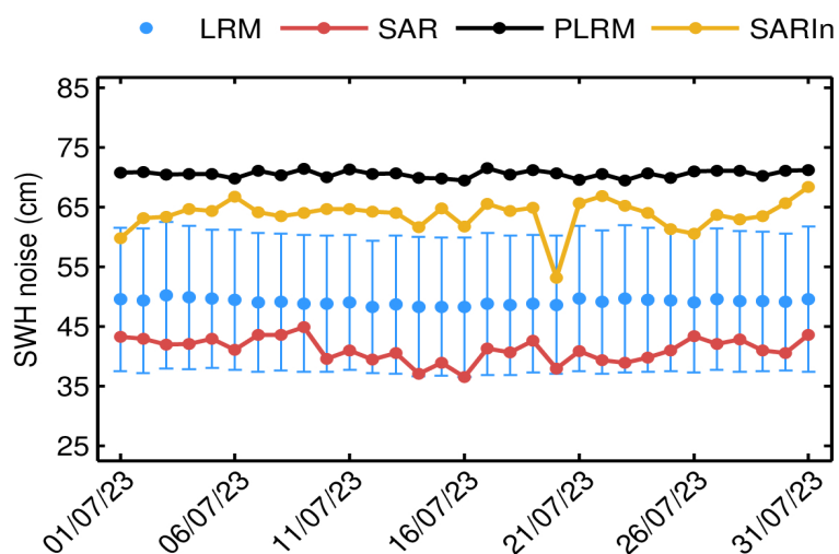
Figure 19. Mean science-valid NOP SWH noise for LRM (blue dot), SAR (red dot), PLRM (black dot) and SARIn (orange dot) for each day in July 2023. The corresponding standard deviation for LRM (blue error bar) is also shown.
