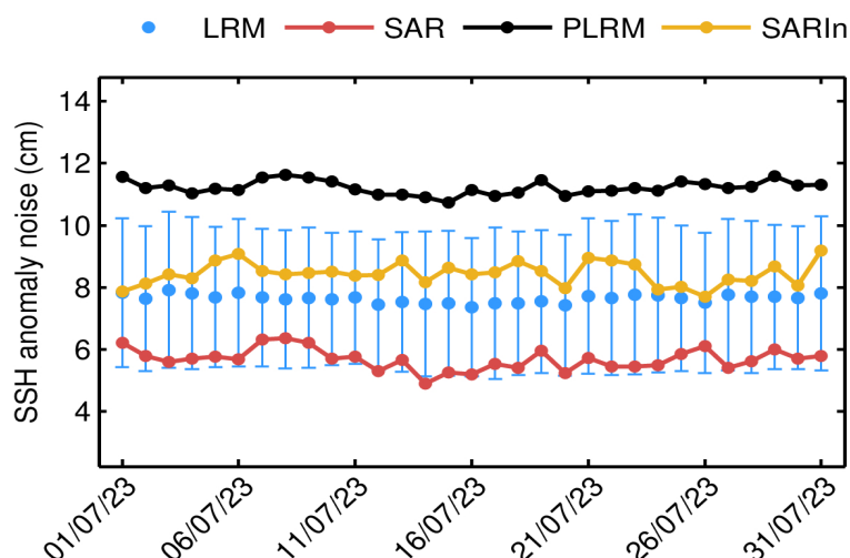
Figure 43. Mean science-valid IOP SSH anomaly noise for LRM (blue dot), SAR (red dot), PLRM (black dot) and SARIn (orange dot) for each day in July 2023. The corresponding standard deviation for LRM (blue error bar) is also shown.
