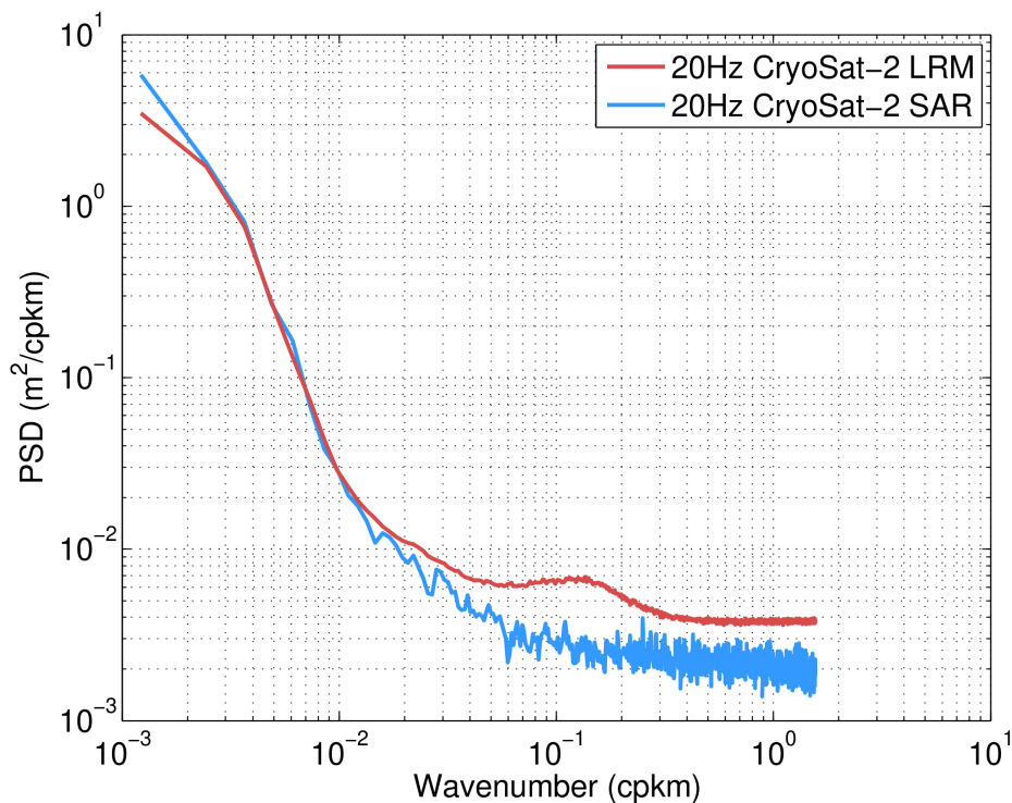
Figure 76. Along-track power spectrum density of the science-valid 20 Hz GOP SSH anomaly over oceans and lakes for LRM (red) and SAR (blue) for July 2023.
