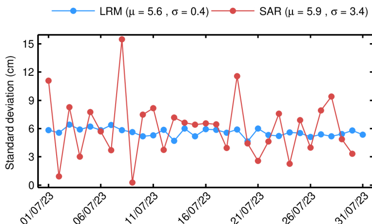
Figure 48. Standard deviation of differences at crossovers for IOP SSH anomaly for each day in July 2023. The values shown in this figure have been computed for the science-valid data further edited according to the following two additional criteria: 1) rejecting crossover differences larger than 20 cm; and 2) rejecting shallow waters (1000 m). The mean ( \mu ) and standard deviation ( \sigma ) are also shown.
