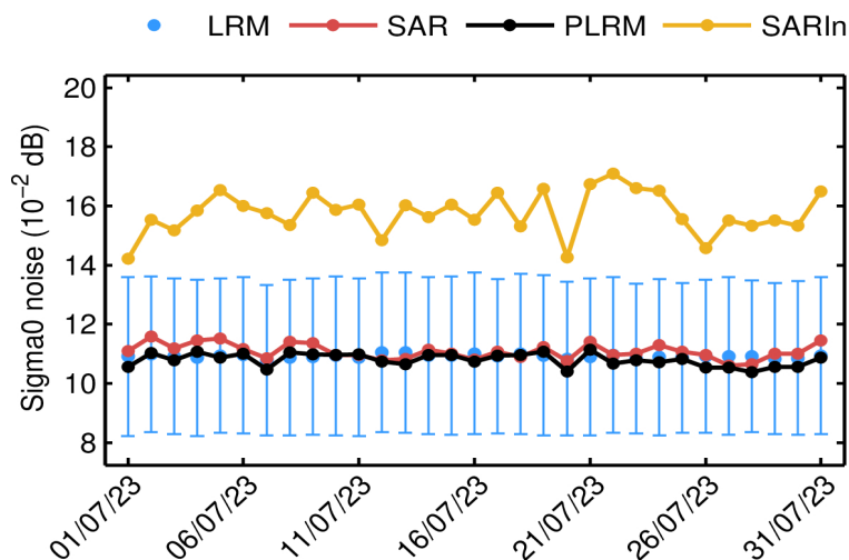
Figure 26. Mean science-valid NOP sigma0 noise for LRM (blue dot), SAR (red dot), PLRM (black dot) and SARIn (orange dot) for each day in July 2023. The corresponding standard deviation for LRM (blue error bar) is also shown.
