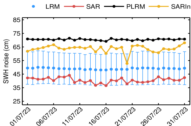
Figure 88. Mean science-valid GOP SWH noise for LRM (blue dot), SAR (red dot), PLRM (black dot) and SARIn (orange dot) for each day in July 2023. The corresponding standard deviation for LRM (blue error bar) is also shown.
