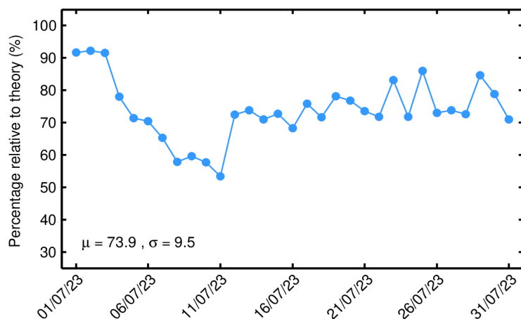
Figure 5. Percentage of science-valid NOP 1-Hz SSH records over ocean and lakes relative to theory for each day in July 2023. The mean ( \mu ) and standard deviation ( \sigma ) are also shown.
