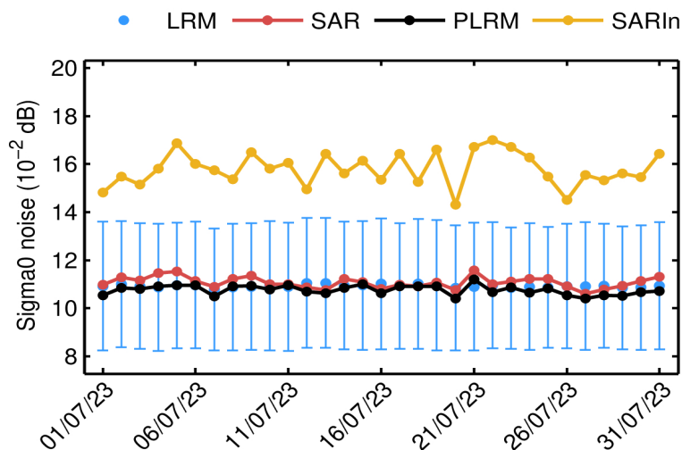
Figure 60. Mean science-valid IOP sigma0 noise for LRM (blue dot), SAR (red dot), PLRM (black dot) and SARIn (orange dot) for each day in July 2023. The corresponding standard deviation for LRM (blue error bar) is also shown.
