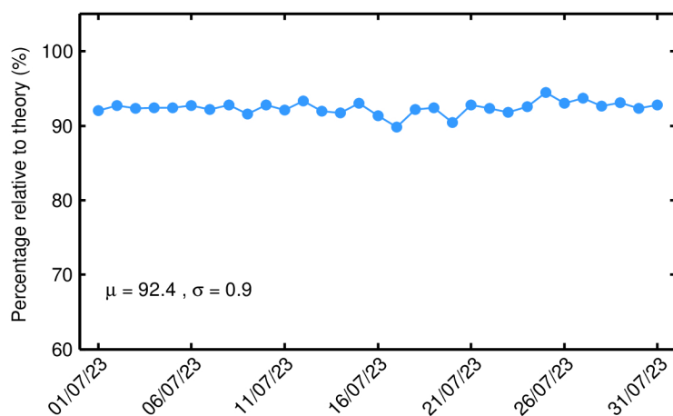
Figure 22. Percentage of science-valid NOP 1-Hz sigma0 records over ocean and lakes relative to theory for each day in July 2023. The mean ( \mu ) and standard deviation ( \sigma ) are also shown.
