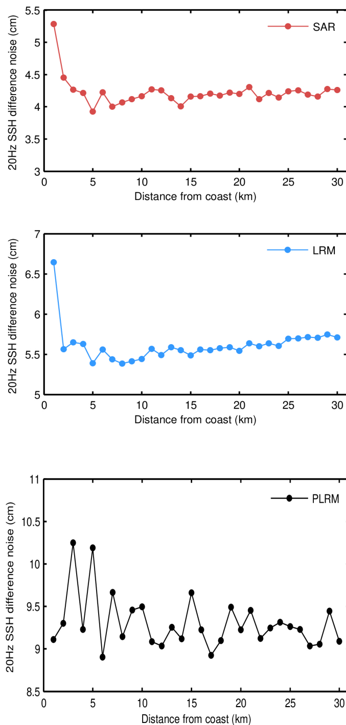
Figure 44. Science-valid IOP 20-Hz SSH anomaly noise as a function of distance from the coast for SAR (top panel), LRM (middle panel), and PLRM (bottom panel) for July 2023. Noise values have been calculated as the median of the absolute value of the difference between consecutive 20-Hz records.
