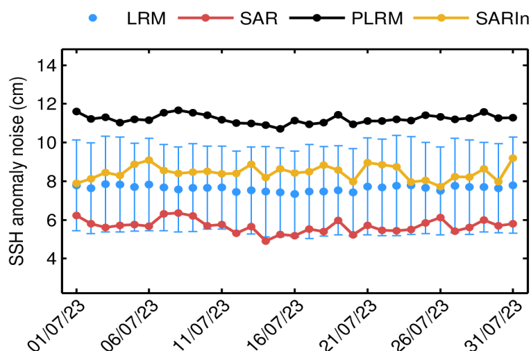
Figure 78. Mean science-valid GOP SSH anomaly noise for LRM (blue dot), SAR (red dot), PLRM (black dot) and SARIn (orange dot) for each day in July 2023. The corresponding standard deviation for LRM (blue error bar) is also shown.
