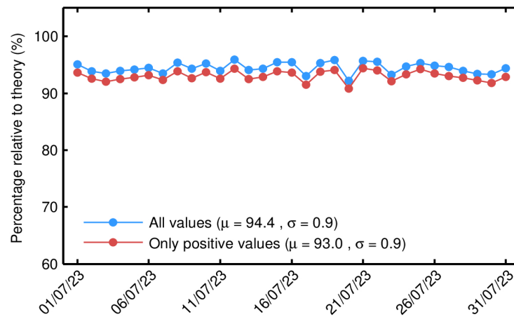
Figure 32. Percentage of science-valid NOP 1-Hz mispointing records over ocean and lakes relative to theory for each day in July 2023. The mean ( \mu ) and standard deviation ( \sigma ) are also shown.
