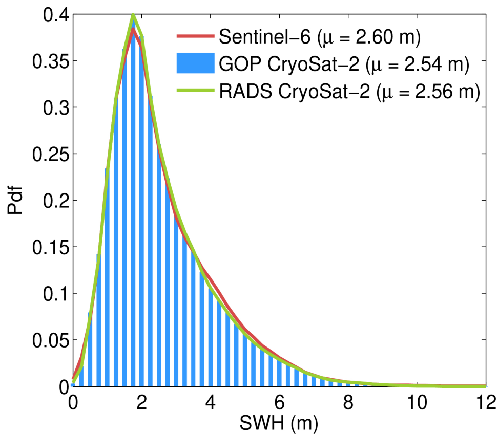
Figure 128. Histograms (normalized to have a total area of 1) of the SWH from GOP (blue bars), reference mission (red line) and RADS CryoSat-2 (green) for July 2023.
