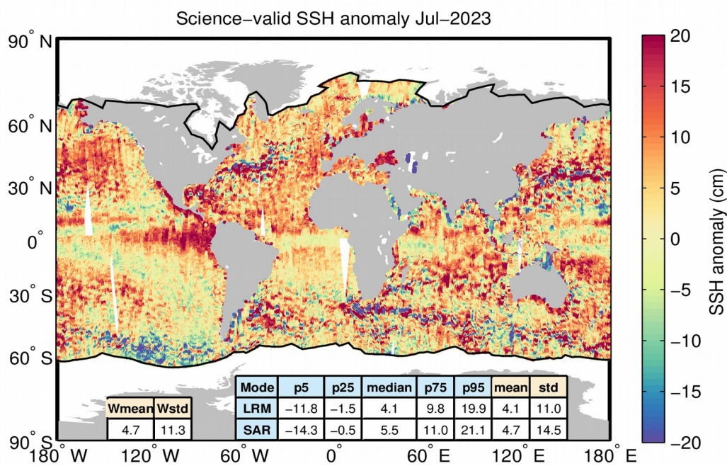
Figure 40. Geographical distribution of science-valid IOP 1-Hz SSH anomaly data over oceans and lakes for July 2023. The statistical values shown in the table refer to the SSH anomaly in cm and are calculated separately for LRM and SAR regions. Wmean and Wstd denote the spatial area-weighted average and its standard deviation. Measurements taken over polar polygons have been excluded from the computation of the statistical values. The black lines mark the outer limit of the Arctic and Antarctic polar polygons.
