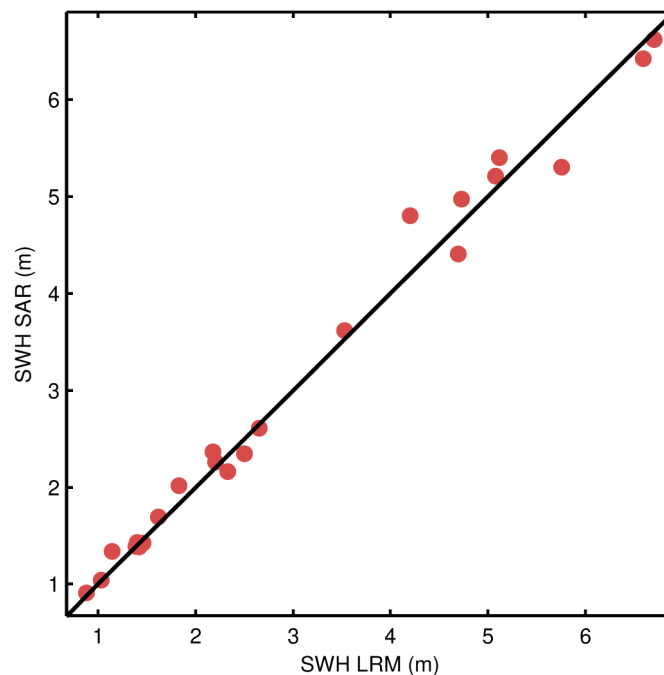
Figure 55. Scatter plot of the science-valid IOP SWH at the two nearest points outside (LRM, x-axis) and inside (SAR, y-axis) the Pacific SAR mode box for each pass. The RMS of the differences is 21.2 cm for the pairs shown in the figure as compared to a RMS of 16.5 cm for the differences between such outside points and their respective nearest neighbour also outside the box in the LRM region.
