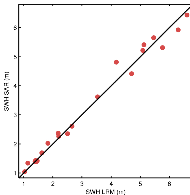
Figure 90. Scatter plot of the science-valid GOP SWH at the two nearest points outside (LRM, x-axis) and inside (SAR, y-axis) the Pacific SAR mode box for each pass. The RMS of the differences is 23.5 cm for the pairs shown in the figure as compared to a RMS of 14.6 cm for the differences between such outside points and their respective nearest neighbour also outside the box in the LRM region.
