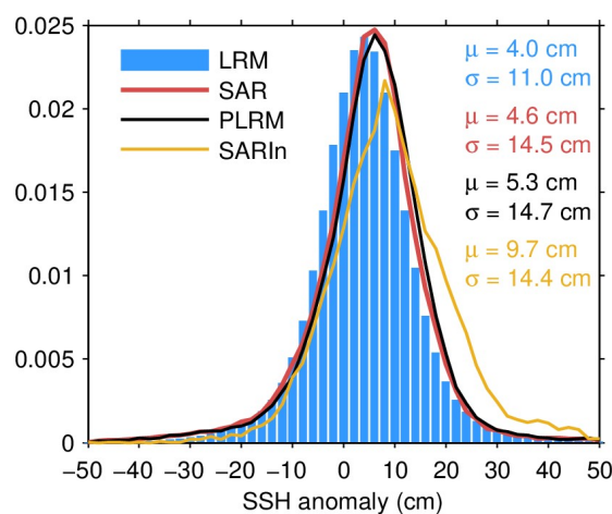
Figure 75. Histogram of science-valid GOP SSH anomaly over oceans and lakes for LRM (blue), SAR (red), PLRM (black) and SARIn (orange) for July 2023. The mean ( \mu ) and
