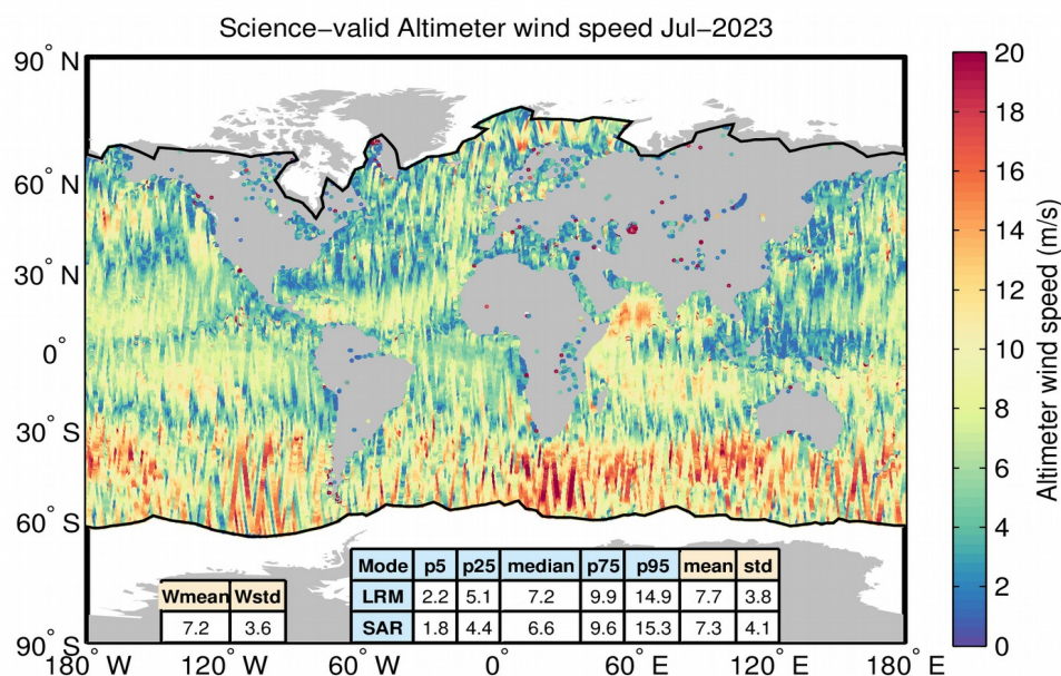
Figure 29. Geographical distribution of science-valid NOP wind data over oceans and lakes for July 2023. The statistical values shown in the table refer to the wind in m and are calculated separately for LRM and SAR regions. Wmean and Wstd denote the spatial area-weighted average and its standard deviation. Measurements taken over polar polygons have been excluded from the computation of the statistical values. The black lines mark the outer limit of the Arctic and Antarctic polar polygons.
