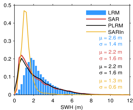
Figure 17. Histogram of science-valid NOP SWH over oceans and lakes for LRM (blue), SAR (red), PLRM (black) and SARIn (orange) for July 2023. The mean ( \mu ) and standard deviation ( \sigma ) are also shown. Values larger than 12 m are excluded from the histogram for the sake of readability but not from the computation of \mu and \sigma .
