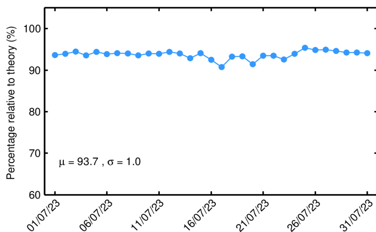
Figure 56. Percentage of science-valid IOP 1-Hz sigma0 records over ocean and lakes relative to theory for each day in July 2023. The mean ( \mu ) and standard deviation ( \sigma ) are also shown.
