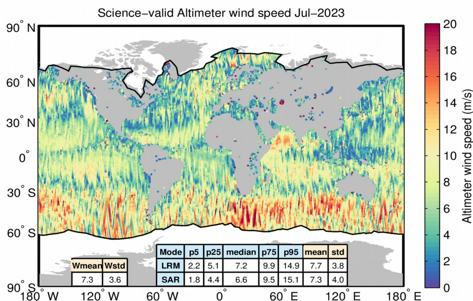
Figure 63. Geographical distribution of science-valid IOP wind data over oceans and lakes for July 2023. The statistical values shown in the table refer to the wind in m and are calculated separately for LRM and SAR regions. Wmean and Wstd denote the spatial area-weighted average and its standard deviation. Measurements taken over polar polygons have been excluded from the computation of the statistical values. The black lines mark the outer limit of the Arctic and Antarctic polar polygons.
