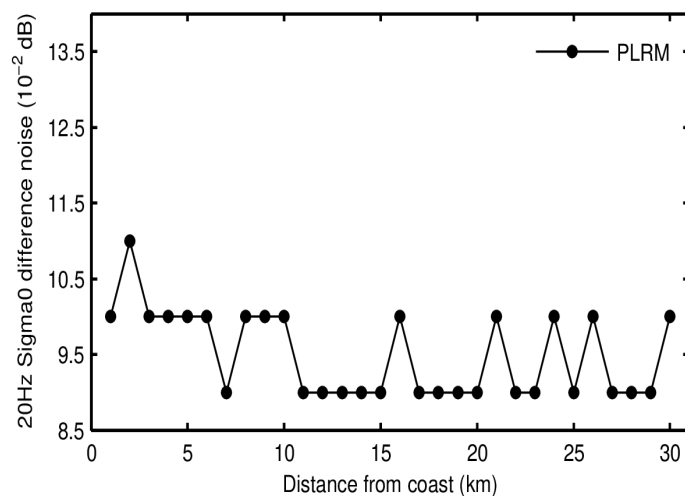
Figure 96. Science-valid GOP 20-Hz sigma0 noise as a function of distance from the coast for SAR (top panel), LRM (middle panel), and PLRM (bottom panel) for July 2023. Noise values have been calculated as the median of the absolute value of the difference between consecutive 20-Hz records.
