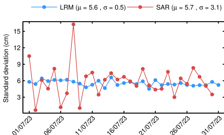
Figure 83. Standard deviation of differences at crossovers for GOP SSH anomaly for each day in July 2023. The values shown in this figure have been computed for the science-valid data further edited according to the following two additional criteria: 1) rejecting crossover differences larger than 20 cm; and 2) rejecting shallow waters (1000 m). The mean ( \mu ) and standard deviation ( \sigma ) are also shown.
