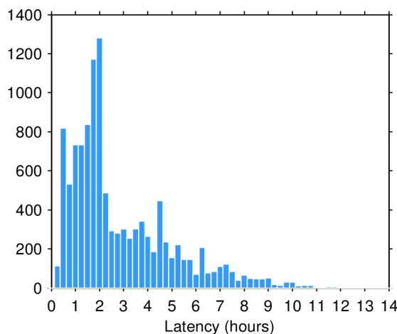
Figure 2. Histogram of the NOP data latency for July 2023. The y-axis denotes the number of files that are made available with a delay of x-hours with respect to the mean time of the records stored in the file.
