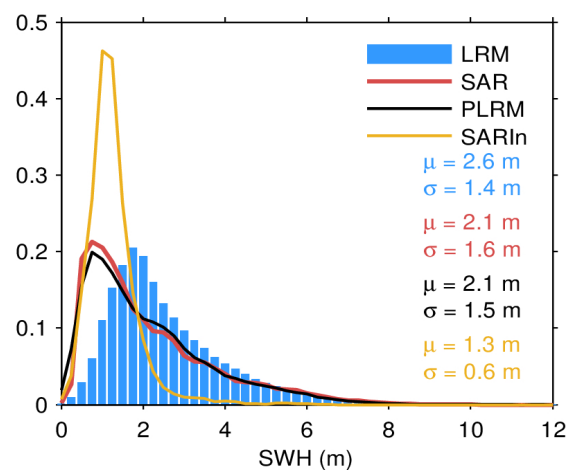
Figure 51. Histogram of science-valid IOP SWH over oceans and lakes for LRM (blue), SAR (red), PLRM (black) and SARIn (orange) for July 2023. The mean ( \mu ) and standard deviation ( \sigma ) are also shown. Values larger than 12 m are excluded from the histogram for the sake of readability but not from the computation of \mu and \sigma .
