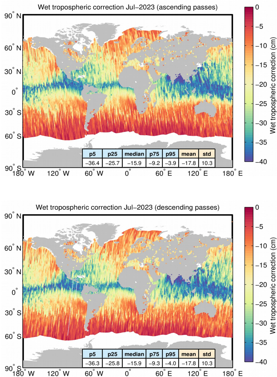
Figure A1. Geographical distribution of the wet tropospheric correction over oceans and lakes for ascending (top) and descending (bottom) passes for July 2023. The statistical values shown in the table refer to the wet tropospheric correction in cm. Measurements taken over polar polygons have been excluded from the computation of the statistical values. The black lines mark the outer limit of the Arctic and Antarctic polar polygons.
