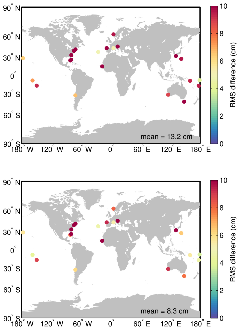
Figure 107. Map showing the RMS difference between the GOP SSH anomaly and the sea level from tide gauge records over the period August 2021 to July 2023 for the cases with (top) and without (bottom) the tidal component. For this comparison the atmospheric component has not been subtracted.
