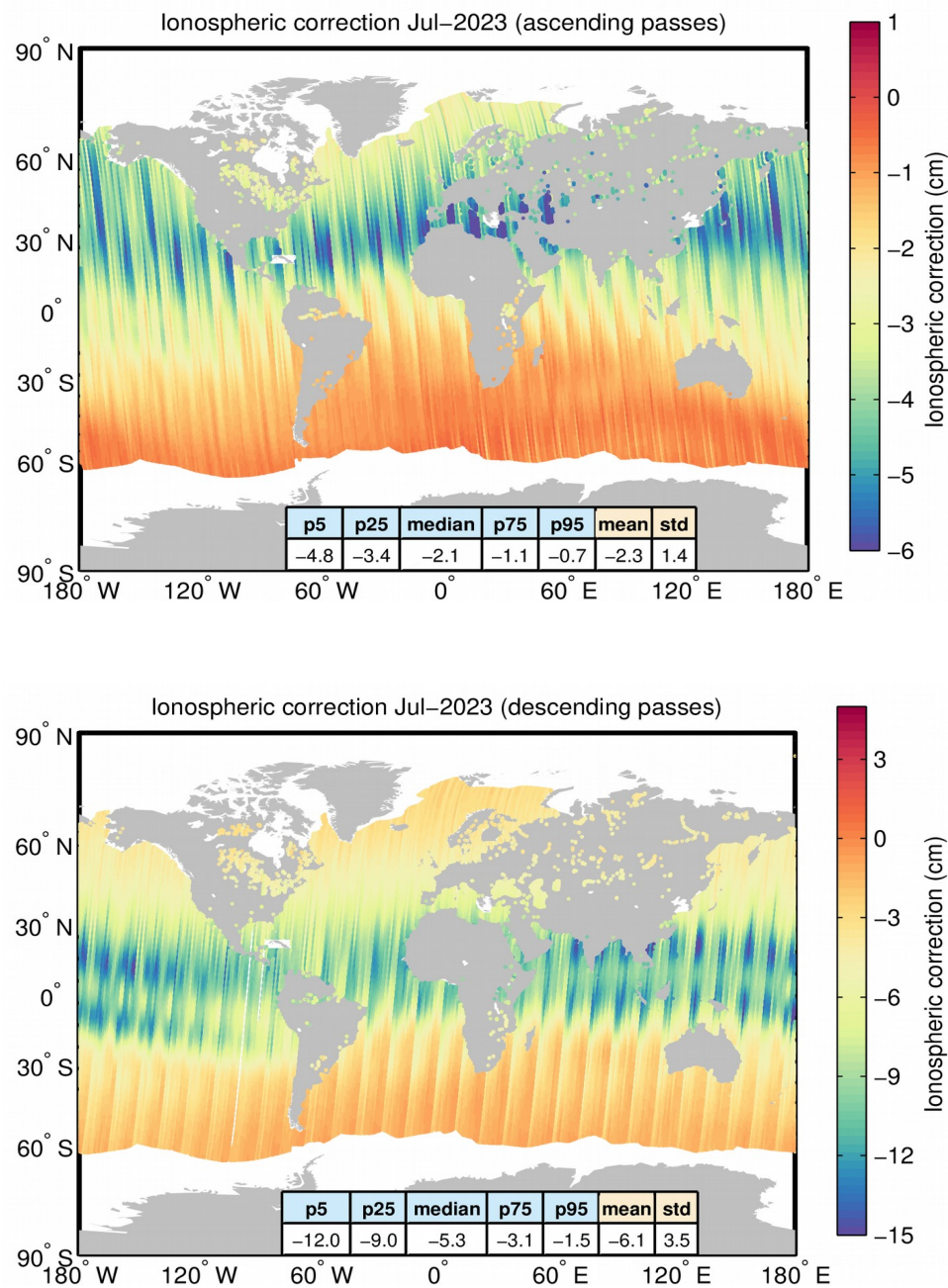
Figure A3. Geographical distribution of the Ionospheric correction over oceans and lakes for ascending (top) and descending (bottom) passes for July 2023. The statistical values shown in the table refer refer to the Ionospheric correction in cm. Measurements taken over polar polygons have been excluded from the computation of the statistical values. The black lines mark the outer limit of the Arctic and Antarctic polar polygons.
