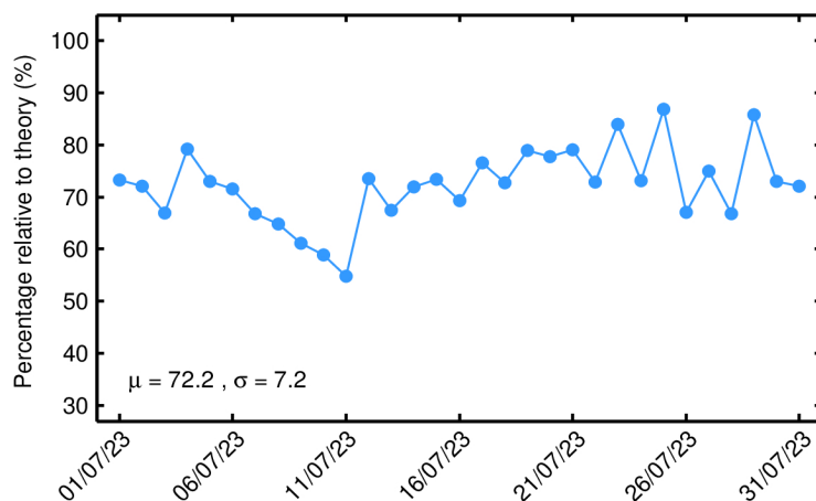
Figure 39. Percentage of science-valid IOP 1-Hz SSH records over ocean and lakes relative to theory for each day in July 2023. The mean ( \mu ) and standard deviation ( \sigma ) are also shown.
