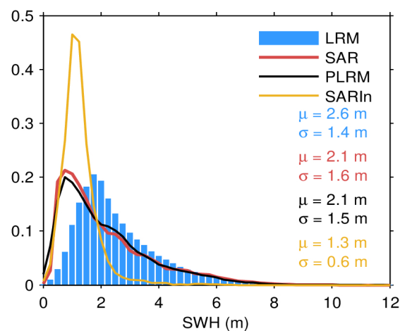
Figure 86. Histogram of science-valid GOP SWH over oceans and lakes for LRM (blue), SAR (red), PLRM (black) and SARIn (orange) and for July 2023. The mean ( \mu ) and standard deviation ( \sigma ) are also shown. Values larger than 12 m are excluded from the histogram for the sake of readability but not from the computation of \mu and \sigma .
