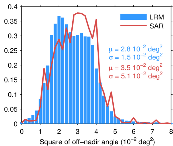
Figure 103. Histogram of science-valid GOP mispointing over oceans and lakes for LRM (blue) and SAR (red) for July 2023. The mean ( \mu ) and standard deviation ( \sigma ) are also shown. Note that values larger than 12 m are excluded from the histogram for the sake of readability but not from the computation of \mu and \sigma .
