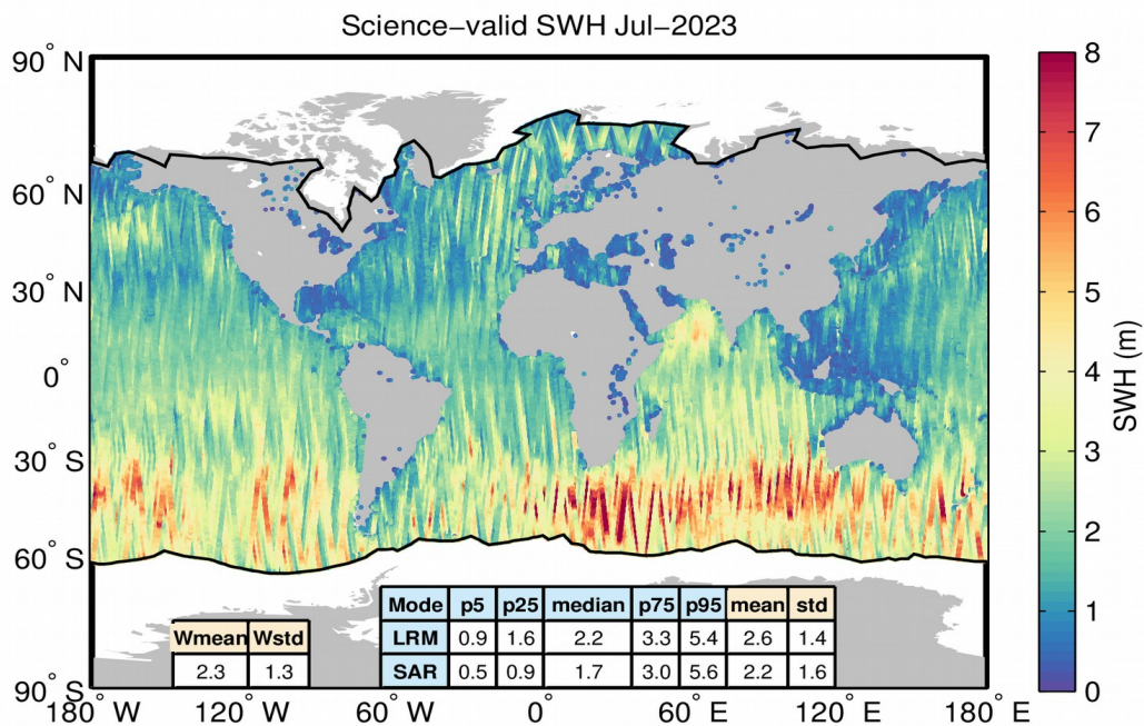
Figure 16. Geographical distribution of science-valid NOP SWH data over oceans and lakes for July 2023. The statistical values shown in the table refer to the SWH in m and are calculated separately for LRM and SAR regions. Wmean and Wstd denote the spatial area-weighted average and its standard deviation. Measurements taken over polar polygons have been excluded from the computation of the statistical values. The black lines mark the outer limit of the Arctic and Antarctic polar polygons.
