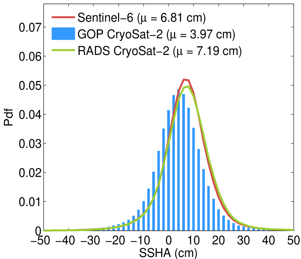
Figure 127. Histograms (normalized to have a total area of 1) of the SSH anomaly from GOP (blue bars), reference mission (red line) and RADS CryoSat-2 (green) for July 2023.
