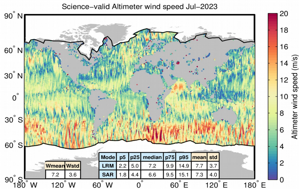
Figure 98. Geographical distribution of science-valid GOP wind data over oceans and lakes for July 2023. The statistical values shown in the table refer to the wind in m and are calculated separately for LRM and SAR regions. Wmean and Wstd denote the spatial area-weighted average and its standard deviation. Measurements taken over polar polygons have been excluded from the computation of the statistical values. The black lines mark the outer limit of the Arctic and Antarctic polar polygons.
