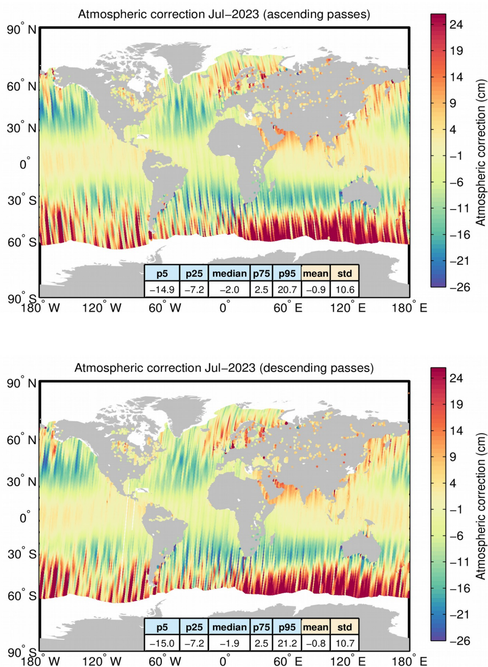
Figure A5. Geographical distribution of the atmospheric correction over oceans and lakes for ascending (top) and descending (bottom) passes for July 2023. The statistical values shown in the table refer to the atmospheric correction in cm. Measurements taken over polar polygons have been excluded from the computation of the statistical values. The black lines mark the outer limit of the Arctic and Antarctic polar polygons.
