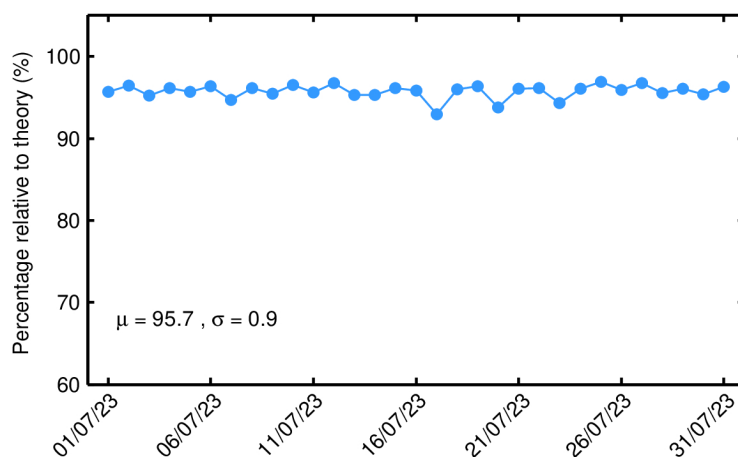
Figure 15. Percentage of science-valid NOP 1-Hz SWH records over ocean and lakes relative to theory for each day in July 2023. The mean ( \mu ) and standard deviation ( \sigma ) are also shown.
