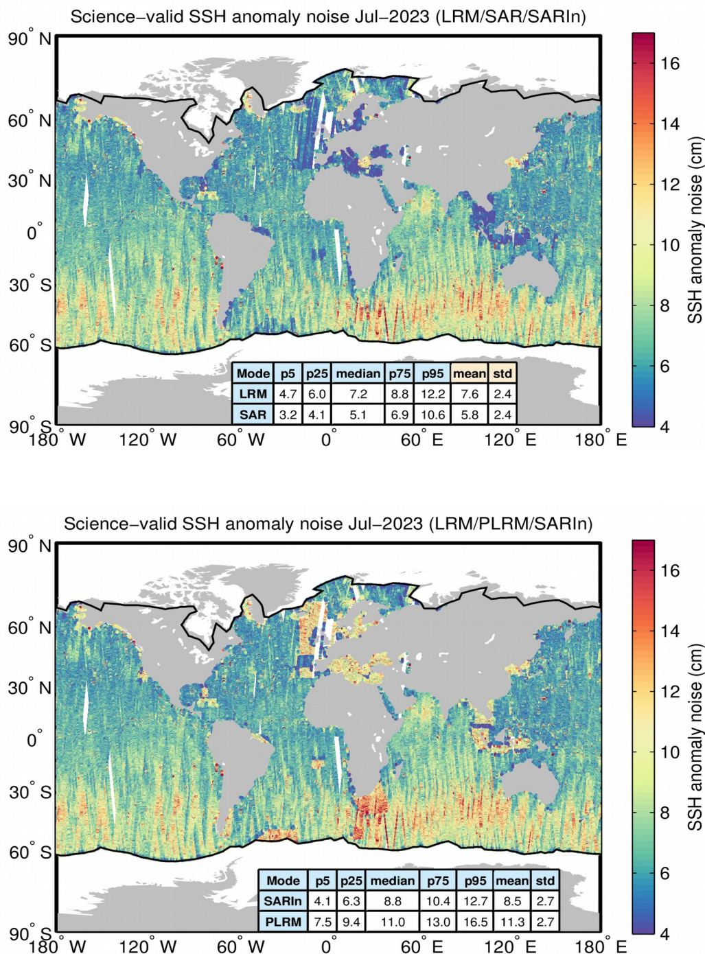
Figure 8. Geographical distribution of flag-valid 20-Hz SSH anomaly measurement noise over oceans and lakes for LRM/SAR/SARIn (top) and LRM/PLRM/SARIn (bottom) and for July 2023. The statistical values shown in the tables refer to the SSH anomaly noise and are calculated separately for LRM, SAR/PLRM, and SARIn regions. Measurements taken
