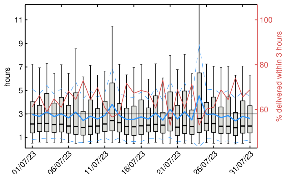
Figure 1. Box-and-whiskers plot for the NOP latency showing for each day in July 2023 the first and third quartiles (bottom and top of the box), the median (thick black), the 5%
