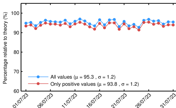
Figure 101. Percentage of science-valid GOP 1-Hz mispointing records over ocean and lakes relative to theory for each day in July 2023. The mean ( \mu ) and standard deviation ( \sigma ) are also shown.
