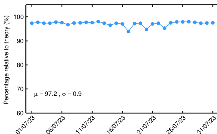
Figure 49. Percentage of science-valid IOP 1-Hz SWH records over ocean and lakes relative to theory for each day in July 2023. The mean ( \mu ) and standard deviation ( \sigma ) are also shown.
