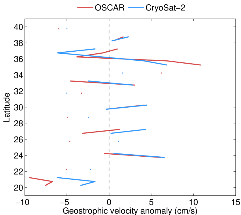
Figure 121. Comparison of the GOP geostrophic velocity anomalies with geostrophic velocities anomalies from the Ocean Surface Current Analyses – Real time (OSCAR) for July 2023 in the Atlantic (top, 20°N – 40°N, 315°E – 325°E) and Pacific (bottom, 20°N – 40°N, 220°E – 230°E) boxes as a function of latitude (i.e., for each latitude the geostrophic velocities have been averaged over the longitudes within the box). GOP geostrophic velocities have been computed using the optimal difference operator by Powell and Leben (2004).
