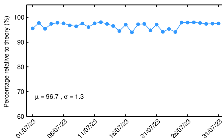
Figure 84. Percentage of science-valid GOP 1-Hz SWH records over ocean and lakes relative to theory for each day in July 2023. The mean ( \mu ) and standard deviation ( \sigma ) are also shown.
