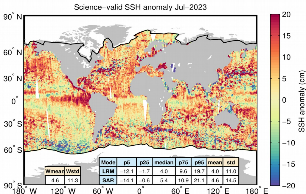
Figure 74. Geographical distribution of science-valid GOP 1-Hz SSH anomaly data over oceans and lakes for July 2023. The statistical values shown in the table refer to the SSH anomaly in cm and are calculated separately for LRM and SAR regions. Wmean and Wstd denote the spatial area-weighted average and its standard deviation. Measurements taken over polar polygons have been excluded from the computation of the statistical values. The black lines mark the outer limit of the Arctic and Antarctic polar polygons.
