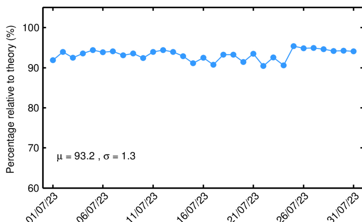
Figure 91. Percentage of science-valid GOP 1-Hz sigma0 records over ocean and lakes relative to theory for each day in July 2023. The mean ( \mu ) and standard deviation ( \sigma ) are also shown.
