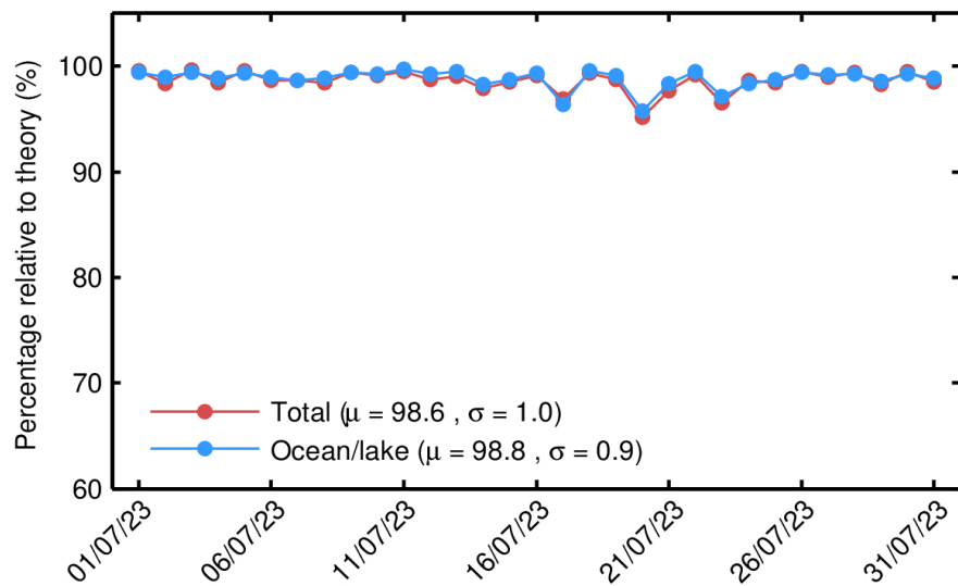
Figure 37. Percentage of IOP 1-Hz records over land and ocean/lake (red) and only over ocean/lake (blue) relative to the theoretically expected number from the orbits ground tracks for each day in July 2023.
