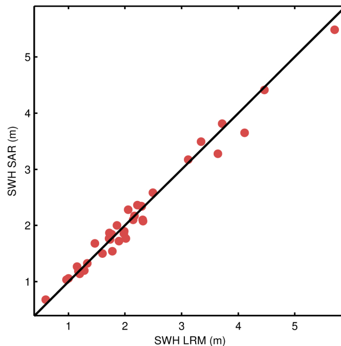
Figure 21. Scatter plot of the science-valid NOP SWH at the two nearest points outside (LRM, x-axis) and inside (SAR, y-axis) the Pacific SAR mode box for each pass. The RMS of the differences is 16.2 cm for the pairs shown in the figure as compared to a RMS of 18.0 cm for the differences between such outside points and their respective nearest neighbour also outside the box in the LRM region.
