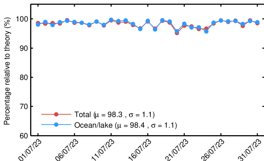
Figure 71. Percentage of GOP 1-Hz records over land and ocean/lake (red) and only over ocean/lake (blue) relative to the theoretically expected number from the orbits ground tracks for each day in July 2023.
