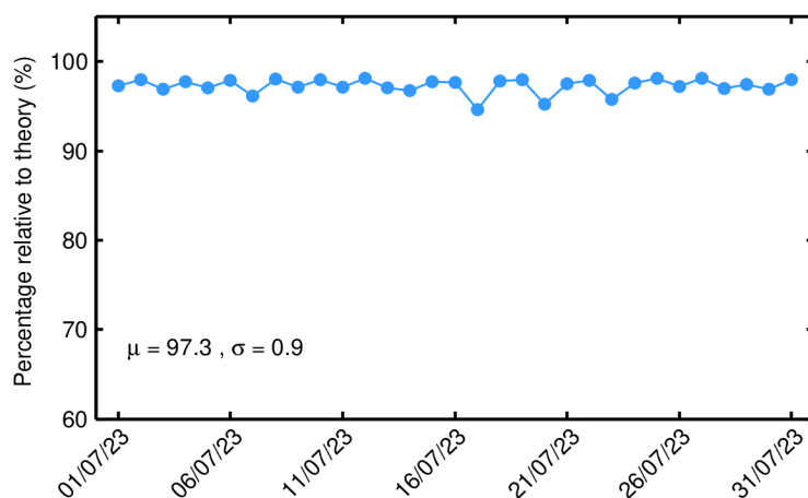
Figure 28. Percentage of science-valid NOP 1-Hz wind records over ocean and lakes relative to theory for each day in July 2023. The mean ( \mu ) and standard deviation ( \sigma ) are also shown.
