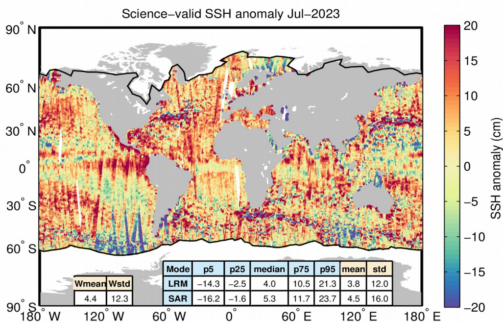
Figure 6. Geographical distribution of science-valid NOP 1-Hz SSH anomaly data over oceans and lakes for July 2023. The statistical values shown in the table refer to the SSH anomaly in cm and are calculated separately for LRM and SAR regions. Wmean and Wstd denote the spatial area-weighted average and its standard deviation. Measurements taken over polar polygons have been excluded from the computation of the statistical values. The black lines mark the outer limit of the Arctic and Antarctic polar polygons.
