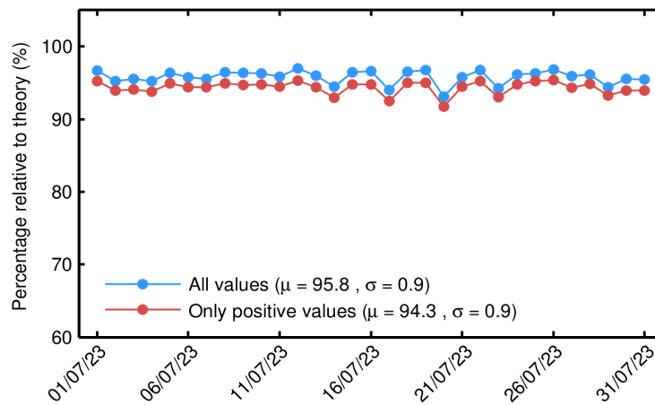
Figure 66. Percentage of science-valid IOP 1-Hz mispointing records over ocean and lakes relative to theory for each day in July 2023. The mean ( \mu ) and standard deviation ( \sigma ) are also shown.
