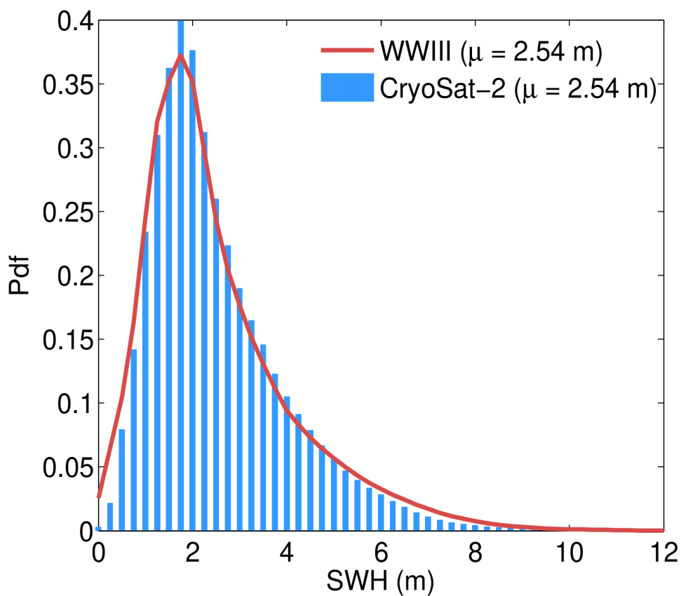
Figure 118. Histograms (normalized to have a total area of 1) of the GOP SWH (blue bars) and the SWH from the Wavewatch III model (red line) for July 2023.
