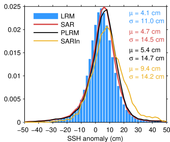
Figure 41. Histogram of science-valid IOP SSH anomaly over oceans and lakes for LRM (blue), SAR (red), PLRM (black) and SARIn (orange) for July 2023. The mean ( \mu ) and standard deviation ( \sigma ) are also shown. Values outside [-50\ 50] cm are excluded from the histogram for the sake of readability but not from the computation of \mu and \sigma .
