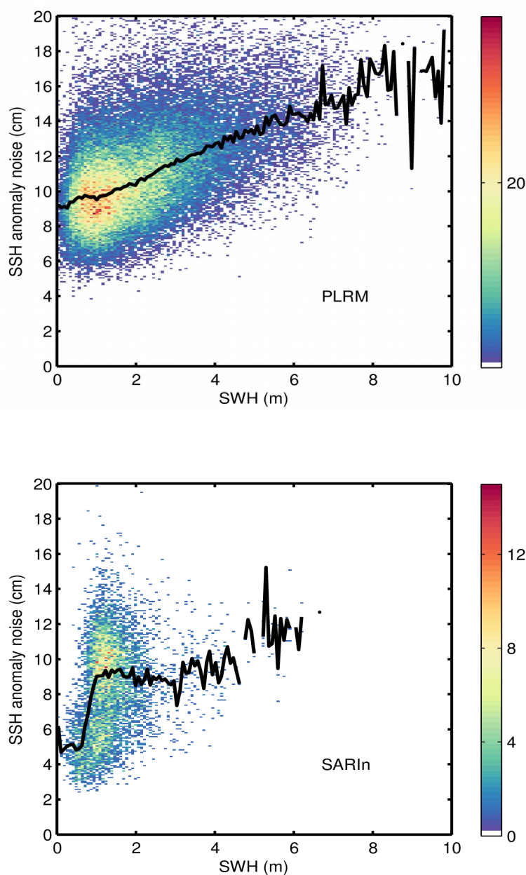
Figure 80. 2D histogram showing science-valid GOP SSH anomaly noise as a function of SWH for SAR, LRM, PLRM, and SARIn (from top to bottom) for July 2023. The black line denotes the median SSH anomaly noise as a function of SWH.
