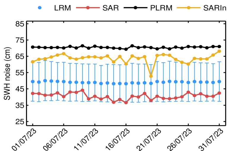
Figure 53. Mean science-valid IOP SWH noise for LRM (blue dot), SAR (red dot), PLRM (black dot) and SARIn (orange dot) for each day in July 2023. The corresponding standard deviation for LRM (blue error bar) is also shown.
