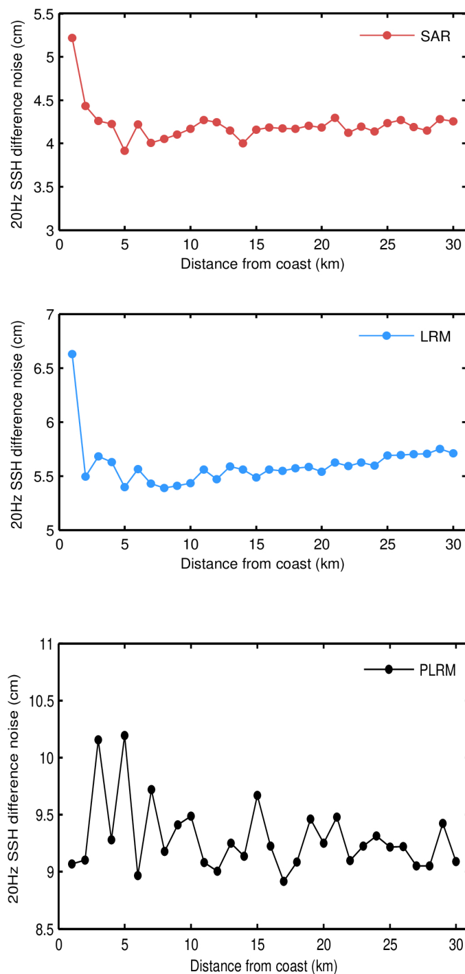
Figure 79. Science-valid GOP 20-Hz SSH anomaly noise as a function of distance from the coast for SAR (top panel), LRM (middle panel), and PLRM (bottom panel) for July 2023. Noise values have been calculated as the median of the absolute value of the difference between consecutive 20-Hz records.
