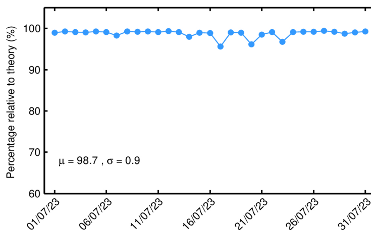
Figure 62. Percentage of science-valid IOP 1-Hz wind records over ocean and lakes relative to theory for each day in July 2023. The mean ( \mu ) and standard deviation ( \sigma ) are also shown.
