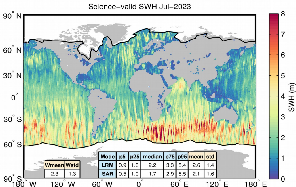
Figure 85. Geographical distribution of science-valid GOP SWH data over oceans and lakes for July 2023. The statistical values shown in the table refer to the SWH in m and are calculated separately for LRM and SAR regions. Wmean and Wstd denote the spatial area-weighted average and its standard deviation. Measurements taken over polar polygons have been excluded from the computation of the statistical values. The black lines mark the outer limit of the Arctic and Antarctic polar polygons.
