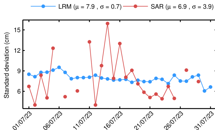
Figure 14. Standard deviation of differences at crossovers for NOP SSH anomaly for each day in July 2023. The values shown in this figure have been computed for the science-valid data further edited according to the following two additional criteria: 1) rejecting crossover differences larger than 20 cm; and 2) rejecting shallow waters (1000 m). The mean ( \mu ) and standard deviation ( \sigma ) are also shown.
