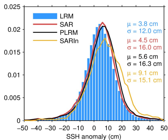
Figure 7. Histogram of science-valid NOP SSH anomaly over oceans and lakes for LRM (blue), SAR (red), PLRM (black) and SARIn (orange) for July 2023. The mean ( \mu ) and standard deviation ( \sigma ) are also shown. Values outside [-50 \ 50] cm are excluded from the histogram for the sake of readability but not from the computation of \mu and \sigma .
