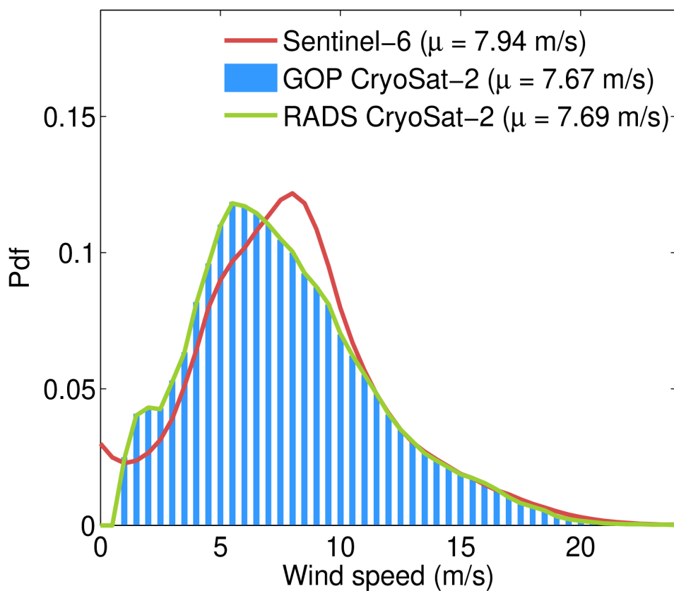
Figure 129. Histograms (normalized to have a total area of 1) of the wind speed from GOP (blue bars), reference mission (red line) and RADS CryoSat-2 (green) for July 2023.
