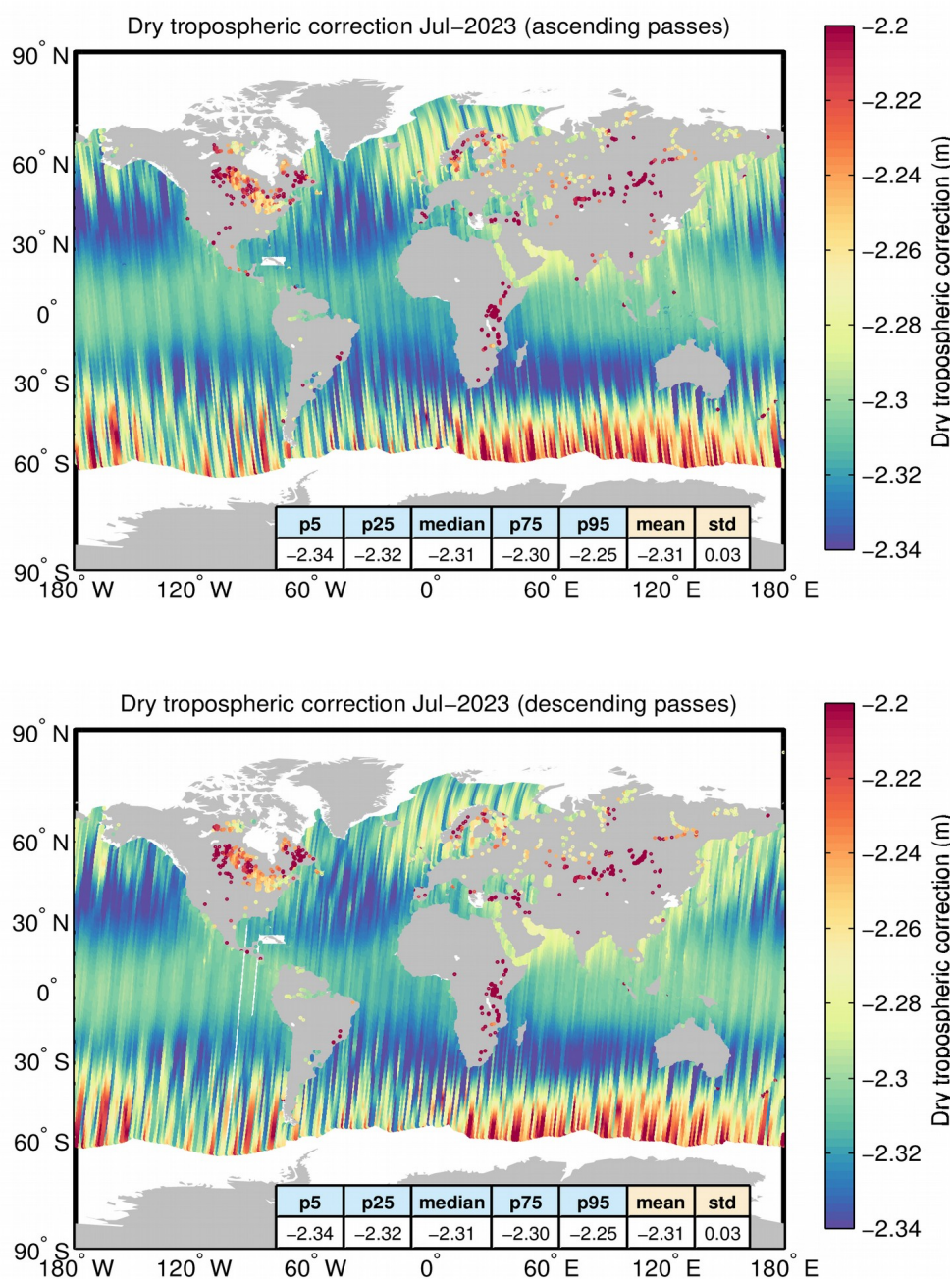
Figure A2. Geographical distribution of the dry tropospheric correction over oceans and lakes for ascending (top) and descending (bottom) passes for July 2023. The statistical values shown in the table refer to the dry tropospheric correction in m. Measurements taken over polar polygons have been excluded from the computation of the statistical values. The black lines mark the outer limit of the Arctic and Antarctic polar polygons.
