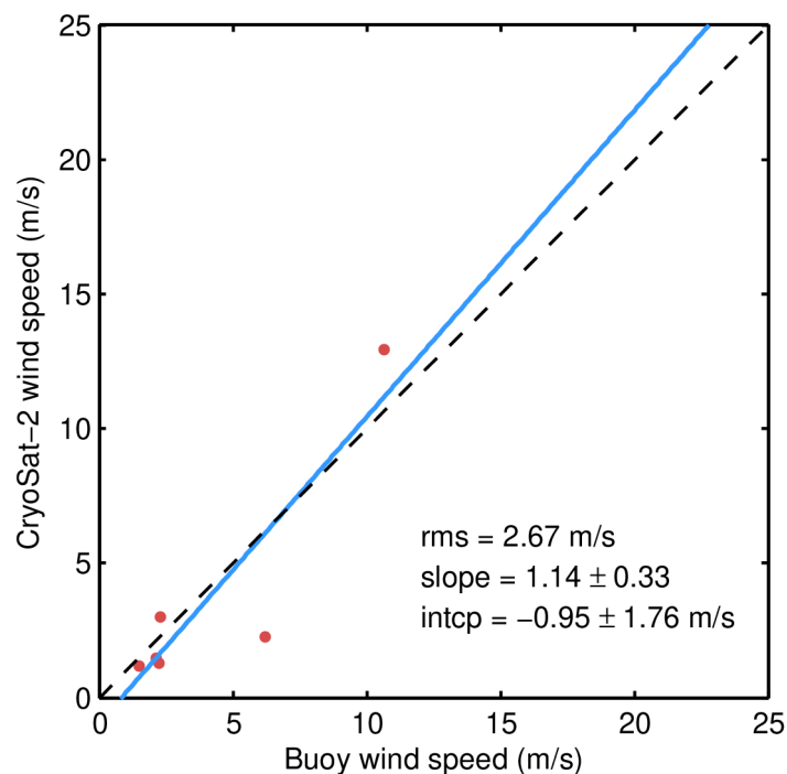
Figure 115. Scatter plot showing a comparison of GOP wind speed with wind speed from NDBC buoy data for July 2023.
