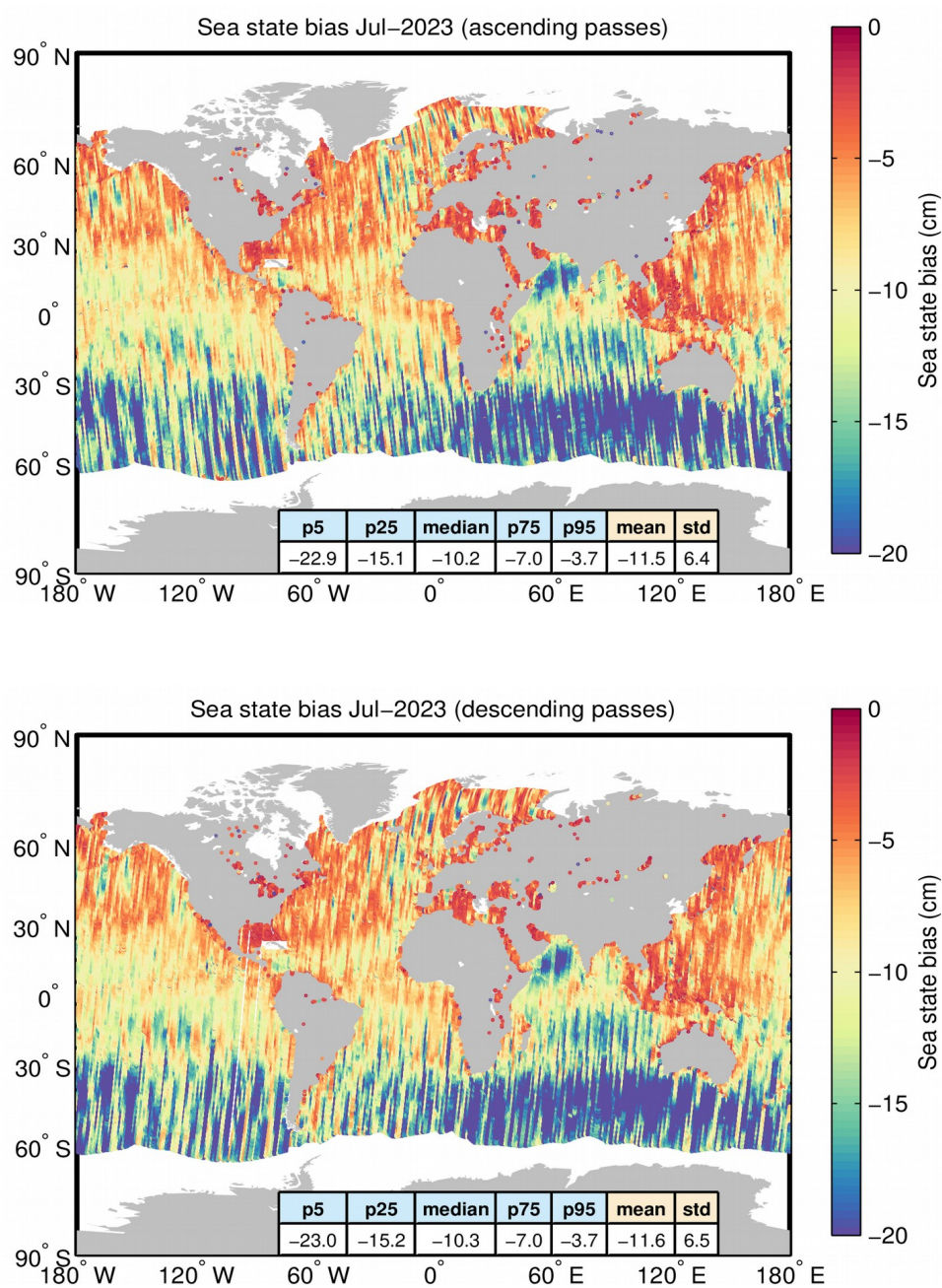
Figure A4. Geographical distribution of the sea state bias over oceans and lakes for ascending (top) and descending (bottom) passes for July 2023. The statistical values shown in the table refer to the sea state bias in cm. Measurements taken over polar polygons have been excluded from the computation of the statistical values. The black lines mark the outer limit of the Arctic and Antarctic polar polygons.
