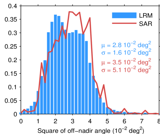
Figure 68. Histogram of science-valid IOP mispointing over oceans and lakes for LRM (blue) and SAR (red) for July 2023. The mean ( \mu ) and standard deviation ( \sigma ) are also shown. Note that values larger than 12 m are excluded from the histogram for the sake of readability but not from the computation of \mu and \sigma .
