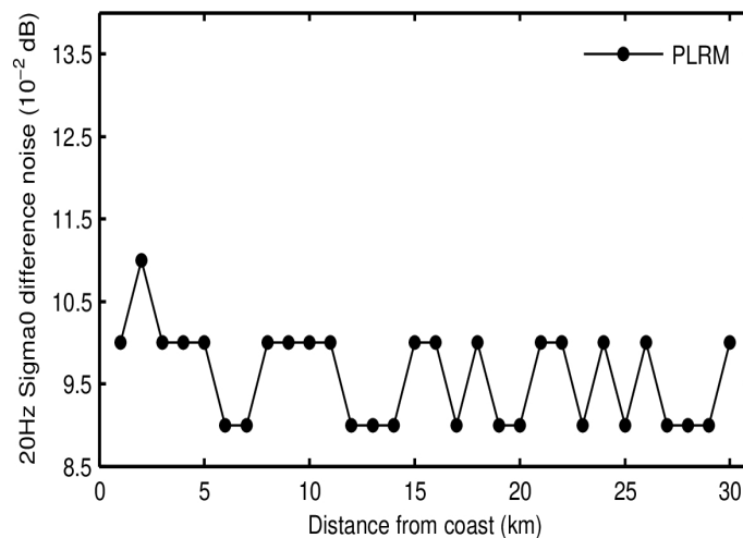
Figure 61. Science-valid IOP 20-Hz sigma0 noise as a function of distance from the coast for SAR (top panel), LRM (middle panel), and PLRM (bottom panel) for July 2023. Noise values have been calculated as the median of the absolute value of the difference between consecutive 20-Hz records.
