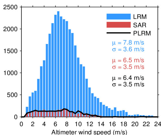
Figure 33. Histogram of flag-valid wind over oceans and lakes for LRM (blue), SAR (red), and PLRM (black) for 08/05/2024. The mean ( \mu ) and standard deviation ( \sigma ) are also shown. Note that values larger than 24 m/s are excluded from the histogram for the sake of readability but not from the computation of \mu and \sigma .
