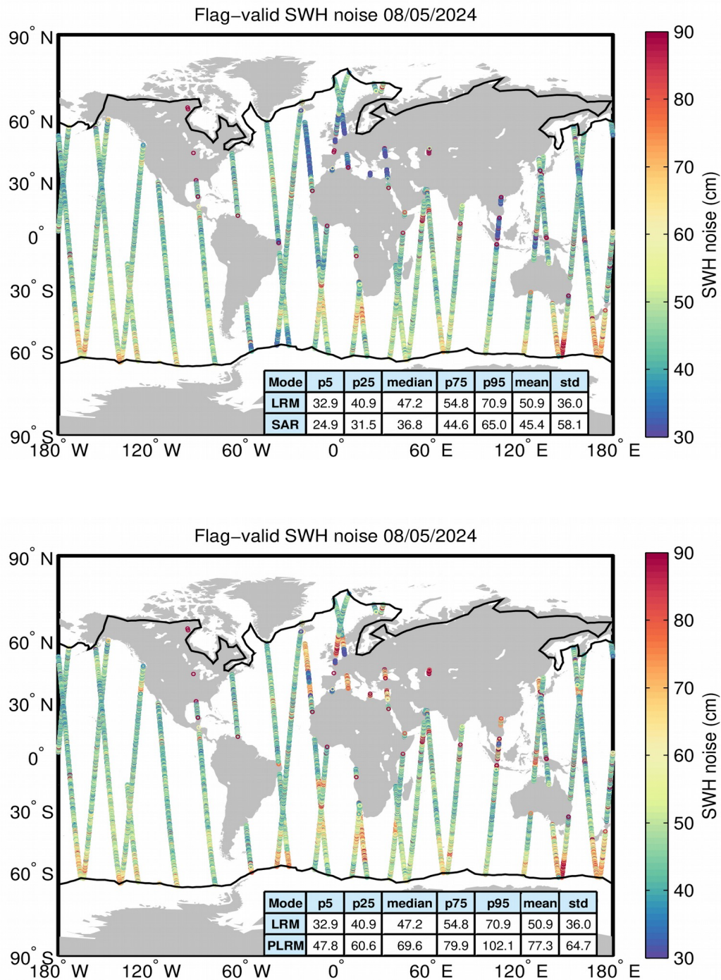
Figure 18. Geographical distribution of flag-valid 20-Hz SWH measurement noise over oceans and lakes for LRM/SAR (top) and LRM/PLRM (bottom) and for 08/05/2024. The statistical values shown in the table refer to the SWH noise and are calculated separately for LRM and SAR/PLRM regions. Measurements taken over polar polygons have been
