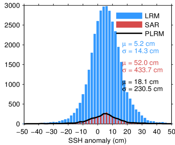
Figure 7. Histogram of flag-valid SSH anomaly over oceans and lakes for LRM (blue), SAR (red), and PLRM (black) for 08/05/2024. The mean ( \mu ) and standard deviation ( \sigma ) are also shown. Note that values outside [-50\ 50] cm are excluded from the histogram for the sake of readability but not from the computation of \mu and \sigma .
