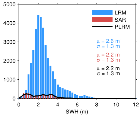
Figure 17. Histogram of flag-valid SWH over oceans and lakes for LRM (blue), SAR (red), and PLRM (black) for 08/05/2024. The mean ( \mu ) and standard deviation ( \sigma ) are also shown. Note that values larger than 12 m are excluded from the histogram for the sake of readability but not from the computation of \mu and \sigma .
