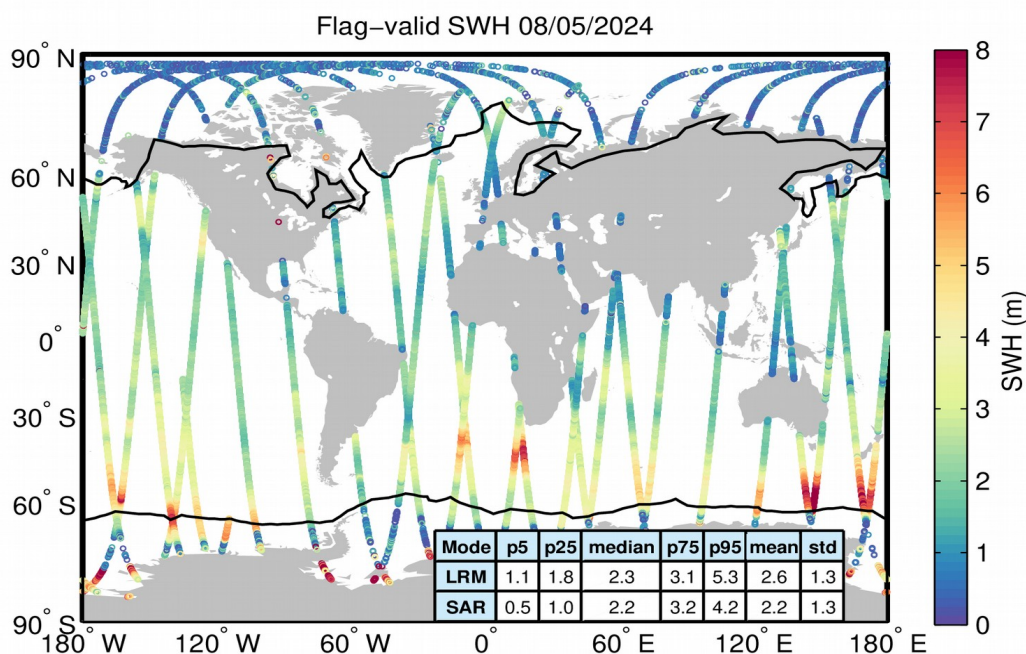
Figure 15. Geographical distribution of flag-valid SWH data over oceans and lakes for 08/05/2024. The statistical values shown in the table refer to the SWH in m and are calculated separately for LRM and SAR regions. Measurements taken over polar polygons have been excluded from the computation of the statistical values. The black lines mark the outer limit of the Arctic and Antarctic polar polygons.
