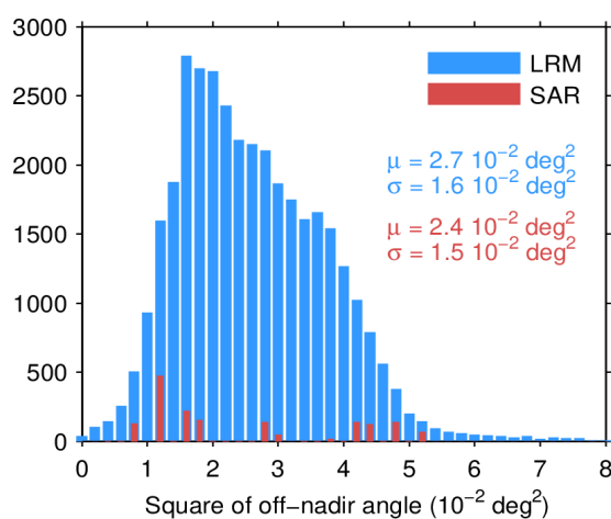
Figure 39. Histogram of flag-valid mispointing over oceans and lakes for LRM (blue) and SAR (red) for 08/05/2024. Only positive values have been considered. The mean ( \mu ) and standard deviation ( \sigma ) are also shown. Note that values larger than 8 \cdot 10^{-2} \text{ deg}^2 are excluded from the histogram for the sake of readability but not from the computation of \mu and \sigma .
