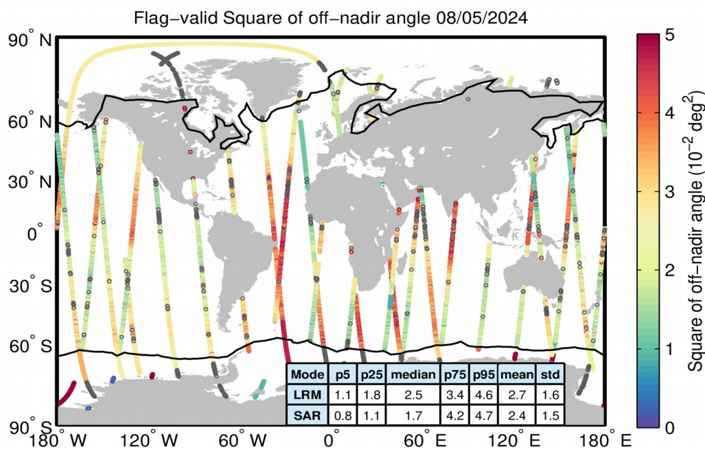
Figure 37. Geographical distribution of flag-valid mispointing data over oceans and lakes for 08/05/2024. The statistical values shown in the table refer to the mispointing in 10^{-2} \text{ deg}^2 and are calculated separately for LRM and SAR regions. Measurements taken over polar polygons have been excluded from the computation of the statistical values. The black lines mark the outer limit of the Arctic and Antarctic polar polygons. Gray circles denote negative values.
