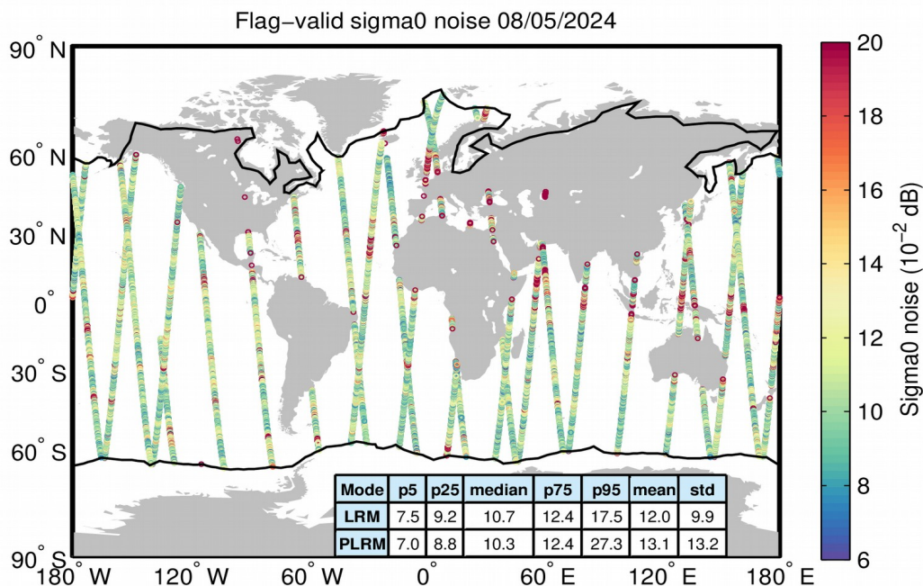
Figure 26. Geographical distribution of flag-valid 20-Hz sigma0 measurement noise over oceans and lakes for LRM/SAR (top) and LRM/PLRM (bottom) and for 08/05/2024. The statistical values shown in the table refer to the sigma0 noise and are calculated separately for LRM and SAR/PLRM regions. Measurements taken over polar polygons have been excluded from the computation of the statistical values. The black lines mark the outer limit of the Arctic and Antarctic polar polygons.
