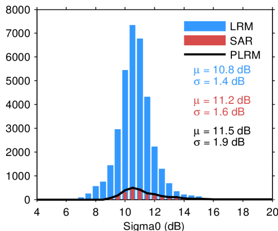
Figure 28. Histogram of science-valid sigma0 over oceans and lakes for LRM (blue), SAR (red), and PLRM (black) for 08/05/2024. The mean ( \mu ) and standard deviation ( \sigma ) are also shown. Note that values outside [4 20] dB are excluded from the histogram for the sake of readability but not from the computation of \mu and \sigma .
