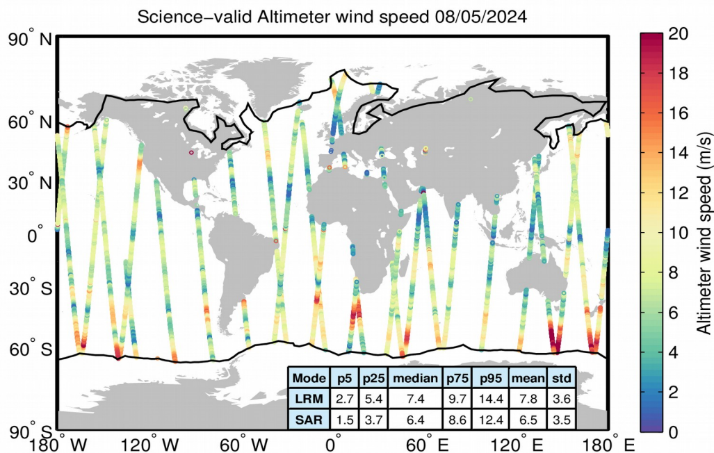
Figure 34. Geographical distribution of science-valid wind data over oceans and lakes for 08/05/2024. The statistical values shown in the table refer to the wind in m/s and are calculated separately for LRM and SAR regions. The black lines mark the outer limit of the Arctic and Antarctic polar polygons. Gray circles denote records that have been rejected based on the editing criteria described in Table 5.
