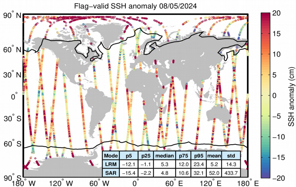
Figure 5. Geographical distribution of flag-valid 1-Hz SSH anomaly data over oceans and lakes for 08/05/2024. The statistical values shown in the table refer to the SSH anomaly in cm and are calculated separately for LRM and SAR regions. Measurements taken over polar polygons have been excluded from the computation of the statistical values. The black lines mark the outer limit of the Arctic and Antarctic polar polygons.
