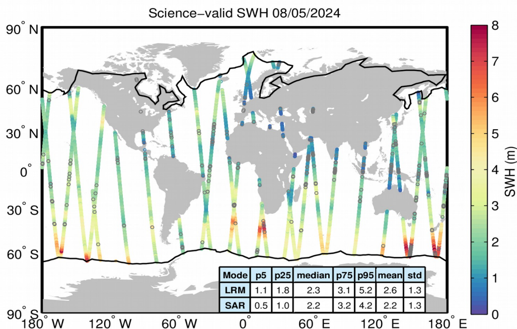
Figure 19. Geographical distribution of science-valid SWH data over oceans and lakes for 08/05/2024. The statistical values shown in the table refer to the SWH in m and are calculated separately for LRM and SAR regions. The black lines mark the outer limit of the Arctic and Antarctic polar polygons. Gray circles denote records that have been rejected based on the editing criteria described in Table 3.
