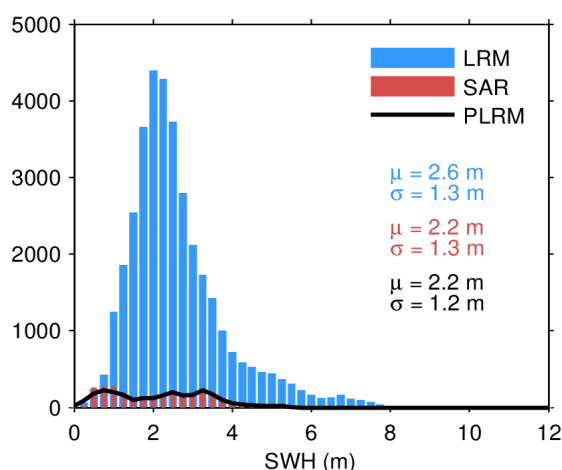
Figure 20. Histogram of science-valid SWH over oceans and lakes for LRM (blue), SAR (red), and PLRM (black) for 08/05/2024. The mean ( \mu ) and standard deviation ( \sigma ) are also
