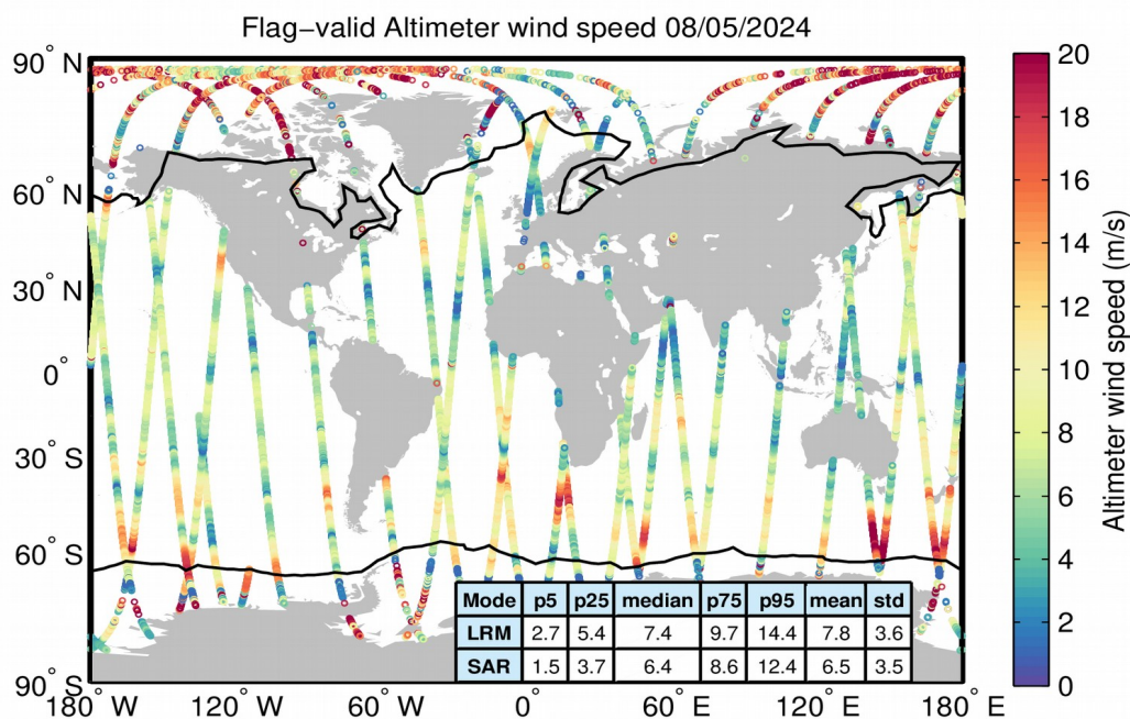
Figure 31. Geographical distribution of flag-valid wind data over oceans and lakes for 08/05/2024. The statistical values shown in the table refer to the wind in m/s and are calculated separately for LRM and SAR regions. Measurements taken over polar polygons have been excluded from the computation of the statistical values. The black lines mark the outer limit of the Arctic and Antarctic polar polygons.
