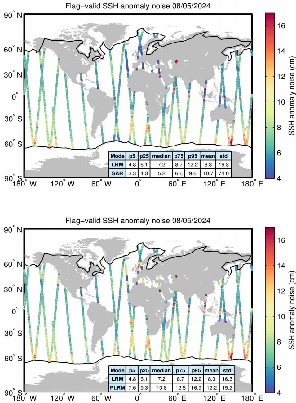
Figure 8. Geographical distribution of flag-valid 20-Hz SSH anomaly measurement noise over oceans and lakes for LRM/SAR (top) and LRM/PLRM (bottom) and for 08/05/2024. The statistical values shown in the tables refer to the SSH anomaly noise and are calculated separately for LRM and SAR/PLRM regions. Measurements taken over polar polygons have been excluded from the computation of the statistical values. The black lines mark the outer limit of the Arctic and Antarctic polar polygons.
