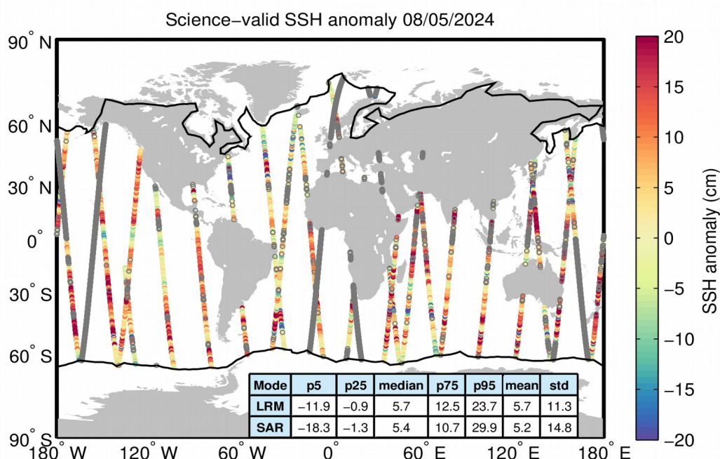
Figure 10. Geographical distribution of science-valid SSH anomaly data over oceans and lakes for 08/05/2024. The statistical values shown in the table refer to the SSH anomaly in cm and are calculated separately for LRM and SAR regions. The black lines mark the
