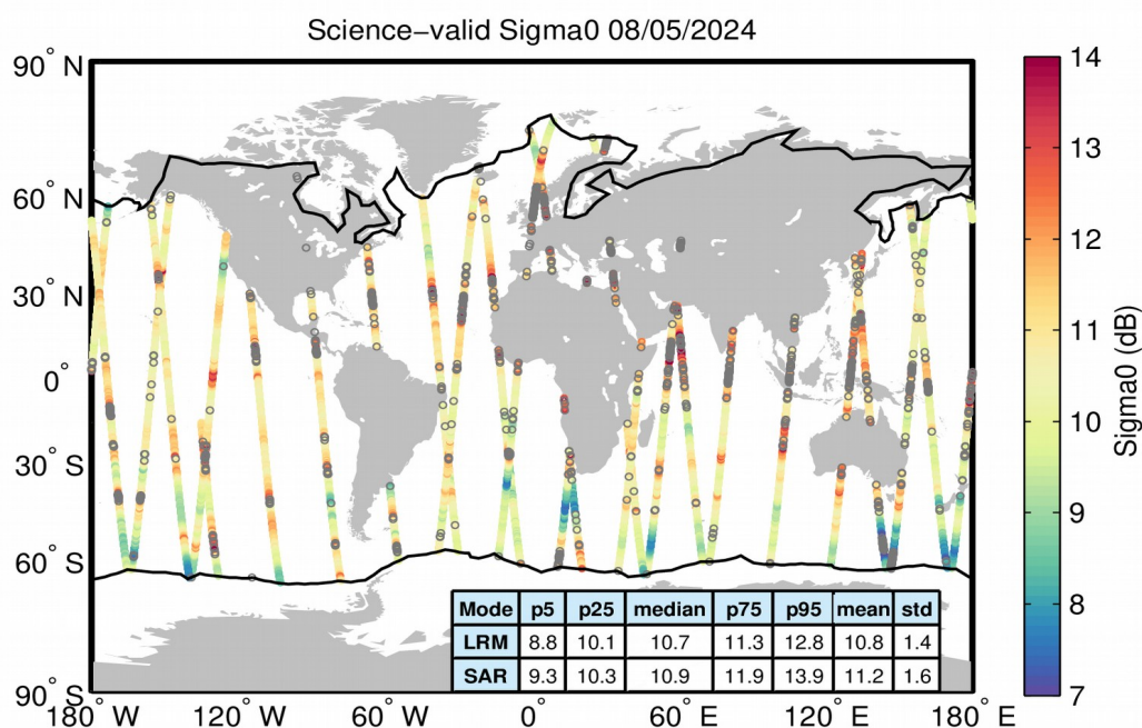
Figure 27. Geographical distribution of science-valid sigma0 data over oceans and lakes for 08/05/2024. The statistical values shown in the table refer to the sigma0 in dB and are calculated separately for LRM and SAR regions. The black lines mark the outer limit of the Arctic and Antarctic polar polygons. Gray circles denote records that have been rejected based on the editing criteria described in Table 4.
