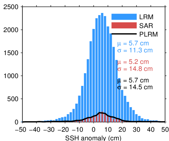
Figure 11. Histogram of science-valid SSH anomaly over oceans and lakes for LRM (blue), SAR (red), and PLRM (black) for 08/05/2024. The mean ( \mu ) and standard deviation ( \sigma ) are also shown. Note that values outside [-50\ 50] cm are excluded from the histogram for the sake of readability but not from the computation of \mu and \sigma .
