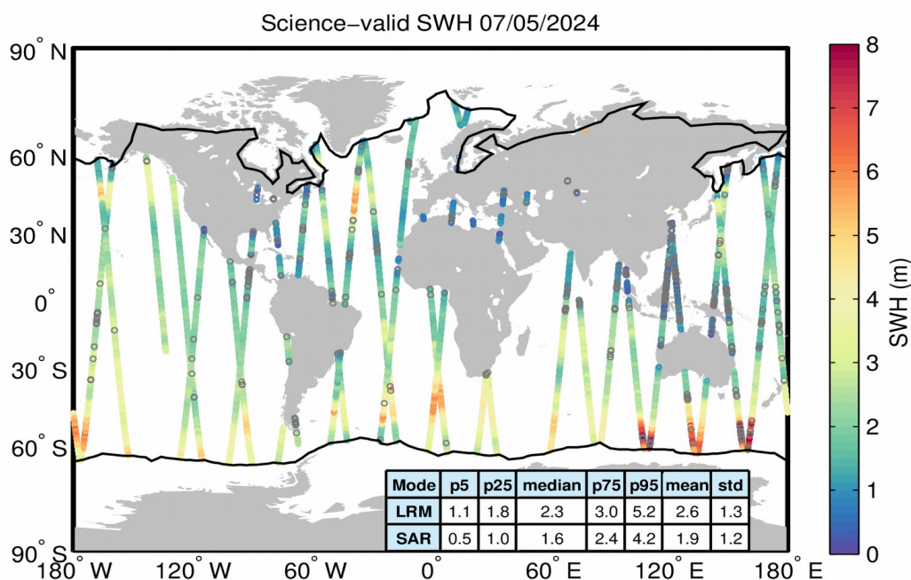
Figure 19. Geographical distribution of science-valid SWH data over oceans and lakes for 07/05/2024. The statistical values shown in the table refer to the SWH in m and are calculated separately for LRM and SAR regions. The black lines mark the outer limit of the Arctic and Antarctic polar polygons. Gray circles denote records that have been rejected based on the editing criteria described in Table 3.
