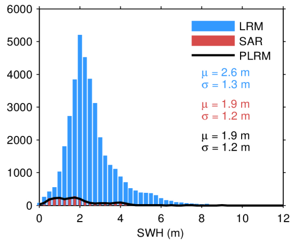
Figure 17. Histogram of flag-valid SWH over oceans and lakes for LRM (blue), SAR (red), and PLRM (black) for 07/05/2024. The mean ( \mu ) and standard deviation ( \sigma ) are also shown. Note that values larger than 12 m are excluded from the histogram for the sake of readability but not from the computation of \mu and \sigma .
