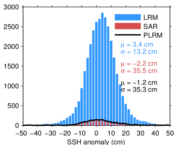
Figure 11. Histogram of science-valid SSH anomaly over oceans and lakes for LRM (blue), SAR (red), and PLRM (black) for 07/05/2024. The mean ( \mu ) and standard deviation ( \sigma ) are also shown. Note that values outside [-50, 50] cm are excluded from the histogram for the sake of readability but not from the computation of \mu and \sigma .
