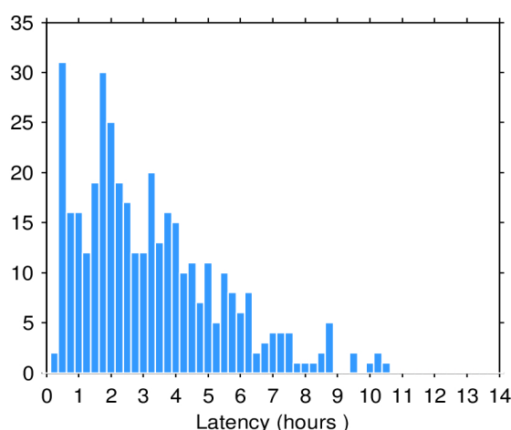
Figure 2. Histogram of the data latency for 07/05/2024. The y-axis denotes the number of files that are made available with a delay of x-hours with respect to the mean time of the records stored in the file.
