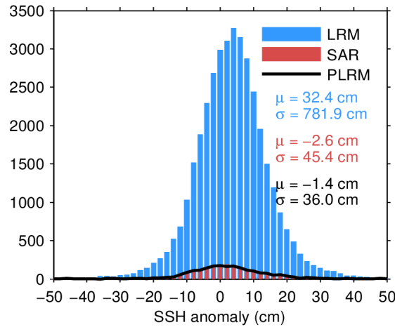
Figure 7. Histogram of flag-valid SSH anomaly over oceans and lakes for LRM (blue), SAR (red), and PLRM (black) for 07/05/2024. The mean ( \mu ) and standard deviation ( \sigma ) are also shown. Note that values outside [-50 50] cm are excluded from the histogram for the sake of readability but not from the computation of \mu and \sigma .
