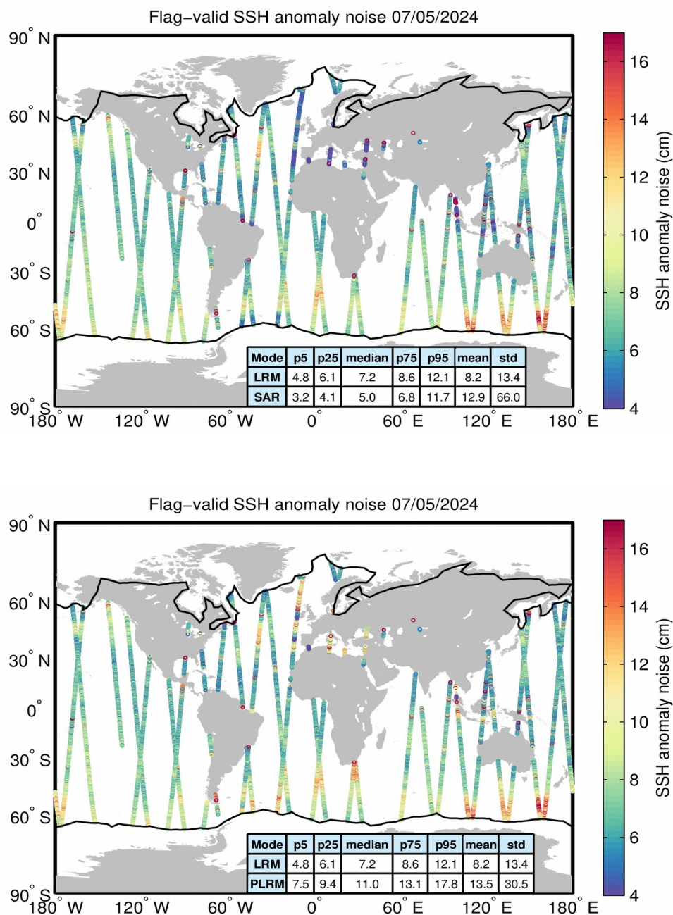
Figure 8. Geographical distribution of flag-valid 20-Hz SSH anomaly measurement noise over oceans and lakes for LRM/SAR (top) and LRM/PLRM (bottom) and for 07/05/2024. The statistical values shown in the tables refer to the SSH anomaly noise and are calculated separately for LRM and SAR/PLRM regions. Measurements taken over polar polygons have been excluded from the computation of the statistical values. The black lines mark the outer limit of the Arctic and Antarctic polar polygons.
