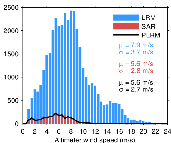
Figure 33. Histogram of flag-valid wind over oceans and lakes for LRM (blue), SAR (red), and PLRM (black) for 07/05/2024. The mean ( \mu ) and standard deviation ( \sigma ) are also shown. Note that values larger than 24 m/s are excluded from the histogram for the sake of readability but not from the computation of \mu and \sigma .
