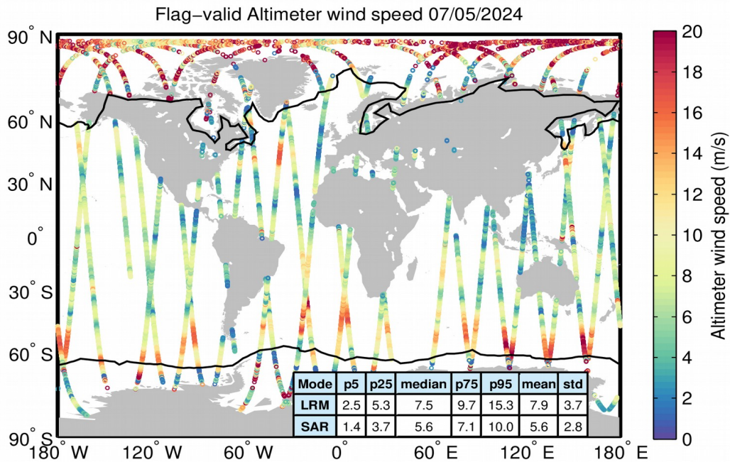
Figure 31. Geographical distribution of flag-valid wind data over oceans and lakes for 07/05/2024. The statistical values shown in the table refer to the wind in m/s and are calculated separately for LRM and SAR regions. Measurements taken over polar polygons have been excluded from the computation of the statistical values. The black lines mark the outer limit of the Arctic and Antarctic polar polygons.
