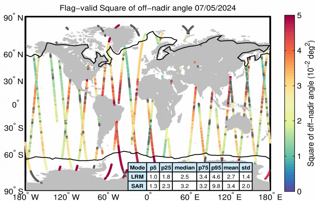
Figure 37. Geographical distribution of flag-valid mispointing data over oceans and lakes for 07/05/2024. The statistical values shown in the table refer to the mispointing in 10^{-2} \text{ deg}^2 and are calculated separately for LRM and SAR regions. Measurements taken over polar polygons have been excluded from the computation of the statistical values. The black lines mark the outer limit of the Arctic and Antarctic polar polygons. Gray circles denote negative values.
