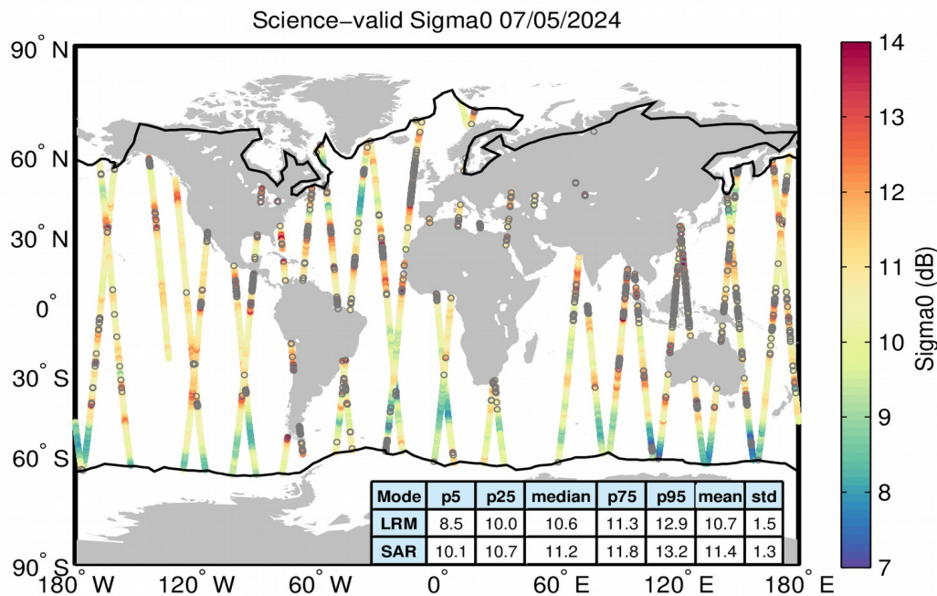
Figure 27. Geographical distribution of science-valid sigma0 data over oceans and lakes for 07/05/2024. The statistical values shown in the table refer to the sigma0 in dB and are calculated separately for LRM and SAR regions. The black lines mark the outer limit of the Arctic and Antarctic polar polygons. Gray circles denote records that have been rejected based on the editing criteria described in Table 4.
