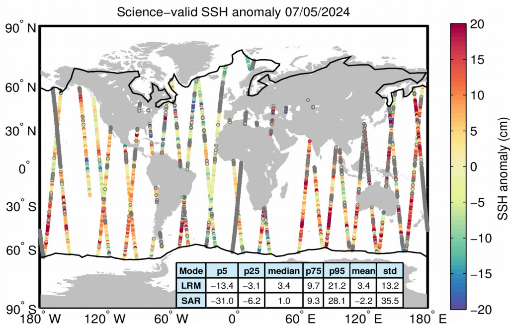
Figure 10. Geographical distribution of science-valid SSH anomaly data over oceans and lakes for 07/05/2024. The statistical values shown in the table refer to the SSH anomaly in cm and are calculated separately for LRM and SAR regions. The black lines mark the
