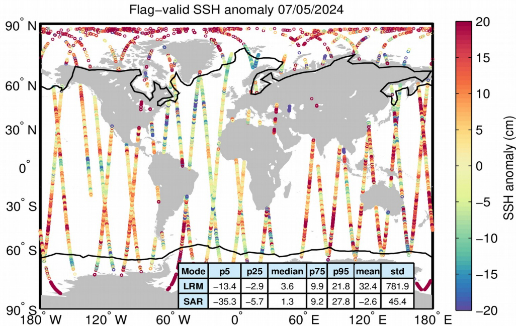
Figure 5. Geographical distribution of flag-valid 1-Hz SSH anomaly data over oceans and lakes for 07/05/2024. The statistical values shown in the table refer to the SSH anomaly in cm and are calculated separately for LRM and SAR regions. Measurements taken over polar polygons have been excluded from the computation of the statistical values. The black lines mark the outer limit of the Arctic and Antarctic polar polygons.
