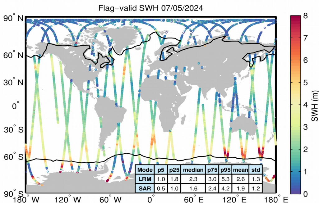
Figure 15. Geographical distribution of flag-valid SWH data over oceans and lakes for 07/05/2024. The statistical values shown in the table refer to the SWH in m and are calculated separately for LRM and SAR regions. Measurements taken over polar polygons have been excluded from the computation of the statistical values. The black lines mark the outer limit of the Arctic and Antarctic polar polygons.
