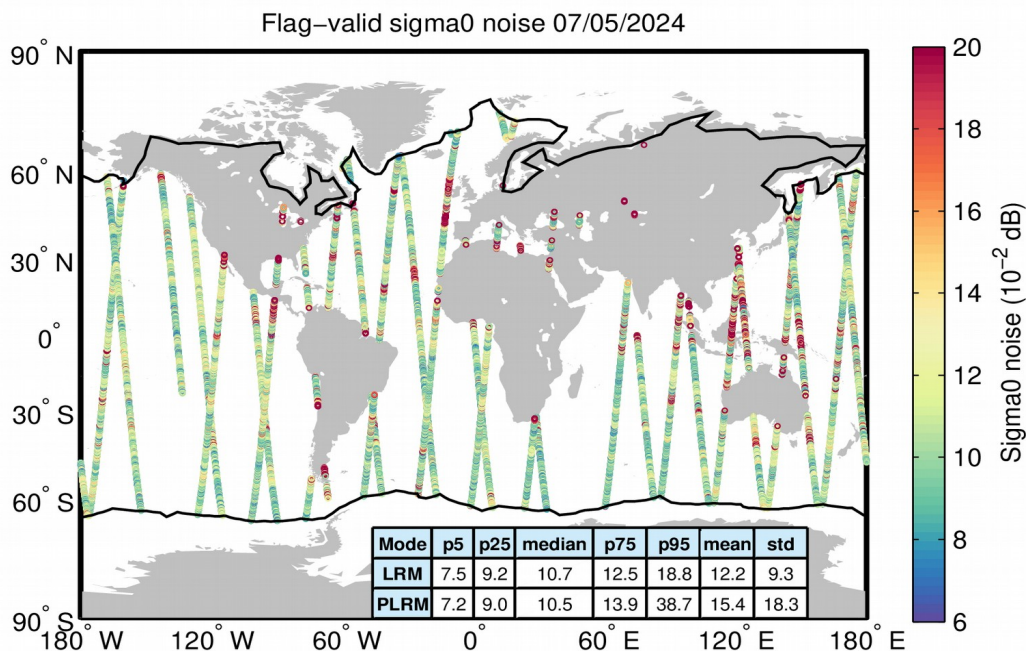
Figure 26. Geographical distribution of flag-valid 20-Hz sigma0 measurement noise over oceans and lakes for LRM/SAR (top) and LRM/PLRM (bottom) and for 07/05/2024. The statistical values shown in the table refer to the sigma0 noise and are calculated separately for LRM and SAR/PLRM regions. Measurements taken over polar polygons have been excluded from the computation of the statistical values. The black lines mark the outer limit of the Arctic and Antarctic polar polygons.
