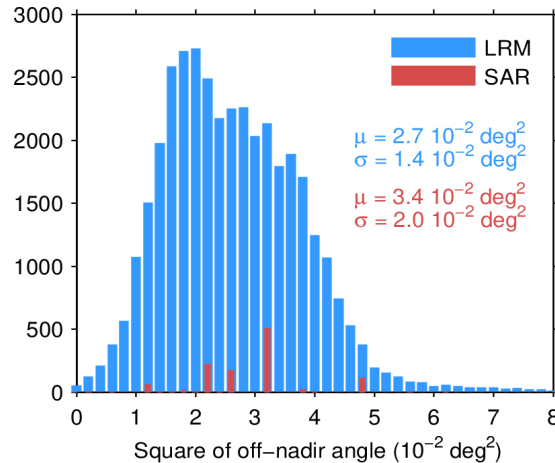
Figure 39. Histogram of flag-valid mispointing over oceans and lakes for LRM (blue) and SAR (red) for 07/05/2024. Only positive values have been considered. The mean ( \mu ) and standard deviation ( \sigma ) are also shown. Note that values larger than 8 \cdot 10^{-2} \text{ deg}^2 are excluded from the histogram for the sake of readability but not from the computation of \mu and \sigma .
