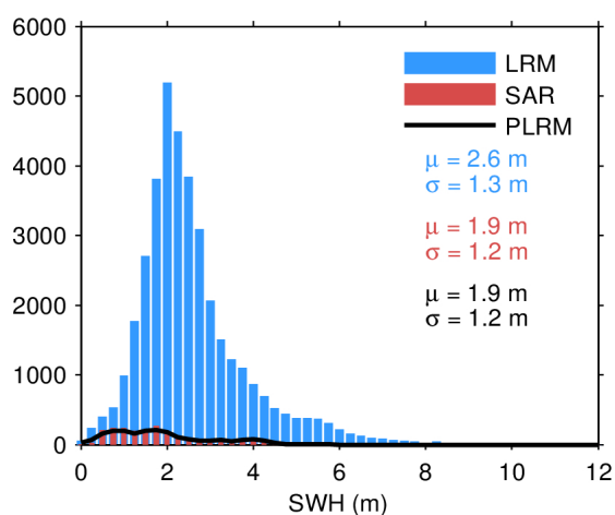
Figure 20. Histogram of science-valid SWH over oceans and lakes for LRM (blue), SAR (red), and PLRM (black) for 07/05/2024. The mean ( \mu ) and standard deviation ( \sigma ) are also
