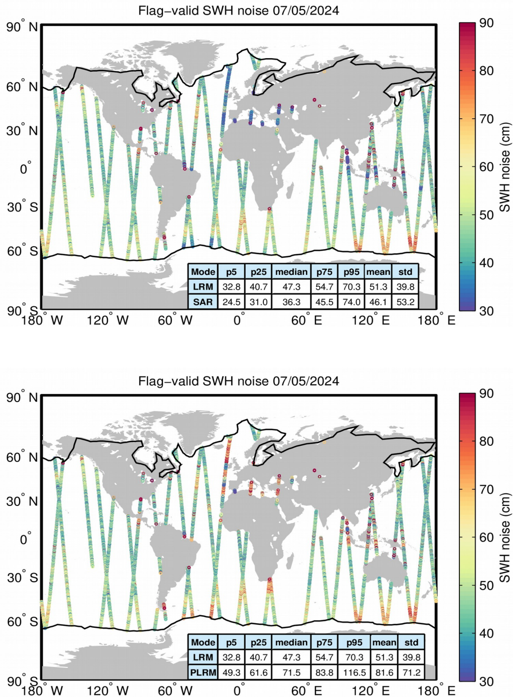
Figure 18. Geographical distribution of flag-valid 20-Hz SWH measurement noise over oceans and lakes for LRM/SAR (top) and LRM/PLRM (bottom) and for 07/05/2024. The statistical values shown in the table refer to the SWH noise and are calculated separately for LRM and SAR/PLRM regions. Measurements taken over polar polygons have been
