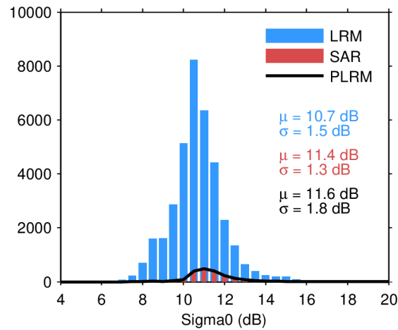
Figure 28. Histogram of science-valid sigma0 over oceans and lakes for LRM (blue), SAR (red), and PLRM (black) for 07/05/2024. The mean ( \mu ) and standard deviation ( \sigma ) are also shown. Note that values outside [4 20] dB are excluded from the histogram for the sake of readability but not from the computation of \mu and \sigma .
