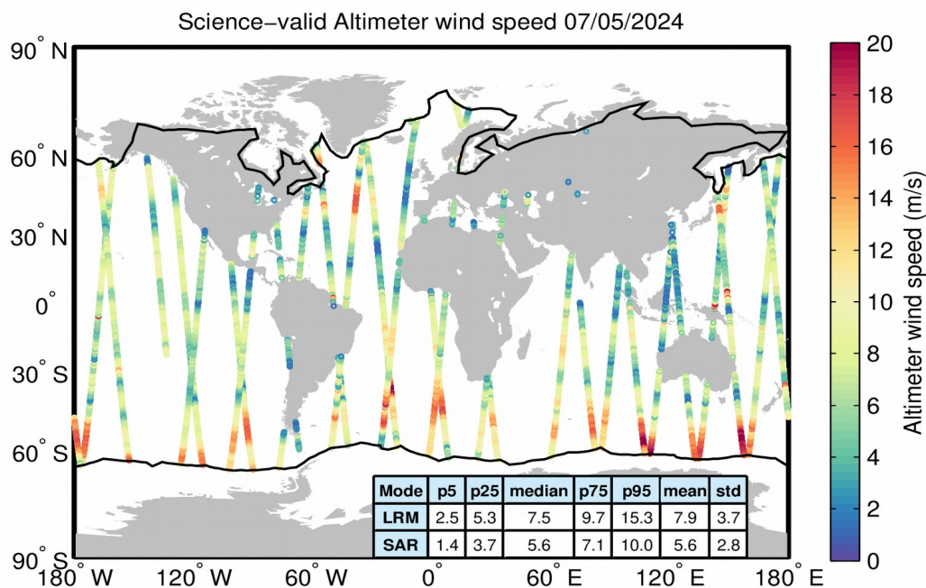
Figure 34. Geographical distribution of science-valid wind data over oceans and lakes for 07/05/2024. The statistical values shown in the table refer to the wind in m/s and are calculated separately for LRM and SAR regions. The black lines mark the outer limit of the Arctic and Antarctic polar polygons. Gray circles denote records that have been rejected based on the editing criteria described in Table 5.
