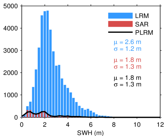
Figure 17. Histogram of flag-valid SWH over oceans and lakes for LRM (blue), SAR (red), and PLRM (black) for 06/05/2024. The mean ( \mu ) and standard deviation ( \sigma ) are also shown. Note that values larger than 12 m are excluded from the histogram for the sake of readability but not from the computation of \mu and \sigma .
