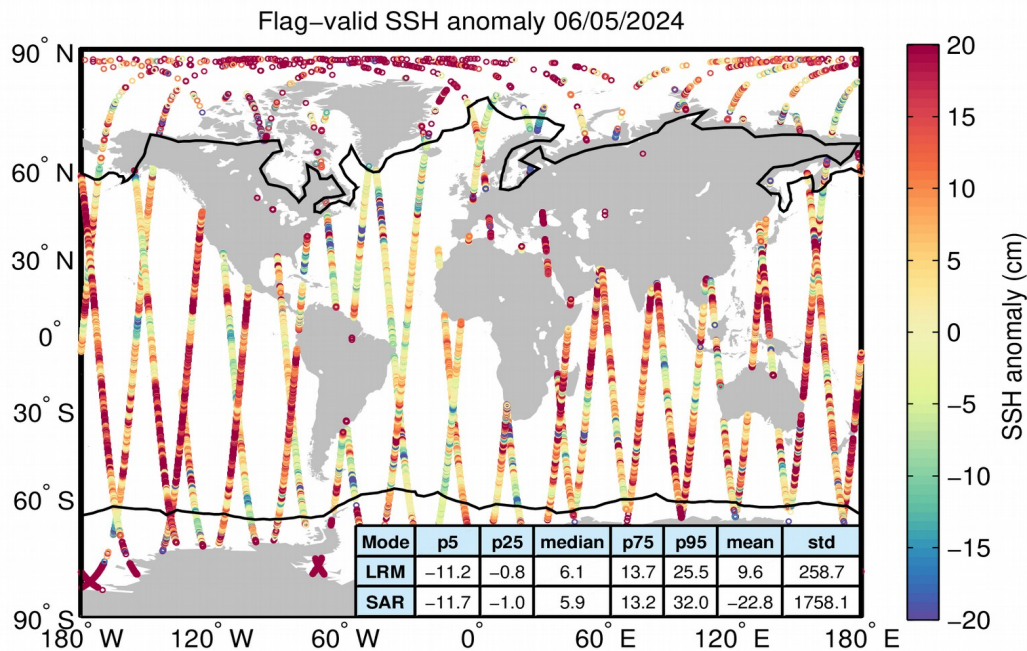
Figure 5. Geographical distribution of flag-valid 1-Hz SSH anomaly data over oceans and lakes for 06/05/2024. The statistical values shown in the table refer to the SSH anomaly in cm and are calculated separately for LRM and SAR regions. Measurements taken over polar polygons have been excluded from the computation of the statistical values. The black lines mark the outer limit of the Arctic and Antarctic polar polygons.
