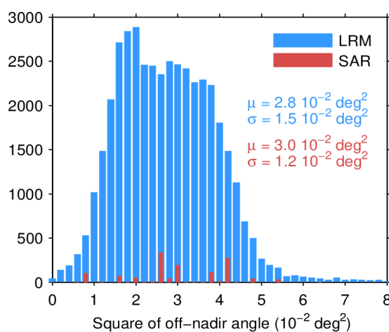
Figure 39. Histogram of flag-valid mispointing over oceans and lakes for LRM (blue) and SAR (red) for 06/05/2024. Only positive values have been considered. The mean ( \mu ) and standard deviation ( \sigma ) are also shown. Note that values larger than 8 \cdot 10^{-2} \text{ deg}^2 are excluded from the histogram for the sake of readability but not from the computation of \mu and \sigma .
