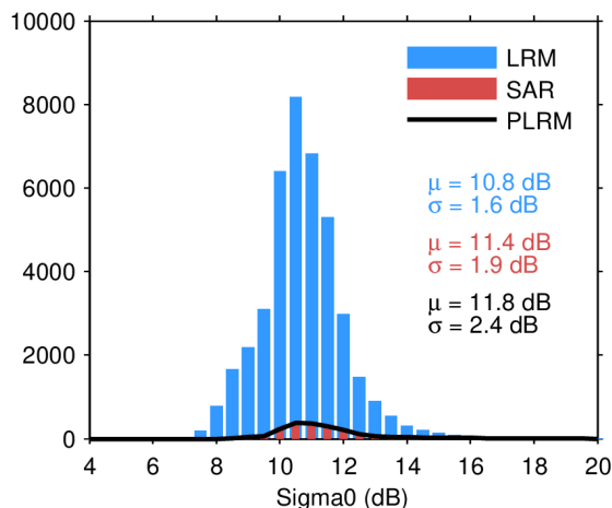
Figure 28. Histogram of science-valid sigma0 over oceans and lakes for LRM (blue), SAR (red), and PLRM (black) for 06/05/2024. The mean ( \mu ) and standard deviation ( \sigma ) are also shown. Note that values outside [4 20] dB are excluded from the histogram for the sake of readability but not from the computation of \mu and \sigma .
