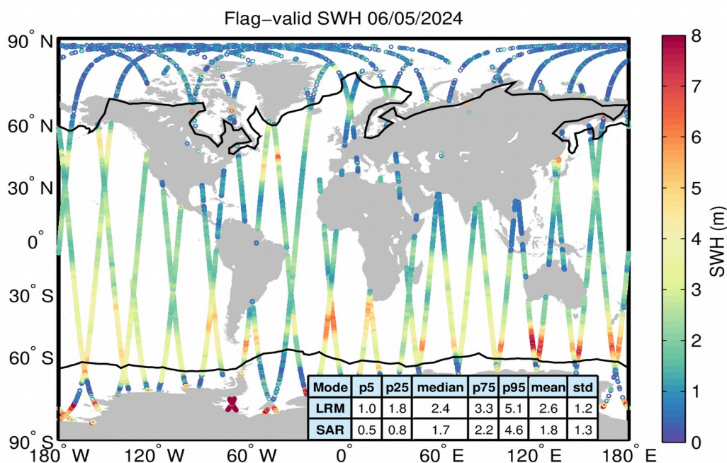
Figure 15. Geographical distribution of flag-valid SWH data over oceans and lakes for 06/05/2024. The statistical values shown in the table refer to the SWH in m and are calculated separately for LRM and SAR regions. Measurements taken over polar polygons have been excluded from the computation of the statistical values. The black lines mark the outer limit of the Arctic and Antarctic polar polygons.
