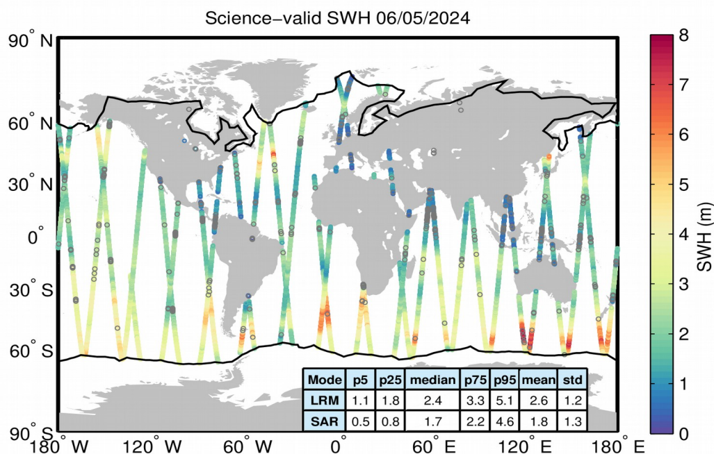
Figure 19. Geographical distribution of science-valid SWH data over oceans and lakes for 06/05/2024. The statistical values shown in the table refer to the SWH in m and are calculated separately for LRM and SAR regions. The black lines mark the outer limit of the Arctic and Antarctic polar polygons. Gray circles denote records that have been rejected based on the editing criteria described in Table 3.
