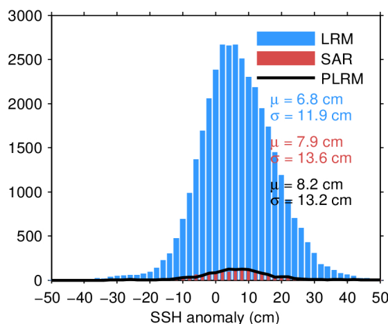
Figure 11. Histogram of science-valid SSH anomaly over oceans and lakes for LRM (blue), SAR (red), and PLRM (black) for 06/05/2024. The mean ( \mu ) and standard deviation ( \sigma ) are also shown. Note that values outside [-50\ 50] cm are excluded from the histogram for the sake of readability but not from the computation of \mu and \sigma .
