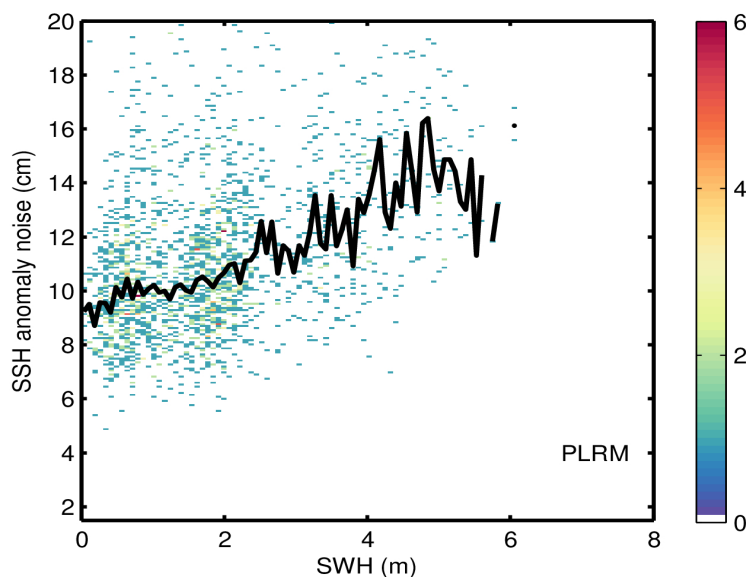
Figure 9. 2D histogram showing flag-valid SSH anomaly noise as a function of SWH for LRM (top), SAR (middle), and PLRM (bottom) for 06/05/2024. The black line denotes the median SSH anomaly noise as a function of SWH.
