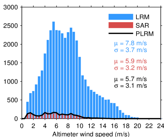
Figure 33. Histogram of flag-valid wind over oceans and lakes for LRM (blue), SAR (red), and PLRM (black) for 06/05/2024. The mean ( \mu ) and standard deviation ( \sigma ) are also shown. Note that values larger than 24 m/s are excluded from the histogram for the sake of readability but not from the computation of \mu and \sigma .
