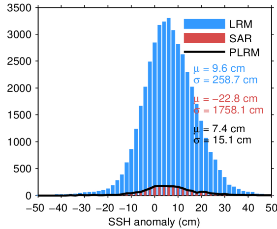
Figure 7. Histogram of flag-valid SSH anomaly over oceans and lakes for LRM (blue), SAR (red), and PLRM (black) for 06/05/2024. The mean ( \mu ) and standard deviation ( \sigma ) are also shown. Note that values outside [-50\ 50] cm are excluded from the histogram for the sake of readability but not from the computation of \mu and \sigma .
