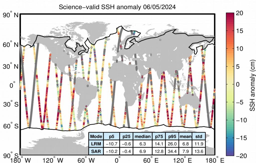
Figure 10. Geographical distribution of science-valid SSH anomaly data over oceans and lakes for 06/05/2024. The statistical values shown in the table refer to the SSH anomaly in cm and are calculated separately for LRM and SAR regions. The black lines mark the
