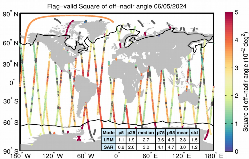
Figure 37. Geographical distribution of flag-valid mispointing data over oceans and lakes for 06/05/2024. The statistical values shown in the table refer to the mispointing in 10^{-2} \text{ deg}^2 and are calculated separately for LRM and SAR regions. Measurements taken over polar polygons have been excluded from the computation of the statistical values. The black lines mark the outer limit of the Arctic and Antarctic polar polygons. Gray circles denote negative values.
