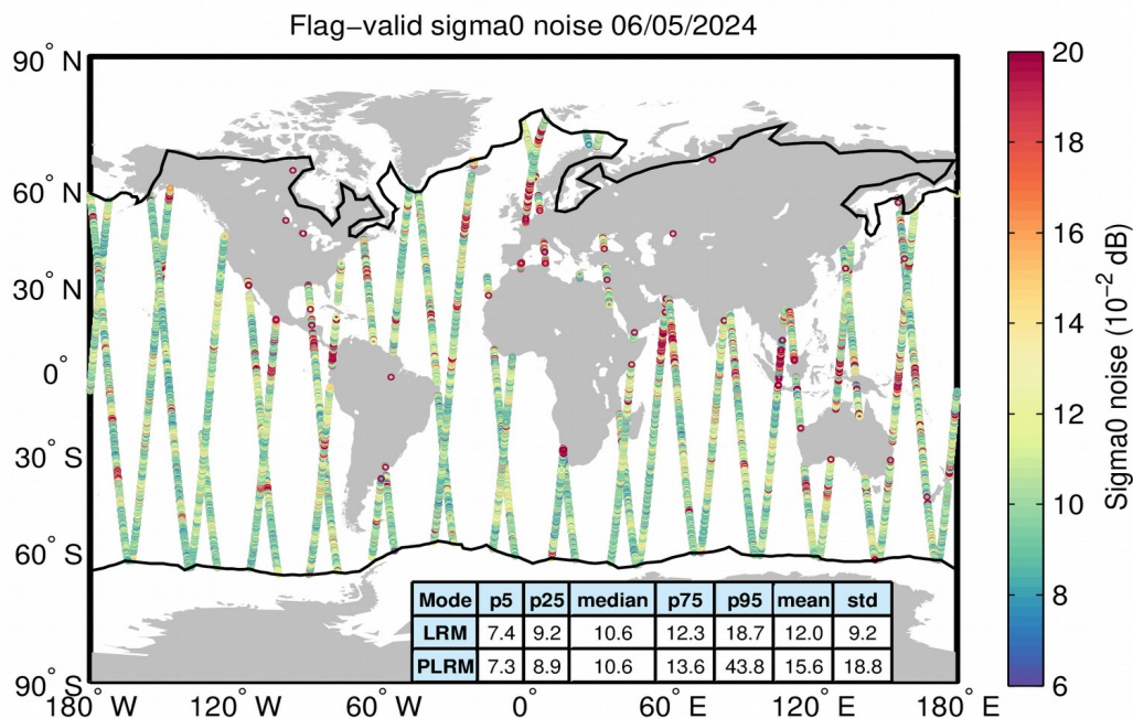
Figure 26. Geographical distribution of flag-valid 20-Hz sigma0 measurement noise over oceans and lakes for LRM/SAR (top) and LRM/PLRM (bottom) and for 06/05/2024. The statistical values shown in the table refer to the sigma0 noise and are calculated separately for LRM and SAR/PLRM regions. Measurements taken over polar polygons have been excluded from the computation of the statistical values. The black lines mark the outer limit of the Arctic and Antarctic polar polygons.
