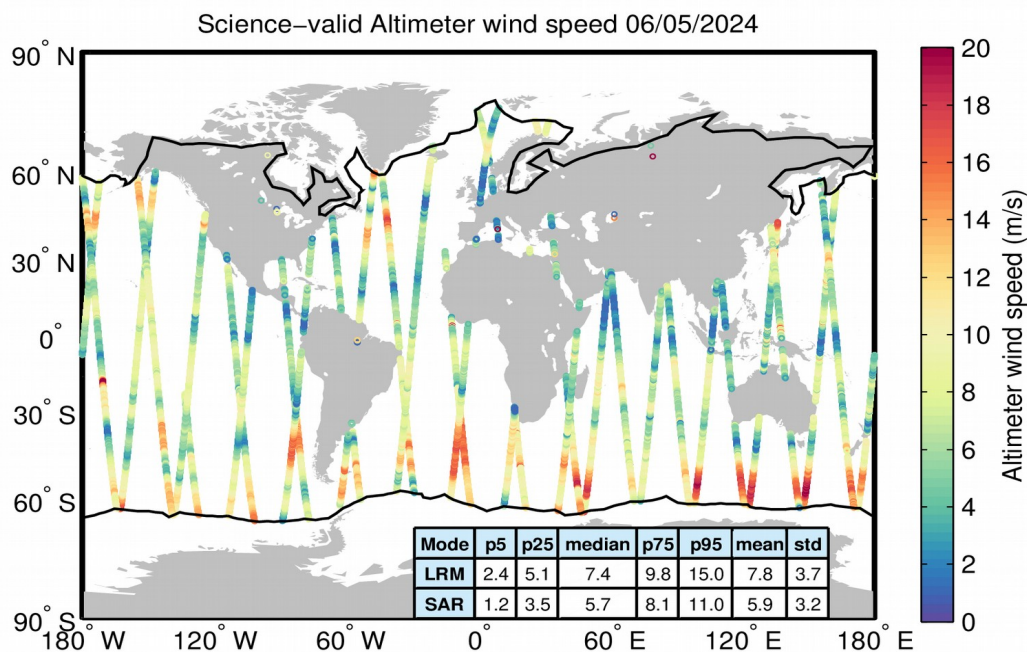
Figure 34. Geographical distribution of science-valid wind data over oceans and lakes for 06/05/2024. The statistical values shown in the table refer to the wind in m/s and are calculated separately for LRM and SAR regions. The black lines mark the outer limit of the Arctic and Antarctic polar polygons. Gray circles denote records that have been rejected based on the editing criteria described in Table 5.
