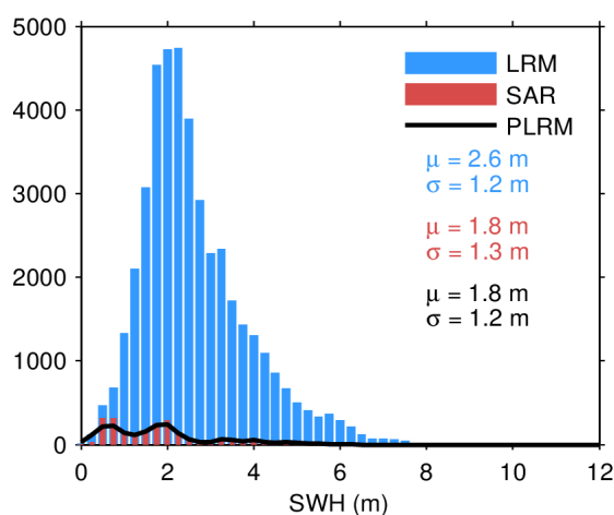
Figure 20. Histogram of science-valid SWH over oceans and lakes for LRM (blue), SAR (red), and PLRM (black) for 06/05/2024. The mean ( \mu ) and standard deviation ( \sigma ) are also
