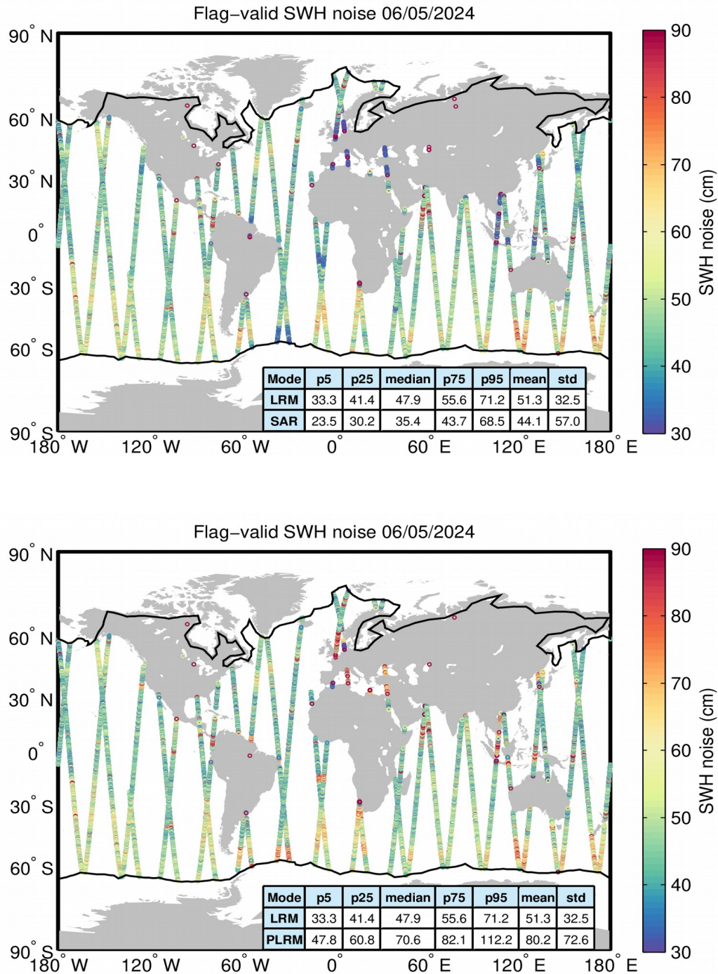
Figure 18. Geographical distribution of flag-valid 20-Hz SWH measurement noise over oceans and lakes for LRM/SAR (top) and LRM/PLRM (bottom) and for 06/05/2024. The statistical values shown in the table refer to the SWH noise and are calculated separately for LRM and SAR/PLRM regions. Measurements taken over polar polygons have been
