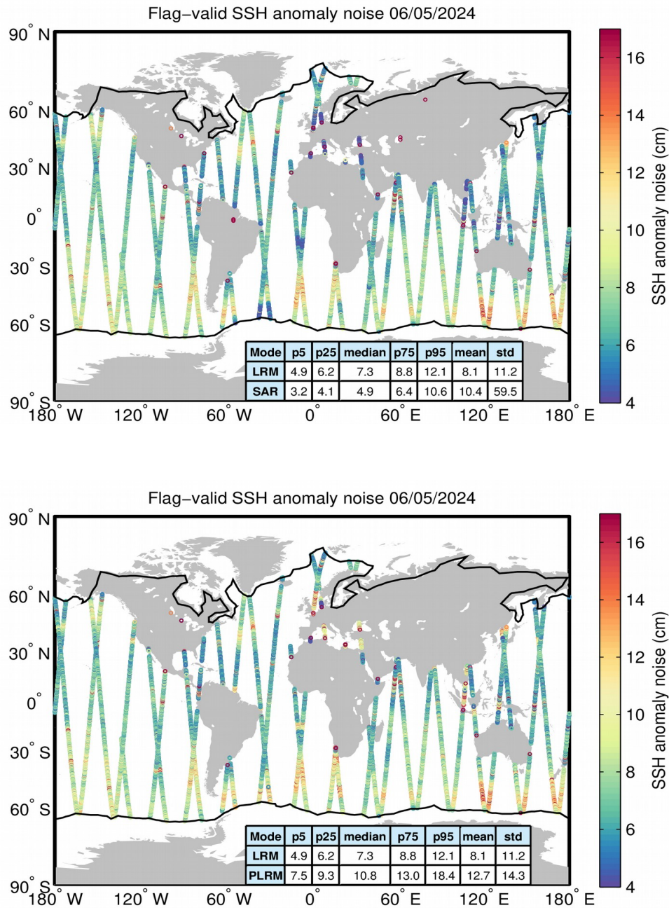
Figure 8. Geographical distribution of flag-valid 20-Hz SSH anomaly measurement noise over oceans and lakes for LRM/SAR (top) and LRM/PLRM (bottom) and for 06/05/2024. The statistical values shown in the tables refer to the SSH anomaly noise and are calculated separately for LRM and SAR/PLRM regions. Measurements taken over polar polygons have been excluded from the computation of the statistical values. The black lines mark the outer limit of the Arctic and Antarctic polar polygons.
