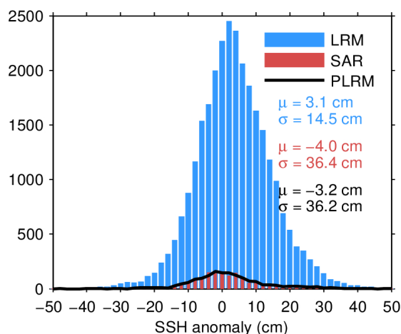
Figure 11. Histogram of science-valid SSH anomaly over oceans and lakes for LRM (blue), SAR (red), and PLRM (black) for 05/05/2024. The mean ( \mu ) and standard deviation ( \sigma ) are also shown. Note that values outside [-50\ 50] cm are excluded from the histogram for the sake of readability but not from the computation of \mu and \sigma .
