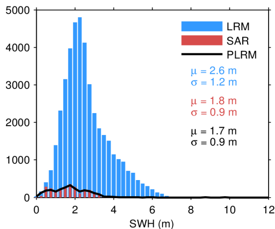
Figure 17. Histogram of flag-valid SWH over oceans and lakes for LRM (blue), SAR (red), and PLRM (black) for 05/05/2024. The mean ( \mu ) and standard deviation ( \sigma ) are also shown. Note that values larger than 12 m are excluded from the histogram for the sake of readability but not from the computation of \mu and \sigma .
