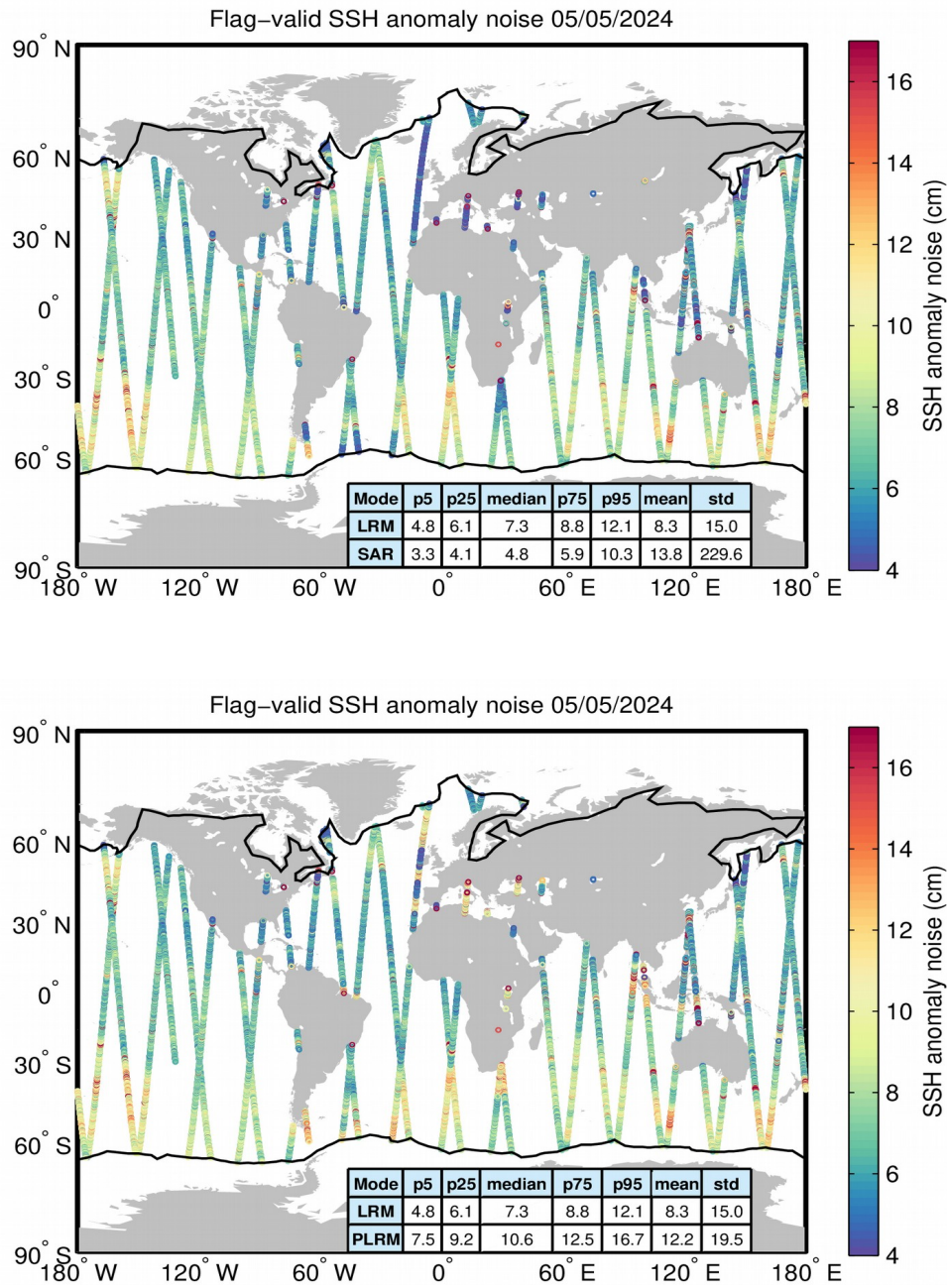
Figure 8. Geographical distribution of flag-valid 20-Hz SSH anomaly measurement noise over oceans and lakes for LRM/SAR (top) and LRM/PLRM (bottom) and for 05/05/2024. The statistical values shown in the tables refer to the SSH anomaly noise and are calculated separately for LRM and SAR/PLRM regions. Measurements taken over polar polygons have been excluded from the computation of the statistical values. The black lines mark the outer limit of the Arctic and Antarctic polar polygons.
