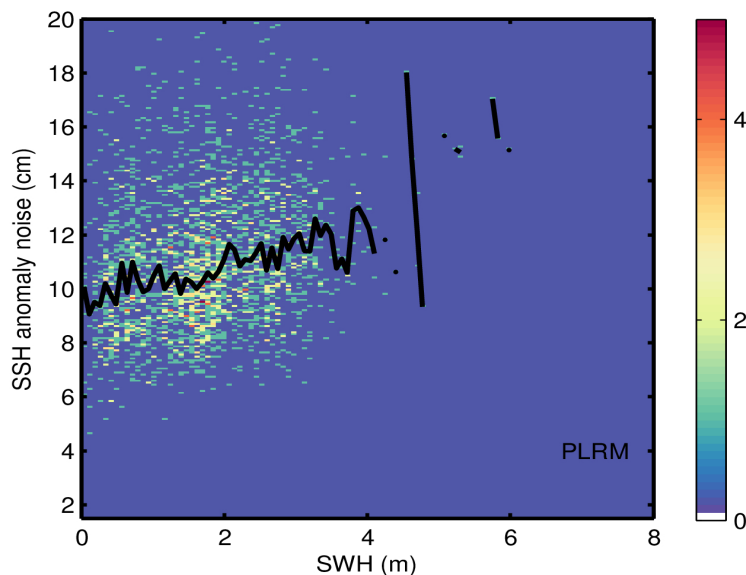
Figure 9. 2D histogram showing flag-valid SSH anomaly noise as a function of SWH for LRM (top), SAR (middle), and PLRM (bottom) for 05/05/2024. The black line denotes the median SSH anomaly noise as a function of SWH.
