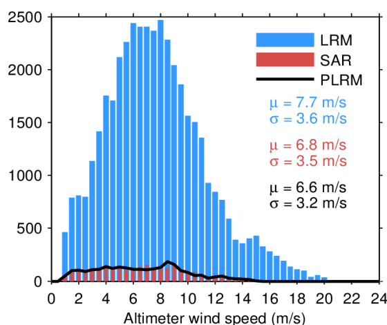
Figure 33. Histogram of flag-valid wind over oceans and lakes for LRM (blue), SAR (red), and PLRM (black) for 05/05/2024. The mean ( \mu ) and standard deviation ( \sigma ) are also shown. Note that values larger than 24 m/s are excluded from the histogram for the sake of readability but not from the computation of \mu and \sigma .
