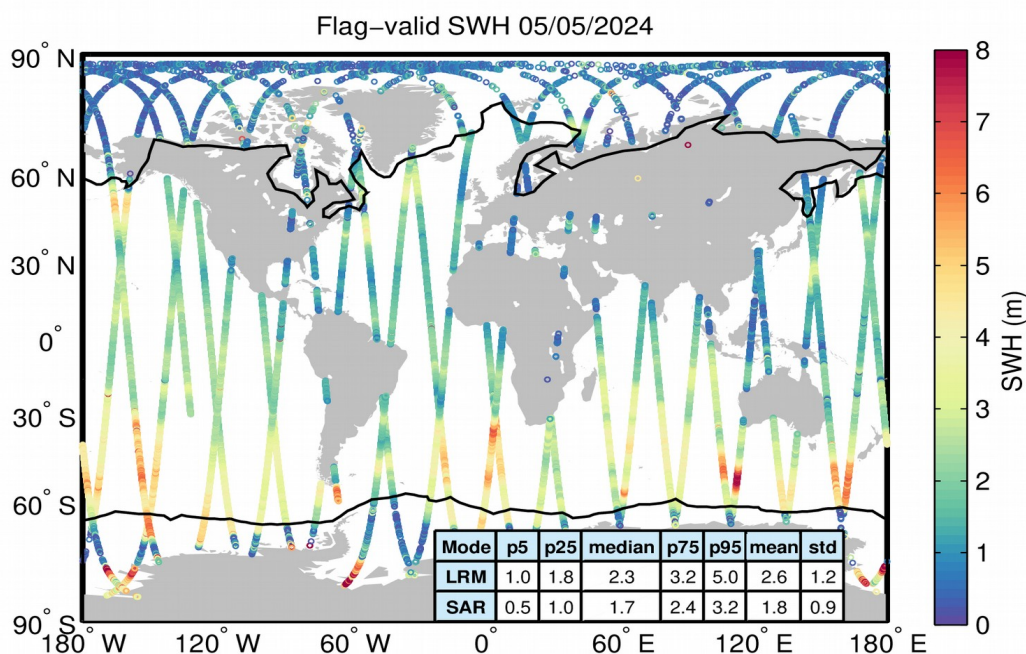
Figure 15. Geographical distribution of flag-valid SWH data over oceans and lakes for 05/05/2024. The statistical values shown in the table refer to the SWH in m and are calculated separately for LRM and SAR regions. Measurements taken over polar polygons have been excluded from the computation of the statistical values. The black lines mark the outer limit of the Arctic and Antarctic polar polygons.
