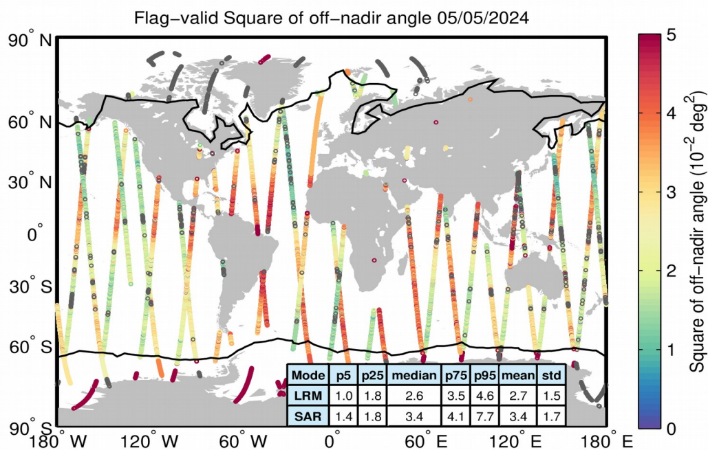
Figure 37. Geographical distribution of flag-valid mispointing data over oceans and lakes for 05/05/2024. The statistical values shown in the table refer to the mispointing in 10^{-2} \text{ deg}^2 and are calculated separately for LRM and SAR regions. Measurements taken over polar polygons have been excluded from the computation of the statistical values. The black lines mark the outer limit of the Arctic and Antarctic polar polygons. Gray circles denote negative values.
