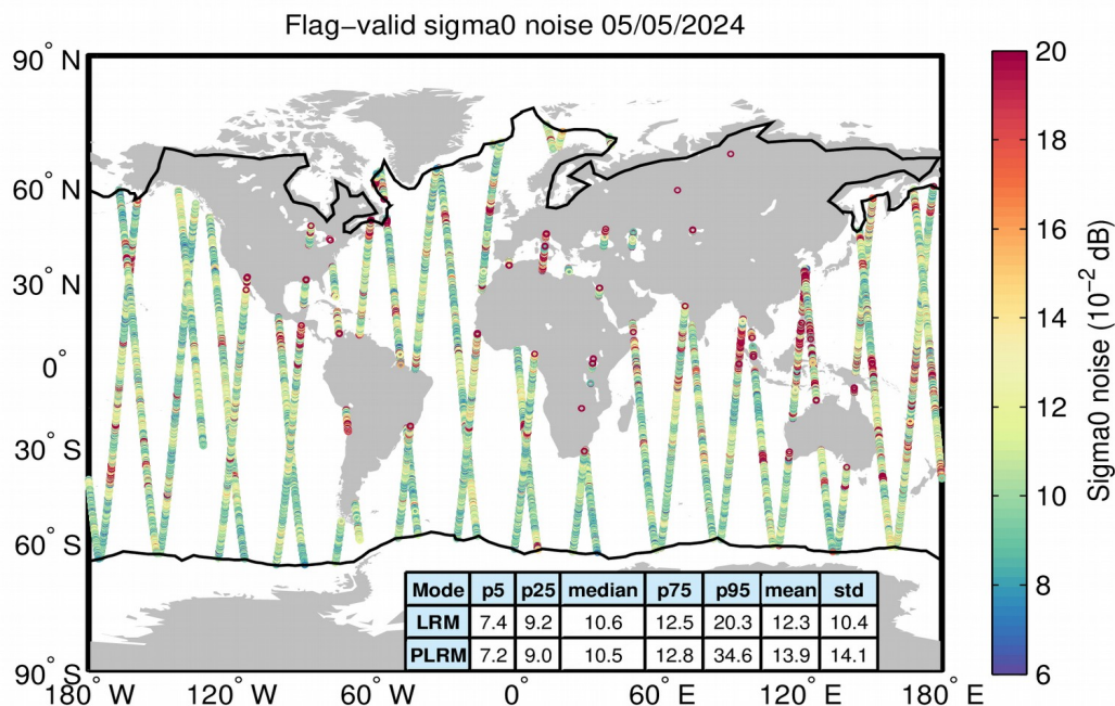
Figure 26. Geographical distribution of flag-valid 20-Hz sigma0 measurement noise over oceans and lakes for LRM/SAR (top) and LRM/PLRM (bottom) and for 05/05/2024. The statistical values shown in the table refer to the sigma0 noise and are calculated separately for LRM and SAR/PLRM regions. Measurements taken over polar polygons have been excluded from the computation of the statistical values. The black lines mark the outer limit of the Arctic and Antarctic polar polygons.
