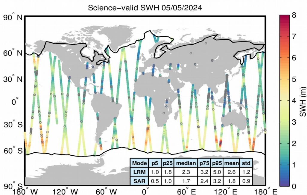
Figure 19. Geographical distribution of science-valid SWH data over oceans and lakes for 05/05/2024. The statistical values shown in the table refer to the SWH in m and are calculated separately for LRM and SAR regions. The black lines mark the outer limit of the Arctic and Antarctic polar polygons. Gray circles denote records that have been rejected based on the editing criteria described in Table 3.
