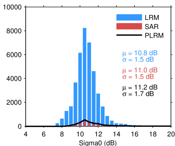
Figure 28. Histogram of science-valid sigma0 over oceans and lakes for LRM (blue), SAR (red), and PLRM (black) for 05/05/2024. The mean ( \mu ) and standard deviation ( \sigma ) are also shown. Note that values outside [4 20] dB are excluded from the histogram for the sake of readability but not from the computation of \mu and \sigma .
