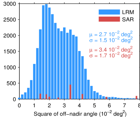
Figure 39. Histogram of flag-valid mispointing over oceans and lakes for LRM (blue) and SAR (red) for 05/05/2024. Only positive values have been considered. The mean ( \mu ) and standard deviation ( \sigma ) are also shown. Note that values larger than 8 \cdot 10^{-2} \text{ deg}^2 are excluded from the histogram for the sake of readability but not from the computation of \mu and \sigma .
