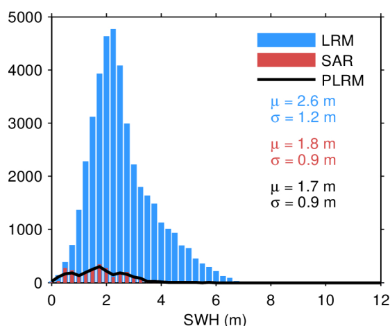
Figure 20. Histogram of science-valid SWH over oceans and lakes for LRM (blue), SAR (red), and PLRM (black) for 05/05/2024. The mean ( \mu ) and standard deviation ( \sigma ) are also
