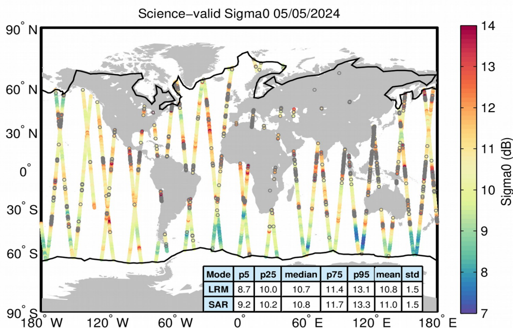
Figure 27. Geographical distribution of science-valid sigma0 data over oceans and lakes for 05/05/2024. The statistical values shown in the table refer to the sigma0 in dB and are calculated separately for LRM and SAR regions. The black lines mark the outer limit of the Arctic and Antarctic polar polygons. Gray circles denote records that have been rejected based on the editing criteria described in Table 4.
