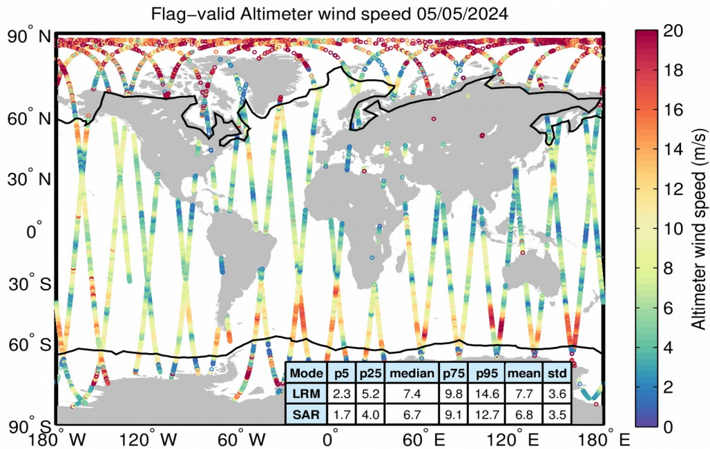
Figure 31. Geographical distribution of flag-valid wind data over oceans and lakes for 05/05/2024. The statistical values shown in the table refer to the wind in m/s and are calculated separately for LRM and SAR regions. Measurements taken over polar polygons have been excluded from the computation of the statistical values. The black lines mark the outer limit of the Arctic and Antarctic polar polygons.
