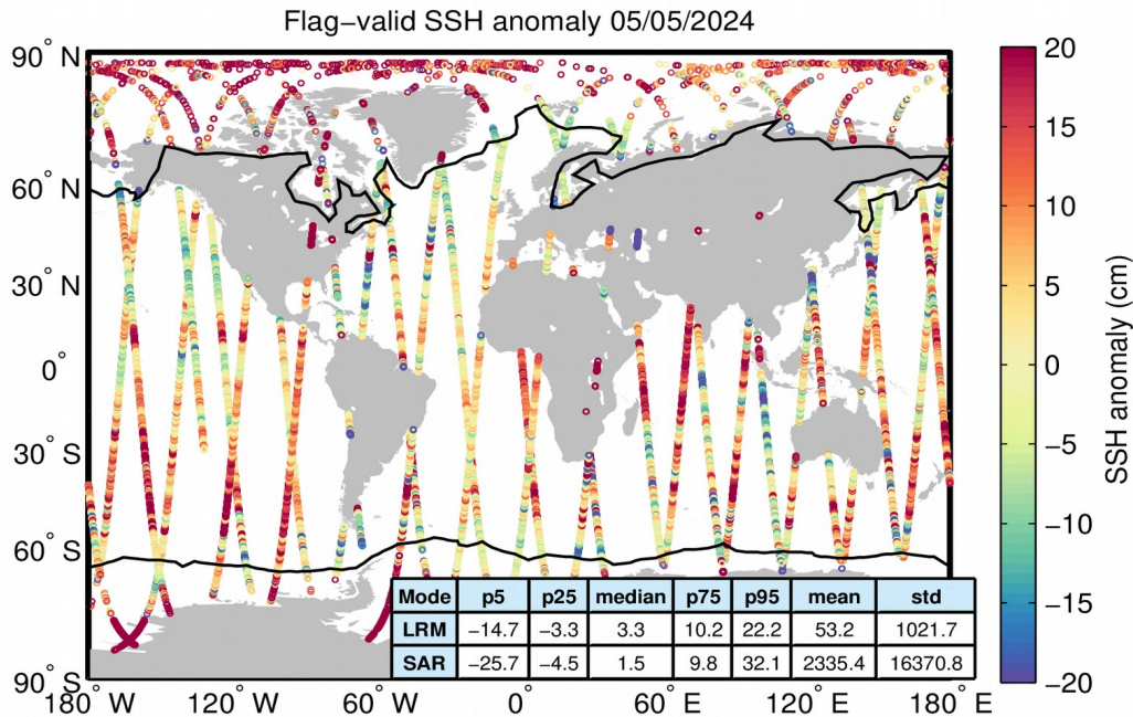
Figure 5. Geographical distribution of flag-valid 1-Hz SSH anomaly data over oceans and lakes for 05/05/2024. The statistical values shown in the table refer to the SSH anomaly in cm and are calculated separately for LRM and SAR regions. Measurements taken over polar polygons have been excluded from the computation of the statistical values. The black lines mark the outer limit of the Arctic and Antarctic polar polygons.
