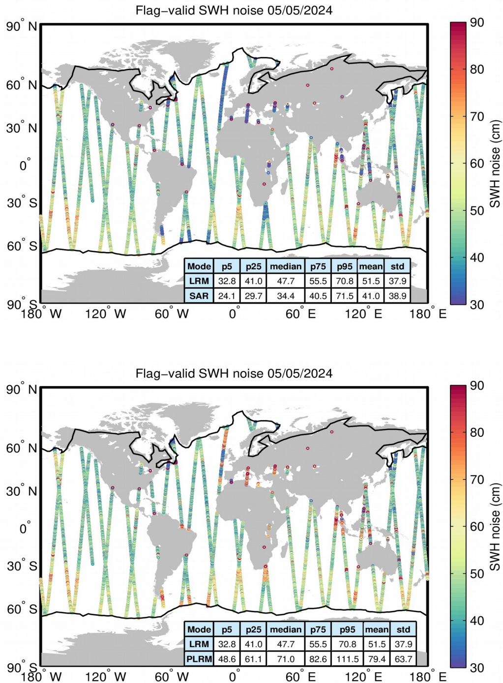
Figure 18. Geographical distribution of flag-valid 20-Hz SWH measurement noise over oceans and lakes for LRM/SAR (top) and LRM/PLRM (bottom) and for 05/05/2024. The statistical values shown in the table refer to the SWH noise and are calculated separately for LRM and SAR/PLRM regions. Measurements taken over polar polygons have been
