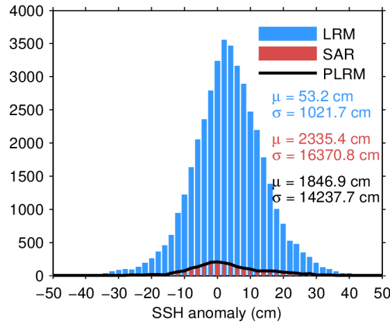
Figure 7. Histogram of flag-valid SSH anomaly over oceans and lakes for LRM (blue), SAR (red), and PLRM (black) for 05/05/2024. The mean ( \mu ) and standard deviation ( \sigma ) are also shown. Note that values outside [-50 50] cm are excluded from the histogram for the sake of readability but not from the computation of \mu and \sigma .
