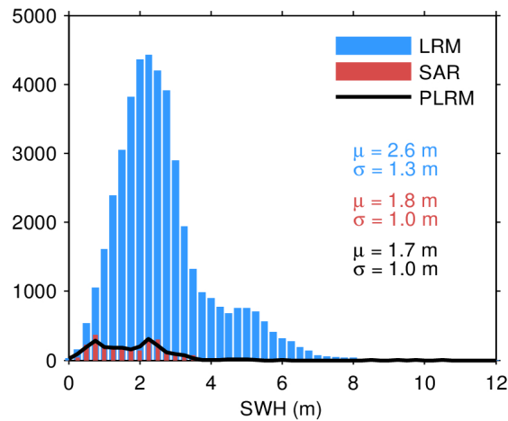
Figure 17. Histogram of flag-valid SWH over oceans and lakes for LRM (blue), SAR (red), and PLRM (black) for 04/05/2024. The mean ( \mu ) and standard deviation ( \sigma ) are also shown. Note that values larger than 12 m are excluded from the histogram for the sake of readability but not from the computation of \mu and \sigma .
