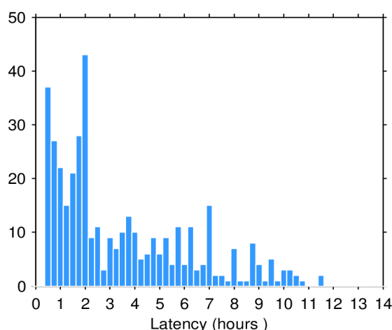
Figure 2. Histogram of the data latency for 04/05/2024. The y-axis denotes the number of files that are made available with a delay of x-hours with respect to the mean time of the records stored in the file.
