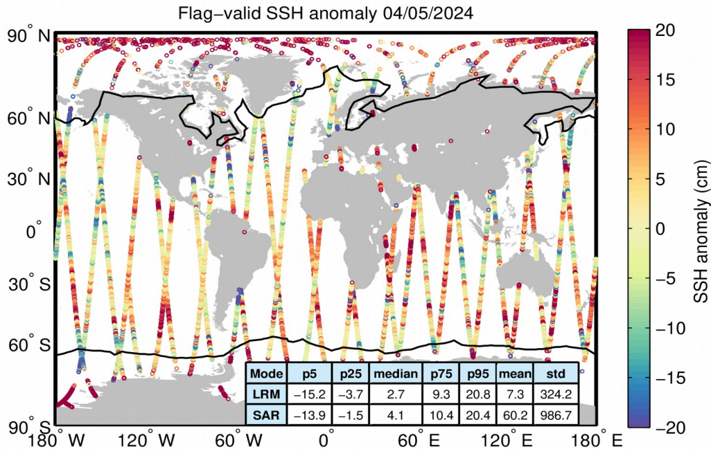
Figure 5. Geographical distribution of flag-valid 1-Hz SSH anomaly data over oceans and lakes for 04/05/2024. The statistical values shown in the table refer to the SSH anomaly in cm and are calculated separately for LRM and SAR regions. Measurements taken over polar polygons have been excluded from the computation of the statistical values. The black lines mark the outer limit of the Arctic and Antarctic polar polygons.
