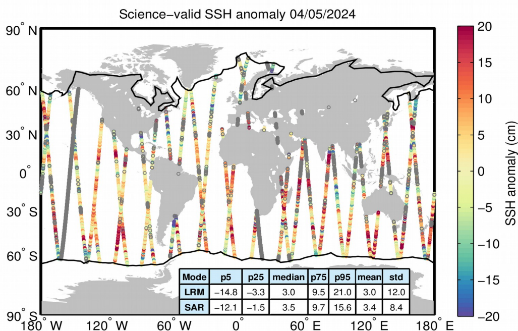
Figure 10. Geographical distribution of science-valid SSH anomaly data over oceans and lakes for 04/05/2024. The statistical values shown in the table refer to the SSH anomaly in cm and are calculated separately for LRM and SAR regions. The black lines mark the
