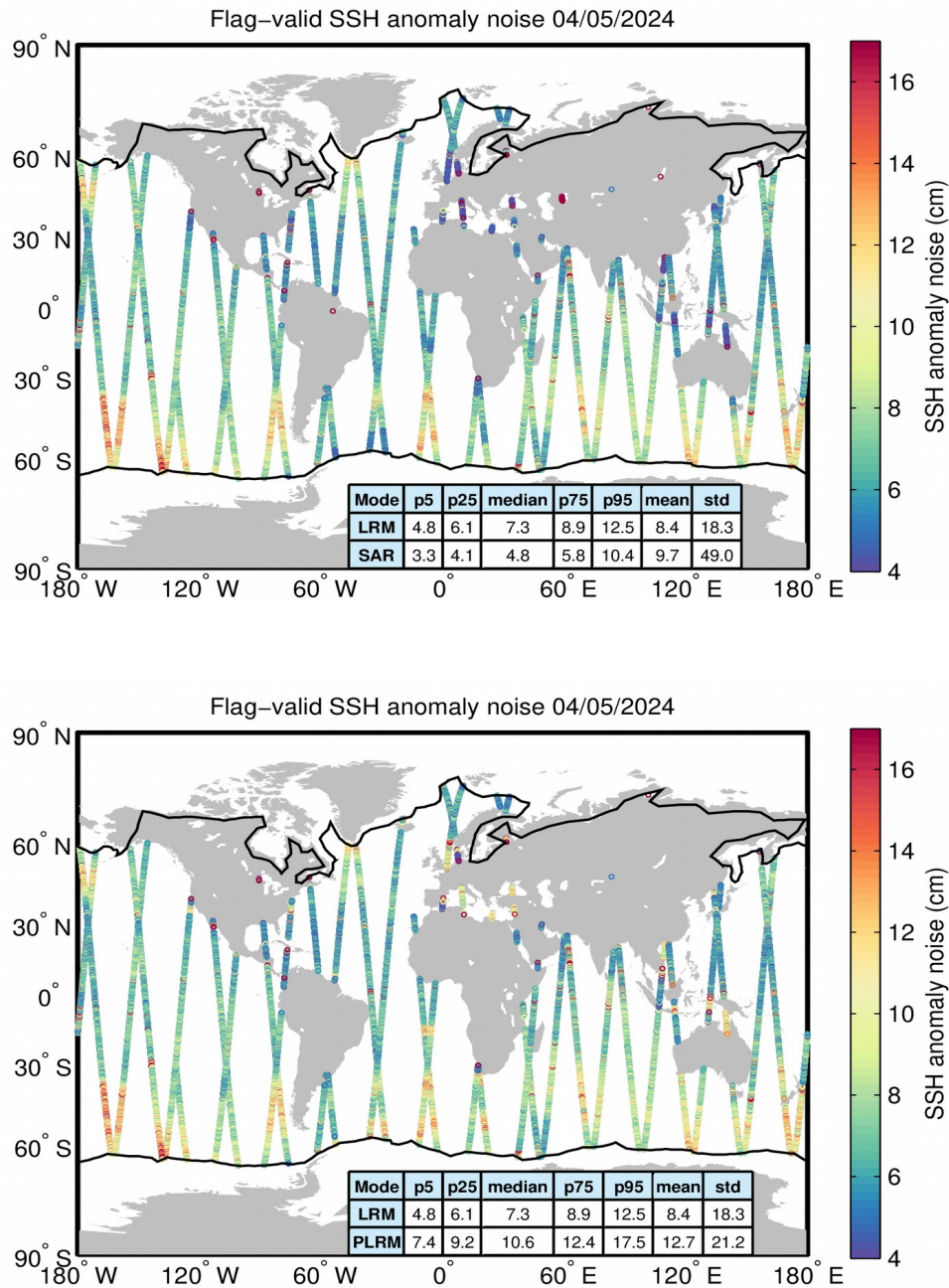
Figure 8. Geographical distribution of flag-valid 20-Hz SSH anomaly measurement noise over oceans and lakes for LRM/SAR (top) and LRM/PLRM (bottom) and for 04/05/2024. The statistical values shown in the tables refer to the SSH anomaly noise and are calculated separately for LRM and SAR/PLRM regions. Measurements taken over polar polygons have been excluded from the computation of the statistical values. The black lines mark the outer limit of the Arctic and Antarctic polar polygons.
