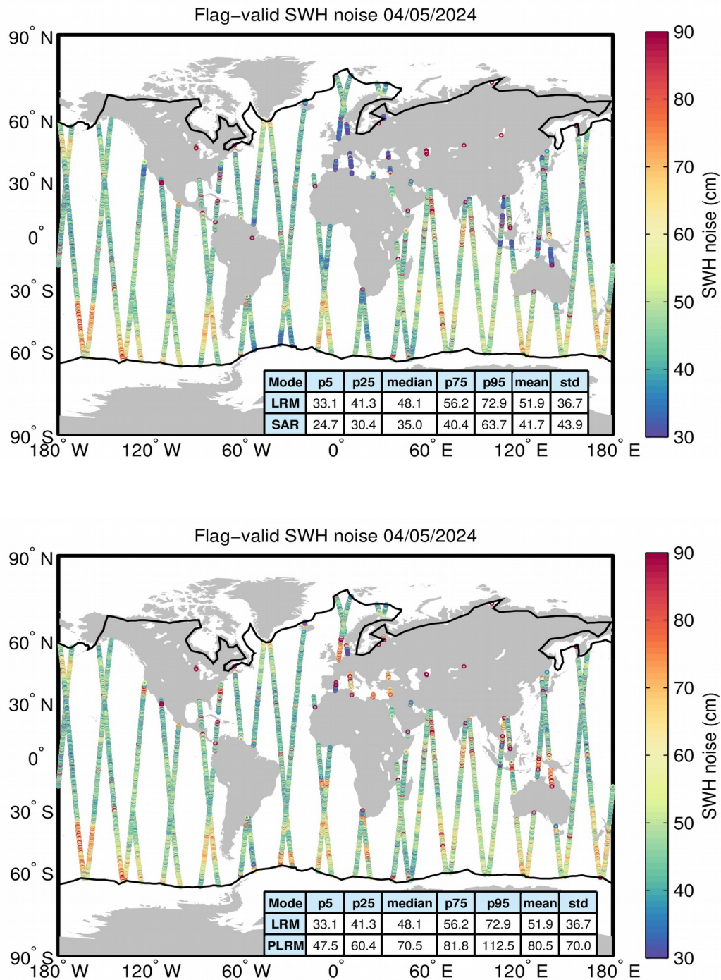
Figure 18. Geographical distribution of flag-valid 20-Hz SWH measurement noise over oceans and lakes for LRM/SAR (top) and LRM/PLRM (bottom) and for 04/05/2024. The statistical values shown in the table refer to the SWH noise and are calculated separately for LRM and SAR/PLRM regions. Measurements taken over polar polygons have been
