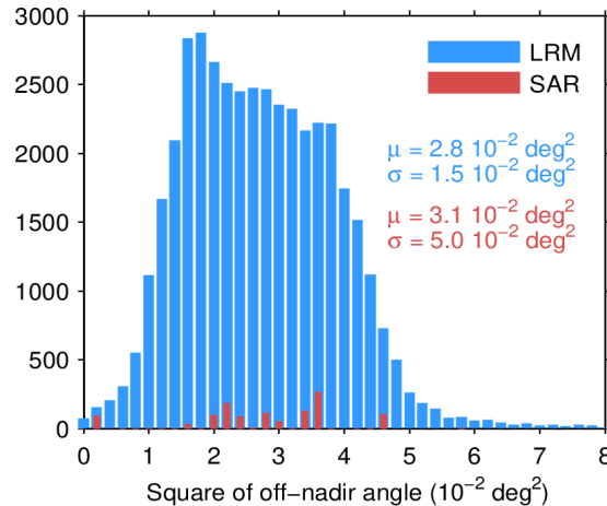
Figure 39. Histogram of flag-valid mispointing over oceans and lakes for LRM (blue) and SAR (red) for 04/05/2024. Only positive values have been considered. The mean ( \mu ) and standard deviation ( \sigma ) are also shown. Note that values larger than 8 \cdot 10^{-2} \text{ deg}^2 are excluded from the histogram for the sake of readability but not from the computation of \mu and \sigma .
