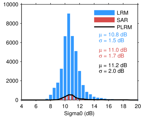
Figure 28. Histogram of science-valid sigma0 over oceans and lakes for LRM (blue), SAR (red), and PLRM (black) for 04/05/2024. The mean ( \mu ) and standard deviation ( \sigma ) are also shown. Note that values outside [4 20] dB are excluded from the histogram for the sake of readability but not from the computation of \mu and \sigma .
