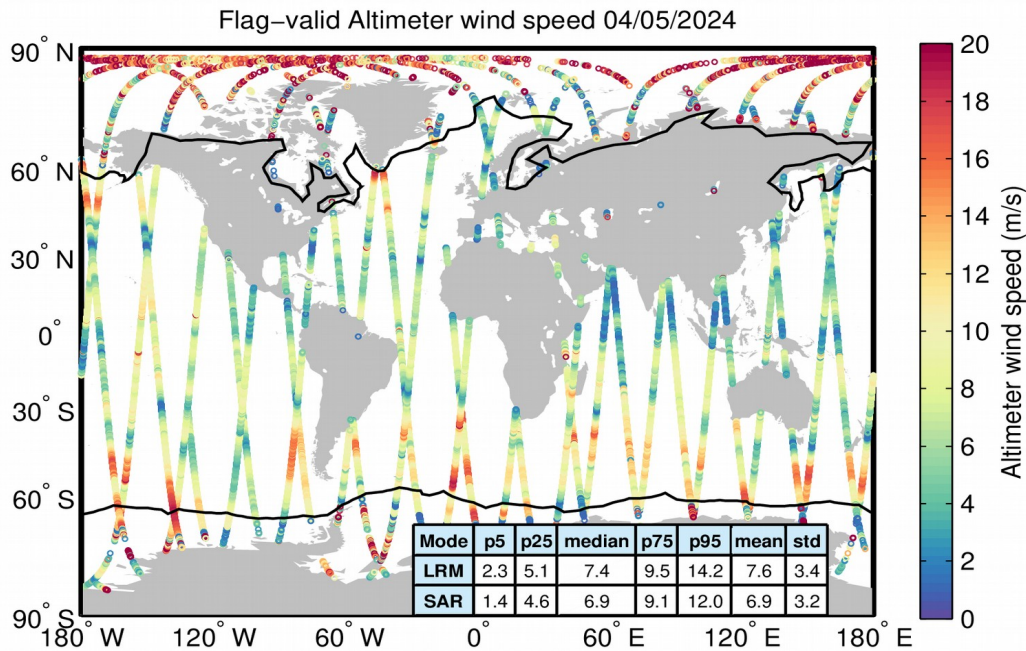
Figure 31. Geographical distribution of flag-valid wind data over oceans and lakes for 04/05/2024. The statistical values shown in the table refer to the wind in m/s and are calculated separately for LRM and SAR regions. Measurements taken over polar polygons have been excluded from the computation of the statistical values. The black lines mark the outer limit of the Arctic and Antarctic polar polygons.
