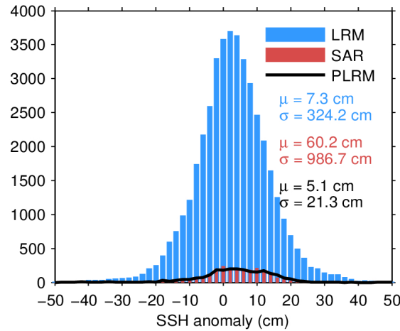
Figure 7. Histogram of flag-valid SSH anomaly over oceans and lakes for LRM (blue), SAR (red), and PLRM (black) for 04/05/2024. The mean ( \mu ) and standard deviation ( \sigma ) are also shown. Note that values outside [-50\ 50] cm are excluded from the histogram for the sake of readability but not from the computation of \mu and \sigma .
