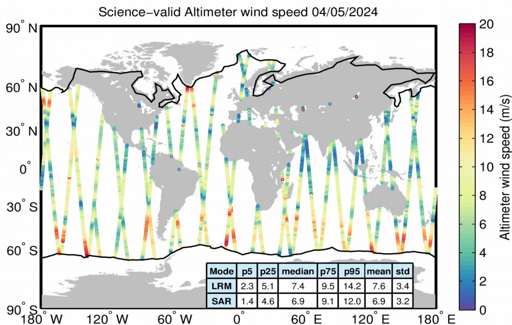
Figure 34. Geographical distribution of science-valid wind data over oceans and lakes for 04/05/2024. The statistical values shown in the table refer to the wind in m/s and are calculated separately for LRM and SAR regions. The black lines mark the outer limit of the Arctic and Antarctic polar polygons. Gray circles denote records that have been rejected based on the editing criteria described in Table 5.
