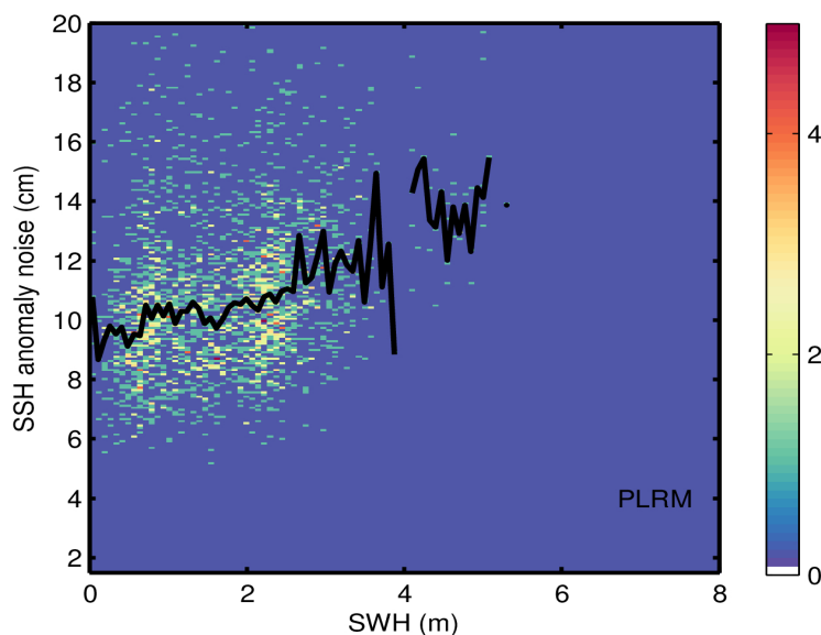
Figure 9. 2D histogram showing flag-valid SSH anomaly noise as a function of SWH for LRM (top), SAR (middle), and PLRM (bottom) for 04/05/2024. The black line denotes the median SSH anomaly noise as a function of SWH.
