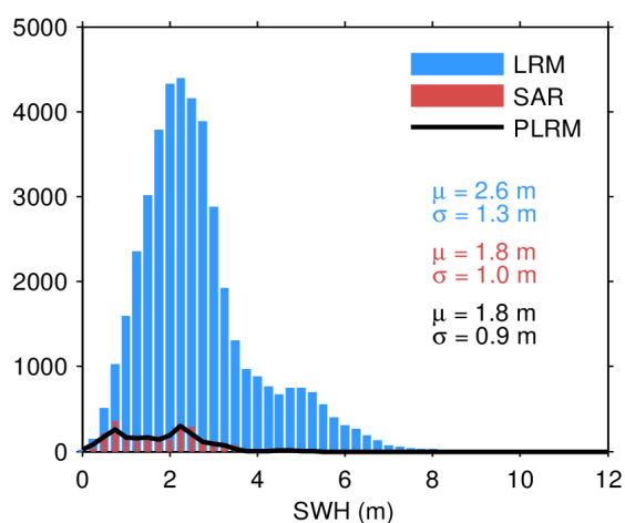
Figure 20. Histogram of science-valid SWH over oceans and lakes for LRM (blue), SAR (red), and PLRM (black) for 04/05/2024. The mean ( \mu ) and standard deviation ( \sigma ) are also
