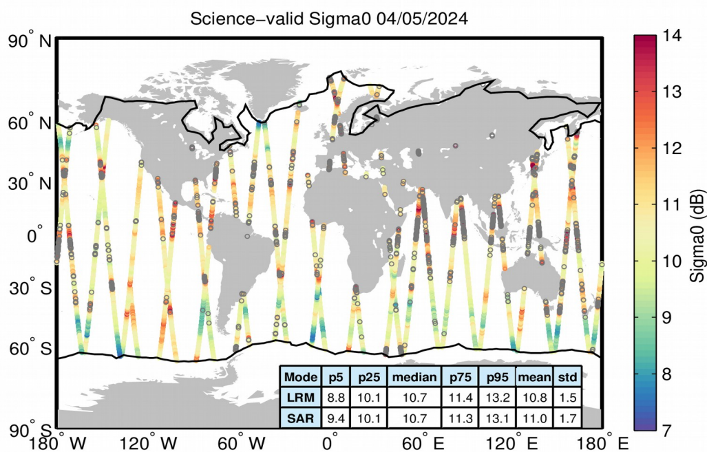
Figure 27. Geographical distribution of science-valid sigma0 data over oceans and lakes for 04/05/2024. The statistical values shown in the table refer to the sigma0 in dB and are calculated separately for LRM and SAR regions. The black lines mark the outer limit of the Arctic and Antarctic polar polygons. Gray circles denote records that have been rejected based on the editing criteria described in Table 4.
