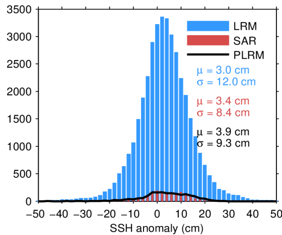
Figure 11. Histogram of science-valid SSH anomaly over oceans and lakes for LRM (blue), SAR (red), and PLRM (black) for 04/05/2024. The mean ( \mu ) and standard deviation ( \sigma ) are also shown. Note that values outside [-50\ 50] cm are excluded from the histogram for the sake of readability but not from the computation of \mu and \sigma .
