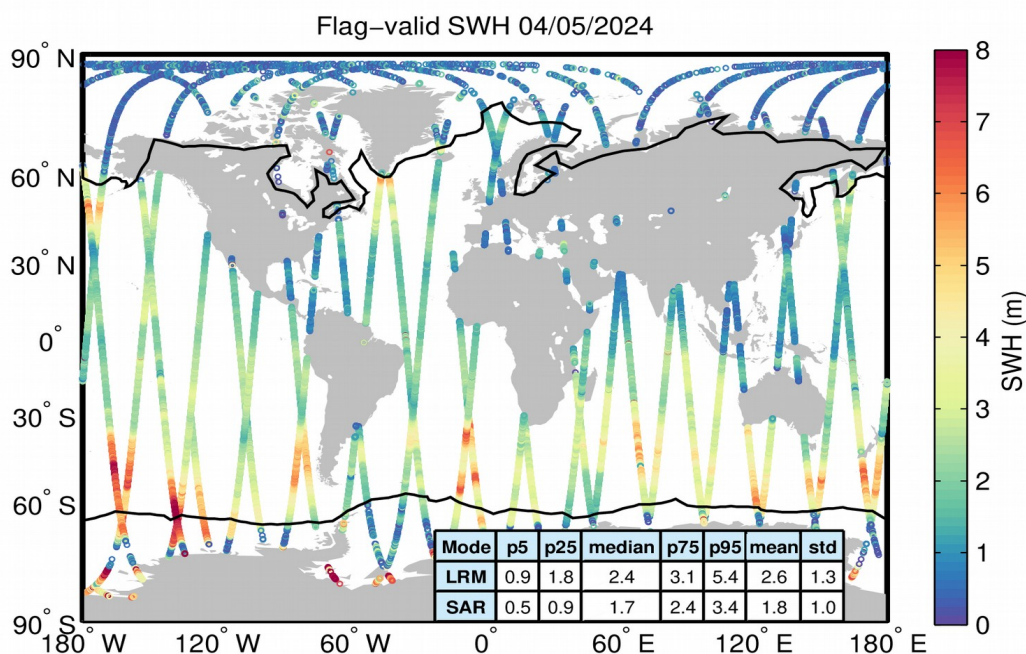
Figure 15. Geographical distribution of flag-valid SWH data over oceans and lakes for 04/05/2024. The statistical values shown in the table refer to the SWH in m and are calculated separately for LRM and SAR regions. Measurements taken over polar polygons have been excluded from the computation of the statistical values. The black lines mark the outer limit of the Arctic and Antarctic polar polygons.
