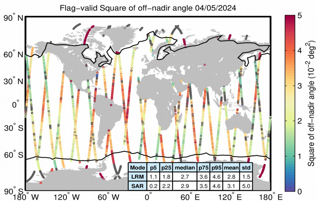
Figure 37. Geographical distribution of flag-valid mispointing data over oceans and lakes for 04/05/2024. The statistical values shown in the table refer to the mispointing in 10^{-2} \text{ deg}^2 and are calculated separately for LRM and SAR regions. Measurements taken over polar polygons have been excluded from the computation of the statistical values. The black lines mark the outer limit of the Arctic and Antarctic polar polygons. Gray circles denote negative values.
