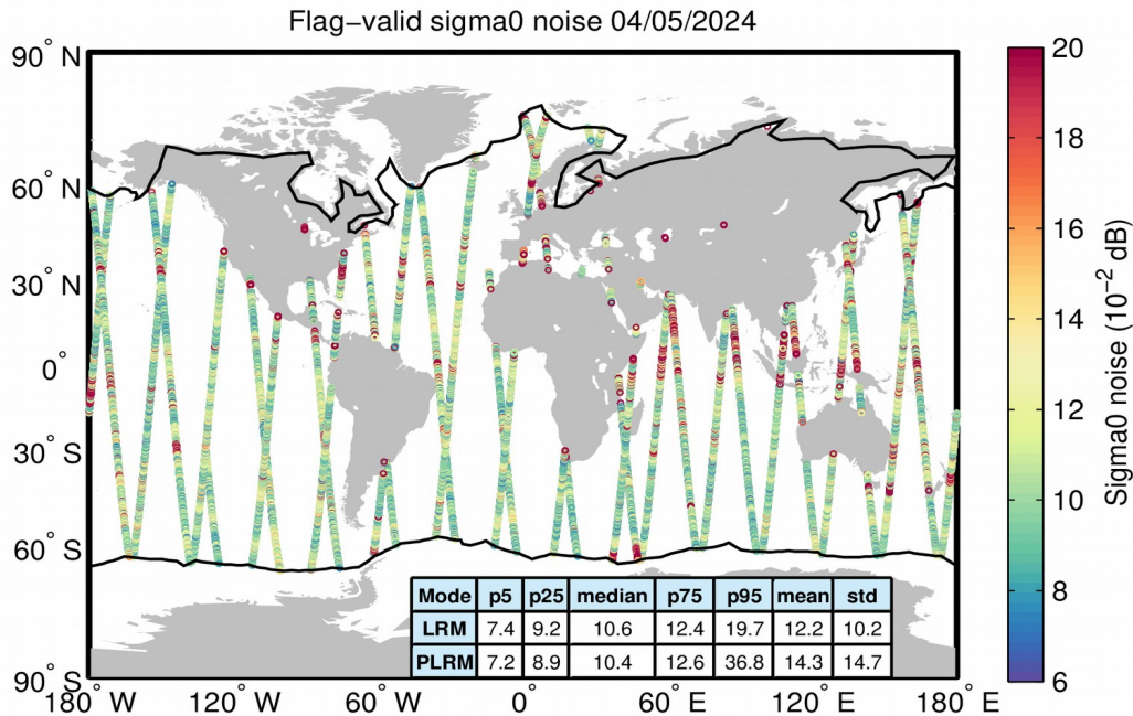
Figure 26. Geographical distribution of flag-valid 20-Hz sigma0 measurement noise over oceans and lakes for LRM/SAR (top) and LRM/PLRM (bottom) and for 04/05/2024. The statistical values shown in the table refer to the sigma0 noise and are calculated separately for LRM and SAR/PLRM regions. Measurements taken over polar polygons have been excluded from the computation of the statistical values. The black lines mark the outer limit of the Arctic and Antarctic polar polygons.
