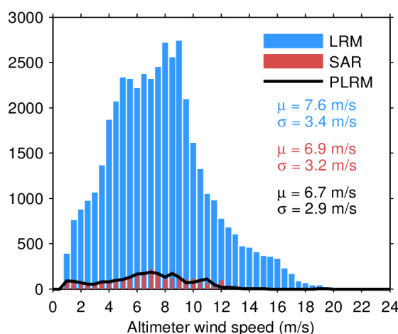
Figure 33. Histogram of flag-valid wind over oceans and lakes for LRM (blue), SAR (red), and PLRM (black) for 04/05/2024. The mean ( \mu ) and standard deviation ( \sigma ) are also shown. Note that values larger than 24 m/s are excluded from the histogram for the sake of readability but not from the computation of \mu and \sigma .
