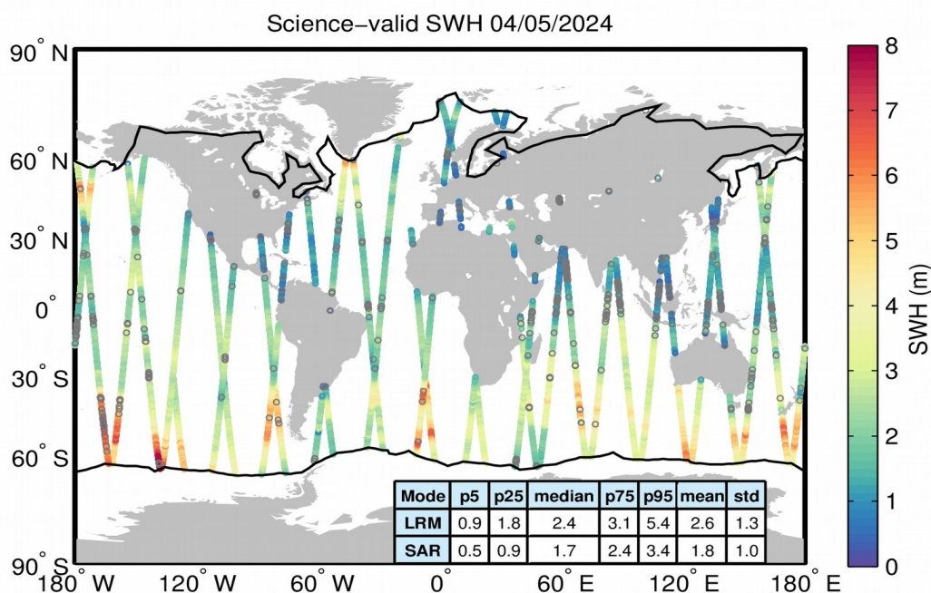
Figure 19. Geographical distribution of science-valid SWH data over oceans and lakes for 04/05/2024. The statistical values shown in the table refer to the SWH in m and are calculated separately for LRM and SAR regions. The black lines mark the outer limit of the Arctic and Antarctic polar polygons. Gray circles denote records that have been rejected based on the editing criteria described in Table 3.
