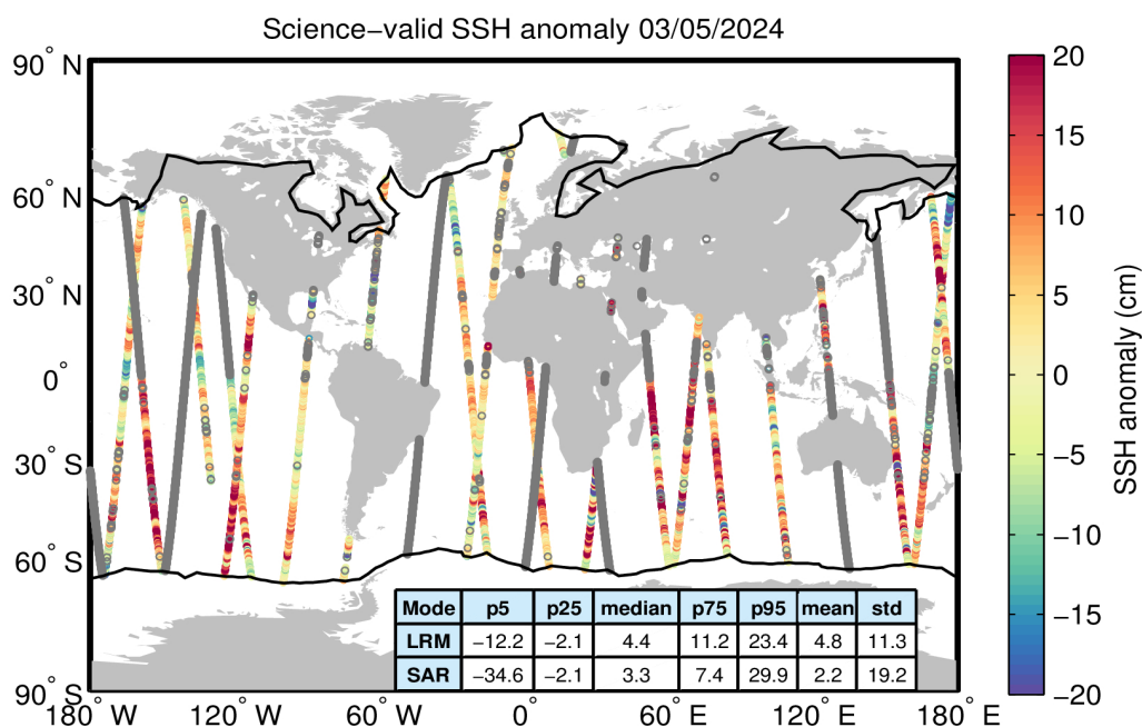
Figure 10. Geographical distribution of science-valid SSH anomaly data over oceans and lakes for 03/05/2024. The statistical values shown in the table refer to the SSH anomaly in cm and are calculated separately for LRM and SAR regions. The black lines mark the
