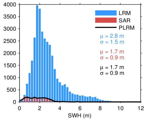
Figure 17. Histogram of flag-valid SWH over oceans and lakes for LRM (blue), SAR (red), and PLRM (black) for 03/05/2024. The mean ( \mu ) and standard deviation ( \sigma ) are also shown. Note that values larger than 12 m are excluded from the histogram for the sake of readability but not from the computation of \mu and \sigma .
