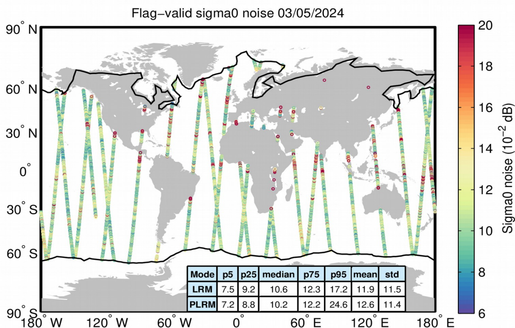
Figure 26. Geographical distribution of flag-valid 20-Hz sigma0 measurement noise over oceans and lakes for LRM/SAR (top) and LRM/PLRM (bottom) and for 03/05/2024. The statistical values shown in the table refer to the sigma0 noise and are calculated separately for LRM and SAR/PLRM regions. Measurements taken over polar polygons have been excluded from the computation of the statistical values. The black lines mark the outer limit of the Arctic and Antarctic polar polygons.
