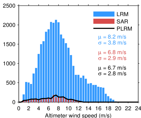
Figure 33. Histogram of flag-valid wind over oceans and lakes for LRM (blue), SAR (red), and PLRM (black) for 03/05/2024. The mean ( \mu ) and standard deviation ( \sigma ) are also shown. Note that values larger than 24 m/s are excluded from the histogram for the sake of readability but not from the computation of \mu and \sigma .
