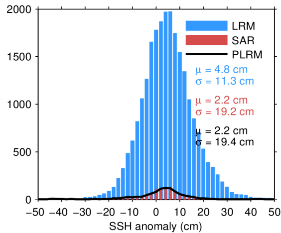
Figure 11. Histogram of science-valid SSH anomaly over oceans and lakes for LRM (blue), SAR (red), and PLRM (black) for 03/05/2024. The mean ( \mu ) and standard deviation ( \sigma ) are also shown. Note that values outside [-50\ 50] cm are excluded from the histogram for the sake of readability but not from the computation of \mu and \sigma .
