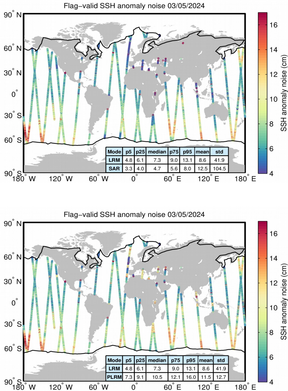
Figure 8. Geographical distribution of flag-valid 20-Hz SSH anomaly measurement noise over oceans and lakes for LRM/SAR (top) and LRM/PLRM (bottom) and for 03/05/2024. The statistical values shown in the tables refer to the SSH anomaly noise and are calculated separately for LRM and SAR/PLRM regions. Measurements taken over polar polygons have been excluded from the computation of the statistical values. The black lines mark the outer limit of the Arctic and Antarctic polar polygons.
