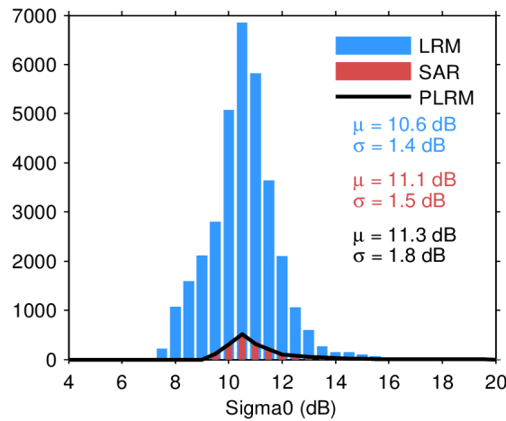
Figure 28. Histogram of science-valid sigma0 over oceans and lakes for LRM (blue), SAR (red), and PLRM (black) for 03/05/2024. The mean ( \mu ) and standard deviation ( \sigma ) are also shown. Note that values outside [4 20] dB are excluded from the histogram for the sake of readability but not from the computation of \mu and \sigma .
