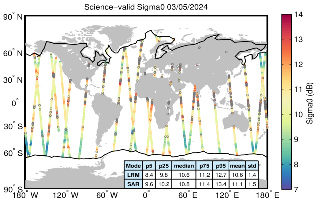
Figure 27. Geographical distribution of science-valid sigma0 data over oceans and lakes for 03/05/2024. The statistical values shown in the table refer to the sigma0 in dB and are calculated separately for LRM and SAR regions. The black lines mark the outer limit of the Arctic and Antarctic polar polygons. Gray circles denote records that have been rejected based on the editing criteria described in Table 4.
