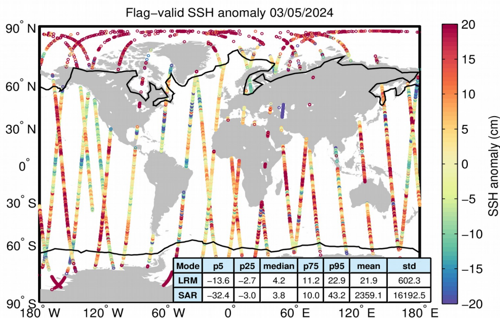
Figure 5. Geographical distribution of flag-valid 1-Hz SSH anomaly data over oceans and lakes for 03/05/2024. The statistical values shown in the table refer to the SSH anomaly in cm and are calculated separately for LRM and SAR regions. Measurements taken over polar polygons have been excluded from the computation of the statistical values. The black lines mark the outer limit of the Arctic and Antarctic polar polygons.
