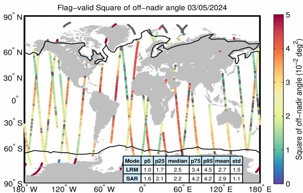
Figure 37. Geographical distribution of flag-valid mispointing data over oceans and lakes for 03/05/2024. The statistical values shown in the table refer to the mispointing in 10^{-2} \text{ deg}^2 and are calculated separately for LRM and SAR regions. Measurements taken over polar polygons have been excluded from the computation of the statistical values. The black lines mark the outer limit of the Arctic and Antarctic polar polygons. Gray circles denote negative values.
