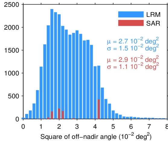
Figure 39. Histogram of flag-valid mispointing over oceans and lakes for LRM (blue) and SAR (red) for 03/05/2024. Only positive values have been considered. The mean ( \mu ) and standard deviation ( \sigma ) are also shown. Note that values larger than 8 \cdot 10^{-2} \text{ deg}^2 are excluded from the histogram for the sake of readability but not from the computation of \mu and \sigma .
