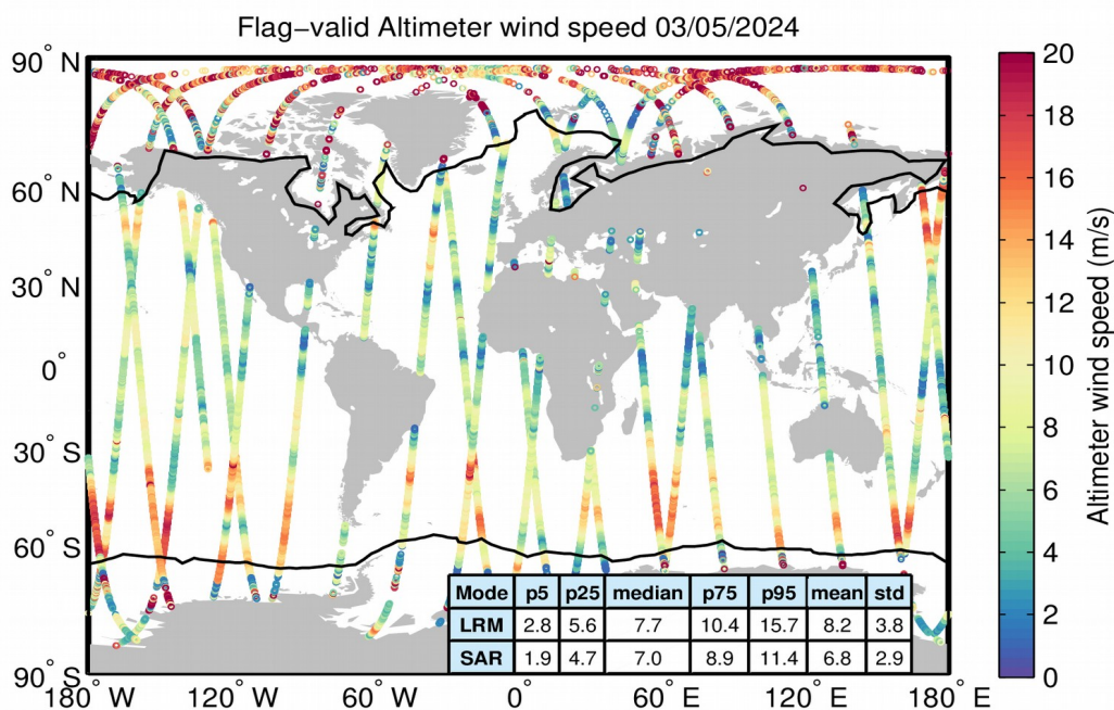
Figure 31. Geographical distribution of flag-valid wind data over oceans and lakes for 03/05/2024. The statistical values shown in the table refer to the wind in m/s and are calculated separately for LRM and SAR regions. Measurements taken over polar polygons have been excluded from the computation of the statistical values. The black lines mark the outer limit of the Arctic and Antarctic polar polygons.
