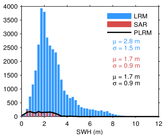
Figure 20. Histogram of science-valid SWH over oceans and lakes for LRM (blue), SAR (red), and PLRM (black) for 03/05/2024. The mean ( \mu ) and standard deviation ( \sigma ) are also
