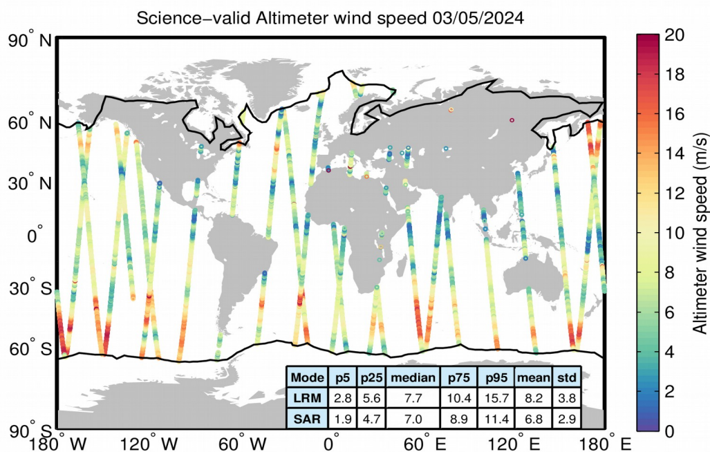
Figure 34. Geographical distribution of science-valid wind data over oceans and lakes for 03/05/2024. The statistical values shown in the table refer to the wind in m/s and are calculated separately for LRM and SAR regions. The black lines mark the outer limit of the Arctic and Antarctic polar polygons. Gray circles denote records that have been rejected based on the editing criteria described in Table 5.
