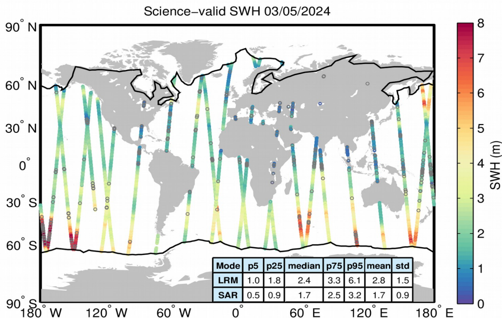
Figure 19. Geographical distribution of science-valid SWH data over oceans and lakes for 03/05/2024. The statistical values shown in the table refer to the SWH in m and are calculated separately for LRM and SAR regions. The black lines mark the outer limit of the Arctic and Antarctic polar polygons. Gray circles denote records that have been rejected based on the editing criteria described in Table 3.
