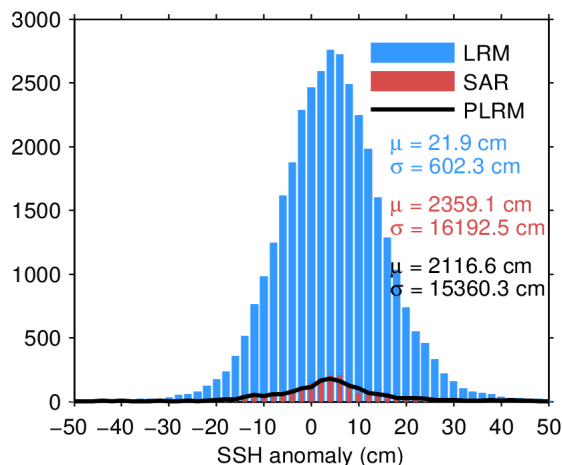
Figure 7. Histogram of flag-valid SSH anomaly over oceans and lakes for LRM (blue), SAR (red), and PLRM (black) for 03/05/2024. The mean ( \mu ) and standard deviation ( \sigma ) are also shown. Note that values outside [-50 50] cm are excluded from the histogram for the sake of readability but not from the computation of \mu and \sigma .
