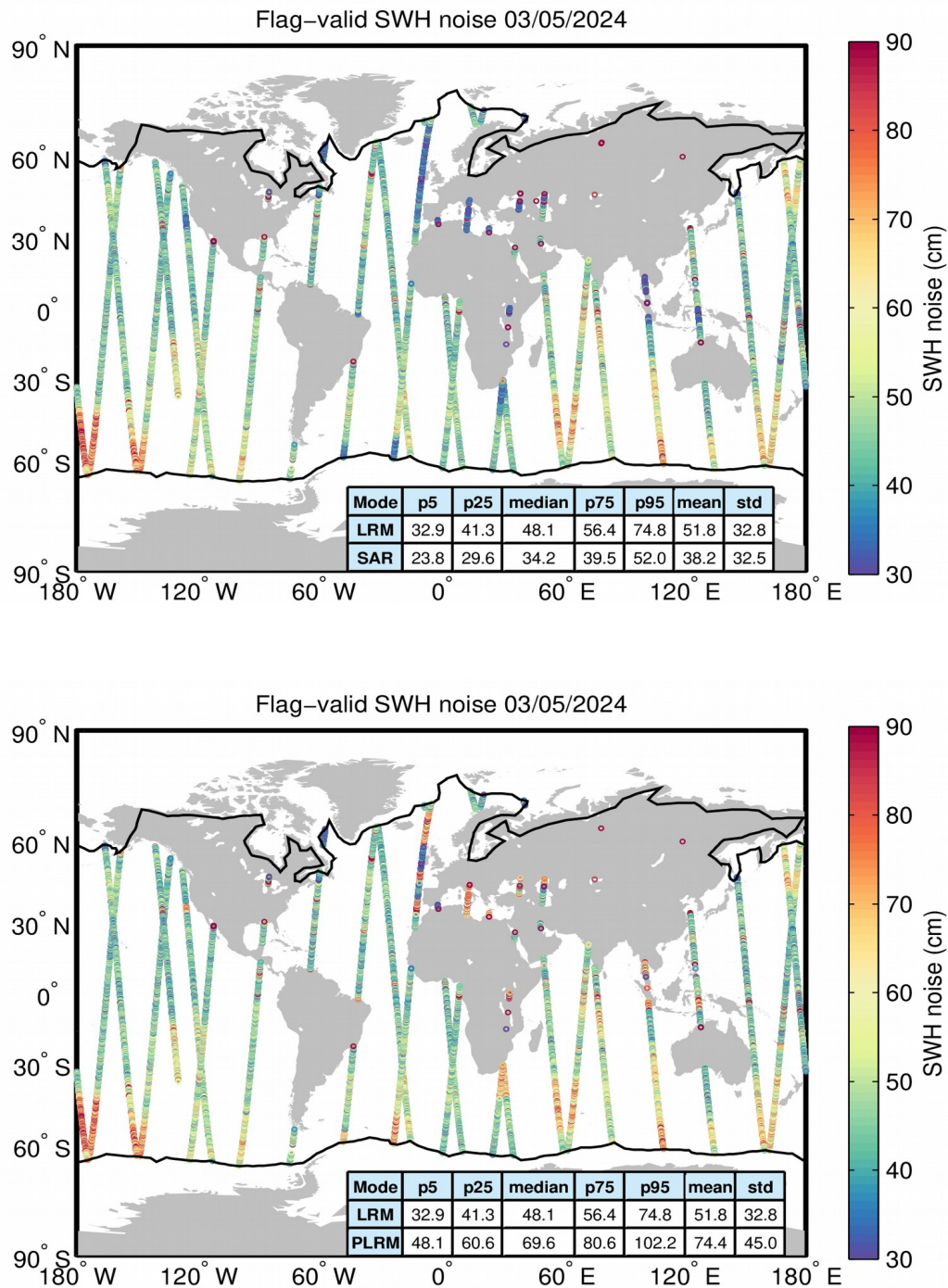
Figure 18. Geographical distribution of flag-valid 20-Hz SWH measurement noise over oceans and lakes for LRM/SAR (top) and LRM/PLRM (bottom) and for 03/05/2024. The statistical values shown in the table refer to the SWH noise and are calculated separately for LRM and SAR/PLRM regions. Measurements taken over polar polygons have been
