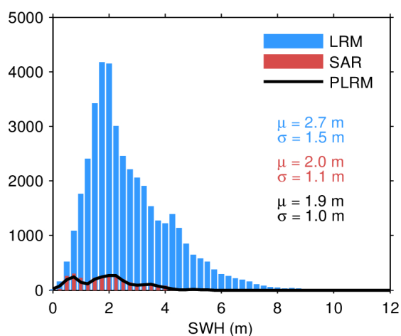
Figure 20. Histogram of science-valid SWH over oceans and lakes for LRM (blue), SAR (red), and PLRM (black) for 02/05/2024. The mean ( \mu ) and standard deviation ( \sigma ) are also
