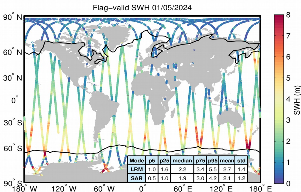
Figure 15. Geographical distribution of flag-valid SWH data over oceans and lakes for 01/05/2024. The statistical values shown in the table refer to the SWH in m and are calculated separately for LRM and SAR regions. Measurements taken over polar polygons have been excluded from the computation of the statistical values. The black lines mark the outer limit of the Arctic and Antarctic polar polygons.
