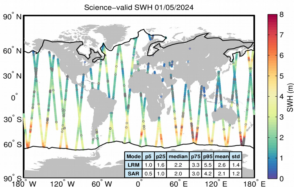
Figure 19. Geographical distribution of science-valid SWH data over oceans and lakes for 01/05/2024. The statistical values shown in the table refer to the SWH in m and are calculated separately for LRM and SAR regions. The black lines mark the outer limit of the Arctic and Antarctic polar polygons. Gray circles denote records that have been rejected based on the editing criteria described in Table 3.
