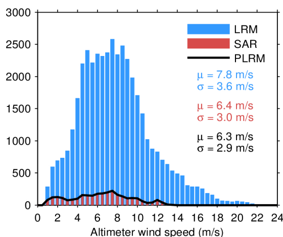
Figure 33. Histogram of flag-valid wind over oceans and lakes for LRM (blue), SAR (red), and PLRM (black) for 01/05/2024. The mean ( \mu ) and standard deviation ( \sigma ) are also shown. Note that values larger than 24 m/s are excluded from the histogram for the sake of readability but not from the computation of \mu and \sigma .
