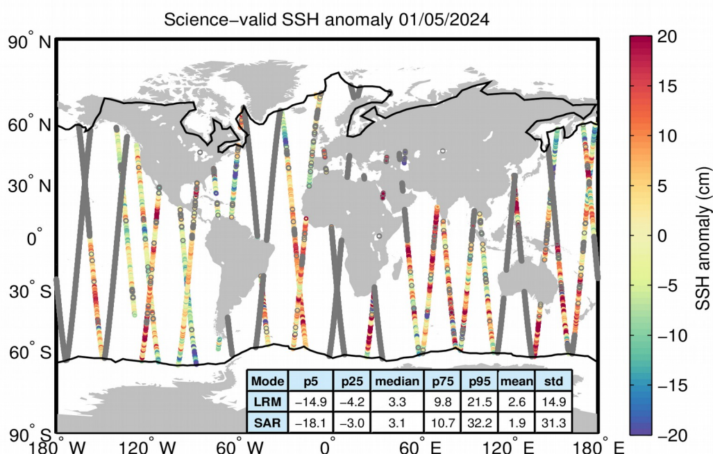
Figure 10. Geographical distribution of science-valid SSH anomaly data over oceans and lakes for 01/05/2024. The statistical values shown in the table refer to the SSH anomaly in cm and are calculated separately for LRM and SAR regions. The black lines mark the
