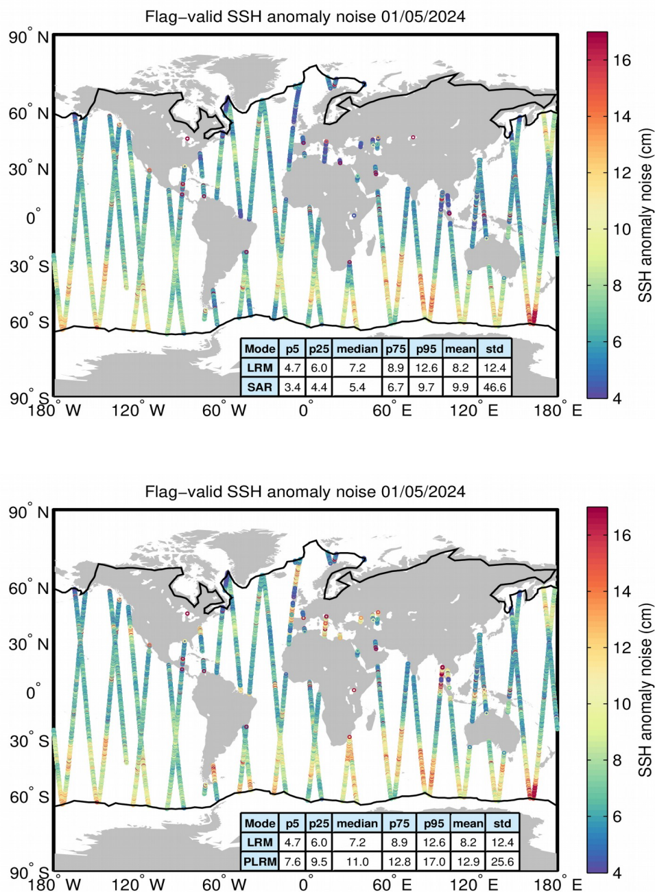
Figure 8. Geographical distribution of flag-valid 20-Hz SSH anomaly measurement noise over oceans and lakes for LRM/SAR (top) and LRM/PLRM (bottom) and for 01/05/2024. The statistical values shown in the tables refer to the SSH anomaly noise and are calculated separately for LRM and SAR/PLRM regions. Measurements taken over polar polygons have been excluded from the computation of the statistical values. The black lines mark the outer limit of the Arctic and Antarctic polar polygons.
