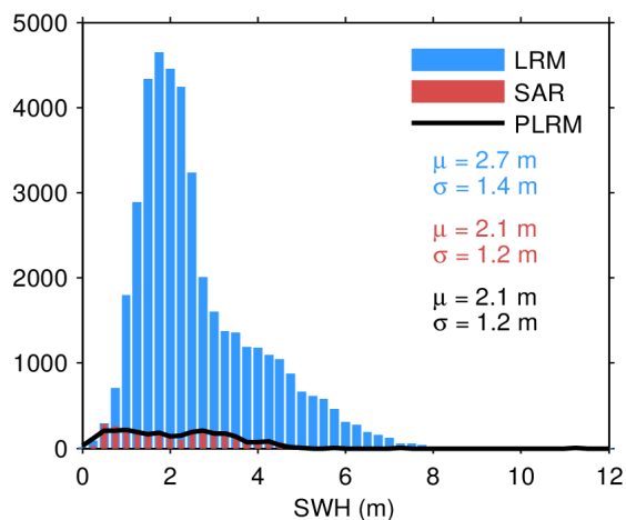
Figure 17. Histogram of flag-valid SWH over oceans and lakes for LRM (blue), SAR (red), and PLRM (black) for 01/05/2024. The mean ( \mu ) and standard deviation ( \sigma ) are also shown. Note that values larger than 12 m are excluded from the histogram for the sake of readability but not from the computation of \mu and \sigma .
