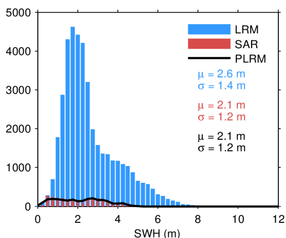
Figure 20. Histogram of science-valid SWH over oceans and lakes for LRM (blue), SAR (red), and PLRM (black) for 01/05/2024. The mean ( \mu ) and standard deviation ( \sigma ) are also
