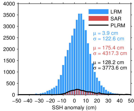
Figure 7. Histogram of flag-valid SSH anomaly over oceans and lakes for LRM (blue), SAR (red), and PLRM (black) for 01/05/2024. The mean ( \mu ) and standard deviation ( \sigma ) are also shown. Note that values outside [-50\ 50] cm are excluded from the histogram for the sake of readability but not from the computation of \mu and \sigma .
