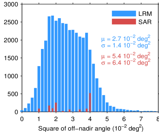
Figure 39. Histogram of flag-valid mispointing over oceans and lakes for LRM (blue) and SAR (red) for 01/05/2024. Only positive values have been considered. The mean ( \mu ) and standard deviation ( \sigma ) are also shown. Note that values larger than 8 10^{-2} \text{ deg}^2 are excluded from the histogram for the sake of readability but not from the computation of \mu and \sigma .
