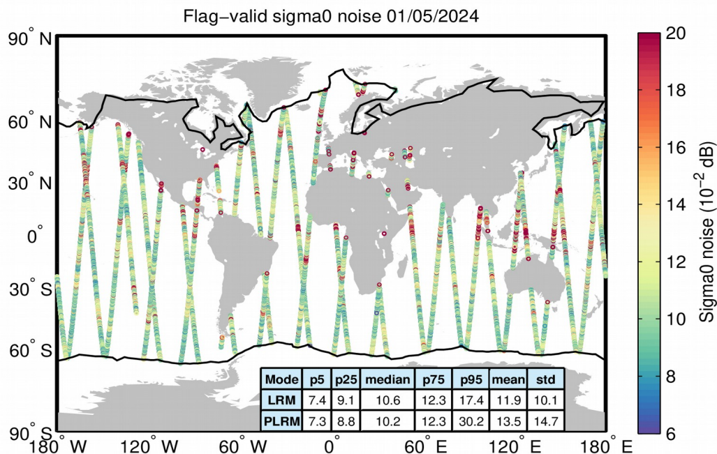
Figure 26. Geographical distribution of flag-valid 20-Hz sigma0 measurement noise over oceans and lakes for LRM/SAR (top) and LRM/PLRM (bottom) and for 01/05/2024. The statistical values shown in the table refer to the sigma0 noise and are calculated separately for LRM and SAR/PLRM regions. Measurements taken over polar polygons have been excluded from the computation of the statistical values. The black lines mark the outer limit of the Arctic and Antarctic polar polygons.
