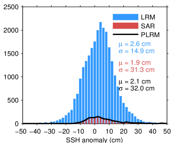
Figure 11. Histogram of science-valid SSH anomaly over oceans and lakes for LRM (blue), SAR (red), and PLRM (black) for 01/05/2024. The mean ( \mu ) and standard deviation ( \sigma ) are also shown. Note that values outside [-50\ 50] cm are excluded from the histogram for the sake of readability but not from the computation of \mu and \sigma .
