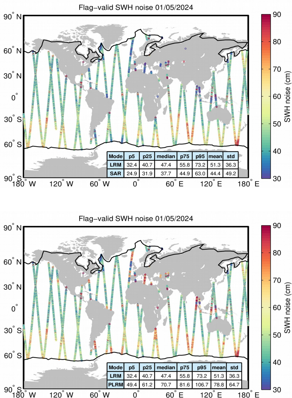
Figure 18. Geographical distribution of flag-valid 20-Hz SWH measurement noise over oceans and lakes for LRM/SAR (top) and LRM/PLRM (bottom) and for 01/05/2024. The statistical values shown in the table refer to the SWH noise and are calculated separately for LRM and SAR/PLRM regions. Measurements taken over polar polygons have been
