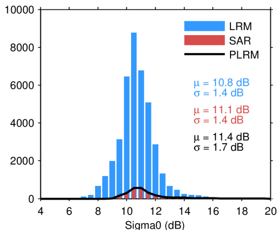
Figure 28. Histogram of science-valid sigma0 over oceans and lakes for LRM (blue), SAR (red), and PLRM (black) for 01/05/2024. The mean ( \mu ) and standard deviation ( \sigma ) are also shown. Note that values outside [4 20] dB are excluded from the histogram for the sake of readability but not from the computation of \mu and \sigma .
