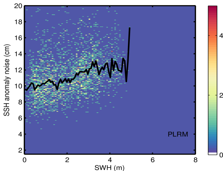
Figure 9. 2D histogram showing flag-valid SSH anomaly noise as a function of SWH for LRM (top), SAR (middle), and PLRM (bottom) for 01/05/2024. The black line denotes the median SSH anomaly noise as a function of SWH.
