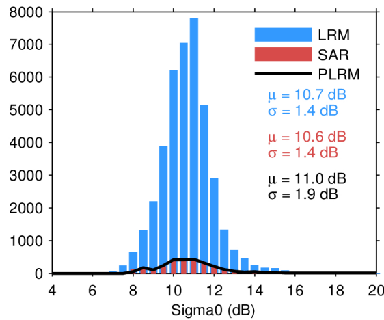
Figure 28. Histogram of science-valid sigma0 over oceans and lakes for LRM (blue), SAR (red), and PLRM (black) for 29/04/2024. The mean ( \mu ) and standard deviation ( \sigma ) are also shown. Note that values outside [4 20] dB are excluded from the histogram for the sake of readability but not from the computation of \mu and \sigma .
