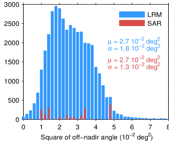
Figure 39. Histogram of flag-valid mispointing over oceans and lakes for LRM (blue) and SAR (red) for 29/04/2024. Only positive values have been considered. The mean ( \mu ) and standard deviation ( \sigma ) are also shown. Note that values larger than 8 \cdot 10^{-2} \text{ deg}^2 are excluded from the histogram for the sake of readability but not from the computation of \mu and \sigma .
