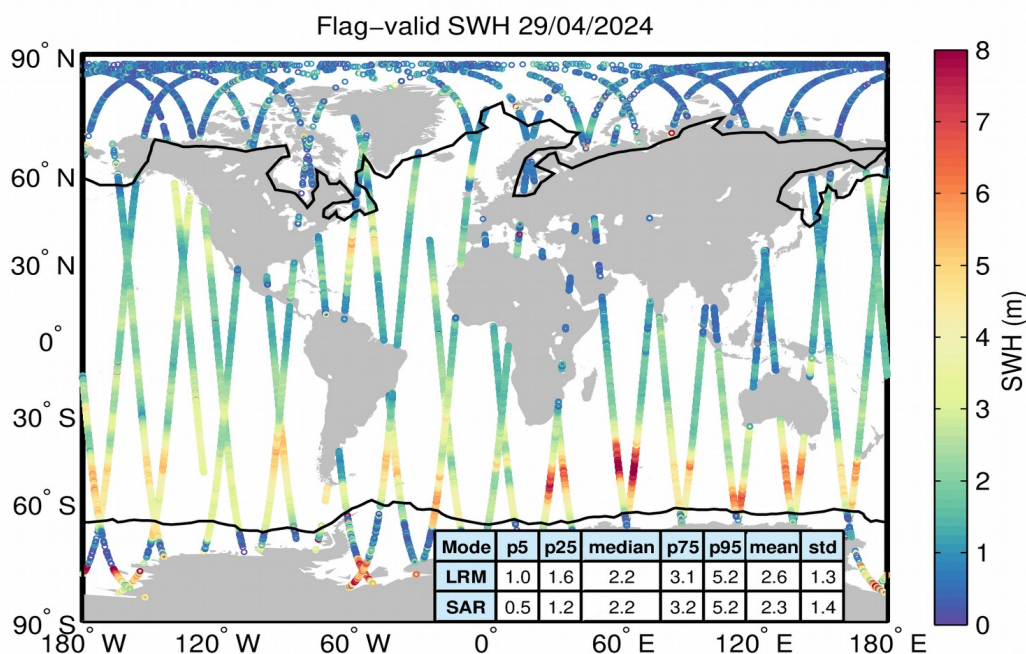
Figure 15. Geographical distribution of flag-valid SWH data over oceans and lakes for 29/04/2024. The statistical values shown in the table refer to the SWH in m and are calculated separately for LRM and SAR regions. Measurements taken over polar polygons have been excluded from the computation of the statistical values. The black lines mark the outer limit of the Arctic and Antarctic polar polygons.
