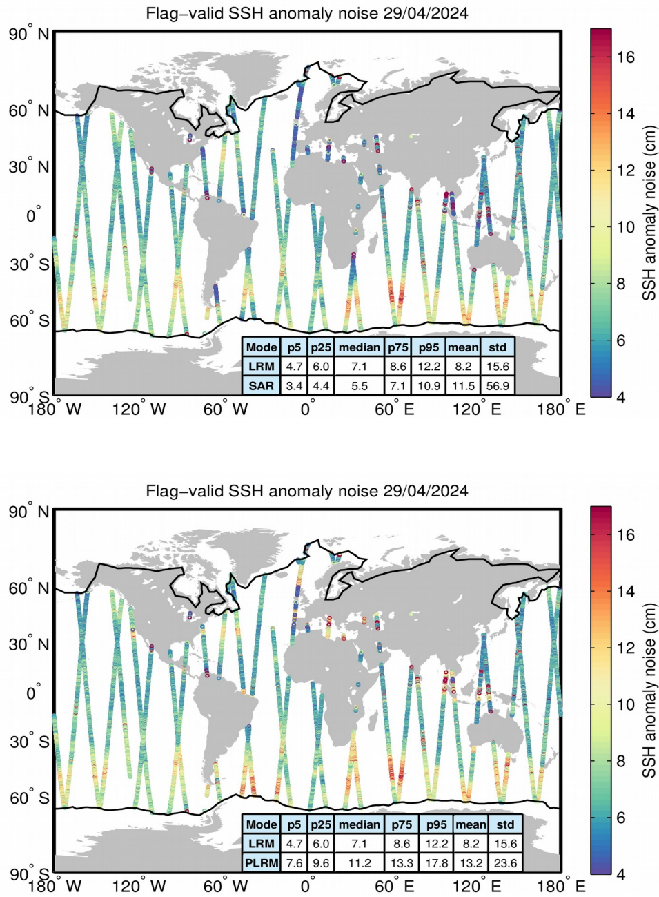
Figure 8. Geographical distribution of flag-valid 20-Hz SSH anomaly measurement noise over oceans and lakes for LRM/SAR (top) and LRM/PLRM (bottom) and for 29/04/2024. The statistical values shown in the tables refer to the SSH anomaly noise and are calculated separately for LRM and SAR/PLRM regions. Measurements taken over polar polygons have been excluded from the computation of the statistical values. The black lines mark the outer limit of the Arctic and Antarctic polar polygons.
