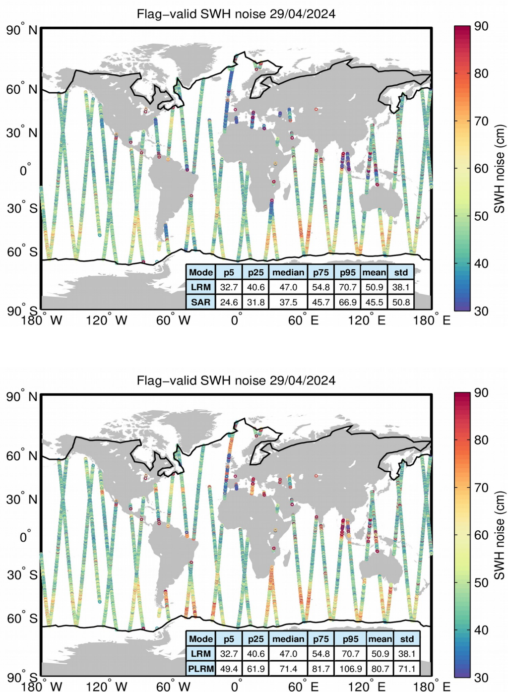
Figure 18. Geographical distribution of flag-valid 20-Hz SWH measurement noise over oceans and lakes for LRM/SAR (top) and LRM/PLRM (bottom) and for 29/04/2024. The statistical values shown in the table refer to the SWH noise and are calculated separately for LRM and SAR/PLRM regions. Measurements taken over polar polygons have been
