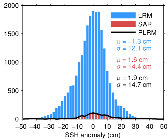
Figure 11. Histogram of science-valid SSH anomaly over oceans and lakes for LRM (blue), SAR (red), and PLRM (black) for 29/04/2024. The mean ( \mu ) and standard deviation ( \sigma ) are also shown. Note that values outside [-50\ 50] cm are excluded from the histogram for the sake of readability but not from the computation of \mu and \sigma .
