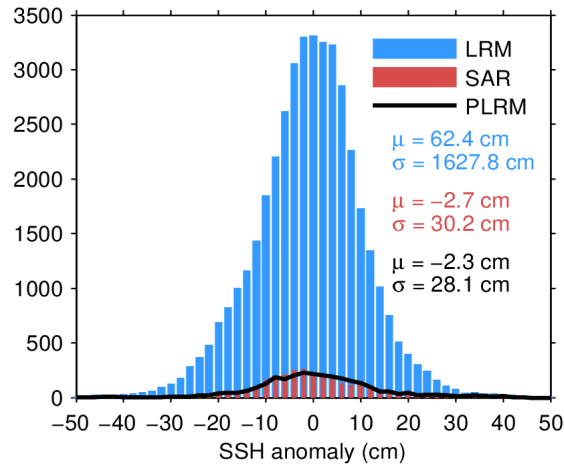
Figure 7. Histogram of flag-valid SSH anomaly over oceans and lakes for LRM (blue), SAR (red), and PLRM (black) for 29/04/2024. The mean ( \mu ) and standard deviation ( \sigma ) are also shown. Note that values outside [-50 50] cm are excluded from the histogram for the sake of readability but not from the computation of \mu and \sigma .
