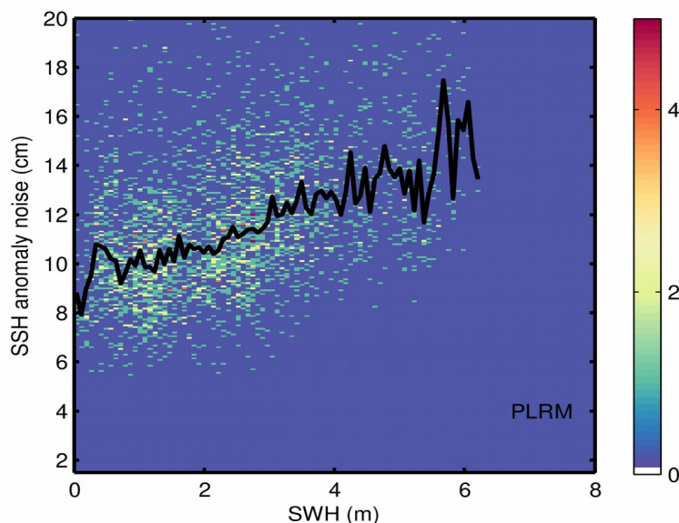
Figure 9. 2D histogram showing flag-valid SSH anomaly noise as a function of SWH for LRM (top), SAR (middle), and PLRM (bottom) for 29/04/2024. The black line denotes the median SSH anomaly noise as a function of SWH.
