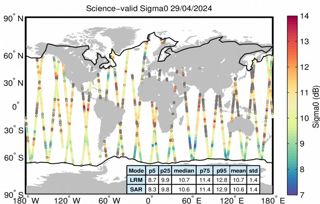
Figure 27. Geographical distribution of science-valid sigma0 data over oceans and lakes for 29/04/2024. The statistical values shown in the table refer to the sigma0 in dB and are calculated separately for LRM and SAR regions. The black lines mark the outer limit of the Arctic and Antarctic polar polygons. Gray circles denote records that have been rejected based on the editing criteria described in Table 4.
