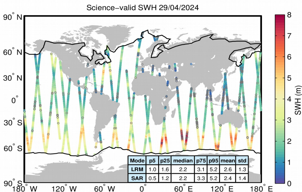
Figure 19. Geographical distribution of science-valid SWH data over oceans and lakes for 29/04/2024. The statistical values shown in the table refer to the SWH in m and are calculated separately for LRM and SAR regions. The black lines mark the outer limit of the Arctic and Antarctic polar polygons. Gray circles denote records that have been rejected based on the editing criteria described in Table 3.
