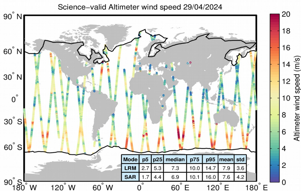
Figure 34. Geographical distribution of science-valid wind data over oceans and lakes for 29/04/2024. The statistical values shown in the table refer to the wind in m/s and are calculated separately for LRM and SAR regions. The black lines mark the outer limit of the Arctic and Antarctic polar polygons. Gray circles denote records that have been rejected based on the editing criteria described in Table 5.
