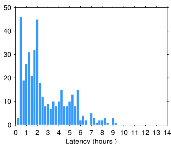
Figure 2. Histogram of the data latency for 29/04/2024. The y-axis denotes the number of files that are made available with a delay of x-hours with respect to the mean time of the records stored in the file.
