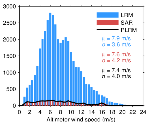
Figure 33. Histogram of flag-valid wind over oceans and lakes for LRM (blue), SAR (red), and PLRM (black) for 29/04/2024. The mean ( \mu ) and standard deviation ( \sigma ) are also shown. Note that values larger than 24 m/s are excluded from the histogram for the sake of readability but not from the computation of \mu and \sigma .
