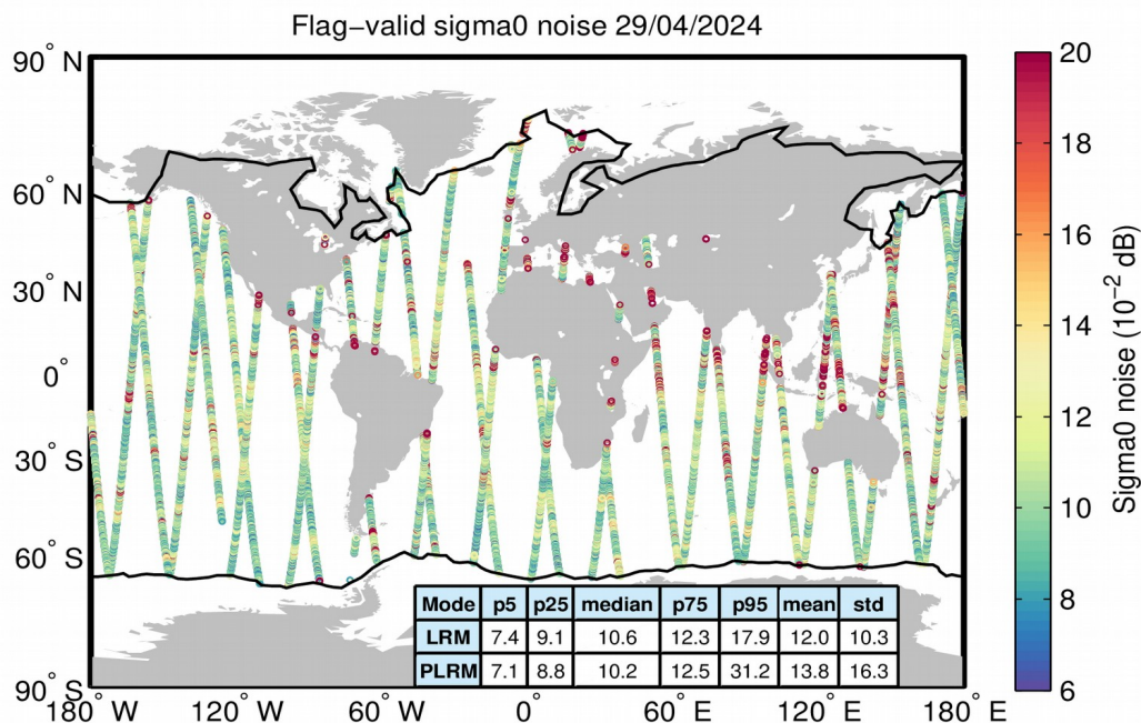
Figure 26. Geographical distribution of flag-valid 20-Hz sigma0 measurement noise over oceans and lakes for LRM/SAR (top) and LRM/PLRM (bottom) and for 29/04/2024. The statistical values shown in the table refer to the sigma0 noise and are calculated separately for LRM and SAR/PLRM regions. Measurements taken over polar polygons have been excluded from the computation of the statistical values. The black lines mark the outer limit of the Arctic and Antarctic polar polygons.
