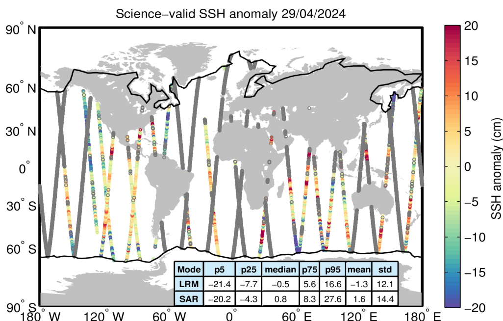
Figure 10. Geographical distribution of science-valid SSH anomaly data over oceans and lakes for 29/04/2024. The statistical values shown in the table refer to the SSH anomaly in cm and are calculated separately for LRM and SAR regions. The black lines mark the
