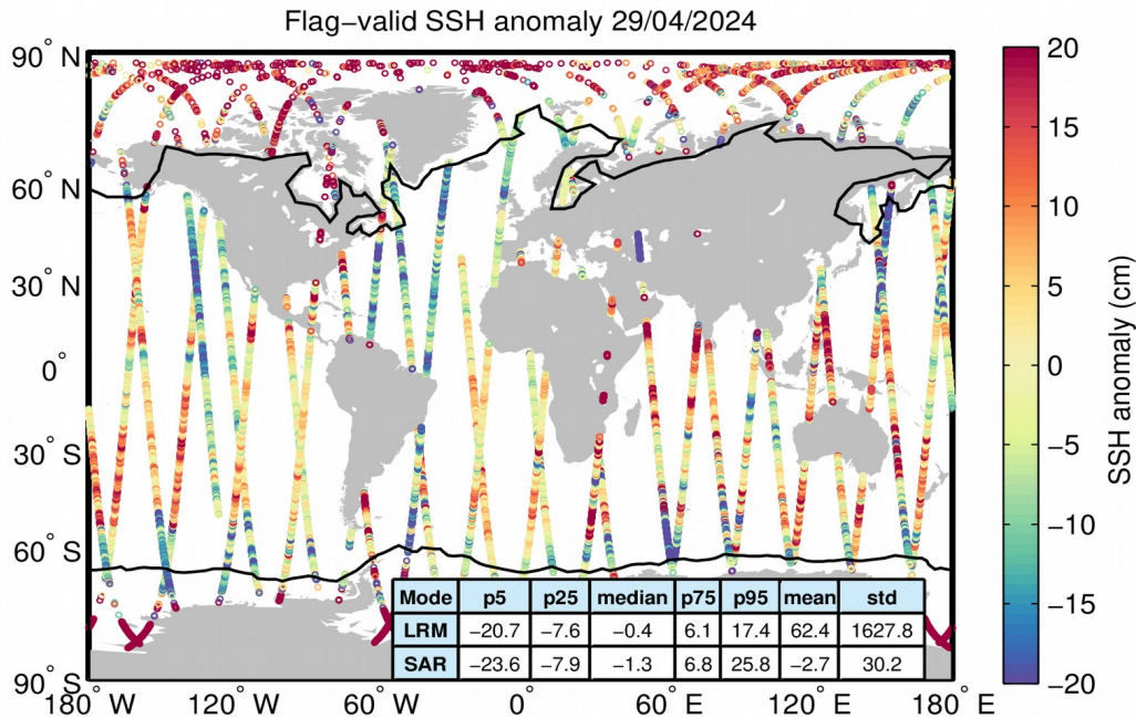
Figure 5. Geographical distribution of flag-valid 1-Hz SSH anomaly data over oceans and lakes for 29/04/2024. The statistical values shown in the table refer to the SSH anomaly in cm and are calculated separately for LRM and SAR regions. Measurements taken over polar polygons have been excluded from the computation of the statistical values. The black lines mark the outer limit of the Arctic and Antarctic polar polygons.
