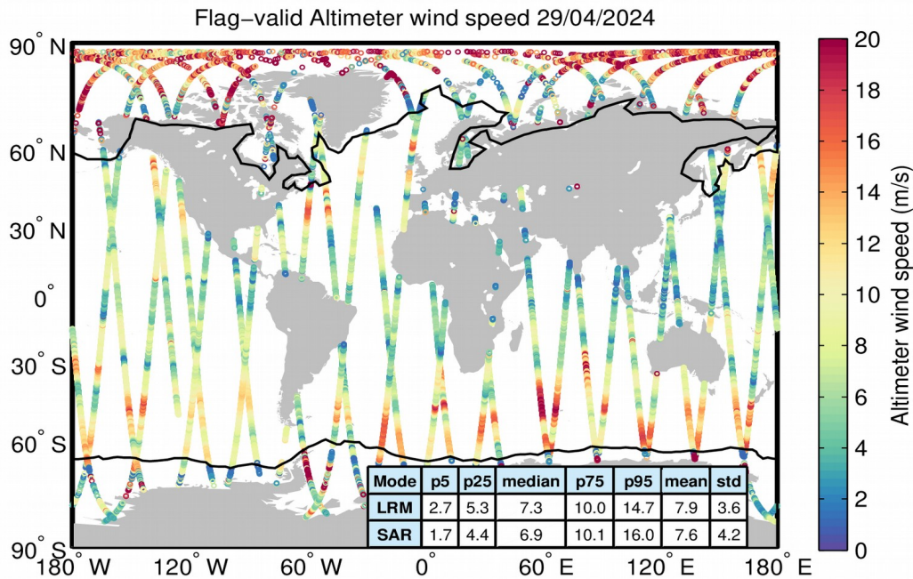
Figure 31. Geographical distribution of flag-valid wind data over oceans and lakes for 29/04/2024. The statistical values shown in the table refer to the wind in m/s and are calculated separately for LRM and SAR regions. Measurements taken over polar polygons have been excluded from the computation of the statistical values. The black lines mark the outer limit of the Arctic and Antarctic polar polygons.
