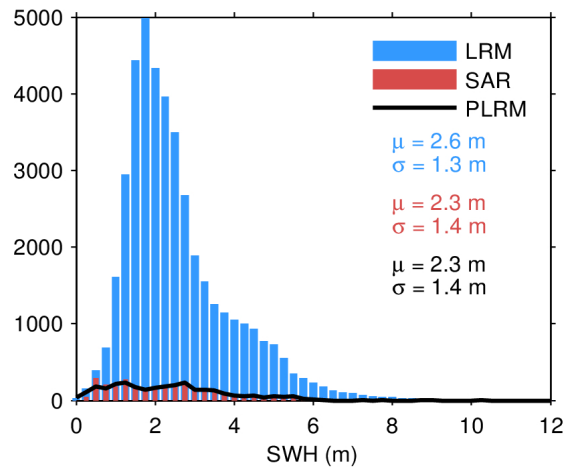
Figure 17. Histogram of flag-valid SWH over oceans and lakes for LRM (blue), SAR (red), and PLRM (black) for 29/04/2024. The mean ( \mu ) and standard deviation ( \sigma ) are also shown. Note that values larger than 12 m are excluded from the histogram for the sake of readability but not from the computation of \mu and \sigma .
