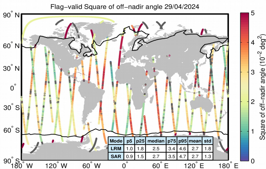
Figure 37. Geographical distribution of flag-valid mispointing data over oceans and lakes for 29/04/2024. The statistical values shown in the table refer to the mispointing in 10^{-2} \text{ deg}^2 and are calculated separately for LRM and SAR regions. Measurements taken over polar polygons have been excluded from the computation of the statistical values. The black lines mark the outer limit of the Arctic and Antarctic polar polygons. Gray circles denote negative values.
