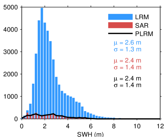
Figure 20. Histogram of science-valid SWH over oceans and lakes for LRM (blue), SAR (red), and PLRM (black) for 29/04/2024. The mean ( \mu ) and standard deviation ( \sigma ) are also
