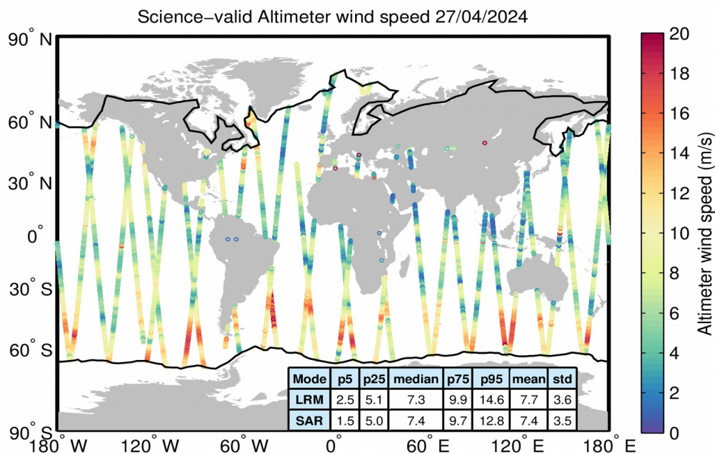
Figure 34. Geographical distribution of science-valid wind data over oceans and lakes for 27/04/2024. The statistical values shown in the table refer to the wind in m/s and are calculated separately for LRM and SAR regions. The black lines mark the outer limit of the Arctic and Antarctic polar polygons. Gray circles denote records that have been rejected based on the editing criteria described in Table 5.
