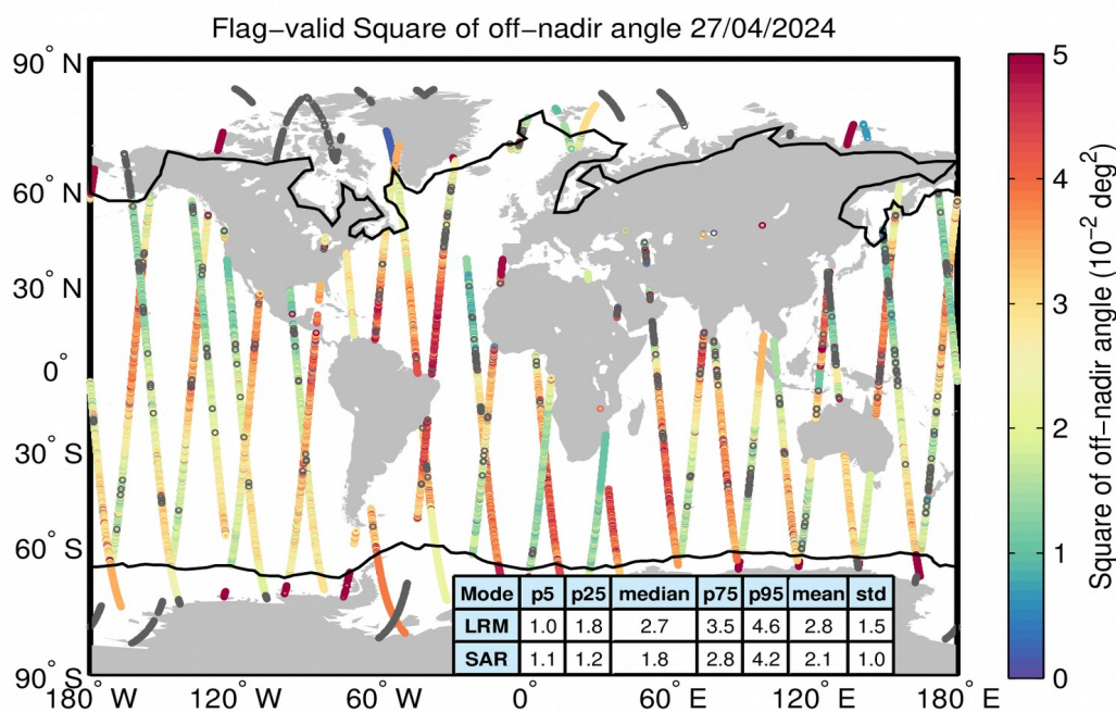
Figure 37. Geographical distribution of flag-valid mispointing data over oceans and lakes for 27/04/2024. The statistical values shown in the table refer to the mispointing in 10^{-2} \text{ deg}^2 and are calculated separately for LRM and SAR regions. Measurements taken over polar polygons have been excluded from the computation of the statistical values. The black lines mark the outer limit of the Arctic and Antarctic polar polygons. Gray circles denote negative values.
