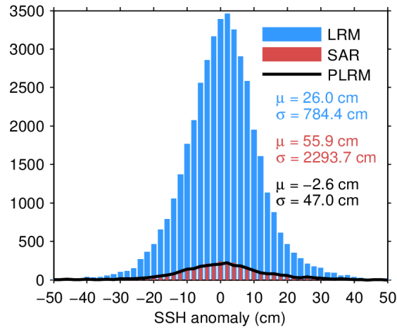
Figure 7. Histogram of flag-valid SSH anomaly over oceans and lakes for LRM (blue), SAR (red), and PLRM (black) for 27/04/2024. The mean ( \mu ) and standard deviation ( \sigma ) are also shown. Note that values outside [-50 50] cm are excluded from the histogram for the sake of readability but not from the computation of \mu and \sigma .
