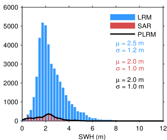
Figure 20. Histogram of science-valid SWH over oceans and lakes for LRM (blue), SAR (red), and PLRM (black) for 27/04/2024. The mean ( \mu ) and standard deviation ( \sigma ) are also
