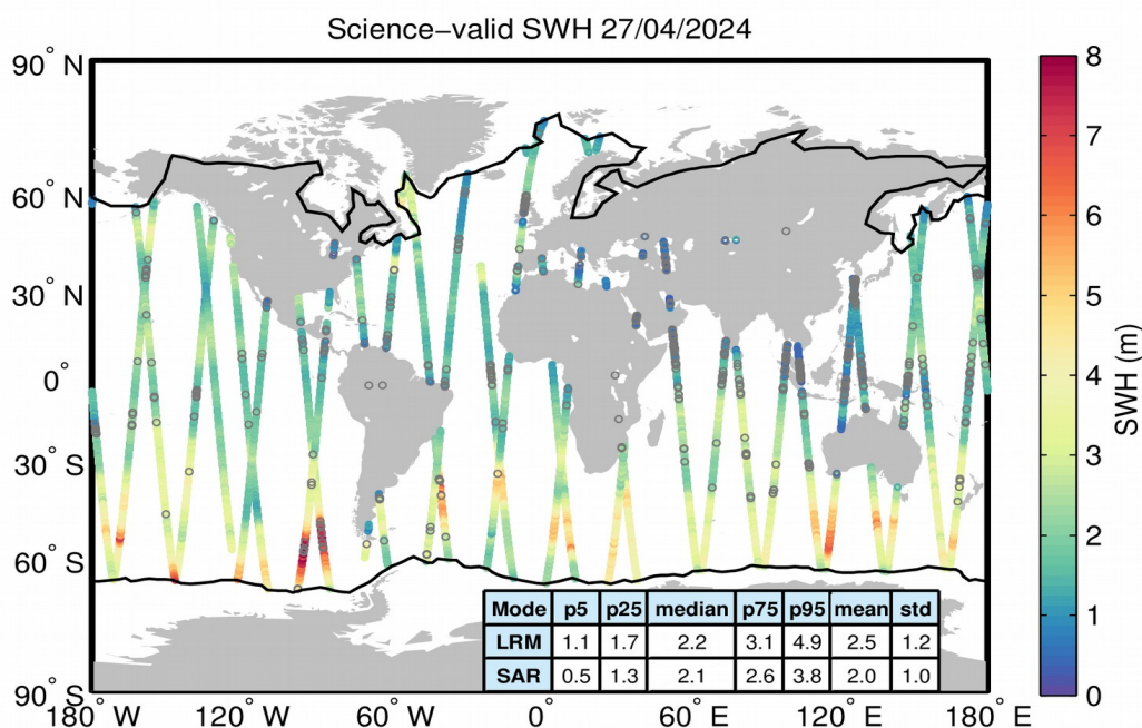
Figure 19. Geographical distribution of science-valid SWH data over oceans and lakes for 27/04/2024. The statistical values shown in the table refer to the SWH in m and are calculated separately for LRM and SAR regions. The black lines mark the outer limit of the Arctic and Antarctic polar polygons. Gray circles denote records that have been rejected based on the editing criteria described in Table 3.
