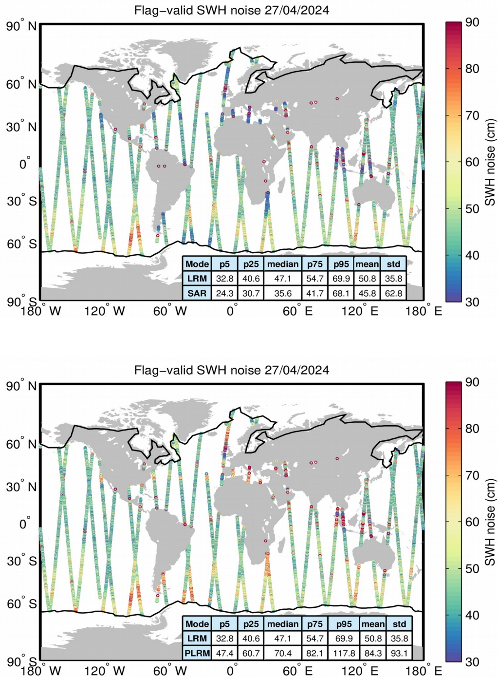
Figure 18. Geographical distribution of flag-valid 20-Hz SWH measurement noise over oceans and lakes for LRM/SAR (top) and LRM/PLRM (bottom) and for 27/04/2024. The statistical values shown in the table refer to the SWH noise and are calculated separately for LRM and SAR/PLRM regions. Measurements taken over polar polygons have been
