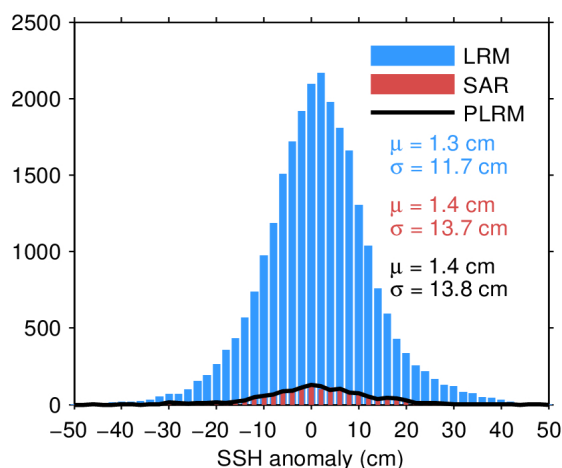
Figure 11. Histogram of science-valid SSH anomaly over oceans and lakes for LRM (blue), SAR (red), and PLRM (black) for 27/04/2024. The mean ( \mu ) and standard deviation ( \sigma ) are also shown. Note that values outside [-50\ 50] cm are excluded from the histogram for the sake of readability but not from the computation of \mu and \sigma .
