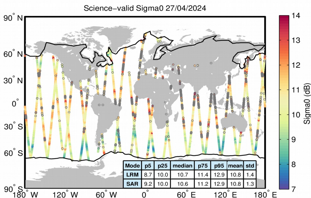
Figure 27. Geographical distribution of science-valid sigma0 data over oceans and lakes for 27/04/2024. The statistical values shown in the table refer to the sigma0 in dB and are calculated separately for LRM and SAR regions. The black lines mark the outer limit of the Arctic and Antarctic polar polygons. Gray circles denote records that have been rejected based on the editing criteria described in Table 4.
