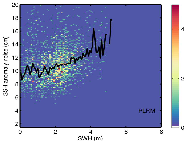
Figure 9. 2D histogram showing flag-valid SSH anomaly noise as a function of SWH for LRM (top), SAR (middle), and PLRM (bottom) for 27/04/2024. The black line denotes the median SSH anomaly noise as a function of SWH.
