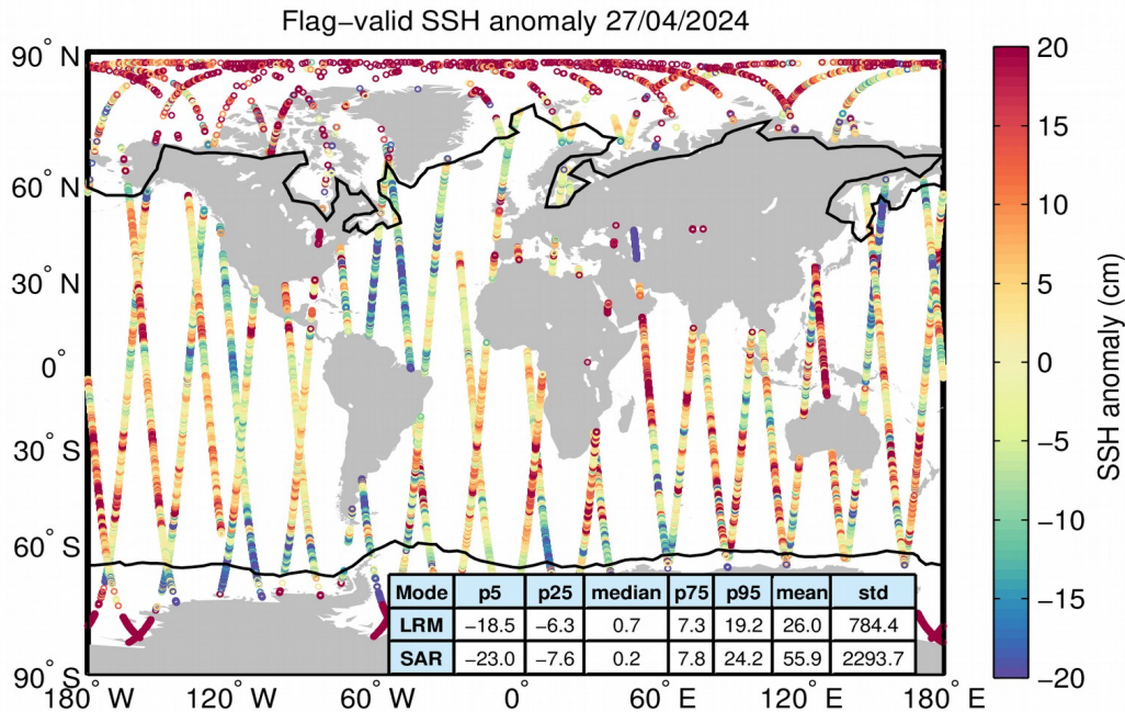
Figure 5. Geographical distribution of flag-valid 1-Hz SSH anomaly data over oceans and lakes for 27/04/2024. The statistical values shown in the table refer to the SSH anomaly in cm and are calculated separately for LRM and SAR regions. Measurements taken over polar polygons have been excluded from the computation of the statistical values. The black lines mark the outer limit of the Arctic and Antarctic polar polygons.
