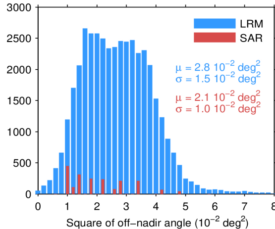
Figure 39. Histogram of flag-valid mispointing over oceans and lakes for LRM (blue) and SAR (red) for 27/04/2024. Only positive values have been considered. The mean ( \mu ) and standard deviation ( \sigma ) are also shown. Note that values larger than 8 \cdot 10^{-2} \text{ deg}^2 are excluded from the histogram for the sake of readability but not from the computation of \mu and \sigma .
