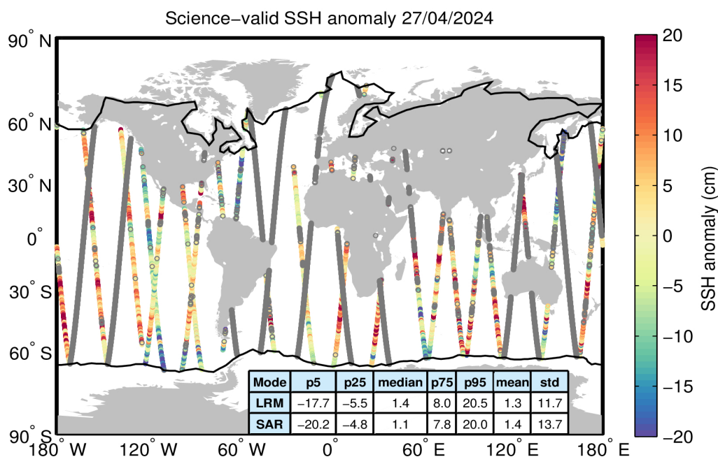
Figure 10. Geographical distribution of science-valid SSH anomaly data over oceans and lakes for 27/04/2024. The statistical values shown in the table refer to the SSH anomaly in cm and are calculated separately for LRM and SAR regions. The black lines mark the
