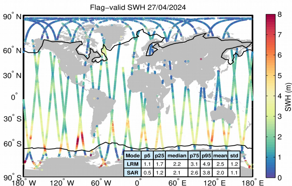
Figure 15. Geographical distribution of flag-valid SWH data over oceans and lakes for 27/04/2024. The statistical values shown in the table refer to the SWH in m and are calculated separately for LRM and SAR regions. Measurements taken over polar polygons have been excluded from the computation of the statistical values. The black lines mark the outer limit of the Arctic and Antarctic polar polygons.
