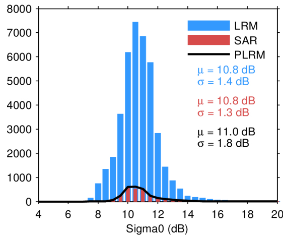
Figure 28. Histogram of science-valid sigma0 over oceans and lakes for LRM (blue), SAR (red), and PLRM (black) for 27/04/2024. The mean ( \mu ) and standard deviation ( \sigma ) are also shown. Note that values outside [4 20] dB are excluded from the histogram for the sake of readability but not from the computation of \mu and \sigma .
