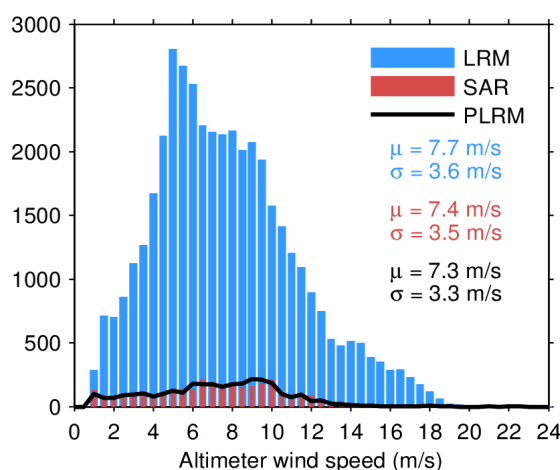
Figure 33. Histogram of flag-valid wind over oceans and lakes for LRM (blue), SAR (red), and PLRM (black) for 27/04/2024. The mean ( \mu ) and standard deviation ( \sigma ) are also shown. Note that values larger than 24 m/s are excluded from the histogram for the sake of readability but not from the computation of \mu and \sigma .
