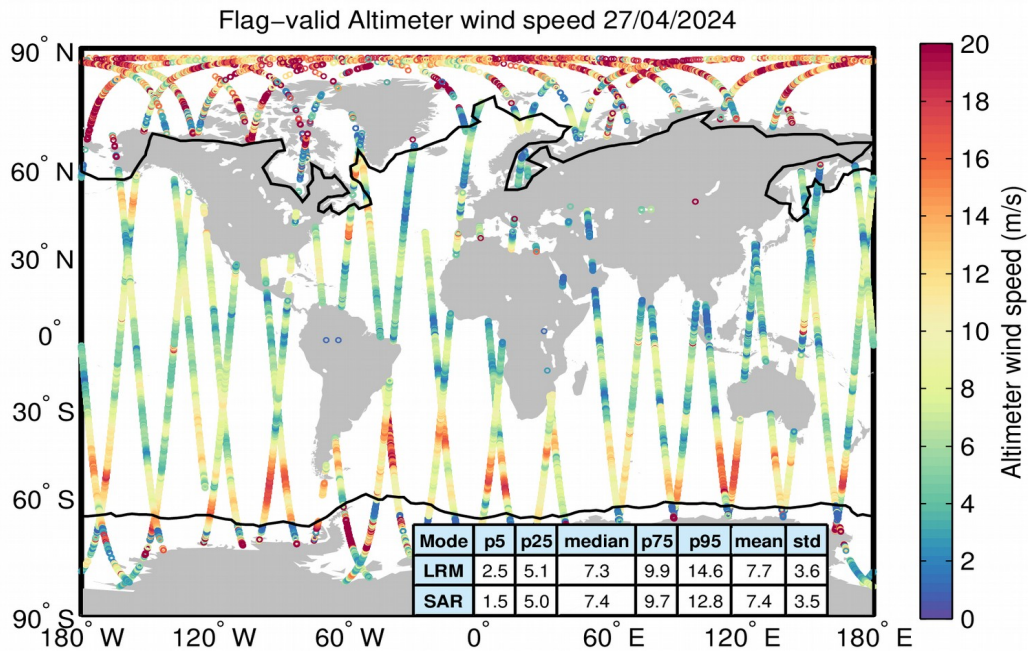
Figure 31. Geographical distribution of flag-valid wind data over oceans and lakes for 27/04/2024. The statistical values shown in the table refer to the wind in m/s and are calculated separately for LRM and SAR regions. Measurements taken over polar polygons have been excluded from the computation of the statistical values. The black lines mark the outer limit of the Arctic and Antarctic polar polygons.
