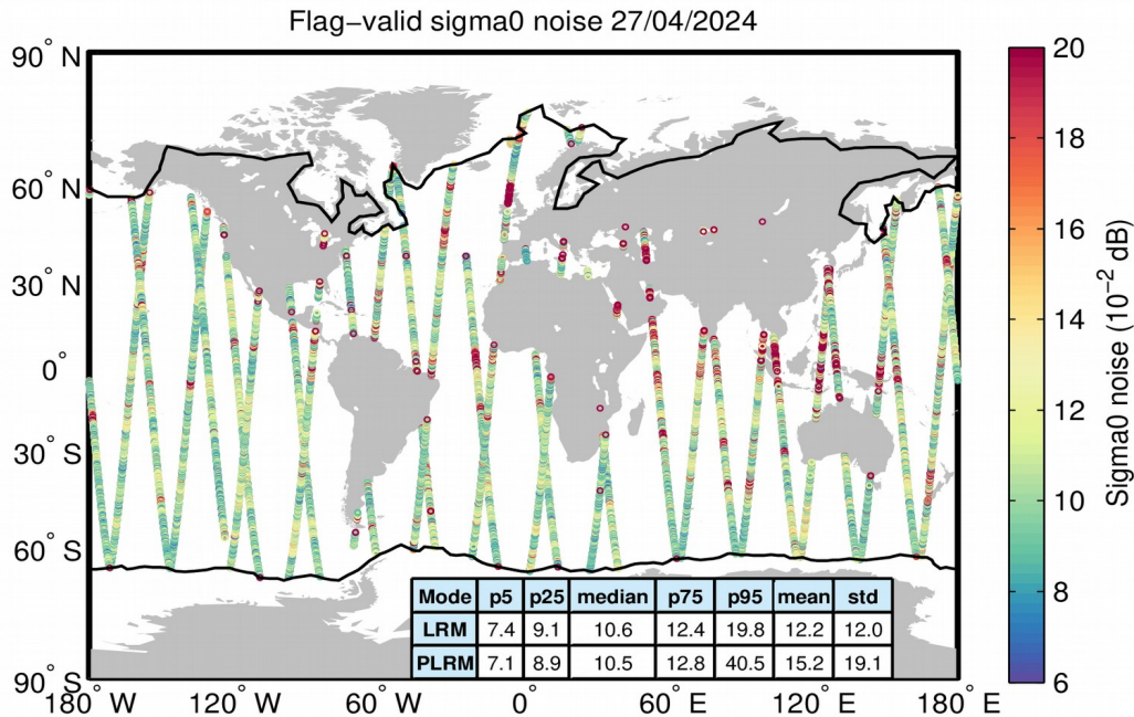
Figure 26. Geographical distribution of flag-valid 20-Hz sigma0 measurement noise over oceans and lakes for LRM/SAR (top) and LRM/PLRM (bottom) and for 27/04/2024. The statistical values shown in the table refer to the sigma0 noise and are calculated separately for LRM and SAR/PLRM regions. Measurements taken over polar polygons have been excluded from the computation of the statistical values. The black lines mark the outer limit of the Arctic and Antarctic polar polygons.
