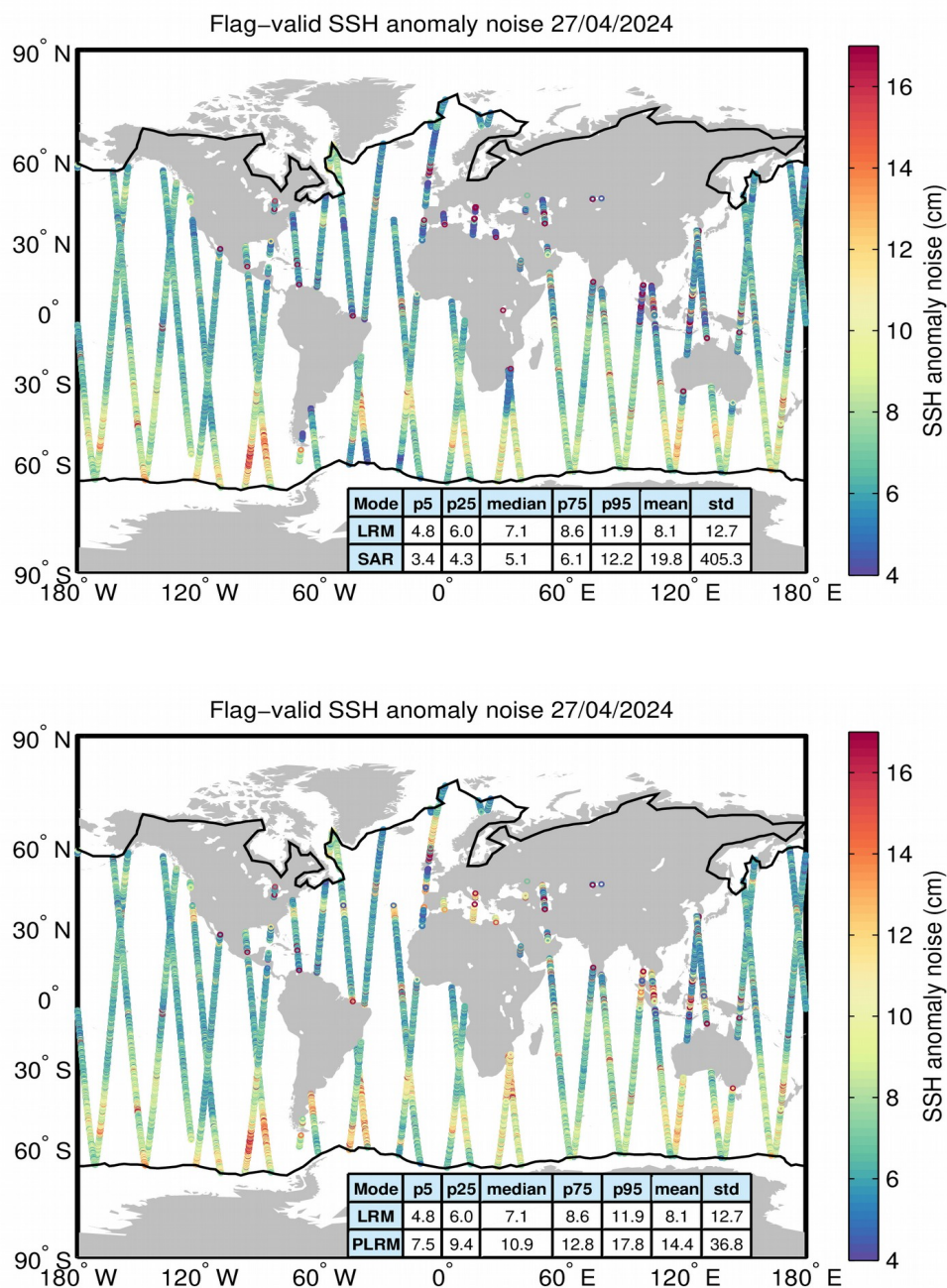
Figure 8. Geographical distribution of flag-valid 20-Hz SSH anomaly measurement noise over oceans and lakes for LRM/SAR (top) and LRM/PLRM (bottom) and for 27/04/2024. The statistical values shown in the tables refer to the SSH anomaly noise and are calculated separately for LRM and SAR/PLRM regions. Measurements taken over polar polygons have been excluded from the computation of the statistical values. The black lines mark the outer limit of the Arctic and Antarctic polar polygons.
