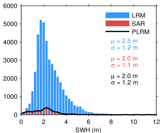
Figure 17. Histogram of flag-valid SWH over oceans and lakes for LRM (blue), SAR (red), and PLRM (black) for 27/04/2024. The mean ( \mu ) and standard deviation ( \sigma ) are also shown. Note that values larger than 12 m are excluded from the histogram for the sake of readability but not from the computation of \mu and \sigma .
