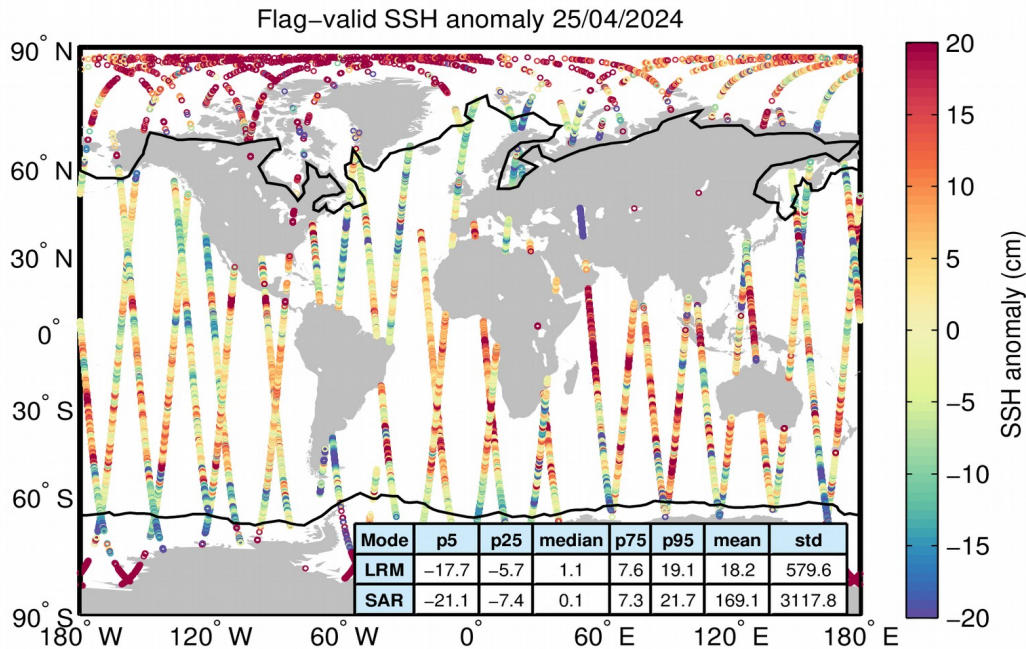
Figure 5. Geographical distribution of flag-valid 1-Hz SSH anomaly data over oceans and lakes for 25/04/2024. The statistical values shown in the table refer to the SSH anomaly in cm and are calculated separately for LRM and SAR regions. Measurements taken over polar polygons have been excluded from the computation of the statistical values. The black lines mark the outer limit of the Arctic and Antarctic polar polygons.
