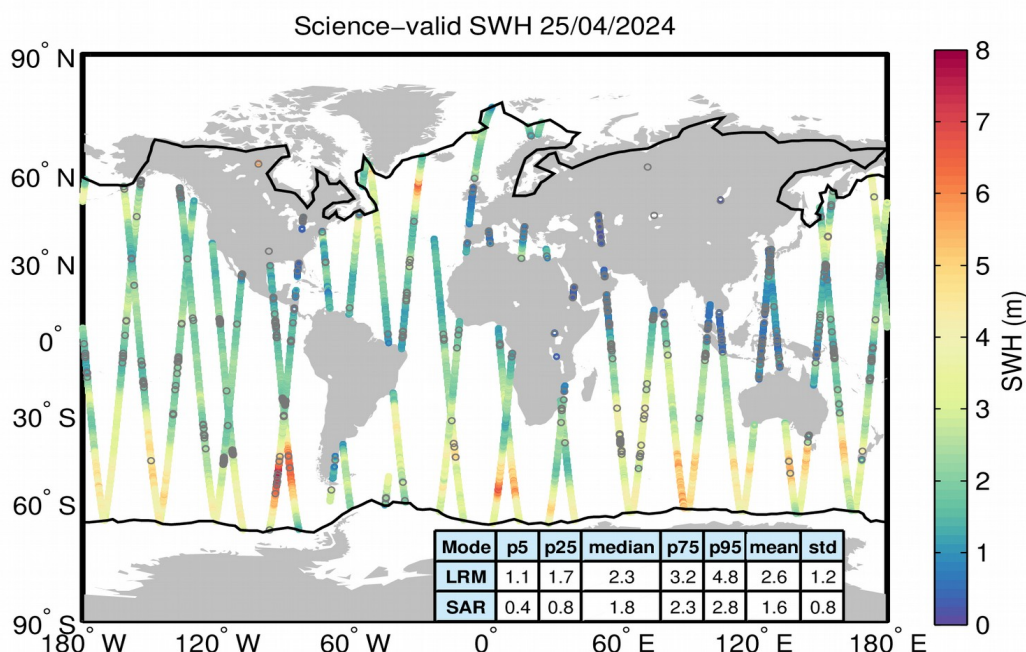
Figure 19. Geographical distribution of science-valid SWH data over oceans and lakes for 25/04/2024. The statistical values shown in the table refer to the SWH in m and are calculated separately for LRM and SAR regions. The black lines mark the outer limit of the Arctic and Antarctic polar polygons. Gray circles denote records that have been rejected based on the editing criteria described in Table 3.
