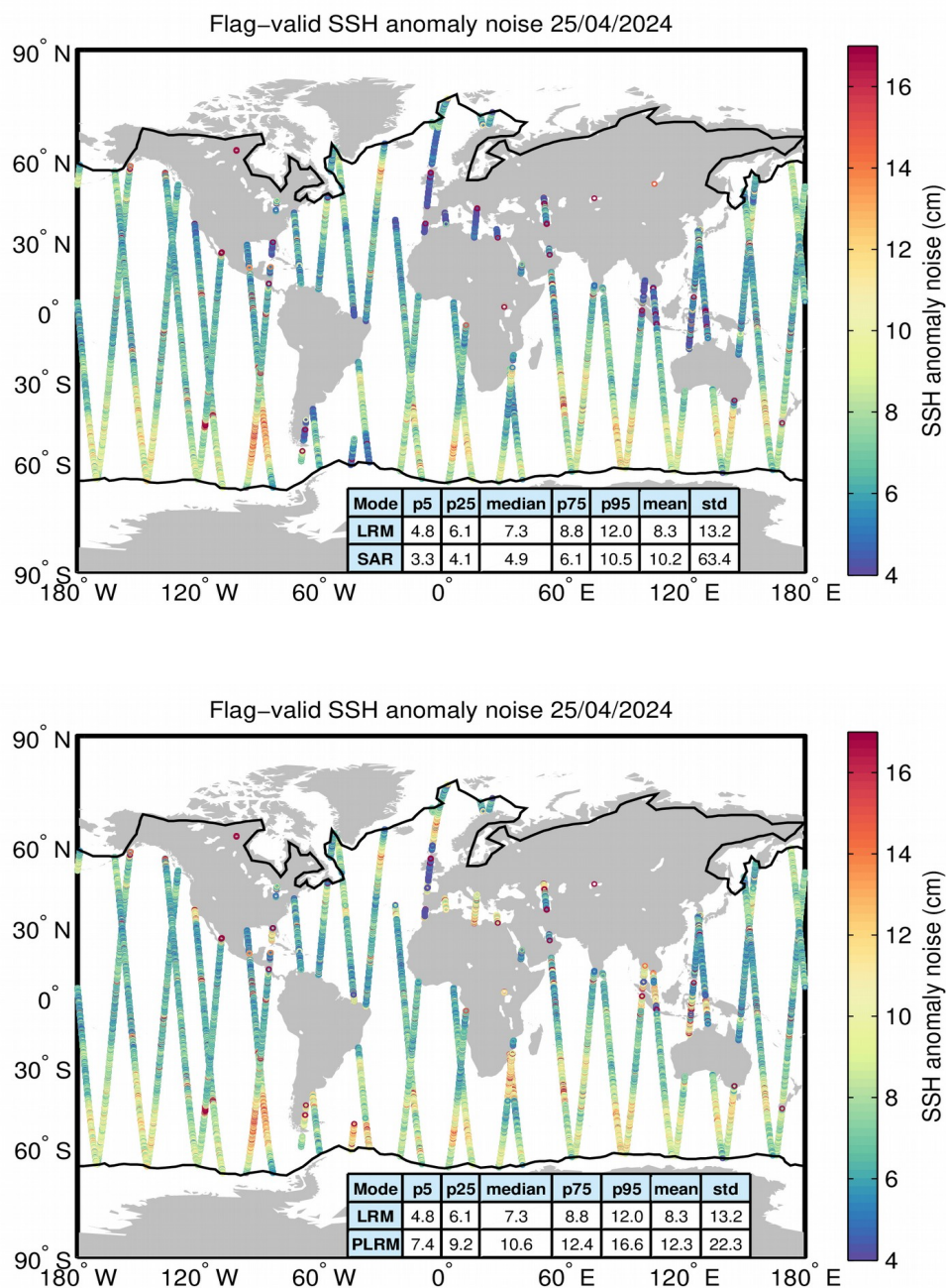
Figure 8. Geographical distribution of flag-valid 20-Hz SSH anomaly measurement noise over oceans and lakes for LRM/SAR (top) and LRM/PLRM (bottom) and for 25/04/2024. The statistical values shown in the tables refer to the SSH anomaly noise and are calculated separately for LRM and SAR/PLRM regions. Measurements taken over polar polygons have been excluded from the computation of the statistical values. The black lines mark the outer limit of the Arctic and Antarctic polar polygons.
