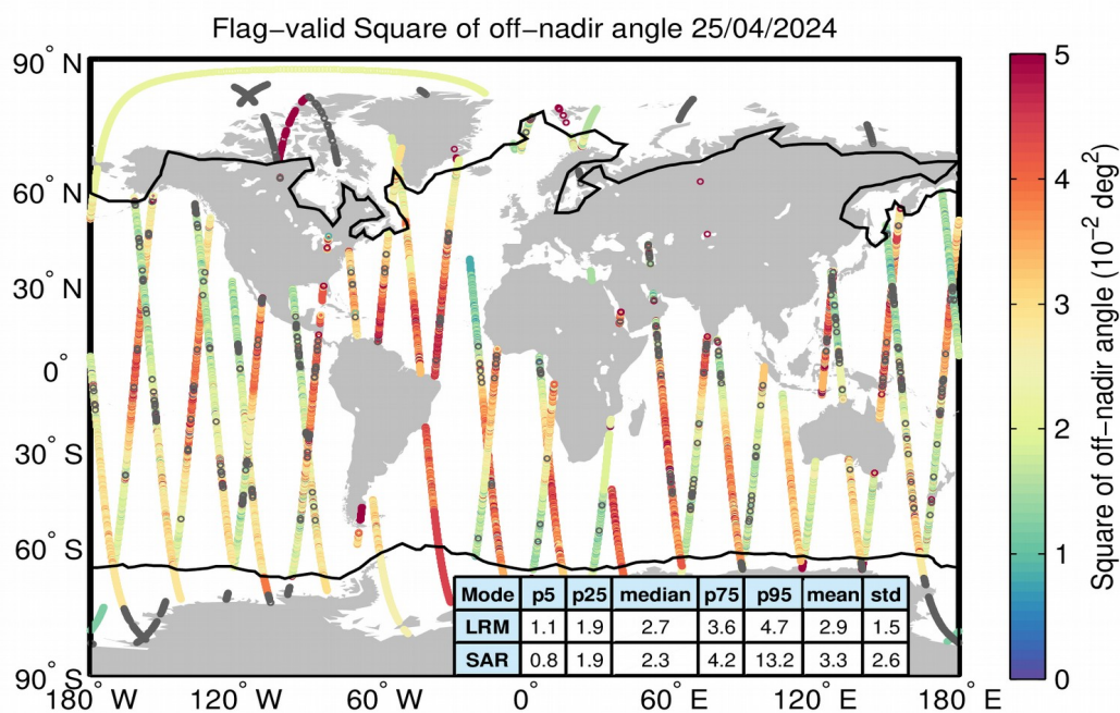
Figure 37. Geographical distribution of flag-valid mispointing data over oceans and lakes for 25/04/2024. The statistical values shown in the table refer to the mispointing in 10^{-2} \text{ deg}^2 and are calculated separately for LRM and SAR regions. Measurements taken over polar polygons have been excluded from the computation of the statistical values. The black lines mark the outer limit of the Arctic and Antarctic polar polygons. Gray circles denote negative values.
