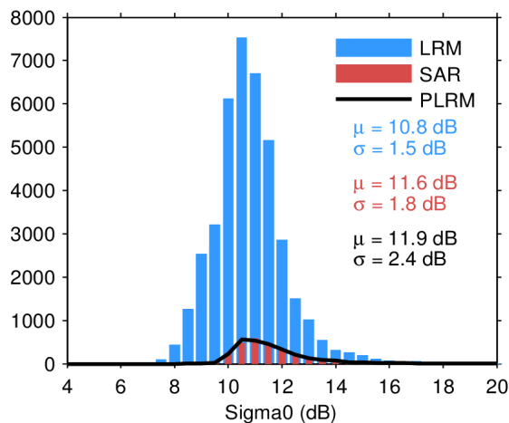
Figure 28. Histogram of science-valid sigma0 over oceans and lakes for LRM (blue), SAR (red), and PLRM (black) for 25/04/2024. The mean ( \mu ) and standard deviation ( \sigma ) are also shown. Note that values outside [4 20] dB are excluded from the histogram for the sake of readability but not from the computation of \mu and \sigma .
