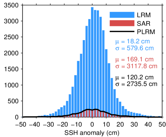
Figure 7. Histogram of flag-valid SSH anomaly over oceans and lakes for LRM (blue), SAR (red), and PLRM (black) for 25/04/2024. The mean ( \mu ) and standard deviation ( \sigma ) are also shown. Note that values outside [-50\ 50] cm are excluded from the histogram for the sake of readability but not from the computation of \mu and \sigma .
