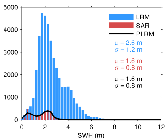
Figure 20. Histogram of science-valid SWH over oceans and lakes for LRM (blue), SAR (red), and PLRM (black) for 25/04/2024. The mean ( \mu ) and standard deviation ( \sigma ) are also
