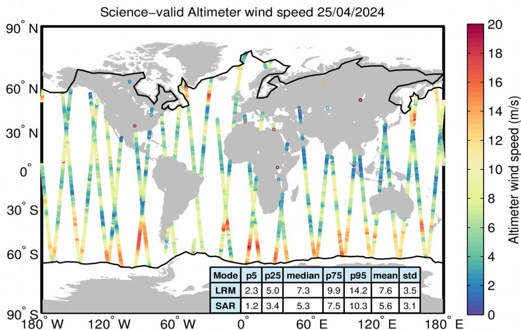
Figure 34. Geographical distribution of science-valid wind data over oceans and lakes for 25/04/2024. The statistical values shown in the table refer to the wind in m/s and are calculated separately for LRM and SAR regions. The black lines mark the outer limit of the Arctic and Antarctic polar polygons. Gray circles denote records that have been rejected based on the editing criteria described in Table 5.
