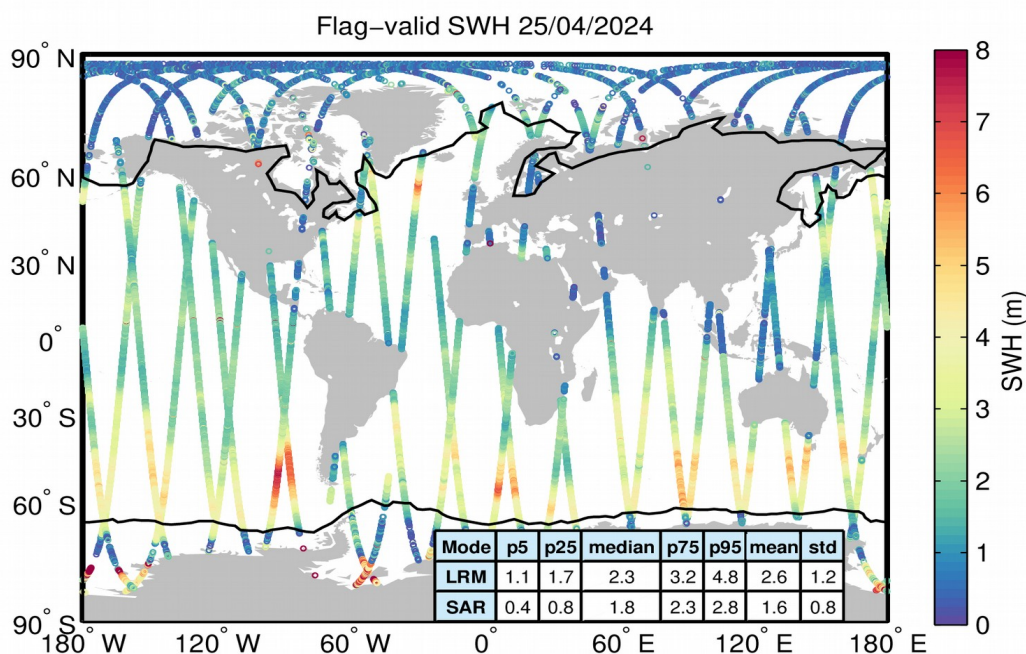
Figure 15. Geographical distribution of flag-valid SWH data over oceans and lakes for 25/04/2024. The statistical values shown in the table refer to the SWH in m and are calculated separately for LRM and SAR regions. Measurements taken over polar polygons have been excluded from the computation of the statistical values. The black lines mark the outer limit of the Arctic and Antarctic polar polygons.
