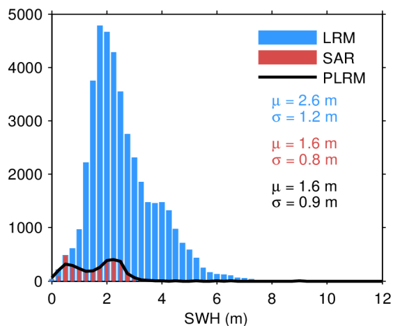
Figure 17. Histogram of flag-valid SWH over oceans and lakes for LRM (blue), SAR (red), and PLRM (black) for 25/04/2024. The mean ( \mu ) and standard deviation ( \sigma ) are also shown. Note that values larger than 12 m are excluded from the histogram for the sake of readability but not from the computation of \mu and \sigma .
