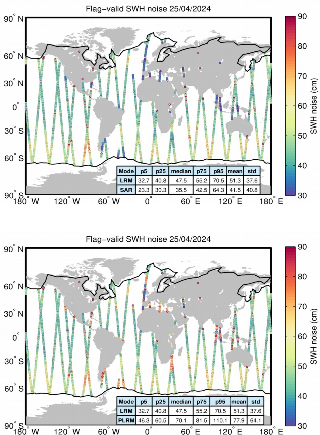
Figure 18. Geographical distribution of flag-valid 20-Hz SWH measurement noise over oceans and lakes for LRM/SAR (top) and LRM/PLRM (bottom) and for 25/04/2024. The statistical values shown in the table refer to the SWH noise and are calculated separately for LRM and SAR/PLRM regions. Measurements taken over polar polygons have been
