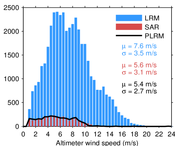
Figure 33. Histogram of flag-valid wind over oceans and lakes for LRM (blue), SAR (red), and PLRM (black) for 25/04/2024. The mean ( \mu ) and standard deviation ( \sigma ) are also shown. Note that values larger than 24 m/s are excluded from the histogram for the sake of readability but not from the computation of \mu and \sigma .
