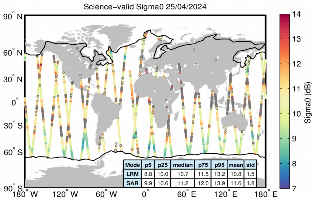
Figure 27. Geographical distribution of science-valid sigma0 data over oceans and lakes for 25/04/2024. The statistical values shown in the table refer to the sigma0 in dB and are calculated separately for LRM and SAR regions. The black lines mark the outer limit of the Arctic and Antarctic polar polygons. Gray circles denote records that have been rejected based on the editing criteria described in Table 4.
