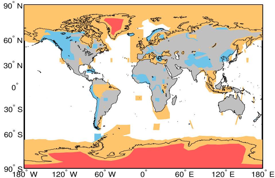
Figure A1. Extent of the regions defining the geographical mode mask for 25/04/2024. The regions where SAR, and SARIn are operated are denoted by the orange and blue polygons, respectively. LRM is operated over areas of the continental ice sheets (red polygons) and over oceans and land not covered by other modes.
