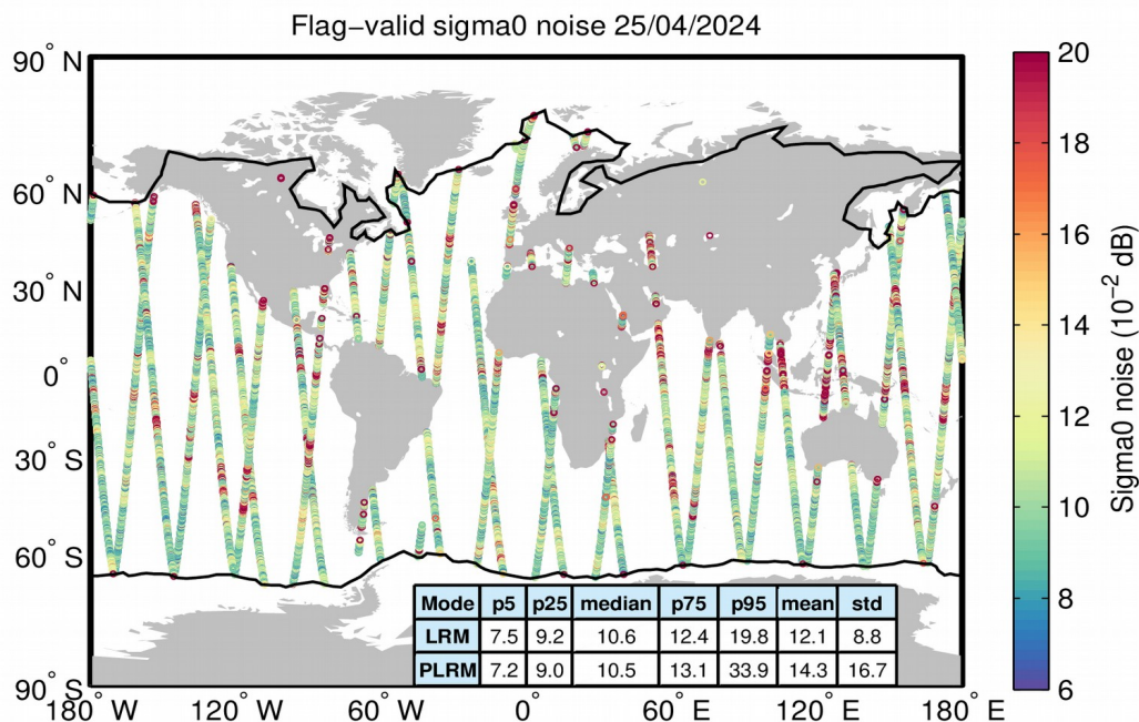
Figure 26. Geographical distribution of flag-valid 20-Hz sigma0 measurement noise over oceans and lakes for LRM/SAR (top) and LRM/PLRM (bottom) and for 25/04/2024. The statistical values shown in the table refer to the sigma0 noise and are calculated separately for LRM and SAR/PLRM regions. Measurements taken over polar polygons have been excluded from the computation of the statistical values. The black lines mark the outer limit of the Arctic and Antarctic polar polygons.
