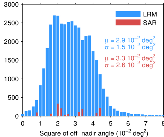
Figure 39. Histogram of flag-valid mispointing over oceans and lakes for LRM (blue) and SAR (red) for 25/04/2024. Only positive values have been considered. The mean ( \mu ) and standard deviation ( \sigma ) are also shown. Note that values larger than 8 \cdot 10^{-2} \text{ deg}^2 are excluded from the histogram for the sake of readability but not from the computation of \mu and \sigma .
