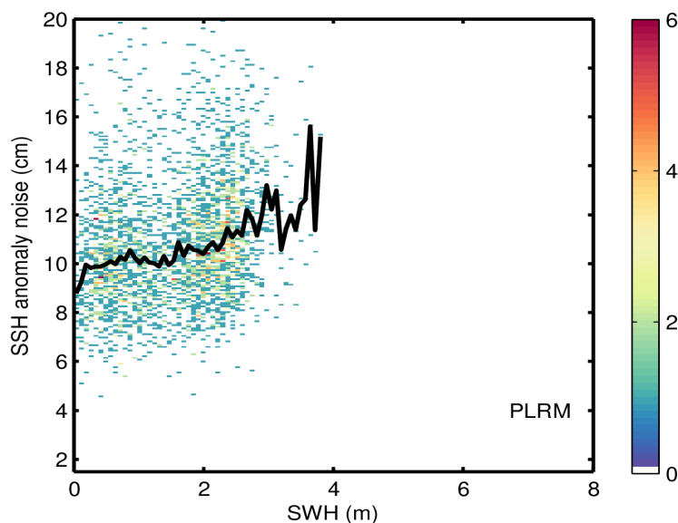
Figure 9. 2D histogram showing flag-valid SSH anomaly noise as a function of SWH for LRM (top), SAR (middle), and PLRM (bottom) for 25/04/2024. The black line denotes the median SSH anomaly noise as a function of SWH.
