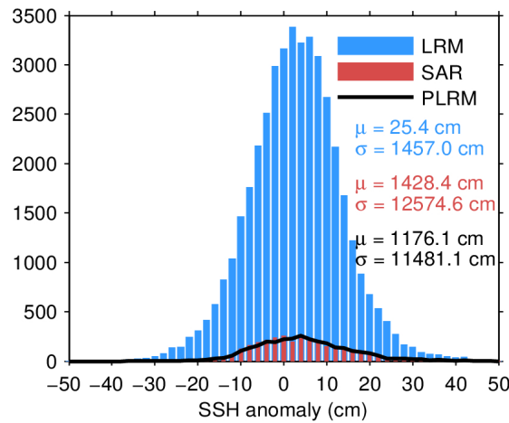
Figure 7. Histogram of flag-valid SSH anomaly over oceans and lakes for LRM (blue), SAR (red), and PLRM (black) for 23/04/2024. The mean ( \mu ) and standard deviation ( \sigma ) are also shown. Note that values outside [-50\ 50] cm are excluded from the histogram for the sake of readability but not from the computation of \mu and \sigma .
