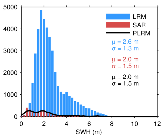
Figure 20. Histogram of science-valid SWH over oceans and lakes for LRM (blue), SAR (red), and PLRM (black) for 23/04/2024. The mean ( \mu ) and standard deviation ( \sigma ) are also
