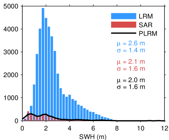
Figure 17. Histogram of flag-valid SWH over oceans and lakes for LRM (blue), SAR (red), and PLRM (black) for 23/04/2024. The mean ( \mu ) and standard deviation ( \sigma ) are also shown. Note that values larger than 12 m are excluded from the histogram for the sake of readability but not from the computation of \mu and \sigma .
