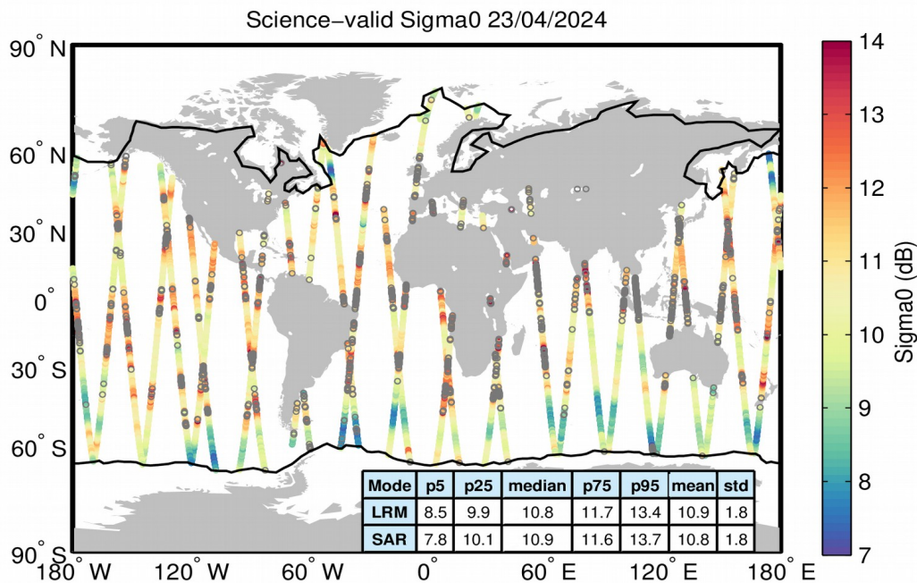
Figure 27. Geographical distribution of science-valid sigma0 data over oceans and lakes for 23/04/2024. The statistical values shown in the table refer to the sigma0 in dB and are calculated separately for LRM and SAR regions. The black lines mark the outer limit of the Arctic and Antarctic polar polygons. Gray circles denote records that have been rejected based on the editing criteria described in Table 4.
