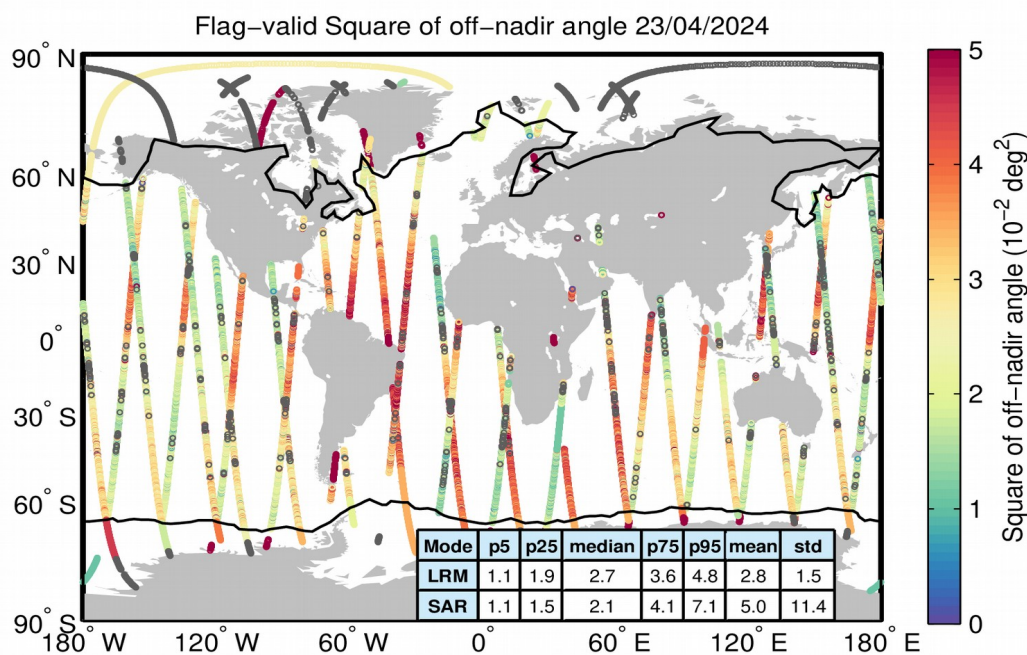
Figure 37. Geographical distribution of flag-valid mispointing data over oceans and lakes for 23/04/2024. The statistical values shown in the table refer to the mispointing in 10^{-2} \text{ deg}^2 and are calculated separately for LRM and SAR regions. Measurements taken over polar polygons have been excluded from the computation of the statistical values. The black lines mark the outer limit of the Arctic and Antarctic polar polygons. Gray circles denote negative values.
