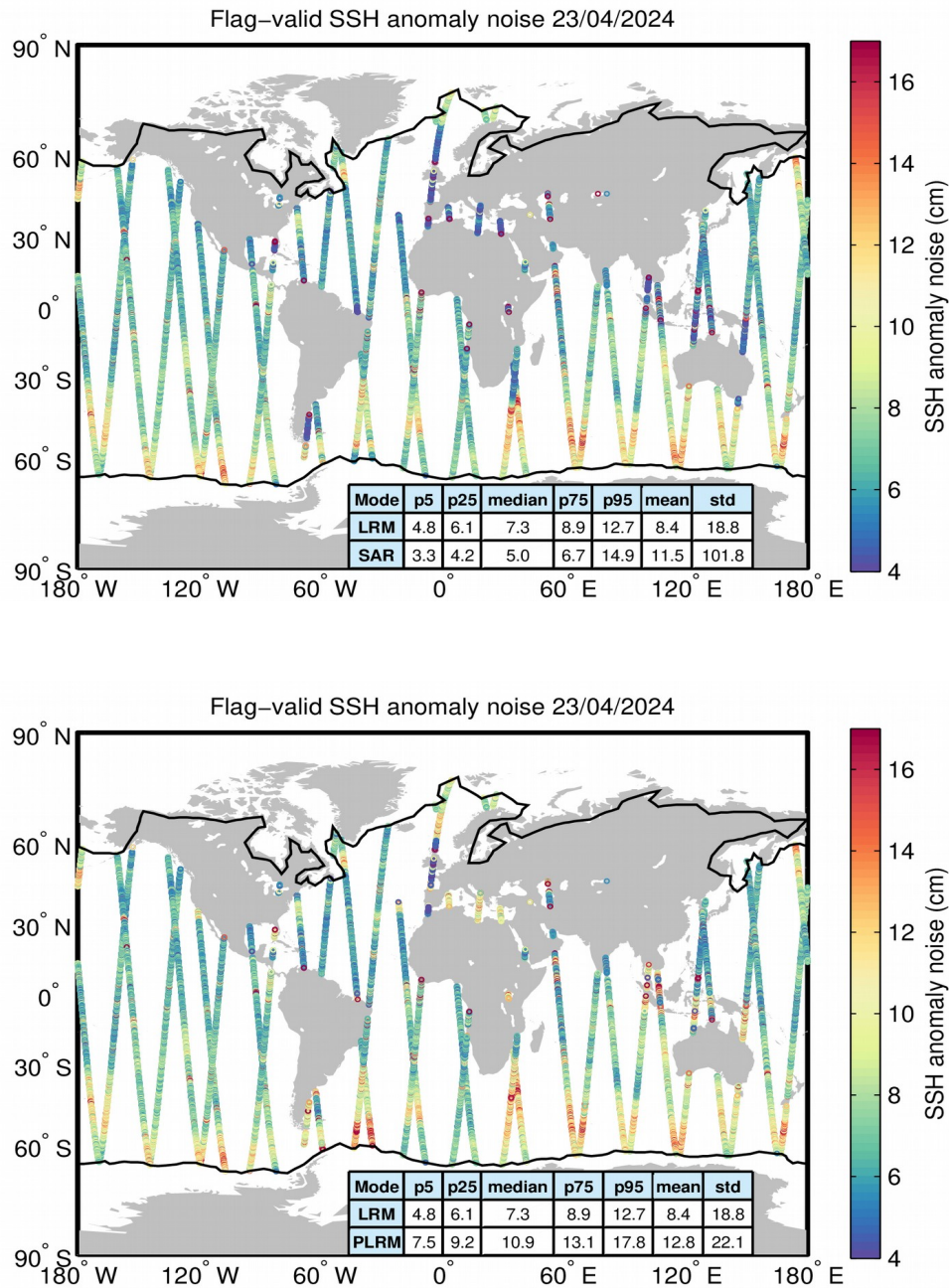
Figure 8. Geographical distribution of flag-valid 20-Hz SSH anomaly measurement noise over oceans and lakes for LRM/SAR (top) and LRM/PLRM (bottom) and for 23/04/2024. The statistical values shown in the tables refer to the SSH anomaly noise and are calculated separately for LRM and SAR/PLRM regions. Measurements taken over polar polygons have been excluded from the computation of the statistical values. The black lines mark the outer limit of the Arctic and Antarctic polar polygons.
