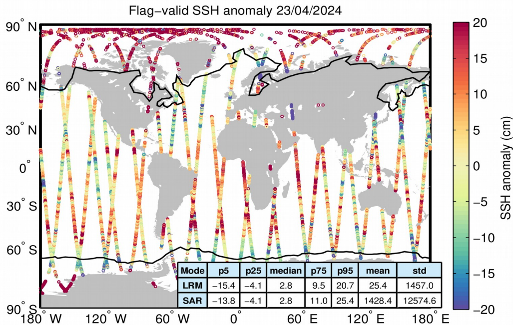
Figure 5. Geographical distribution of flag-valid 1-Hz SSH anomaly data over oceans and lakes for 23/04/2024. The statistical values shown in the table refer to the SSH anomaly in cm and are calculated separately for LRM and SAR regions. Measurements taken over polar polygons have been excluded from the computation of the statistical values. The black lines mark the outer limit of the Arctic and Antarctic polar polygons.
