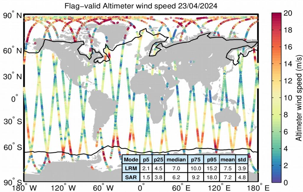
Figure 31. Geographical distribution of flag-valid wind data over oceans and lakes for 23/04/2024. The statistical values shown in the table refer to the wind in m/s and are calculated separately for LRM and SAR regions. Measurements taken over polar polygons have been excluded from the computation of the statistical values. The black lines mark the outer limit of the Arctic and Antarctic polar polygons.
