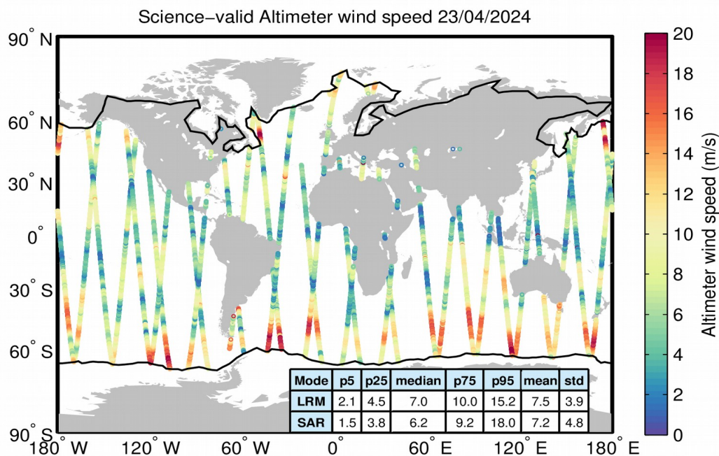
Figure 34. Geographical distribution of science-valid wind data over oceans and lakes for 23/04/2024. The statistical values shown in the table refer to the wind in m/s and are calculated separately for LRM and SAR regions. The black lines mark the outer limit of the Arctic and Antarctic polar polygons. Gray circles denote records that have been rejected based on the editing criteria described in Table 5.
