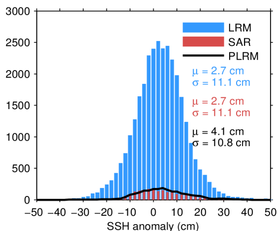
Figure 11. Histogram of science-valid SSH anomaly over oceans and lakes for LRM (blue), SAR (red), and PLRM (black) for 23/04/2024. The mean ( \mu ) and standard deviation ( \sigma ) are also shown. Note that values outside [-50, 50] cm are excluded from the histogram for the sake of readability but not from the computation of \mu and \sigma .
