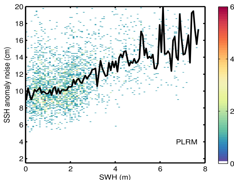
Figure 9. 2D histogram showing flag-valid SSH anomaly noise as a function of SWH for LRM (top), SAR (middle), and PLRM (bottom) for 23/04/2024. The black line denotes the median SSH anomaly noise as a function of SWH.
