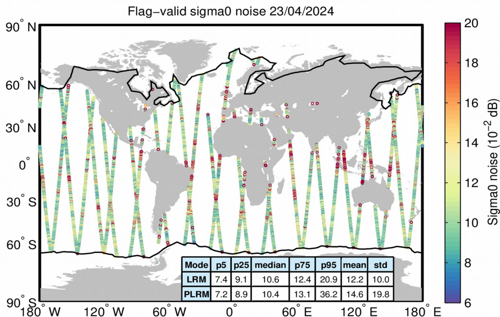
Figure 26. Geographical distribution of flag-valid 20-Hz sigma0 measurement noise over oceans and lakes for LRM/SAR (top) and LRM/PLRM (bottom) and for 23/04/2024. The statistical values shown in the table refer to the sigma0 noise and are calculated separately for LRM and SAR/PLRM regions. Measurements taken over polar polygons have been excluded from the computation of the statistical values. The black lines mark the outer limit of the Arctic and Antarctic polar polygons.
