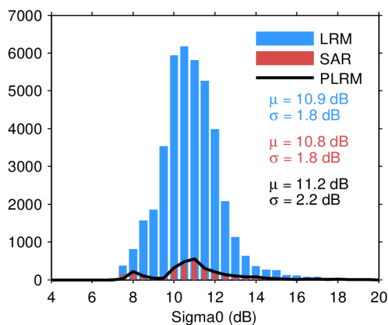
Figure 28. Histogram of science-valid sigma0 over oceans and lakes for LRM (blue), SAR (red), and PLRM (black) for 23/04/2024. The mean ( \mu ) and standard deviation ( \sigma ) are also shown. Note that values outside [4 20] dB are excluded from the histogram for the sake of readability but not from the computation of \mu and \sigma .
