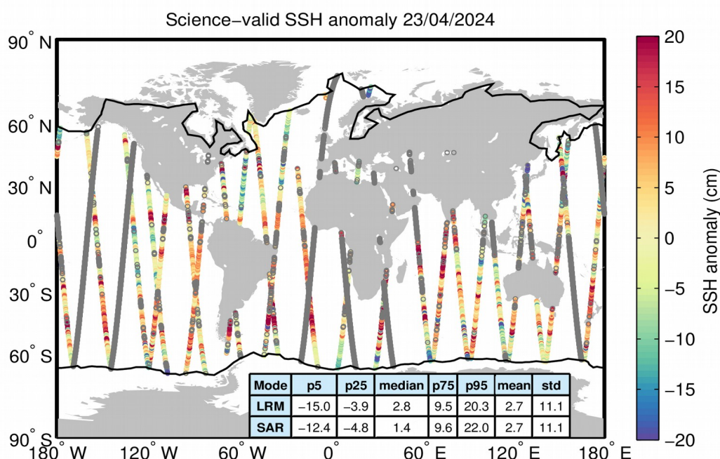
Figure 10. Geographical distribution of science-valid SSH anomaly data over oceans and lakes for 23/04/2024. The statistical values shown in the table refer to the SSH anomaly in cm and are calculated separately for LRM and SAR regions. The black lines mark the
