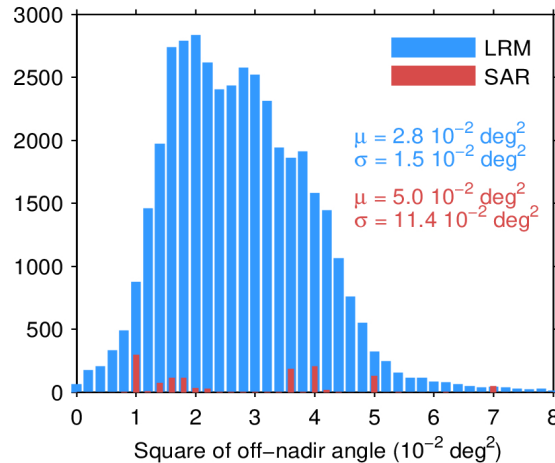
Figure 39. Histogram of flag-valid mispointing over oceans and lakes for LRM (blue) and SAR (red) for 23/04/2024. Only positive values have been considered. The mean ( \mu ) and standard deviation ( \sigma ) are also shown. Note that values larger than 8 \cdot 10^{-2} \text{ deg}^2 are excluded from the histogram for the sake of readability but not from the computation of \mu and \sigma .
