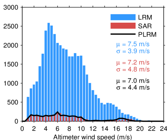
Figure 33. Histogram of flag-valid wind over oceans and lakes for LRM (blue), SAR (red), and PLRM (black) for 23/04/2024. The mean ( \mu ) and standard deviation ( \sigma ) are also shown. Note that values larger than 24 m/s are excluded from the histogram for the sake of readability but not from the computation of \mu and \sigma .
