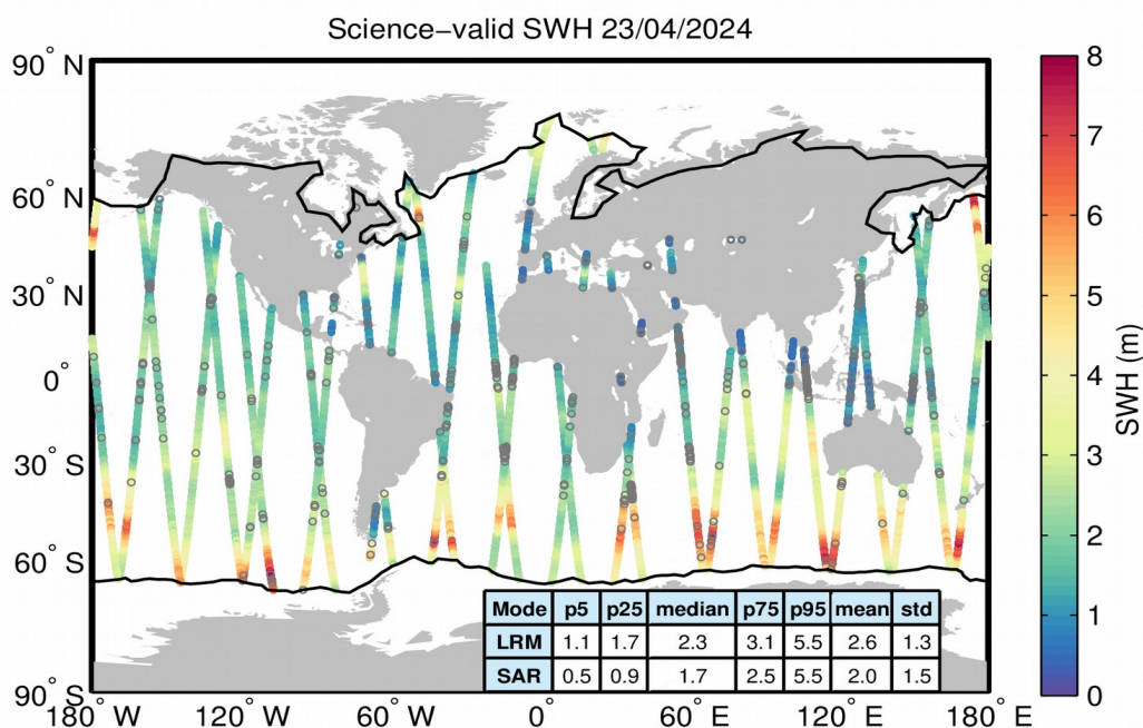
Figure 19. Geographical distribution of science-valid SWH data over oceans and lakes for 23/04/2024. The statistical values shown in the table refer to the SWH in m and are calculated separately for LRM and SAR regions. The black lines mark the outer limit of the Arctic and Antarctic polar polygons. Gray circles denote records that have been rejected based on the editing criteria described in Table 3.
