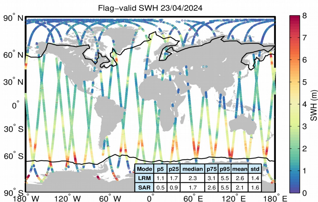
Figure 15. Geographical distribution of flag-valid SWH data over oceans and lakes for 23/04/2024. The statistical values shown in the table refer to the SWH in m and are calculated separately for LRM and SAR regions. Measurements taken over polar polygons have been excluded from the computation of the statistical values. The black lines mark the outer limit of the Arctic and Antarctic polar polygons.
