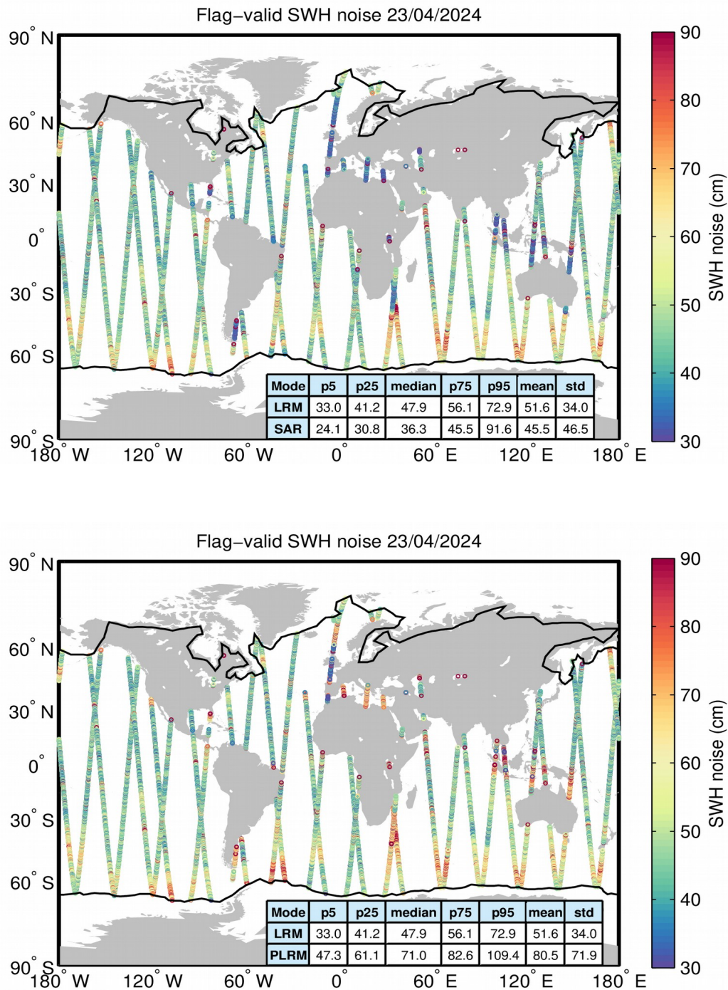
Figure 18. Geographical distribution of flag-valid 20-Hz SWH measurement noise over oceans and lakes for LRM/SAR (top) and LRM/PLRM (bottom) and for 23/04/2024. The statistical values shown in the table refer to the SWH noise and are calculated separately for LRM and SAR/PLRM regions. Measurements taken over polar polygons have been
