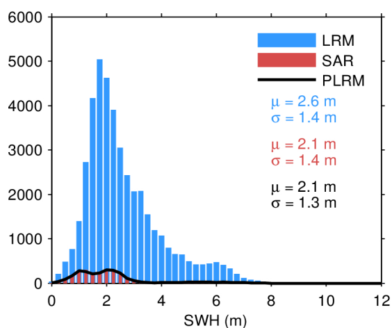
Figure 20. Histogram of science-valid SWH over oceans and lakes for LRM (blue), SAR (red), and PLRM (black) for 22/04/2024. The mean ( \mu ) and standard deviation ( \sigma ) are also
