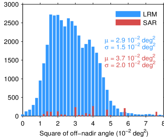
Figure 39. Histogram of flag-valid mispointing over oceans and lakes for LRM (blue) and SAR (red) for 19/04/2024. Only positive values have been considered. The mean ( \mu ) and standard deviation ( \sigma ) are also shown. Note that values larger than 8 \cdot 10^{-2} \text{ deg}^2 are excluded from the histogram for the sake of readability but not from the computation of \mu and \sigma .
