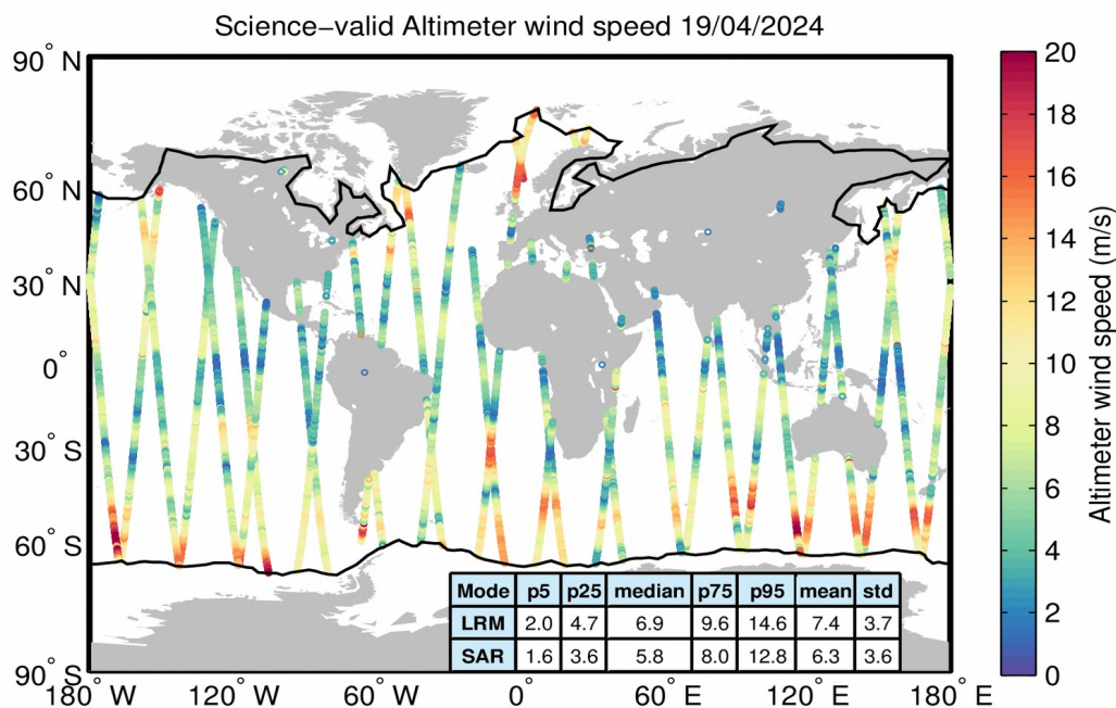
Figure 34. Geographical distribution of science-valid wind data over oceans and lakes for 19/04/2024. The statistical values shown in the table refer to the wind in m/s and are calculated separately for LRM and SAR regions. The black lines mark the outer limit of the Arctic and Antarctic polar polygons. Gray circles denote records that have been rejected based on the editing criteria described in Table 5.
