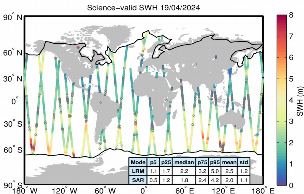
Figure 19. Geographical distribution of science-valid SWH data over oceans and lakes for 19/04/2024. The statistical values shown in the table refer to the SWH in m and are calculated separately for LRM and SAR regions. The black lines mark the outer limit of the Arctic and Antarctic polar polygons. Gray circles denote records that have been rejected based on the editing criteria described in Table 3.
