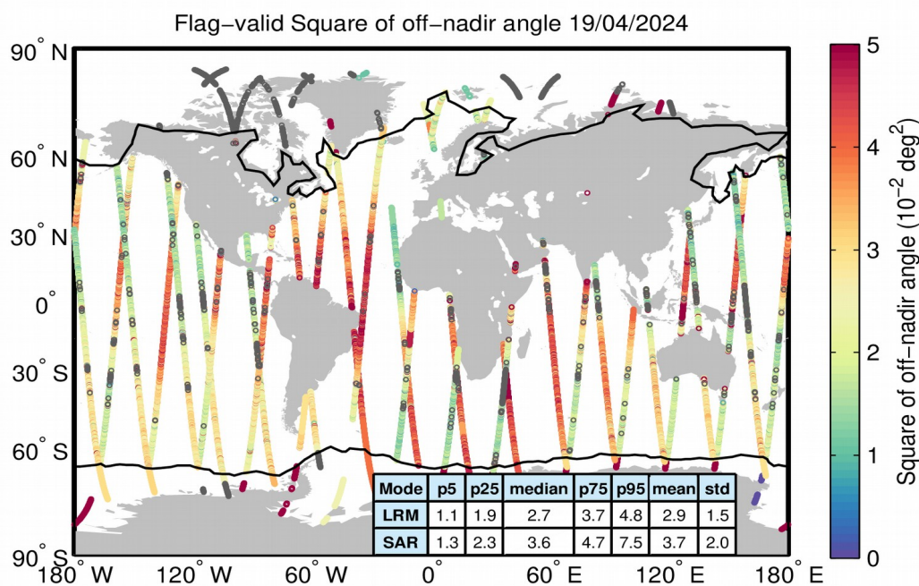
Figure 37. Geographical distribution of flag-valid mispointing data over oceans and lakes for 19/04/2024. The statistical values shown in the table refer to the mispointing in 10^{-2} \text{ deg}^2 and are calculated separately for LRM and SAR regions. Measurements taken over polar polygons have been excluded from the computation of the statistical values. The black lines mark the outer limit of the Arctic and Antarctic polar polygons. Gray circles denote negative values.
