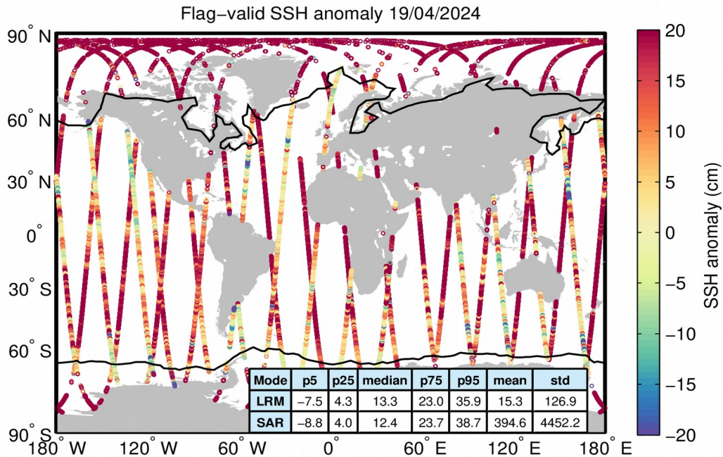
Figure 5. Geographical distribution of flag-valid 1-Hz SSH anomaly data over oceans and lakes for 19/04/2024. The statistical values shown in the table refer to the SSH anomaly in cm and are calculated separately for LRM and SAR regions. Measurements taken over polar polygons have been excluded from the computation of the statistical values. The black lines mark the outer limit of the Arctic and Antarctic polar polygons.
