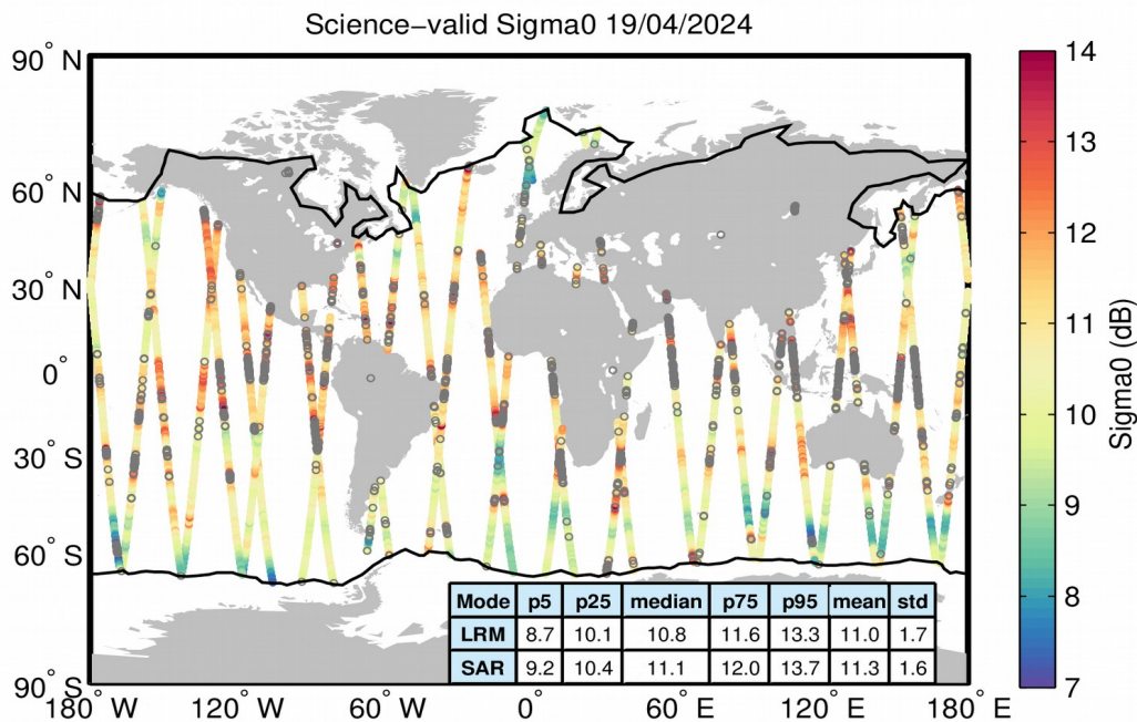
Figure 27. Geographical distribution of science-valid sigma0 data over oceans and lakes for 19/04/2024. The statistical values shown in the table refer to the sigma0 in dB and are calculated separately for LRM and SAR regions. The black lines mark the outer limit of the Arctic and Antarctic polar polygons. Gray circles denote records that have been rejected based on the editing criteria described in Table 4.
