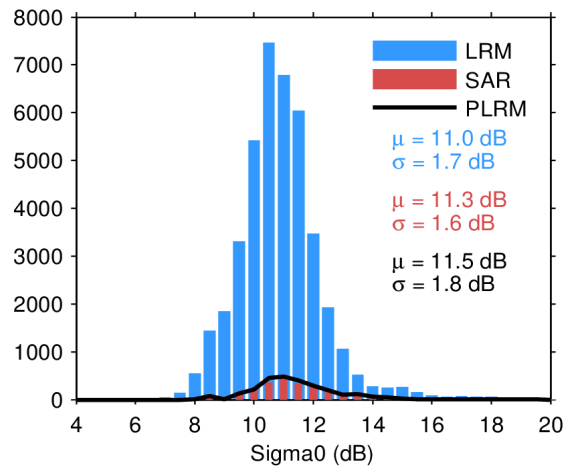
Figure 28. Histogram of science-valid sigma0 over oceans and lakes for LRM (blue), SAR (red), and PLRM (black) for 19/04/2024. The mean ( \mu ) and standard deviation ( \sigma ) are also shown. Note that values outside [4 20] dB are excluded from the histogram for the sake of readability but not from the computation of \mu and \sigma .
