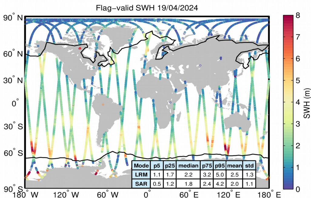
Figure 15. Geographical distribution of flag-valid SWH data over oceans and lakes for 19/04/2024. The statistical values shown in the table refer to the SWH in m and are calculated separately for LRM and SAR regions. Measurements taken over polar polygons have been excluded from the computation of the statistical values. The black lines mark the outer limit of the Arctic and Antarctic polar polygons.
