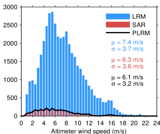
Figure 33. Histogram of flag-valid wind over oceans and lakes for LRM (blue), SAR (red), and PLRM (black) for 19/04/2024. The mean ( \mu ) and standard deviation ( \sigma ) are also shown. Note that values larger than 24 m/s are excluded from the histogram for the sake of readability but not from the computation of \mu and \sigma .
