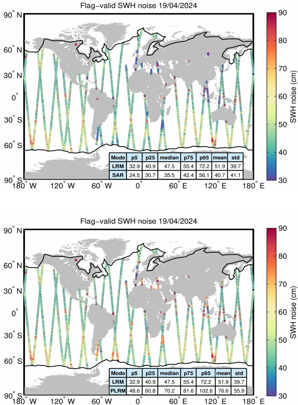
Figure 18. Geographical distribution of flag-valid 20-Hz SWH measurement noise over oceans and lakes for LRM/SAR (top) and LRM/PLRM (bottom) and for 19/04/2024. The statistical values shown in the table refer to the SWH noise and are calculated separately for LRM and SAR/PLRM regions. Measurements taken over polar polygons have been
