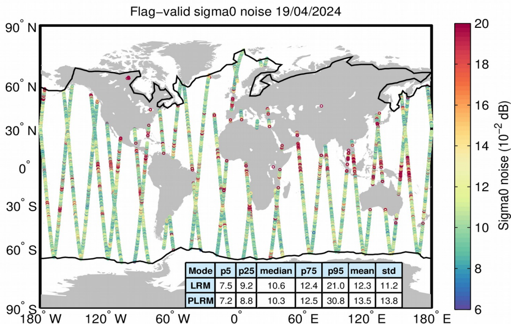
Figure 26. Geographical distribution of flag-valid 20-Hz sigma0 measurement noise over oceans and lakes for LRM/SAR (top) and LRM/PLRM (bottom) and for 19/04/2024. The statistical values shown in the table refer to the sigma0 noise and are calculated separately for LRM and SAR/PLRM regions. Measurements taken over polar polygons have been excluded from the computation of the statistical values. The black lines mark the outer limit of the Arctic and Antarctic polar polygons.
