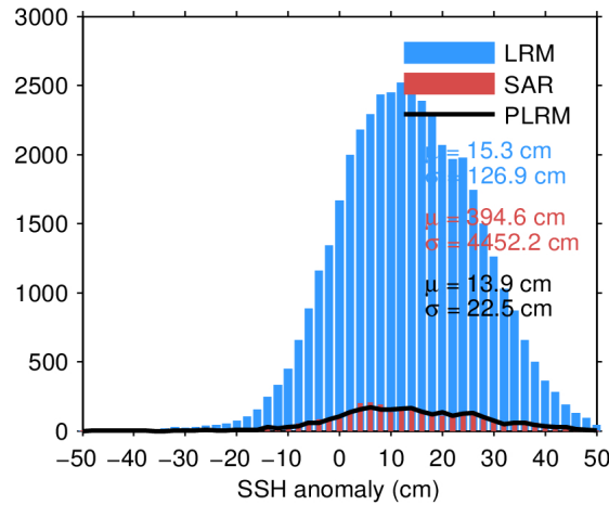
Figure 7. Histogram of flag-valid SSH anomaly over oceans and lakes for LRM (blue), SAR (red), and PLRM (black) for 19/04/2024. The mean ( \mu ) and standard deviation ( \sigma ) are also shown. Note that values outside [-50\ 50] cm are excluded from the histogram for the sake of readability but not from the computation of \mu and \sigma .
