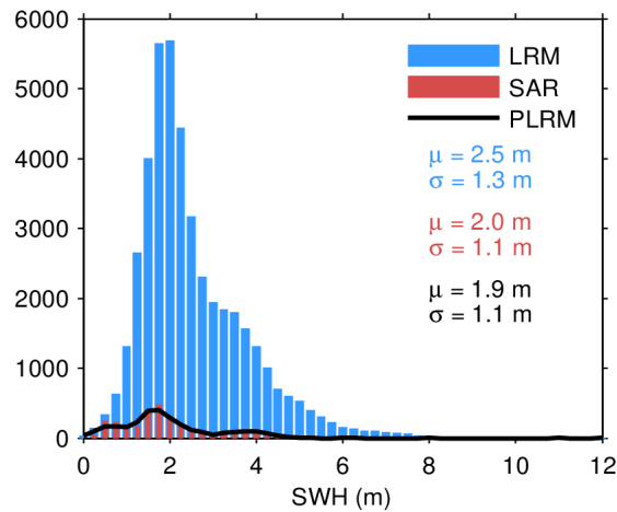
Figure 17. Histogram of flag-valid SWH over oceans and lakes for LRM (blue), SAR (red), and PLRM (black) for 19/04/2024. The mean ( \mu ) and standard deviation ( \sigma ) are also shown. Note that values larger than 12 m are excluded from the histogram for the sake of readability but not from the computation of \mu and \sigma .
