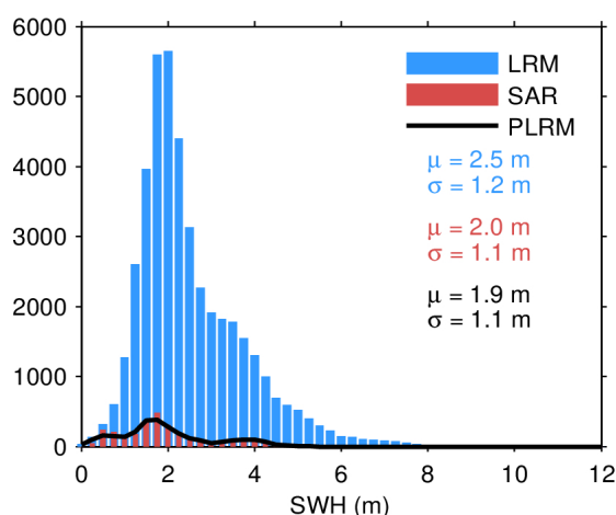
Figure 20. Histogram of science-valid SWH over oceans and lakes for LRM (blue), SAR (red), and PLRM (black) for 19/04/2024. The mean ( \mu ) and standard deviation ( \sigma ) are also
