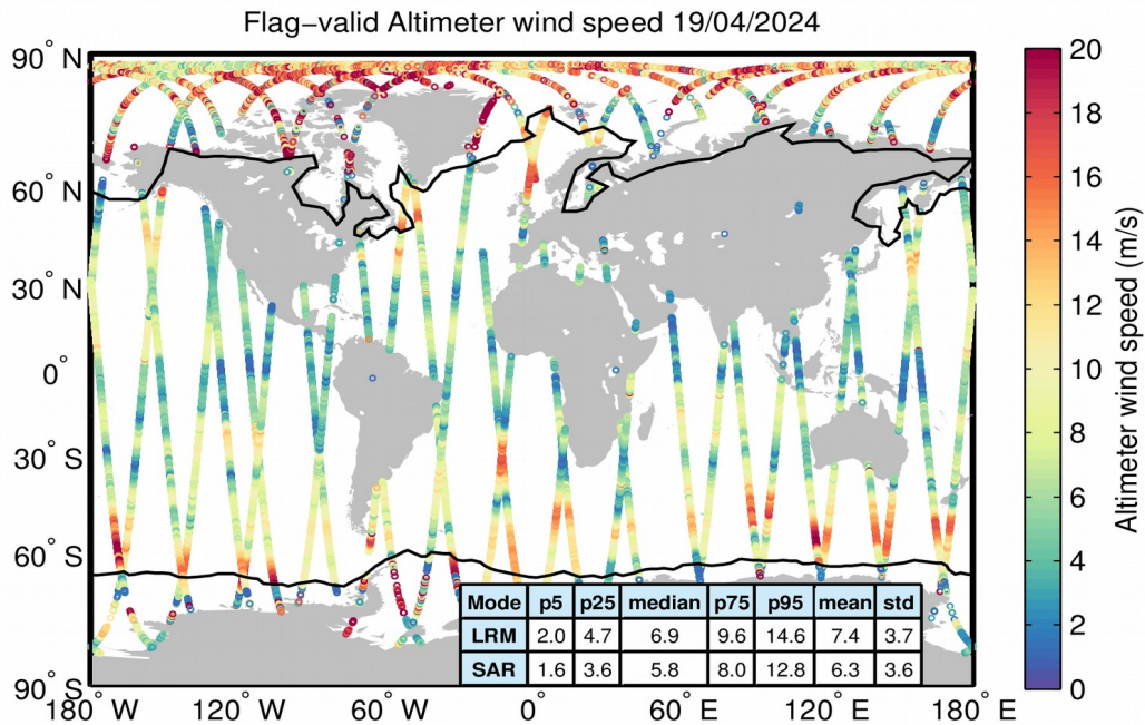
Figure 31. Geographical distribution of flag-valid wind data over oceans and lakes for 19/04/2024. The statistical values shown in the table refer to the wind in m/s and are calculated separately for LRM and SAR regions. Measurements taken over polar polygons have been excluded from the computation of the statistical values. The black lines mark the outer limit of the Arctic and Antarctic polar polygons.
