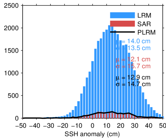
Figure 11. Histogram of science-valid SSH anomaly over oceans and lakes for LRM (blue), SAR (red), and PLRM (black) for 19/04/2024. The mean ( \mu ) and standard deviation ( \sigma ) are also shown. Note that values outside [-50\ 50] cm are excluded from the histogram for the sake of readability but not from the computation of \mu and \sigma .
