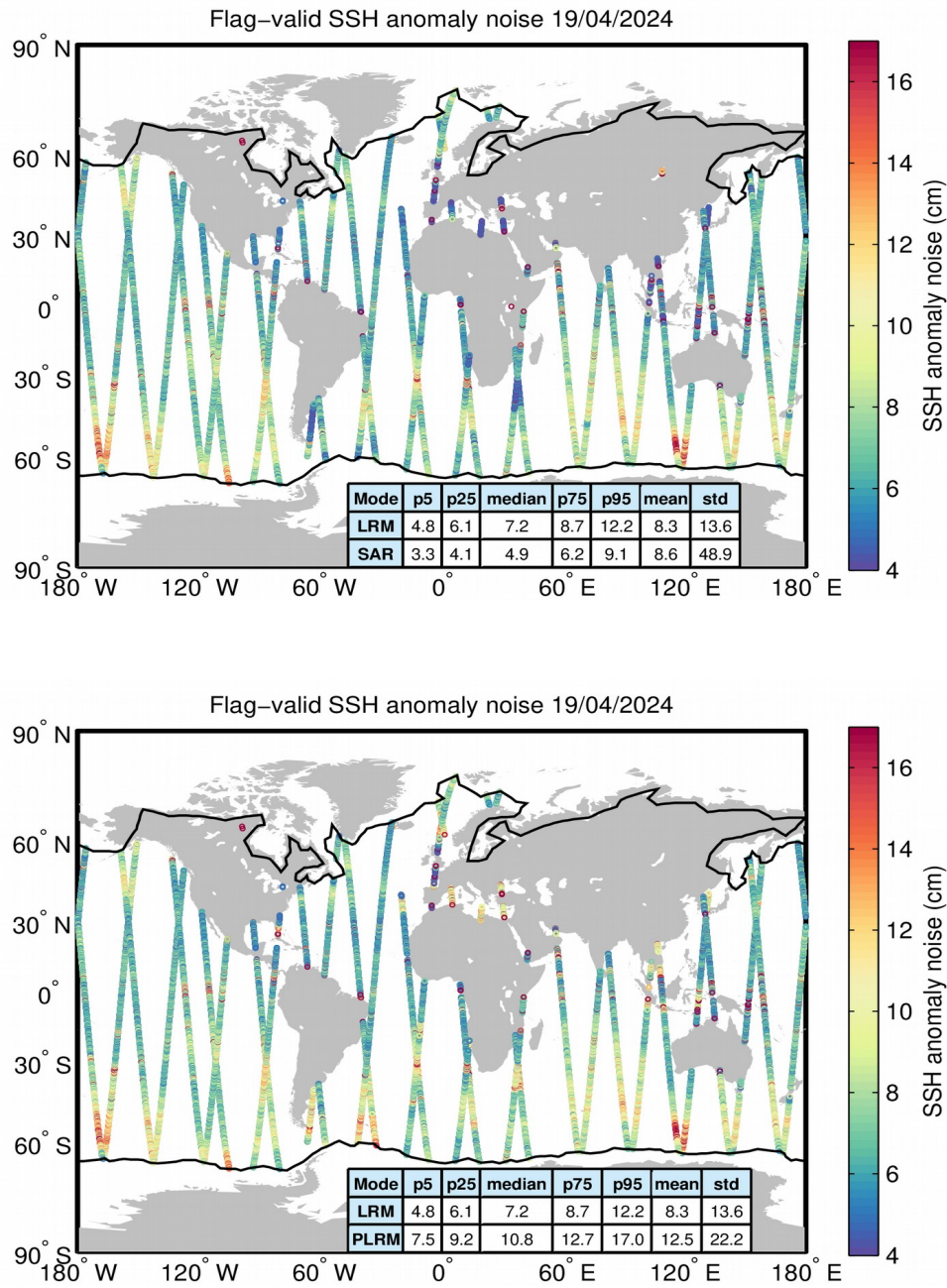
Figure 8. Geographical distribution of flag-valid 20-Hz SSH anomaly measurement noise over oceans and lakes for LRM/SAR (top) and LRM/PLRM (bottom) and for 19/04/2024. The statistical values shown in the tables refer to the SSH anomaly noise and are calculated separately for LRM and SAR/PLRM regions. Measurements taken over polar polygons have been excluded from the computation of the statistical values. The black lines mark the outer limit of the Arctic and Antarctic polar polygons.
