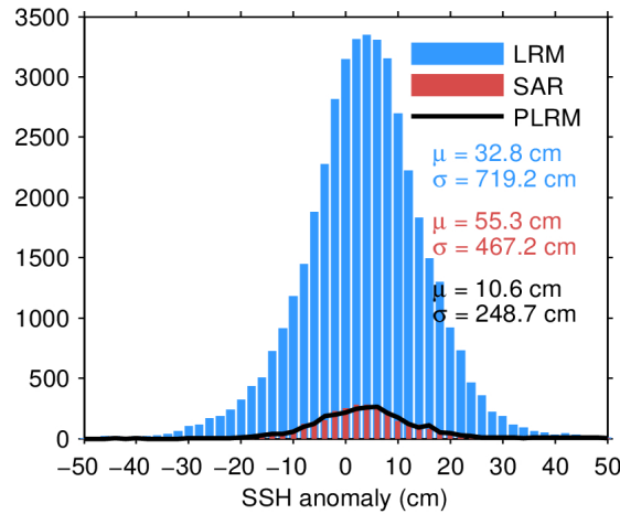
Figure 7. Histogram of flag-valid SSH anomaly over oceans and lakes for LRM (blue), SAR (red), and PLRM (black) for 18/04/2024. The mean ( \mu ) and standard deviation ( \sigma ) are also shown. Note that values outside [-50 50] cm are excluded from the histogram for the sake of readability but not from the computation of \mu and \sigma .
