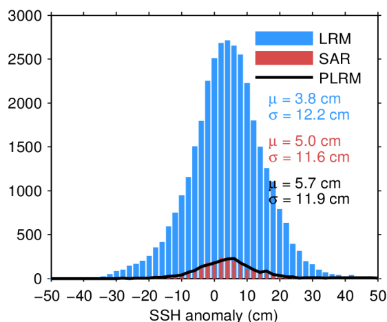
Figure 11. Histogram of science-valid SSH anomaly over oceans and lakes for LRM (blue), SAR (red), and PLRM (black) for 18/04/2024. The mean ( \mu ) and standard deviation ( \sigma ) are also shown. Note that values outside [-50\ 50] cm are excluded from the histogram for the sake of readability but not from the computation of \mu and \sigma .
