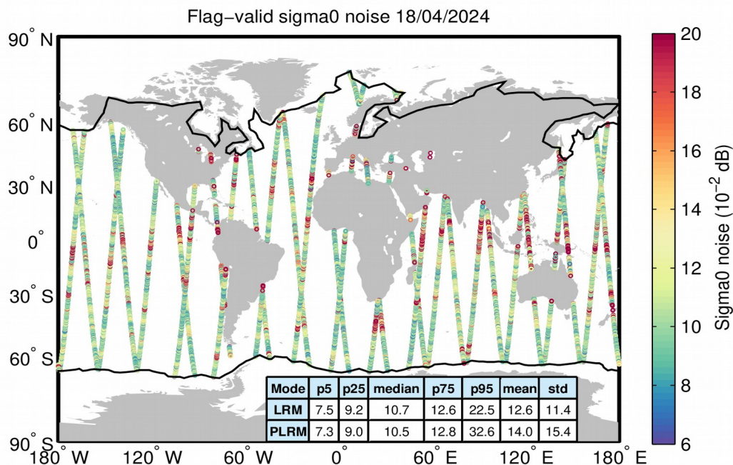
Figure 26. Geographical distribution of flag-valid 20-Hz sigma0 measurement noise over oceans and lakes for LRM/SAR (top) and LRM/PLRM (bottom) and for 18/04/2024. The statistical values shown in the table refer to the sigma0 noise and are calculated separately for LRM and SAR/PLRM regions. Measurements taken over polar polygons have been excluded from the computation of the statistical values. The black lines mark the outer limit of the Arctic and Antarctic polar polygons.
