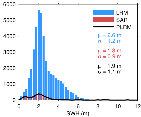
Figure 17. Histogram of flag-valid SWH over oceans and lakes for LRM (blue), SAR (red), and PLRM (black) for 18/04/2024. The mean ( \mu ) and standard deviation ( \sigma ) are also shown. Note that values larger than 12 m are excluded from the histogram for the sake of readability but not from the computation of \mu and \sigma .
