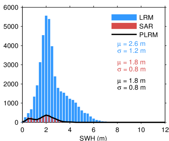
Figure 20. Histogram of science-valid SWH over oceans and lakes for LRM (blue), SAR (red), and PLRM (black) for 18/04/2024. The mean ( \mu ) and standard deviation ( \sigma ) are also
