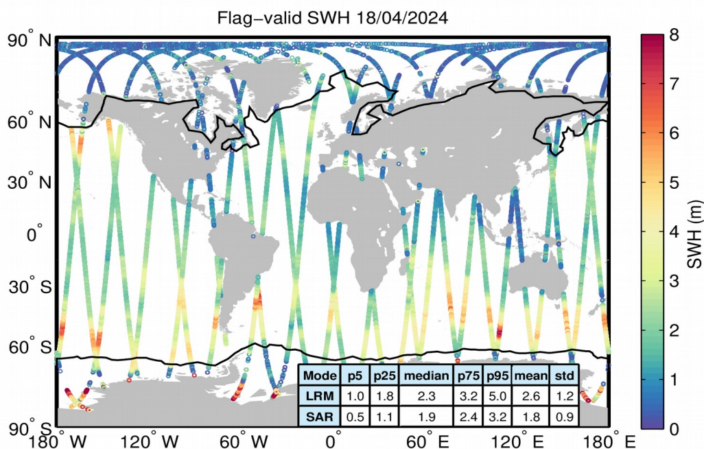
Figure 15. Geographical distribution of flag-valid SWH data over oceans and lakes for 18/04/2024. The statistical values shown in the table refer to the SWH in m and are calculated separately for LRM and SAR regions. Measurements taken over polar polygons have been excluded from the computation of the statistical values. The black lines mark the outer limit of the Arctic and Antarctic polar polygons.
