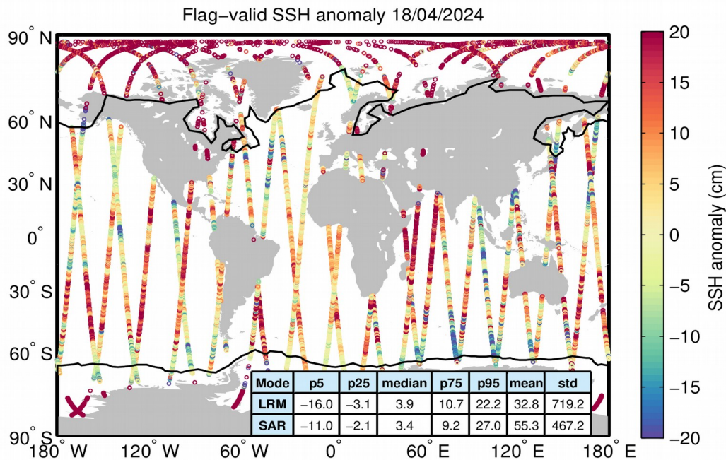
Figure 5. Geographical distribution of flag-valid 1-Hz SSH anomaly data over oceans and lakes for 18/04/2024. The statistical values shown in the table refer to the SSH anomaly in cm and are calculated separately for LRM and SAR regions. Measurements taken over polar polygons have been excluded from the computation of the statistical values. The black lines mark the outer limit of the Arctic and Antarctic polar polygons.
