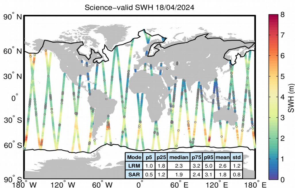
Figure 19. Geographical distribution of science-valid SWH data over oceans and lakes for 18/04/2024. The statistical values shown in the table refer to the SWH in m and are calculated separately for LRM and SAR regions. The black lines mark the outer limit of the Arctic and Antarctic polar polygons. Gray circles denote records that have been rejected based on the editing criteria described in Table 3.
