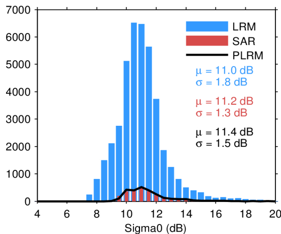
Figure 28. Histogram of science-valid sigma0 over oceans and lakes for LRM (blue), SAR (red), and PLRM (black) for 18/04/2024. The mean ( \mu ) and standard deviation ( \sigma ) are also shown. Note that values outside [4 20] dB are excluded from the histogram for the sake of readability but not from the computation of \mu and \sigma .
