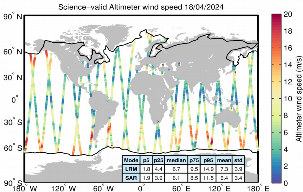
Figure 34. Geographical distribution of science-valid wind data over oceans and lakes for 18/04/2024. The statistical values shown in the table refer to the wind in m/s and are calculated separately for LRM and SAR regions. The black lines mark the outer limit of the Arctic and Antarctic polar polygons. Gray circles denote records that have been rejected based on the editing criteria described in Table 5.
