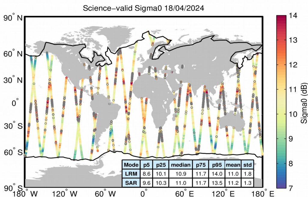
Figure 27. Geographical distribution of science-valid sigma0 data over oceans and lakes for 18/04/2024. The statistical values shown in the table refer to the sigma0 in dB and are calculated separately for LRM and SAR regions. The black lines mark the outer limit of the Arctic and Antarctic polar polygons. Gray circles denote records that have been rejected based on the editing criteria described in Table 4.
