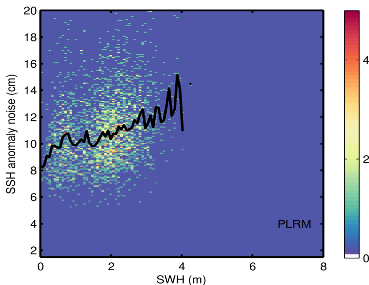
Figure 9. 2D histogram showing flag-valid SSH anomaly noise as a function of SWH for LRM (top), SAR (middle), and PLRM (bottom) for 18/04/2024. The black line denotes the median SSH anomaly noise as a function of SWH.
