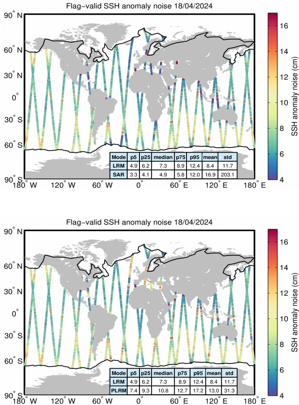
Figure 8. Geographical distribution of flag-valid 20-Hz SSH anomaly measurement noise over oceans and lakes for LRM/SAR (top) and LRM/PLRM (bottom) and for 18/04/2024. The statistical values shown in the tables refer to the SSH anomaly noise and are calculated separately for LRM and SAR/PLRM regions. Measurements taken over polar polygons have been excluded from the computation of the statistical values. The black lines mark the outer limit of the Arctic and Antarctic polar polygons.
