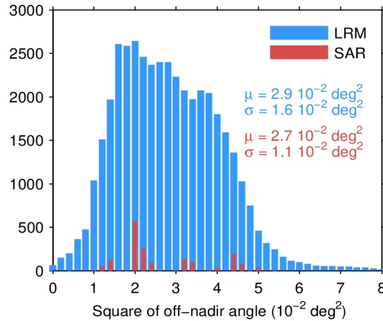
Figure 39. Histogram of flag-valid mispointing over oceans and lakes for LRM (blue) and SAR (red) for 18/04/2024. Only positive values have been considered. The mean ( \mu ) and standard deviation ( \sigma ) are also shown. Note that values larger than 8 \times 10^{-2} \text{ deg}^2 are excluded from the histogram for the sake of readability but not from the computation of \mu and \sigma .
