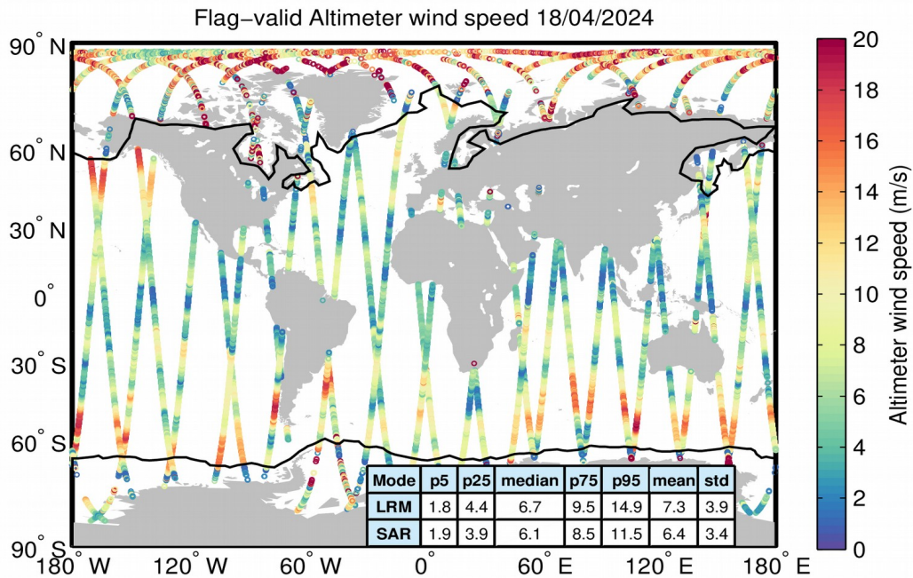
Figure 31. Geographical distribution of flag-valid wind data over oceans and lakes for 18/04/2024. The statistical values shown in the table refer to the wind in m/s and are calculated separately for LRM and SAR regions. Measurements taken over polar polygons have been excluded from the computation of the statistical values. The black lines mark the outer limit of the Arctic and Antarctic polar polygons.
