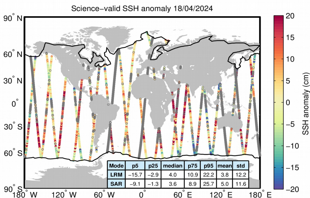
Figure 10. Geographical distribution of science-valid SSH anomaly data over oceans and lakes for 18/04/2024. The statistical values shown in the table refer to the SSH anomaly in cm and are calculated separately for LRM and SAR regions. The black lines mark the
