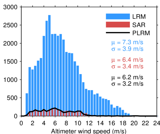
Figure 33. Histogram of flag-valid wind over oceans and lakes for LRM (blue), SAR (red), and PLRM (black) for 18/04/2024. The mean ( \mu ) and standard deviation ( \sigma ) are also shown. Note that values larger than 24 m/s are excluded from the histogram for the sake of readability but not from the computation of \mu and \sigma .
