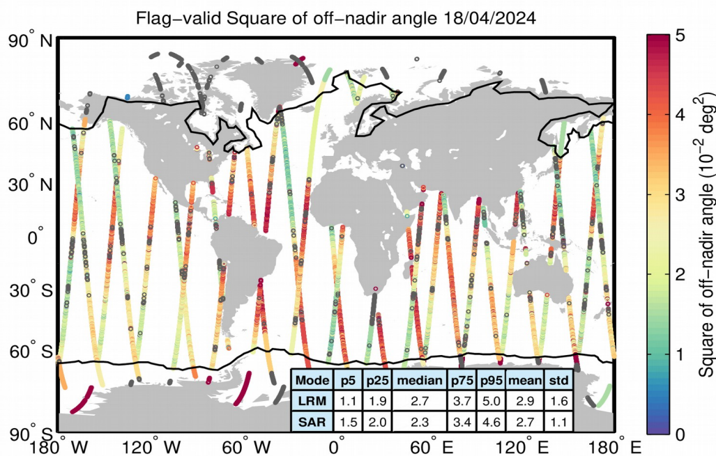
Figure 37. Geographical distribution of flag-valid mispointing data over oceans and lakes for 18/04/2024. The statistical values shown in the table refer to the mispointing in 10^{-2} \text{ deg}^2 and are calculated separately for LRM and SAR regions. Measurements taken over polar polygons have been excluded from the computation of the statistical values. The black lines mark the outer limit of the Arctic and Antarctic polar polygons. Gray circles denote negative values.
