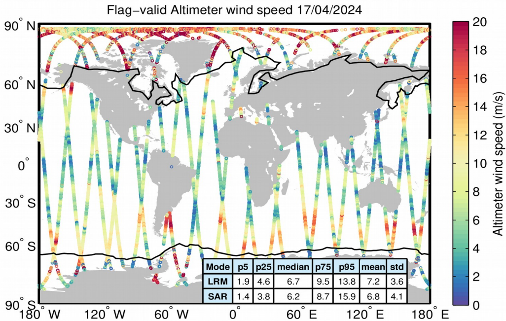
Figure 31. Geographical distribution of flag-valid wind data over oceans and lakes for 17/04/2024. The statistical values shown in the table refer to the wind in m/s and are calculated separately for LRM and SAR regions. Measurements taken over polar polygons have been excluded from the computation of the statistical values. The black lines mark the outer limit of the Arctic and Antarctic polar polygons.
