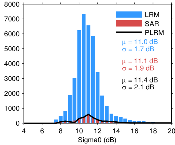
Figure 28. Histogram of science-valid sigma0 over oceans and lakes for LRM (blue), SAR (red), and PLRM (black) for 17/04/2024. The mean ( \mu ) and standard deviation ( \sigma ) are also shown. Note that values outside [4 20] dB are excluded from the histogram for the sake of readability but not from the computation of \mu and \sigma .
