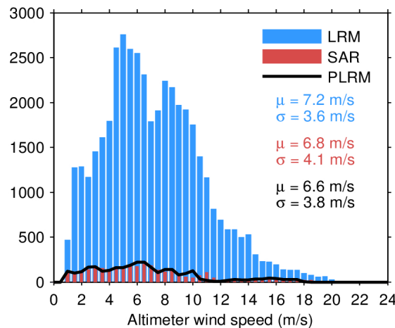
Figure 33. Histogram of flag-valid wind over oceans and lakes for LRM (blue), SAR (red), and PLRM (black) for 17/04/2024. The mean ( \mu ) and standard deviation ( \sigma ) are also shown. Note that values larger than 24 m/s are excluded from the histogram for the sake of readability but not from the computation of \mu and \sigma .
