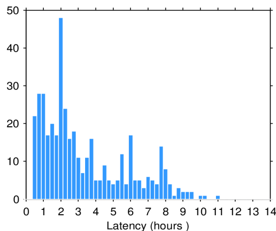
Figure 2. Histogram of the data latency for 17/04/2024. The y-axis denotes the number of files that are made available with a delay of x-hours with respect to the mean time of the records stored in the file.
