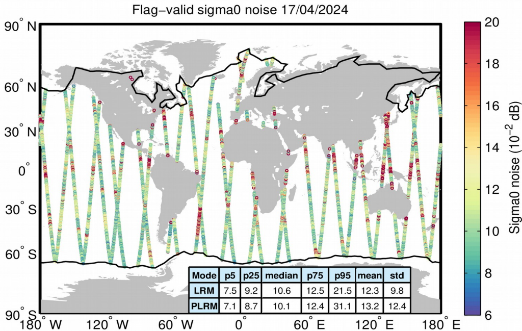
Figure 26. Geographical distribution of flag-valid 20-Hz sigma0 measurement noise over oceans and lakes for LRM/SAR (top) and LRM/PLRM (bottom) and for 17/04/2024. The statistical values shown in the table refer to the sigma0 noise and are calculated separately for LRM and SAR/PLRM regions. Measurements taken over polar polygons have been excluded from the computation of the statistical values. The black lines mark the outer limit of the Arctic and Antarctic polar polygons.
