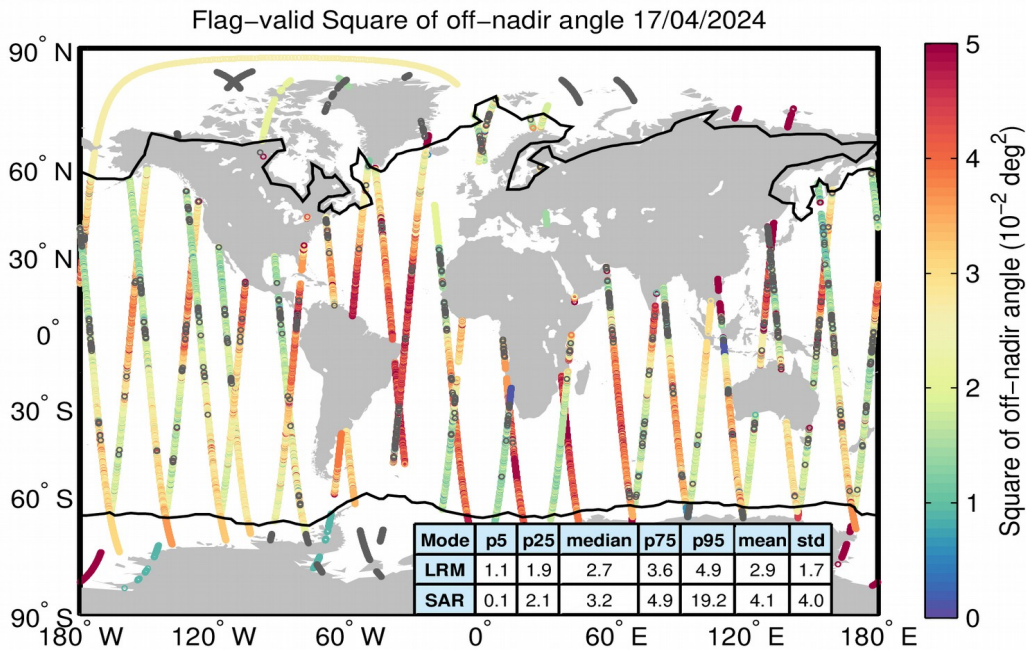
Figure 37. Geographical distribution of flag-valid mispointing data over oceans and lakes for 17/04/2024. The statistical values shown in the table refer to the mispointing in 10^{-2} \text{ deg}^2 and are calculated separately for LRM and SAR regions. Measurements taken over polar polygons have been excluded from the computation of the statistical values. The black lines mark the outer limit of the Arctic and Antarctic polar polygons. Gray circles denote negative values.
