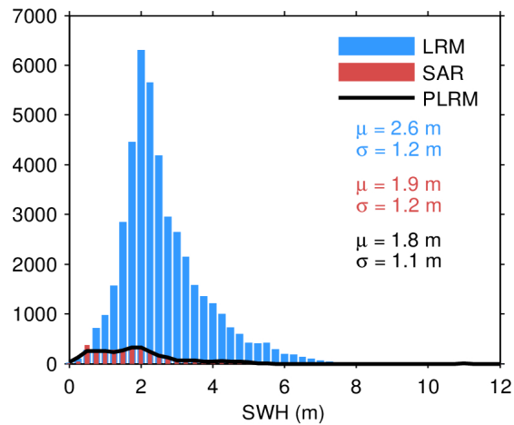
Figure 17. Histogram of flag-valid SWH over oceans and lakes for LRM (blue), SAR (red), and PLRM (black) for 17/04/2024. The mean ( \mu ) and standard deviation ( \sigma ) are also shown. Note that values larger than 12 m are excluded from the histogram for the sake of readability but not from the computation of \mu and \sigma .
