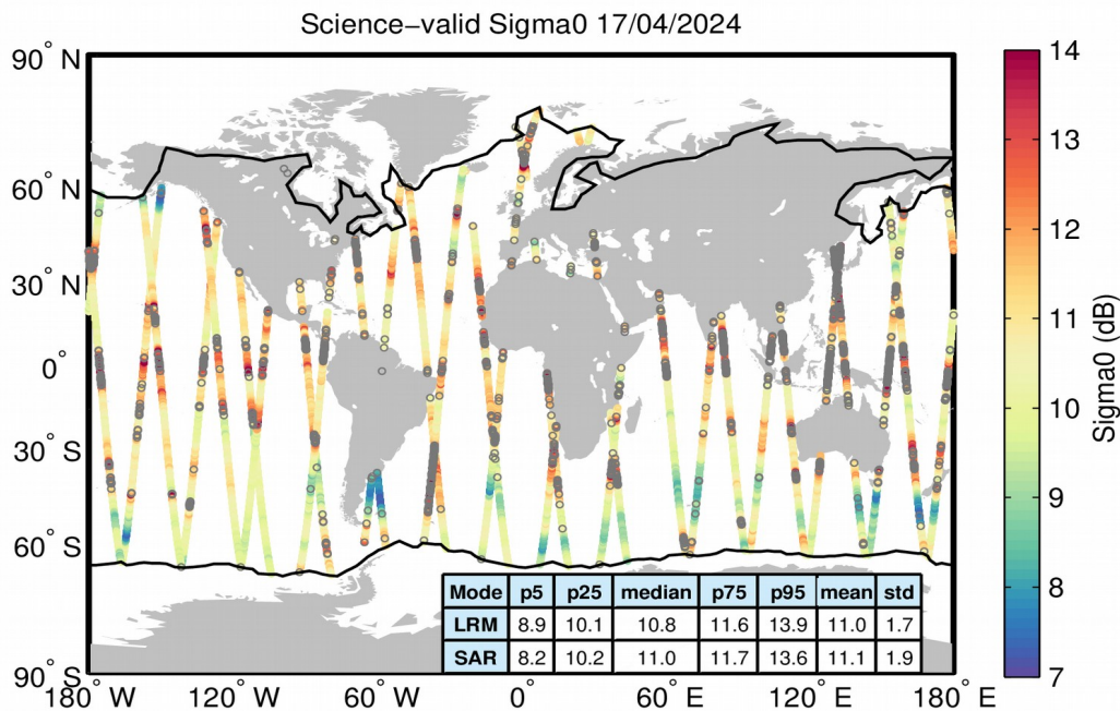
Figure 27. Geographical distribution of science-valid sigma0 data over oceans and lakes for 17/04/2024. The statistical values shown in the table refer to the sigma0 in dB and are calculated separately for LRM and SAR regions. The black lines mark the outer limit of the Arctic and Antarctic polar polygons. Gray circles denote records that have been rejected based on the editing criteria described in Table 4.
