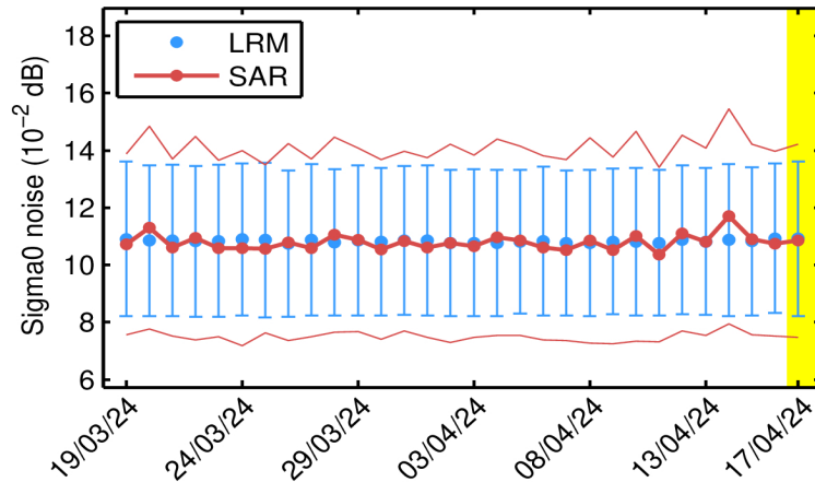
Figure 30. Average science-valid sigma0 noise for LRM (blue dot) and SAR (red dot). The corresponding standard deviation (blue error bar and thin red lines, respectively) for each day in last 30-day window is also shown. The yellow shading highlights the day analyzed in this report.
