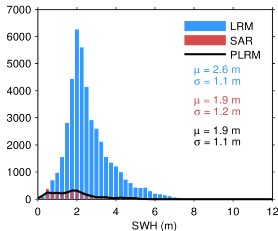
Figure 20. Histogram of science-valid SWH over oceans and lakes for LRM (blue), SAR (red), and PLRM (black) for 17/04/2024. The mean ( \mu ) and standard deviation ( \sigma ) are also
