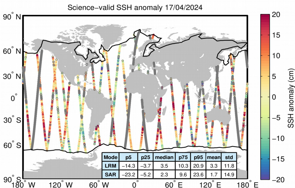
Figure 10. Geographical distribution of science-valid SSH anomaly data over oceans and lakes for 17/04/2024. The statistical values shown in the table refer to the SSH anomaly in cm and are calculated separately for LRM and SAR regions. The black lines mark the
