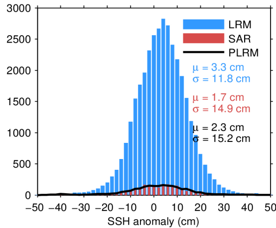
Figure 11. Histogram of science-valid SSH anomaly over oceans and lakes for LRM (blue), SAR (red), and PLRM (black) for 17/04/2024. The mean ( \mu ) and standard deviation ( \sigma ) are also shown. Note that values outside [-50\ 50] cm are excluded from the histogram for the sake of readability but not from the computation of \mu and \sigma .
