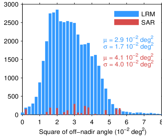
Figure 39. Histogram of flag-valid mispointing over oceans and lakes for LRM (blue) and SAR (red) for 17/04/2024. Only positive values have been considered. The mean ( \mu ) and standard deviation ( \sigma ) are also shown. Note that values larger than 8 \cdot 10^{-2} \text{ deg}^2 are excluded from the histogram for the sake of readability but not from the computation of \mu and \sigma .
