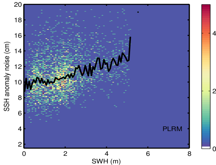
Figure 9. 2D histogram showing flag-valid SSH anomaly noise as a function of SWH for LRM (top), SAR (middle), and PLRM (bottom) for 17/04/2024. The black line denotes the median SSH anomaly noise as a function of SWH.
