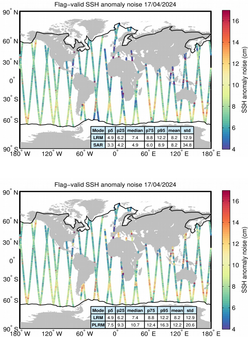
Figure 8. Geographical distribution of flag-valid 20-Hz SSH anomaly measurement noise over oceans and lakes for LRM/SAR (top) and LRM/PLRM (bottom) and for 17/04/2024. The statistical values shown in the tables refer to the SSH anomaly noise and are calculated separately for LRM and SAR/PLRM regions. Measurements taken over polar polygons have been excluded from the computation of the statistical values. The black lines mark the outer limit of the Arctic and Antarctic polar polygons.
