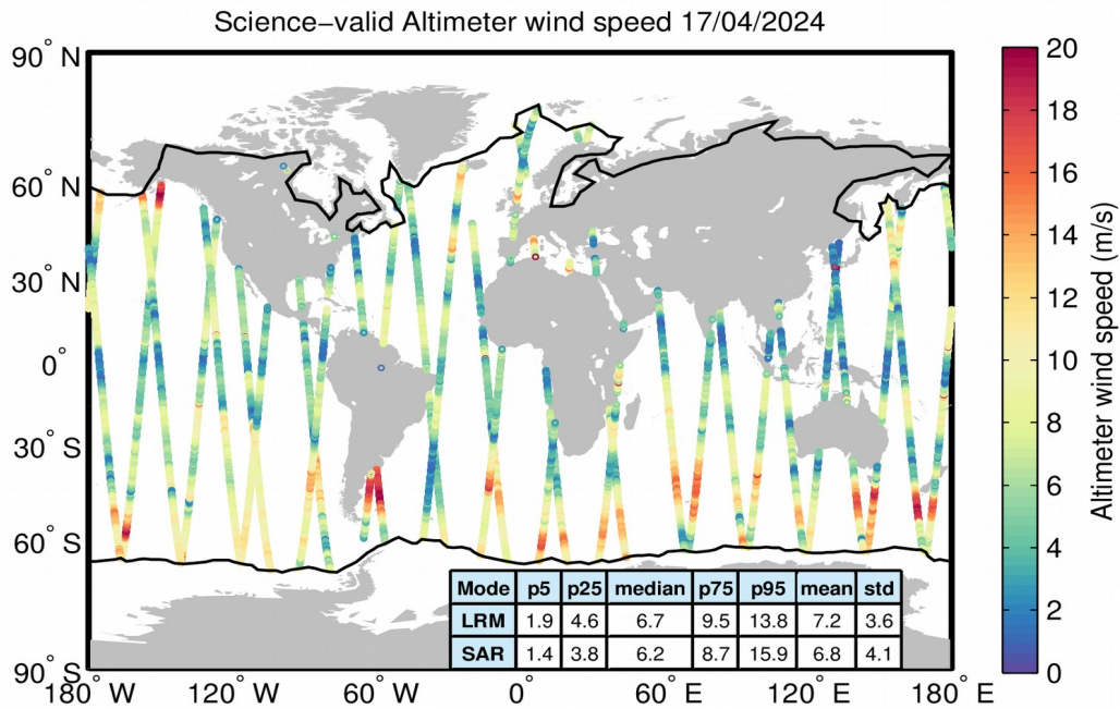
Figure 34. Geographical distribution of science-valid wind data over oceans and lakes for 17/04/2024. The statistical values shown in the table refer to the wind in m/s and are calculated separately for LRM and SAR regions. The black lines mark the outer limit of the Arctic and Antarctic polar polygons. Gray circles denote records that have been rejected based on the editing criteria described in Table 5.
