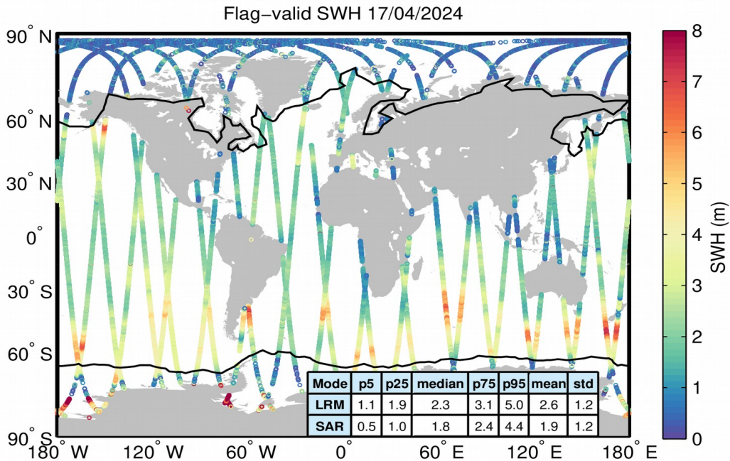
Figure 15. Geographical distribution of flag-valid SWH data over oceans and lakes for 17/04/2024. The statistical values shown in the table refer to the SWH in m and are calculated separately for LRM and SAR regions. Measurements taken over polar polygons have been excluded from the computation of the statistical values. The black lines mark the outer limit of the Arctic and Antarctic polar polygons.
