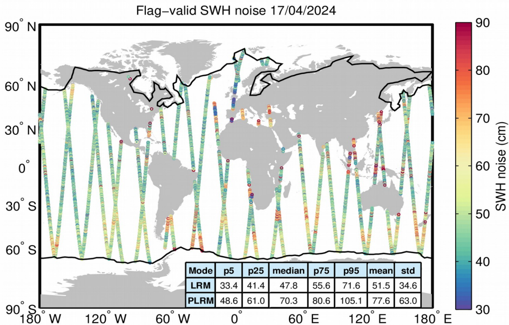
Figure 18. Geographical distribution of flag-valid 20-Hz SWH measurement noise over oceans and lakes for LRM/SAR (top) and LRM/PLRM (bottom) and for 17/04/2024. The statistical values shown in the table refer to the SWH noise and are calculated separately for LRM and SAR/PLRM regions. Measurements taken over polar polygons have been
