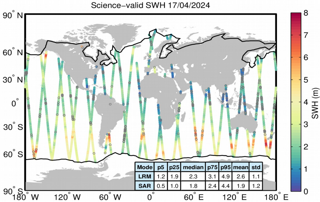
Figure 19. Geographical distribution of science-valid SWH data over oceans and lakes for 17/04/2024. The statistical values shown in the table refer to the SWH in m and are calculated separately for LRM and SAR regions. The black lines mark the outer limit of the Arctic and Antarctic polar polygons. Gray circles denote records that have been rejected based on the editing criteria described in Table 3.
