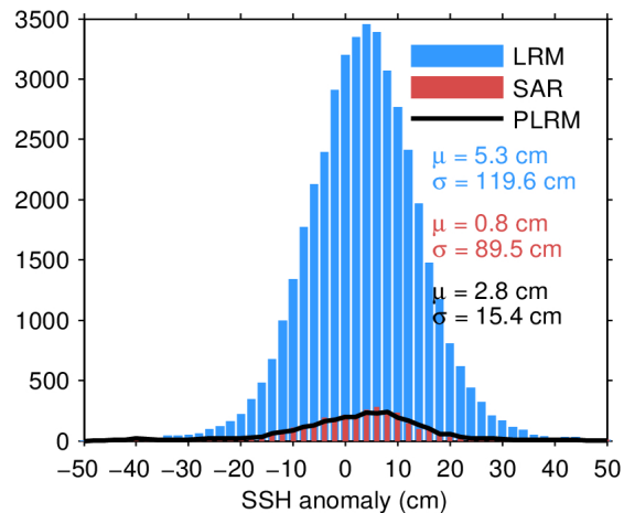
Figure 7. Histogram of flag-valid SSH anomaly over oceans and lakes for LRM (blue), SAR (red), and PLRM (black) for 17/04/2024. The mean ( \mu ) and standard deviation ( \sigma ) are also shown. Note that values outside [-50 50] cm are excluded from the histogram for the sake of readability but not from the computation of \mu and \sigma .
