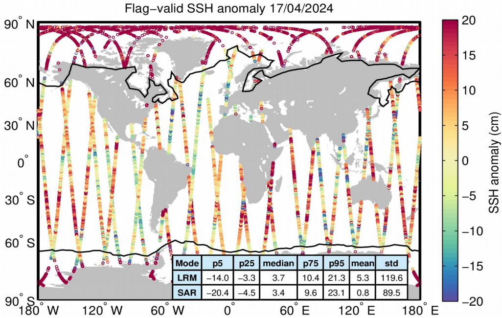
Figure 5. Geographical distribution of flag-valid 1-Hz SSH anomaly data over oceans and lakes for 17/04/2024. The statistical values shown in the table refer to the SSH anomaly in cm and are calculated separately for LRM and SAR regions. Measurements taken over polar polygons have been excluded from the computation of the statistical values. The black lines mark the outer limit of the Arctic and Antarctic polar polygons.
