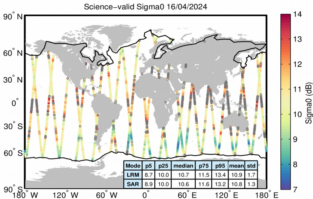
Figure 27. Geographical distribution of science-valid sigma0 data over oceans and lakes for 16/04/2024. The statistical values shown in the table refer to the sigma0 in dB and are calculated separately for LRM and SAR regions. The black lines mark the outer limit of the Arctic and Antarctic polar polygons. Gray circles denote records that have been rejected based on the editing criteria described in Table 4.
