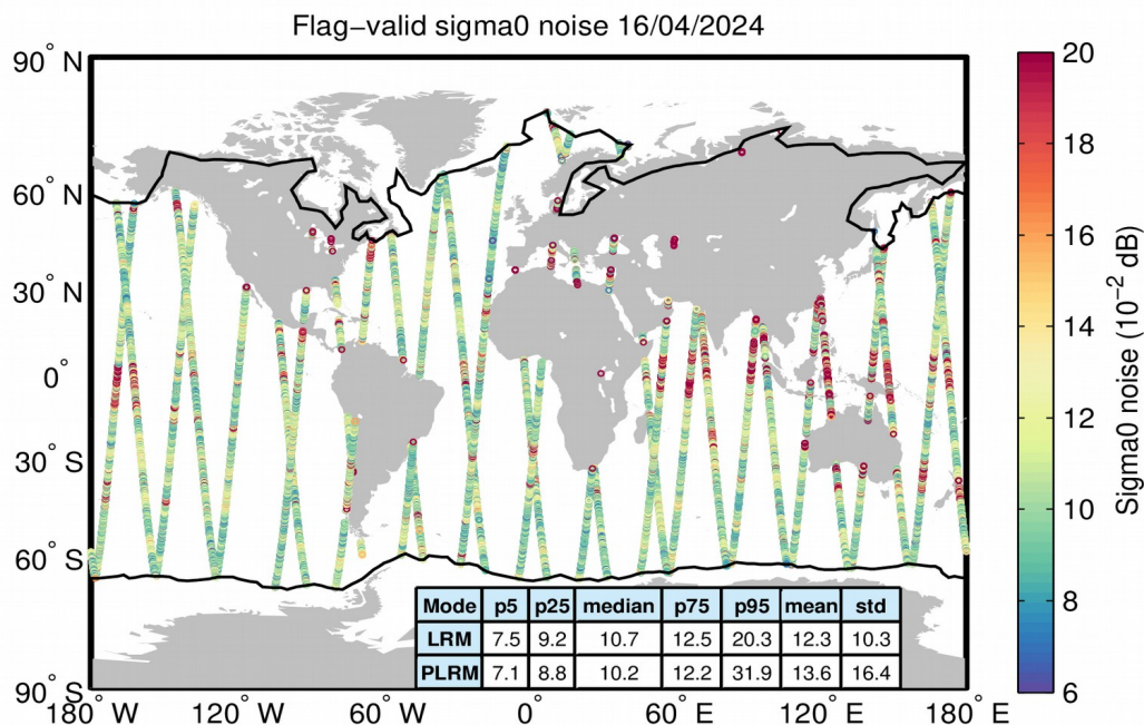
Figure 26. Geographical distribution of flag-valid 20-Hz sigma0 measurement noise over oceans and lakes for LRM/SAR (top) and LRM/PLRM (bottom) and for 16/04/2024. The statistical values shown in the table refer to the sigma0 noise and are calculated separately for LRM and SAR/PLRM regions. Measurements taken over polar polygons have been excluded from the computation of the statistical values. The black lines mark the outer limit of the Arctic and Antarctic polar polygons.
