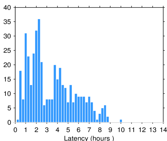
Figure 2. Histogram of the data latency for 16/04/2024. The y-axis denotes the number of files that are made available with a delay of x-hours with respect to the mean time of the records stored in the file.
