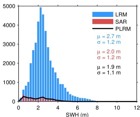
Figure 20. Histogram of science-valid SWH over oceans and lakes for LRM (blue), SAR (red), and PLRM (black) for 16/04/2024. The mean ( \mu ) and standard deviation ( \sigma ) are also
