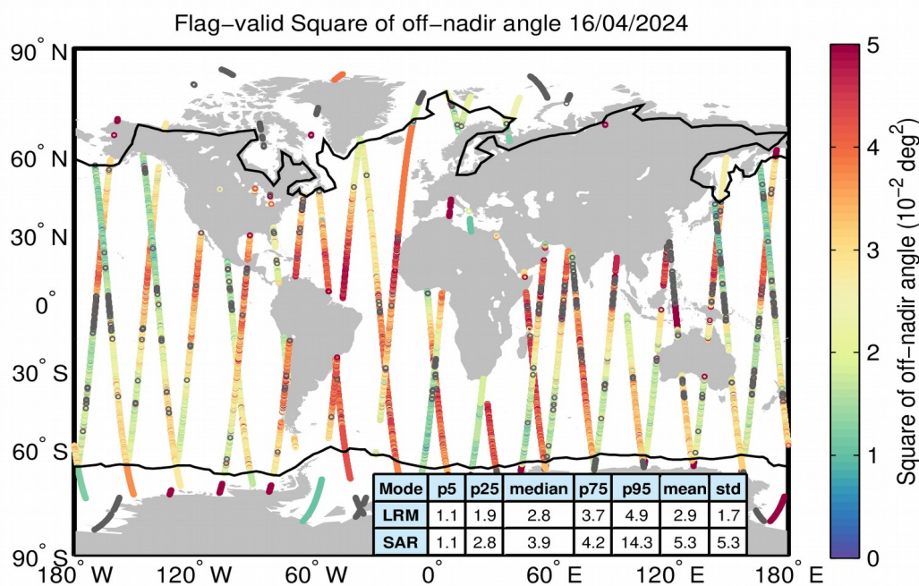
Figure 37. Geographical distribution of flag-valid mispointing data over oceans and lakes for 16/04/2024. The statistical values shown in the table refer to the mispointing in 10^{-2} \text{ deg}^2 and are calculated separately for LRM and SAR regions. Measurements taken over polar polygons have been excluded from the computation of the statistical values. The black lines mark the outer limit of the Arctic and Antarctic polar polygons. Gray circles denote negative values.
