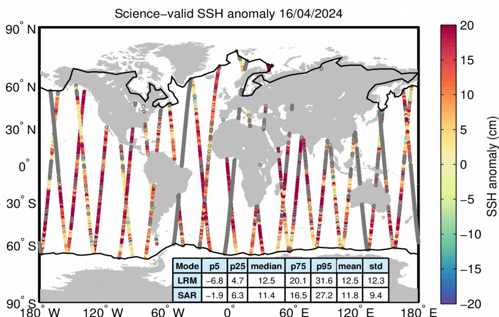
Figure 10. Geographical distribution of science-valid SSH anomaly data over oceans and lakes for 16/04/2024. The statistical values shown in the table refer to the SSH anomaly in cm and are calculated separately for LRM and SAR regions. The black lines mark the
