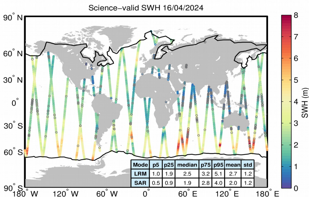
Figure 19. Geographical distribution of science-valid SWH data over oceans and lakes for 16/04/2024. The statistical values shown in the table refer to the SWH in m and are calculated separately for LRM and SAR regions. The black lines mark the outer limit of the Arctic and Antarctic polar polygons. Gray circles denote records that have been rejected based on the editing criteria described in Table 3.
