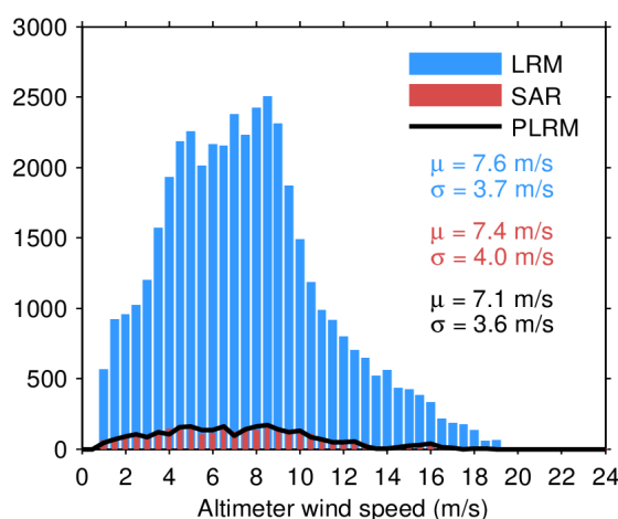
Figure 33. Histogram of flag-valid wind over oceans and lakes for LRM (blue), SAR (red), and PLRM (black) for 16/04/2024. The mean ( \mu ) and standard deviation ( \sigma ) are also shown. Note that values larger than 24 m/s are excluded from the histogram for the sake of readability but not from the computation of \mu and \sigma .
