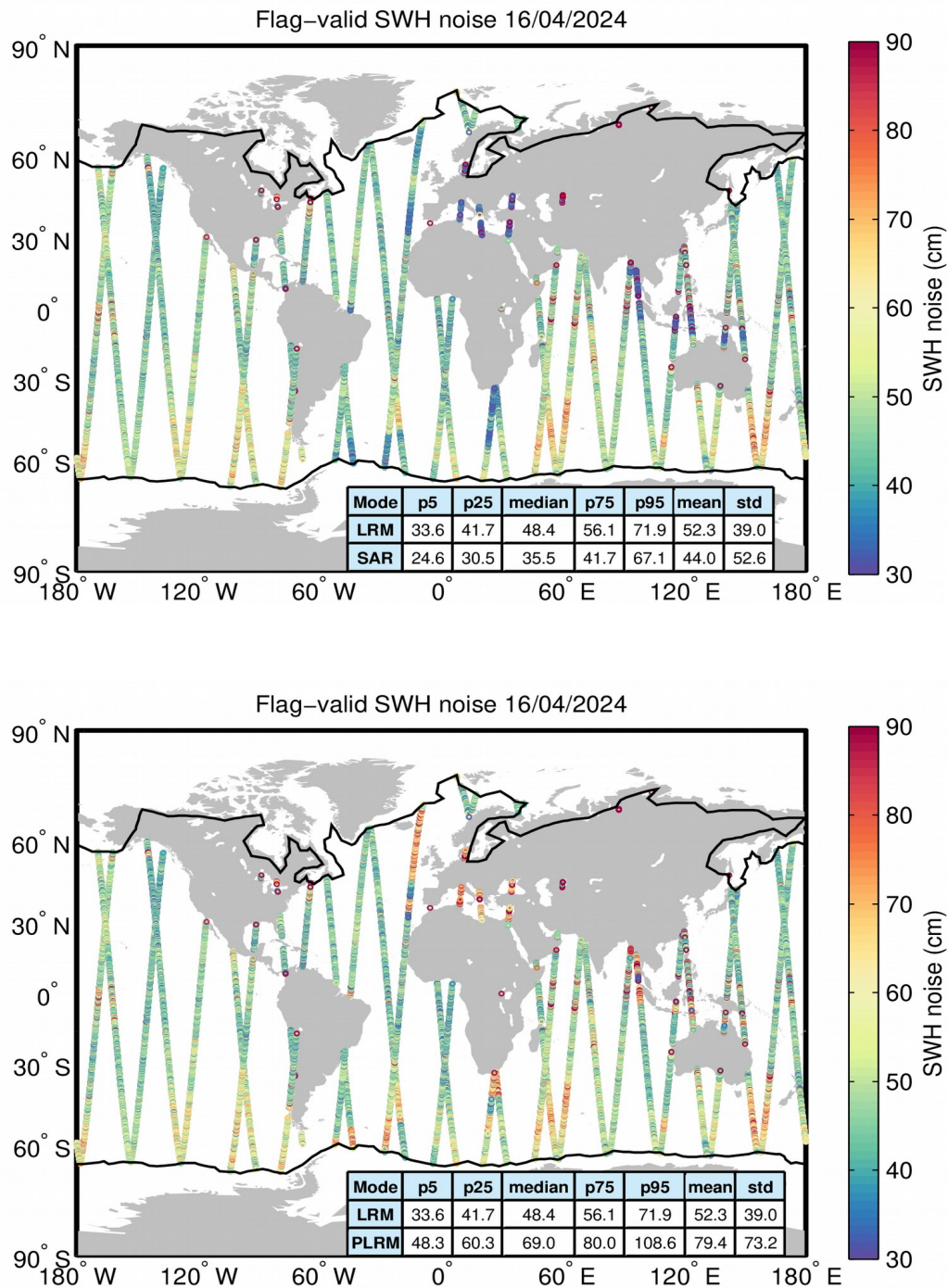
Figure 18. Geographical distribution of flag-valid 20-Hz SWH measurement noise over oceans and lakes for LRM/SAR (top) and LRM/PLRM (bottom) and for 16/04/2024. The statistical values shown in the table refer to the SWH noise and are calculated separately for LRM and SAR/PLRM regions. Measurements taken over polar polygons have been
