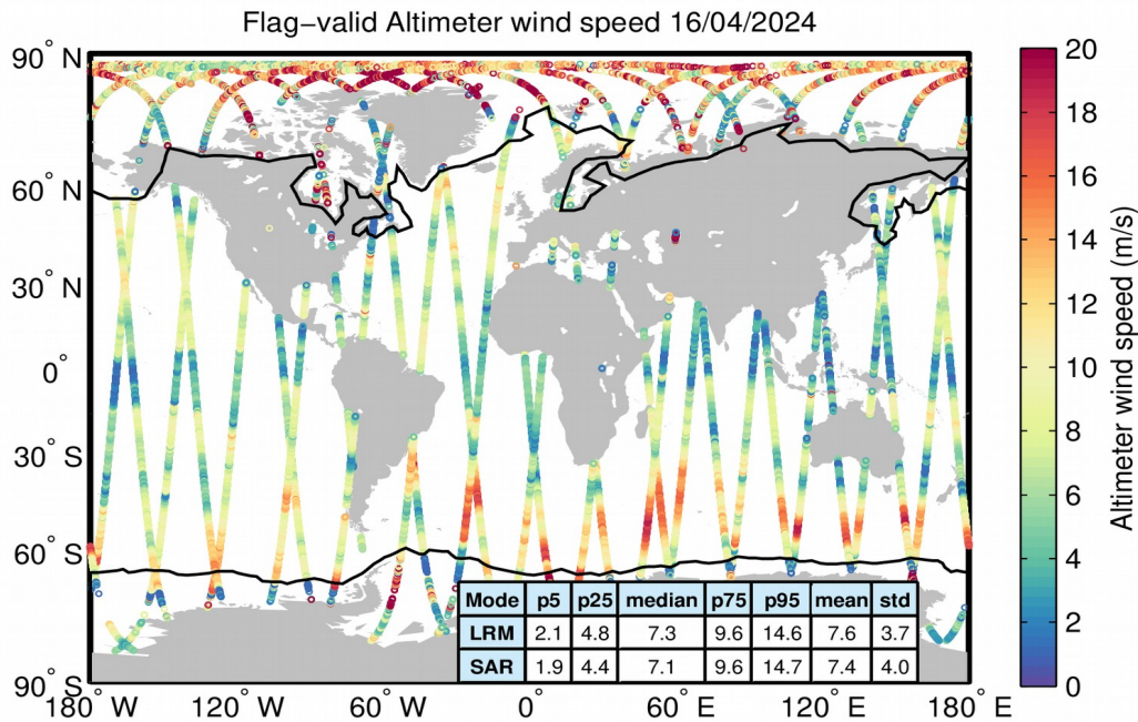
Figure 31. Geographical distribution of flag-valid wind data over oceans and lakes for 16/04/2024. The statistical values shown in the table refer to the wind in m/s and are calculated separately for LRM and SAR regions. Measurements taken over polar polygons have been excluded from the computation of the statistical values. The black lines mark the outer limit of the Arctic and Antarctic polar polygons.
