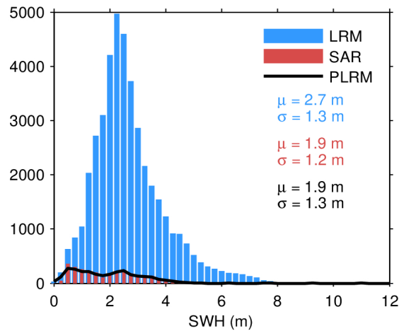
Figure 17. Histogram of flag-valid SWH over oceans and lakes for LRM (blue), SAR (red), and PLRM (black) for 16/04/2024. The mean ( \mu ) and standard deviation ( \sigma ) are also shown. Note that values larger than 12 m are excluded from the histogram for the sake of readability but not from the computation of \mu and \sigma .
