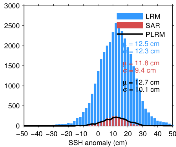
Figure 11. Histogram of science-valid SSH anomaly over oceans and lakes for LRM (blue), SAR (red), and PLRM (black) for 16/04/2024. The mean ( \mu ) and standard deviation ( \sigma ) are also shown. Note that values outside [-50, 50] cm are excluded from the histogram for the sake of readability but not from the computation of \mu and \sigma .
