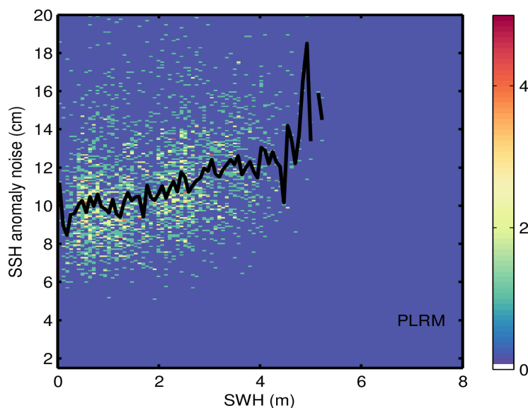
Figure 9. 2D histogram showing flag-valid SSH anomaly noise as a function of SWH for LRM (top), SAR (middle), and PLRM (bottom) for 16/04/2024. The black line denotes the median SSH anomaly noise as a function of SWH.
