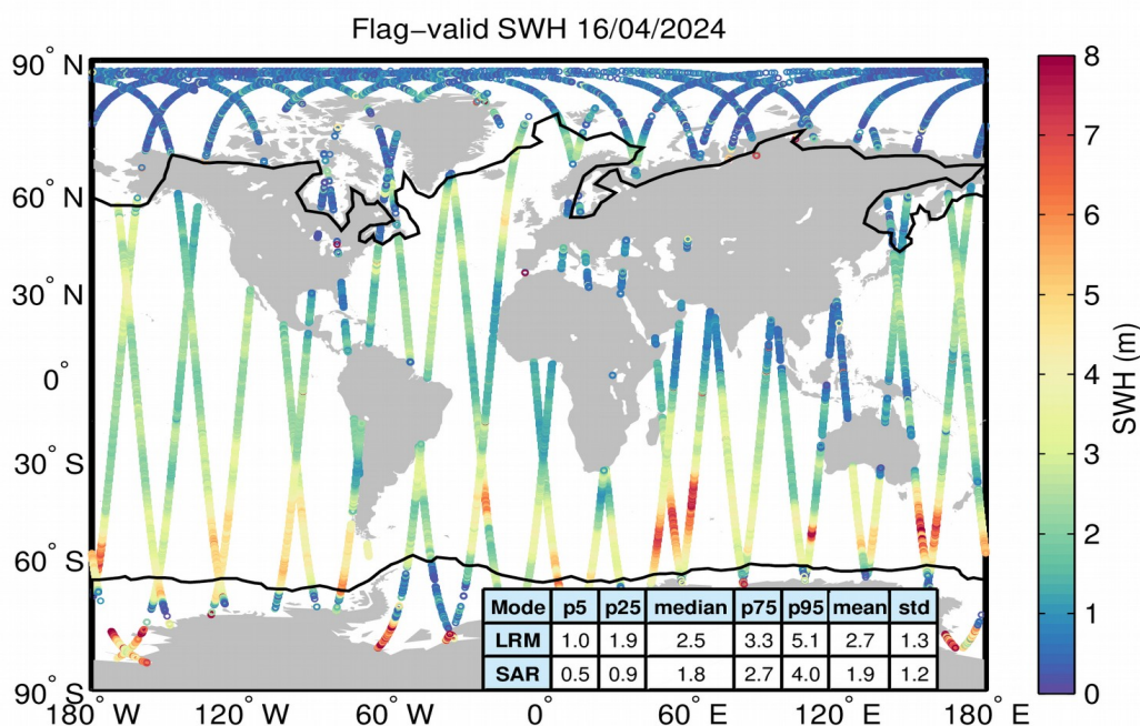
Figure 15. Geographical distribution of flag-valid SWH data over oceans and lakes for 16/04/2024. The statistical values shown in the table refer to the SWH in m and are calculated separately for LRM and SAR regions. Measurements taken over polar polygons have been excluded from the computation of the statistical values. The black lines mark the outer limit of the Arctic and Antarctic polar polygons.
