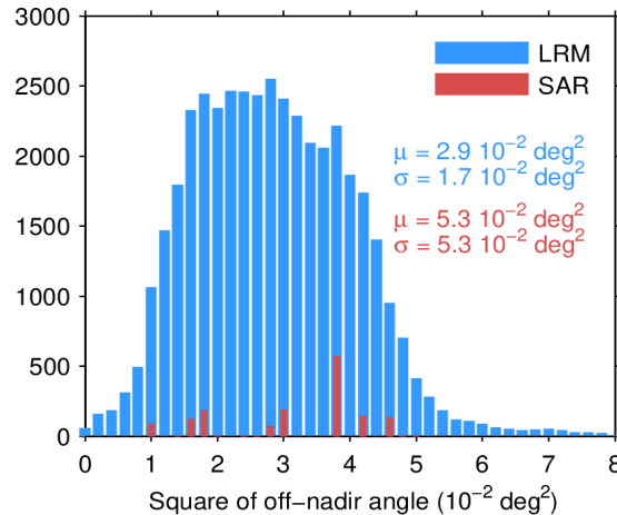
Figure 39. Histogram of flag-valid mispointing over oceans and lakes for LRM (blue) and SAR (red) for 16/04/2024. Only positive values have been considered. The mean ( \mu ) and standard deviation ( \sigma ) are also shown. Note that values larger than 8 \cdot 10^{-2} \text{ deg}^2 are excluded from the histogram for the sake of readability but not from the computation of \mu and \sigma .
