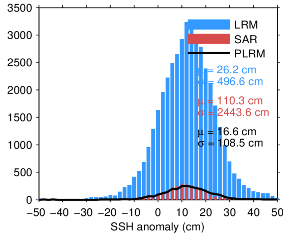
Figure 7. Histogram of flag-valid SSH anomaly over oceans and lakes for LRM (blue), SAR (red), and PLRM (black) for 16/04/2024. The mean ( \mu ) and standard deviation ( \sigma ) are also shown. Note that values outside [-50 50] cm are excluded from the histogram for the sake of readability but not from the computation of \mu and \sigma .
