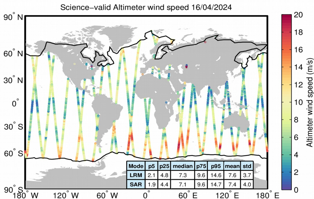
Figure 34. Geographical distribution of science-valid wind data over oceans and lakes for 16/04/2024. The statistical values shown in the table refer to the wind in m/s and are calculated separately for LRM and SAR regions. The black lines mark the outer limit of the Arctic and Antarctic polar polygons. Gray circles denote records that have been rejected based on the editing criteria described in Table 5.
