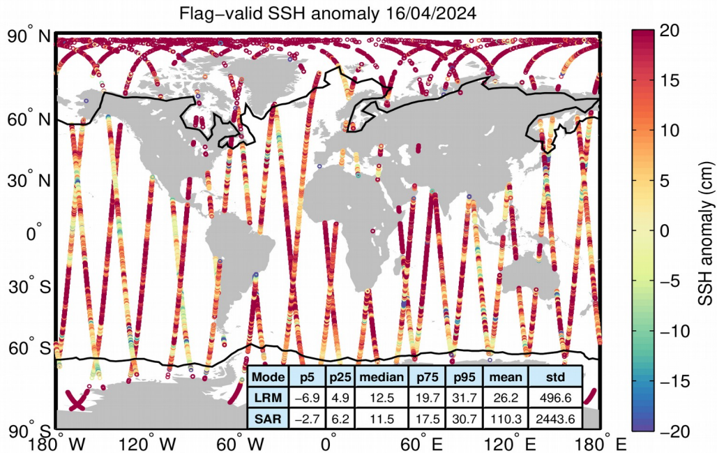
Figure 5. Geographical distribution of flag-valid 1-Hz SSH anomaly data over oceans and lakes for 16/04/2024. The statistical values shown in the table refer to the SSH anomaly in cm and are calculated separately for LRM and SAR regions. Measurements taken over polar polygons have been excluded from the computation of the statistical values. The black lines mark the outer limit of the Arctic and Antarctic polar polygons.
