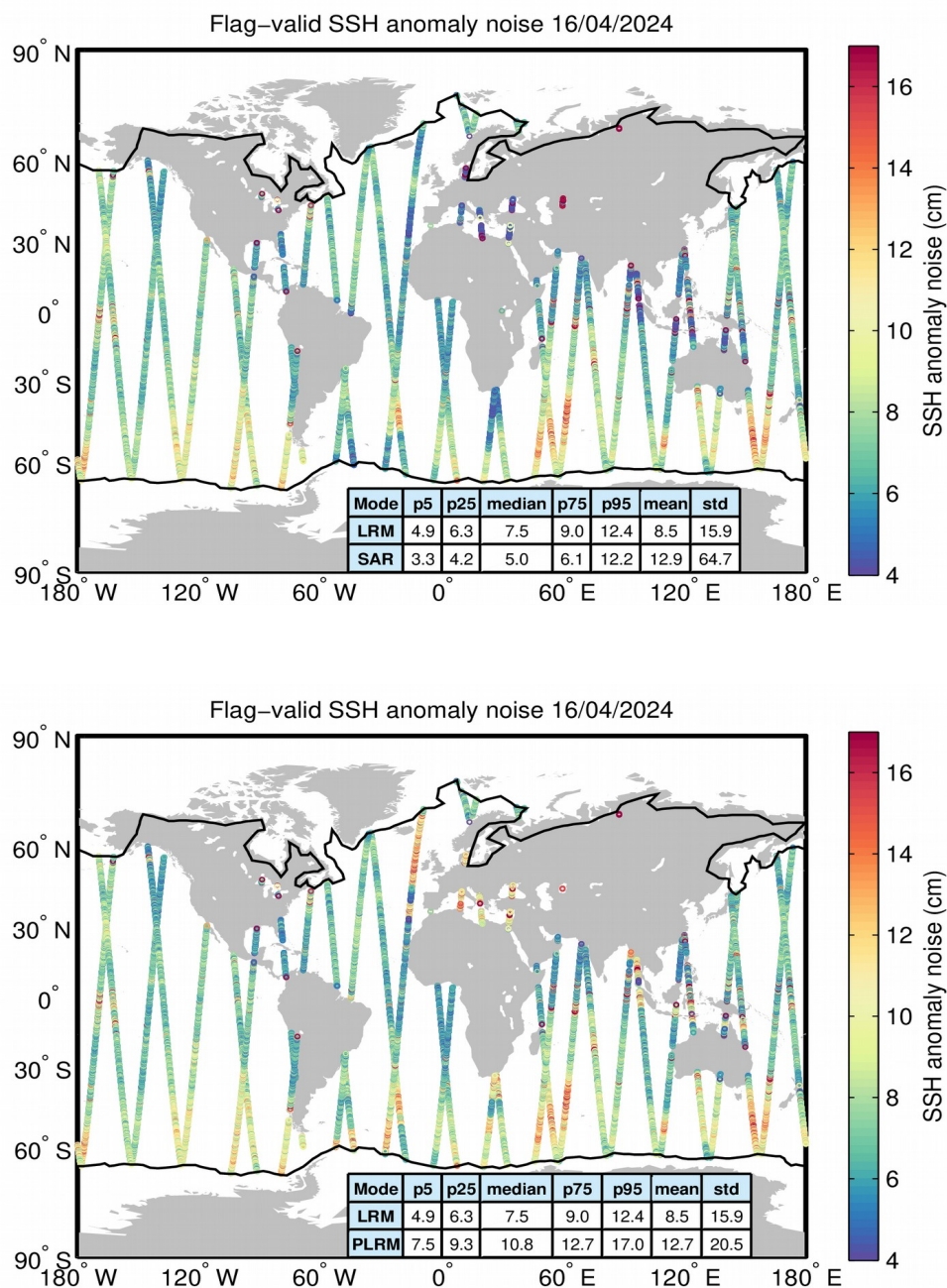
Figure 8. Geographical distribution of flag-valid 20-Hz SSH anomaly measurement noise over oceans and lakes for LRM/SAR (top) and LRM/PLRM (bottom) and for 16/04/2024. The statistical values shown in the tables refer to the SSH anomaly noise and are calculated separately for LRM and SAR/PLRM regions. Measurements taken over polar polygons have been excluded from the computation of the statistical values. The black lines mark the outer limit of the Arctic and Antarctic polar polygons.
