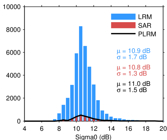
Figure 28. Histogram of science-valid sigma0 over oceans and lakes for LRM (blue), SAR (red), and PLRM (black) for 16/04/2024. The mean ( \mu ) and standard deviation ( \sigma ) are also shown. Note that values outside [4 20] dB are excluded from the histogram for the sake of readability but not from the computation of \mu and \sigma .
