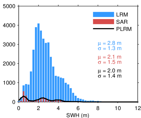
Figure 20. Histogram of science-valid SWH over oceans and lakes for LRM (blue), SAR (red), and PLRM (black) for 14/04/2024. The mean ( \mu ) and standard deviation ( \sigma ) are also
