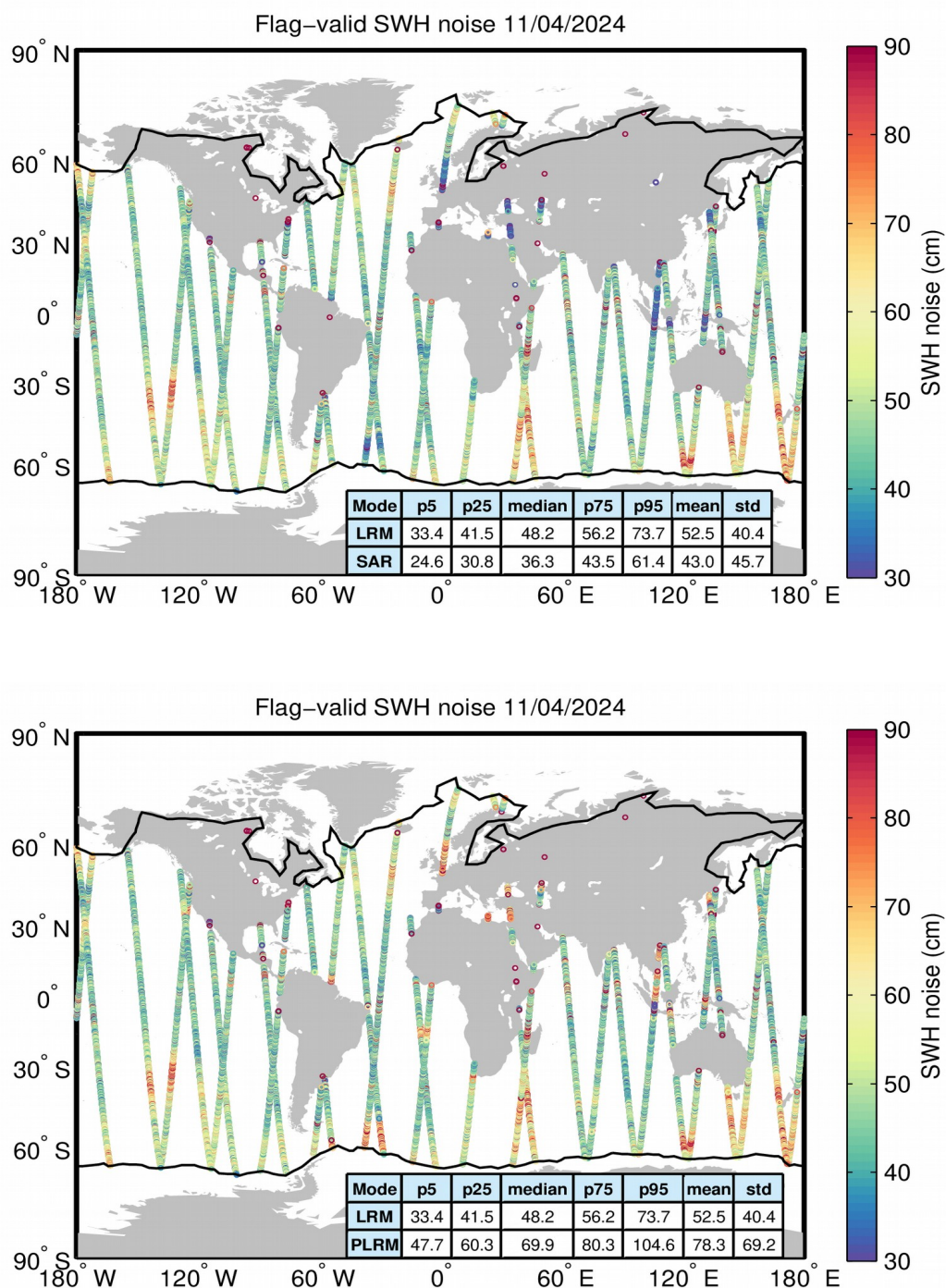
Figure 18. Geographical distribution of flag-valid 20-Hz SWH measurement noise over oceans and lakes for LRM/SAR (top) and LRM/PLRM (bottom) and for 11/04/2024. The statistical values shown in the table refer to the SWH noise and are calculated separately for LRM and SAR/PLRM regions. Measurements taken over polar polygons have been
