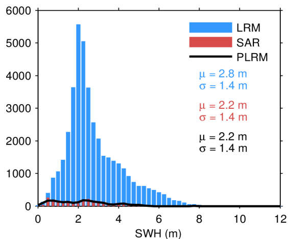
Figure 17. Histogram of flag-valid SWH over oceans and lakes for LRM (blue), SAR (red), and PLRM (black) for 11/04/2024. The mean ( \mu ) and standard deviation ( \sigma ) are also shown. Note that values larger than 12 m are excluded from the histogram for the sake of readability but not from the computation of \mu and \sigma .
