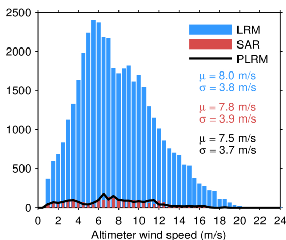
Figure 33. Histogram of flag-valid wind over oceans and lakes for LRM (blue), SAR (red), and PLRM (black) for 11/04/2024. The mean ( \mu ) and standard deviation ( \sigma ) are also shown. Note that values larger than 24 m/s are excluded from the histogram for the sake of readability but not from the computation of \mu and \sigma .
