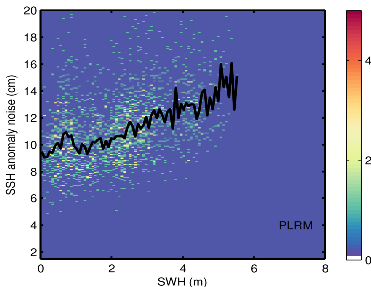
Figure 9. 2D histogram showing flag-valid SSH anomaly noise as a function of SWH for LRM (top), SAR (middle), and PLRM (bottom) for 11/04/2024. The black line denotes the median SSH anomaly noise as a function of SWH.
