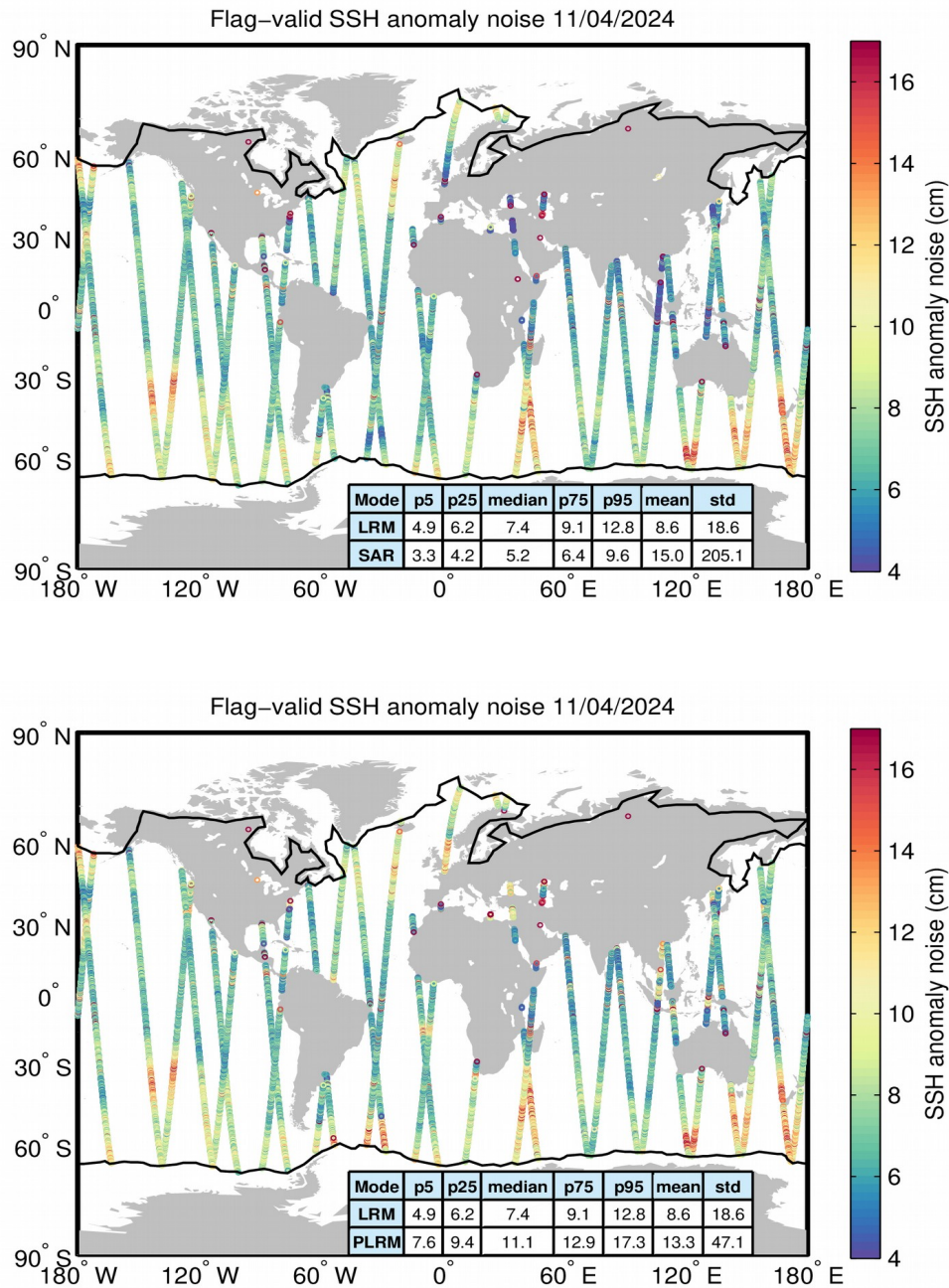
Figure 8. Geographical distribution of flag-valid 20-Hz SSH anomaly measurement noise over oceans and lakes for LRM/SAR (top) and LRM/PLRM (bottom) and for 11/04/2024. The statistical values shown in the tables refer to the SSH anomaly noise and are calculated separately for LRM and SAR/PLRM regions. Measurements taken over polar polygons have been excluded from the computation of the statistical values. The black lines mark the outer limit of the Arctic and Antarctic polar polygons.
