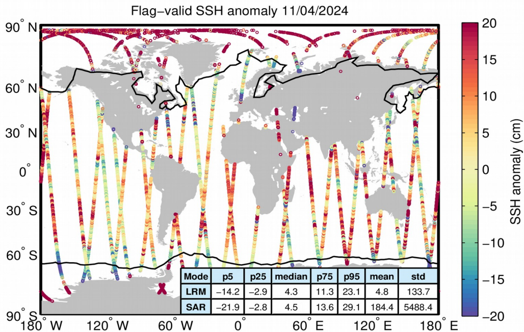
Figure 5. Geographical distribution of flag-valid 1-Hz SSH anomaly data over oceans and lakes for 11/04/2024. The statistical values shown in the table refer to the SSH anomaly in cm and are calculated separately for LRM and SAR regions. Measurements taken over polar polygons have been excluded from the computation of the statistical values. The black lines mark the outer limit of the Arctic and Antarctic polar polygons.
