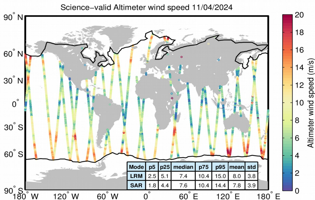
Figure 34. Geographical distribution of science-valid wind data over oceans and lakes for 11/04/2024. The statistical values shown in the table refer to the wind in m/s and are calculated separately for LRM and SAR regions. The black lines mark the outer limit of the Arctic and Antarctic polar polygons. Gray circles denote records that have been rejected based on the editing criteria described in Table 5.
