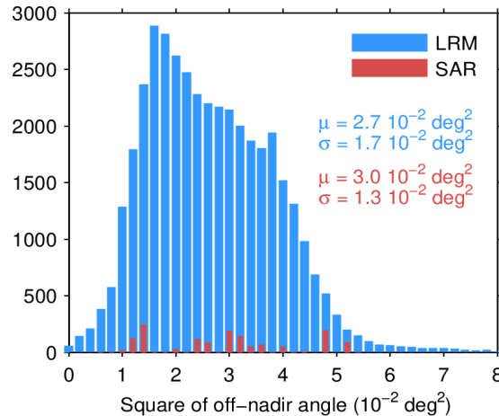
Figure 39. Histogram of flag-valid mispointing over oceans and lakes for LRM (blue) and SAR (red) for 11/04/2024. Only positive values have been considered. The mean ( \mu ) and standard deviation ( \sigma ) are also shown. Note that values larger than 8 \cdot 10^{-2} \text{ deg}^2 are excluded from the histogram for the sake of readability but not from the computation of \mu and \sigma .
