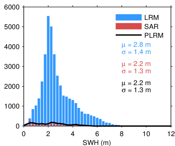
Figure 20. Histogram of science-valid SWH over oceans and lakes for LRM (blue), SAR (red), and PLRM (black) for 11/04/2024. The mean ( \mu ) and standard deviation ( \sigma ) are also
