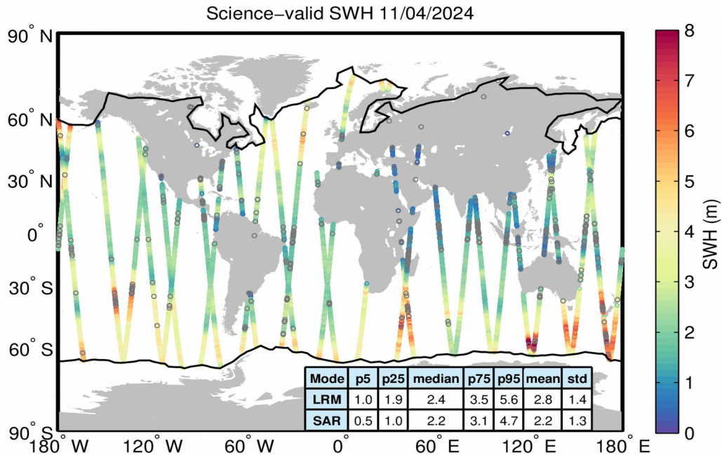
Figure 19. Geographical distribution of science-valid SWH data over oceans and lakes for 11/04/2024. The statistical values shown in the table refer to the SWH in m and are calculated separately for LRM and SAR regions. The black lines mark the outer limit of the Arctic and Antarctic polar polygons. Gray circles denote records that have been rejected based on the editing criteria described in Table 3.
