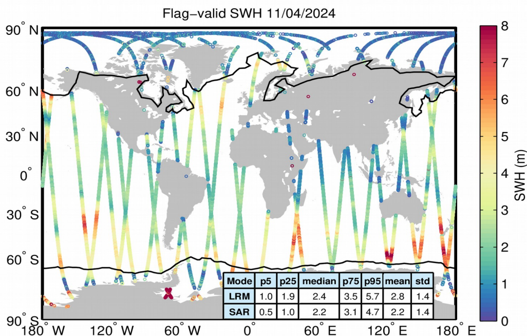
Figure 15. Geographical distribution of flag-valid SWH data over oceans and lakes for 11/04/2024. The statistical values shown in the table refer to the SWH in m and are calculated separately for LRM and SAR regions. Measurements taken over polar polygons have been excluded from the computation of the statistical values. The black lines mark the outer limit of the Arctic and Antarctic polar polygons.
