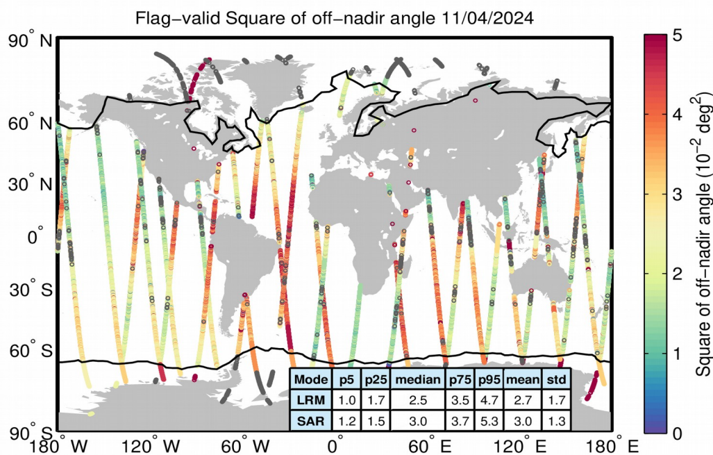
Figure 37. Geographical distribution of flag-valid mispointing data over oceans and lakes for 11/04/2024. The statistical values shown in the table refer to the mispointing in 10^{-2} \text{ deg}^2 and are calculated separately for LRM and SAR regions. Measurements taken over polar polygons have been excluded from the computation of the statistical values. The black lines mark the outer limit of the Arctic and Antarctic polar polygons. Gray circles denote negative values.
