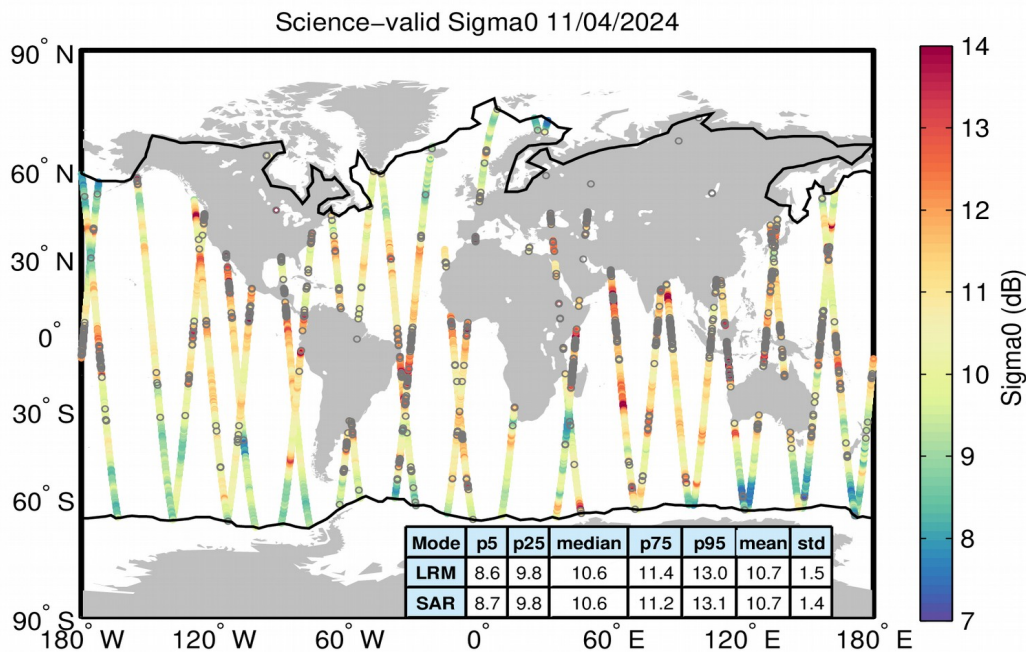
Figure 27. Geographical distribution of science-valid sigma0 data over oceans and lakes for 11/04/2024. The statistical values shown in the table refer to the sigma0 in dB and are calculated separately for LRM and SAR regions. The black lines mark the outer limit of the Arctic and Antarctic polar polygons. Gray circles denote records that have been rejected based on the editing criteria described in Table 4.
