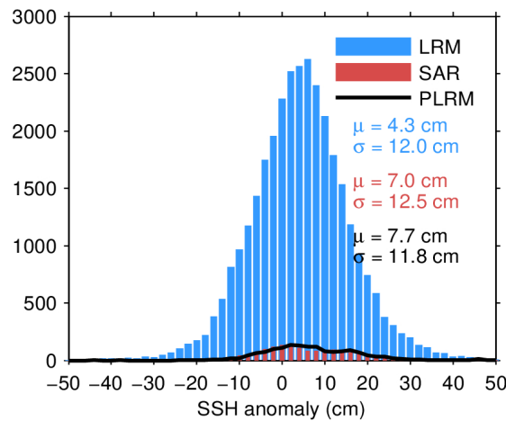
Figure 11. Histogram of science-valid SSH anomaly over oceans and lakes for LRM (blue), SAR (red), and PLRM (black) for 11/04/2024. The mean ( \mu ) and standard deviation ( \sigma ) are also shown. Note that values outside [-50\ 50] cm are excluded from the histogram for the sake of readability but not from the computation of \mu and \sigma .
