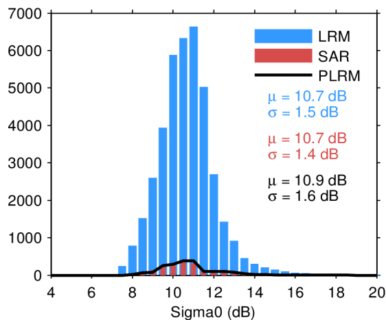
Figure 28. Histogram of science-valid sigma0 over oceans and lakes for LRM (blue), SAR (red), and PLRM (black) for 11/04/2024. The mean ( \mu ) and standard deviation ( \sigma ) are also shown. Note that values outside [4 20] dB are excluded from the histogram for the sake of readability but not from the computation of \mu and \sigma .
