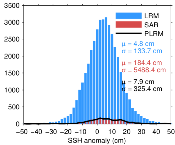
Figure 7. Histogram of flag-valid SSH anomaly over oceans and lakes for LRM (blue), SAR (red), and PLRM (black) for 11/04/2024. The mean ( \mu ) and standard deviation ( \sigma ) are also shown. Note that values outside [-50 50] cm are excluded from the histogram for the sake of readability but not from the computation of \mu and \sigma .
