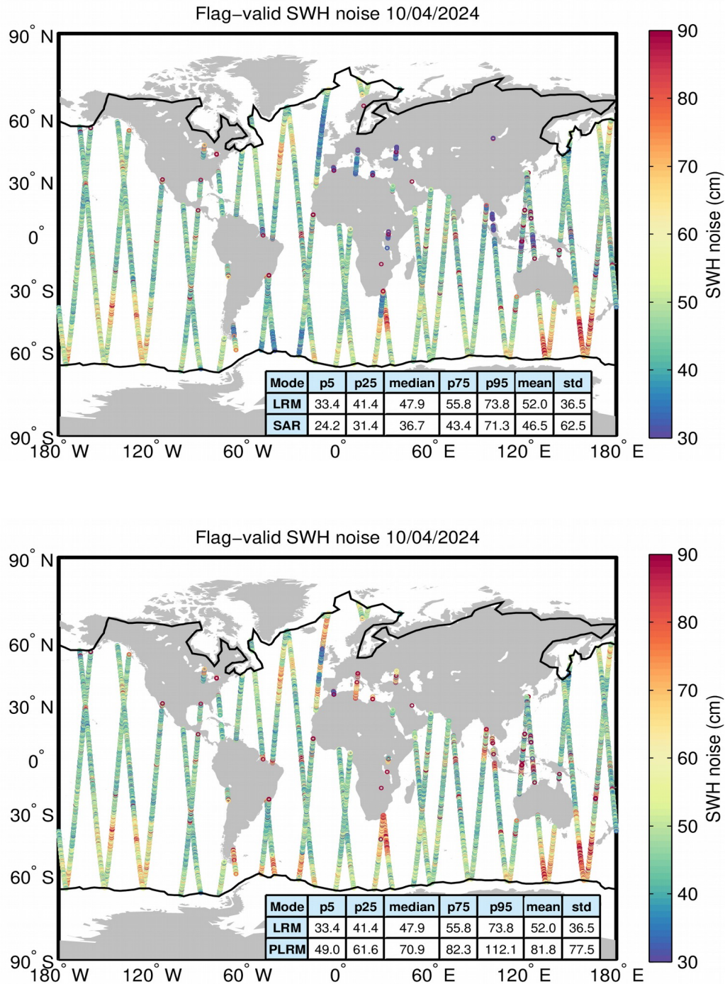
Figure 18. Geographical distribution of flag-valid 20-Hz SWH measurement noise over oceans and lakes for LRM/SAR (top) and LRM/PLRM (bottom) and for 10/04/2024. The statistical values shown in the table refer to the SWH noise and are calculated separately for LRM and SAR/PLRM regions. Measurements taken over polar polygons have been
