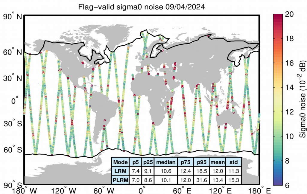
Figure 26. Geographical distribution of flag-valid 20-Hz sigma0 measurement noise over oceans and lakes for LRM/SAR (top) and LRM/PLRM (bottom) and for 09/04/2024. The statistical values shown in the table refer to the sigma0 noise and are calculated separately for LRM and SAR/PLRM regions. Measurements taken over polar polygons have been excluded from the computation of the statistical values. The black lines mark the outer limit of the Arctic and Antarctic polar polygons.
