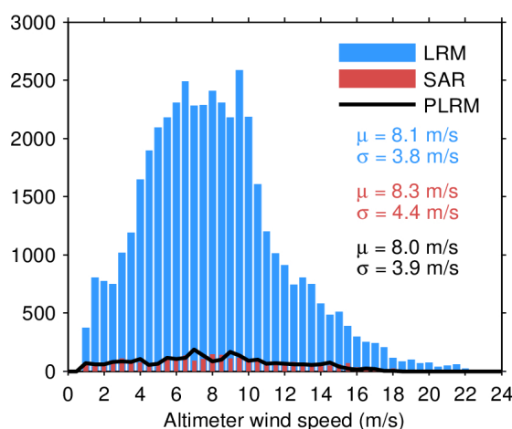
Figure 33. Histogram of flag-valid wind over oceans and lakes for LRM (blue), SAR (red), and PLRM (black) for 09/04/2024. The mean ( \mu ) and standard deviation ( \sigma ) are also shown. Note that values larger than 24 m/s are excluded from the histogram for the sake of readability but not from the computation of \mu and \sigma .
