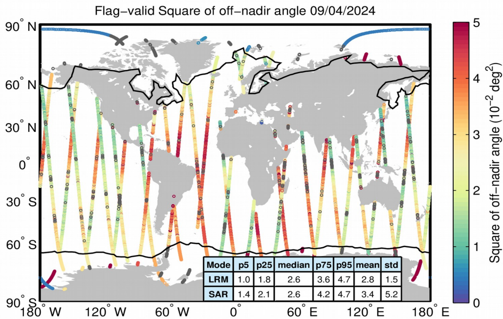
Figure 37. Geographical distribution of flag-valid mispointing data over oceans and lakes for 09/04/2024. The statistical values shown in the table refer to the mispointing in 10^{-2} \text{ deg}^2 and are calculated separately for LRM and SAR regions. Measurements taken over polar polygons have been excluded from the computation of the statistical values. The black lines mark the outer limit of the Arctic and Antarctic polar polygons. Gray circles denote negative values.
