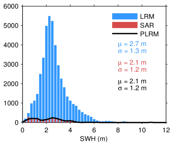
Figure 17. Histogram of flag-valid SWH over oceans and lakes for LRM (blue), SAR (red), and PLRM (black) for 09/04/2024. The mean ( \mu ) and standard deviation ( \sigma ) are also shown. Note that values larger than 12 m are excluded from the histogram for the sake of readability but not from the computation of \mu and \sigma .
