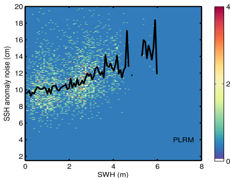
Figure 9. 2D histogram showing flag-valid SSH anomaly noise as a function of SWH for LRM (top), SAR (middle), and PLRM (bottom) for 09/04/2024. The black line denotes the median SSH anomaly noise as a function of SWH.
