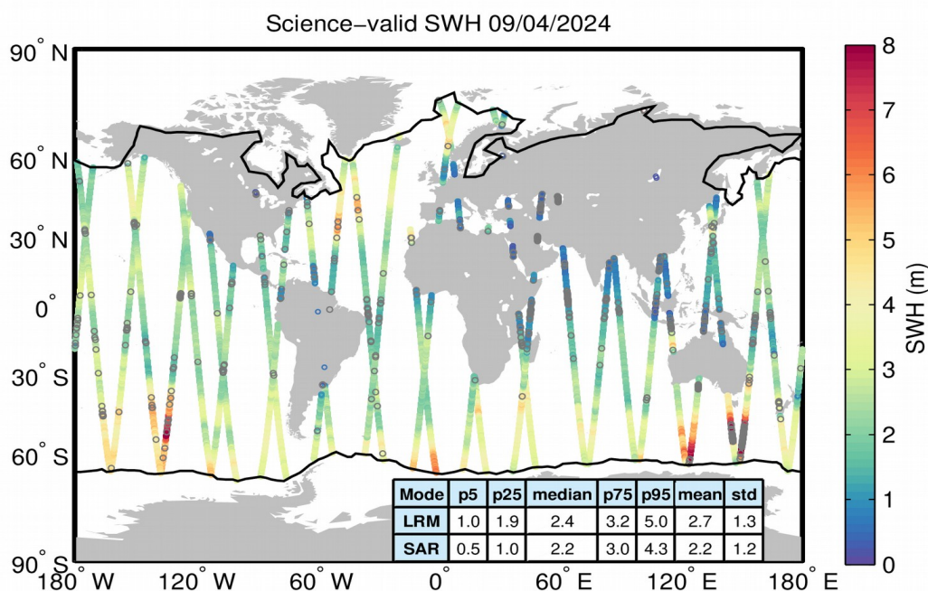
Figure 19. Geographical distribution of science-valid SWH data over oceans and lakes for 09/04/2024. The statistical values shown in the table refer to the SWH in m and are calculated separately for LRM and SAR regions. The black lines mark the outer limit of the Arctic and Antarctic polar polygons. Gray circles denote records that have been rejected based on the editing criteria described in Table 3.
