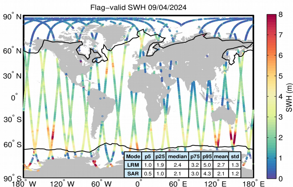
Figure 15. Geographical distribution of flag-valid SWH data over oceans and lakes for 09/04/2024. The statistical values shown in the table refer to the SWH in m and are calculated separately for LRM and SAR regions. Measurements taken over polar polygons have been excluded from the computation of the statistical values. The black lines mark the outer limit of the Arctic and Antarctic polar polygons.
