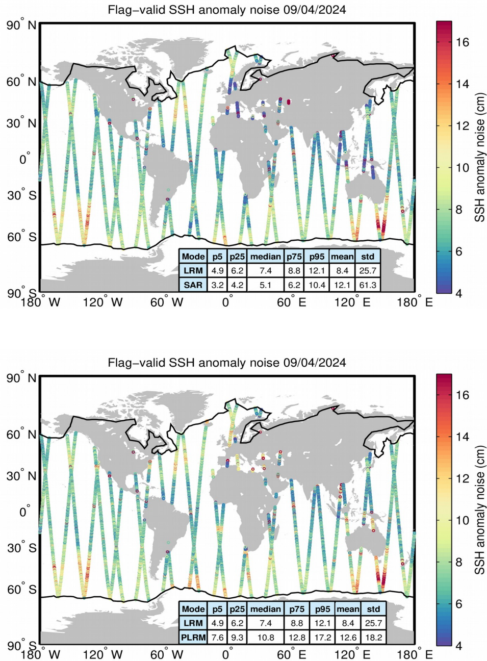
Figure 8. Geographical distribution of flag-valid 20-Hz SSH anomaly measurement noise over oceans and lakes for LRM/SAR (top) and LRM/PLRM (bottom) and for 09/04/2024. The statistical values shown in the tables refer to the SSH anomaly noise and are calculated separately for LRM and SAR/PLRM regions. Measurements taken over polar polygons have been excluded from the computation of the statistical values. The black lines mark the outer limit of the Arctic and Antarctic polar polygons.
