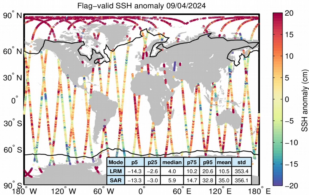
Figure 5. Geographical distribution of flag-valid 1-Hz SSH anomaly data over oceans and lakes for 09/04/2024. The statistical values shown in the table refer to the SSH anomaly in cm and are calculated separately for LRM and SAR regions. Measurements taken over polar polygons have been excluded from the computation of the statistical values. The black lines mark the outer limit of the Arctic and Antarctic polar polygons.
