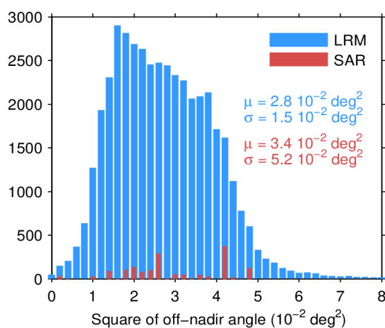
Figure 39. Histogram of flag-valid mispointing over oceans and lakes for LRM (blue) and SAR (red) for 09/04/2024. Only positive values have been considered. The mean ( \mu ) and standard deviation ( \sigma ) are also shown. Note that values larger than 8 \cdot 10^{-2} \text{ deg}^2 are excluded from the histogram for the sake of readability but not from the computation of \mu and \sigma .
