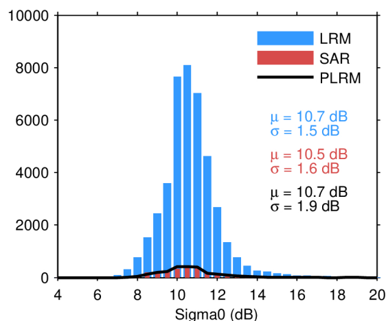
Figure 28. Histogram of science-valid sigma0 over oceans and lakes for LRM (blue), SAR (red), and PLRM (black) for 09/04/2024. The mean ( \mu ) and standard deviation ( \sigma ) are also shown. Note that values outside [4 20] dB are excluded from the histogram for the sake of readability but not from the computation of \mu and \sigma .
