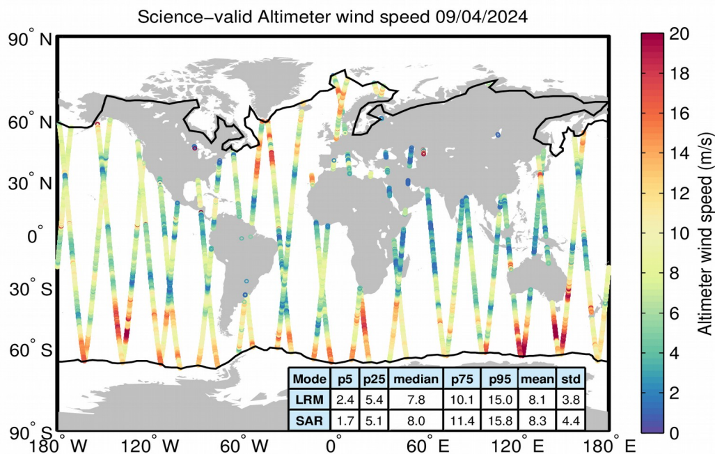
Figure 34. Geographical distribution of science-valid wind data over oceans and lakes for 09/04/2024. The statistical values shown in the table refer to the wind in m/s and are calculated separately for LRM and SAR regions. The black lines mark the outer limit of the Arctic and Antarctic polar polygons. Gray circles denote records that have been rejected based on the editing criteria described in Table 5.
