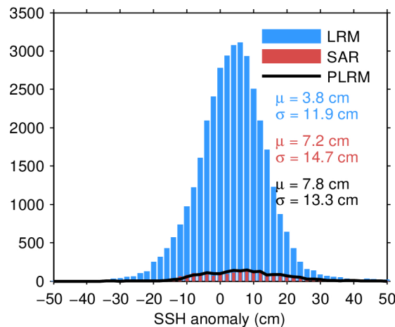
Figure 11. Histogram of science-valid SSH anomaly over oceans and lakes for LRM (blue), SAR (red), and PLRM (black) for 09/04/2024. The mean ( \mu ) and standard deviation ( \sigma ) are also shown. Note that values outside [-50\ 50] cm are excluded from the histogram for the sake of readability but not from the computation of \mu and \sigma .
