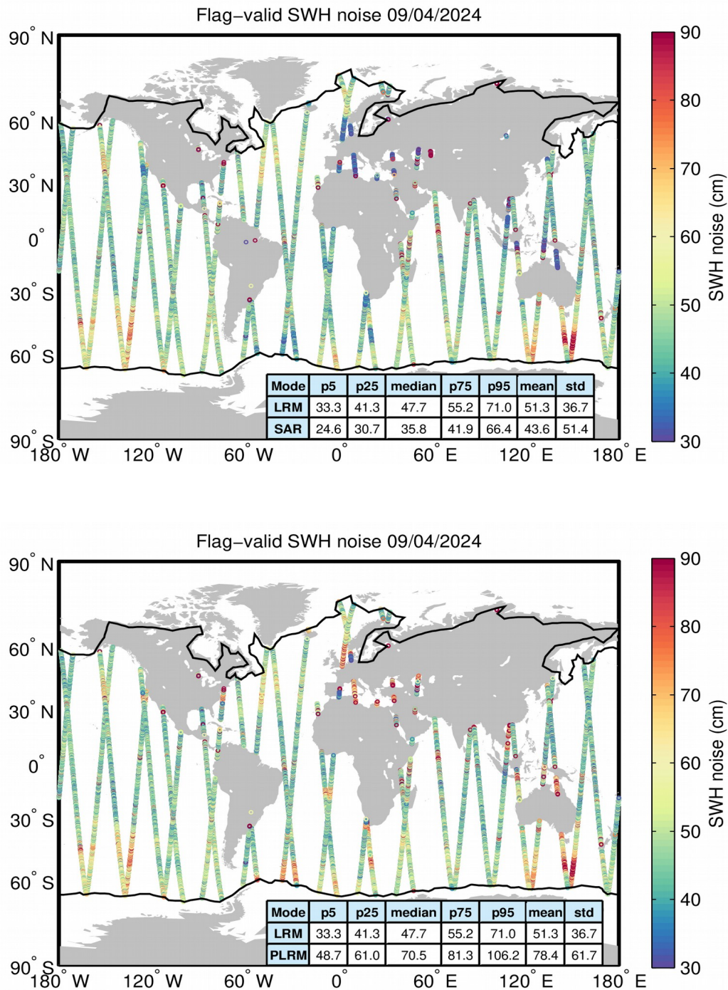
Figure 18. Geographical distribution of flag-valid 20-Hz SWH measurement noise over oceans and lakes for LRM/SAR (top) and LRM/PLRM (bottom) and for 09/04/2024. The statistical values shown in the table refer to the SWH noise and are calculated separately for LRM and SAR/PLRM regions. Measurements taken over polar polygons have been
