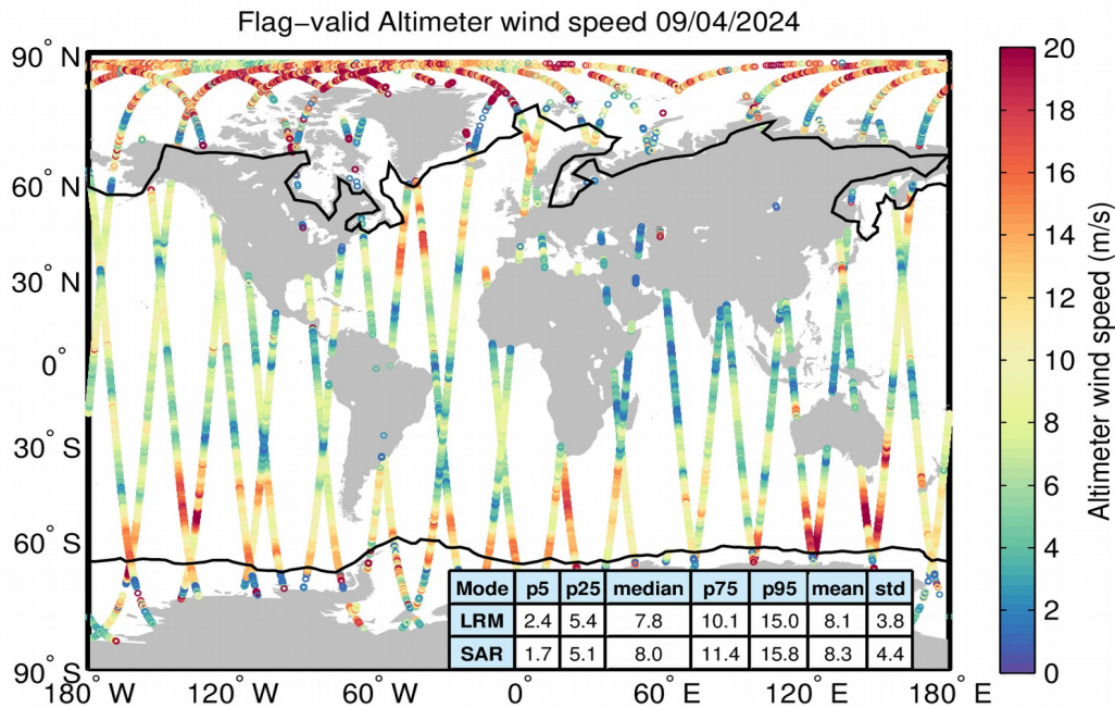
Figure 31. Geographical distribution of flag-valid wind data over oceans and lakes for 09/04/2024. The statistical values shown in the table refer to the wind in m/s and are calculated separately for LRM and SAR regions. Measurements taken over polar polygons have been excluded from the computation of the statistical values. The black lines mark the outer limit of the Arctic and Antarctic polar polygons.
