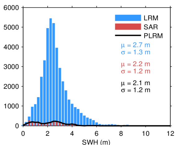
Figure 20. Histogram of science-valid SWH over oceans and lakes for LRM (blue), SAR (red), and PLRM (black) for 09/04/2024. The mean ( \mu ) and standard deviation ( \sigma ) are also
