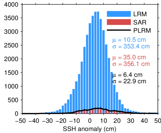
Figure 7. Histogram of flag-valid SSH anomaly over oceans and lakes for LRM (blue), SAR (red), and PLRM (black) for 09/04/2024. The mean ( \mu ) and standard deviation ( \sigma ) are also shown. Note that values outside [-50 50] cm are excluded from the histogram for the sake of readability but not from the computation of \mu and \sigma .
