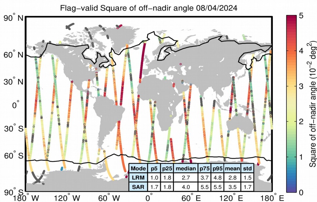
Figure 37. Geographical distribution of flag-valid mispointing data over oceans and lakes for 08/04/2024. The statistical values shown in the table refer to the mispointing in 10^{-2} \text{ deg}^2 and are calculated separately for LRM and SAR regions. Measurements taken over polar polygons have been excluded from the computation of the statistical values. The black lines mark the outer limit of the Arctic and Antarctic polar polygons. Gray circles denote negative values.
