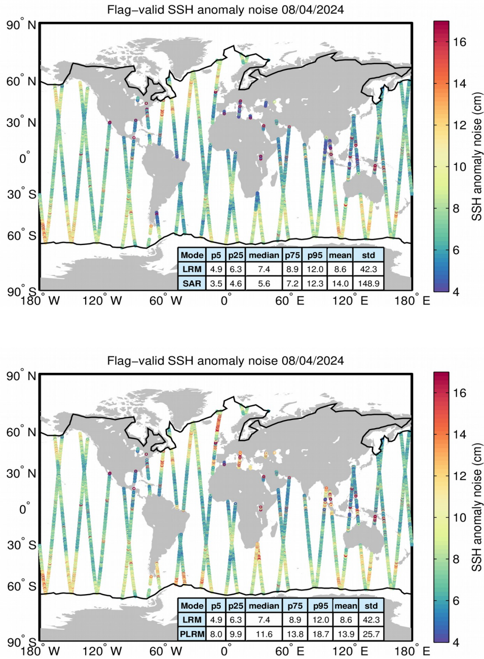
Figure 8. Geographical distribution of flag-valid 20-Hz SSH anomaly measurement noise over oceans and lakes for LRM/SAR (top) and LRM/PLRM (bottom) and for 08/04/2024. The statistical values shown in the tables refer to the SSH anomaly noise and are calculated separately for LRM and SAR/PLRM regions. Measurements taken over polar polygons have been excluded from the computation of the statistical values. The black lines mark the outer limit of the Arctic and Antarctic polar polygons.
