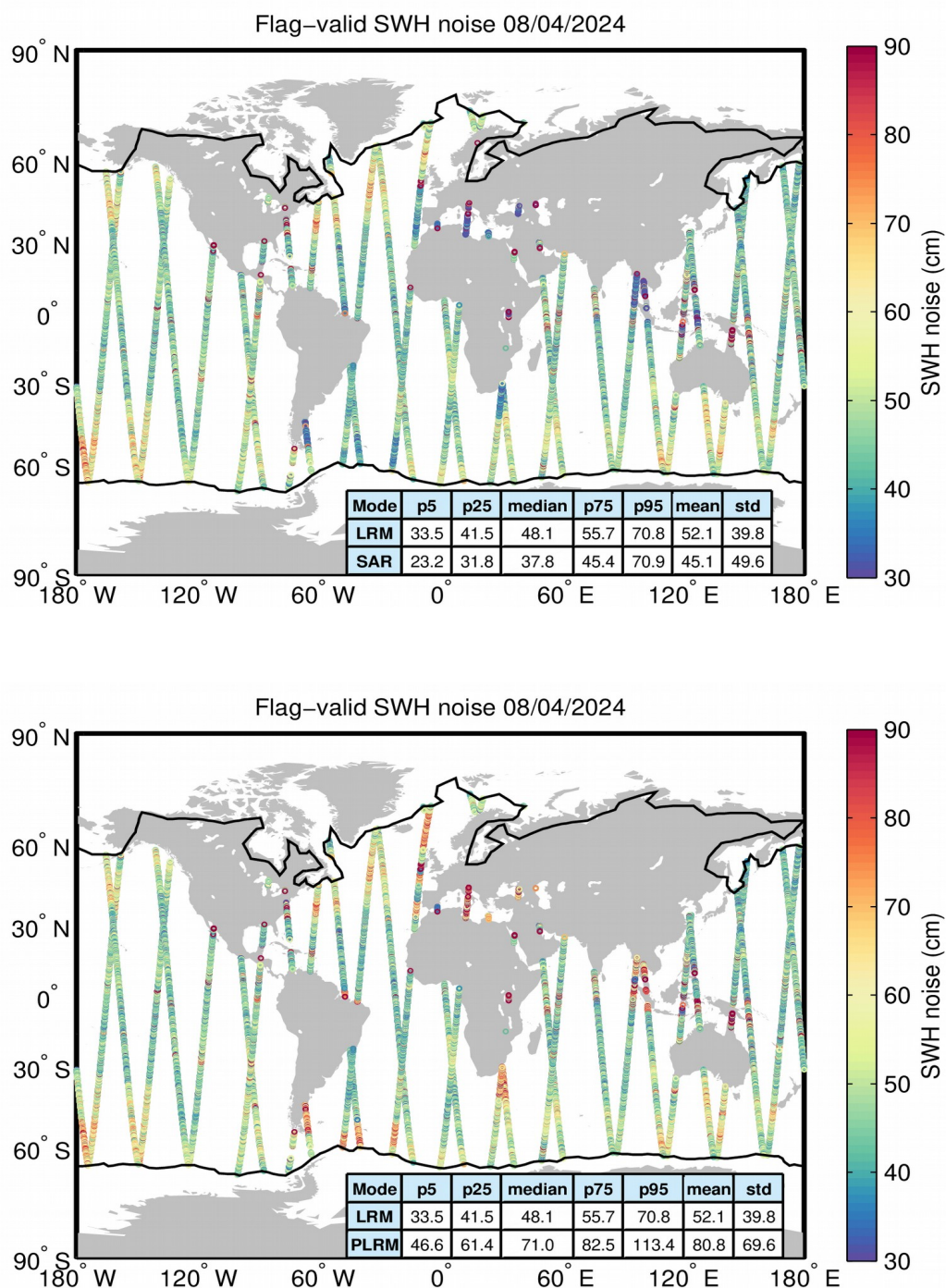
Figure 18. Geographical distribution of flag-valid 20-Hz SWH measurement noise over oceans and lakes for LRM/SAR (top) and LRM/PLRM (bottom) and for 08/04/2024. The statistical values shown in the table refer to the SWH noise and are calculated separately for LRM and SAR/PLRM regions. Measurements taken over polar polygons have been
