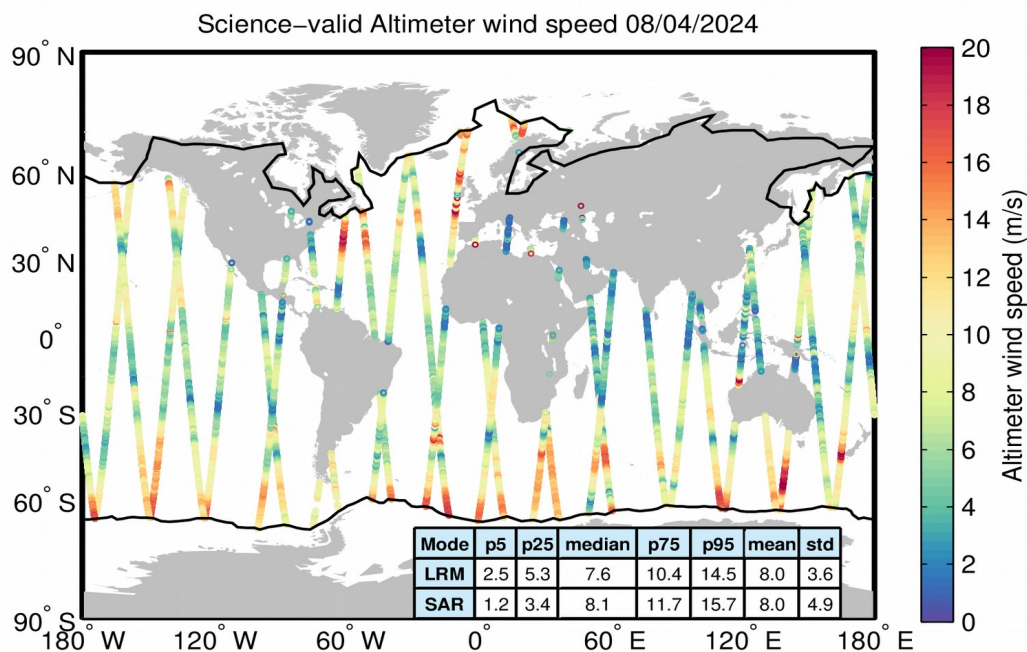
Figure 34. Geographical distribution of science-valid wind data over oceans and lakes for 08/04/2024. The statistical values shown in the table refer to the wind in m/s and are calculated separately for LRM and SAR regions. The black lines mark the outer limit of the Arctic and Antarctic polar polygons. Gray circles denote records that have been rejected based on the editing criteria described in Table 5.
