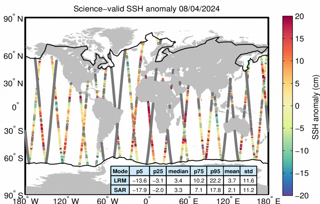
Figure 10. Geographical distribution of science-valid SSH anomaly data over oceans and lakes for 08/04/2024. The statistical values shown in the table refer to the SSH anomaly in cm and are calculated separately for LRM and SAR regions. The black lines mark the
