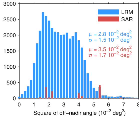
Figure 39. Histogram of flag-valid mispointing over oceans and lakes for LRM (blue) and SAR (red) for 08/04/2024. Only positive values have been considered. The mean ( \mu ) and standard deviation ( \sigma ) are also shown. Note that values larger than 8 \cdot 10^{-2} \text{ deg}^2 are excluded from the histogram for the sake of readability but not from the computation of \mu and \sigma .
