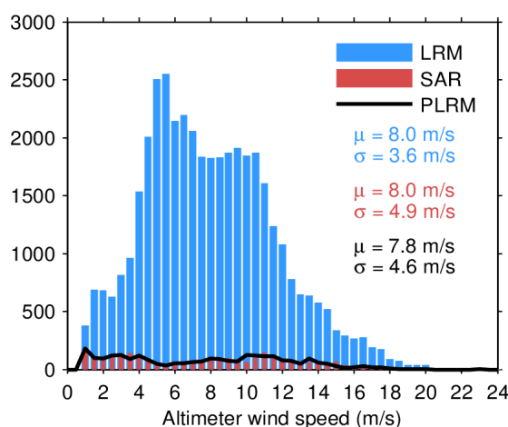
Figure 33. Histogram of flag-valid wind over oceans and lakes for LRM (blue), SAR (red), and PLRM (black) for 08/04/2024. The mean ( \mu ) and standard deviation ( \sigma ) are also shown. Note that values larger than 24 m/s are excluded from the histogram for the sake of readability but not from the computation of \mu and \sigma .
