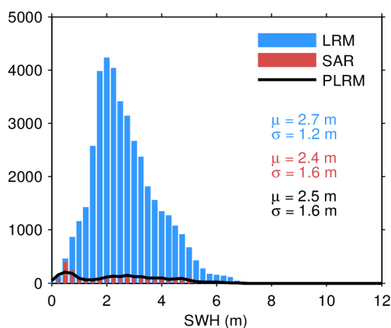
Figure 20. Histogram of science-valid SWH over oceans and lakes for LRM (blue), SAR (red), and PLRM (black) for 08/04/2024. The mean ( \mu ) and standard deviation ( \sigma ) are also
