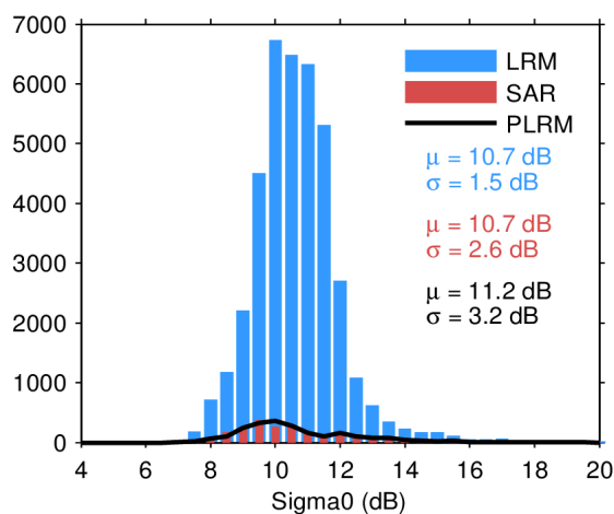
Figure 28. Histogram of science-valid sigma0 over oceans and lakes for LRM (blue), SAR (red), and PLRM (black) for 08/04/2024. The mean ( \mu ) and standard deviation ( \sigma ) are also shown. Note that values outside [4 20] dB are excluded from the histogram for the sake of readability but not from the computation of \mu and \sigma .
