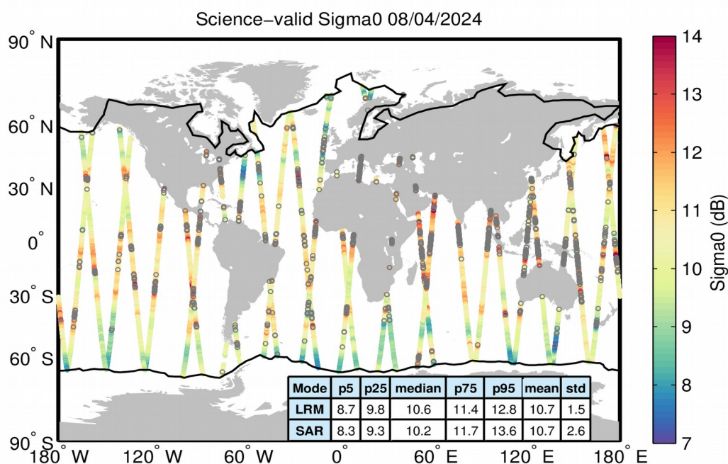
Figure 27. Geographical distribution of science-valid sigma0 data over oceans and lakes for 08/04/2024. The statistical values shown in the table refer to the sigma0 in dB and are calculated separately for LRM and SAR regions. The black lines mark the outer limit of the Arctic and Antarctic polar polygons. Gray circles denote records that have been rejected based on the editing criteria described in Table 4.
