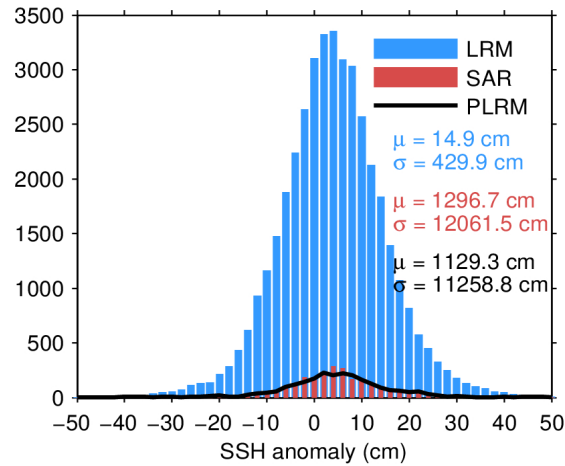
Figure 7. Histogram of flag-valid SSH anomaly over oceans and lakes for LRM (blue), SAR (red), and PLRM (black) for 08/04/2024. The mean ( \mu ) and standard deviation ( \sigma ) are also shown. Note that values outside [-50 50] cm are excluded from the histogram for the sake of readability but not from the computation of \mu and \sigma .
