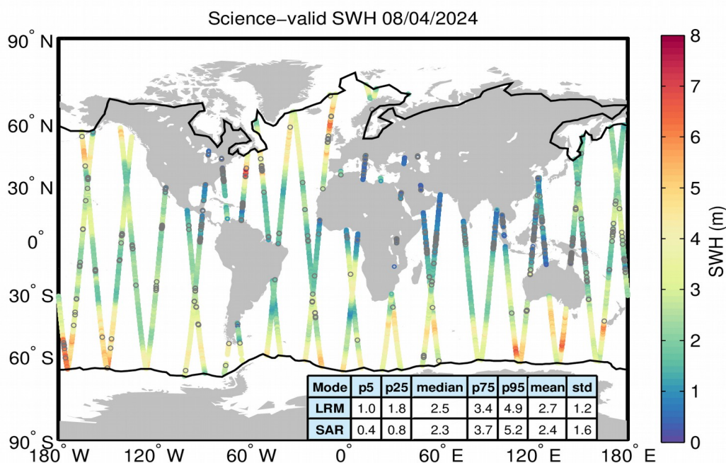
Figure 19. Geographical distribution of science-valid SWH data over oceans and lakes for 08/04/2024. The statistical values shown in the table refer to the SWH in m and are calculated separately for LRM and SAR regions. The black lines mark the outer limit of the Arctic and Antarctic polar polygons. Gray circles denote records that have been rejected based on the editing criteria described in Table 3.
