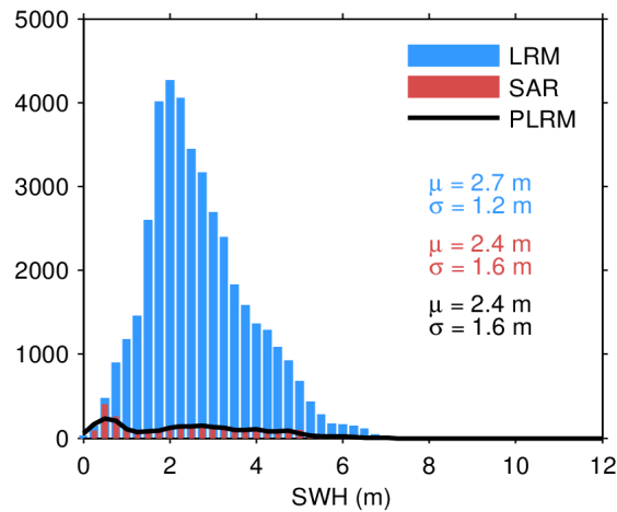
Figure 17. Histogram of flag-valid SWH over oceans and lakes for LRM (blue), SAR (red), and PLRM (black) for 08/04/2024. The mean ( \mu ) and standard deviation ( \sigma ) are also shown. Note that values larger than 12 m are excluded from the histogram for the sake of readability but not from the computation of \mu and \sigma .
