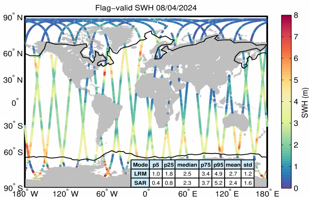
Figure 15. Geographical distribution of flag-valid SWH data over oceans and lakes for 08/04/2024. The statistical values shown in the table refer to the SWH in m and are calculated separately for LRM and SAR regions. Measurements taken over polar polygons have been excluded from the computation of the statistical values. The black lines mark the outer limit of the Arctic and Antarctic polar polygons.
