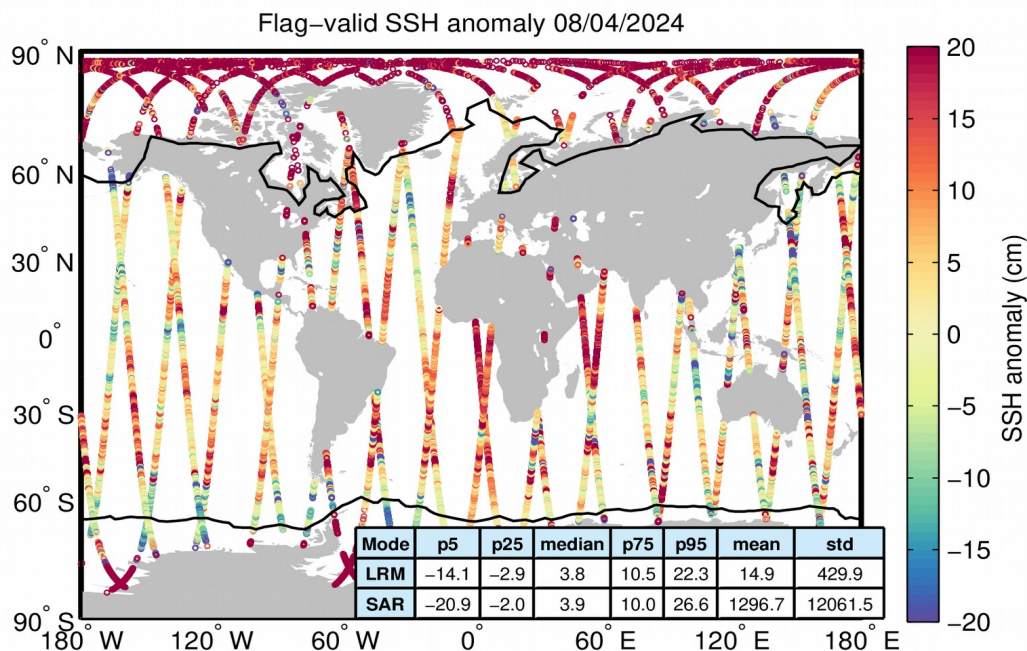
Figure 5. Geographical distribution of flag-valid 1-Hz SSH anomaly data over oceans and lakes for 08/04/2024. The statistical values shown in the table refer to the SSH anomaly in cm and are calculated separately for LRM and SAR regions. Measurements taken over polar polygons have been excluded from the computation of the statistical values. The black lines mark the outer limit of the Arctic and Antarctic polar polygons.
