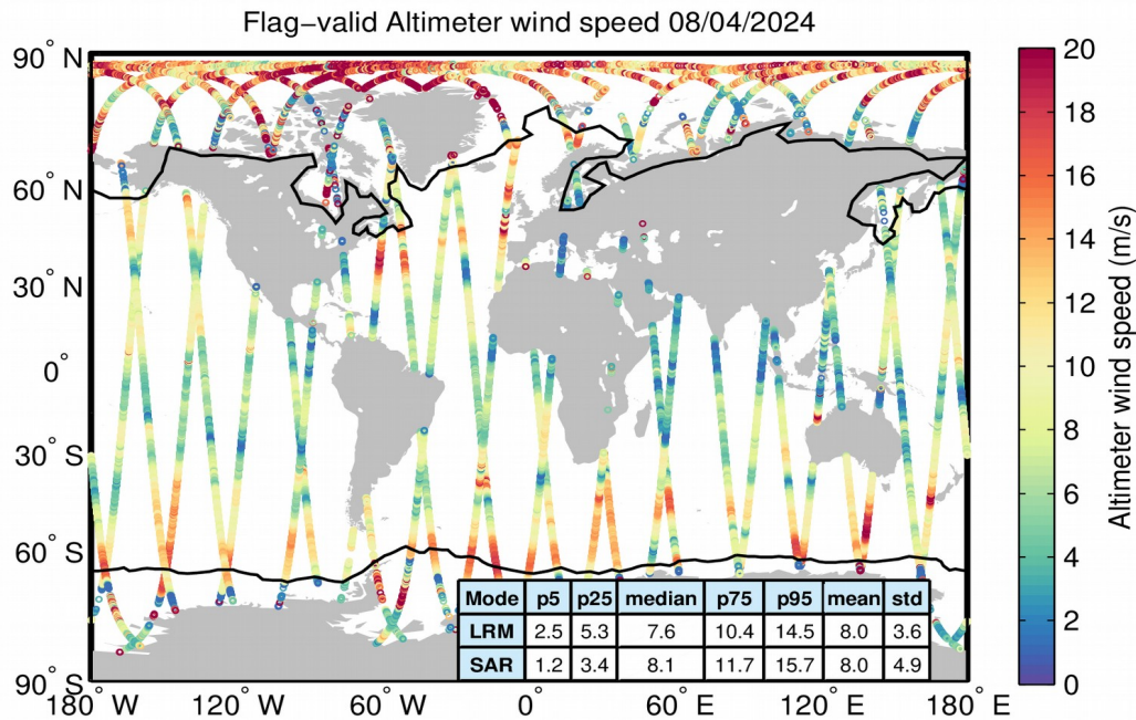
Figure 31. Geographical distribution of flag-valid wind data over oceans and lakes for 08/04/2024. The statistical values shown in the table refer to the wind in m/s and are calculated separately for LRM and SAR regions. Measurements taken over polar polygons have been excluded from the computation of the statistical values. The black lines mark the outer limit of the Arctic and Antarctic polar polygons.
