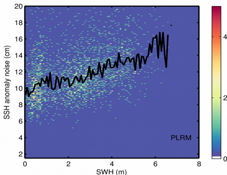
Figure 9. 2D histogram showing flag-valid SSH anomaly noise as a function of SWH for LRM (top), SAR (middle), and PLRM (bottom) for 08/04/2024. The black line denotes the median SSH anomaly noise as a function of SWH.
