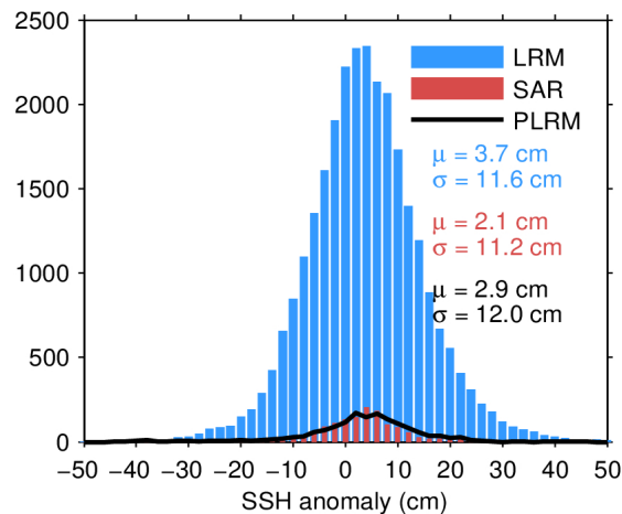
Figure 11. Histogram of science-valid SSH anomaly over oceans and lakes for LRM (blue), SAR (red), and PLRM (black) for 08/04/2024. The mean ( \mu ) and standard deviation ( \sigma ) are also shown. Note that values outside [-50\ 50] cm are excluded from the histogram for the sake of readability but not from the computation of \mu and \sigma .
