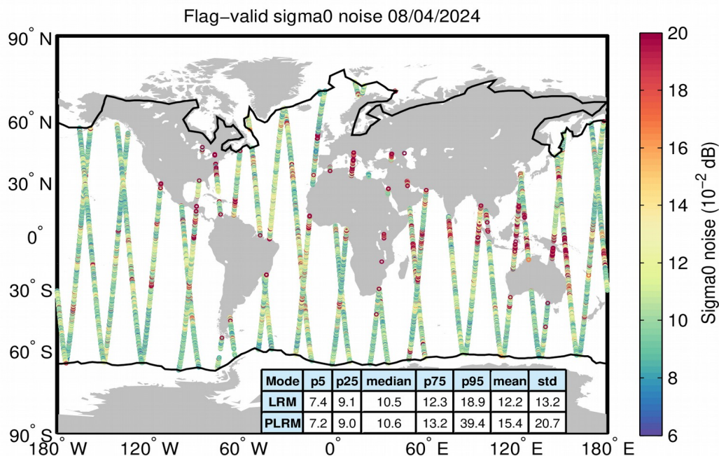
Figure 26. Geographical distribution of flag-valid 20-Hz sigma0 measurement noise over oceans and lakes for LRM/SAR (top) and LRM/PLRM (bottom) and for 08/04/2024. The statistical values shown in the table refer to the sigma0 noise and are calculated separately for LRM and SAR/PLRM regions. Measurements taken over polar polygons have been excluded from the computation of the statistical values. The black lines mark the outer limit of the Arctic and Antarctic polar polygons.
