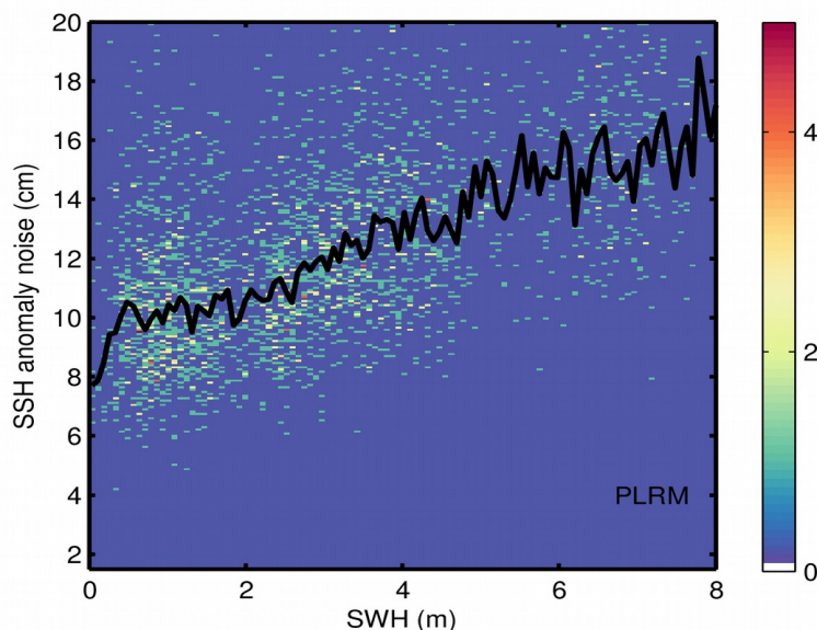
Figure 9. 2D histogram showing flag-valid SSH anomaly noise as a function of SWH for LRM (top), SAR (middle), and PLRM (bottom) for 28/03/2024. The black line denotes the median SSH anomaly noise as a function of SWH.
