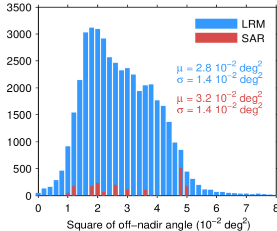
Figure 39. Histogram of flag-valid mispointing over oceans and lakes for LRM (blue) and SAR (red) for 28/03/2024. Only positive values have been considered. The mean ( \mu ) and standard deviation ( \sigma ) are also shown. Note that values larger than 8 \cdot 10^{-2} \text{ deg}^2 are excluded from the histogram for the sake of readability but not from the computation of \mu and \sigma .
