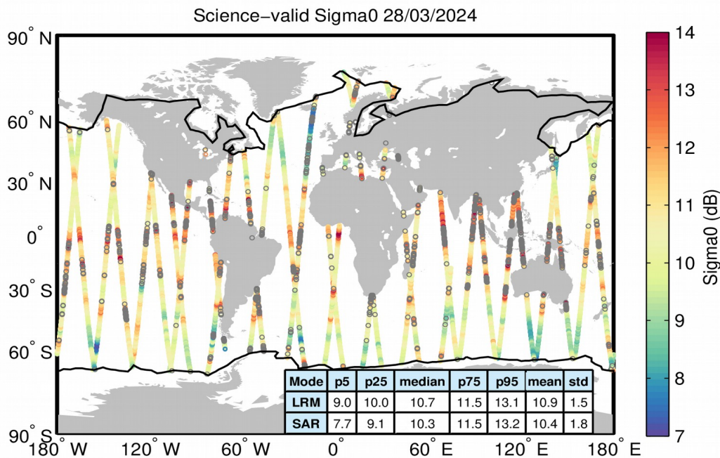
Figure 27. Geographical distribution of science-valid sigma0 data over oceans and lakes for 28/03/2024. The statistical values shown in the table refer to the sigma0 in dB and are calculated separately for LRM and SAR regions. The black lines mark the outer limit of the Arctic and Antarctic polar polygons. Gray circles denote records that have been rejected based on the editing criteria described in Table 4.
