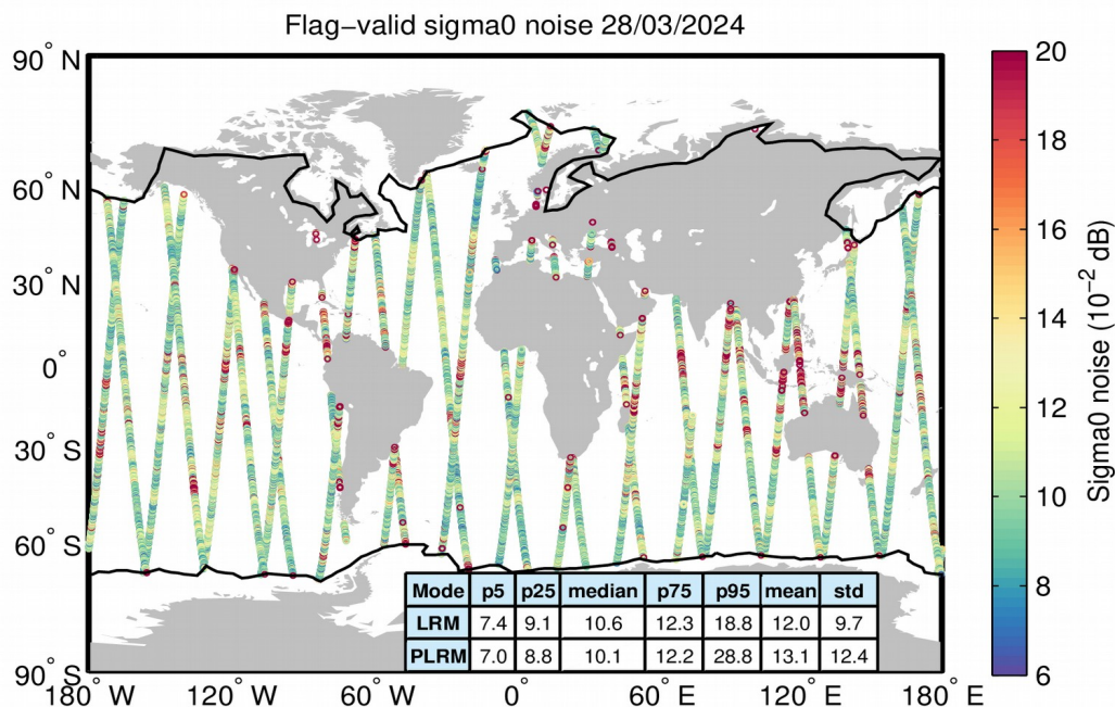
Figure 26. Geographical distribution of flag-valid 20-Hz sigma0 measurement noise over oceans and lakes for LRM/SAR (top) and LRM/PLRM (bottom) and for 28/03/2024. The statistical values shown in the table refer to the sigma0 noise and are calculated separately for LRM and SAR/PLRM regions. Measurements taken over polar polygons have been excluded from the computation of the statistical values. The black lines mark the outer limit of the Arctic and Antarctic polar polygons.
