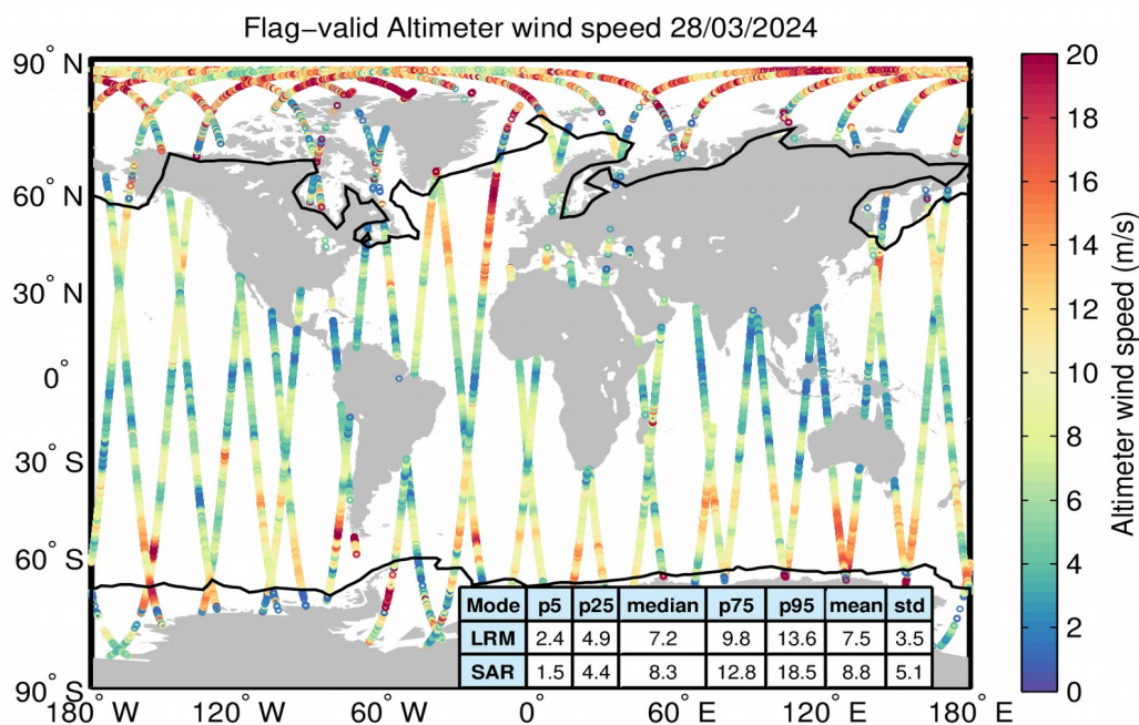
Figure 31. Geographical distribution of flag-valid wind data over oceans and lakes for 28/03/2024. The statistical values shown in the table refer to the wind in m/s and are calculated separately for LRM and SAR regions. Measurements taken over polar polygons have been excluded from the computation of the statistical values. The black lines mark the outer limit of the Arctic and Antarctic polar polygons.
