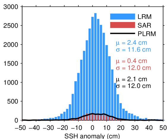
Figure 11. Histogram of science-valid SSH anomaly over oceans and lakes for LRM (blue), SAR (red), and PLRM (black) for 28/03/2024. The mean ( \mu ) and standard deviation ( \sigma ) are also shown. Note that values outside [-50\ 50] cm are excluded from the histogram for the sake of readability but not from the computation of \mu and \sigma .
