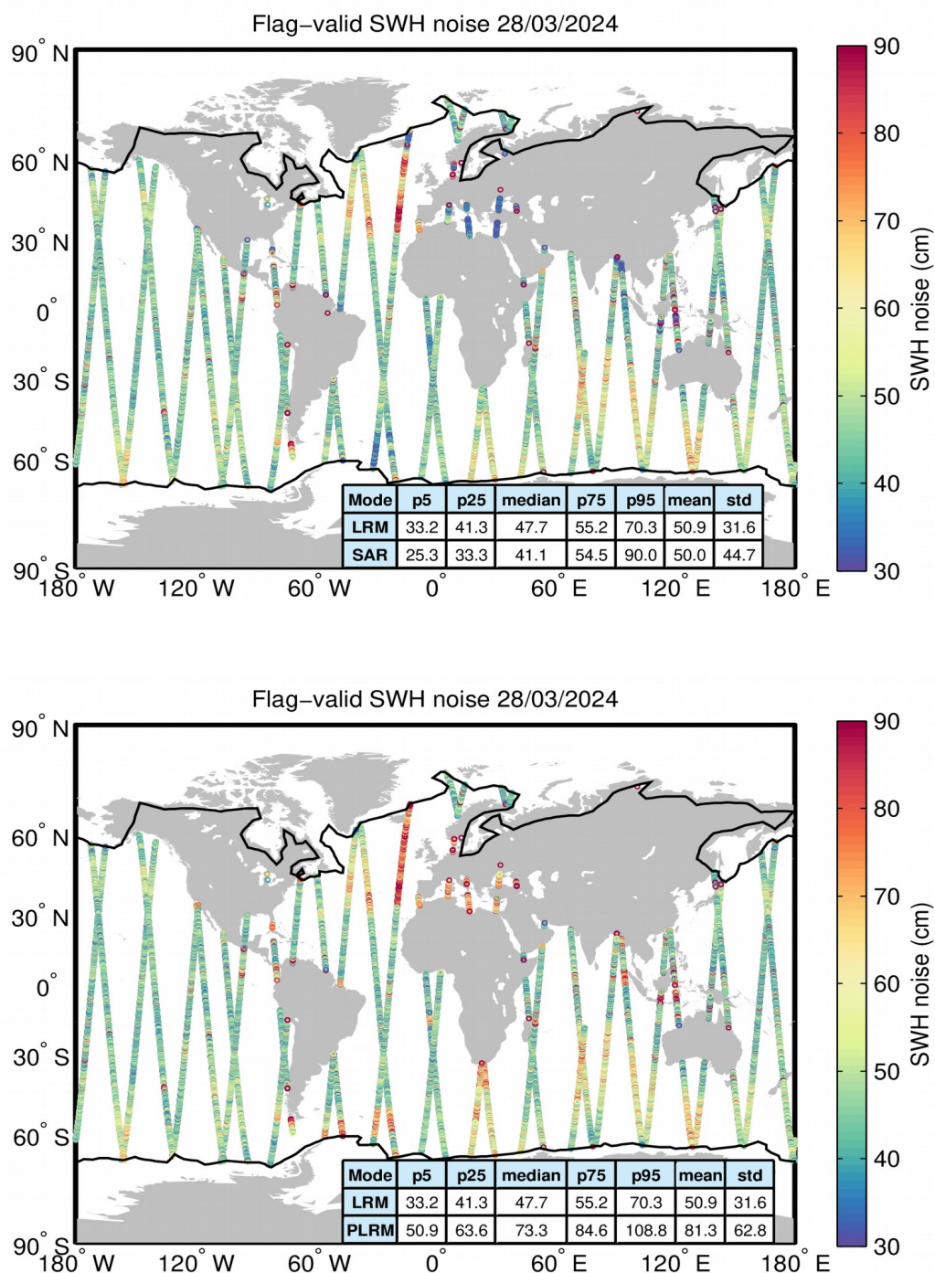
Figure 18. Geographical distribution of flag-valid 20-Hz SWH measurement noise over oceans and lakes for LRM/SAR (top) and LRM/PLRM (bottom) and for 28/03/2024. The statistical values shown in the table refer to the SWH noise and are calculated separately for LRM and SAR/PLRM regions. Measurements taken over polar polygons have been
