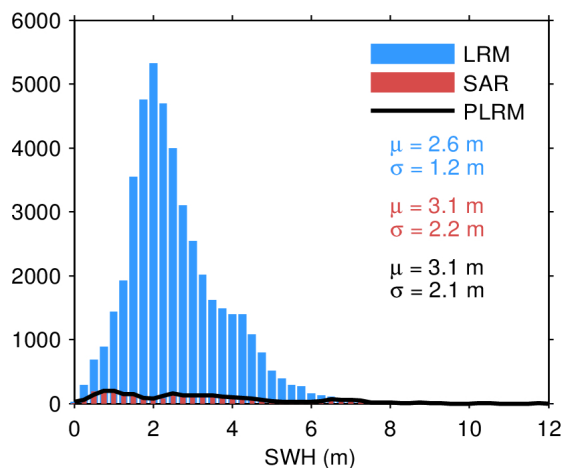
Figure 17. Histogram of flag-valid SWH over oceans and lakes for LRM (blue), SAR (red), and PLRM (black) for 28/03/2024. The mean ( \mu ) and standard deviation ( \sigma ) are also shown. Note that values larger than 12 m are excluded from the histogram for the sake of readability but not from the computation of \mu and \sigma .
