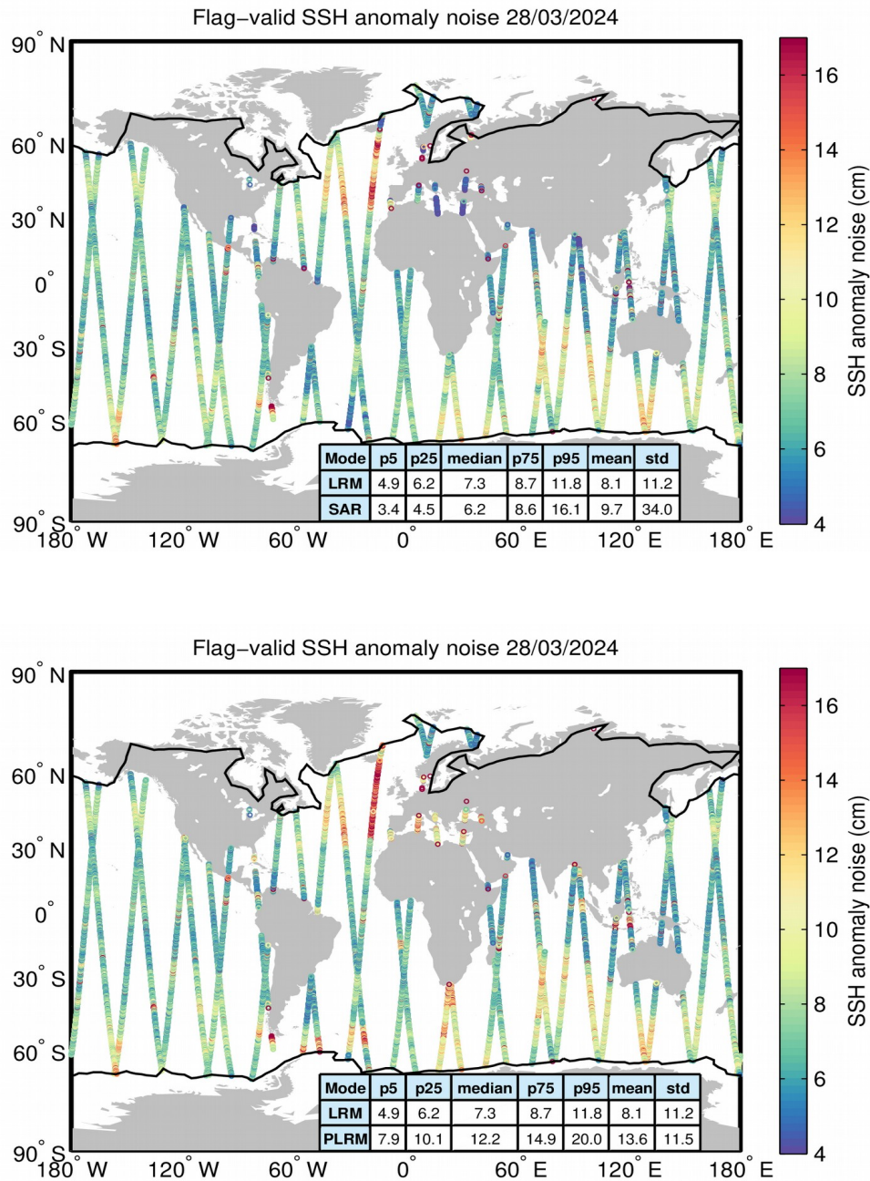
Figure 8. Geographical distribution of flag-valid 20-Hz SSH anomaly measurement noise over oceans and lakes for LRM/SAR (top) and LRM/PLRM (bottom) and for 28/03/2024. The statistical values shown in the tables refer to the SSH anomaly noise and are calculated separately for LRM and SAR/PLRM regions. Measurements taken over polar polygons have been excluded from the computation of the statistical values. The black lines mark the outer limit of the Arctic and Antarctic polar polygons.
