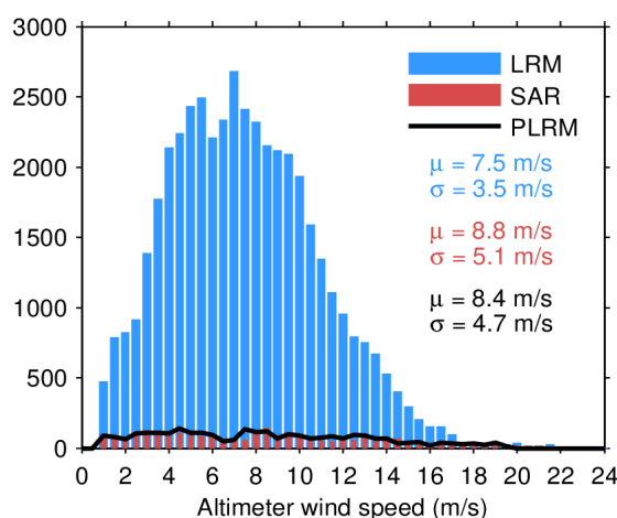
Figure 33. Histogram of flag-valid wind over oceans and lakes for LRM (blue), SAR (red), and PLRM (black) for 28/03/2024. The mean ( \mu ) and standard deviation ( \sigma ) are also shown. Note that values larger than 24 m/s are excluded from the histogram for the sake of readability but not from the computation of \mu and \sigma .
