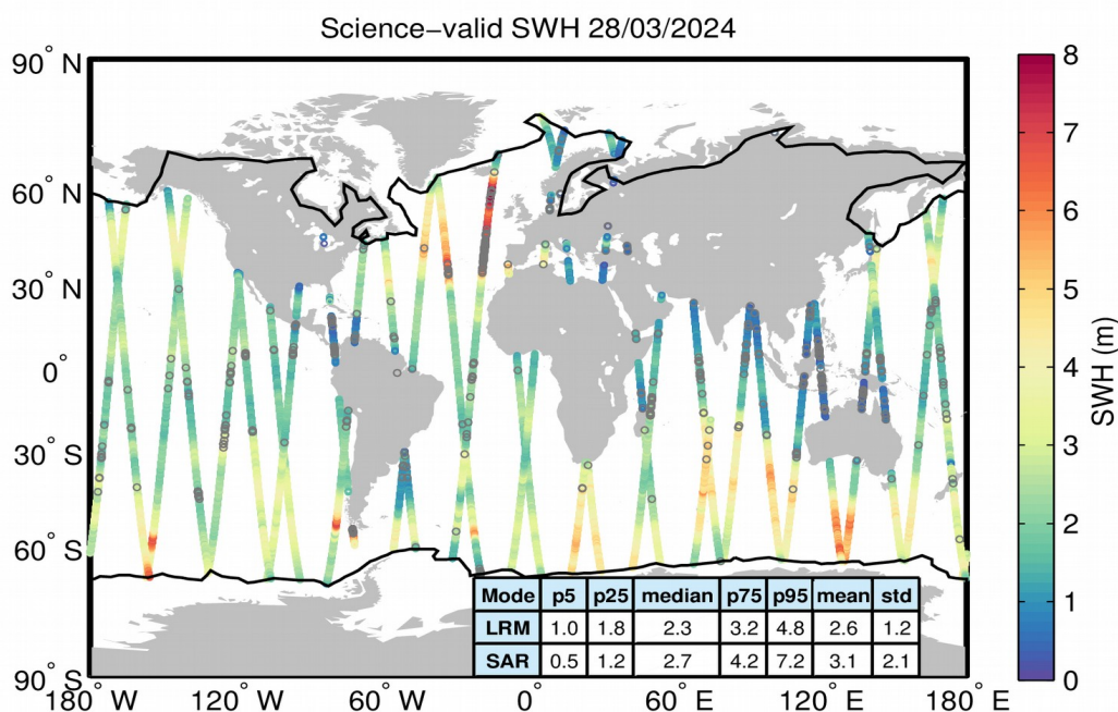
Figure 19. Geographical distribution of science-valid SWH data over oceans and lakes for 28/03/2024. The statistical values shown in the table refer to the SWH in m and are calculated separately for LRM and SAR regions. The black lines mark the outer limit of the Arctic and Antarctic polar polygons. Gray circles denote records that have been rejected based on the editing criteria described in Table 3.
