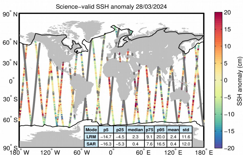
Figure 10. Geographical distribution of science-valid SSH anomaly data over oceans and lakes for 28/03/2024. The statistical values shown in the table refer to the SSH anomaly in cm and are calculated separately for LRM and SAR regions. The black lines mark the
