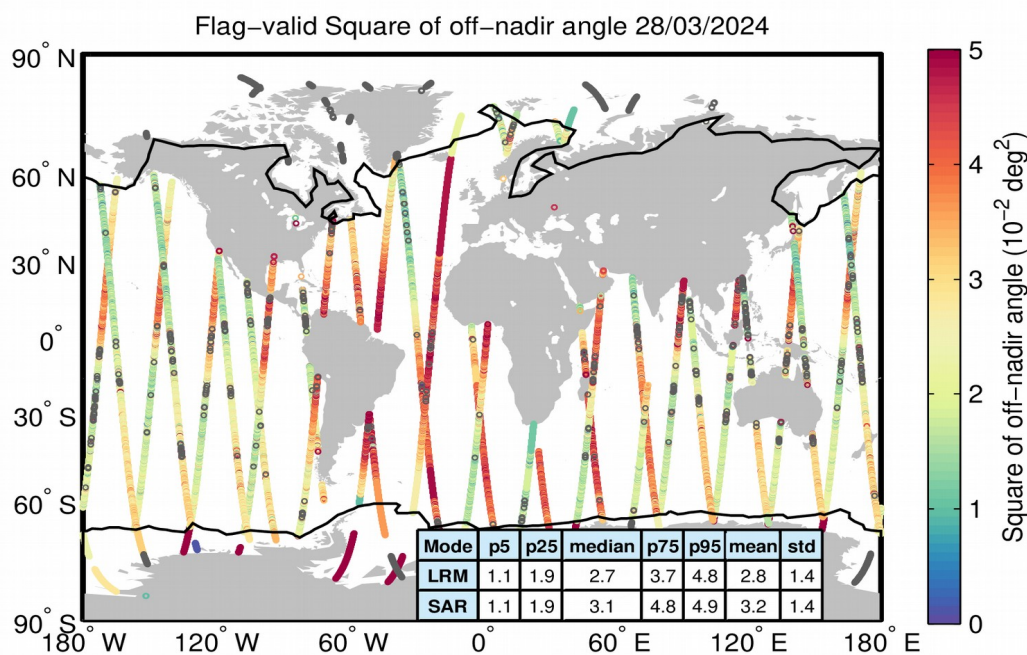
Figure 37. Geographical distribution of flag-valid mispointing data over oceans and lakes for 28/03/2024. The statistical values shown in the table refer to the mispointing in 10^{-2} \text{ deg}^2 and are calculated separately for LRM and SAR regions. Measurements taken over polar polygons have been excluded from the computation of the statistical values. The black lines mark the outer limit of the Arctic and Antarctic polar polygons. Gray circles denote negative values.
