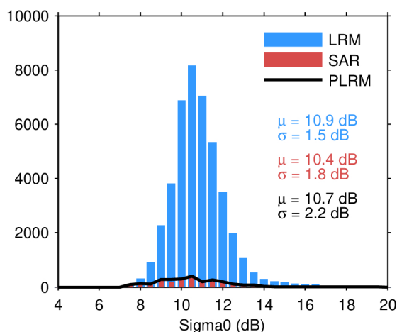
Figure 28. Histogram of science-valid sigma0 over oceans and lakes for LRM (blue), SAR (red), and PLRM (black) for 28/03/2024. The mean ( \mu ) and standard deviation ( \sigma ) are also shown. Note that values outside [4 20] dB are excluded from the histogram for the sake of readability but not from the computation of \mu and \sigma .
