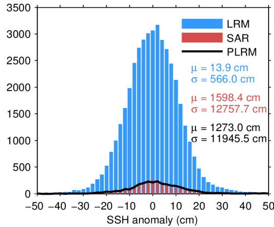
Figure 7. Histogram of flag-valid SSH anomaly over oceans and lakes for LRM (blue), SAR (red), and PLRM (black) for 27/03/2024. The mean ( \mu ) and standard deviation ( \sigma ) are also shown. Note that values outside [-50 50] cm are excluded from the histogram for the sake of readability but not from the computation of \mu and \sigma .
