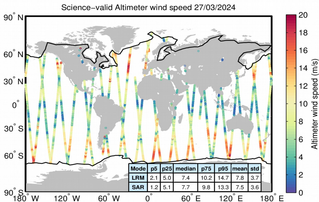
Figure 34. Geographical distribution of science-valid wind data over oceans and lakes for 27/03/2024. The statistical values shown in the table refer to the wind in m/s and are calculated separately for LRM and SAR regions. The black lines mark the outer limit of the Arctic and Antarctic polar polygons. Gray circles denote records that have been rejected based on the editing criteria described in Table 5.
