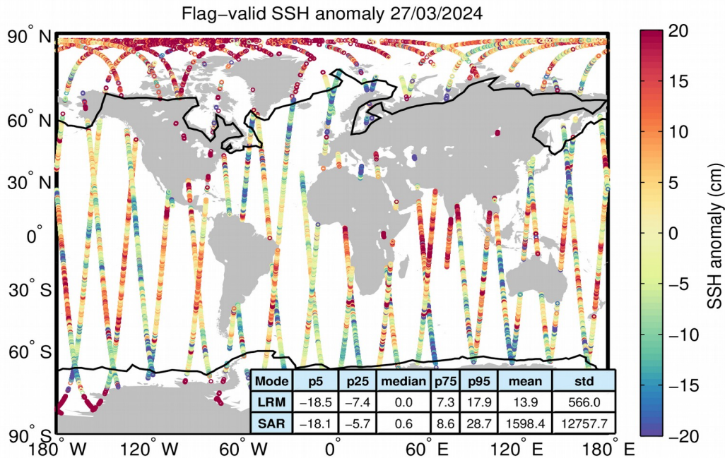
Figure 5. Geographical distribution of flag-valid 1-Hz SSH anomaly data over oceans and lakes for 27/03/2024. The statistical values shown in the table refer to the SSH anomaly in cm and are calculated separately for LRM and SAR regions. Measurements taken over polar polygons have been excluded from the computation of the statistical values. The black lines mark the outer limit of the Arctic and Antarctic polar polygons.
