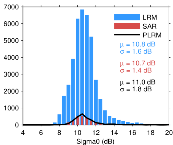
Figure 28. Histogram of science-valid sigma0 over oceans and lakes for LRM (blue), SAR (red), and PLRM (black) for 27/03/2024. The mean ( \mu ) and standard deviation ( \sigma ) are also shown. Note that values outside [4 20] dB are excluded from the histogram for the sake of readability but not from the computation of \mu and \sigma .
