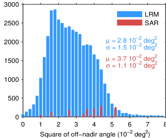
Figure 39. Histogram of flag-valid mispointing over oceans and lakes for LRM (blue) and SAR (red) for 27/03/2024. Only positive values have been considered. The mean ( \mu ) and standard deviation ( \sigma ) are also shown. Note that values larger than 8 \cdot 10^{-2} \text{ deg}^2 are excluded from the histogram for the sake of readability but not from the computation of \mu and \sigma .
