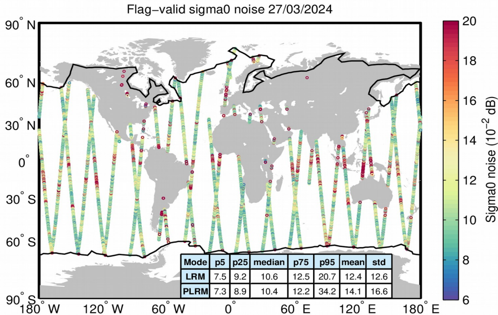
Figure 26. Geographical distribution of flag-valid 20-Hz sigma0 measurement noise over oceans and lakes for LRM/SAR (top) and LRM/PLRM (bottom) and for 27/03/2024. The statistical values shown in the table refer to the sigma0 noise and are calculated separately for LRM and SAR/PLRM regions. Measurements taken over polar polygons have been excluded from the computation of the statistical values. The black lines mark the outer limit of the Arctic and Antarctic polar polygons.
