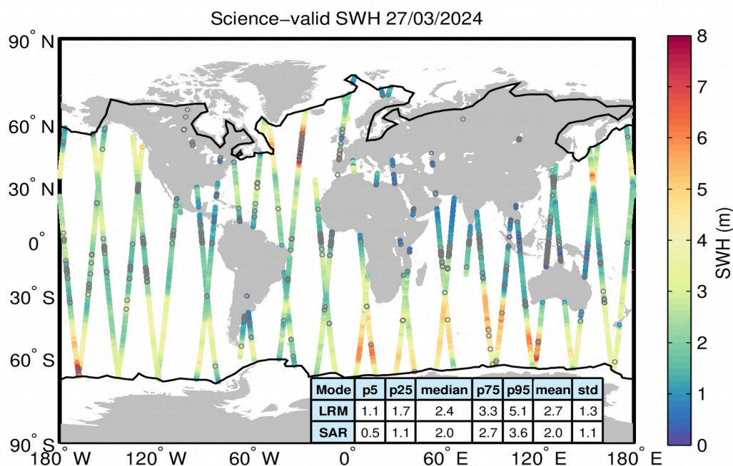
Figure 19. Geographical distribution of science-valid SWH data over oceans and lakes for 27/03/2024. The statistical values shown in the table refer to the SWH in m and are calculated separately for LRM and SAR regions. The black lines mark the outer limit of the Arctic and Antarctic polar polygons. Gray circles denote records that have been rejected based on the editing criteria described in Table 3.
