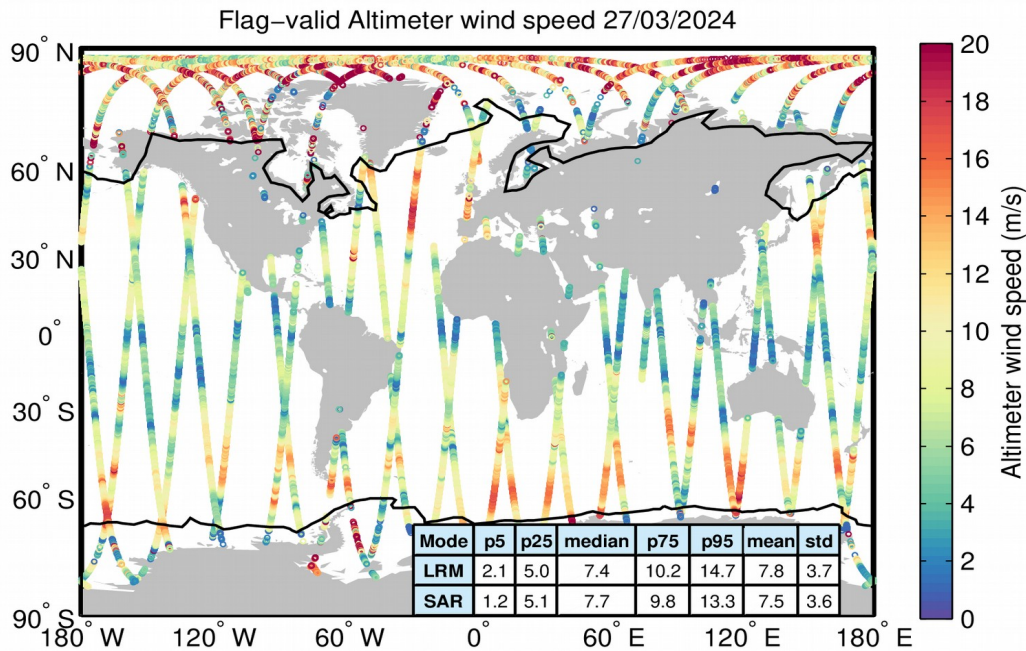
Figure 31. Geographical distribution of flag-valid wind data over oceans and lakes for 27/03/2024. The statistical values shown in the table refer to the wind in m/s and are calculated separately for LRM and SAR regions. Measurements taken over polar polygons have been excluded from the computation of the statistical values. The black lines mark the outer limit of the Arctic and Antarctic polar polygons.
