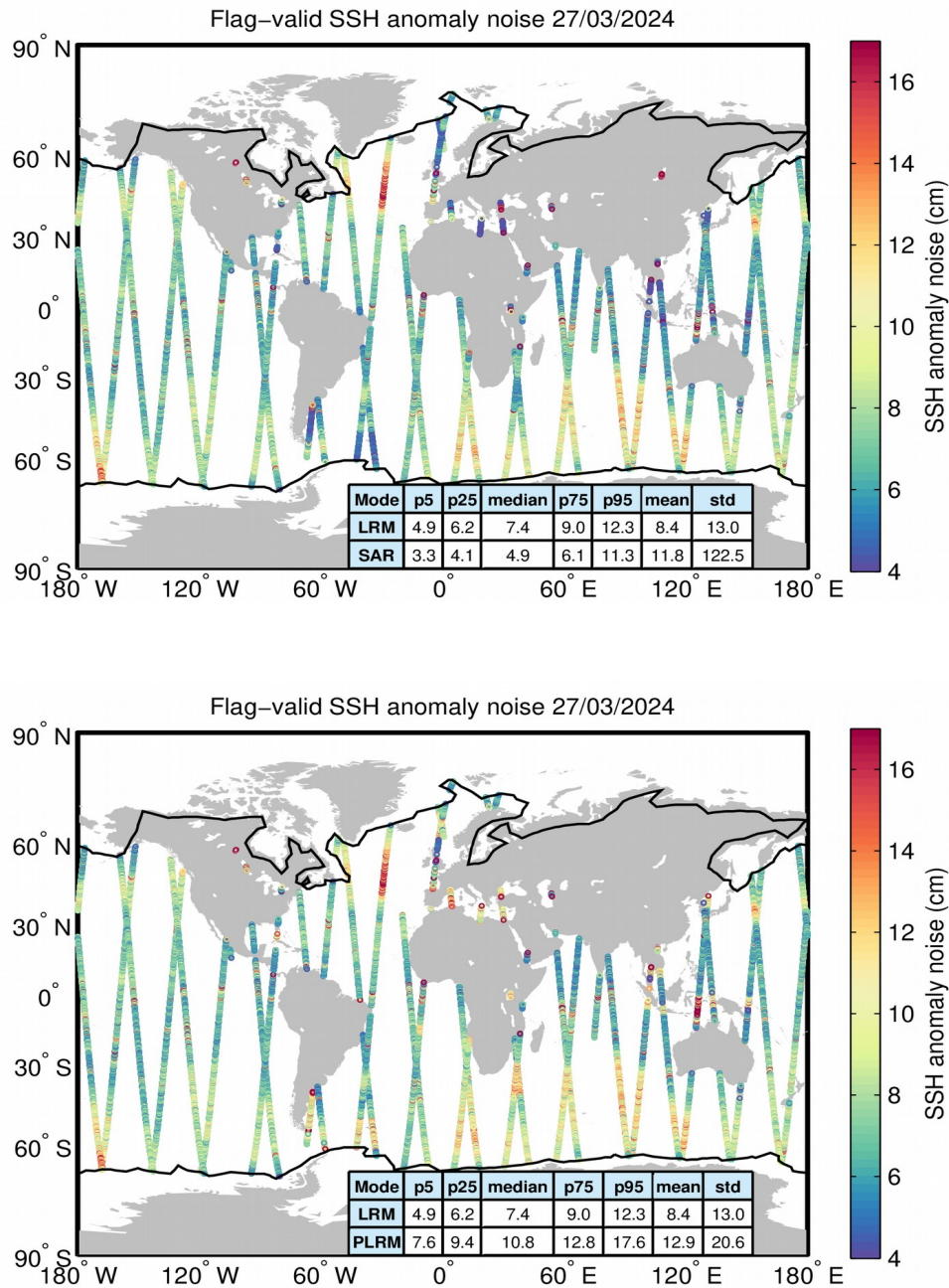
Figure 8. Geographical distribution of flag-valid 20-Hz SSH anomaly measurement noise over oceans and lakes for LRM/SAR (top) and LRM/PLRM (bottom) and for 27/03/2024. The statistical values shown in the tables refer to the SSH anomaly noise and are calculated separately for LRM and SAR/PLRM regions. Measurements taken over polar polygons have been excluded from the computation of the statistical values. The black lines mark the outer limit of the Arctic and Antarctic polar polygons.
