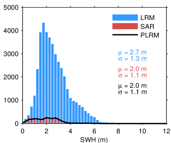
Figure 20. Histogram of science-valid SWH over oceans and lakes for LRM (blue), SAR (red), and PLRM (black) for 27/03/2024. The mean ( \mu ) and standard deviation ( \sigma ) are also
