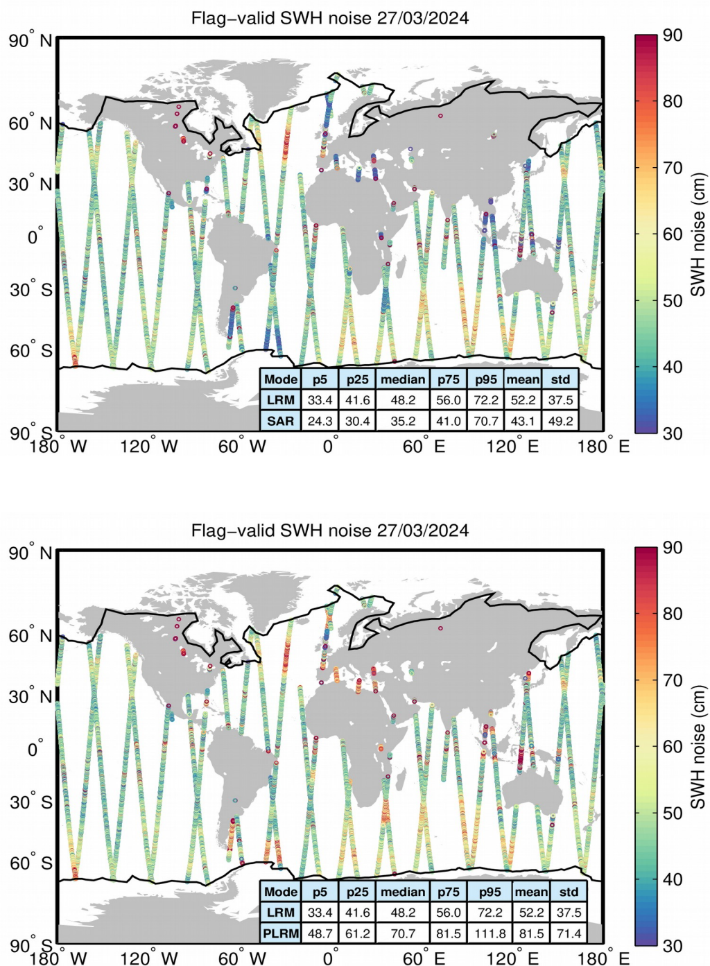
Figure 18. Geographical distribution of flag-valid 20-Hz SWH measurement noise over oceans and lakes for LRM/SAR (top) and LRM/PLRM (bottom) and for 27/03/2024. The statistical values shown in the table refer to the SWH noise and are calculated separately for LRM and SAR/PLRM regions. Measurements taken over polar polygons have been
