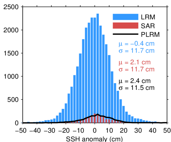
Figure 11. Histogram of science-valid SSH anomaly over oceans and lakes for LRM (blue), SAR (red), and PLRM (black) for 27/03/2024. The mean ( \mu ) and standard deviation ( \sigma ) are also shown. Note that values outside [-50, 50] cm are excluded from the histogram for the sake of readability but not from the computation of \mu and \sigma .
