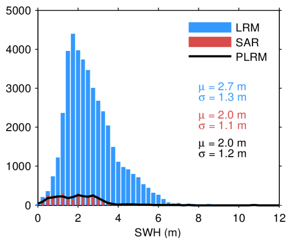
Figure 17. Histogram of flag-valid SWH over oceans and lakes for LRM (blue), SAR (red), and PLRM (black) for 27/03/2024. The mean ( \mu ) and standard deviation ( \sigma ) are also shown. Note that values larger than 12 m are excluded from the histogram for the sake of readability but not from the computation of \mu and \sigma .
