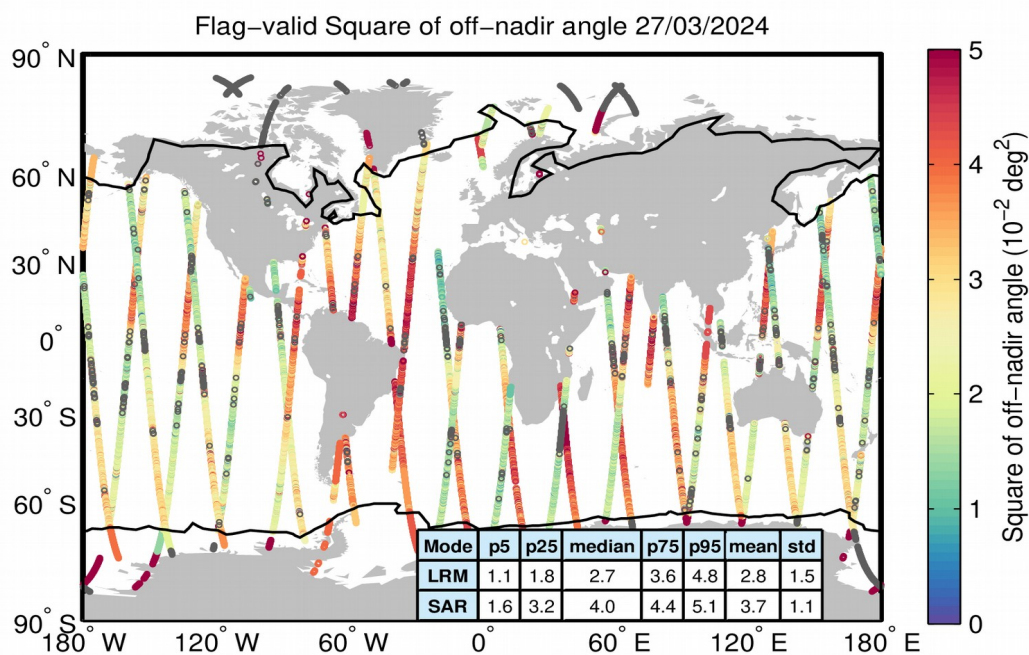
Figure 37. Geographical distribution of flag-valid mispointing data over oceans and lakes for 27/03/2024. The statistical values shown in the table refer to the mispointing in 10^{-2} \text{ deg}^2 and are calculated separately for LRM and SAR regions. Measurements taken over polar polygons have been excluded from the computation of the statistical values. The black lines mark the outer limit of the Arctic and Antarctic polar polygons. Gray circles denote negative values.
