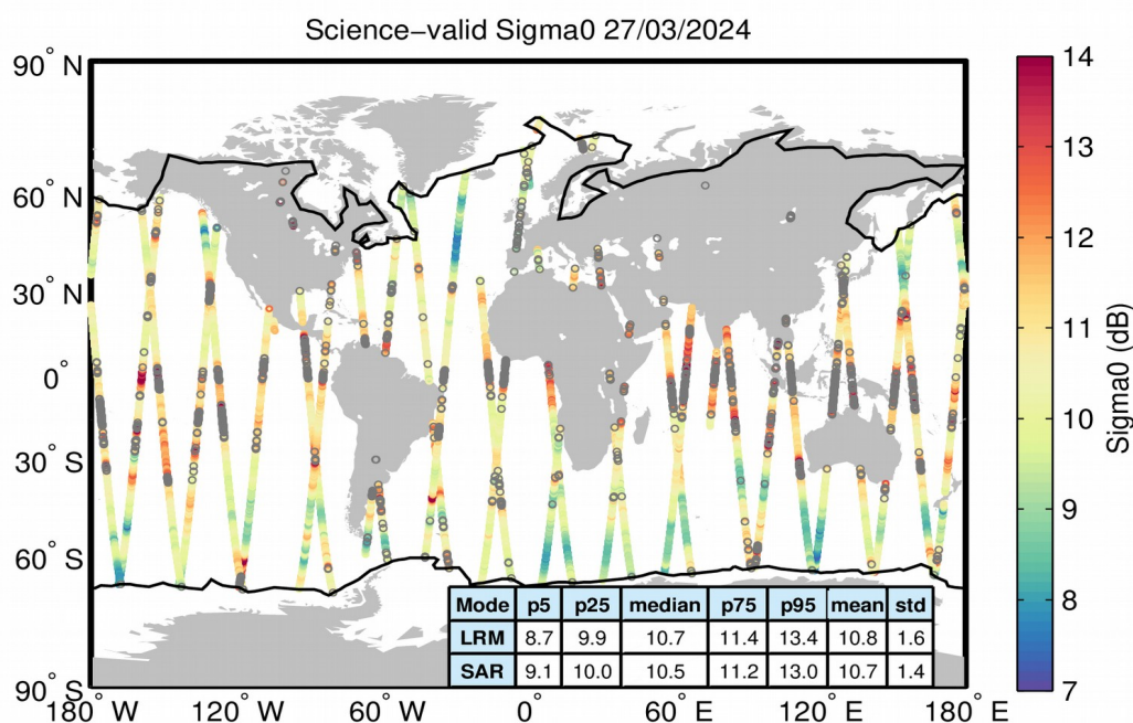
Figure 27. Geographical distribution of science-valid sigma0 data over oceans and lakes for 27/03/2024. The statistical values shown in the table refer to the sigma0 in dB and are calculated separately for LRM and SAR regions. The black lines mark the outer limit of the Arctic and Antarctic polar polygons. Gray circles denote records that have been rejected based on the editing criteria described in Table 4.
