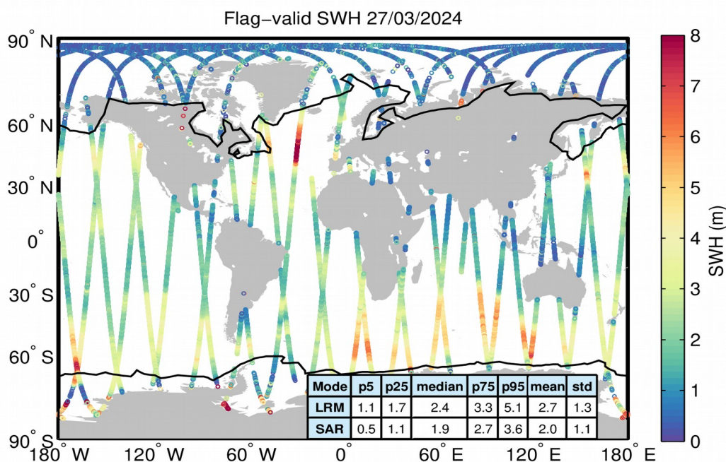
Figure 15. Geographical distribution of flag-valid SWH data over oceans and lakes for 27/03/2024. The statistical values shown in the table refer to the SWH in m and are calculated separately for LRM and SAR regions. Measurements taken over polar polygons have been excluded from the computation of the statistical values. The black lines mark the outer limit of the Arctic and Antarctic polar polygons.
