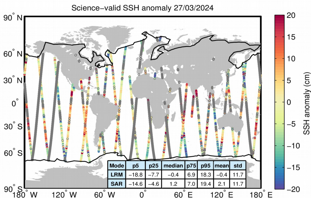
Figure 10. Geographical distribution of science-valid SSH anomaly data over oceans and lakes for 27/03/2024. The statistical values shown in the table refer to the SSH anomaly in cm and are calculated separately for LRM and SAR regions. The black lines mark the
