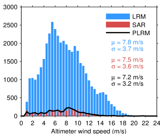
Figure 33. Histogram of flag-valid wind over oceans and lakes for LRM (blue), SAR (red), and PLRM (black) for 27/03/2024. The mean ( \mu ) and standard deviation ( \sigma ) are also shown. Note that values larger than 24 m/s are excluded from the histogram for the sake of readability but not from the computation of \mu and \sigma .
