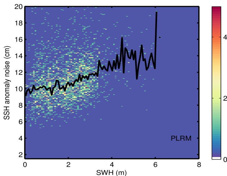
Figure 9. 2D histogram showing flag-valid SSH anomaly noise as a function of SWH for LRM (top), SAR (middle), and PLRM (bottom) for 27/03/2024. The black line denotes the median SSH anomaly noise as a function of SWH.
