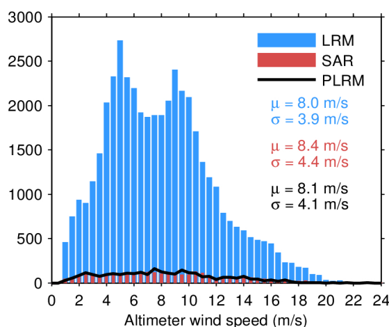
Figure 33. Histogram of flag-valid wind over oceans and lakes for LRM (blue), SAR (red), and PLRM (black) for 26/03/2024. The mean ( \mu ) and standard deviation ( \sigma ) are also shown. Note that values larger than 24 m/s are excluded from the histogram for the sake of readability but not from the computation of \mu and \sigma .
