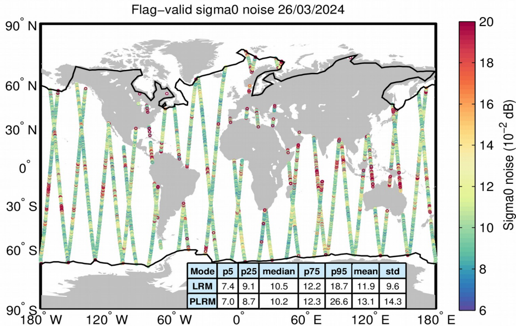
Figure 26. Geographical distribution of flag-valid 20-Hz sigma0 measurement noise over oceans and lakes for LRM/SAR (top) and LRM/PLRM (bottom) and for 26/03/2024. The statistical values shown in the table refer to the sigma0 noise and are calculated separately for LRM and SAR/PLRM regions. Measurements taken over polar polygons have been excluded from the computation of the statistical values. The black lines mark the outer limit of the Arctic and Antarctic polar polygons.
