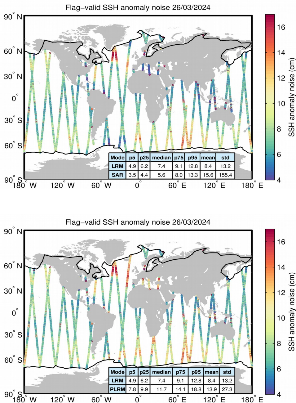
Figure 8. Geographical distribution of flag-valid 20-Hz SSH anomaly measurement noise over oceans and lakes for LRM/SAR (top) and LRM/PLRM (bottom) and for 26/03/2024. The statistical values shown in the tables refer to the SSH anomaly noise and are calculated separately for LRM and SAR/PLRM regions. Measurements taken over polar polygons have been excluded from the computation of the statistical values. The black lines mark the outer limit of the Arctic and Antarctic polar polygons.
