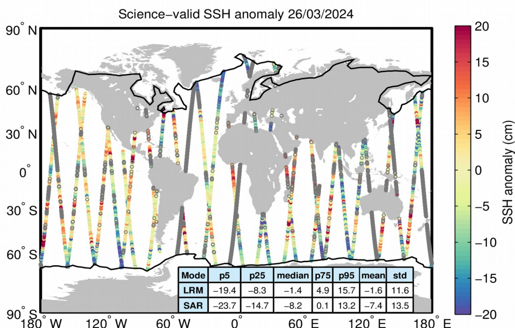
Figure 10. Geographical distribution of science-valid SSH anomaly data over oceans and lakes for 26/03/2024. The statistical values shown in the table refer to the SSH anomaly in cm and are calculated separately for LRM and SAR regions. The black lines mark the
