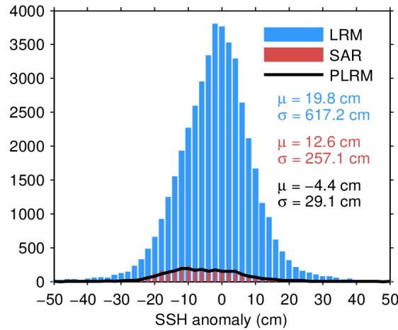
Figure 7. Histogram of flag-valid SSH anomaly over oceans and lakes for LRM (blue), SAR (red), and PLRM (black) for 26/03/2024. The mean ( \mu ) and standard deviation ( \sigma ) are also shown. Note that values outside [-50 50] cm are excluded from the histogram for the sake of readability but not from the computation of \mu and \sigma .
