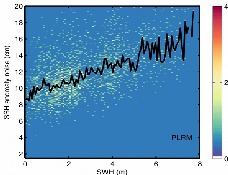
Figure 9. 2D histogram showing flag-valid SSH anomaly noise as a function of SWH for LRM (top), SAR (middle), and PLRM (bottom) for 26/03/2024. The black line denotes the median SSH anomaly noise as a function of SWH.
