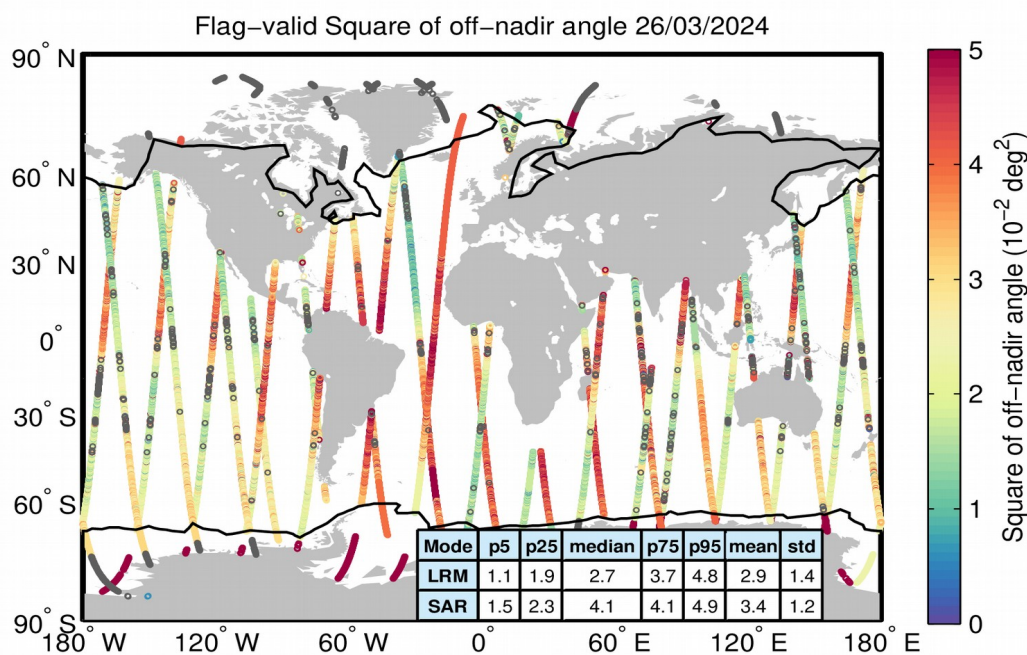
Figure 37. Geographical distribution of flag-valid mispointing data over oceans and lakes for 26/03/2024. The statistical values shown in the table refer to the mispointing in 10^{-2} \text{ deg}^2 and are calculated separately for LRM and SAR regions. Measurements taken over polar polygons have been excluded from the computation of the statistical values. The black lines mark the outer limit of the Arctic and Antarctic polar polygons. Gray circles denote negative values.
