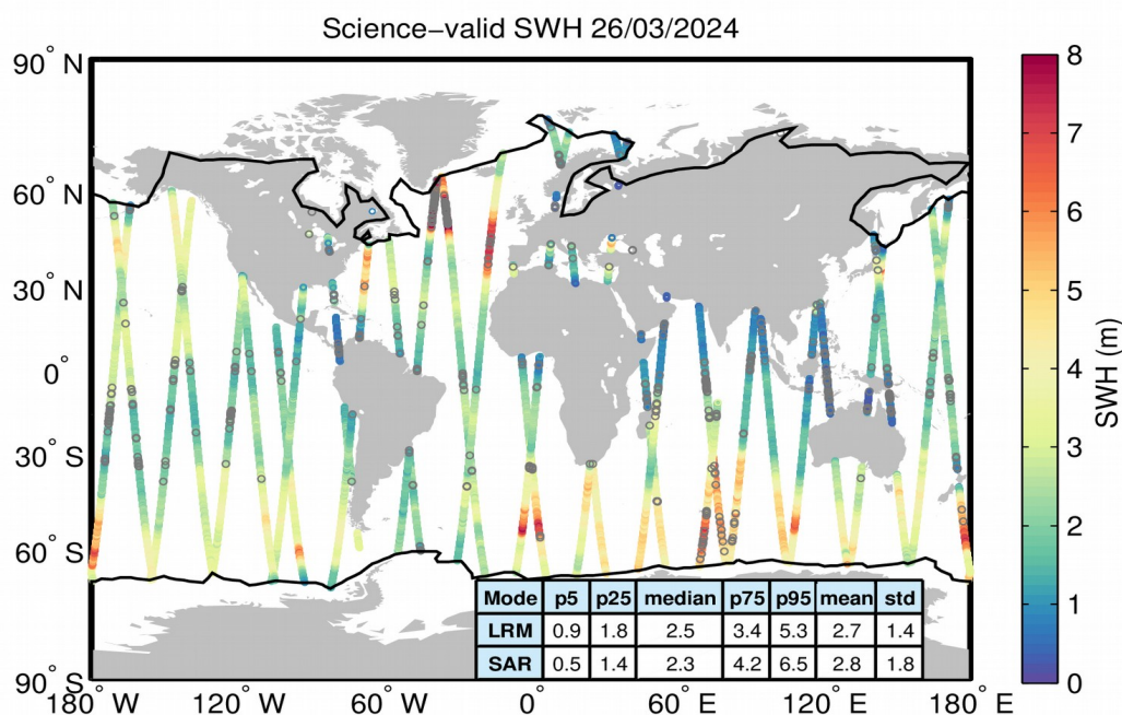
Figure 19. Geographical distribution of science-valid SWH data over oceans and lakes for 26/03/2024. The statistical values shown in the table refer to the SWH in m and are calculated separately for LRM and SAR regions. The black lines mark the outer limit of the Arctic and Antarctic polar polygons. Gray circles denote records that have been rejected based on the editing criteria described in Table 3.
