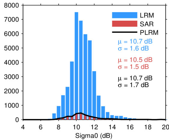
Figure 28. Histogram of science-valid sigma0 over oceans and lakes for LRM (blue), SAR (red), and PLRM (black) for 26/03/2024. The mean ( \mu ) and standard deviation ( \sigma ) are also shown. Note that values outside [4 20] dB are excluded from the histogram for the sake of readability but not from the computation of \mu and \sigma .
