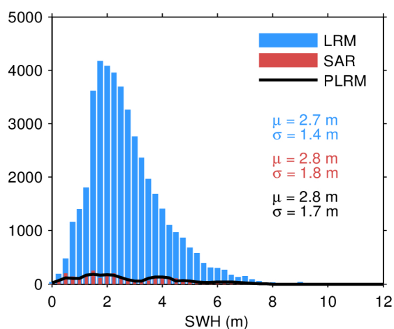
Figure 20. Histogram of science-valid SWH over oceans and lakes for LRM (blue), SAR (red), and PLRM (black) for 26/03/2024. The mean ( \mu ) and standard deviation ( \sigma ) are also
