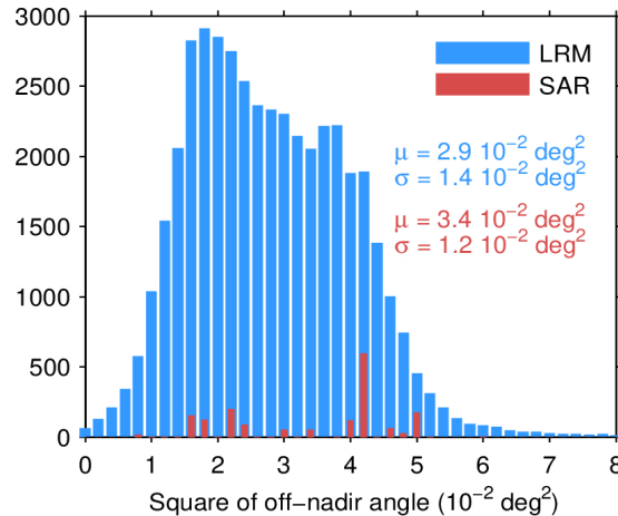
Figure 39. Histogram of flag-valid mispointing over oceans and lakes for LRM (blue) and SAR (red) for 26/03/2024. Only positive values have been considered. The mean ( \mu ) and standard deviation ( \sigma ) are also shown. Note that values larger than 8 \cdot 10^{-2} \text{ deg}^2 are excluded from the histogram for the sake of readability but not from the computation of \mu and \sigma .
