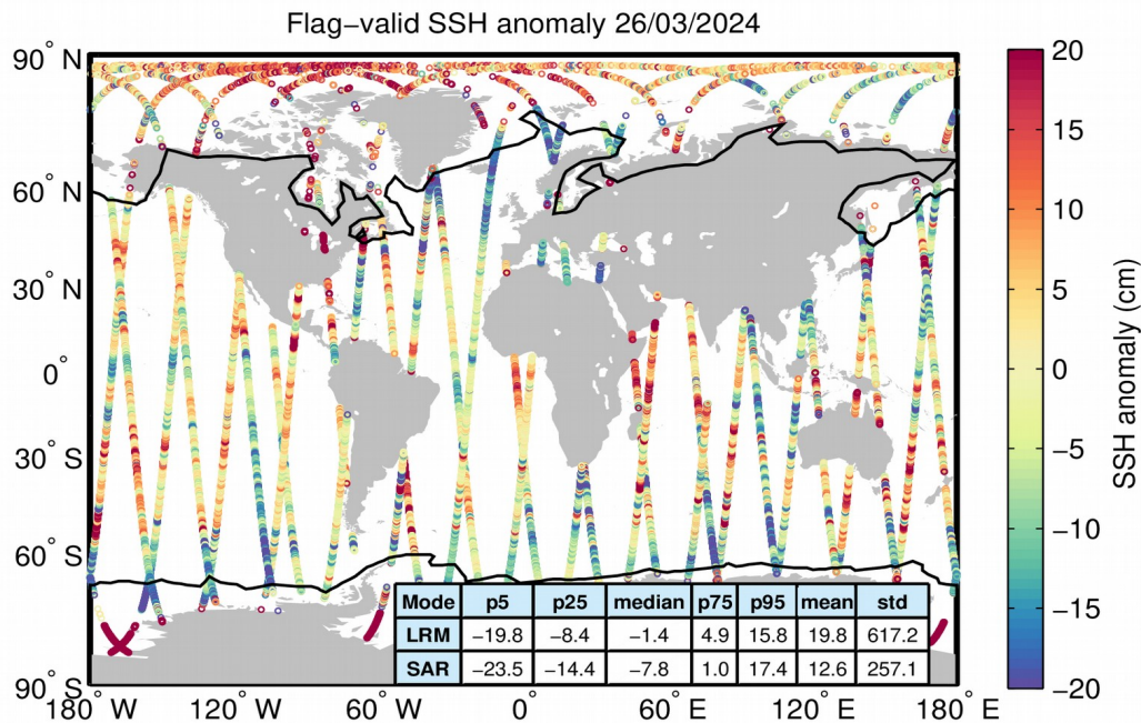
Figure 5. Geographical distribution of flag-valid 1-Hz SSH anomaly data over oceans and lakes for 26/03/2024. The statistical values shown in the table refer to the SSH anomaly in cm and are calculated separately for LRM and SAR regions. Measurements taken over polar polygons have been excluded from the computation of the statistical values. The black lines mark the outer limit of the Arctic and Antarctic polar polygons.
