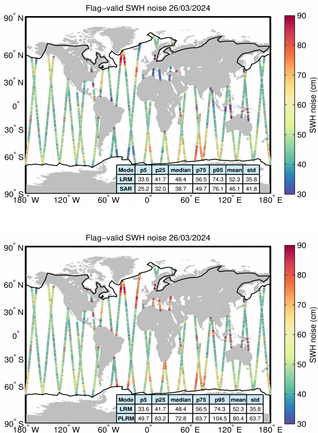
Figure 18. Geographical distribution of flag-valid 20-Hz SWH measurement noise over oceans and lakes for LRM/SAR (top) and LRM/PLRM (bottom) and for 26/03/2024. The statistical values shown in the table refer to the SWH noise and are calculated separately for LRM and SAR/PLRM regions. Measurements taken over polar polygons have been
