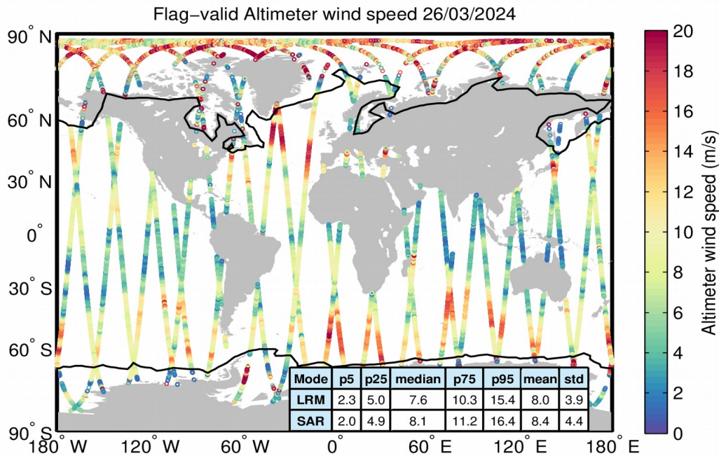
Figure 31. Geographical distribution of flag-valid wind data over oceans and lakes for 26/03/2024. The statistical values shown in the table refer to the wind in m/s and are calculated separately for LRM and SAR regions. Measurements taken over polar polygons have been excluded from the computation of the statistical values. The black lines mark the outer limit of the Arctic and Antarctic polar polygons.
