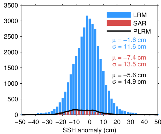
Figure 11. Histogram of science-valid SSH anomaly over oceans and lakes for LRM (blue), SAR (red), and PLRM (black) for 26/03/2024. The mean ( \mu ) and standard deviation ( \sigma ) are also shown. Note that values outside [-50\ 50] cm are excluded from the histogram for the sake of readability but not from the computation of \mu and \sigma .
