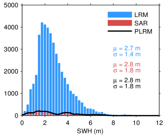
Figure 17. Histogram of flag-valid SWH over oceans and lakes for LRM (blue), SAR (red), and PLRM (black) for 26/03/2024. The mean ( \mu ) and standard deviation ( \sigma ) are also shown. Note that values larger than 12 m are excluded from the histogram for the sake of readability but not from the computation of \mu and \sigma .
