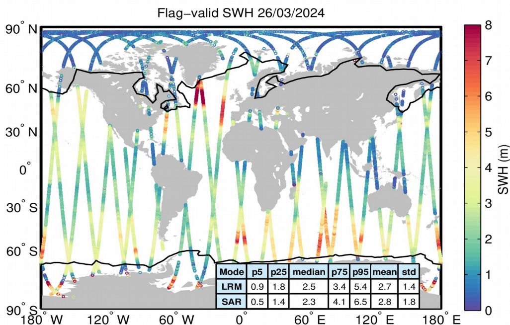
Figure 15. Geographical distribution of flag-valid SWH data over oceans and lakes for 26/03/2024. The statistical values shown in the table refer to the SWH in m and are calculated separately for LRM and SAR regions. Measurements taken over polar polygons have been excluded from the computation of the statistical values. The black lines mark the outer limit of the Arctic and Antarctic polar polygons.
