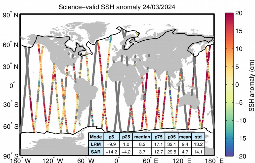
Figure 10. Geographical distribution of science-valid SSH anomaly data over oceans and lakes for 24/03/2024. The statistical values shown in the table refer to the SSH anomaly in cm and are calculated separately for LRM and SAR regions. The black lines mark the
