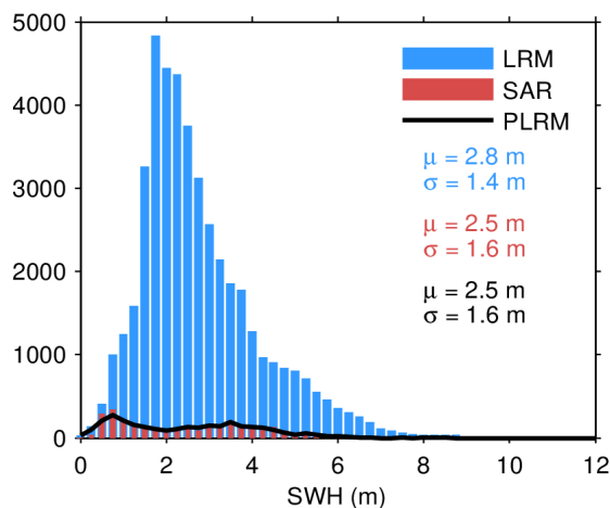
Figure 17. Histogram of flag-valid SWH over oceans and lakes for LRM (blue), SAR (red), and PLRM (black) for 24/03/2024. The mean ( \mu ) and standard deviation ( \sigma ) are also shown. Note that values larger than 12 m are excluded from the histogram for the sake of readability but not from the computation of \mu and \sigma .
