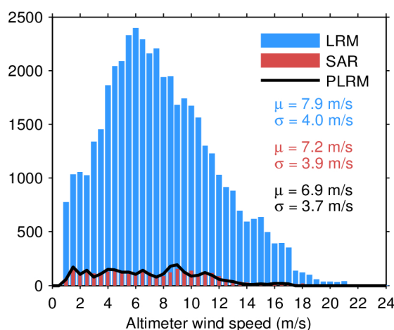
Figure 33. Histogram of flag-valid wind over oceans and lakes for LRM (blue), SAR (red), and PLRM (black) for 24/03/2024. The mean ( \mu ) and standard deviation ( \sigma ) are also shown. Note that values larger than 24 m/s are excluded from the histogram for the sake of readability but not from the computation of \mu and \sigma .
