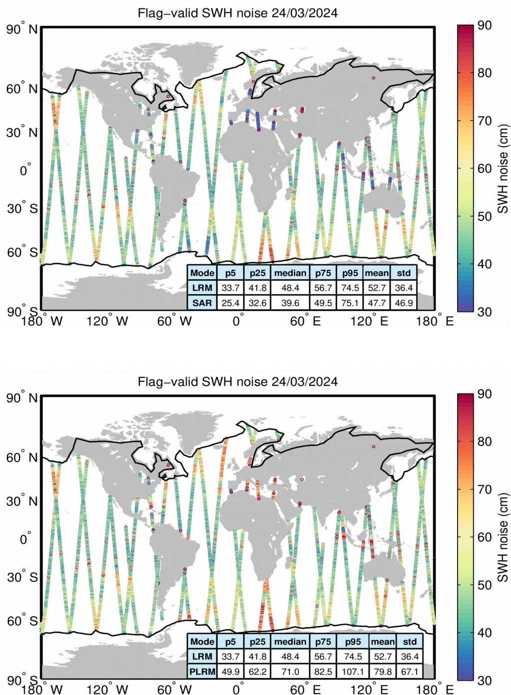
Figure 18. Geographical distribution of flag-valid 20-Hz SWH measurement noise over oceans and lakes for LRM/SAR (top) and LRM/PLRM (bottom) and for 24/03/2024. The statistical values shown in the table refer to the SWH noise and are calculated separately for LRM and SAR/PLRM regions. Measurements taken over polar polygons have been
