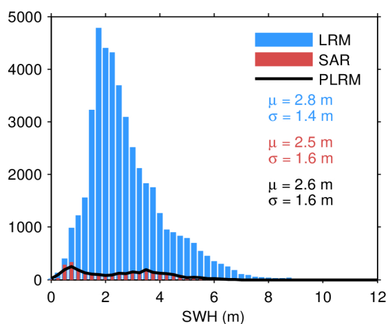
Figure 20. Histogram of science-valid SWH over oceans and lakes for LRM (blue), SAR (red), and PLRM (black) for 24/03/2024. The mean ( \mu ) and standard deviation ( \sigma ) are also
