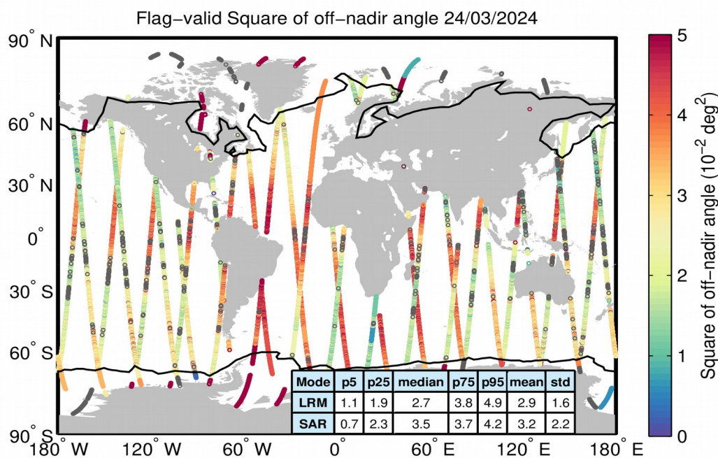
Figure 37. Geographical distribution of flag-valid mispointing data over oceans and lakes for 24/03/2024. The statistical values shown in the table refer to the mispointing in 10^{-2} \text{ deg}^2 and are calculated separately for LRM and SAR regions. Measurements taken over polar polygons have been excluded from the computation of the statistical values. The black lines mark the outer limit of the Arctic and Antarctic polar polygons. Gray circles denote negative values.
