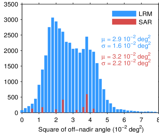
Figure 39. Histogram of flag-valid mispointing over oceans and lakes for LRM (blue) and SAR (red) for 24/03/2024. Only positive values have been considered. The mean ( \mu ) and standard deviation ( \sigma ) are also shown. Note that values larger than 8 \cdot 10^{-2} \text{ deg}^2 are excluded from the histogram for the sake of readability but not from the computation of \mu and \sigma .
