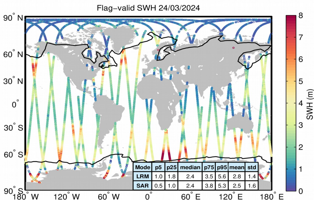
Figure 15. Geographical distribution of flag-valid SWH data over oceans and lakes for 24/03/2024. The statistical values shown in the table refer to the SWH in m and are calculated separately for LRM and SAR regions. Measurements taken over polar polygons have been excluded from the computation of the statistical values. The black lines mark the outer limit of the Arctic and Antarctic polar polygons.
