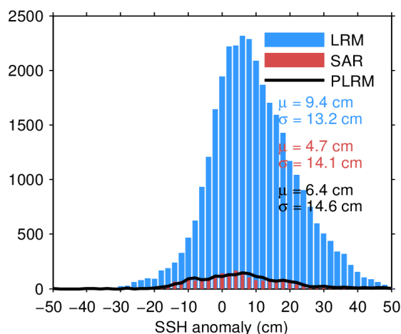
Figure 11. Histogram of science-valid SSH anomaly over oceans and lakes for LRM (blue), SAR (red), and PLRM (black) for 24/03/2024. The mean ( \mu ) and standard deviation ( \sigma ) are also shown. Note that values outside [-50, 50] cm are excluded from the histogram for the sake of readability but not from the computation of \mu and \sigma .
