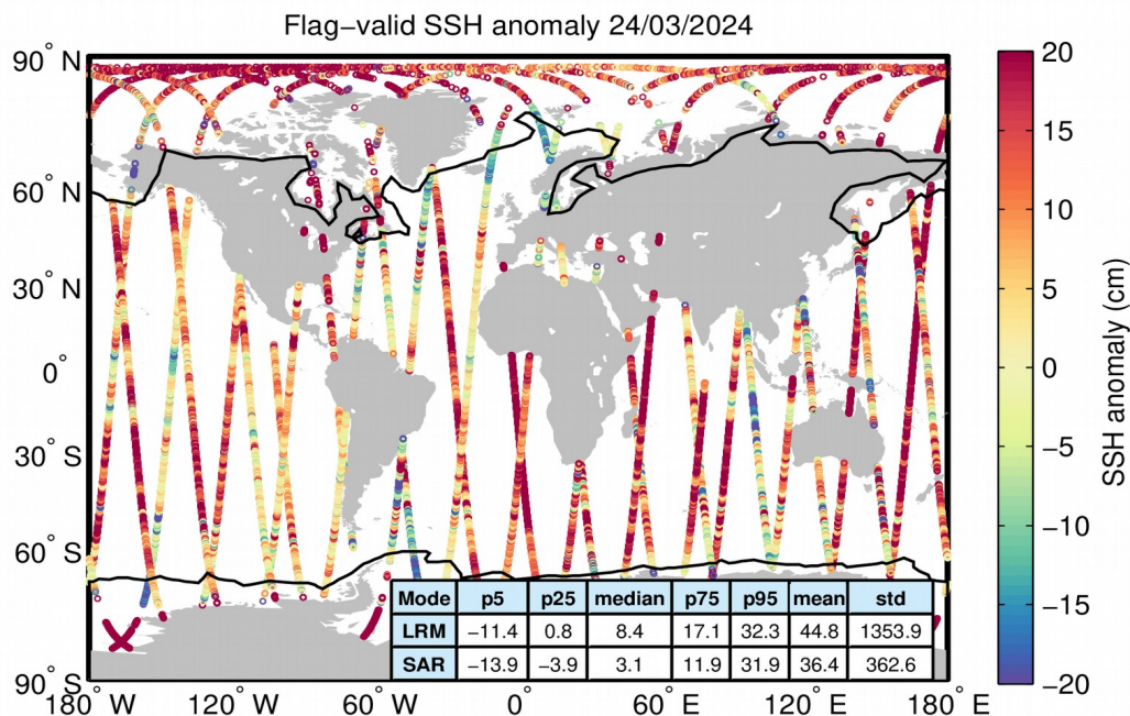
Figure 5. Geographical distribution of flag-valid 1-Hz SSH anomaly data over oceans and lakes for 24/03/2024. The statistical values shown in the table refer to the SSH anomaly in cm and are calculated separately for LRM and SAR regions. Measurements taken over polar polygons have been excluded from the computation of the statistical values. The black lines mark the outer limit of the Arctic and Antarctic polar polygons.
