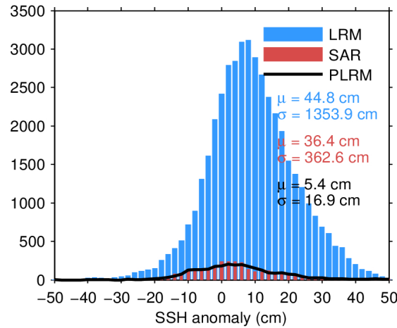
Figure 7. Histogram of flag-valid SSH anomaly over oceans and lakes for LRM (blue), SAR (red), and PLRM (black) for 24/03/2024. The mean ( \mu ) and standard deviation ( \sigma ) are also shown. Note that values outside [-50 50] cm are excluded from the histogram for the sake of readability but not from the computation of \mu and \sigma .
