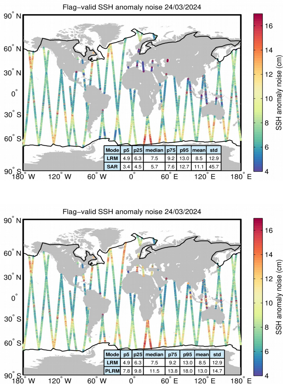
Figure 8. Geographical distribution of flag-valid 20-Hz SSH anomaly measurement noise over oceans and lakes for LRM/SAR (top) and LRM/PLRM (bottom) and for 24/03/2024. The statistical values shown in the tables refer to the SSH anomaly noise and are calculated separately for LRM and SAR/PLRM regions. Measurements taken over polar polygons have been excluded from the computation of the statistical values. The black lines mark the outer limit of the Arctic and Antarctic polar polygons.
