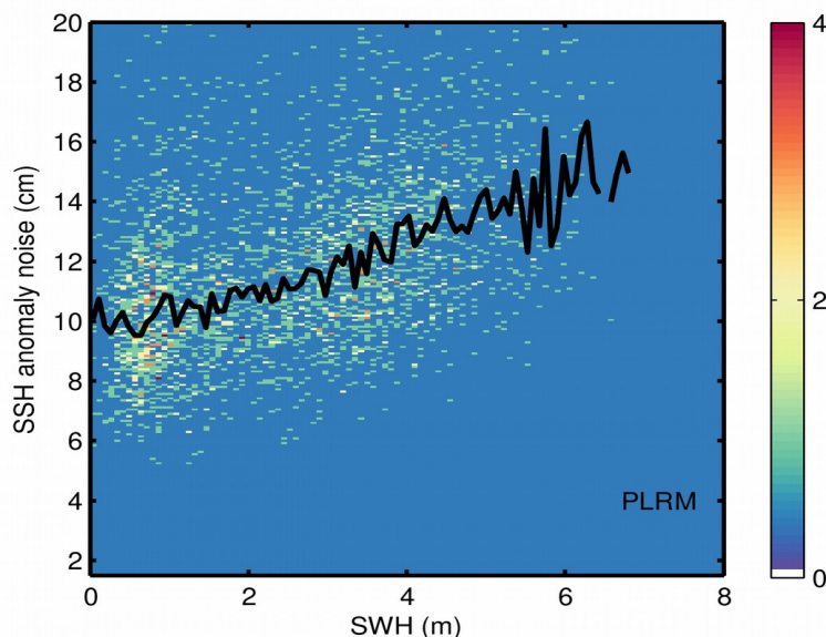
Figure 9. 2D histogram showing flag-valid SSH anomaly noise as a function of SWH for LRM (top), SAR (middle), and PLRM (bottom) for 24/03/2024. The black line denotes the median SSH anomaly noise as a function of SWH.
