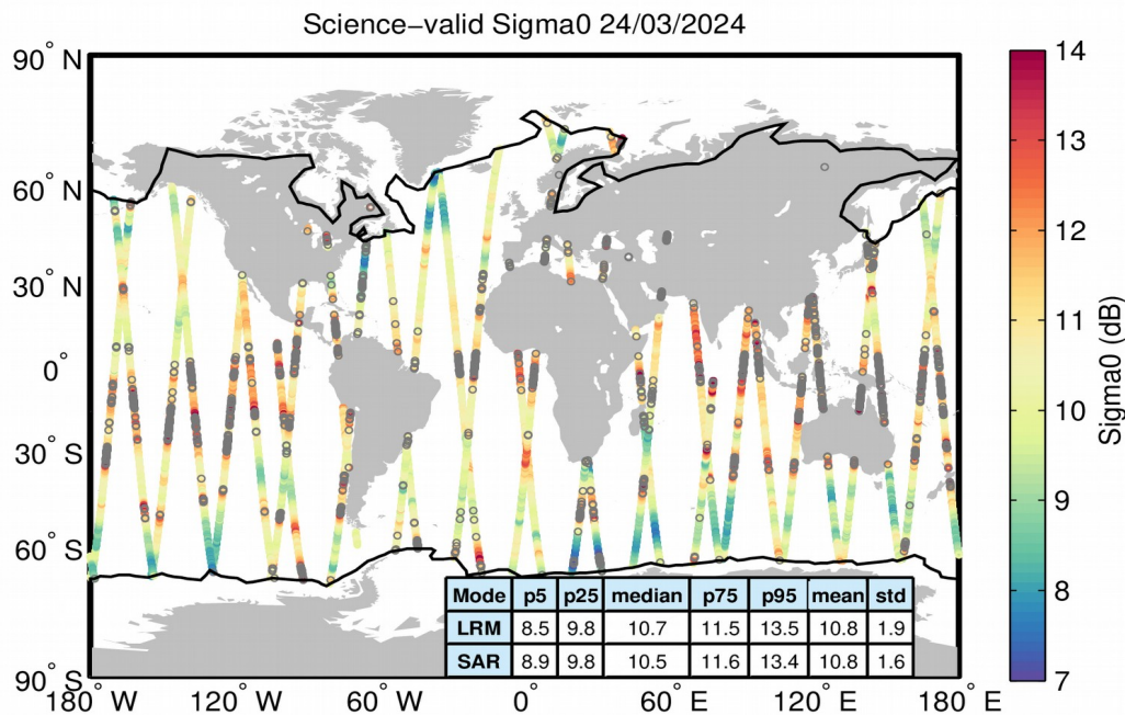
Figure 27. Geographical distribution of science-valid sigma0 data over oceans and lakes for 24/03/2024. The statistical values shown in the table refer to the sigma0 in dB and are calculated separately for LRM and SAR regions. The black lines mark the outer limit of the Arctic and Antarctic polar polygons. Gray circles denote records that have been rejected based on the editing criteria described in Table 4.
