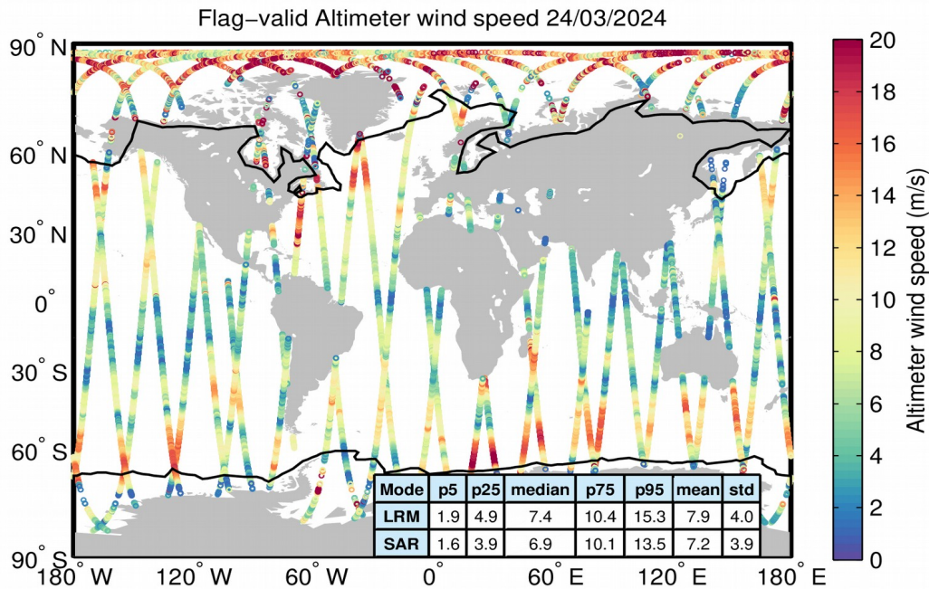
Figure 31. Geographical distribution of flag-valid wind data over oceans and lakes for 24/03/2024. The statistical values shown in the table refer to the wind in m/s and are calculated separately for LRM and SAR regions. Measurements taken over polar polygons have been excluded from the computation of the statistical values. The black lines mark the outer limit of the Arctic and Antarctic polar polygons.
