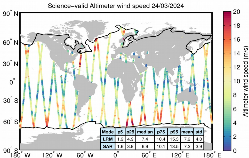
Figure 34. Geographical distribution of science-valid wind data over oceans and lakes for 24/03/2024. The statistical values shown in the table refer to the wind in m/s and are calculated separately for LRM and SAR regions. The black lines mark the outer limit of the Arctic and Antarctic polar polygons. Gray circles denote records that have been rejected based on the editing criteria described in Table 5.
