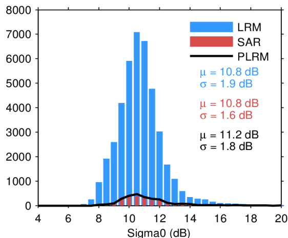
Figure 28. Histogram of science-valid sigma0 over oceans and lakes for LRM (blue), SAR (red), and PLRM (black) for 24/03/2024. The mean ( \mu ) and standard deviation ( \sigma ) are also shown. Note that values outside [4 20] dB are excluded from the histogram for the sake of readability but not from the computation of \mu and \sigma .
