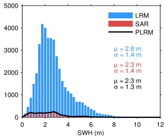
Figure 20. Histogram of science-valid SWH over oceans and lakes for LRM (blue), SAR (red), and PLRM (black) for 23/03/2024. The mean ( \mu ) and standard deviation ( \sigma ) are also
