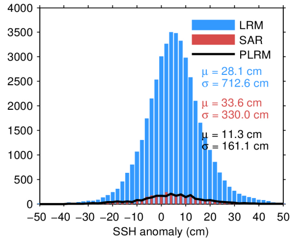
Figure 7. Histogram of flag-valid SSH anomaly over oceans and lakes for LRM (blue), SAR (red), and PLRM (black) for 22/03/2024. The mean ( \mu ) and standard deviation ( \sigma ) are also shown. Note that values outside [-50 50] cm are excluded from the histogram for the sake of readability but not from the computation of \mu and \sigma .
