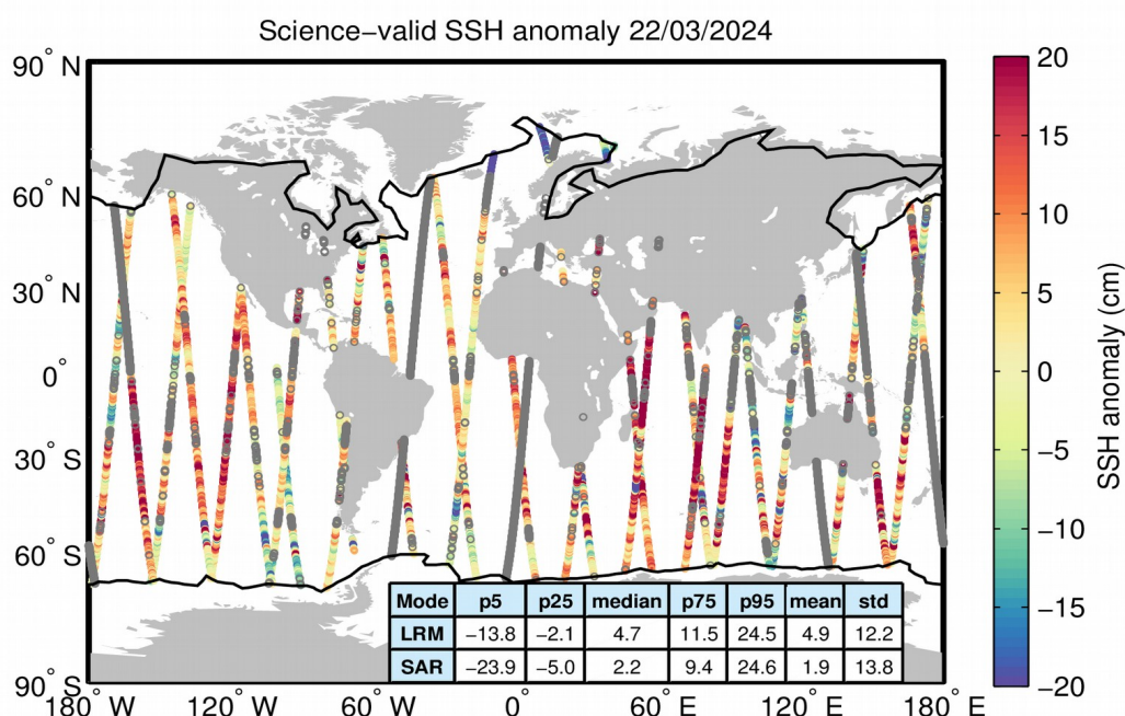
Figure 10. Geographical distribution of science-valid SSH anomaly data over oceans and lakes for 22/03/2024. The statistical values shown in the table refer to the SSH anomaly in cm and are calculated separately for LRM and SAR regions. The black lines mark the
