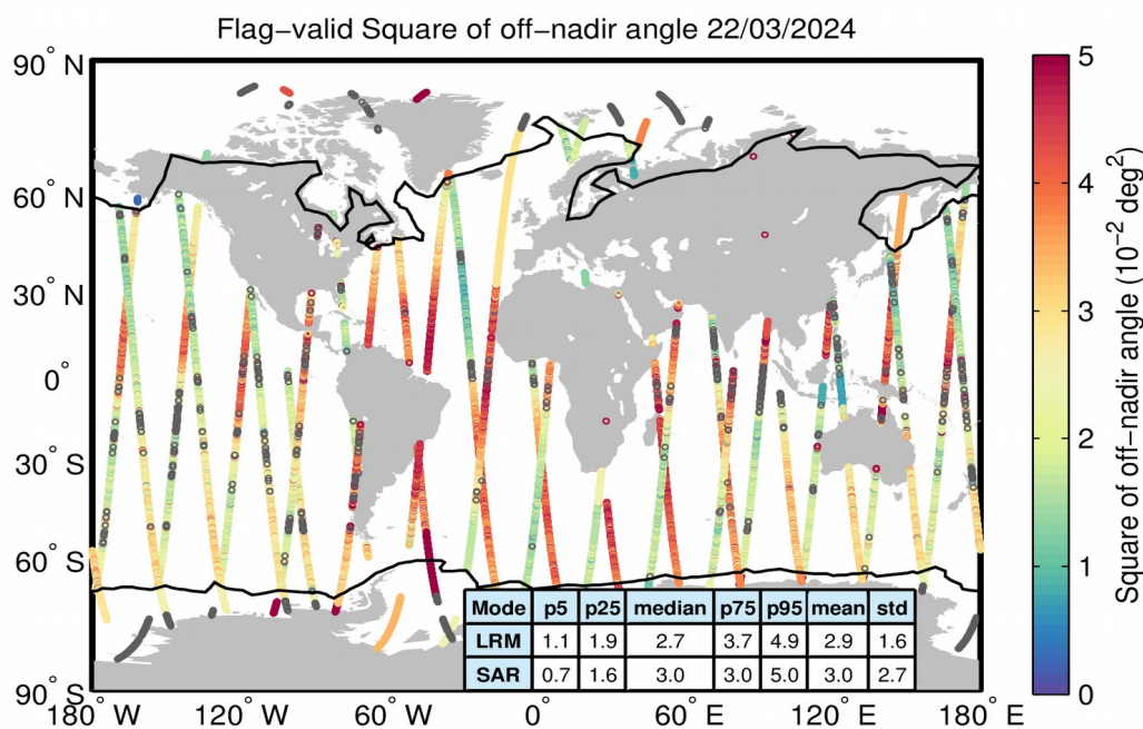
Figure 37. Geographical distribution of flag-valid mispointing data over oceans and lakes for 22/03/2024. The statistical values shown in the table refer to the mispointing in 10^{-2} \text{ deg}^2 and are calculated separately for LRM and SAR regions. Measurements taken over polar polygons have been excluded from the computation of the statistical values. The black lines mark the outer limit of the Arctic and Antarctic polar polygons. Gray circles denote negative values.
