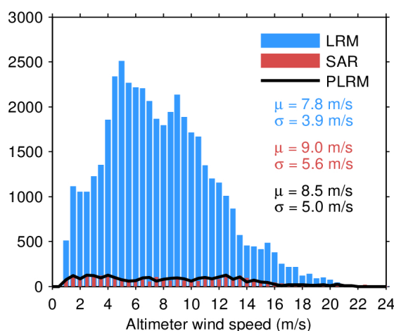
Figure 33. Histogram of flag-valid wind over oceans and lakes for LRM (blue), SAR (red), and PLRM (black) for 22/03/2024. The mean ( \mu ) and standard deviation ( \sigma ) are also shown. Note that values larger than 24 m/s are excluded from the histogram for the sake of readability but not from the computation of \mu and \sigma .
