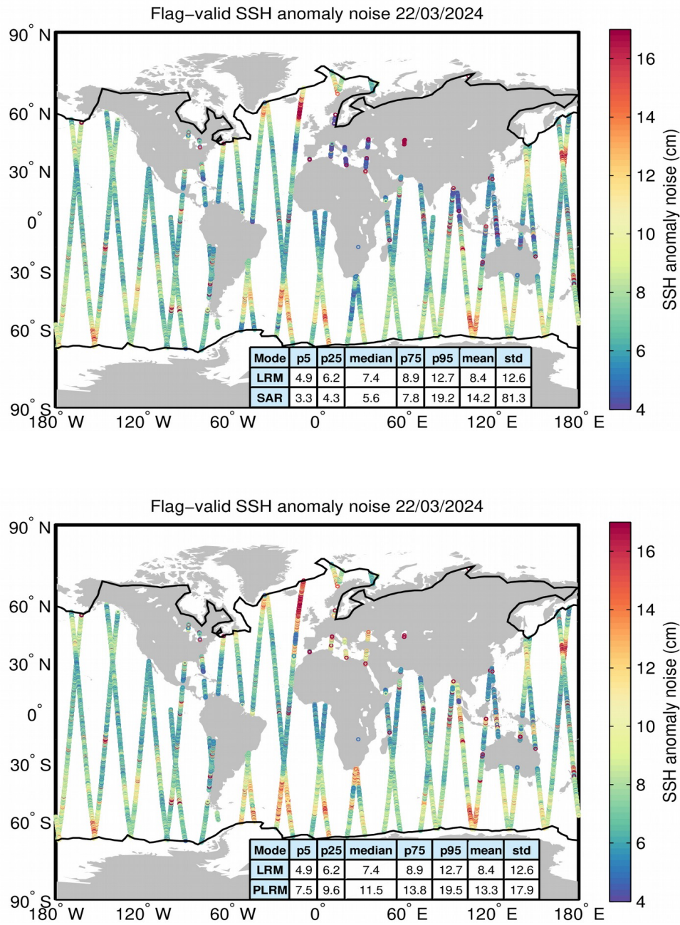
Figure 8. Geographical distribution of flag-valid 20-Hz SSH anomaly measurement noise over oceans and lakes for LRM/SAR (top) and LRM/PLRM (bottom) and for 22/03/2024. The statistical values shown in the tables refer to the SSH anomaly noise and are calculated separately for LRM and SAR/PLRM regions. Measurements taken over polar polygons have been excluded from the computation of the statistical values. The black lines mark the outer limit of the Arctic and Antarctic polar polygons.
