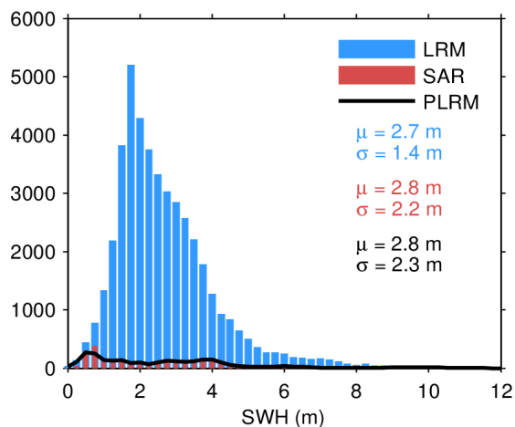
Figure 17. Histogram of flag-valid SWH over oceans and lakes for LRM (blue), SAR (red), and PLRM (black) for 22/03/2024. The mean ( \mu ) and standard deviation ( \sigma ) are also shown. Note that values larger than 12 m are excluded from the histogram for the sake of readability but not from the computation of \mu and \sigma .
