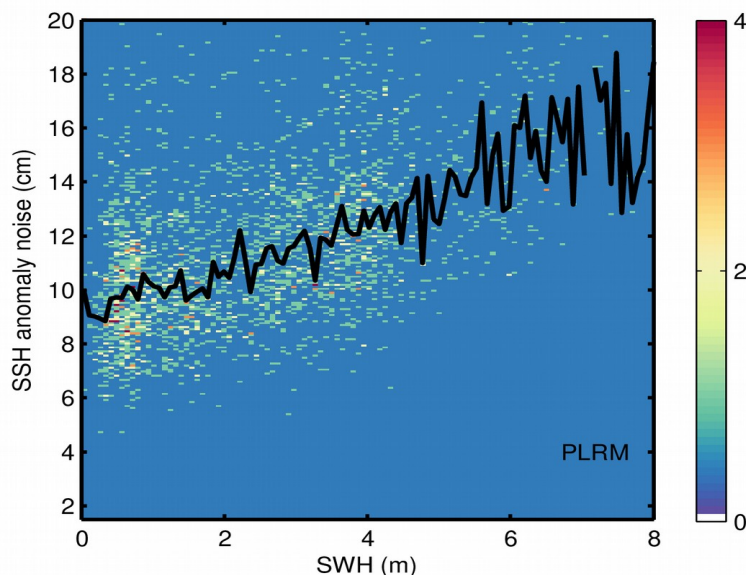
Figure 9. 2D histogram showing flag-valid SSH anomaly noise as a function of SWH for LRM (top), SAR (middle), and PLRM (bottom) for 22/03/2024. The black line denotes the median SSH anomaly noise as a function of SWH.
