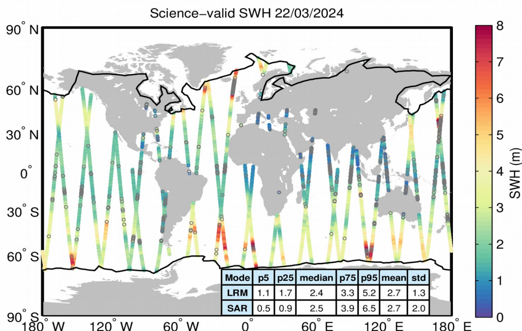
Figure 19. Geographical distribution of science-valid SWH data over oceans and lakes for 22/03/2024. The statistical values shown in the table refer to the SWH in m and are calculated separately for LRM and SAR regions. The black lines mark the outer limit of the Arctic and Antarctic polar polygons. Gray circles denote records that have been rejected based on the editing criteria described in Table 3.
