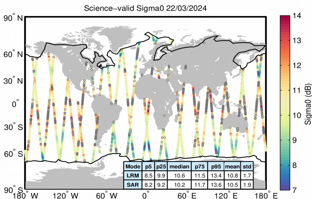
Figure 27. Geographical distribution of science-valid sigma0 data over oceans and lakes for 22/03/2024. The statistical values shown in the table refer to the sigma0 in dB and are calculated separately for LRM and SAR regions. The black lines mark the outer limit of the Arctic and Antarctic polar polygons. Gray circles denote records that have been rejected based on the editing criteria described in Table 4.
