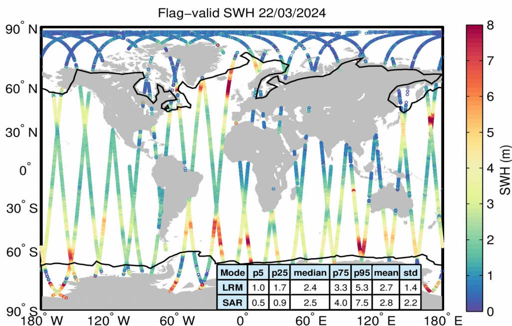
Figure 15. Geographical distribution of flag-valid SWH data over oceans and lakes for 22/03/2024. The statistical values shown in the table refer to the SWH in m and are calculated separately for LRM and SAR regions. Measurements taken over polar polygons have been excluded from the computation of the statistical values. The black lines mark the outer limit of the Arctic and Antarctic polar polygons.
