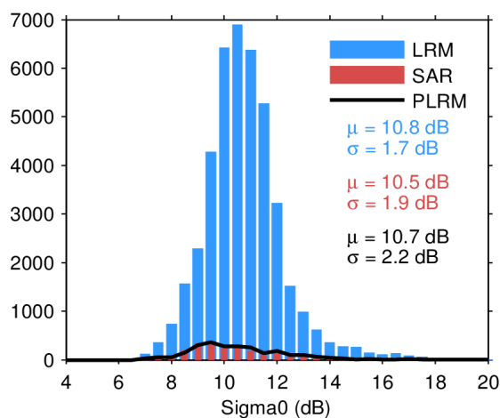
Figure 28. Histogram of science-valid sigma0 over oceans and lakes for LRM (blue), SAR (red), and PLRM (black) for 22/03/2024. The mean ( \mu ) and standard deviation ( \sigma ) are also shown. Note that values outside [4 20] dB are excluded from the histogram for the sake of readability but not from the computation of \mu and \sigma .
