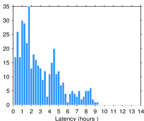
Figure 2. Histogram of the data latency for 22/03/2024. The y-axis denotes the number of files that are made available with a delay of x-hours with respect to the mean time of the records stored in the file.
