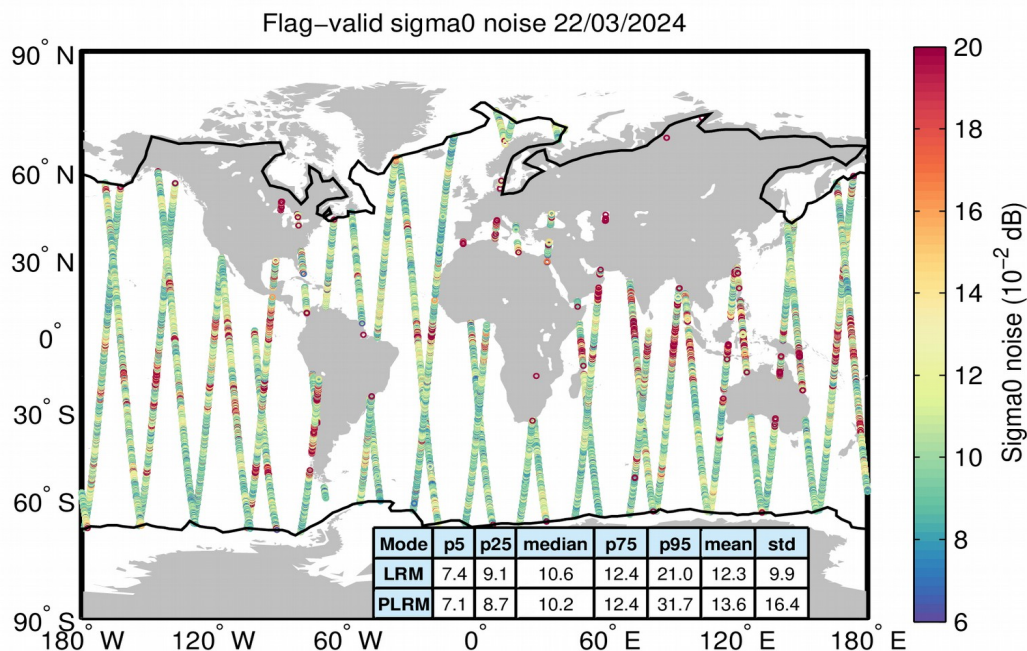
Figure 26. Geographical distribution of flag-valid 20-Hz sigma0 measurement noise over oceans and lakes for LRM/SAR (top) and LRM/PLRM (bottom) and for 22/03/2024. The statistical values shown in the table refer to the sigma0 noise and are calculated separately for LRM and SAR/PLRM regions. Measurements taken over polar polygons have been excluded from the computation of the statistical values. The black lines mark the outer limit of the Arctic and Antarctic polar polygons.
