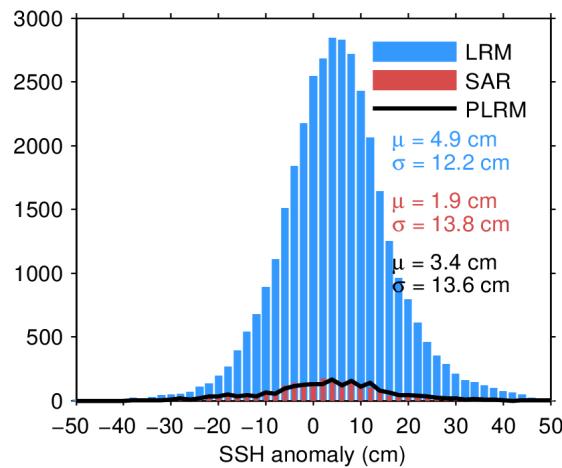
Figure 11. Histogram of science-valid SSH anomaly over oceans and lakes for LRM (blue), SAR (red), and PLRM (black) for 22/03/2024. The mean ( \mu ) and standard deviation ( \sigma ) are also shown. Note that values outside [-50\ 50] cm are excluded from the histogram for the sake of readability but not from the computation of \mu and \sigma .
