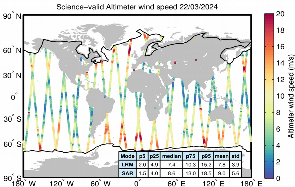
Figure 34. Geographical distribution of science-valid wind data over oceans and lakes for 22/03/2024. The statistical values shown in the table refer to the wind in m/s and are calculated separately for LRM and SAR regions. The black lines mark the outer limit of the Arctic and Antarctic polar polygons. Gray circles denote records that have been rejected based on the editing criteria described in Table 5.
