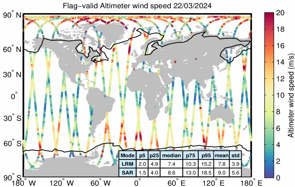
Figure 31. Geographical distribution of flag-valid wind data over oceans and lakes for 22/03/2024. The statistical values shown in the table refer to the wind in m/s and are calculated separately for LRM and SAR regions. Measurements taken over polar polygons have been excluded from the computation of the statistical values. The black lines mark the outer limit of the Arctic and Antarctic polar polygons.
