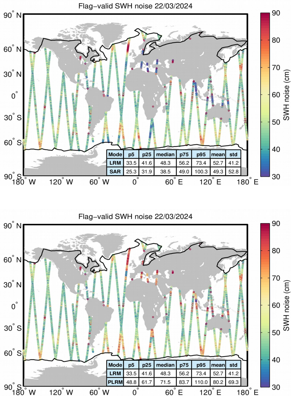
Figure 18. Geographical distribution of flag-valid 20-Hz SWH measurement noise over oceans and lakes for LRM/SAR (top) and LRM/PLRM (bottom) and for 22/03/2024. The statistical values shown in the table refer to the SWH noise and are calculated separately for LRM and SAR/PLRM regions. Measurements taken over polar polygons have been
