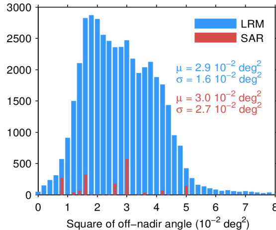
Figure 39. Histogram of flag-valid mispointing over oceans and lakes for LRM (blue) and SAR (red) for 22/03/2024. Only positive values have been considered. The mean ( \mu ) and standard deviation ( \sigma ) are also shown. Note that values larger than 8 \cdot 10^{-2} \text{ deg}^2 are excluded from the histogram for the sake of readability but not from the computation of \mu and \sigma .
