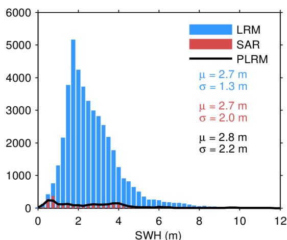
Figure 20. Histogram of science-valid SWH over oceans and lakes for LRM (blue), SAR (red), and PLRM (black) for 22/03/2024. The mean ( \mu ) and standard deviation ( \sigma ) are also
