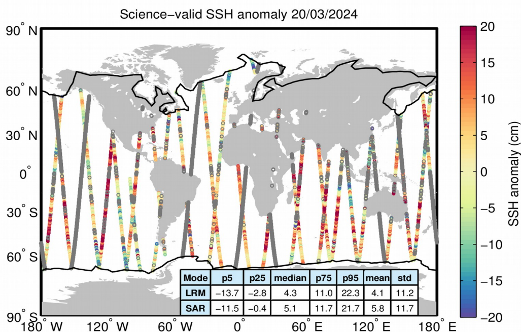
Figure 10. Geographical distribution of science-valid SSH anomaly data over oceans and lakes for 20/03/2024. The statistical values shown in the table refer to the SSH anomaly in cm and are calculated separately for LRM and SAR regions. The black lines mark the
