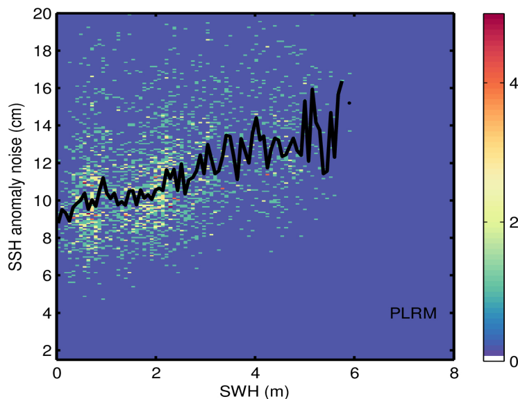
Figure 9. 2D histogram showing flag-valid SSH anomaly noise as a function of SWH for LRM (top), SAR (middle), and PLRM (bottom) for 20/03/2024. The black line denotes the median SSH anomaly noise as a function of SWH.
