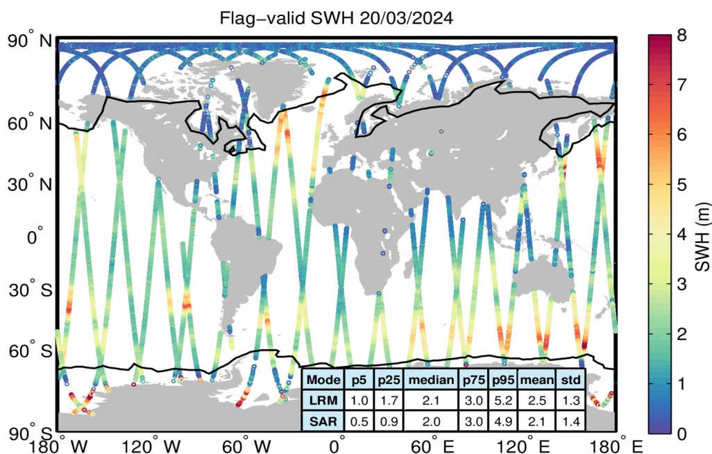
Figure 15. Geographical distribution of flag-valid SWH data over oceans and lakes for 20/03/2024. The statistical values shown in the table refer to the SWH in m and are calculated separately for LRM and SAR regions. Measurements taken over polar polygons have been excluded from the computation of the statistical values. The black lines mark the outer limit of the Arctic and Antarctic polar polygons.
