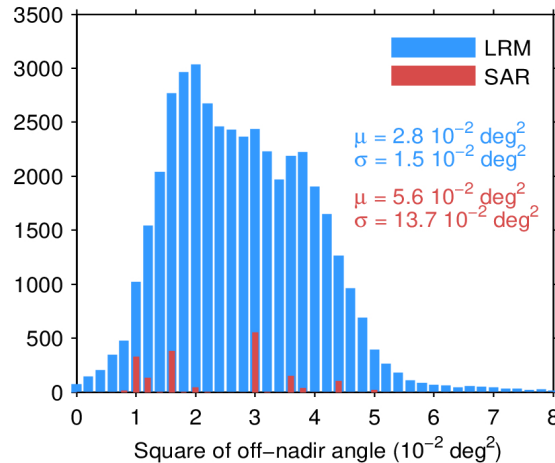
Figure 39. Histogram of flag-valid mispointing over oceans and lakes for LRM (blue) and SAR (red) for 20/03/2024. Only positive values have been considered. The mean ( \mu ) and standard deviation ( \sigma ) are also shown. Note that values larger than 8 \cdot 10^{-2} \text{ deg}^2 are excluded from the histogram for the sake of readability but not from the computation of \mu and \sigma .
