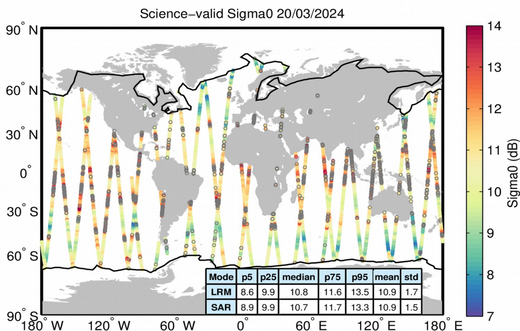
Figure 27. Geographical distribution of science-valid sigma0 data over oceans and lakes for 20/03/2024. The statistical values shown in the table refer to the sigma0 in dB and are calculated separately for LRM and SAR regions. The black lines mark the outer limit of the Arctic and Antarctic polar polygons. Gray circles denote records that have been rejected based on the editing criteria described in Table 4.
