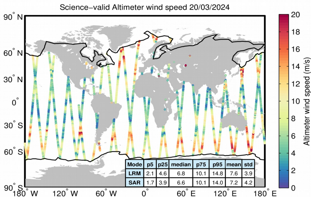
Figure 34. Geographical distribution of science-valid wind data over oceans and lakes for 20/03/2024. The statistical values shown in the table refer to the wind in m/s and are calculated separately for LRM and SAR regions. The black lines mark the outer limit of the Arctic and Antarctic polar polygons. Gray circles denote records that have been rejected based on the editing criteria described in Table 5.
