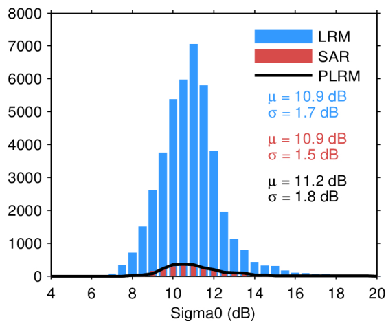
Figure 28. Histogram of science-valid sigma0 over oceans and lakes for LRM (blue), SAR (red), and PLRM (black) for 20/03/2024. The mean ( \mu ) and standard deviation ( \sigma ) are also shown. Note that values outside [4 20] dB are excluded from the histogram for the sake of readability but not from the computation of \mu and \sigma .
