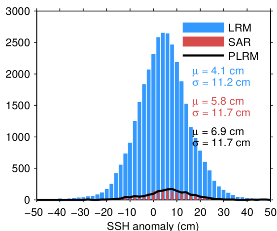
Figure 11. Histogram of science-valid SSH anomaly over oceans and lakes for LRM (blue), SAR (red), and PLRM (black) for 20/03/2024. The mean ( \mu ) and standard deviation ( \sigma ) are also shown. Note that values outside [-50, 50] cm are excluded from the histogram for the sake of readability but not from the computation of \mu and \sigma .
