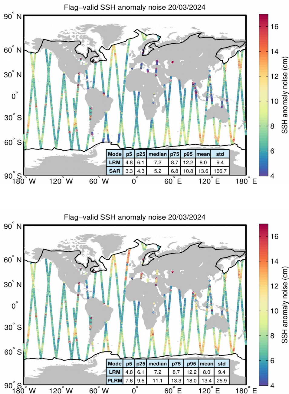
Figure 8. Geographical distribution of flag-valid 20-Hz SSH anomaly measurement noise over oceans and lakes for LRM/SAR (top) and LRM/PLRM (bottom) and for 20/03/2024. The statistical values shown in the tables refer to the SSH anomaly noise and are calculated separately for LRM and SAR/PLRM regions. Measurements taken over polar polygons have been excluded from the computation of the statistical values. The black lines mark the outer limit of the Arctic and Antarctic polar polygons.
