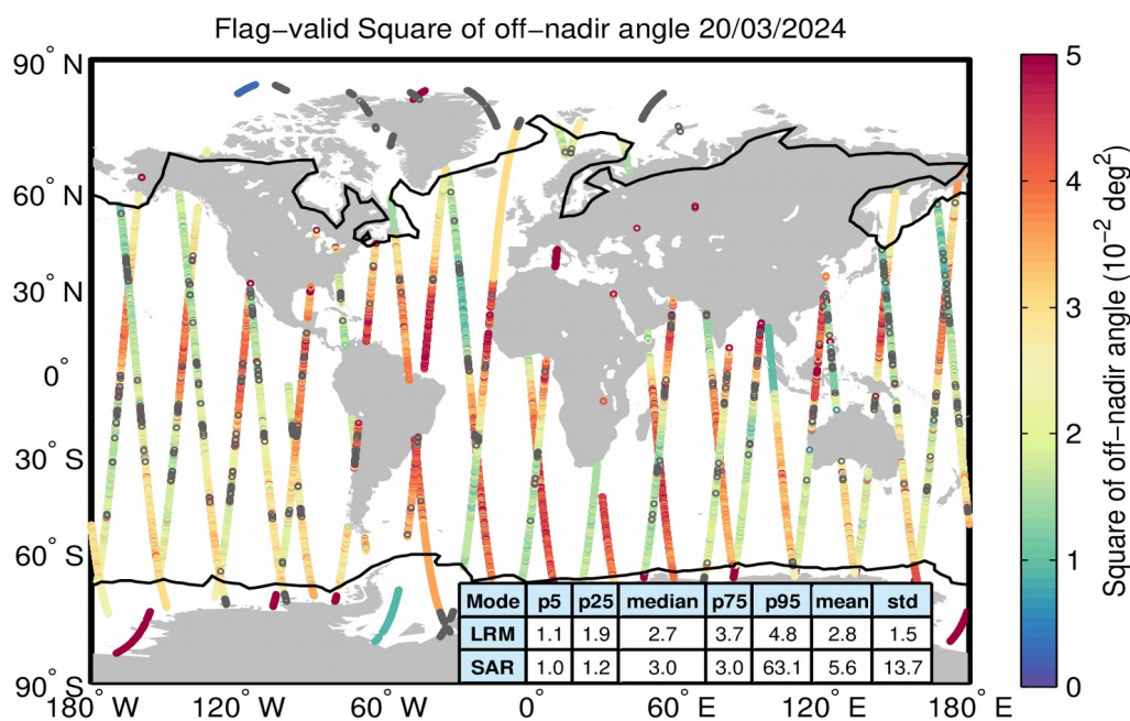
Figure 37. Geographical distribution of flag-valid mispointing data over oceans and lakes for 20/03/2024. The statistical values shown in the table refer to the mispointing in 10^{-2} \text{ deg}^2 and are calculated separately for LRM and SAR regions. Measurements taken over polar polygons have been excluded from the computation of the statistical values. The black lines mark the outer limit of the Arctic and Antarctic polar polygons. Gray circles denote negative values.
