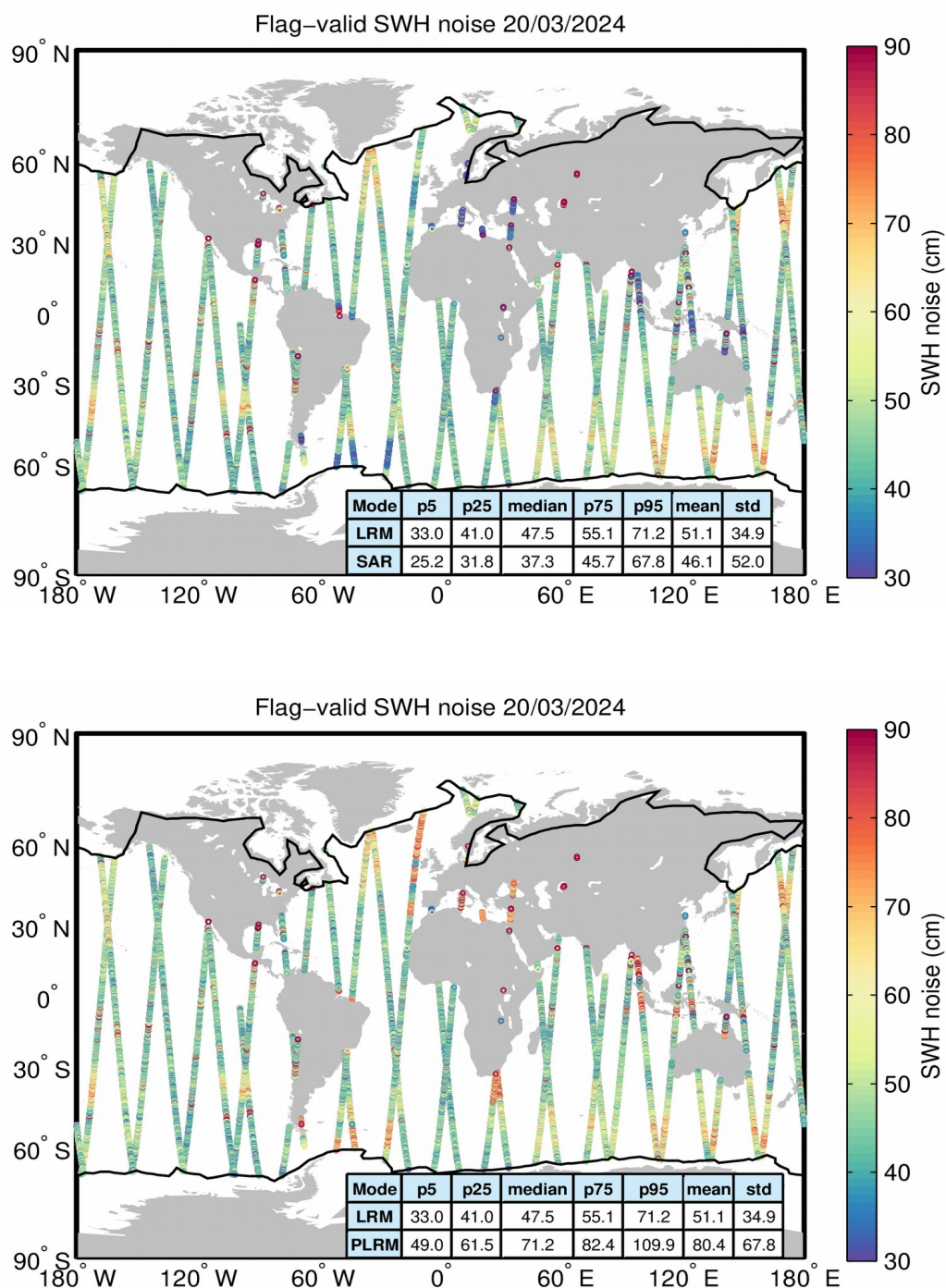
Figure 18. Geographical distribution of flag-valid 20-Hz SWH measurement noise over oceans and lakes for LRM/SAR (top) and LRM/PLRM (bottom) and for 20/03/2024. The statistical values shown in the table refer to the SWH noise and are calculated separately for LRM and SAR/PLRM regions. Measurements taken over polar polygons have been
