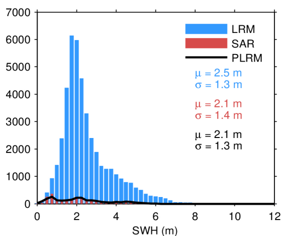
Figure 20. Histogram of science-valid SWH over oceans and lakes for LRM (blue), SAR (red), and PLRM (black) for 20/03/2024. The mean ( \mu ) and standard deviation ( \sigma ) are also
