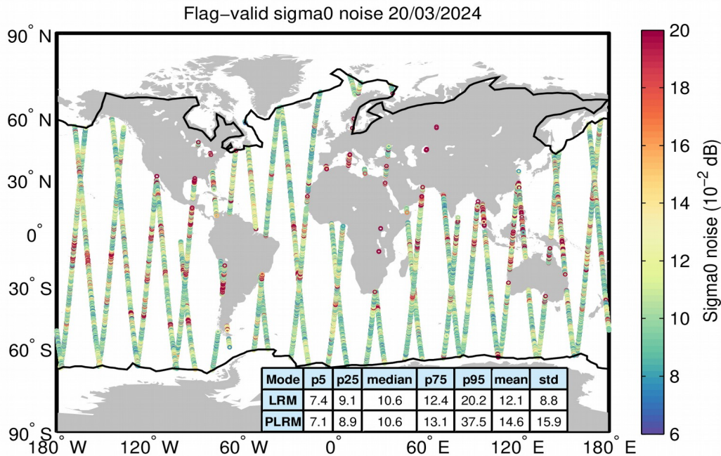
Figure 26. Geographical distribution of flag-valid 20-Hz sigma0 measurement noise over oceans and lakes for LRM/SAR (top) and LRM/PLRM (bottom) and for 20/03/2024. The statistical values shown in the table refer to the sigma0 noise and are calculated separately for LRM and SAR/PLRM regions. Measurements taken over polar polygons have been excluded from the computation of the statistical values. The black lines mark the outer limit of the Arctic and Antarctic polar polygons.
