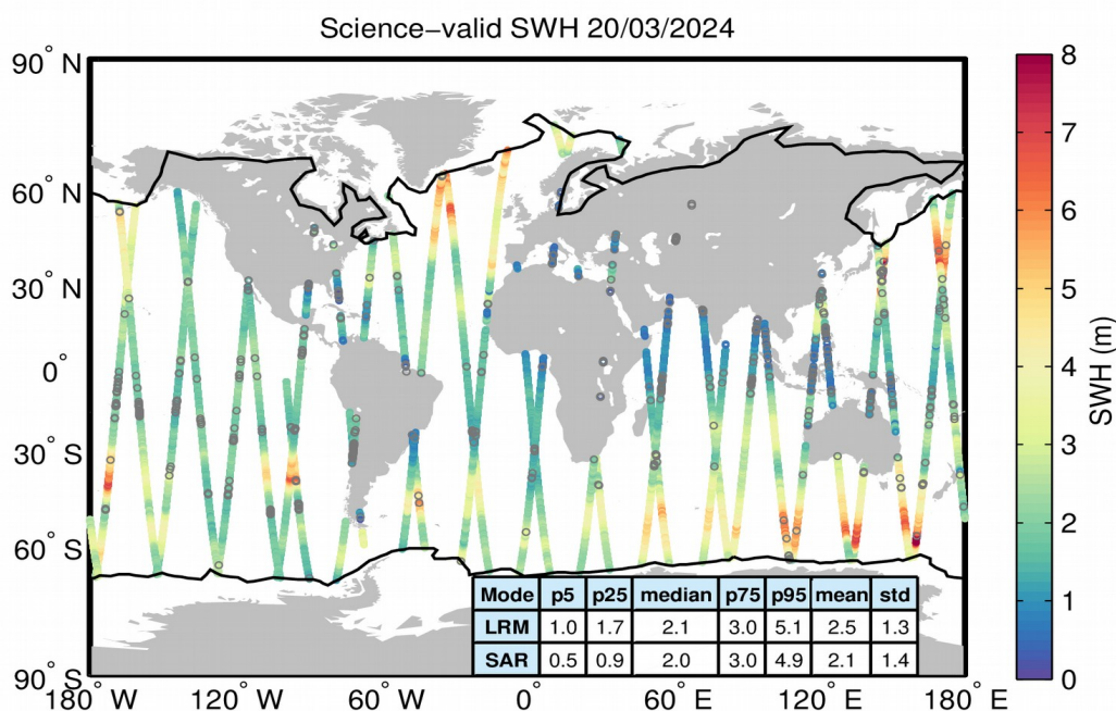
Figure 19. Geographical distribution of science-valid SWH data over oceans and lakes for 20/03/2024. The statistical values shown in the table refer to the SWH in m and are calculated separately for LRM and SAR regions. The black lines mark the outer limit of the Arctic and Antarctic polar polygons. Gray circles denote records that have been rejected based on the editing criteria described in Table 3.
