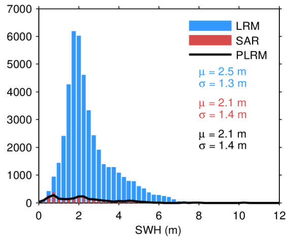
Figure 17. Histogram of flag-valid SWH over oceans and lakes for LRM (blue), SAR (red), and PLRM (black) for 20/03/2024. The mean ( \mu ) and standard deviation ( \sigma ) are also shown. Note that values larger than 12 m are excluded from the histogram for the sake of readability but not from the computation of \mu and \sigma .
