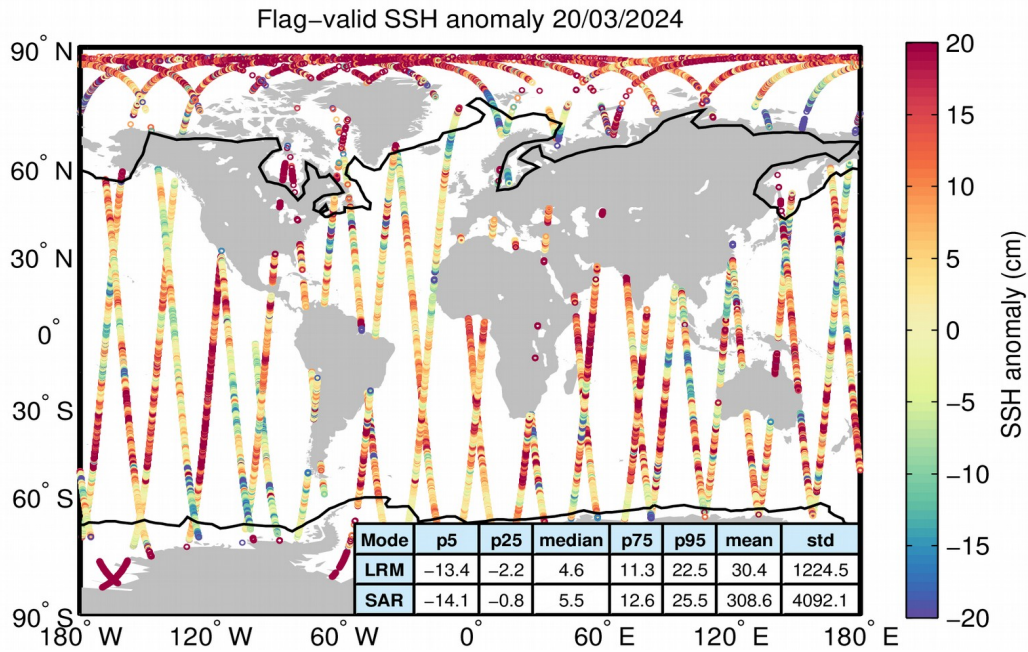
Figure 5. Geographical distribution of flag-valid 1-Hz SSH anomaly data over oceans and lakes for 20/03/2024. The statistical values shown in the table refer to the SSH anomaly in cm and are calculated separately for LRM and SAR regions. Measurements taken over polar polygons have been excluded from the computation of the statistical values. The black lines mark the outer limit of the Arctic and Antarctic polar polygons.
