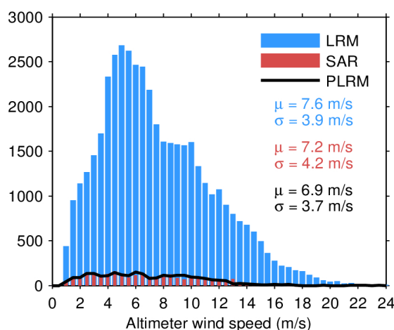
Figure 33. Histogram of flag-valid wind over oceans and lakes for LRM (blue), SAR (red), and PLRM (black) for 20/03/2024. The mean ( \mu ) and standard deviation ( \sigma ) are also shown. Note that values larger than 24 m/s are excluded from the histogram for the sake of readability but not from the computation of \mu and \sigma .
