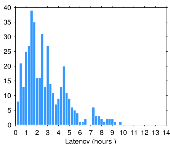
Figure 2. Histogram of the data latency for 20/03/2024. The y-axis denotes the number of files that are made available with a delay of x-hours with respect to the mean time of the records stored in the file.
