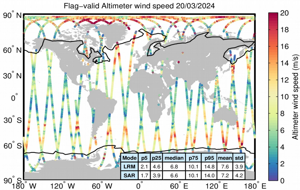
Figure 31. Geographical distribution of flag-valid wind data over oceans and lakes for 20/03/2024. The statistical values shown in the table refer to the wind in m/s and are calculated separately for LRM and SAR regions. Measurements taken over polar polygons have been excluded from the computation of the statistical values. The black lines mark the outer limit of the Arctic and Antarctic polar polygons.
