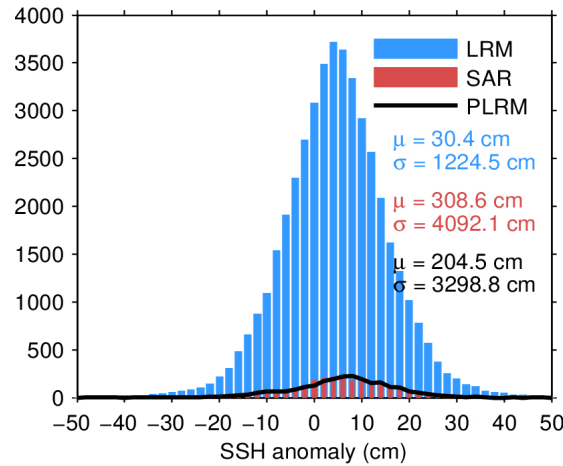
Figure 7. Histogram of flag-valid SSH anomaly over oceans and lakes for LRM (blue), SAR (red), and PLRM (black) for 20/03/2024. The mean ( \mu ) and standard deviation ( \sigma ) are also shown. Note that values outside [-50 50] cm are excluded from the histogram for the sake of readability but not from the computation of \mu and \sigma .
