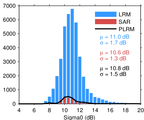
Figure 28. Histogram of science-valid sigma0 over oceans and lakes for LRM (blue), SAR (red), and PLRM (black) for 19/03/2024. The mean ( \mu ) and standard deviation ( \sigma ) are also shown. Note that values outside [4 20] dB are excluded from the histogram for the sake of readability but not from the computation of \mu and \sigma .
