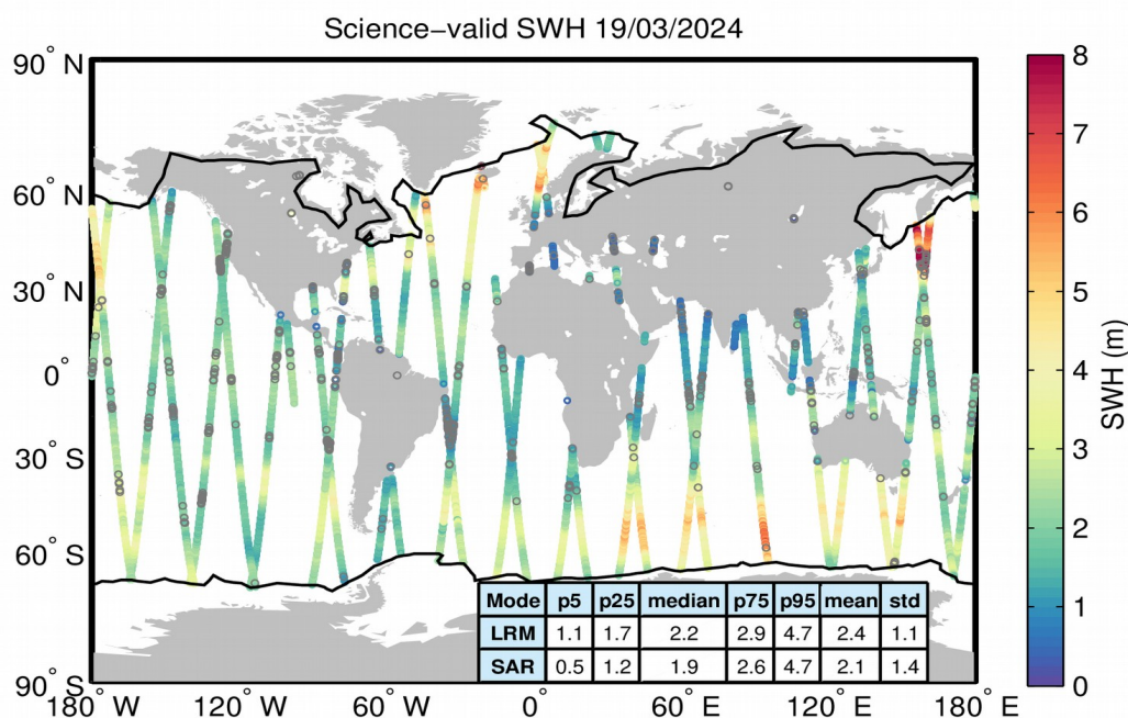
Figure 19. Geographical distribution of science-valid SWH data over oceans and lakes for 19/03/2024. The statistical values shown in the table refer to the SWH in m and are calculated separately for LRM and SAR regions. The black lines mark the outer limit of the Arctic and Antarctic polar polygons. Gray circles denote records that have been rejected based on the editing criteria described in Table 3.
