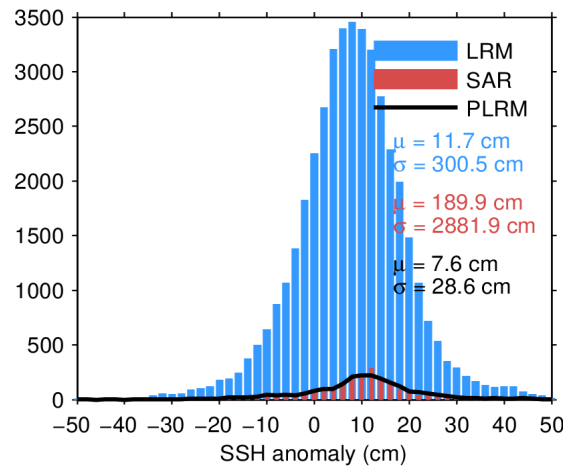
Figure 7. Histogram of flag-valid SSH anomaly over oceans and lakes for LRM (blue), SAR (red), and PLRM (black) for 19/03/2024. The mean ( \mu ) and standard deviation ( \sigma ) are also shown. Note that values outside [-50 50] cm are excluded from the histogram for the sake of readability but not from the computation of \mu and \sigma .
