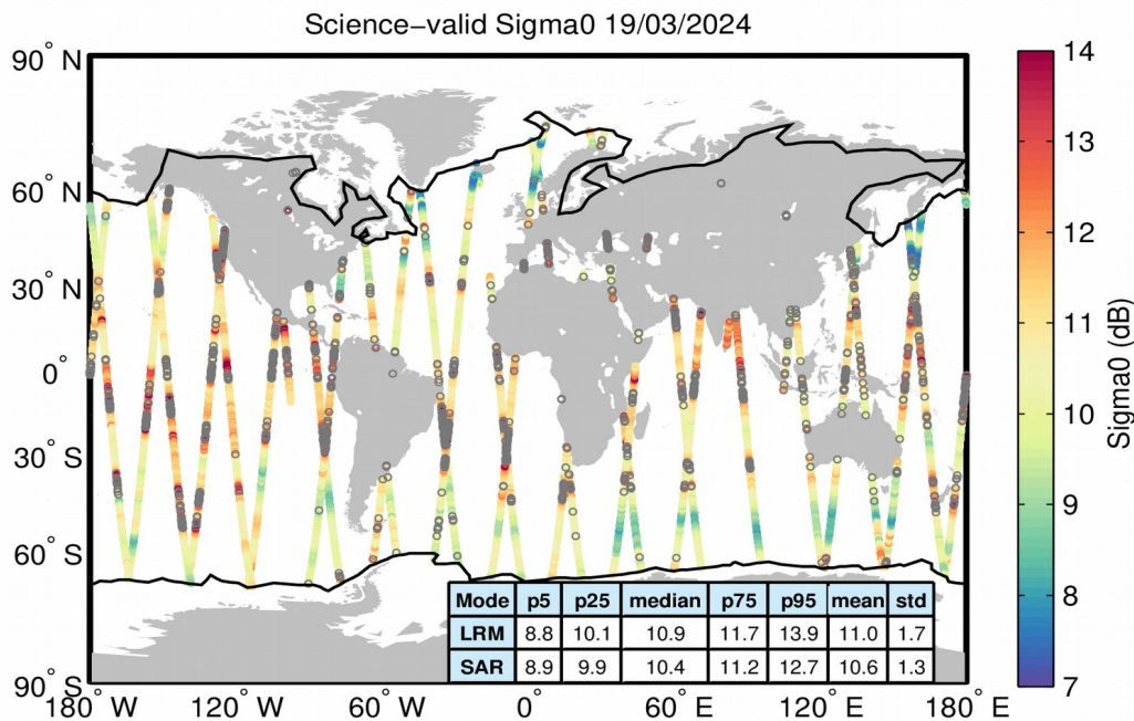
Figure 27. Geographical distribution of science-valid sigma0 data over oceans and lakes for 19/03/2024. The statistical values shown in the table refer to the sigma0 in dB and are calculated separately for LRM and SAR regions. The black lines mark the outer limit of the Arctic and Antarctic polar polygons. Gray circles denote records that have been rejected based on the editing criteria described in Table 4.
