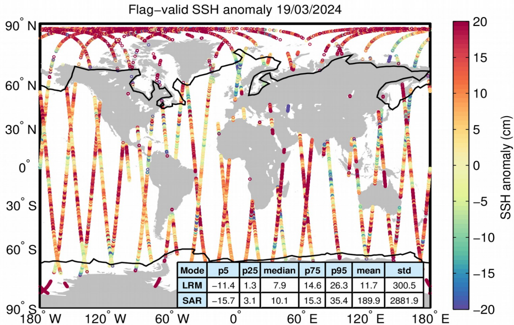
Figure 5. Geographical distribution of flag-valid 1-Hz SSH anomaly data over oceans and lakes for 19/03/2024. The statistical values shown in the table refer to the SSH anomaly in cm and are calculated separately for LRM and SAR regions. Measurements taken over polar polygons have been excluded from the computation of the statistical values. The black lines mark the outer limit of the Arctic and Antarctic polar polygons.
