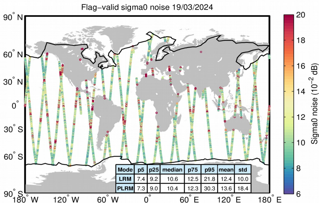
Figure 26. Geographical distribution of flag-valid 20-Hz sigma0 measurement noise over oceans and lakes for LRM/SAR (top) and LRM/PLRM (bottom) and for 19/03/2024. The statistical values shown in the table refer to the sigma0 noise and are calculated separately for LRM and SAR/PLRM regions. Measurements taken over polar polygons have been excluded from the computation of the statistical values. The black lines mark the outer limit of the Arctic and Antarctic polar polygons.
