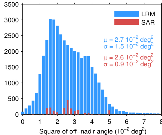
Figure 39. Histogram of flag-valid mispointing over oceans and lakes for LRM (blue) and SAR (red) for 19/03/2024. Only positive values have been considered. The mean ( \mu ) and standard deviation ( \sigma ) are also shown. Note that values larger than 8 \cdot 10^{-2} \text{ deg}^2 are excluded from the histogram for the sake of readability but not from the computation of \mu and \sigma .
