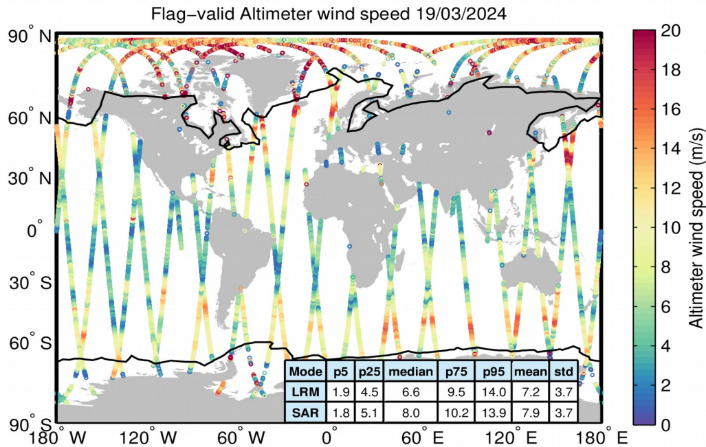
Figure 31. Geographical distribution of flag-valid wind data over oceans and lakes for 19/03/2024. The statistical values shown in the table refer to the wind in m/s and are calculated separately for LRM and SAR regions. Measurements taken over polar polygons have been excluded from the computation of the statistical values. The black lines mark the outer limit of the Arctic and Antarctic polar polygons.
