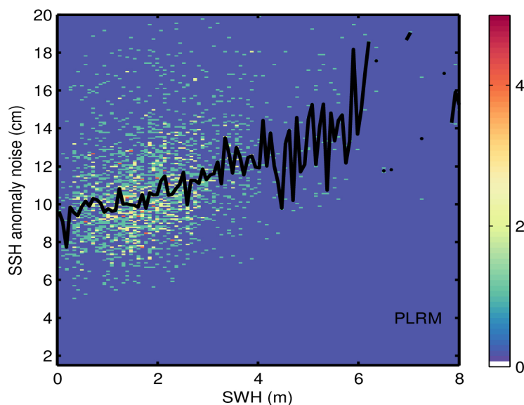
Figure 9. 2D histogram showing flag-valid SSH anomaly noise as a function of SWH for LRM (top), SAR (middle), and PLRM (bottom) for 19/03/2024. The black line denotes the median SSH anomaly noise as a function of SWH.
