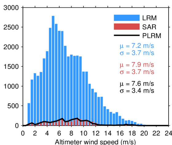
Figure 33. Histogram of flag-valid wind over oceans and lakes for LRM (blue), SAR (red), and PLRM (black) for 19/03/2024. The mean ( \mu ) and standard deviation ( \sigma ) are also shown. Note that values larger than 24 m/s are excluded from the histogram for the sake of readability but not from the computation of \mu and \sigma .
