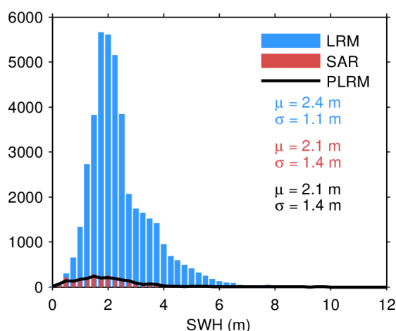
Figure 20. Histogram of science-valid SWH over oceans and lakes for LRM (blue), SAR (red), and PLRM (black) for 19/03/2024. The mean ( \mu ) and standard deviation ( \sigma ) are also
