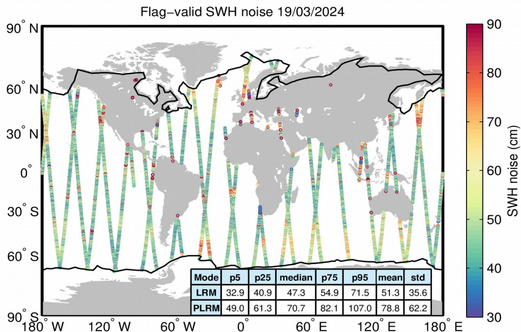
Figure 18. Geographical distribution of flag-valid 20-Hz SWH measurement noise over oceans and lakes for LRM/SAR (top) and LRM/PLRM (bottom) and for 19/03/2024. The statistical values shown in the table refer to the SWH noise and are calculated separately for LRM and SAR/PLRM regions. Measurements taken over polar polygons have been
