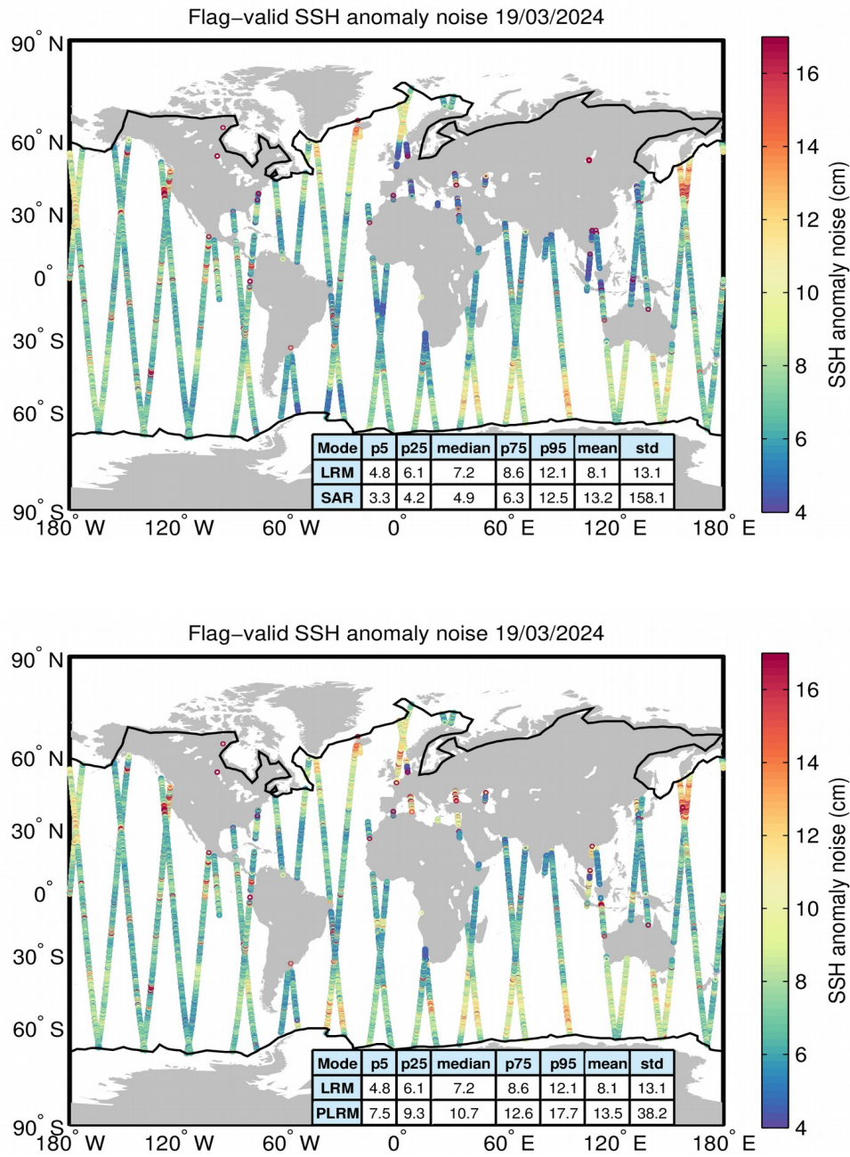
Figure 8. Geographical distribution of flag-valid 20-Hz SSH anomaly measurement noise over oceans and lakes for LRM/SAR (top) and LRM/PLRM (bottom) and for 19/03/2024. The statistical values shown in the tables refer to the SSH anomaly noise and are calculated separately for LRM and SAR/PLRM regions. Measurements taken over polar polygons have been excluded from the computation of the statistical values. The black lines mark the outer limit of the Arctic and Antarctic polar polygons.
