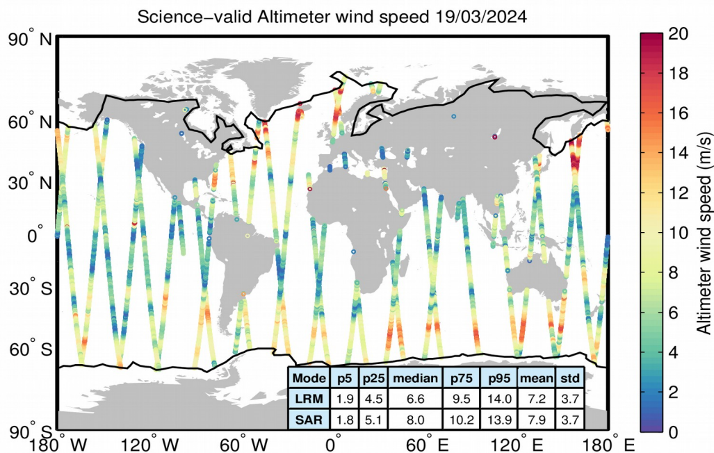
Figure 34. Geographical distribution of science-valid wind data over oceans and lakes for 19/03/2024. The statistical values shown in the table refer to the wind in m/s and are calculated separately for LRM and SAR regions. The black lines mark the outer limit of the Arctic and Antarctic polar polygons. Gray circles denote records that have been rejected based on the editing criteria described in Table 5.
