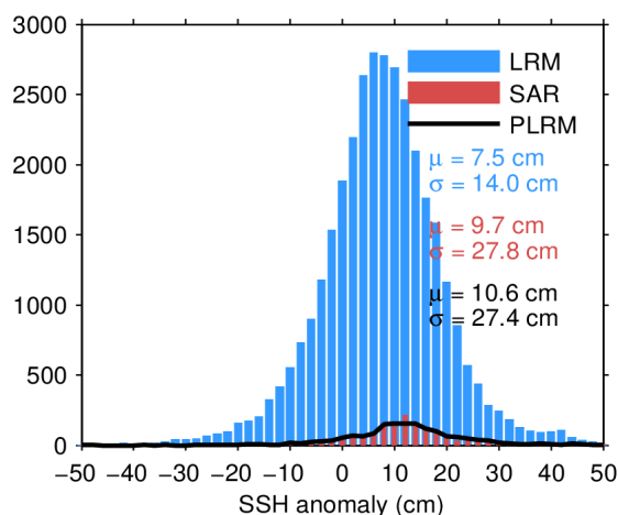
Figure 11. Histogram of science-valid SSH anomaly over oceans and lakes for LRM (blue), SAR (red), and PLRM (black) for 19/03/2024. The mean ( \mu ) and standard deviation ( \sigma ) are also shown. Note that values outside [-50\ 50] cm are excluded from the histogram for the sake of readability but not from the computation of \mu and \sigma .
