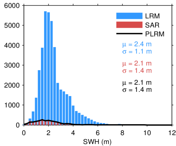
Figure 17. Histogram of flag-valid SWH over oceans and lakes for LRM (blue), SAR (red), and PLRM (black) for 19/03/2024. The mean ( \mu ) and standard deviation ( \sigma ) are also shown. Note that values larger than 12 m are excluded from the histogram for the sake of readability but not from the computation of \mu and \sigma .
