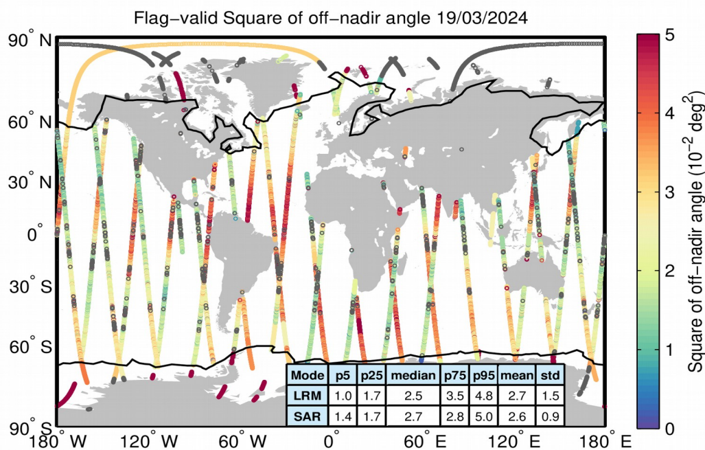
Figure 37. Geographical distribution of flag-valid mispointing data over oceans and lakes for 19/03/2024. The statistical values shown in the table refer to the mispointing in 10^{-2} \text{ deg}^2 and are calculated separately for LRM and SAR regions. Measurements taken over polar polygons have been excluded from the computation of the statistical values. The black lines mark the outer limit of the Arctic and Antarctic polar polygons. Gray circles denote negative values.
