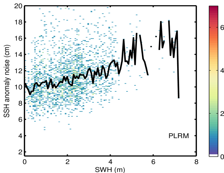
Figure 9. 2D histogram showing flag-valid SSH anomaly noise as a function of SWH for LRM (top), SAR (middle), and PLRM (bottom) for 18/03/2024. The black line denotes the median SSH anomaly noise as a function of SWH.
