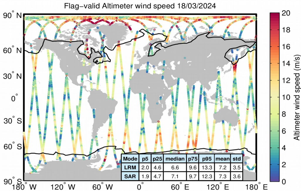
Figure 31. Geographical distribution of flag-valid wind data over oceans and lakes for 18/03/2024. The statistical values shown in the table refer to the wind in m/s and are calculated separately for LRM and SAR regions. Measurements taken over polar polygons have been excluded from the computation of the statistical values. The black lines mark the outer limit of the Arctic and Antarctic polar polygons.
