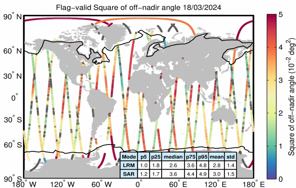
Figure 37. Geographical distribution of flag-valid mispointing data over oceans and lakes for 18/03/2024. The statistical values shown in the table refer to the mispointing in 10^{-2} \text{ deg}^2 and are calculated separately for LRM and SAR regions. Measurements taken over polar polygons have been excluded from the computation of the statistical values. The black lines mark the outer limit of the Arctic and Antarctic polar polygons. Gray circles denote negative values.
