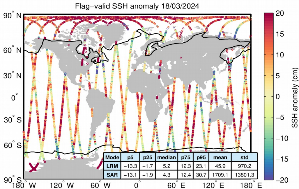
Figure 5. Geographical distribution of flag-valid 1-Hz SSH anomaly data over oceans and lakes for 18/03/2024. The statistical values shown in the table refer to the SSH anomaly in cm and are calculated separately for LRM and SAR regions. Measurements taken over polar polygons have been excluded from the computation of the statistical values. The black lines mark the outer limit of the Arctic and Antarctic polar polygons.
