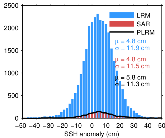
Figure 11. Histogram of science-valid SSH anomaly over oceans and lakes for LRM (blue), SAR (red), and PLRM (black) for 18/03/2024. The mean ( \mu ) and standard deviation ( \sigma ) are also shown. Note that values outside [-50\ 50] cm are excluded from the histogram for the sake of readability but not from the computation of \mu and \sigma .
