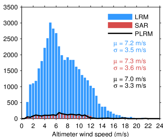
Figure 33. Histogram of flag-valid wind over oceans and lakes for LRM (blue), SAR (red), and PLRM (black) for 18/03/2024. The mean ( \mu ) and standard deviation ( \sigma ) are also shown. Note that values larger than 24 m/s are excluded from the histogram for the sake of readability but not from the computation of \mu and \sigma .
