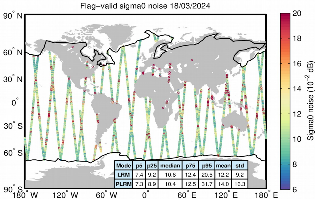
Figure 26. Geographical distribution of flag-valid 20-Hz sigma0 measurement noise over oceans and lakes for LRM/SAR (top) and LRM/PLRM (bottom) and for 18/03/2024. The statistical values shown in the table refer to the sigma0 noise and are calculated separately for LRM and SAR/PLRM regions. Measurements taken over polar polygons have been excluded from the computation of the statistical values. The black lines mark the outer limit of the Arctic and Antarctic polar polygons.
