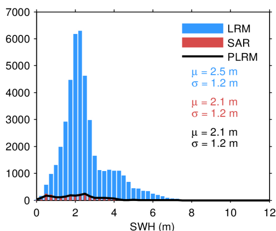
Figure 20. Histogram of science-valid SWH over oceans and lakes for LRM (blue), SAR (red), and PLRM (black) for 18/03/2024. The mean ( \mu ) and standard deviation ( \sigma ) are also
