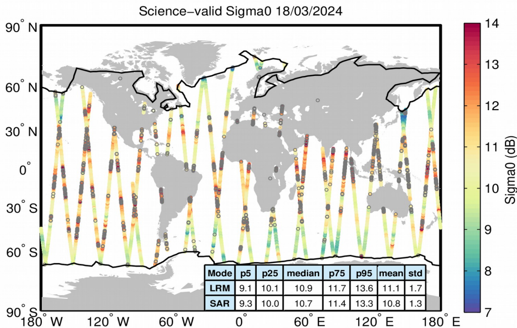
Figure 27. Geographical distribution of science-valid sigma0 data over oceans and lakes for 18/03/2024. The statistical values shown in the table refer to the sigma0 in dB and are calculated separately for LRM and SAR regions. The black lines mark the outer limit of the Arctic and Antarctic polar polygons. Gray circles denote records that have been rejected based on the editing criteria described in Table 4.
