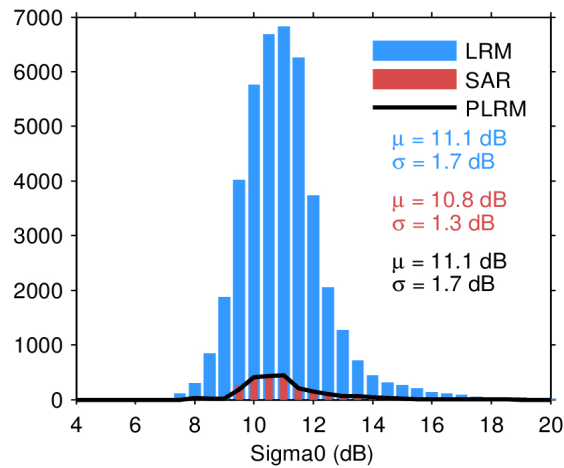
Figure 28. Histogram of science-valid sigma0 over oceans and lakes for LRM (blue), SAR (red), and PLRM (black) for 18/03/2024. The mean ( \mu ) and standard deviation ( \sigma ) are also shown. Note that values outside [4 20] dB are excluded from the histogram for the sake of readability but not from the computation of \mu and \sigma .
