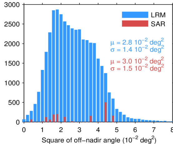
Figure 39. Histogram of flag-valid mispointing over oceans and lakes for LRM (blue) and SAR (red) for 18/03/2024. Only positive values have been considered. The mean ( \mu ) and standard deviation ( \sigma ) are also shown. Note that values larger than 8 \cdot 10^{-2} \text{ deg}^2 are excluded from the histogram for the sake of readability but not from the computation of \mu and \sigma .
