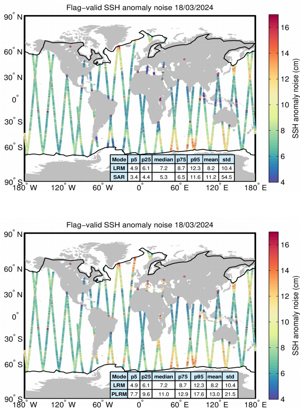
Figure 8. Geographical distribution of flag-valid 20-Hz SSH anomaly measurement noise over oceans and lakes for LRM/SAR (top) and LRM/PLRM (bottom) and for 18/03/2024. The statistical values shown in the tables refer to the SSH anomaly noise and are calculated separately for LRM and SAR/PLRM regions. Measurements taken over polar polygons have been excluded from the computation of the statistical values. The black lines mark the outer limit of the Arctic and Antarctic polar polygons.
