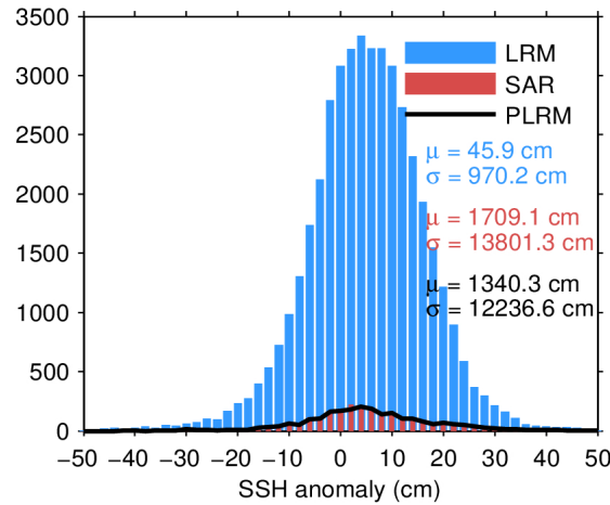
Figure 7. Histogram of flag-valid SSH anomaly over oceans and lakes for LRM (blue), SAR (red), and PLRM (black) for 18/03/2024. The mean ( \mu ) and standard deviation ( \sigma ) are also shown. Note that values outside [-50 50] cm are excluded from the histogram for the sake of readability but not from the computation of \mu and \sigma .
