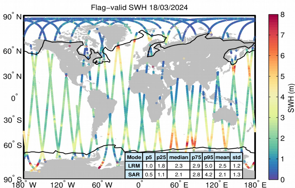
Figure 15. Geographical distribution of flag-valid SWH data over oceans and lakes for 18/03/2024. The statistical values shown in the table refer to the SWH in m and are calculated separately for LRM and SAR regions. Measurements taken over polar polygons have been excluded from the computation of the statistical values. The black lines mark the outer limit of the Arctic and Antarctic polar polygons.
