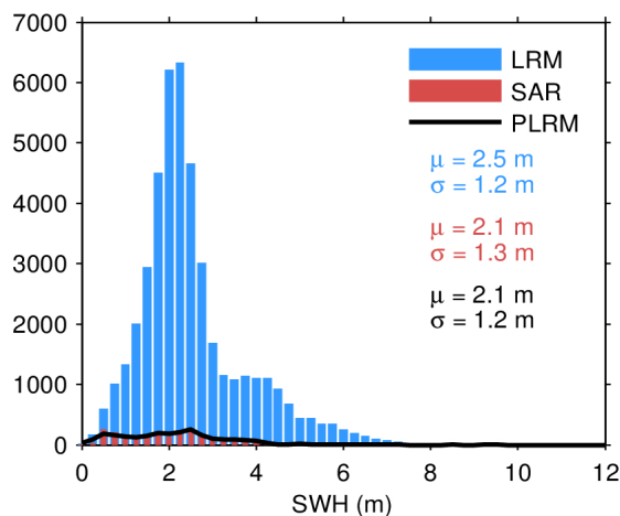
Figure 17. Histogram of flag-valid SWH over oceans and lakes for LRM (blue), SAR (red), and PLRM (black) for 18/03/2024. The mean ( \mu ) and standard deviation ( \sigma ) are also shown. Note that values larger than 12 m are excluded from the histogram for the sake of readability but not from the computation of \mu and \sigma .
